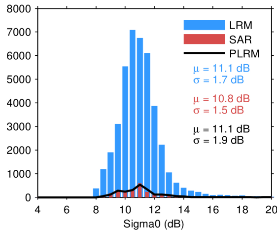
Figure 28. Histogram of science-valid sigma0 over oceans and lakes for LRM (blue), SAR (red), and PLRM (black) for 17/03/2024. The mean ( \mu ) and standard deviation ( \sigma ) are also shown. Note that values outside [4 20] dB are excluded from the histogram for the sake of readability but not from the computation of \mu and \sigma .
