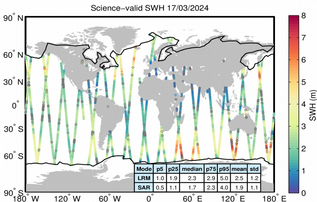
Figure 19. Geographical distribution of science-valid SWH data over oceans and lakes for 17/03/2024. The statistical values shown in the table refer to the SWH in m and are calculated separately for LRM and SAR regions. The black lines mark the outer limit of the Arctic and Antarctic polar polygons. Gray circles denote records that have been rejected based on the editing criteria described in Table 3.
