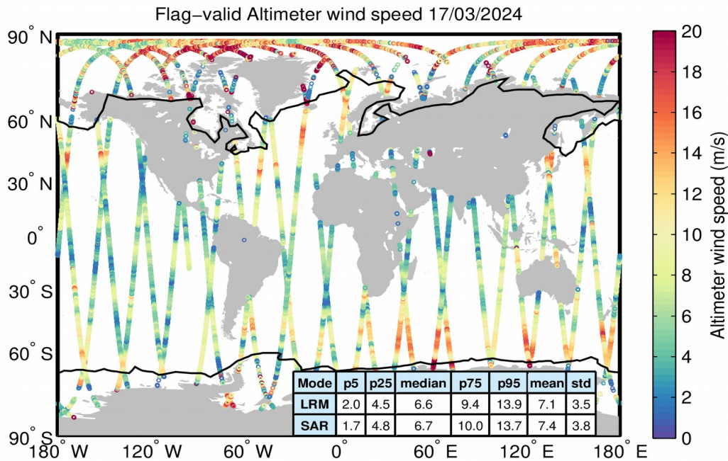
Figure 31. Geographical distribution of flag-valid wind data over oceans and lakes for 17/03/2024. The statistical values shown in the table refer to the wind in m/s and are calculated separately for LRM and SAR regions. Measurements taken over polar polygons have been excluded from the computation of the statistical values. The black lines mark the outer limit of the Arctic and Antarctic polar polygons.
