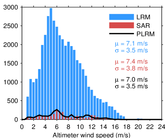
Figure 33. Histogram of flag-valid wind over oceans and lakes for LRM (blue), SAR (red), and PLRM (black) for 17/03/2024. The mean ( \mu ) and standard deviation ( \sigma ) are also shown. Note that values larger than 24 m/s are excluded from the histogram for the sake of readability but not from the computation of \mu and \sigma .
