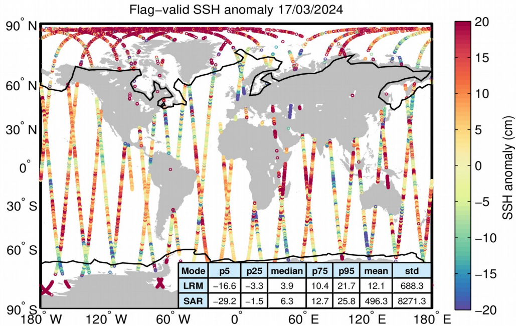
Figure 5. Geographical distribution of flag-valid 1-Hz SSH anomaly data over oceans and lakes for 17/03/2024. The statistical values shown in the table refer to the SSH anomaly in cm and are calculated separately for LRM and SAR regions. Measurements taken over polar polygons have been excluded from the computation of the statistical values. The black lines mark the outer limit of the Arctic and Antarctic polar polygons.
