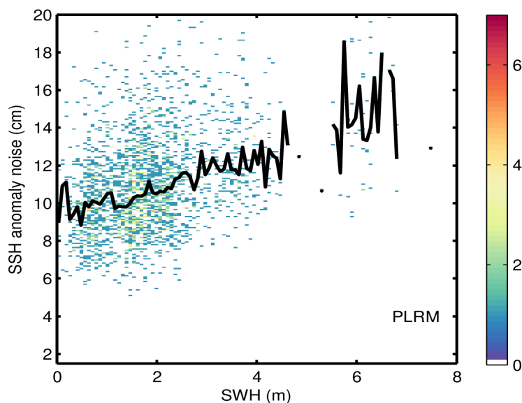
Figure 9. 2D histogram showing flag-valid SSH anomaly noise as a function of SWH for LRM (top), SAR (middle), and PLRM (bottom) for 17/03/2024. The black line denotes the median SSH anomaly noise as a function of SWH.
