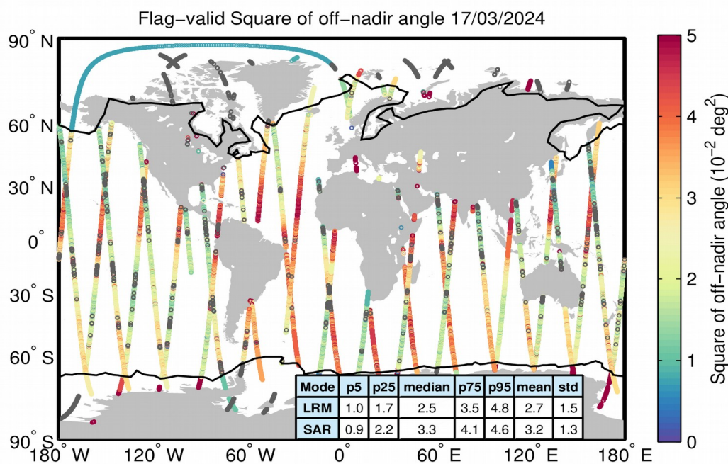
Figure 37. Geographical distribution of flag-valid mispointing data over oceans and lakes for 17/03/2024. The statistical values shown in the table refer to the mispointing in 10^{-2} \text{ deg}^2 and are calculated separately for LRM and SAR regions. Measurements taken over polar polygons have been excluded from the computation of the statistical values. The black lines mark the outer limit of the Arctic and Antarctic polar polygons. Gray circles denote negative values.
