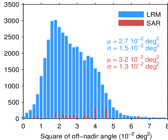
Figure 39. Histogram of flag-valid mispointing over oceans and lakes for LRM (blue) and SAR (red) for 17/03/2024. Only positive values have been considered. The mean ( \mu ) and standard deviation ( \sigma ) are also shown. Note that values larger than 8 \cdot 10^{-2} \text{ deg}^2 are excluded from the histogram for the sake of readability but not from the computation of \mu and \sigma .
