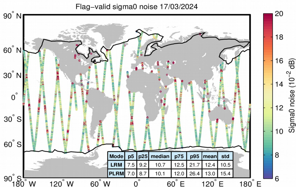
Figure 26. Geographical distribution of flag-valid 20-Hz sigma0 measurement noise over oceans and lakes for LRM/SAR (top) and LRM/PLRM (bottom) and for 17/03/2024. The statistical values shown in the table refer to the sigma0 noise and are calculated separately for LRM and SAR/PLRM regions. Measurements taken over polar polygons have been excluded from the computation of the statistical values. The black lines mark the outer limit of the Arctic and Antarctic polar polygons.
