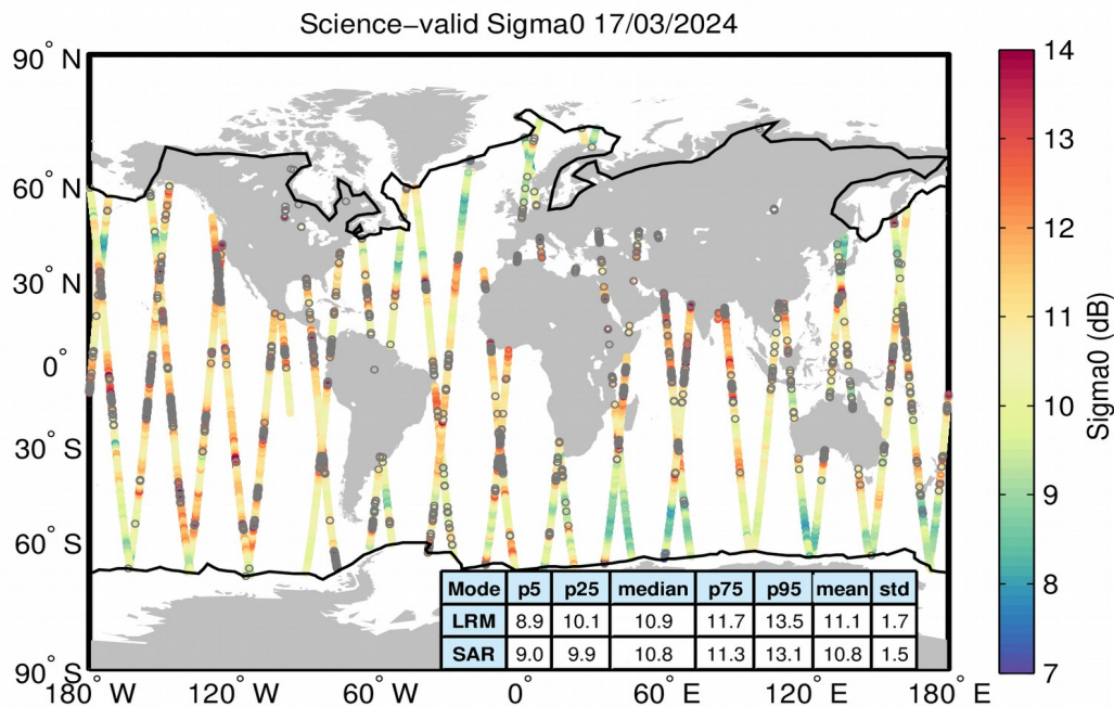
Figure 27. Geographical distribution of science-valid sigma0 data over oceans and lakes for 17/03/2024. The statistical values shown in the table refer to the sigma0 in dB and are calculated separately for LRM and SAR regions. The black lines mark the outer limit of the Arctic and Antarctic polar polygons. Gray circles denote records that have been rejected based on the editing criteria described in Table 4.
