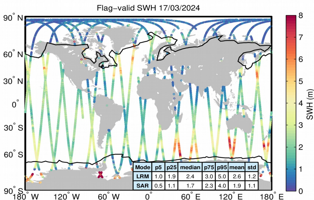
Figure 15. Geographical distribution of flag-valid SWH data over oceans and lakes for 17/03/2024. The statistical values shown in the table refer to the SWH in m and are calculated separately for LRM and SAR regions. Measurements taken over polar polygons have been excluded from the computation of the statistical values. The black lines mark the outer limit of the Arctic and Antarctic polar polygons.
