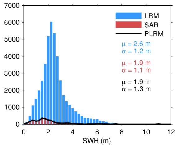
Figure 17. Histogram of flag-valid SWH over oceans and lakes for LRM (blue), SAR (red), and PLRM (black) for 17/03/2024. The mean ( \mu ) and standard deviation ( \sigma ) are also shown. Note that values larger than 12 m are excluded from the histogram for the sake of readability but not from the computation of \mu and \sigma .
