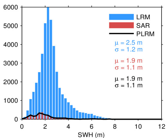
Figure 20. Histogram of science-valid SWH over oceans and lakes for LRM (blue), SAR (red), and PLRM (black) for 17/03/2024. The mean ( \mu ) and standard deviation ( \sigma ) are also
