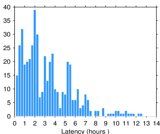
Figure 2. Histogram of the data latency for 17/03/2024. The y-axis denotes the number of files that are made available with a delay of x-hours with respect to the mean time of the records stored in the file.
