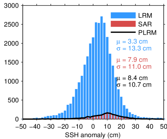
Figure 11. Histogram of science-valid SSH anomaly over oceans and lakes for LRM (blue), SAR (red), and PLRM (black) for 17/03/2024. The mean ( \mu ) and standard deviation ( \sigma ) are also shown. Note that values outside [-50\ 50] cm are excluded from the histogram for the sake of readability but not from the computation of \mu and \sigma .
