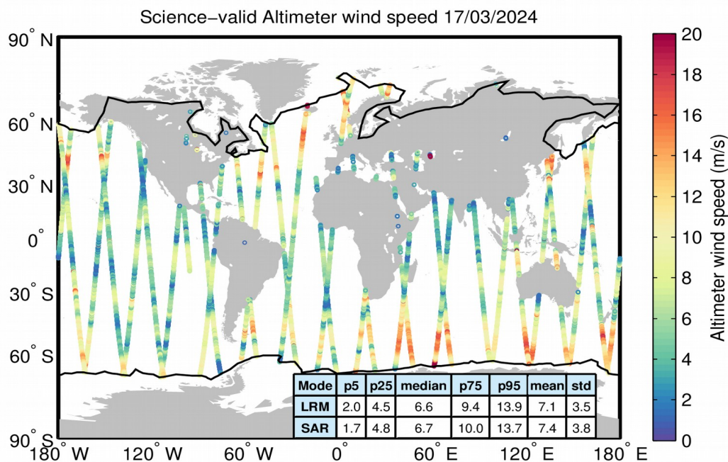
Figure 34. Geographical distribution of science-valid wind data over oceans and lakes for 17/03/2024. The statistical values shown in the table refer to the wind in m/s and are calculated separately for LRM and SAR regions. The black lines mark the outer limit of the Arctic and Antarctic polar polygons. Gray circles denote records that have been rejected based on the editing criteria described in Table 5.
