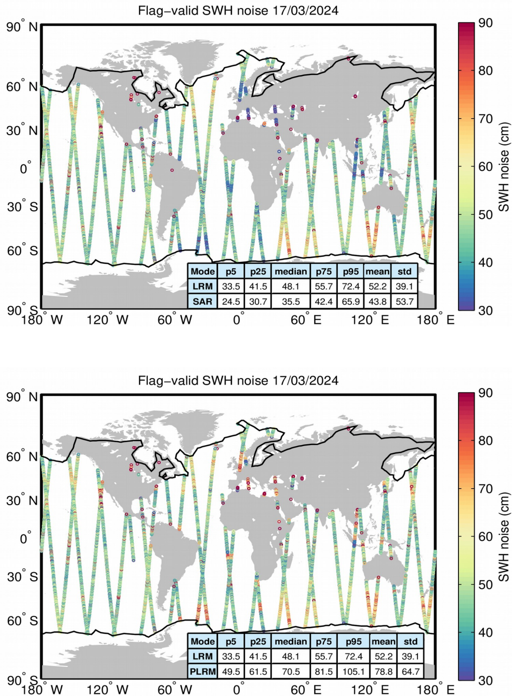
Figure 18. Geographical distribution of flag-valid 20-Hz SWH measurement noise over oceans and lakes for LRM/SAR (top) and LRM/PLRM (bottom) and for 17/03/2024. The statistical values shown in the table refer to the SWH noise and are calculated separately for LRM and SAR/PLRM regions. Measurements taken over polar polygons have been
