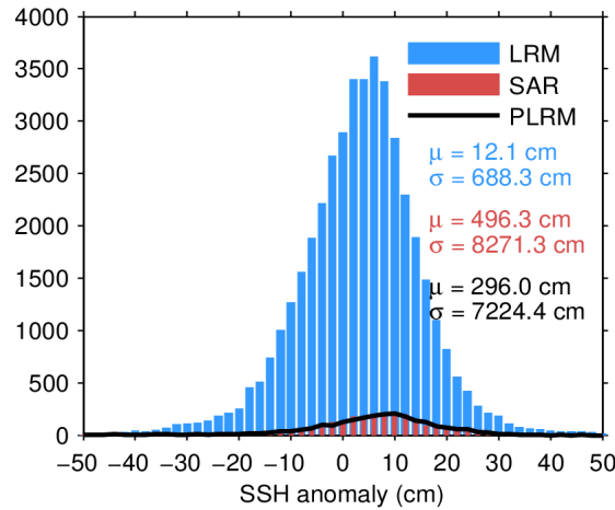
Figure 7. Histogram of flag-valid SSH anomaly over oceans and lakes for LRM (blue), SAR (red), and PLRM (black) for 17/03/2024. The mean ( \mu ) and standard deviation ( \sigma ) are also shown. Note that values outside [-50, 50] cm are excluded from the histogram for the sake of readability but not from the computation of \mu and \sigma .
