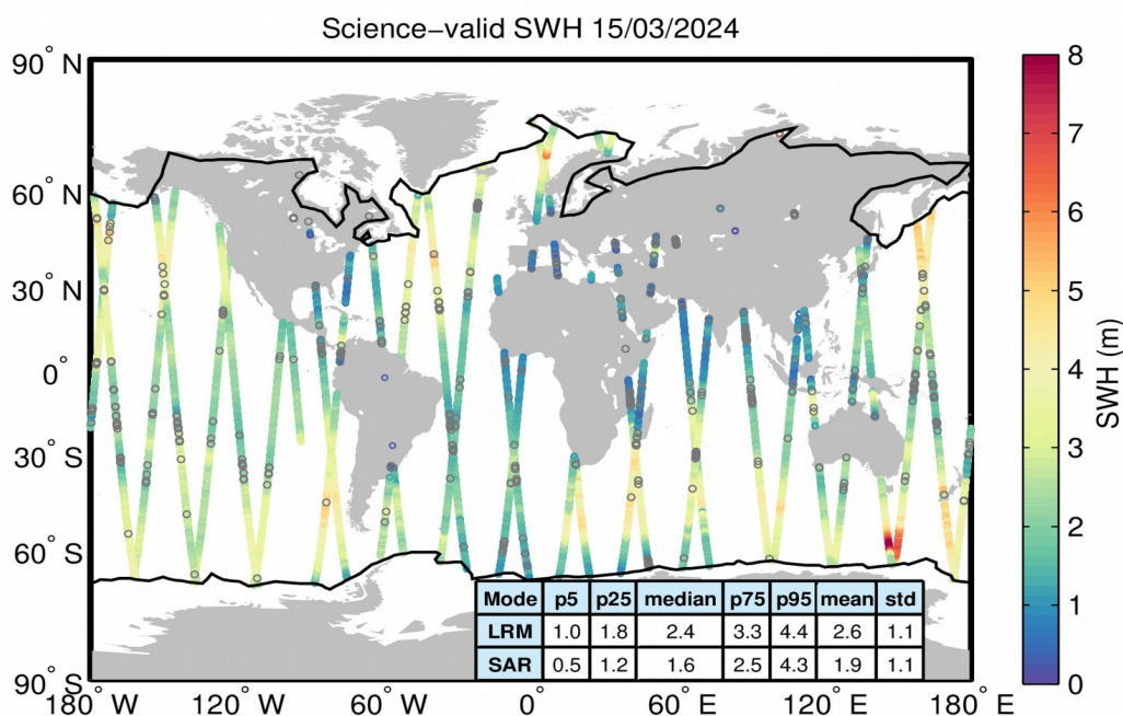
Figure 19. Geographical distribution of science-valid SWH data over oceans and lakes for 15/03/2024. The statistical values shown in the table refer to the SWH in m and are calculated separately for LRM and SAR regions. The black lines mark the outer limit of the Arctic and Antarctic polar polygons. Gray circles denote records that have been rejected based on the editing criteria described in Table 3.
