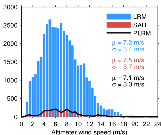
Figure 33. Histogram of flag-valid wind over oceans and lakes for LRM (blue), SAR (red), and PLRM (black) for 15/03/2024. The mean ( \mu ) and standard deviation ( \sigma ) are also shown. Note that values larger than 24 m/s are excluded from the histogram for the sake of readability but not from the computation of \mu and \sigma .
