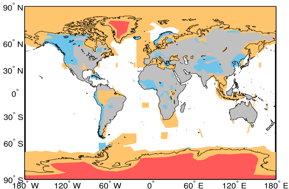
Figure A1. Extent of the regions defining the geographical mode mask for 15/03/2024. The regions where SAR, and SARIn are operated are denoted by the orange and blue polygons, respectively. LRM is operated over areas of the continental ice sheets (red polygons) and over oceans and land not covered by other modes.
