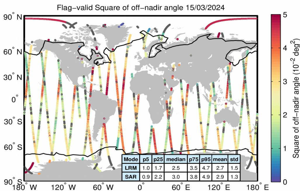
Figure 37. Geographical distribution of flag-valid mispointing data over oceans and lakes for 15/03/2024. The statistical values shown in the table refer to the mispointing in 10^{-2} \text{ deg}^2 and are calculated separately for LRM and SAR regions. Measurements taken over polar polygons have been excluded from the computation of the statistical values. The black lines mark the outer limit of the Arctic and Antarctic polar polygons. Gray circles denote negative values.
