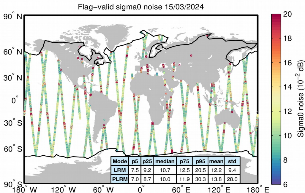
Figure 26. Geographical distribution of flag-valid 20-Hz sigma0 measurement noise over oceans and lakes for LRM/SAR (top) and LRM/PLRM (bottom) and for 15/03/2024. The statistical values shown in the table refer to the sigma0 noise and are calculated separately for LRM and SAR/PLRM regions. Measurements taken over polar polygons have been excluded from the computation of the statistical values. The black lines mark the outer limit of the Arctic and Antarctic polar polygons.
