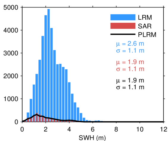
Figure 20. Histogram of science-valid SWH over oceans and lakes for LRM (blue), SAR (red), and PLRM (black) for 15/03/2024. The mean ( \mu ) and standard deviation ( \sigma ) are also
