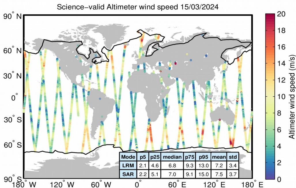
Figure 34. Geographical distribution of science-valid wind data over oceans and lakes for 15/03/2024. The statistical values shown in the table refer to the wind in m/s and are calculated separately for LRM and SAR regions. The black lines mark the outer limit of the Arctic and Antarctic polar polygons. Gray circles denote records that have been rejected based on the editing criteria described in Table 5.
