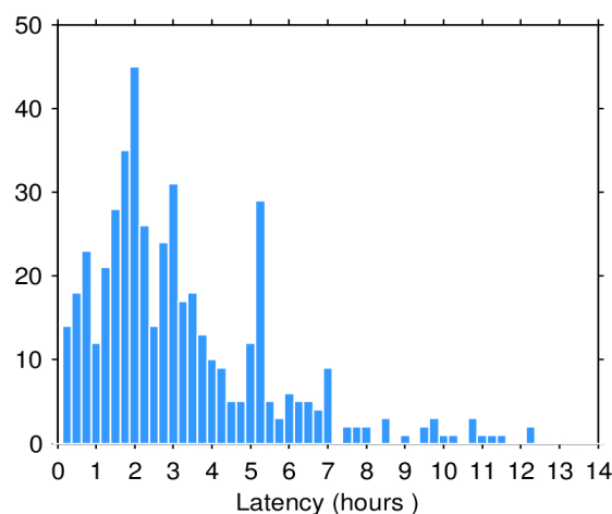
Figure 2. Histogram of the data latency for 15/03/2024. The y-axis denotes the number of files that are made available with a delay of x-hours with respect to the mean time of the records stored in the file.
