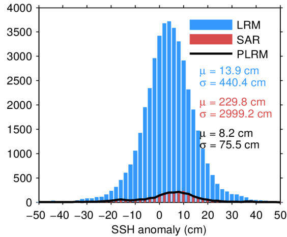
Figure 7. Histogram of flag-valid SSH anomaly over oceans and lakes for LRM (blue), SAR (red), and PLRM (black) for 15/03/2024. The mean ( \mu ) and standard deviation ( \sigma ) are also shown. Note that values outside [-50 50] cm are excluded from the histogram for the sake of readability but not from the computation of \mu and \sigma .
