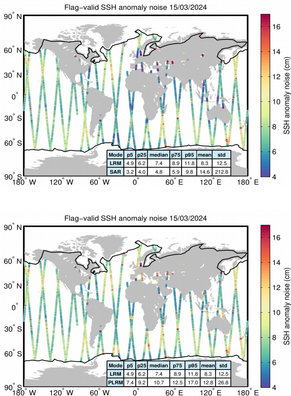
Figure 8. Geographical distribution of flag-valid 20-Hz SSH anomaly measurement noise over oceans and lakes for LRM/SAR (top) and LRM/PLRM (bottom) and for 15/03/2024. The statistical values shown in the tables refer to the SSH anomaly noise and are calculated separately for LRM and SAR/PLRM regions. Measurements taken over polar polygons have been excluded from the computation of the statistical values. The black lines mark the outer limit of the Arctic and Antarctic polar polygons.
