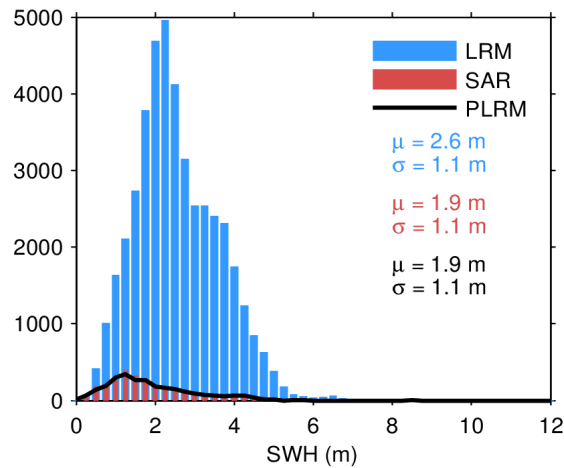
Figure 17. Histogram of flag-valid SWH over oceans and lakes for LRM (blue), SAR (red), and PLRM (black) for 15/03/2024. The mean ( \mu ) and standard deviation ( \sigma ) are also shown. Note that values larger than 12 m are excluded from the histogram for the sake of readability but not from the computation of \mu and \sigma .
