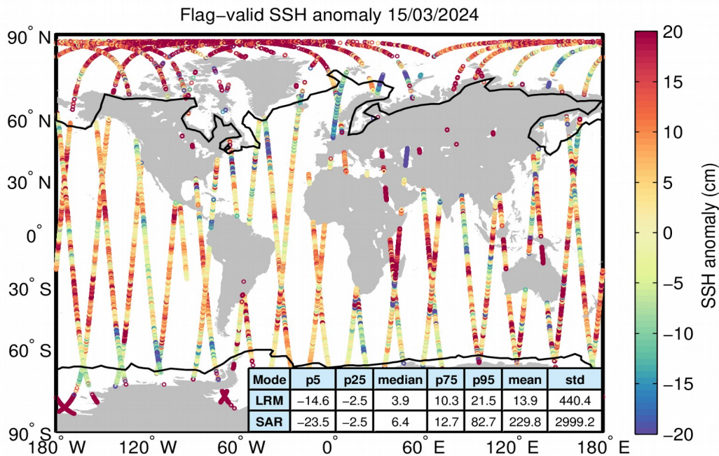
Figure 5. Geographical distribution of flag-valid 1-Hz SSH anomaly data over oceans and lakes for 15/03/2024. The statistical values shown in the table refer to the SSH anomaly in cm and are calculated separately for LRM and SAR regions. Measurements taken over polar polygons have been excluded from the computation of the statistical values. The black lines mark the outer limit of the Arctic and Antarctic polar polygons.
