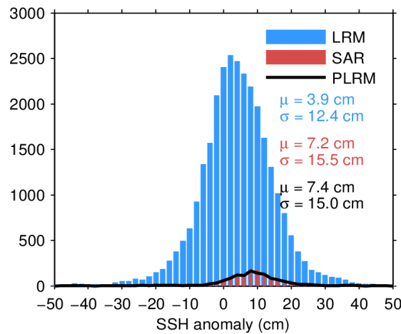
Figure 11. Histogram of science-valid SSH anomaly over oceans and lakes for LRM (blue), SAR (red), and PLRM (black) for 15/03/2024. The mean ( \mu ) and standard deviation ( \sigma ) are also shown. Note that values outside [-50\ 50] cm are excluded from the histogram for the sake of readability but not from the computation of \mu and \sigma .
