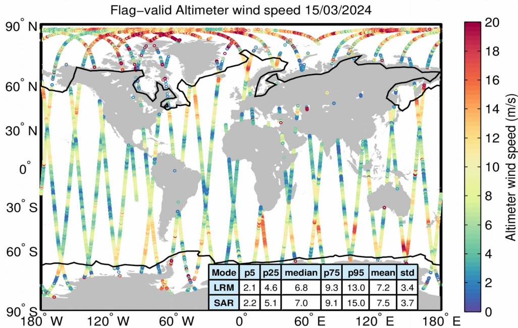
Figure 31. Geographical distribution of flag-valid wind data over oceans and lakes for 15/03/2024. The statistical values shown in the table refer to the wind in m/s and are calculated separately for LRM and SAR regions. Measurements taken over polar polygons have been excluded from the computation of the statistical values. The black lines mark the outer limit of the Arctic and Antarctic polar polygons.
