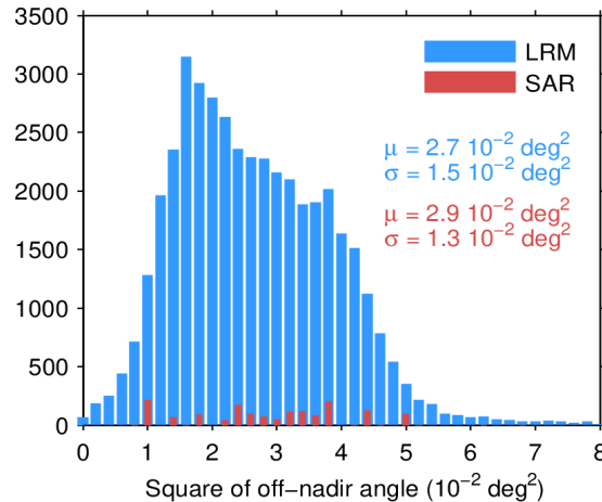
Figure 39. Histogram of flag-valid mispointing over oceans and lakes for LRM (blue) and SAR (red) for 15/03/2024. Only positive values have been considered. The mean ( \mu ) and standard deviation ( \sigma ) are also shown. Note that values larger than 8 \cdot 10^{-2} \text{ deg}^2 are excluded from the histogram for the sake of readability but not from the computation of \mu and \sigma .
