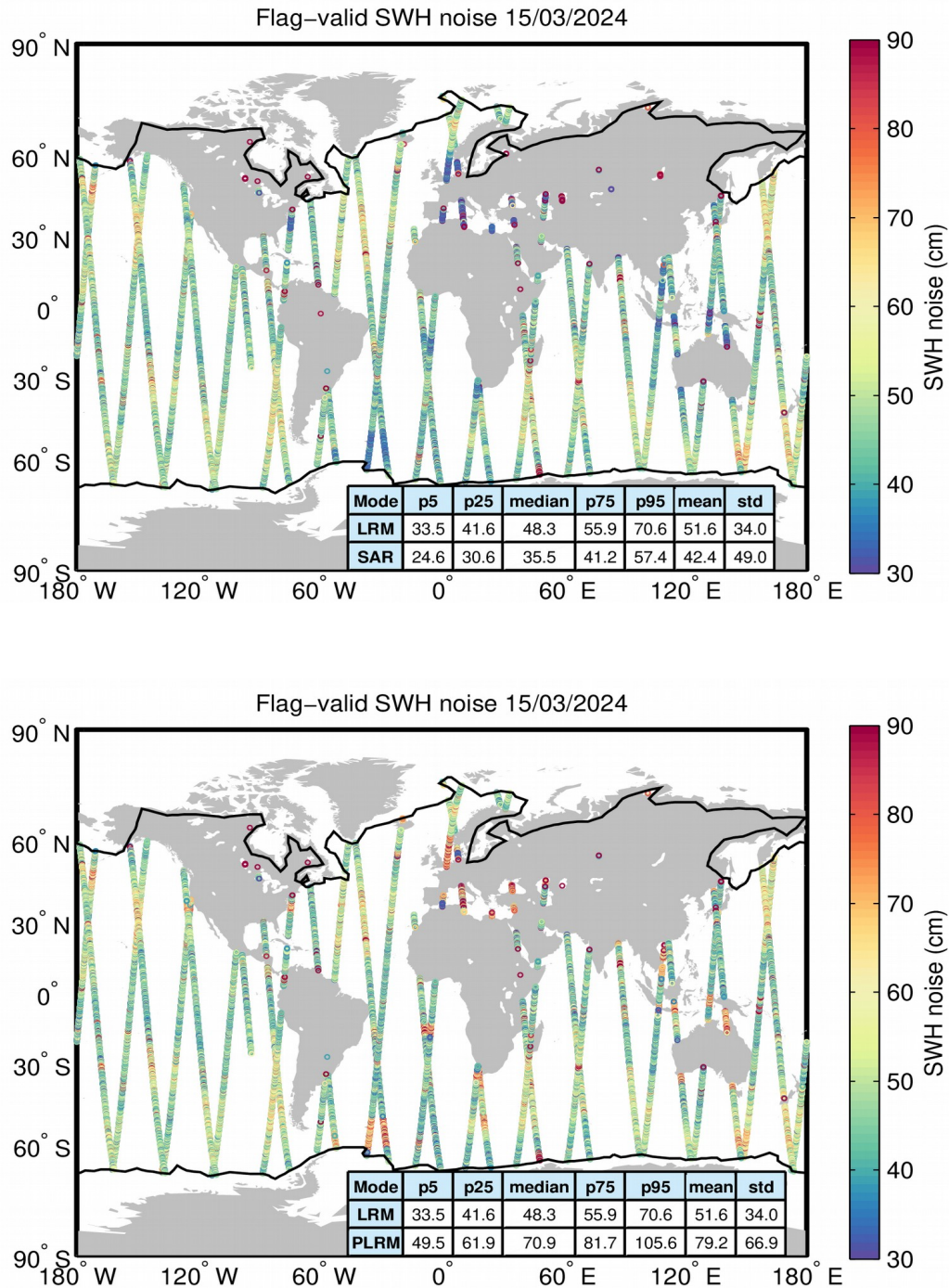
Figure 18. Geographical distribution of flag-valid 20-Hz SWH measurement noise over oceans and lakes for LRM/SAR (top) and LRM/PLRM (bottom) and for 15/03/2024. The statistical values shown in the table refer to the SWH noise and are calculated separately for LRM and SAR/PLRM regions. Measurements taken over polar polygons have been
