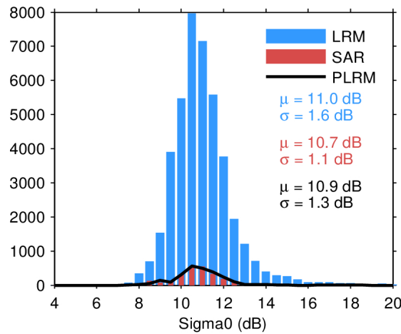
Figure 28. Histogram of science-valid sigma0 over oceans and lakes for LRM (blue), SAR (red), and PLRM (black) for 15/03/2024. The mean ( \mu ) and standard deviation ( \sigma ) are also shown. Note that values outside [4 20] dB are excluded from the histogram for the sake of readability but not from the computation of \mu and \sigma .
