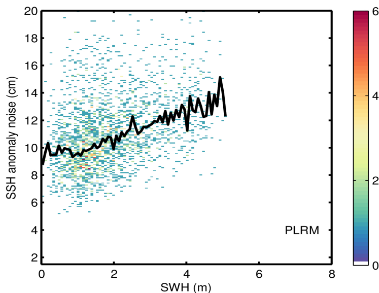
Figure 9. 2D histogram showing flag-valid SSH anomaly noise as a function of SWH for LRM (top), SAR (middle), and PLRM (bottom) for 15/03/2024. The black line denotes the median SSH anomaly noise as a function of SWH.
