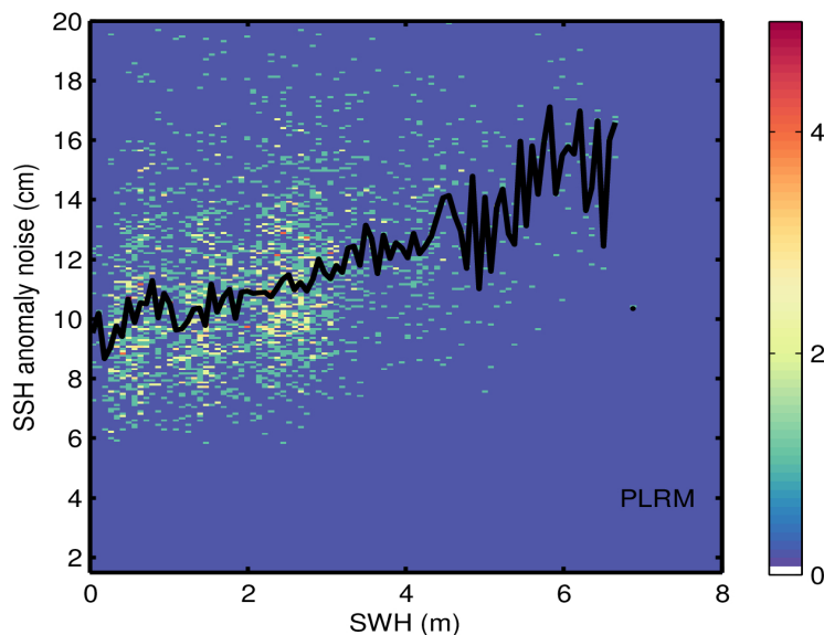
Figure 9. 2D histogram showing flag-valid SSH anomaly noise as a function of SWH for LRM (top), SAR (middle), and PLRM (bottom) for 14/03/2024. The black line denotes the median SSH anomaly noise as a function of SWH.
