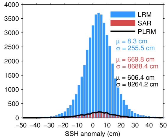
Figure 7. Histogram of flag-valid SSH anomaly over oceans and lakes for LRM (blue), SAR (red), and PLRM (black) for 14/03/2024. The mean ( \mu ) and standard deviation ( \sigma ) are also shown. Note that values outside [-50 50] cm are excluded from the histogram for the sake of readability but not from the computation of \mu and \sigma .
