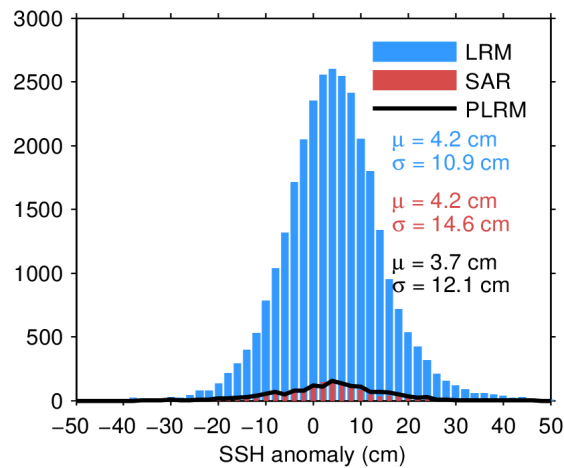
Figure 11. Histogram of science-valid SSH anomaly over oceans and lakes for LRM (blue), SAR (red), and PLRM (black) for 14/03/2024. The mean ( \mu ) and standard deviation ( \sigma ) are also shown. Note that values outside [-50\ 50] cm are excluded from the histogram for the sake of readability but not from the computation of \mu and \sigma .
