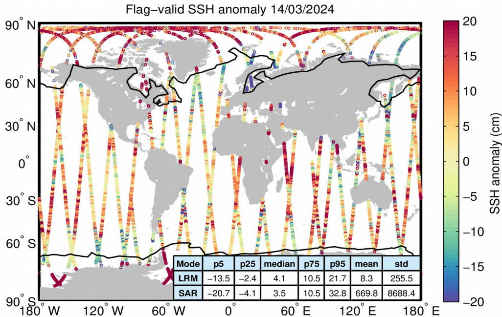
Figure 5. Geographical distribution of flag-valid 1-Hz SSH anomaly data over oceans and lakes for 14/03/2024. The statistical values shown in the table refer to the SSH anomaly in cm and are calculated separately for LRM and SAR regions. Measurements taken over polar polygons have been excluded from the computation of the statistical values. The black lines mark the outer limit of the Arctic and Antarctic polar polygons.
