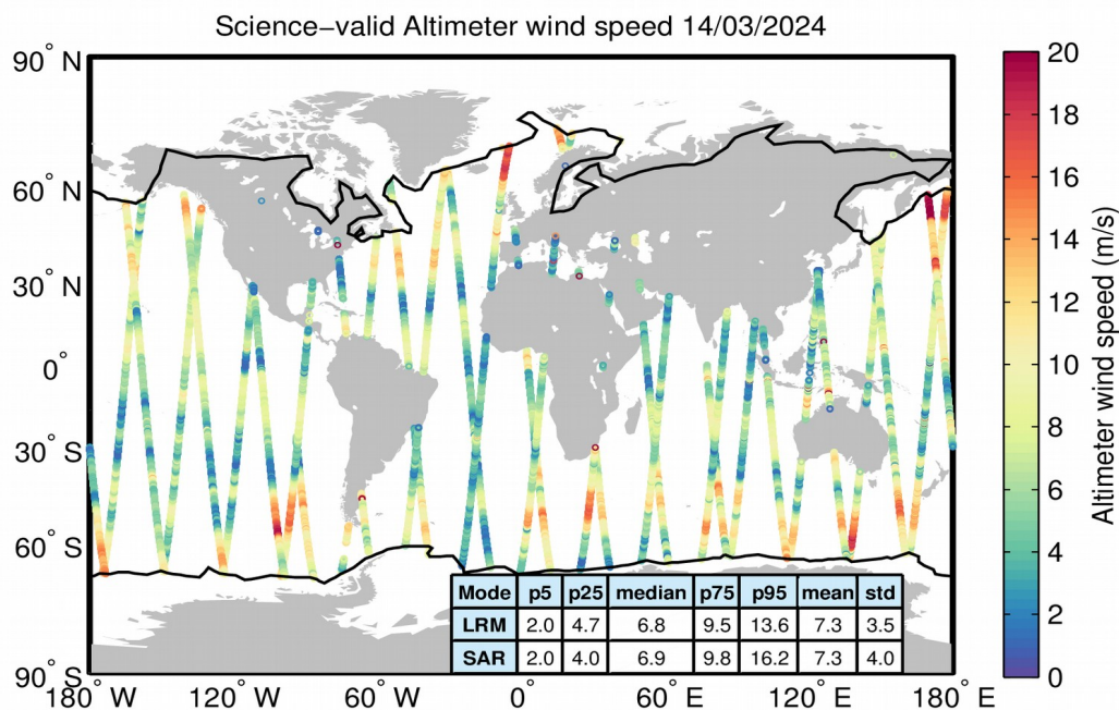
Figure 34. Geographical distribution of science-valid wind data over oceans and lakes for 14/03/2024. The statistical values shown in the table refer to the wind in m/s and are calculated separately for LRM and SAR regions. The black lines mark the outer limit of the Arctic and Antarctic polar polygons. Gray circles denote records that have been rejected based on the editing criteria described in Table 5.
