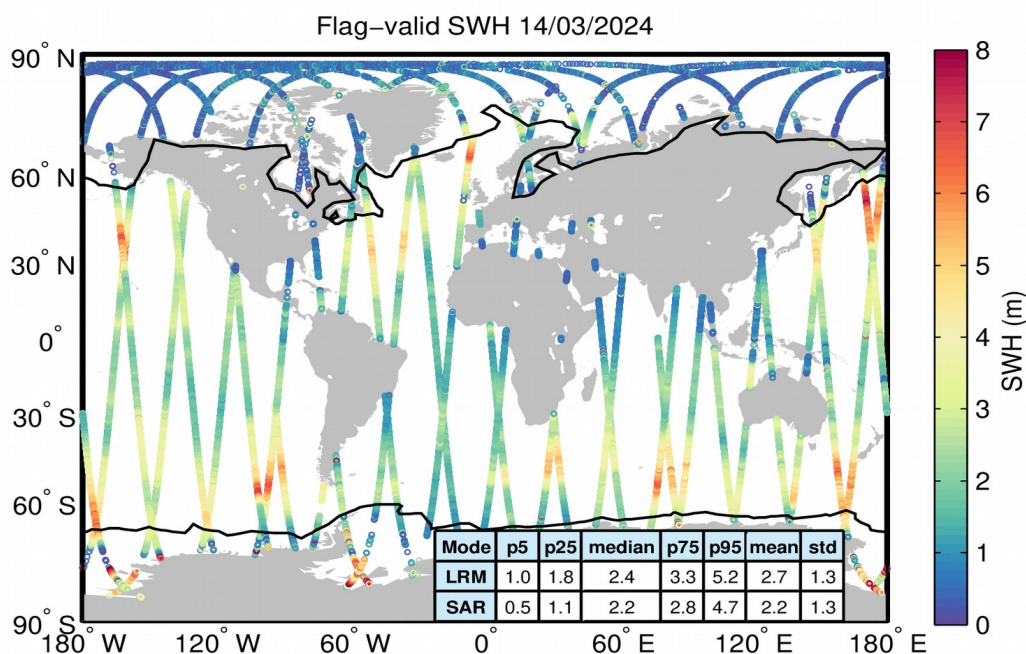
Figure 15. Geographical distribution of flag-valid SWH data over oceans and lakes for 14/03/2024. The statistical values shown in the table refer to the SWH in m and are calculated separately for LRM and SAR regions. Measurements taken over polar polygons have been excluded from the computation of the statistical values. The black lines mark the outer limit of the Arctic and Antarctic polar polygons.
