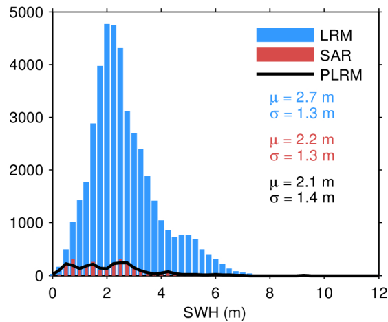
Figure 17. Histogram of flag-valid SWH over oceans and lakes for LRM (blue), SAR (red), and PLRM (black) for 14/03/2024. The mean ( \mu ) and standard deviation ( \sigma ) are also shown. Note that values larger than 12 m are excluded from the histogram for the sake of readability but not from the computation of \mu and \sigma .
