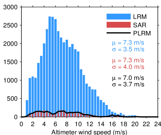
Figure 33. Histogram of flag-valid wind over oceans and lakes for LRM (blue), SAR (red), and PLRM (black) for 14/03/2024. The mean ( \mu ) and standard deviation ( \sigma ) are also shown. Note that values larger than 24 m/s are excluded from the histogram for the sake of readability but not from the computation of \mu and \sigma .
