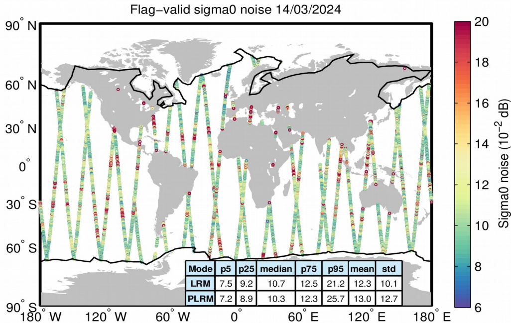
Figure 26. Geographical distribution of flag-valid 20-Hz sigma0 measurement noise over oceans and lakes for LRM/SAR (top) and LRM/PLRM (bottom) and for 14/03/2024. The statistical values shown in the table refer to the sigma0 noise and are calculated separately for LRM and SAR/PLRM regions. Measurements taken over polar polygons have been excluded from the computation of the statistical values. The black lines mark the outer limit of the Arctic and Antarctic polar polygons.
