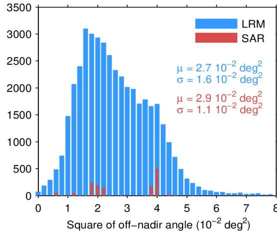
Figure 39. Histogram of flag-valid mispointing over oceans and lakes for LRM (blue) and SAR (red) for 14/03/2024. Only positive values have been considered. The mean ( \mu ) and standard deviation ( \sigma ) are also shown. Note that values larger than 8 \cdot 10^{-2} \text{ deg}^2 are excluded from the histogram for the sake of readability but not from the computation of \mu and \sigma .
