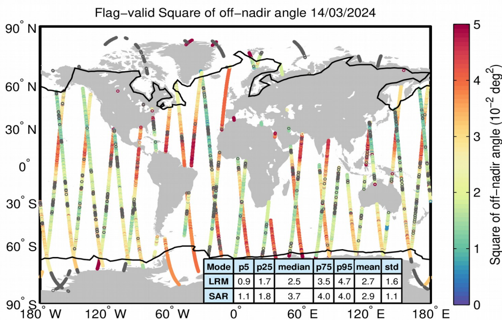
Figure 37. Geographical distribution of flag-valid mispointing data over oceans and lakes for 14/03/2024. The statistical values shown in the table refer to the mispointing in 10^{-2} \text{ deg}^2 and are calculated separately for LRM and SAR regions. Measurements taken over polar polygons have been excluded from the computation of the statistical values. The black lines mark the outer limit of the Arctic and Antarctic polar polygons. Gray circles denote negative values.
