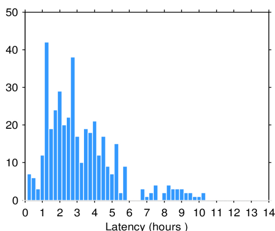
Figure 2. Histogram of the data latency for 14/03/2024. The y-axis denotes the number of files that are made available with a delay of x-hours with respect to the mean time of the records stored in the file.
