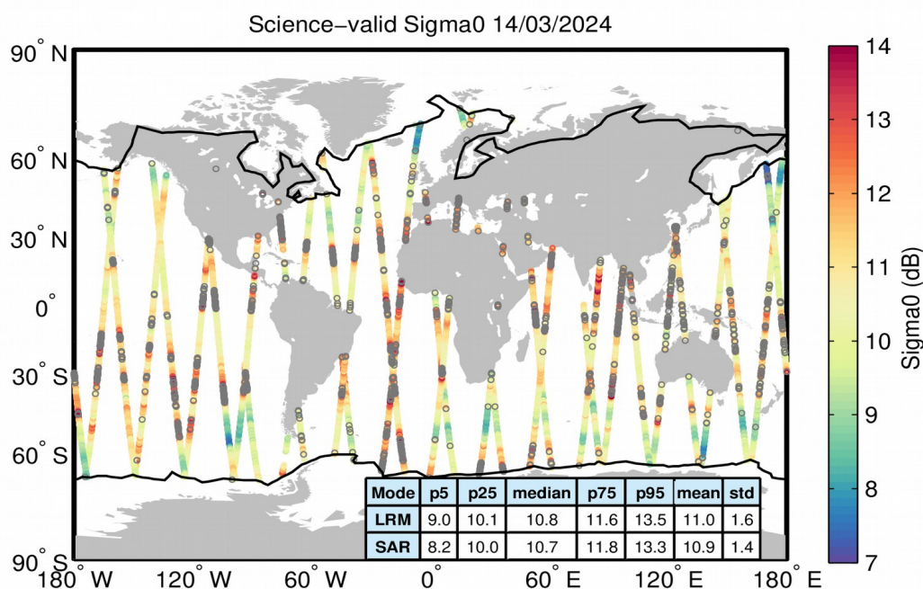
Figure 27. Geographical distribution of science-valid sigma0 data over oceans and lakes for 14/03/2024. The statistical values shown in the table refer to the sigma0 in dB and are calculated separately for LRM and SAR regions. The black lines mark the outer limit of the Arctic and Antarctic polar polygons. Gray circles denote records that have been rejected based on the editing criteria described in Table 4.
