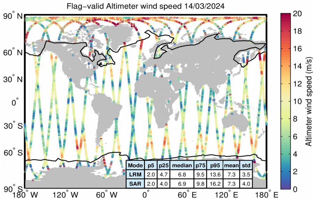
Figure 31. Geographical distribution of flag-valid wind data over oceans and lakes for 14/03/2024. The statistical values shown in the table refer to the wind in m/s and are calculated separately for LRM and SAR regions. Measurements taken over polar polygons have been excluded from the computation of the statistical values. The black lines mark the outer limit of the Arctic and Antarctic polar polygons.
