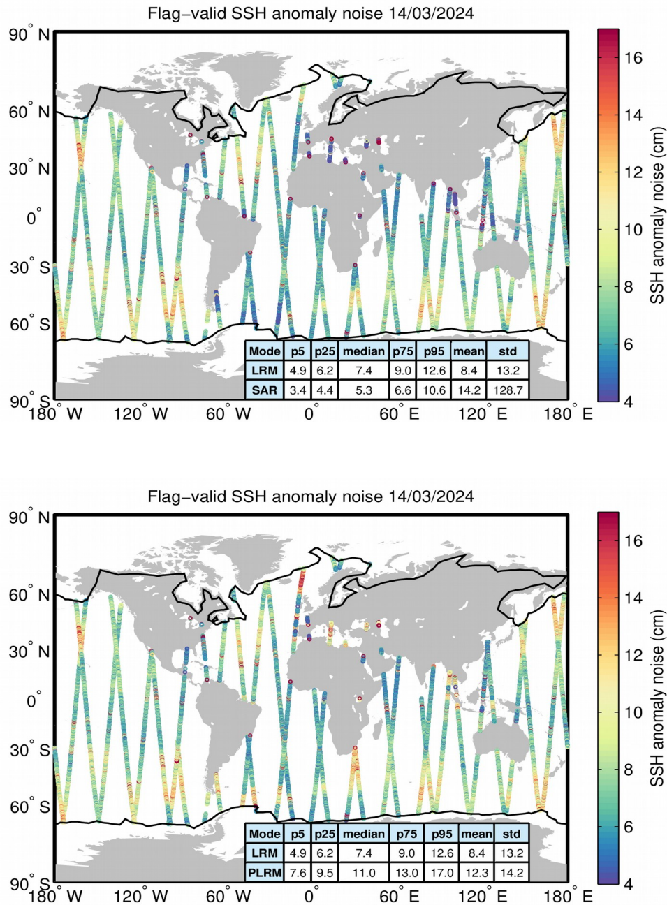
Figure 8. Geographical distribution of flag-valid 20-Hz SSH anomaly measurement noise over oceans and lakes for LRM/SAR (top) and LRM/PLRM (bottom) and for 14/03/2024. The statistical values shown in the tables refer to the SSH anomaly noise and are calculated separately for LRM and SAR/PLRM regions. Measurements taken over polar polygons have been excluded from the computation of the statistical values. The black lines mark the outer limit of the Arctic and Antarctic polar polygons.
