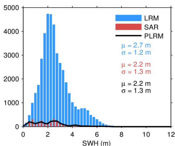
Figure 20. Histogram of science-valid SWH over oceans and lakes for LRM (blue), SAR (red), and PLRM (black) for 14/03/2024. The mean ( \mu ) and standard deviation ( \sigma ) are also
