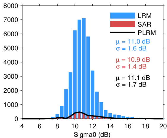
Figure 28. Histogram of science-valid sigma0 over oceans and lakes for LRM (blue), SAR (red), and PLRM (black) for 14/03/2024. The mean ( \mu ) and standard deviation ( \sigma ) are also shown. Note that values outside [4 20] dB are excluded from the histogram for the sake of readability but not from the computation of \mu and \sigma .
