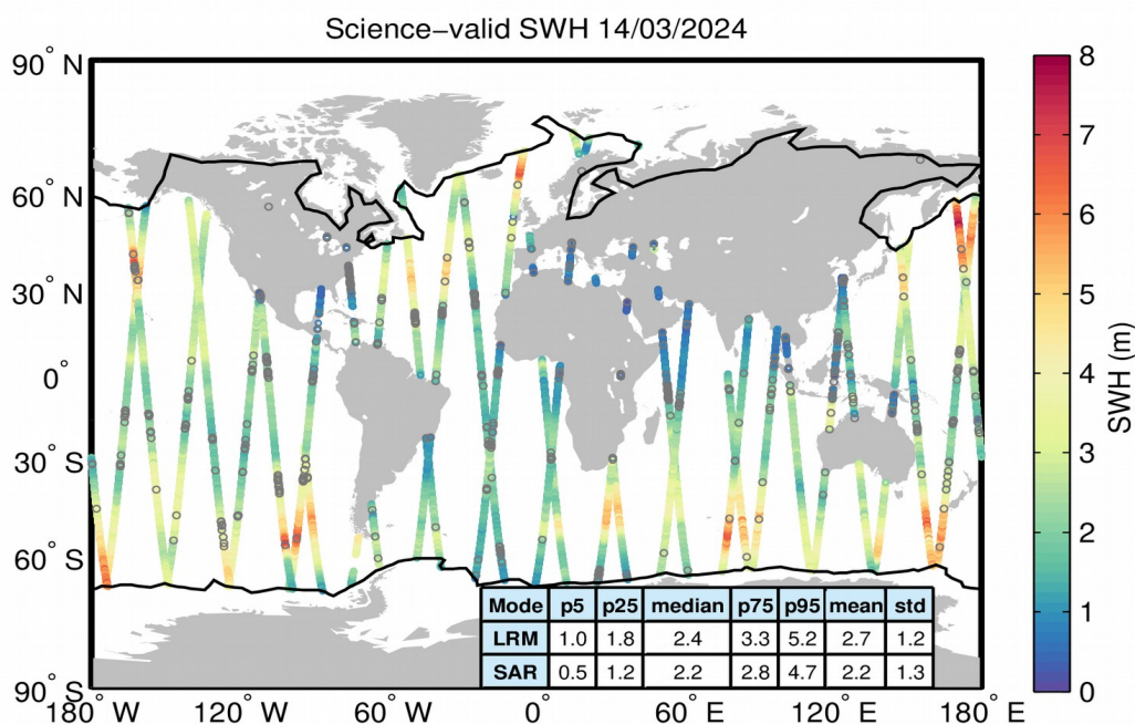
Figure 19. Geographical distribution of science-valid SWH data over oceans and lakes for 14/03/2024. The statistical values shown in the table refer to the SWH in m and are calculated separately for LRM and SAR regions. The black lines mark the outer limit of the Arctic and Antarctic polar polygons. Gray circles denote records that have been rejected based on the editing criteria described in Table 3.
