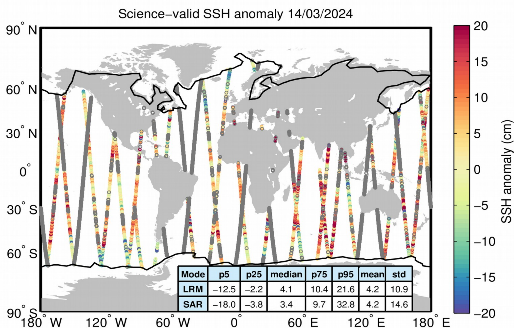
Figure 10. Geographical distribution of science-valid SSH anomaly data over oceans and lakes for 14/03/2024. The statistical values shown in the table refer to the SSH anomaly in cm and are calculated separately for LRM and SAR regions. The black lines mark the
