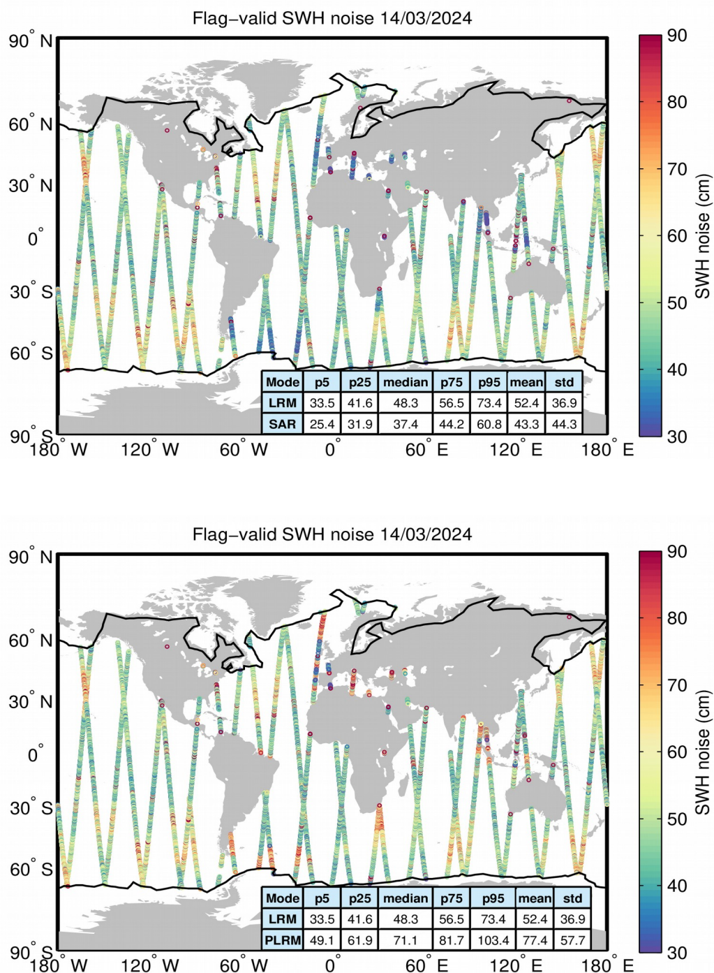
Figure 18. Geographical distribution of flag-valid 20-Hz SWH measurement noise over oceans and lakes for LRM/SAR (top) and LRM/PLRM (bottom) and for 14/03/2024. The statistical values shown in the table refer to the SWH noise and are calculated separately for LRM and SAR/PLRM regions. Measurements taken over polar polygons have been
