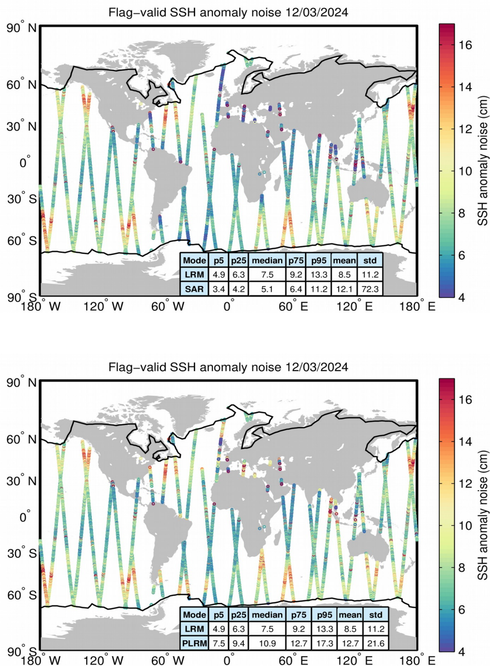
Figure 8. Geographical distribution of flag-valid 20-Hz SSH anomaly measurement noise over oceans and lakes for LRM/SAR (top) and LRM/PLRM (bottom) and for 12/03/2024. The statistical values shown in the tables refer to the SSH anomaly noise and are calculated separately for LRM and SAR/PLRM regions. Measurements taken over polar polygons have been excluded from the computation of the statistical values. The black lines mark the outer limit of the Arctic and Antarctic polar polygons.
