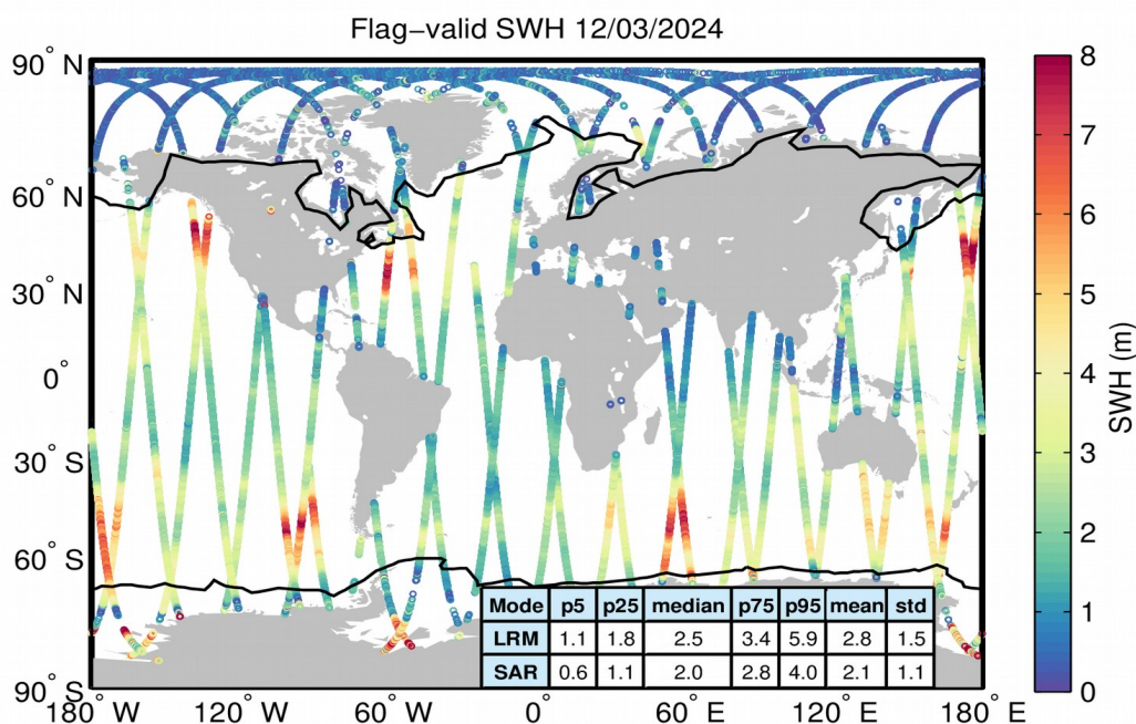
Figure 15. Geographical distribution of flag-valid SWH data over oceans and lakes for 12/03/2024. The statistical values shown in the table refer to the SWH in m and are calculated separately for LRM and SAR regions. Measurements taken over polar polygons have been excluded from the computation of the statistical values. The black lines mark the outer limit of the Arctic and Antarctic polar polygons.
