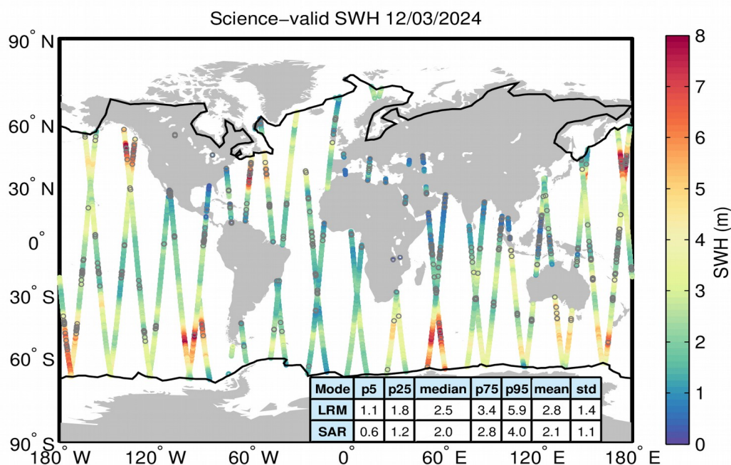
Figure 19. Geographical distribution of science-valid SWH data over oceans and lakes for 12/03/2024. The statistical values shown in the table refer to the SWH in m and are calculated separately for LRM and SAR regions. The black lines mark the outer limit of the Arctic and Antarctic polar polygons. Gray circles denote records that have been rejected based on the editing criteria described in Table 3.
