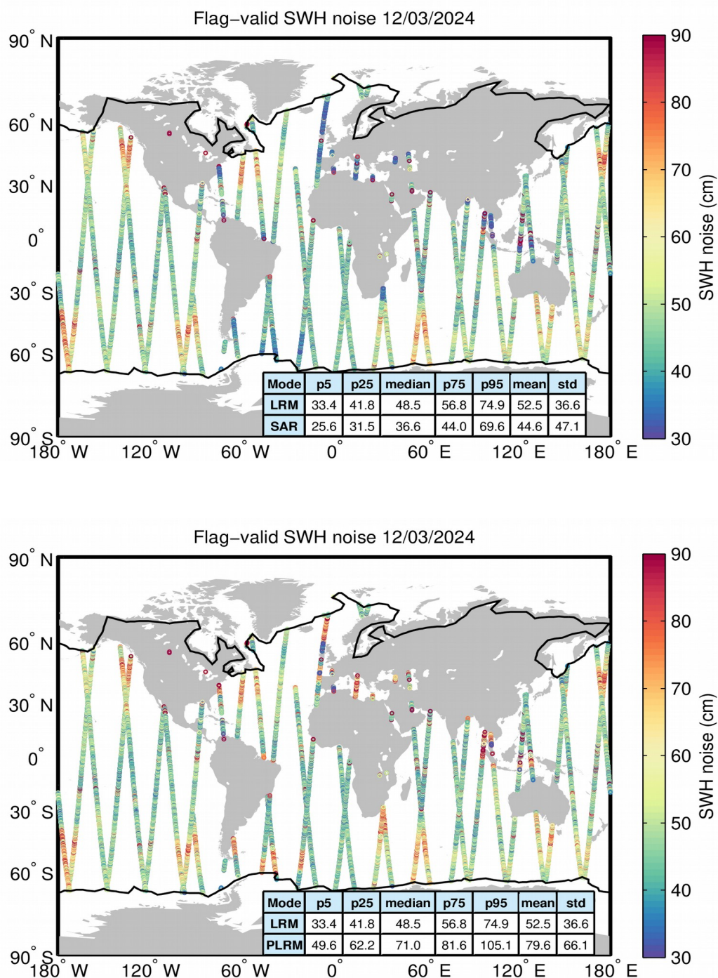
Figure 18. Geographical distribution of flag-valid 20-Hz SWH measurement noise over oceans and lakes for LRM/SAR (top) and LRM/PLRM (bottom) and for 12/03/2024. The statistical values shown in the table refer to the SWH noise and are calculated separately for LRM and SAR/PLRM regions. Measurements taken over polar polygons have been
