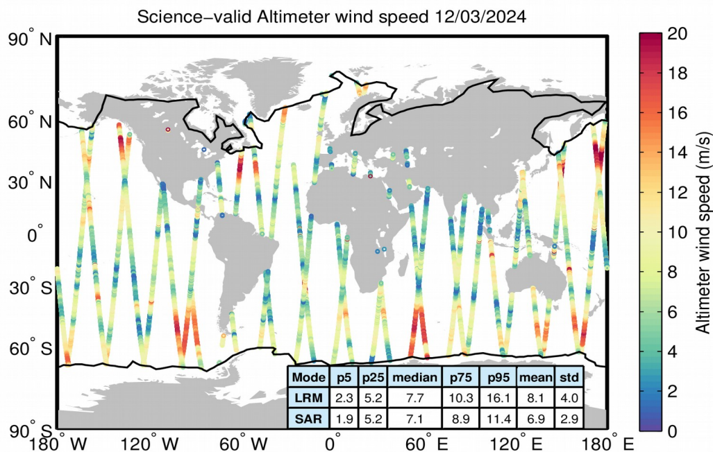
Figure 34. Geographical distribution of science-valid wind data over oceans and lakes for 12/03/2024. The statistical values shown in the table refer to the wind in m/s and are calculated separately for LRM and SAR regions. The black lines mark the outer limit of the Arctic and Antarctic polar polygons. Gray circles denote records that have been rejected based on the editing criteria described in Table 5.
