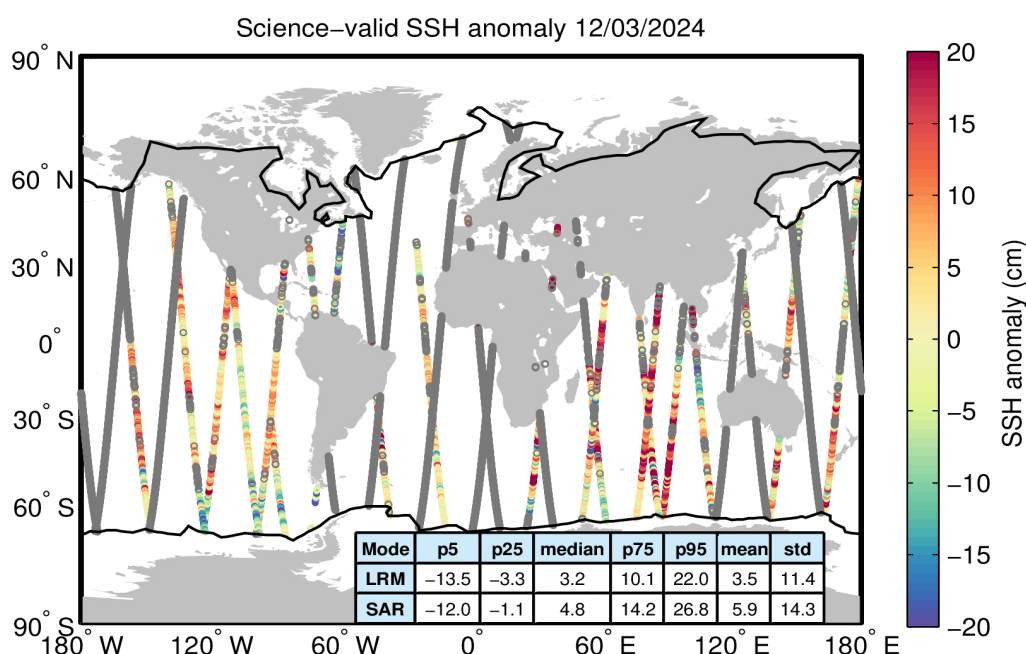
Figure 10. Geographical distribution of science-valid SSH anomaly data over oceans and lakes for 12/03/2024. The statistical values shown in the table refer to the SSH anomaly in cm and are calculated separately for LRM and SAR regions. The black lines mark the
