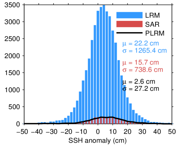
Figure 7. Histogram of flag-valid SSH anomaly over oceans and lakes for LRM (blue), SAR (red), and PLRM (black) for 12/03/2024. The mean ( \mu ) and standard deviation ( \sigma ) are also shown. Note that values outside [-50\ 50] cm are excluded from the histogram for the sake of readability but not from the computation of \mu and \sigma .
