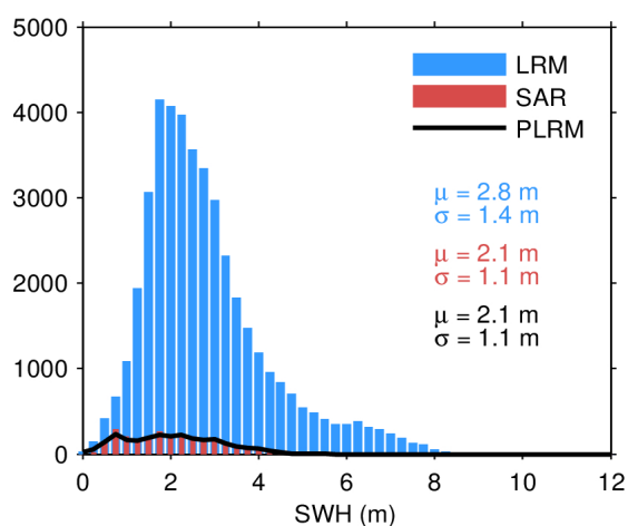
Figure 20. Histogram of science-valid SWH over oceans and lakes for LRM (blue), SAR (red), and PLRM (black) for 12/03/2024. The mean ( \mu ) and standard deviation ( \sigma ) are also
