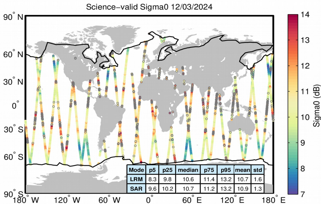
Figure 27. Geographical distribution of science-valid sigma0 data over oceans and lakes for 12/03/2024. The statistical values shown in the table refer to the sigma0 in dB and are calculated separately for LRM and SAR regions. The black lines mark the outer limit of the Arctic and Antarctic polar polygons. Gray circles denote records that have been rejected based on the editing criteria described in Table 4.
