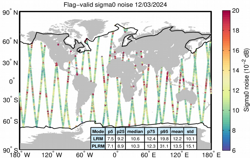
Figure 26. Geographical distribution of flag-valid 20-Hz sigma0 measurement noise over oceans and lakes for LRM/SAR (top) and LRM/PLRM (bottom) and for 12/03/2024. The statistical values shown in the table refer to the sigma0 noise and are calculated separately for LRM and SAR/PLRM regions. Measurements taken over polar polygons have been excluded from the computation of the statistical values. The black lines mark the outer limit of the Arctic and Antarctic polar polygons.
