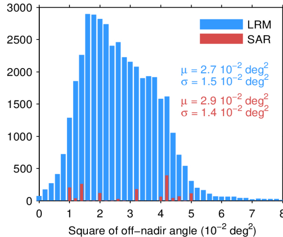
Figure 39. Histogram of flag-valid mispointing over oceans and lakes for LRM (blue) and SAR (red) for 12/03/2024. Only positive values have been considered. The mean ( \mu ) and standard deviation ( \sigma ) are also shown. Note that values larger than 8 \cdot 10^{-2} \text{ deg}^2 are excluded from the histogram for the sake of readability but not from the computation of \mu and \sigma .
