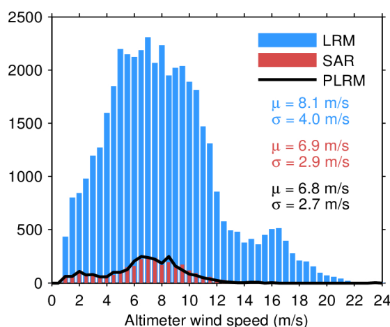
Figure 33. Histogram of flag-valid wind over oceans and lakes for LRM (blue), SAR (red), and PLRM (black) for 12/03/2024. The mean ( \mu ) and standard deviation ( \sigma ) are also shown. Note that values larger than 24 m/s are excluded from the histogram for the sake of readability but not from the computation of \mu and \sigma .
