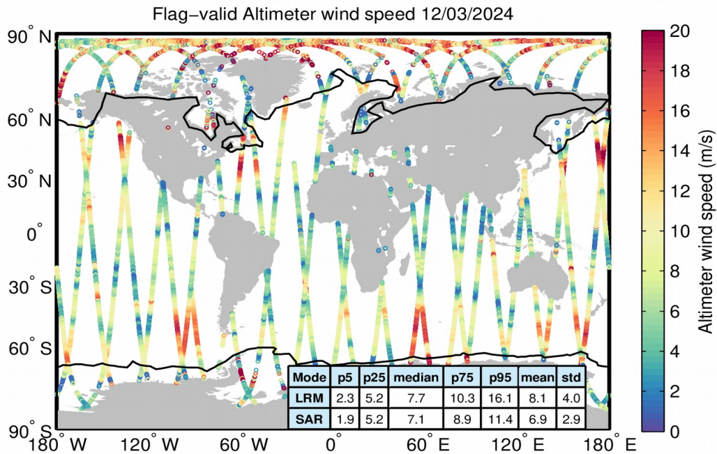
Figure 31. Geographical distribution of flag-valid wind data over oceans and lakes for 12/03/2024. The statistical values shown in the table refer to the wind in m/s and are calculated separately for LRM and SAR regions. Measurements taken over polar polygons have been excluded from the computation of the statistical values. The black lines mark the outer limit of the Arctic and Antarctic polar polygons.
