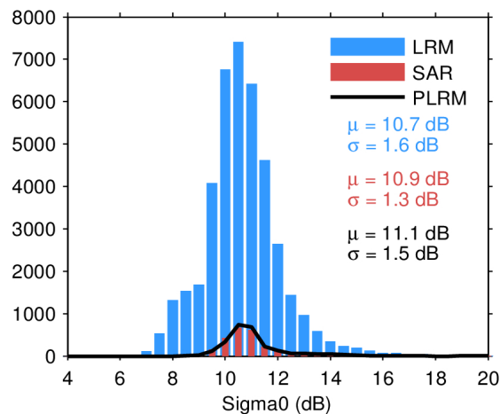
Figure 28. Histogram of science-valid sigma0 over oceans and lakes for LRM (blue), SAR (red), and PLRM (black) for 12/03/2024. The mean ( \mu ) and standard deviation ( \sigma ) are also shown. Note that values outside [4 20] dB are excluded from the histogram for the sake of readability but not from the computation of \mu and \sigma .
