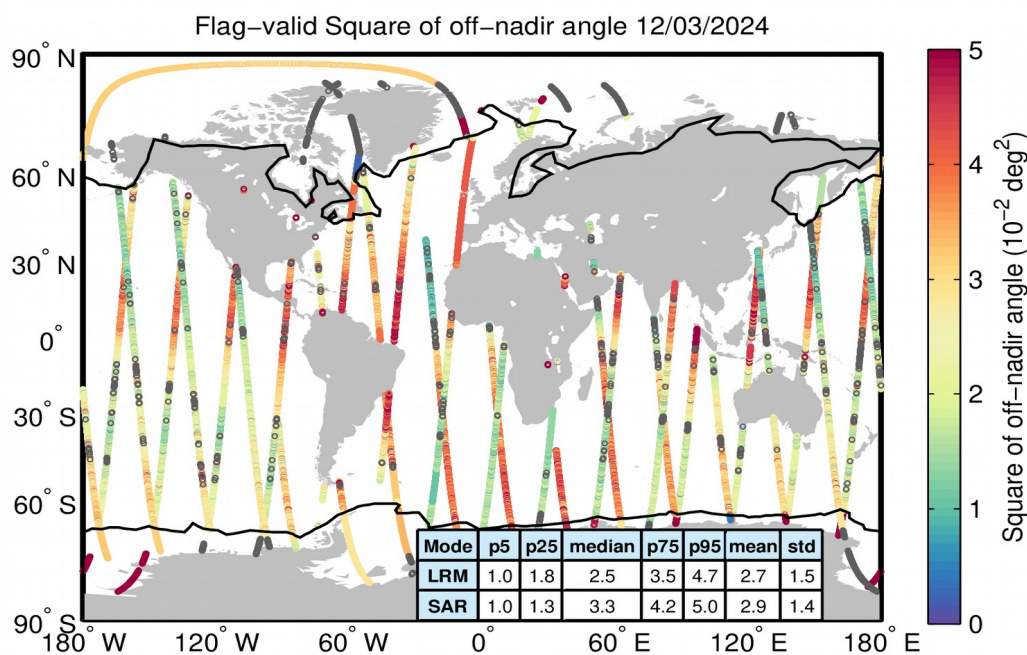
Figure 37. Geographical distribution of flag-valid mispointing data over oceans and lakes for 12/03/2024. The statistical values shown in the table refer to the mispointing in 10^{-2} \text{ deg}^2 and are calculated separately for LRM and SAR regions. Measurements taken over polar polygons have been excluded from the computation of the statistical values. The black lines mark the outer limit of the Arctic and Antarctic polar polygons. Gray circles denote negative values.
