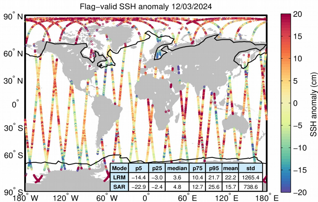
Figure 5. Geographical distribution of flag-valid 1-Hz SSH anomaly data over oceans and lakes for 12/03/2024. The statistical values shown in the table refer to the SSH anomaly in cm and are calculated separately for LRM and SAR regions. Measurements taken over polar polygons have been excluded from the computation of the statistical values. The black lines mark the outer limit of the Arctic and Antarctic polar polygons.
