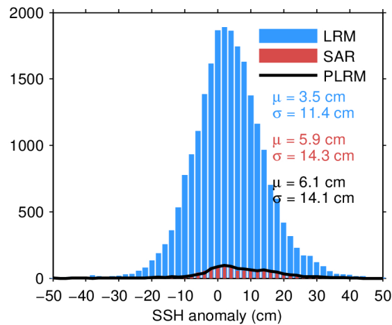
Figure 11. Histogram of science-valid SSH anomaly over oceans and lakes for LRM (blue), SAR (red), and PLRM (black) for 12/03/2024. The mean ( \mu ) and standard deviation ( \sigma ) are also shown. Note that values outside [-50\ 50] cm are excluded from the histogram for the sake of readability but not from the computation of \mu and \sigma .
