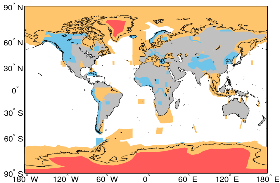
Figure A1. Extent of the regions defining the geographical mode mask for 12/03/2024. The regions where SAR, and SARIn are operated are denoted by the orange and blue polygons, respectively. LRM is operated over areas of the continental ice sheets (red polygons) and over oceans and land not covered by other modes.
