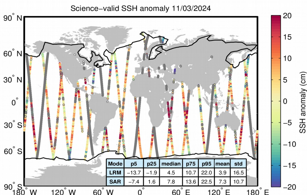
Figure 10. Geographical distribution of science-valid SSH anomaly data over oceans and lakes for 11/03/2024. The statistical values shown in the table refer to the SSH anomaly in cm and are calculated separately for LRM and SAR regions. The black lines mark the
