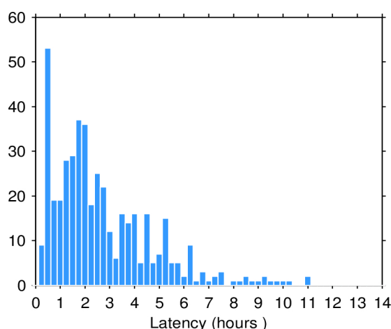
Figure 2. Histogram of the data latency for 11/03/2024. The y-axis denotes the number of files that are made available with a delay of x-hours with respect to the mean time of the records stored in the file.
