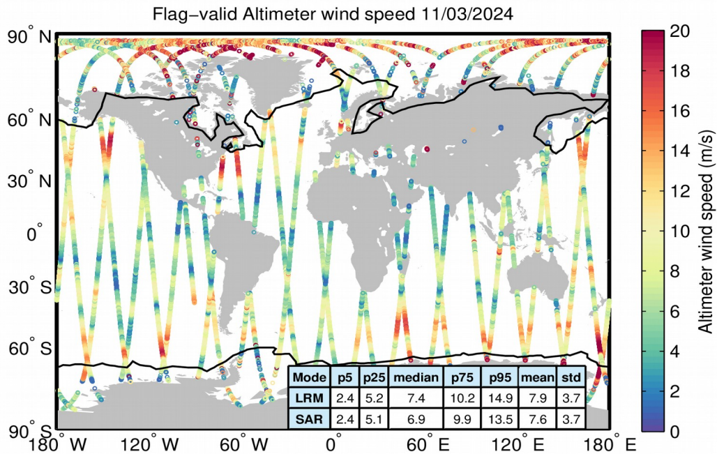
Figure 31. Geographical distribution of flag-valid wind data over oceans and lakes for 11/03/2024. The statistical values shown in the table refer to the wind in m/s and are calculated separately for LRM and SAR regions. Measurements taken over polar polygons have been excluded from the computation of the statistical values. The black lines mark the outer limit of the Arctic and Antarctic polar polygons.
