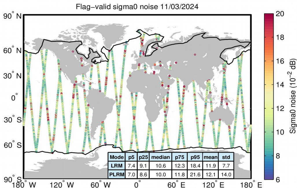
Figure 26. Geographical distribution of flag-valid 20-Hz sigma0 measurement noise over oceans and lakes for LRM/SAR (top) and LRM/PLRM (bottom) and for 11/03/2024. The statistical values shown in the table refer to the sigma0 noise and are calculated separately for LRM and SAR/PLRM regions. Measurements taken over polar polygons have been excluded from the computation of the statistical values. The black lines mark the outer limit of the Arctic and Antarctic polar polygons.
