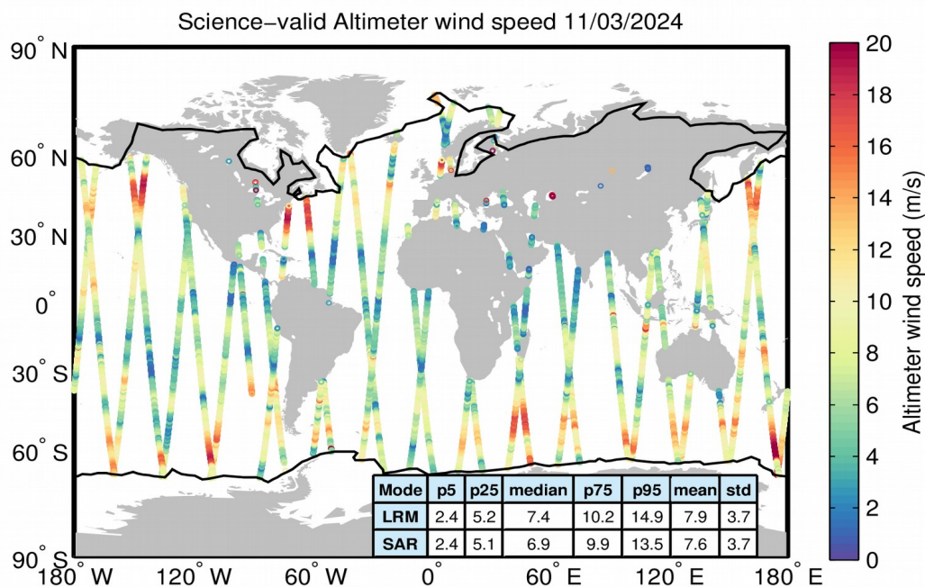
Figure 34. Geographical distribution of science-valid wind data over oceans and lakes for 11/03/2024. The statistical values shown in the table refer to the wind in m/s and are calculated separately for LRM and SAR regions. The black lines mark the outer limit of the Arctic and Antarctic polar polygons. Gray circles denote records that have been rejected based on the editing criteria described in Table 5.
