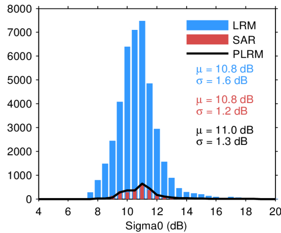
Figure 28. Histogram of science-valid sigma0 over oceans and lakes for LRM (blue), SAR (red), and PLRM (black) for 11/03/2024. The mean ( \mu ) and standard deviation ( \sigma ) are also shown. Note that values outside [4 20] dB are excluded from the histogram for the sake of readability but not from the computation of \mu and \sigma .
