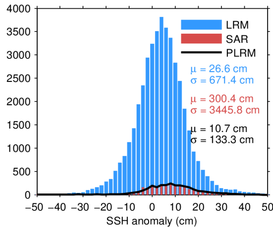
Figure 7. Histogram of flag-valid SSH anomaly over oceans and lakes for LRM (blue), SAR (red), and PLRM (black) for 11/03/2024. The mean ( \mu ) and standard deviation ( \sigma ) are also shown. Note that values outside [-50 50] cm are excluded from the histogram for the sake of readability but not from the computation of \mu and \sigma .
