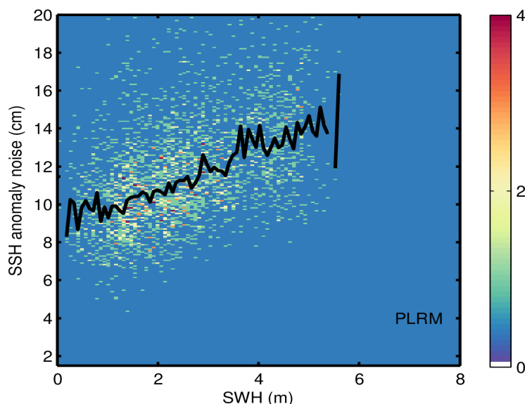
Figure 9. 2D histogram showing flag-valid SSH anomaly noise as a function of SWH for LRM (top), SAR (middle), and PLRM (bottom) for 11/03/2024. The black line denotes the median SSH anomaly noise as a function of SWH.
