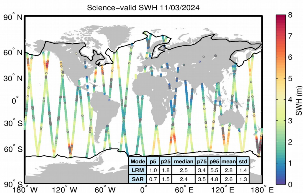
Figure 19. Geographical distribution of science-valid SWH data over oceans and lakes for 11/03/2024. The statistical values shown in the table refer to the SWH in m and are calculated separately for LRM and SAR regions. The black lines mark the outer limit of the Arctic and Antarctic polar polygons. Gray circles denote records that have been rejected based on the editing criteria described in Table 3.
