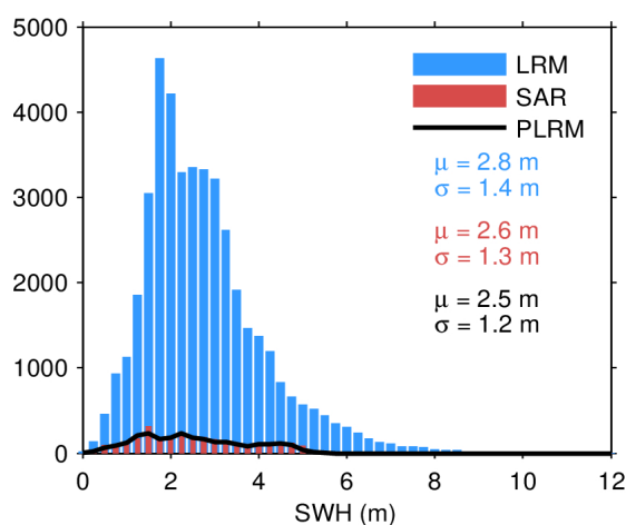
Figure 20. Histogram of science-valid SWH over oceans and lakes for LRM (blue), SAR (red), and PLRM (black) for 11/03/2024. The mean ( \mu ) and standard deviation ( \sigma ) are also
