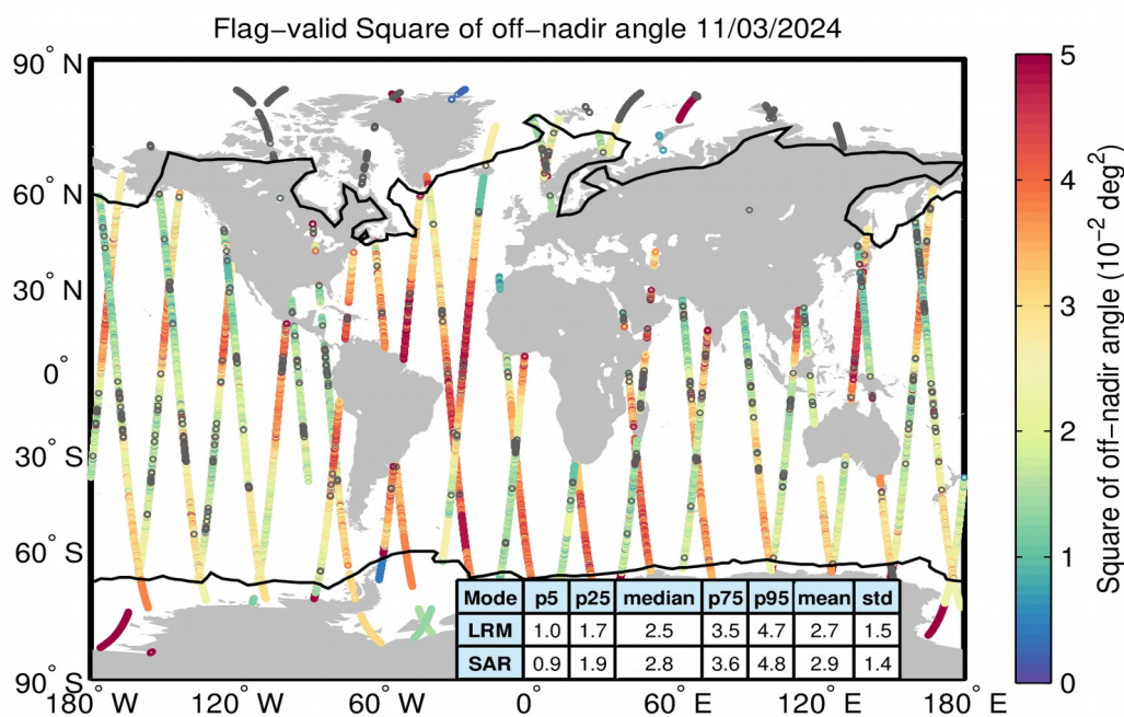
Figure 37. Geographical distribution of flag-valid mispointing data over oceans and lakes for 11/03/2024. The statistical values shown in the table refer to the mispointing in 10^{-2} \text{ deg}^2 and are calculated separately for LRM and SAR regions. Measurements taken over polar polygons have been excluded from the computation of the statistical values. The black lines mark the outer limit of the Arctic and Antarctic polar polygons. Gray circles denote negative values.
