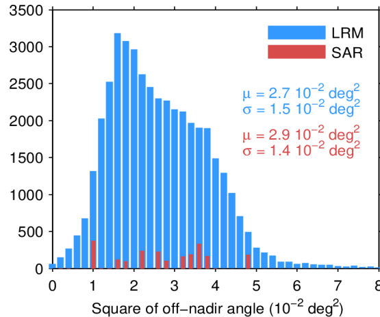
Figure 39. Histogram of flag-valid mispointing over oceans and lakes for LRM (blue) and SAR (red) for 11/03/2024. Only positive values have been considered. The mean ( \mu ) and standard deviation ( \sigma ) are also shown. Note that values larger than 8 \cdot 10^{-2} \text{ deg}^2 are excluded from the histogram for the sake of readability but not from the computation of \mu and \sigma .
