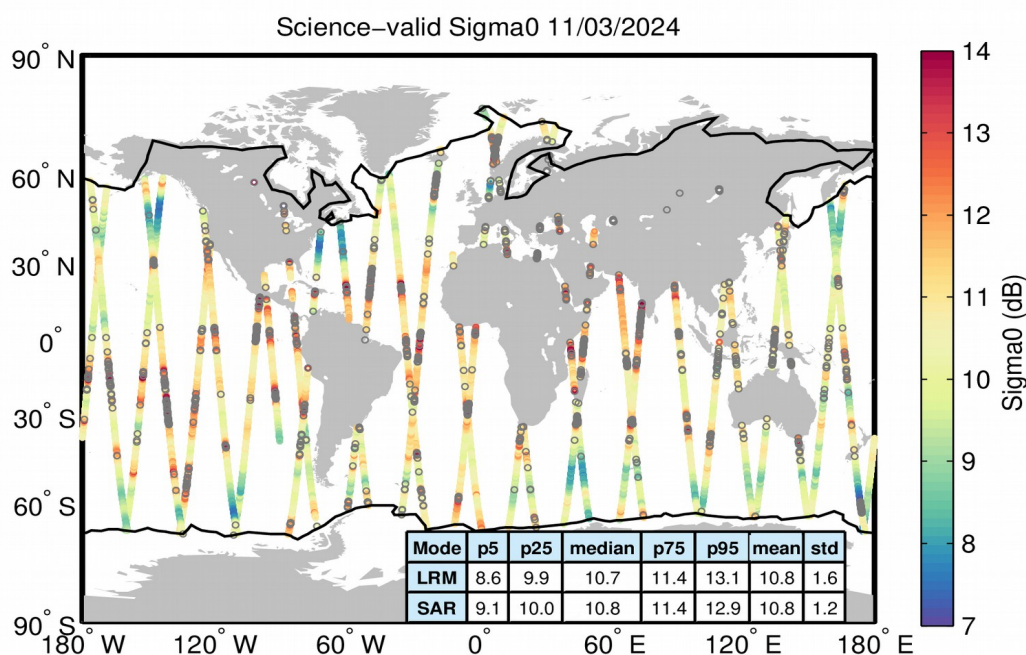
Figure 27. Geographical distribution of science-valid sigma0 data over oceans and lakes for 11/03/2024. The statistical values shown in the table refer to the sigma0 in dB and are calculated separately for LRM and SAR regions. The black lines mark the outer limit of the Arctic and Antarctic polar polygons. Gray circles denote records that have been rejected based on the editing criteria described in Table 4.
