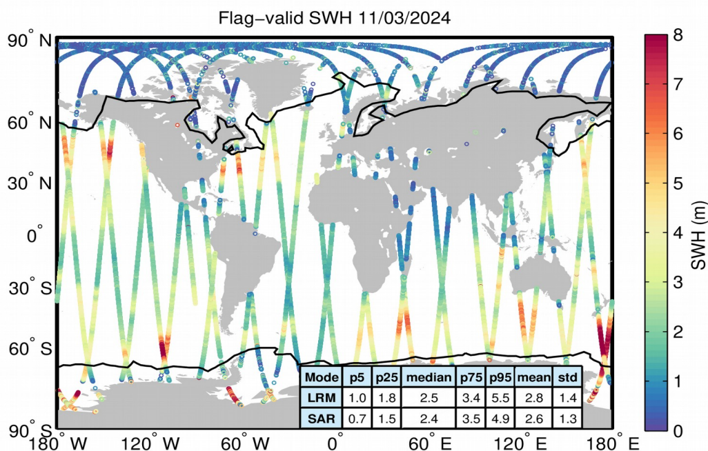
Figure 15. Geographical distribution of flag-valid SWH data over oceans and lakes for 11/03/2024. The statistical values shown in the table refer to the SWH in m and are calculated separately for LRM and SAR regions. Measurements taken over polar polygons have been excluded from the computation of the statistical values. The black lines mark the outer limit of the Arctic and Antarctic polar polygons.
