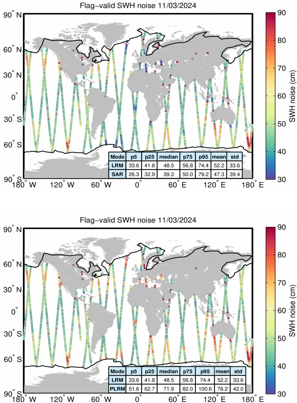
Figure 18. Geographical distribution of flag-valid 20-Hz SWH measurement noise over oceans and lakes for LRM/SAR (top) and LRM/PLRM (bottom) and for 11/03/2024. The statistical values shown in the table refer to the SWH noise and are calculated separately for LRM and SAR/PLRM regions. Measurements taken over polar polygons have been
