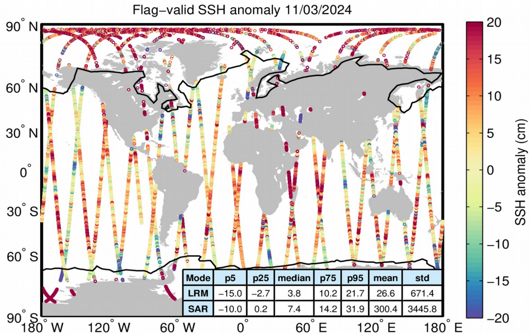
Figure 5. Geographical distribution of flag-valid 1-Hz SSH anomaly data over oceans and lakes for 11/03/2024. The statistical values shown in the table refer to the SSH anomaly in cm and are calculated separately for LRM and SAR regions. Measurements taken over polar polygons have been excluded from the computation of the statistical values. The black lines mark the outer limit of the Arctic and Antarctic polar polygons.
