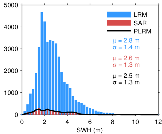
Figure 17. Histogram of flag-valid SWH over oceans and lakes for LRM (blue), SAR (red), and PLRM (black) for 11/03/2024. The mean ( \mu ) and standard deviation ( \sigma ) are also shown. Note that values larger than 12 m are excluded from the histogram for the sake of readability but not from the computation of \mu and \sigma .
