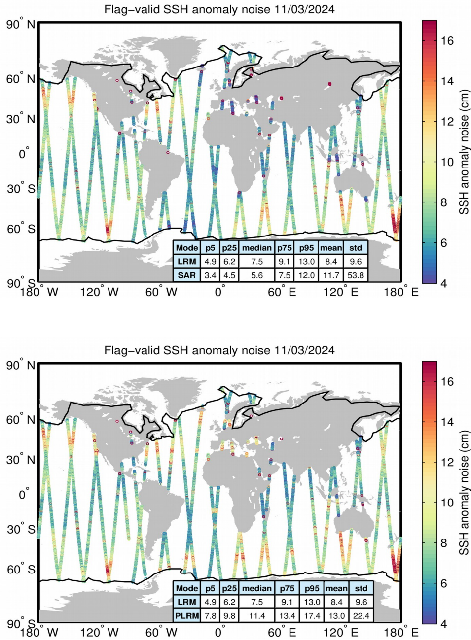
Figure 8. Geographical distribution of flag-valid 20-Hz SSH anomaly measurement noise over oceans and lakes for LRM/SAR (top) and LRM/PLRM (bottom) and for 11/03/2024. The statistical values shown in the tables refer to the SSH anomaly noise and are calculated separately for LRM and SAR/PLRM regions. Measurements taken over polar polygons have been excluded from the computation of the statistical values. The black lines mark the outer limit of the Arctic and Antarctic polar polygons.
