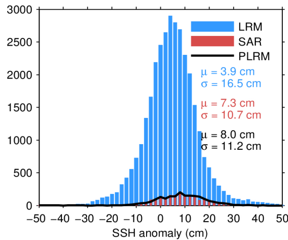
Figure 11. Histogram of science-valid SSH anomaly over oceans and lakes for LRM (blue), SAR (red), and PLRM (black) for 11/03/2024. The mean ( \mu ) and standard deviation ( \sigma ) are also shown. Note that values outside [-50\ 50] cm are excluded from the histogram for the sake of readability but not from the computation of \mu and \sigma .
