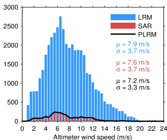
Figure 33. Histogram of flag-valid wind over oceans and lakes for LRM (blue), SAR (red), and PLRM (black) for 11/03/2024. The mean ( \mu ) and standard deviation ( \sigma ) are also shown. Note that values larger than 24 m/s are excluded from the histogram for the sake of readability but not from the computation of \mu and \sigma .
