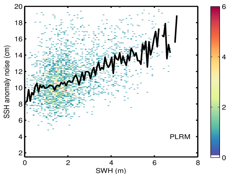
Figure 9. 2D histogram showing flag-valid SSH anomaly noise as a function of SWH for LRM (top), SAR (middle), and PLRM (bottom) for 10/03/2024. The black line denotes the median SSH anomaly noise as a function of SWH.
