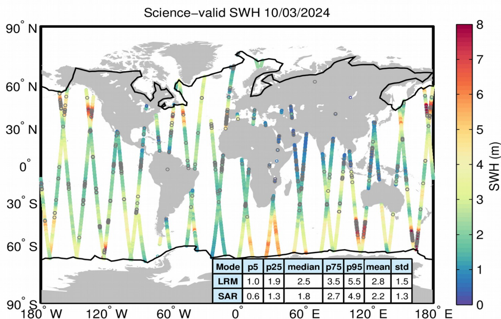
Figure 19. Geographical distribution of science-valid SWH data over oceans and lakes for 10/03/2024. The statistical values shown in the table refer to the SWH in m and are calculated separately for LRM and SAR regions. The black lines mark the outer limit of the Arctic and Antarctic polar polygons. Gray circles denote records that have been rejected based on the editing criteria described in Table 3.
