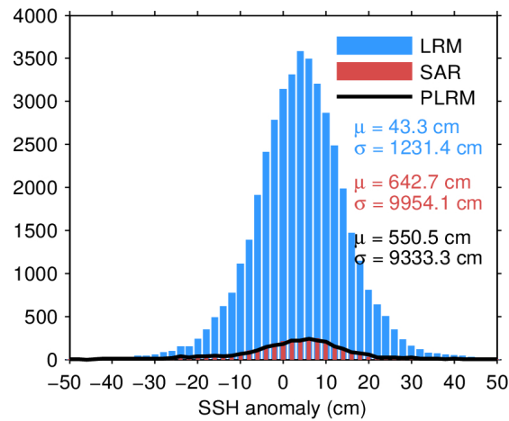
Figure 7. Histogram of flag-valid SSH anomaly over oceans and lakes for LRM (blue), SAR (red), and PLRM (black) for 10/03/2024. The mean ( \mu ) and standard deviation ( \sigma ) are also shown. Note that values outside [-50 50] cm are excluded from the histogram for the sake of readability but not from the computation of \mu and \sigma .
