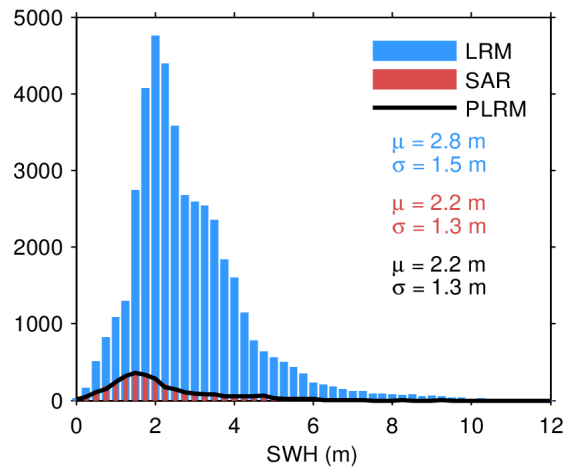
Figure 17. Histogram of flag-valid SWH over oceans and lakes for LRM (blue), SAR (red), and PLRM (black) for 10/03/2024. The mean ( \mu ) and standard deviation ( \sigma ) are also shown. Note that values larger than 12 m are excluded from the histogram for the sake of readability but not from the computation of \mu and \sigma .
