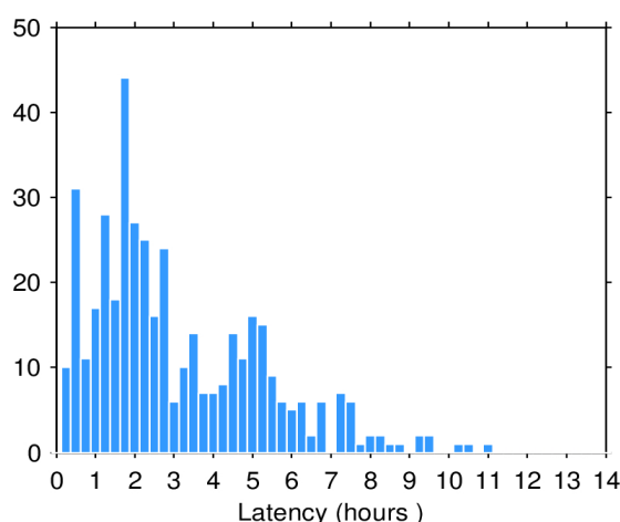
Figure 2. Histogram of the data latency for 10/03/2024. The y-axis denotes the number of files that are made available with a delay of x-hours with respect to the mean time of the records stored in the file.
