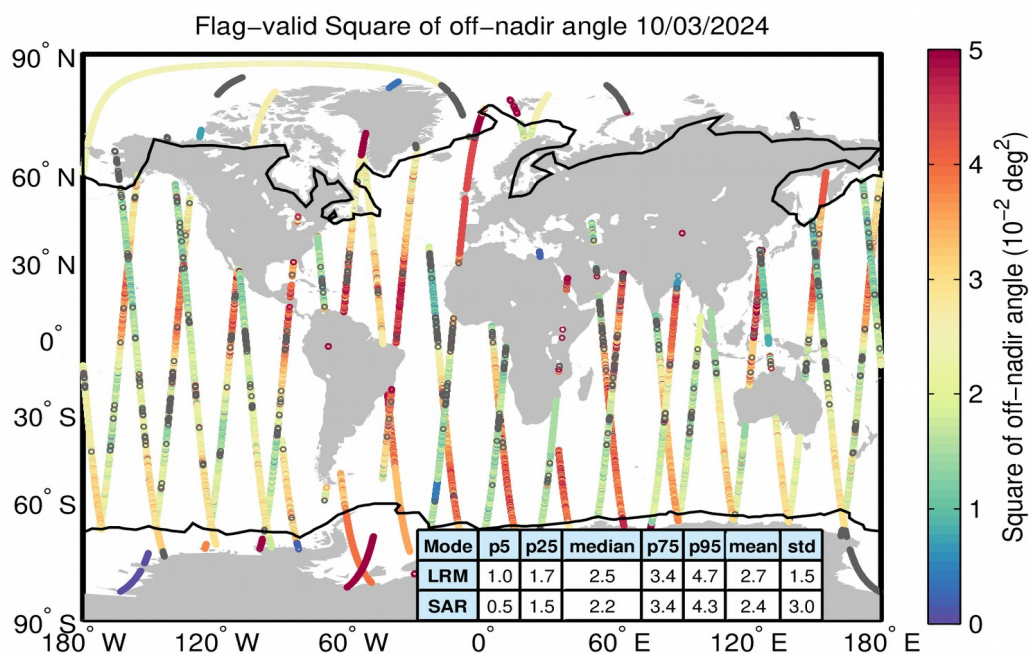
Figure 37. Geographical distribution of flag-valid mispointing data over oceans and lakes for 10/03/2024. The statistical values shown in the table refer to the mispointing in 10^{-2} \text{ deg}^2 and are calculated separately for LRM and SAR regions. Measurements taken over polar polygons have been excluded from the computation of the statistical values. The black lines mark the outer limit of the Arctic and Antarctic polar polygons. Gray circles denote negative values.
