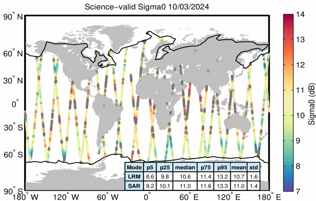
Figure 27. Geographical distribution of science-valid sigma0 data over oceans and lakes for 10/03/2024. The statistical values shown in the table refer to the sigma0 in dB and are calculated separately for LRM and SAR regions. The black lines mark the outer limit of the Arctic and Antarctic polar polygons. Gray circles denote records that have been rejected based on the editing criteria described in Table 4.
