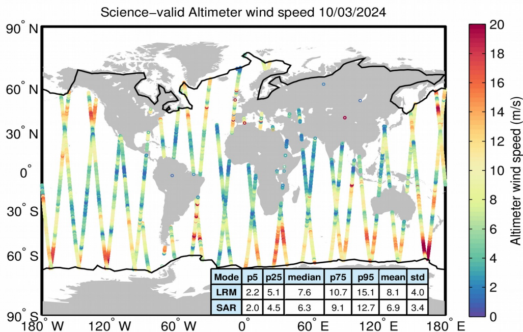
Figure 34. Geographical distribution of science-valid wind data over oceans and lakes for 10/03/2024. The statistical values shown in the table refer to the wind in m/s and are calculated separately for LRM and SAR regions. The black lines mark the outer limit of the Arctic and Antarctic polar polygons. Gray circles denote records that have been rejected based on the editing criteria described in Table 5.
