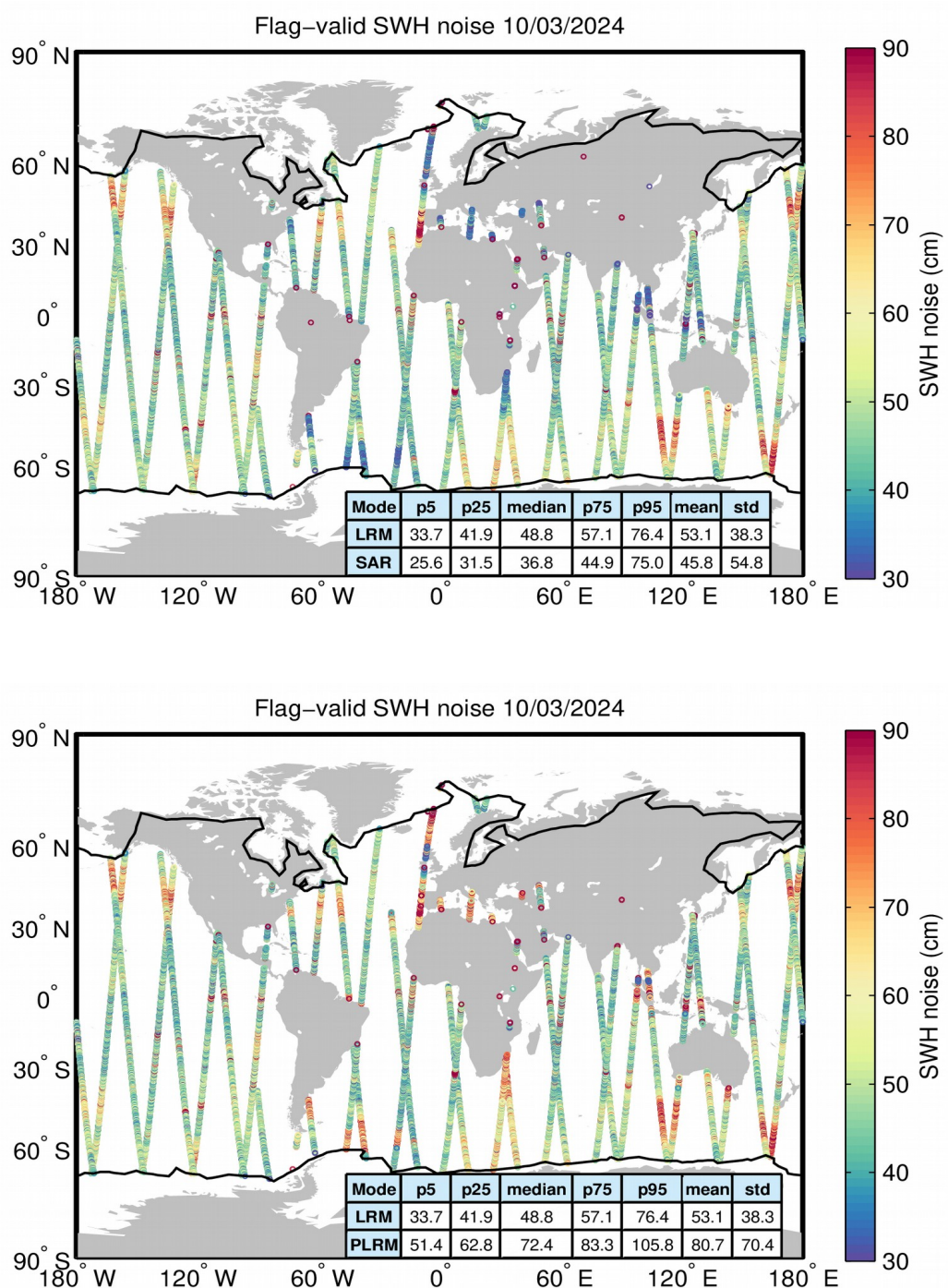
Figure 18. Geographical distribution of flag-valid 20-Hz SWH measurement noise over oceans and lakes for LRM/SAR (top) and LRM/PLRM (bottom) and for 10/03/2024. The statistical values shown in the table refer to the SWH noise and are calculated separately for LRM and SAR/PLRM regions. Measurements taken over polar polygons have been
