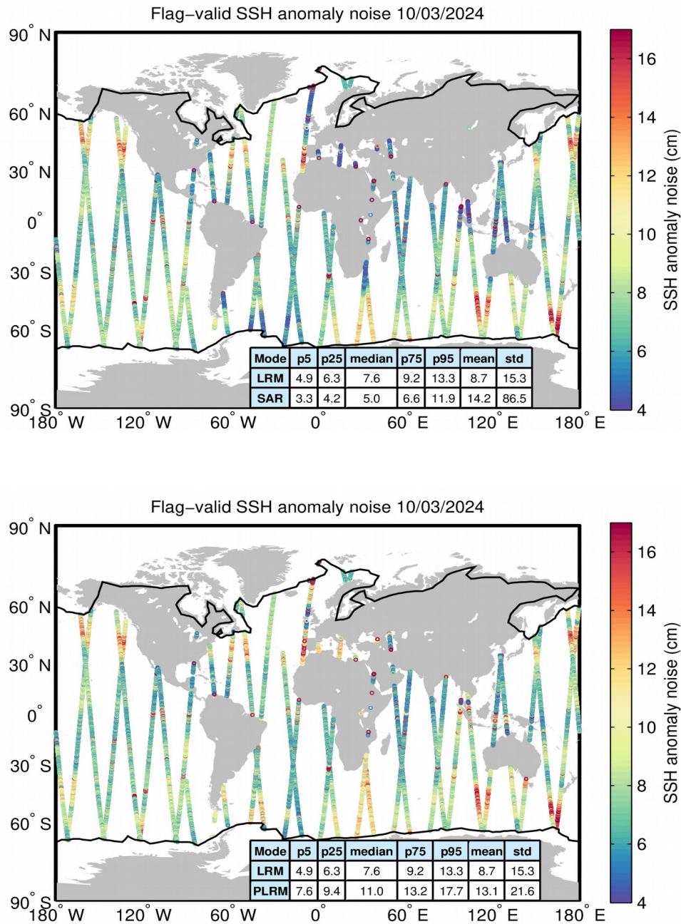
Figure 8. Geographical distribution of flag-valid 20-Hz SSH anomaly measurement noise over oceans and lakes for LRM/SAR (top) and LRM/PLRM (bottom) and for 10/03/2024. The statistical values shown in the tables refer to the SSH anomaly noise and are calculated separately for LRM and SAR/PLRM regions. Measurements taken over polar polygons have been excluded from the computation of the statistical values. The black lines mark the outer limit of the Arctic and Antarctic polar polygons.
