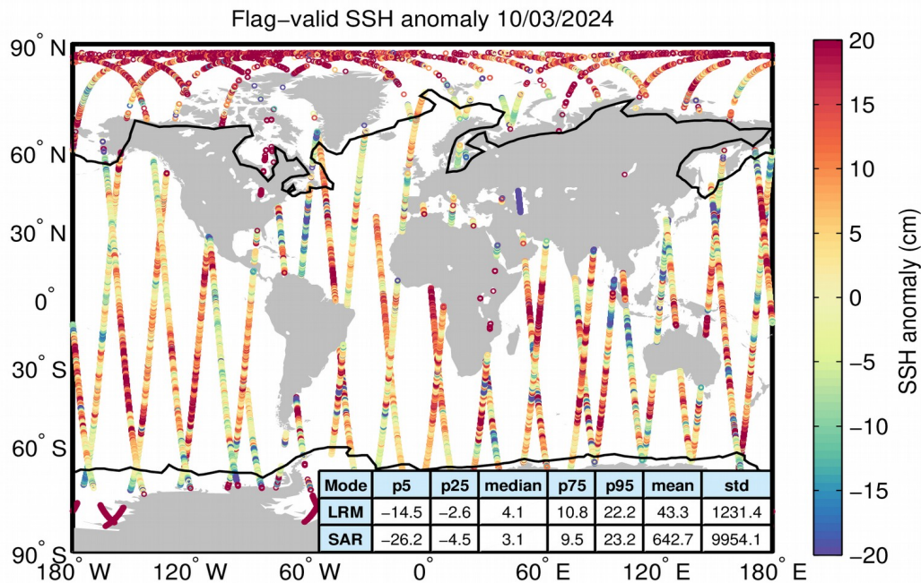
Figure 5. Geographical distribution of flag-valid 1-Hz SSH anomaly data over oceans and lakes for 10/03/2024. The statistical values shown in the table refer to the SSH anomaly in cm and are calculated separately for LRM and SAR regions. Measurements taken over polar polygons have been excluded from the computation of the statistical values. The black lines mark the outer limit of the Arctic and Antarctic polar polygons.
