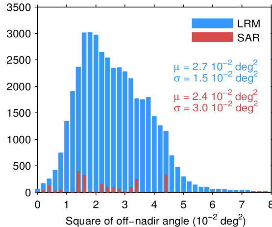
Figure 39. Histogram of flag-valid mispointing over oceans and lakes for LRM (blue) and SAR (red) for 10/03/2024. Only positive values have been considered. The mean ( \mu ) and standard deviation ( \sigma ) are also shown. Note that values larger than 8 \cdot 10^{-2} \text{ deg}^2 are excluded from the histogram for the sake of readability but not from the computation of \mu and \sigma .
