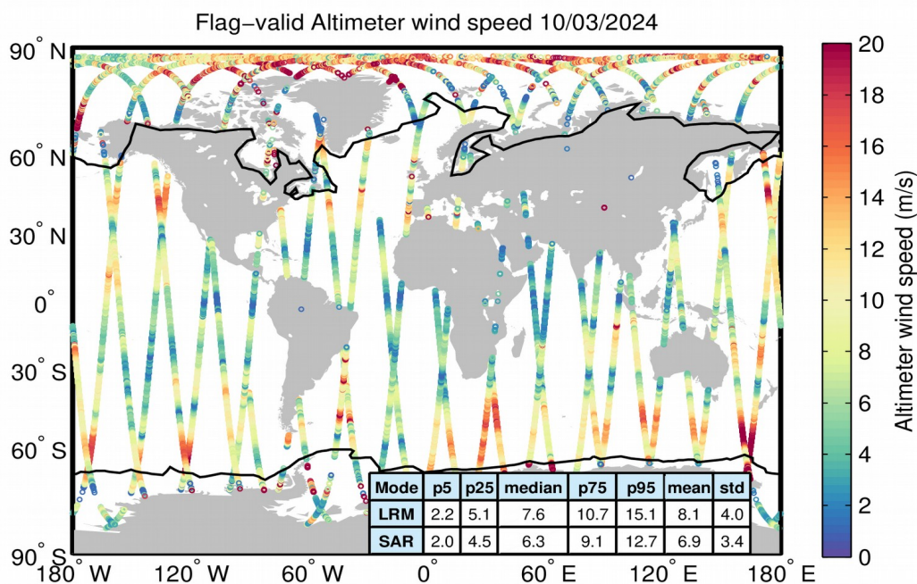
Figure 31. Geographical distribution of flag-valid wind data over oceans and lakes for 10/03/2024. The statistical values shown in the table refer to the wind in m/s and are calculated separately for LRM and SAR regions. Measurements taken over polar polygons have been excluded from the computation of the statistical values. The black lines mark the outer limit of the Arctic and Antarctic polar polygons.
