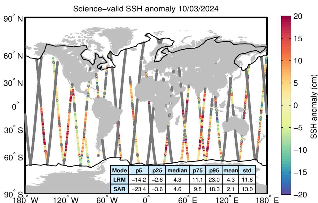
Figure 10. Geographical distribution of science-valid SSH anomaly data over oceans and lakes for 10/03/2024. The statistical values shown in the table refer to the SSH anomaly in cm and are calculated separately for LRM and SAR regions. The black lines mark the
