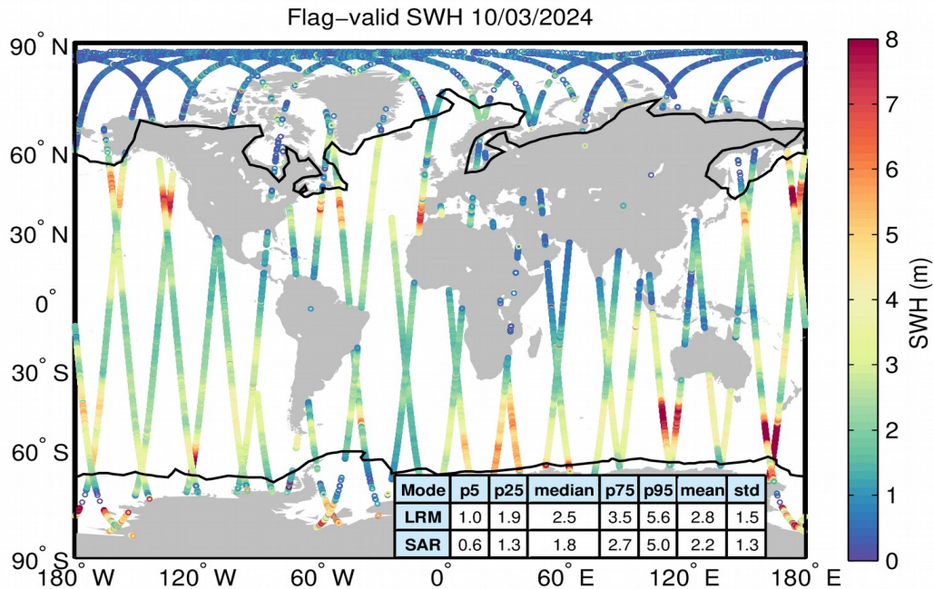
Figure 15. Geographical distribution of flag-valid SWH data over oceans and lakes for 10/03/2024. The statistical values shown in the table refer to the SWH in m and are calculated separately for LRM and SAR regions. Measurements taken over polar polygons have been excluded from the computation of the statistical values. The black lines mark the outer limit of the Arctic and Antarctic polar polygons.
