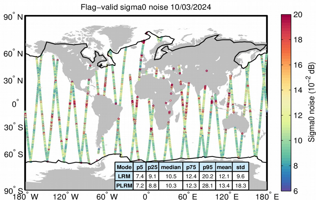
Figure 26. Geographical distribution of flag-valid 20-Hz sigma0 measurement noise over oceans and lakes for LRM/SAR (top) and LRM/PLRM (bottom) and for 10/03/2024. The statistical values shown in the table refer to the sigma0 noise and are calculated separately for LRM and SAR/PLRM regions. Measurements taken over polar polygons have been excluded from the computation of the statistical values. The black lines mark the outer limit of the Arctic and Antarctic polar polygons.
