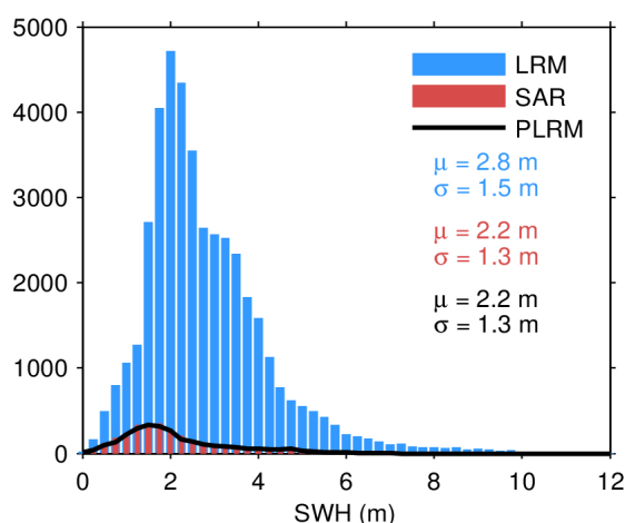
Figure 20. Histogram of science-valid SWH over oceans and lakes for LRM (blue), SAR (red), and PLRM (black) for 10/03/2024. The mean ( \mu ) and standard deviation ( \sigma ) are also
