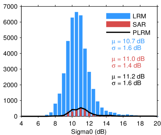
Figure 28. Histogram of science-valid sigma0 over oceans and lakes for LRM (blue), SAR (red), and PLRM (black) for 10/03/2024. The mean ( \mu ) and standard deviation ( \sigma ) are also shown. Note that values outside [4 20] dB are excluded from the histogram for the sake of readability but not from the computation of \mu and \sigma .
