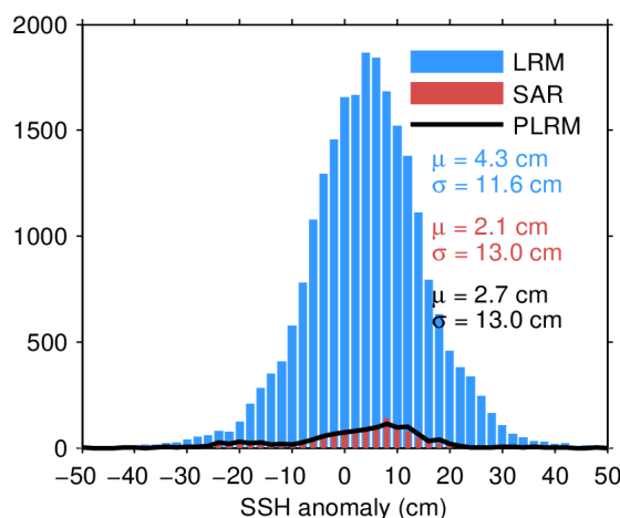
Figure 11. Histogram of science-valid SSH anomaly over oceans and lakes for LRM (blue), SAR (red), and PLRM (black) for 10/03/2024. The mean ( \mu ) and standard deviation ( \sigma ) are also shown. Note that values outside [-50\ 50] cm are excluded from the histogram for the sake of readability but not from the computation of \mu and \sigma .
