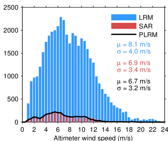
Figure 33. Histogram of flag-valid wind over oceans and lakes for LRM (blue), SAR (red), and PLRM (black) for 10/03/2024. The mean ( \mu ) and standard deviation ( \sigma ) are also shown. Note that values larger than 24 m/s are excluded from the histogram for the sake of readability but not from the computation of \mu and \sigma .
