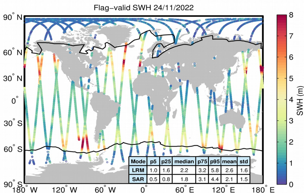
Figure 15. Geographical distribution of flag-valid SWH data over oceans and lakes for 24/11/2022. The statistical values shown in the table refer to the SWH in m and are calculated separately for LRM and SAR regions. Measurements taken over polar polygons have been excluded from the computation of the statistical values. The black lines mark the outer limit of the Arctic and Antarctic polar polygons.
