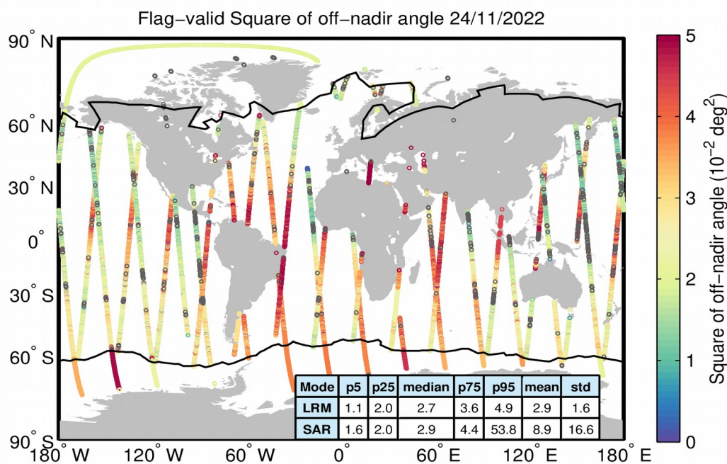
Figure 37. Geographical distribution of flag-valid mispointing data over oceans and lakes for 24/11/2022. The statistical values shown in the table refer to the mispointing in 10^{-2} \text{ deg}^2 and are calculated separately for LRM and SAR regions. Measurements taken over polar polygons have been excluded from the computation of the statistical values. The black lines mark the outer limit of the Arctic and Antarctic polar polygons. Gray circles denote negative values.
