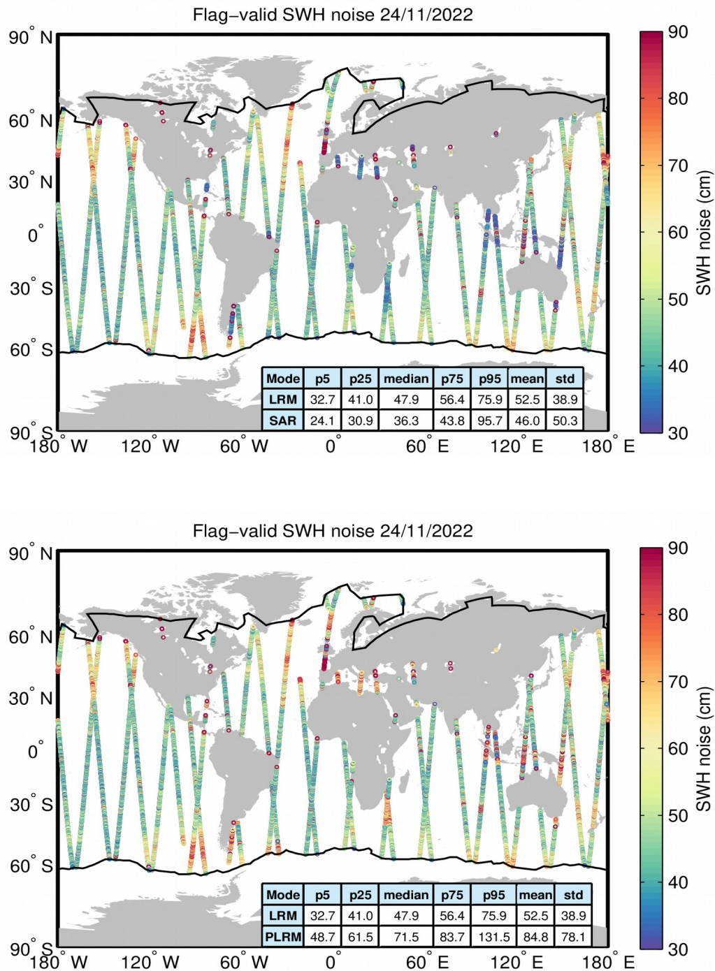
Figure 18. Geographical distribution of flag-valid 20-Hz SWH measurement noise over oceans and lakes for LRM/SAR (top) and LRM/PLRM (bottom) and for 24/11/2022. The statistical values shown in the table refer to the SWH noise and are calculated separately for LRM and SAR/PLRM regions. Measurements taken over polar polygons have been
