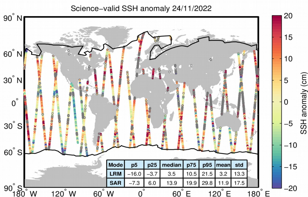
Figure 10. Geographical distribution of science-valid SSH anomaly data over oceans and lakes for 24/11/2022. The statistical values shown in the table refer to the SSH anomaly in cm and are calculated separately for LRM and SAR regions. The black lines mark the
