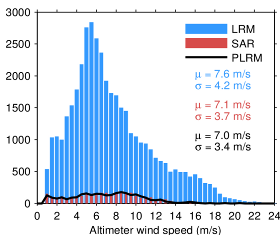
Figure 33. Histogram of flag-valid wind over oceans and lakes for LRM (blue), SAR (red), and PLRM (black) for 24/11/2022. The mean ( \mu ) and standard deviation ( \sigma ) are also shown. Note that values larger than 24 m/s are excluded from the histogram for the sake of readability but not from the computation of \mu and \sigma .
