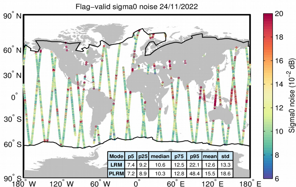
Figure 26. Geographical distribution of flag-valid 20-Hz sigma0 measurement noise over oceans and lakes for LRM/SAR (top) and LRM/PLRM (bottom) and for 24/11/2022. The statistical values shown in the table refer to the sigma0 noise and are calculated separately for LRM and SAR/PLRM regions. Measurements taken over polar polygons have been excluded from the computation of the statistical values. The black lines mark the outer limit of the Arctic and Antarctic polar polygons.
