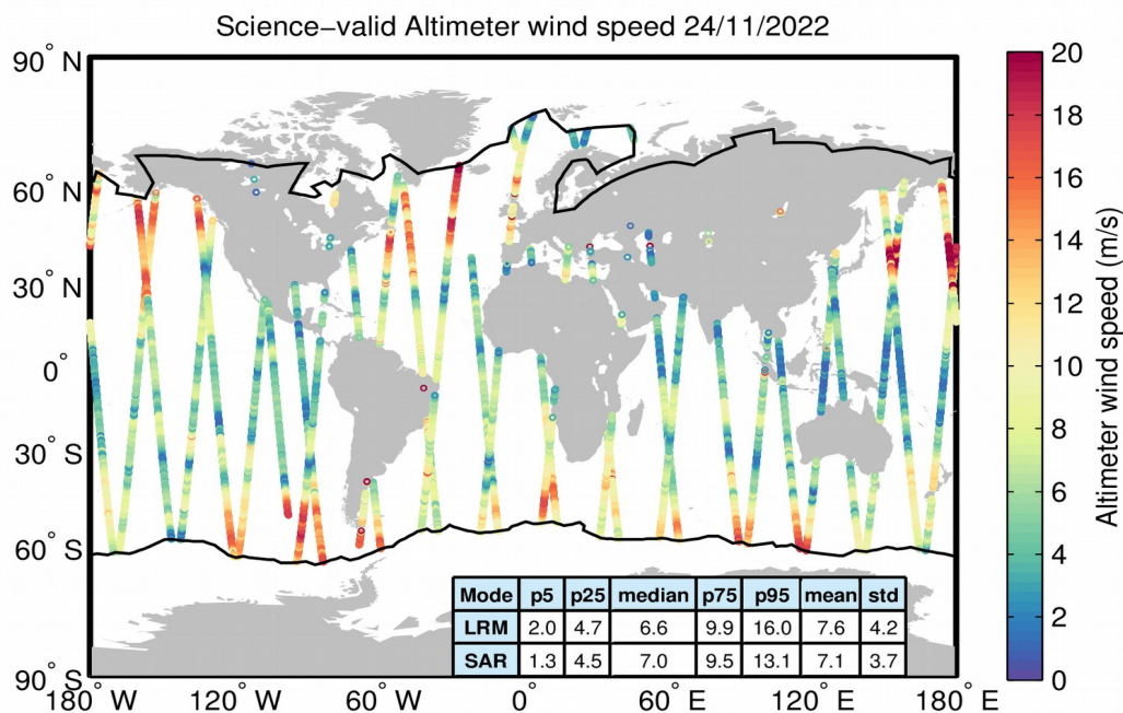
Figure 34. Geographical distribution of science-valid wind data over oceans and lakes for 24/11/2022. The statistical values shown in the table refer to the wind in m/s and are calculated separately for LRM and SAR regions. The black lines mark the outer limit of the Arctic and Antarctic polar polygons. Gray circles denote records that have been rejected based on the editing criteria described in Table 5.
