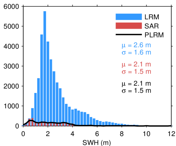
Figure 17. Histogram of flag-valid SWH over oceans and lakes for LRM (blue), SAR (red), and PLRM (black) for 24/11/2022. The mean ( \mu ) and standard deviation ( \sigma ) are also shown. Note that values larger than 12 m are excluded from the histogram for the sake of readability but not from the computation of \mu and \sigma .
