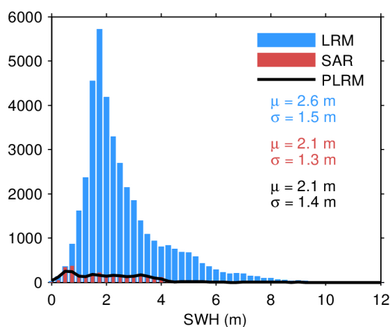
Figure 20. Histogram of science-valid SWH over oceans and lakes for LRM (blue), SAR (red), and PLRM (black) for 24/11/2022. The mean ( \mu ) and standard deviation ( \sigma ) are also
