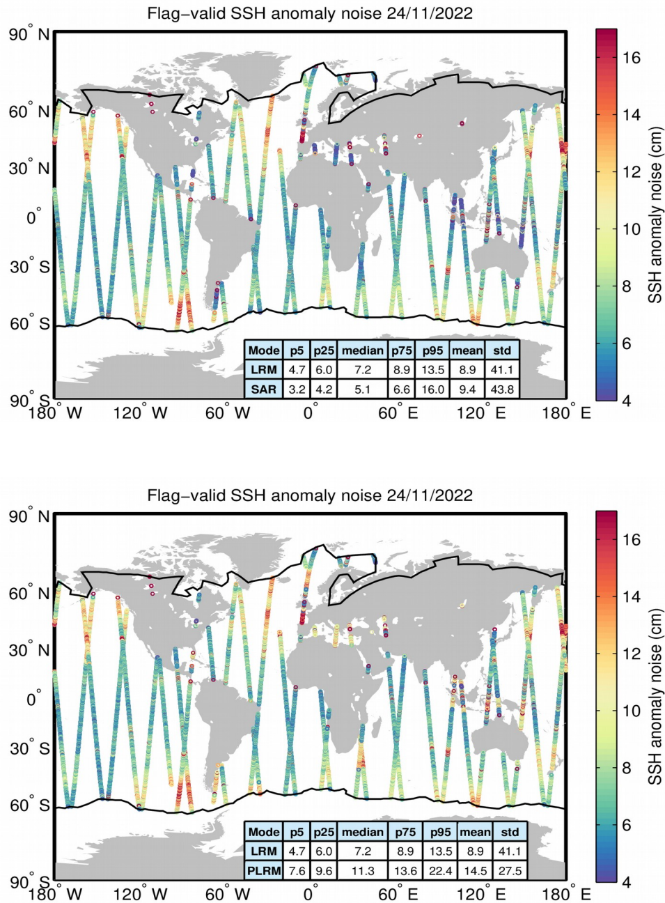
Figure 8. Geographical distribution of flag-valid 20-Hz SSH anomaly measurement noise over oceans and lakes for LRM/SAR (top) and LRM/PLRM (bottom) and for 24/11/2022. The statistical values shown in the tables refer to the SSH anomaly noise and are calculated separately for LRM and SAR/PLRM regions. Measurements taken over polar polygons have been excluded from the computation of the statistical values. The black lines mark the outer limit of the Arctic and Antarctic polar polygons.
