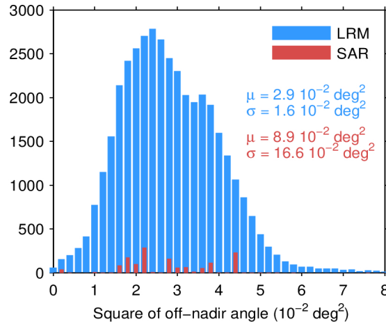
Figure 39. Histogram of flag-valid mispointing over oceans and lakes for LRM (blue) and SAR (red) for 24/11/2022. Only positive values have been considered. The mean ( \mu ) and standard deviation ( \sigma ) are also shown. Note that values larger than 8 \cdot 10^{-2} \text{ deg}^2 are excluded from the histogram for the sake of readability but not from the computation of \mu and \sigma .
