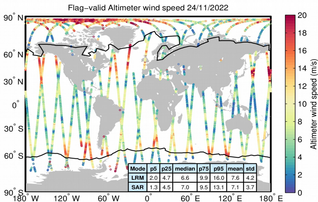
Figure 31. Geographical distribution of flag-valid wind data over oceans and lakes for 24/11/2022. The statistical values shown in the table refer to the wind in m/s and are calculated separately for LRM and SAR regions. Measurements taken over polar polygons have been excluded from the computation of the statistical values. The black lines mark the outer limit of the Arctic and Antarctic polar polygons.
