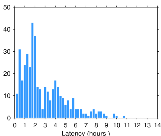
Figure 2. Histogram of the data latency for 24/11/2022. The y-axis denotes the number of files that are made available with a delay of x-hours with respect to the mean time of the records stored in the file.
