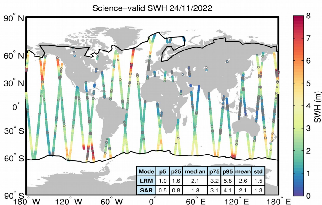
Figure 19. Geographical distribution of science-valid SWH data over oceans and lakes for 24/11/2022. The statistical values shown in the table refer to the SWH in m and are calculated separately for LRM and SAR regions. The black lines mark the outer limit of the Arctic and Antarctic polar polygons. Gray circles denote records that have been rejected based on the editing criteria described in Table 3.
