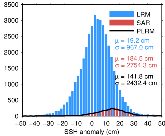
Figure 7. Histogram of flag-valid SSH anomaly over oceans and lakes for LRM (blue), SAR (red), and PLRM (black) for 24/11/2022. The mean ( \mu ) and standard deviation ( \sigma ) are also shown. Note that values outside [-50 50] cm are excluded from the histogram for the sake of readability but not from the computation of \mu and \sigma .
