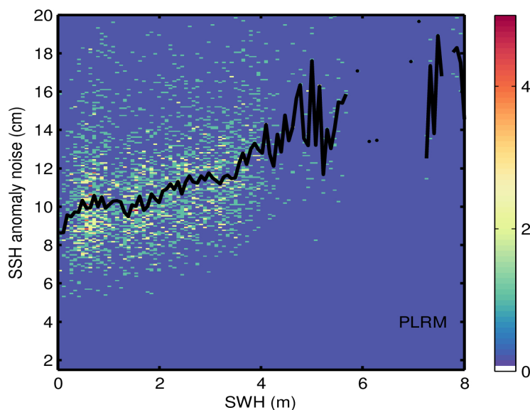
Figure 9. 2D histogram showing flag-valid SSH anomaly noise as a function of SWH for LRM (top), SAR (middle), and PLRM (bottom) for 24/11/2022. The black line denotes the median SSH anomaly noise as a function of SWH.
