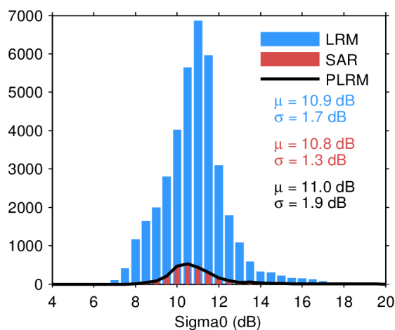
Figure 28. Histogram of science-valid sigma0 over oceans and lakes for LRM (blue), SAR (red), and PLRM (black) for 24/11/2022. The mean ( \mu ) and standard deviation ( \sigma ) are also shown. Note that values outside [4 20] dB are excluded from the histogram for the sake of readability but not from the computation of \mu and \sigma .
