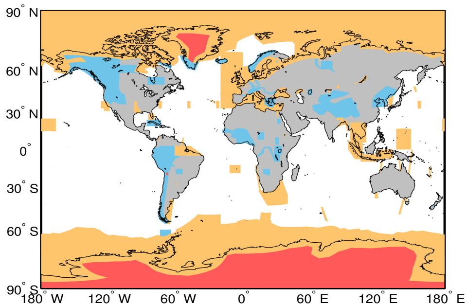
Figure A1. Extent of the regions defining the geographical mode mask for 24/11/2022. The regions where SAR, and SARIn are operated are denoted by the orange and blue polygons, respectively. LRM is operated over areas of the continental ice sheets (red polygons) and over oceans and land not covered by other modes.
