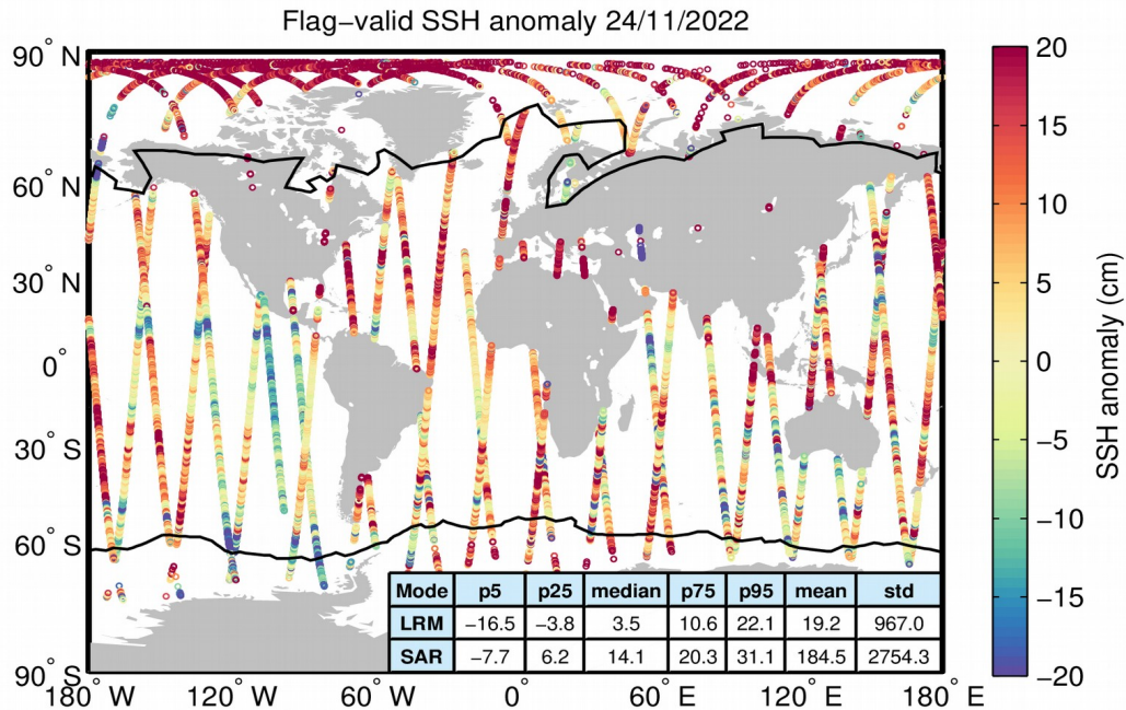
Figure 5. Geographical distribution of flag-valid 1-Hz SSH anomaly data over oceans and lakes for 24/11/2022. The statistical values shown in the table refer to the SSH anomaly in cm and are calculated separately for LRM and SAR regions. Measurements taken over polar polygons have been excluded from the computation of the statistical values. The black lines mark the outer limit of the Arctic and Antarctic polar polygons.
