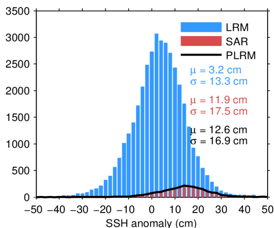
Figure 11. Histogram of science-valid SSH anomaly over oceans and lakes for LRM (blue), SAR (red), and PLRM (black) for 24/11/2022. The mean ( \mu ) and standard deviation ( \sigma ) are also shown. Note that values outside [-50\ 50] cm are excluded from the histogram for the sake of readability but not from the computation of \mu and \sigma .
