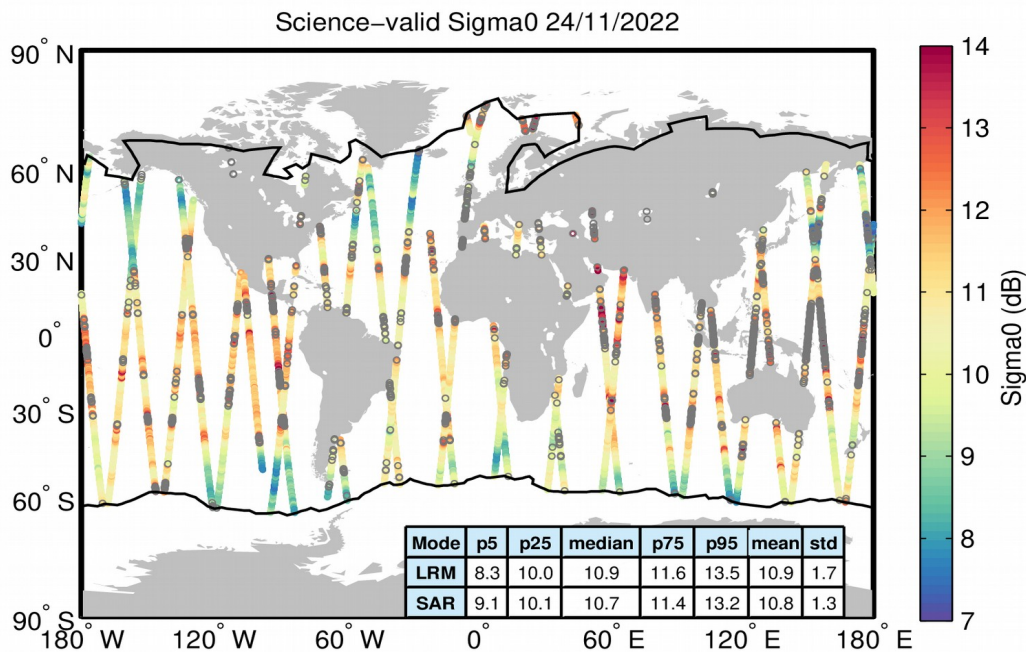
Figure 27. Geographical distribution of science-valid sigma0 data over oceans and lakes for 24/11/2022. The statistical values shown in the table refer to the sigma0 in dB and are calculated separately for LRM and SAR regions. The black lines mark the outer limit of the Arctic and Antarctic polar polygons. Gray circles denote records that have been rejected based on the editing criteria described in Table 4.
