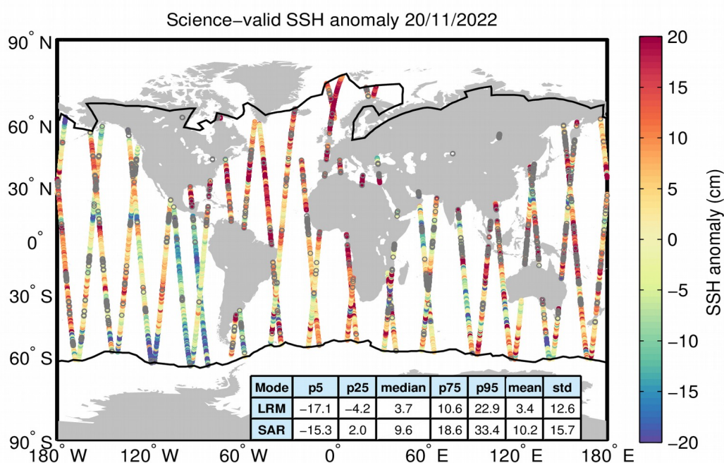
Figure 10. Geographical distribution of science-valid SSH anomaly data over oceans and lakes for 20/11/2022. The statistical values shown in the table refer to the SSH anomaly in cm and are calculated separately for LRM and SAR regions. The black lines mark the
