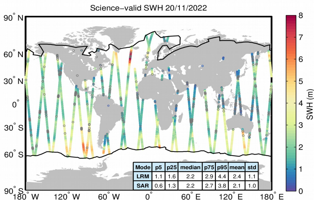
Figure 19. Geographical distribution of science-valid SWH data over oceans and lakes for 20/11/2022. The statistical values shown in the table refer to the SWH in m and are calculated separately for LRM and SAR regions. The black lines mark the outer limit of the Arctic and Antarctic polar polygons. Gray circles denote records that have been rejected based on the editing criteria described in Table 3.
