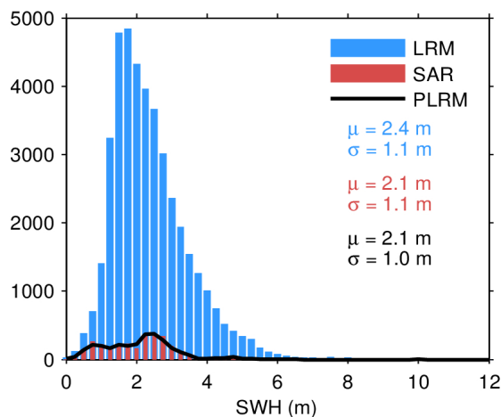
Figure 17. Histogram of flag-valid SWH over oceans and lakes for LRM (blue), SAR (red), and PLRM (black) for 20/11/2022. The mean ( \mu ) and standard deviation ( \sigma ) are also shown. Note that values larger than 12 m are excluded from the histogram for the sake of readability but not from the computation of \mu and \sigma .
