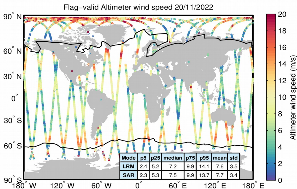
Figure 31. Geographical distribution of flag-valid wind data over oceans and lakes for 20/11/2022. The statistical values shown in the table refer to the wind in m/s and are calculated separately for LRM and SAR regions. Measurements taken over polar polygons have been excluded from the computation of the statistical values. The black lines mark the outer limit of the Arctic and Antarctic polar polygons.
