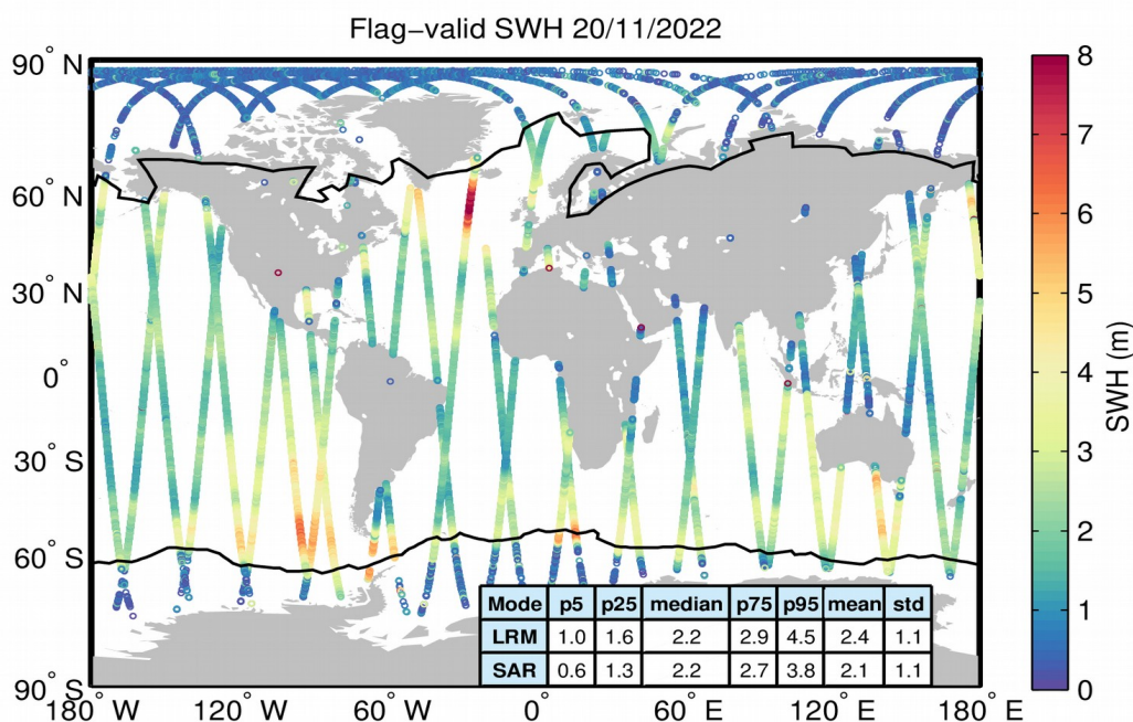
Figure 15. Geographical distribution of flag-valid SWH data over oceans and lakes for 20/11/2022. The statistical values shown in the table refer to the SWH in m and are calculated separately for LRM and SAR regions. Measurements taken over polar polygons have been excluded from the computation of the statistical values. The black lines mark the outer limit of the Arctic and Antarctic polar polygons.
