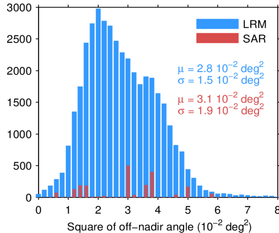
Figure 39. Histogram of flag-valid mispointing over oceans and lakes for LRM (blue) and SAR (red) for 20/11/2022. Only positive values have been considered. The mean ( \mu ) and standard deviation ( \sigma ) are also shown. Note that values larger than 8 \cdot 10^{-2} \text{ deg}^2 are excluded from the histogram for the sake of readability but not from the computation of \mu and \sigma .
