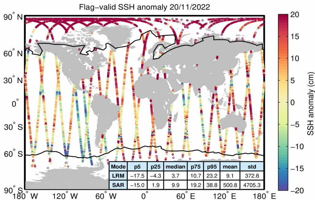
Figure 5. Geographical distribution of flag-valid 1-Hz SSH anomaly data over oceans and lakes for 20/11/2022. The statistical values shown in the table refer to the SSH anomaly in cm and are calculated separately for LRM and SAR regions. Measurements taken over polar polygons have been excluded from the computation of the statistical values. The black lines mark the outer limit of the Arctic and Antarctic polar polygons.
