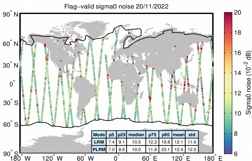
Figure 26. Geographical distribution of flag-valid 20-Hz sigma0 measurement noise over oceans and lakes for LRM/SAR (top) and LRM/PLRM (bottom) and for 20/11/2022. The statistical values shown in the table refer to the sigma0 noise and are calculated separately for LRM and SAR/PLRM regions. Measurements taken over polar polygons have been excluded from the computation of the statistical values. The black lines mark the outer limit of the Arctic and Antarctic polar polygons.
