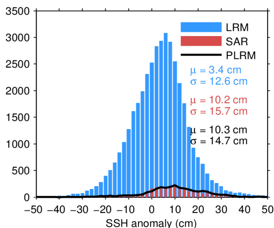
Figure 11. Histogram of science-valid SSH anomaly over oceans and lakes for LRM (blue), SAR (red), and PLRM (black) for 20/11/2022. The mean ( \mu ) and standard deviation ( \sigma ) are also shown. Note that values outside [-50, 50] cm are excluded from the histogram for the sake of readability but not from the computation of \mu and \sigma .
