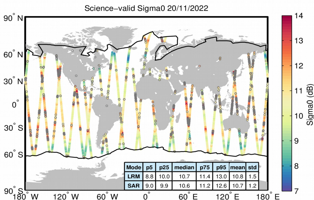
Figure 27. Geographical distribution of science-valid sigma0 data over oceans and lakes for 20/11/2022. The statistical values shown in the table refer to the sigma0 in dB and are calculated separately for LRM and SAR regions. The black lines mark the outer limit of the Arctic and Antarctic polar polygons. Gray circles denote records that have been rejected based on the editing criteria described in Table 4.
