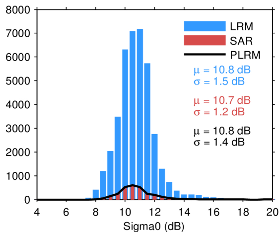
Figure 28. Histogram of science-valid sigma0 over oceans and lakes for LRM (blue), SAR (red), and PLRM (black) for 20/11/2022. The mean ( \mu ) and standard deviation ( \sigma ) are also shown. Note that values outside [4 20] dB are excluded from the histogram for the sake of readability but not from the computation of \mu and \sigma .
