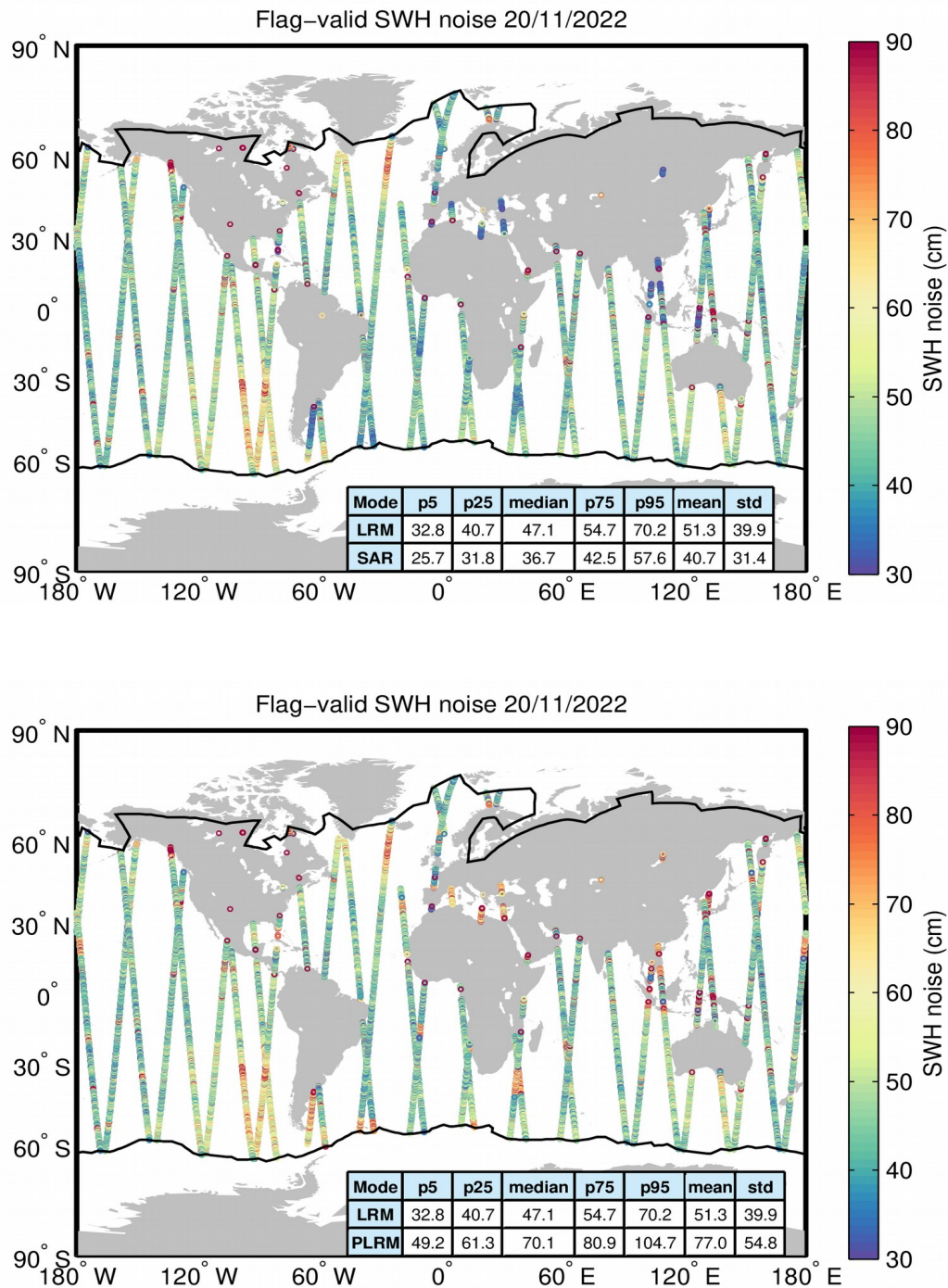
Figure 18. Geographical distribution of flag-valid 20-Hz SWH measurement noise over oceans and lakes for LRM/SAR (top) and LRM/PLRM (bottom) and for 20/11/2022. The statistical values shown in the table refer to the SWH noise and are calculated separately for LRM and SAR/PLRM regions. Measurements taken over polar polygons have been
