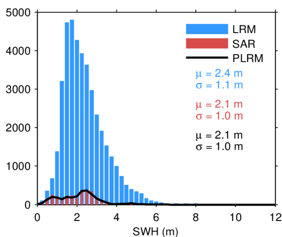
Figure 20. Histogram of science-valid SWH over oceans and lakes for LRM (blue), SAR (red), and PLRM (black) for 20/11/2022. The mean ( \mu ) and standard deviation ( \sigma ) are also
