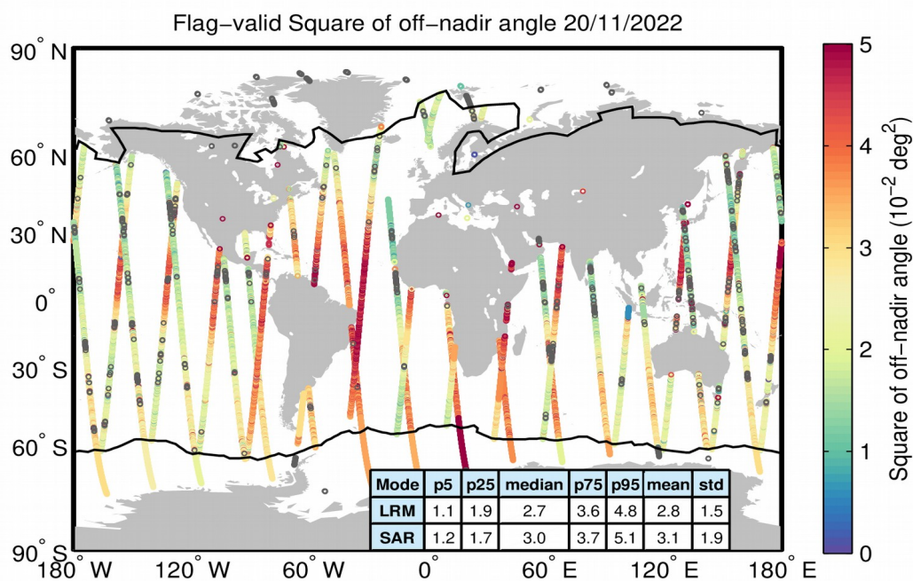
Figure 37. Geographical distribution of flag-valid mispointing data over oceans and lakes for 20/11/2022. The statistical values shown in the table refer to the mispointing in 10^{-2} \text{ deg}^2 and are calculated separately for LRM and SAR regions. Measurements taken over polar polygons have been excluded from the computation of the statistical values. The black lines mark the outer limit of the Arctic and Antarctic polar polygons. Gray circles denote negative values.
