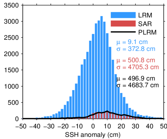
Figure 7. Histogram of flag-valid SSH anomaly over oceans and lakes for LRM (blue), SAR (red), and PLRM (black) for 20/11/2022. The mean ( \mu ) and standard deviation ( \sigma ) are also shown. Note that values outside [-50\ 50] cm are excluded from the histogram for the sake of readability but not from the computation of \mu and \sigma .
