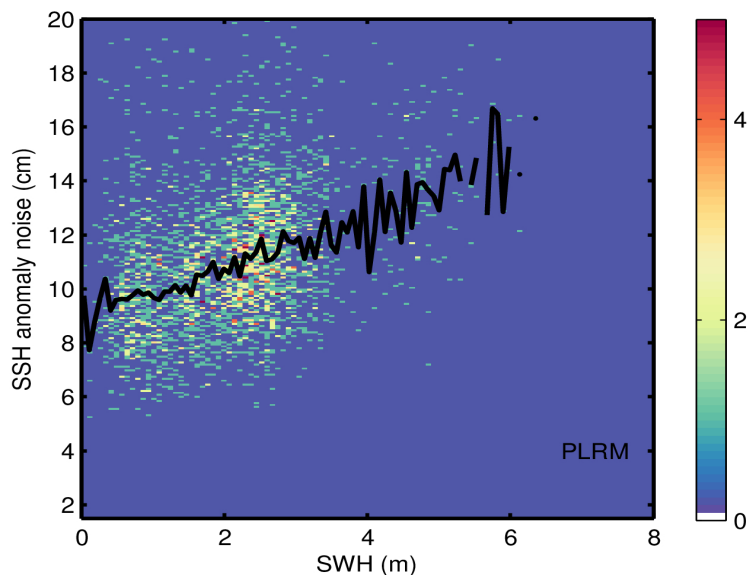
Figure 9. 2D histogram showing flag-valid SSH anomaly noise as a function of SWH for LRM (top), SAR (middle), and PLRM (bottom) for 20/11/2022. The black line denotes the median SSH anomaly noise as a function of SWH.
