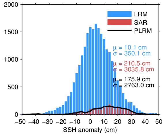
Figure 7. Histogram of flag-valid SSH anomaly over oceans and lakes for LRM (blue), SAR (red), and PLRM (black) for 23/09/2022. The mean ( \mu ) and standard deviation ( \sigma ) are also shown. Note that values outside [-50 50] cm are excluded from the histogram for the sake of readability but not from the computation of \mu and \sigma .
