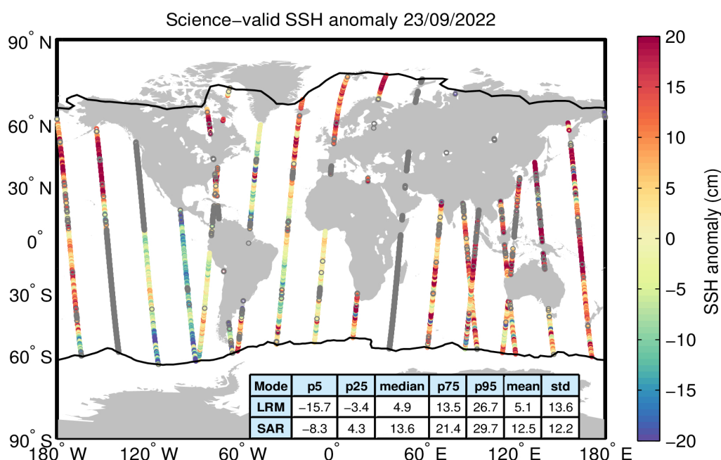
Figure 10. Geographical distribution of science-valid SSH anomaly data over oceans and lakes for 23/09/2022. The statistical values shown in the table refer to the SSH anomaly in cm and are calculated separately for LRM and SAR regions. The black lines mark the
