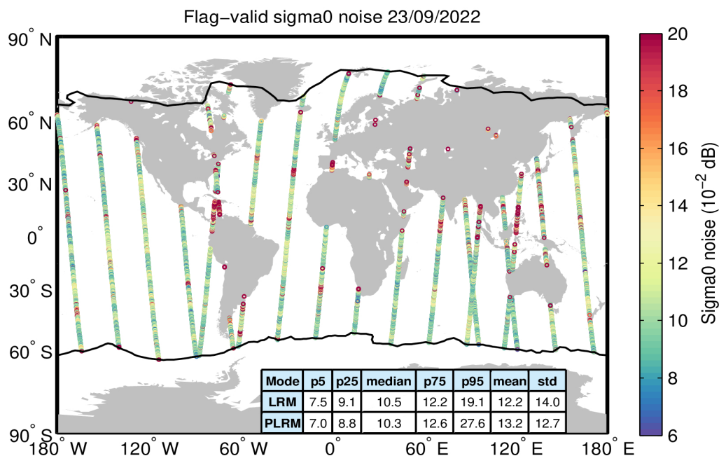
Figure 26. Geographical distribution of flag-valid 20-Hz sigma0 measurement noise over oceans and lakes for LRM/SAR (top) and LRM/PLRM (bottom) and for 23/09/2022. The statistical values shown in the table refer to the sigma0 noise and are calculated separately for LRM and SAR/PLRM regions. Measurements taken over polar polygons have been excluded from the computation of the statistical values. The black lines mark the outer limit of the Arctic and Antarctic polar polygons.
