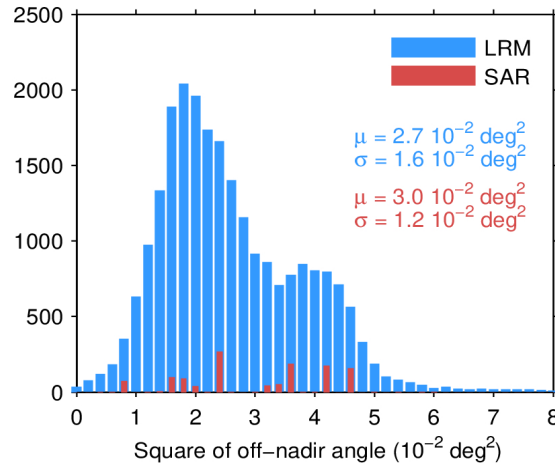
Figure 39. Histogram of flag-valid mispointing over oceans and lakes for LRM (blue) and SAR (red) for 23/09/2022. Only positive values have been considered. The mean ( \mu ) and standard deviation ( \sigma ) are also shown. Note that values larger than 8 \cdot 10^{-2} \text{ deg}^2 are excluded from the histogram for the sake of readability but not from the computation of \mu and \sigma .
