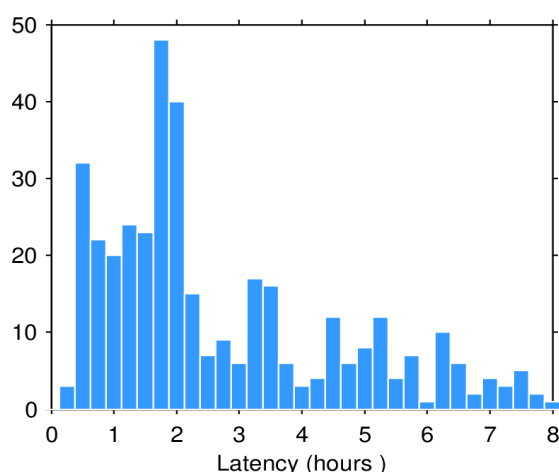
Figure 2. Histogram of the data latency for 23/09/2022. The y-axis denotes the number of files that are made available with a delay of x-hours with respect to the mean time of the records stored in the file.
