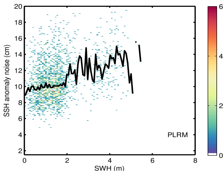
Figure 9. 2D histogram showing flag-valid SSH anomaly noise as a function of SWH for LRM (top), SAR (middle), and PLRM (bottom) for 23/09/2022. The black line denotes the median SSH anomaly noise as a function of SWH.
