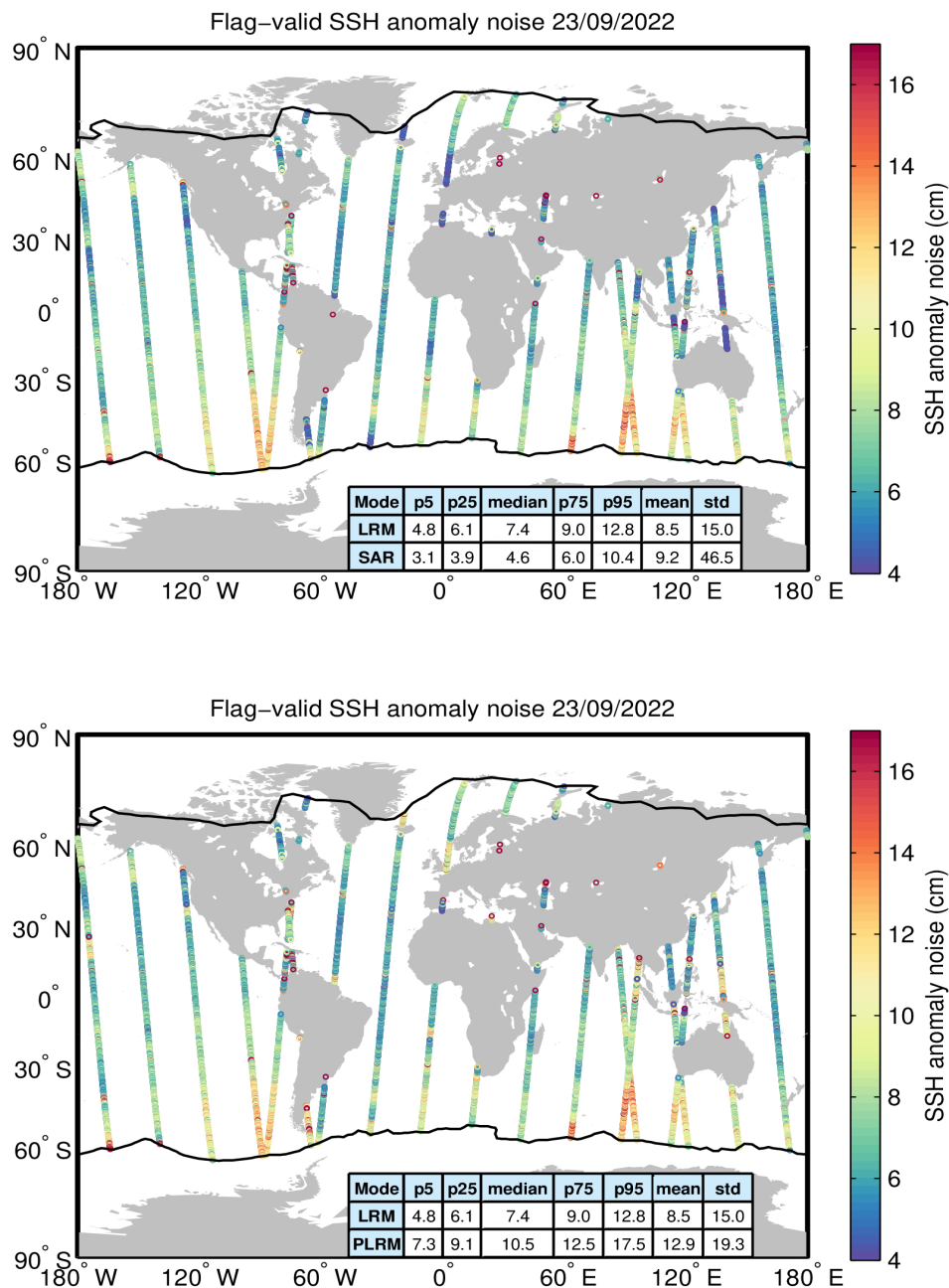
Figure 8. Geographical distribution of flag-valid 20-Hz SSH anomaly measurement noise over oceans and lakes for LRM/SAR (top) and LRM/PLRM (bottom) and for 23/09/2022. The statistical values shown in the tables refer to the SSH anomaly noise and are calculated separately for LRM and SAR/PLRM regions. Measurements taken over polar polygons have been excluded from the computation of the statistical values. The black lines mark the outer limit of the Arctic and Antarctic polar polygons.
