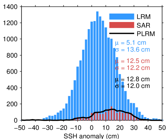
Figure 11. Histogram of science-valid SSH anomaly over oceans and lakes for LRM (blue), SAR (red), and PLRM (black) for 23/09/2022. The mean ( \mu ) and standard deviation ( \sigma ) are also shown. Note that values outside [-50\ 50] cm are excluded from the histogram for the sake of readability but not from the computation of \mu and \sigma .
