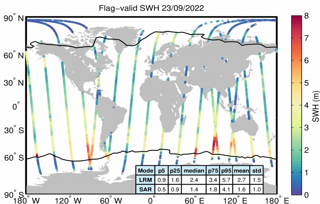
Figure 15. Geographical distribution of flag-valid SWH data over oceans and lakes for 23/09/2022. The statistical values shown in the table refer to the SWH in m and are calculated separately for LRM and SAR regions. Measurements taken over polar polygons have been excluded from the computation of the statistical values. The black lines mark the outer limit of the Arctic and Antarctic polar polygons.
