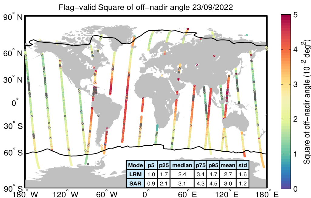
Figure 37. Geographical distribution of flag-valid mispointing data over oceans and lakes for 23/09/2022. The statistical values shown in the table refer to the mispointing in 10^{-2} \text{ deg}^2 and are calculated separately for LRM and SAR regions. Measurements taken over polar polygons have been excluded from the computation of the statistical values. The black lines mark the outer limit of the Arctic and Antarctic polar polygons. Gray circles denote negative values.
