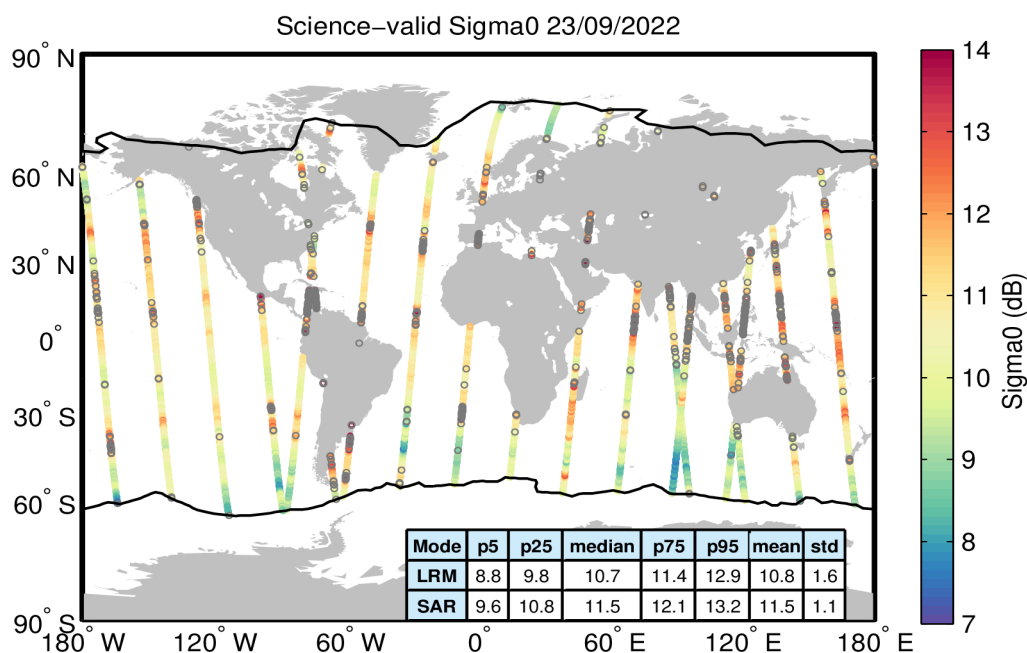
Figure 27. Geographical distribution of science-valid sigma0 data over oceans and lakes for 23/09/2022. The statistical values shown in the table refer to the sigma0 in dB and are calculated separately for LRM and SAR regions. The black lines mark the outer limit of the Arctic and Antarctic polar polygons. Gray circles denote records that have been rejected based on the editing criteria described in Table 4.
