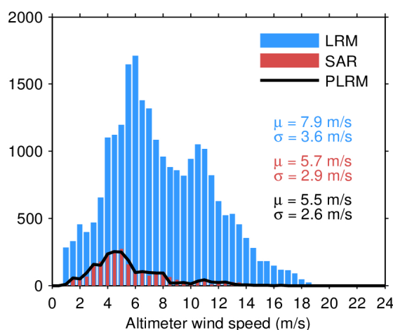
Figure 33. Histogram of flag-valid wind over oceans and lakes for LRM (blue), SAR (red), and PLRM (black) for 23/09/2022. The mean ( \mu ) and standard deviation ( \sigma ) are also shown. Note that values larger than 24 m/s are excluded from the histogram for the sake of readability but not from the computation of \mu and \sigma .
