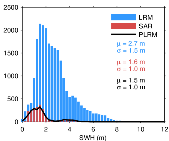
Figure 20. Histogram of science-valid SWH over oceans and lakes for LRM (blue), SAR (red), and PLRM (black) for 23/09/2022. The mean ( \mu ) and standard deviation ( \sigma ) are also
