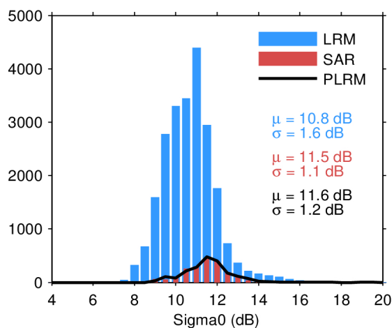
Figure 28. Histogram of science-valid sigma0 over oceans and lakes for LRM (blue), SAR (red), and PLRM (black) for 23/09/2022. The mean ( \mu ) and standard deviation ( \sigma ) are also shown. Note that values outside [4 20] dB are excluded from the histogram for the sake of readability but not from the computation of \mu and \sigma .
