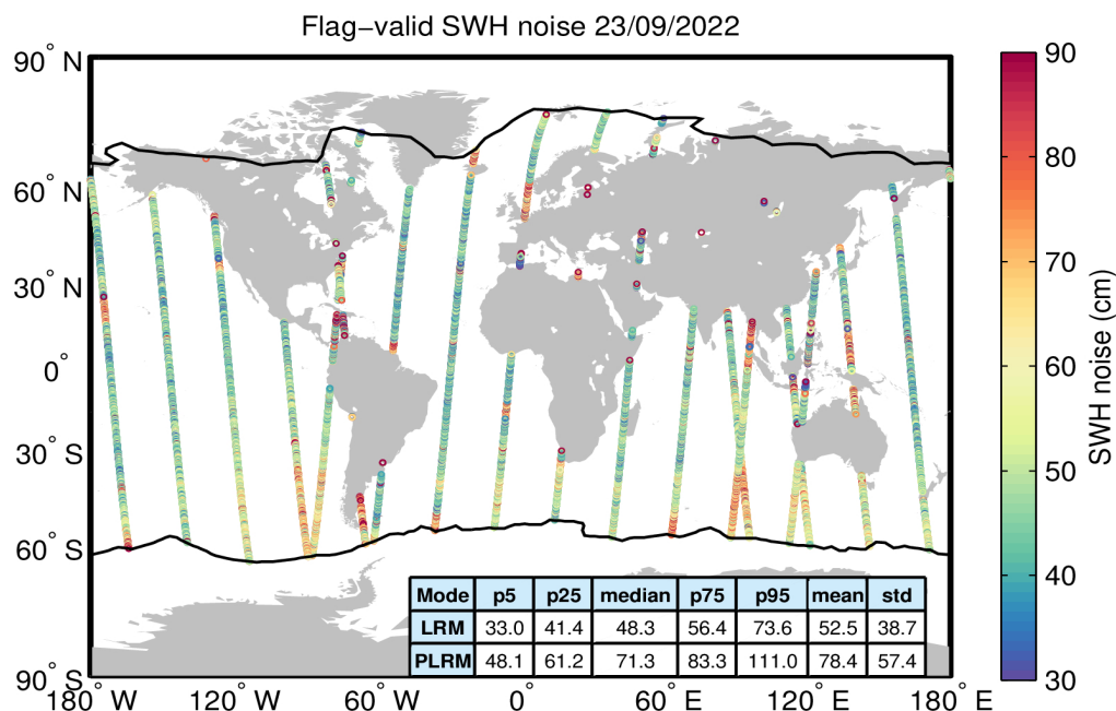
Figure 18. Geographical distribution of flag-valid 20-Hz SWH measurement noise over oceans and lakes for LRM/SAR (top) and LRM/PLRM (bottom) and for 23/09/2022. The statistical values shown in the table refer to the SWH noise and are calculated separately for LRM and SAR/PLRM regions. Measurements taken over polar polygons have been
