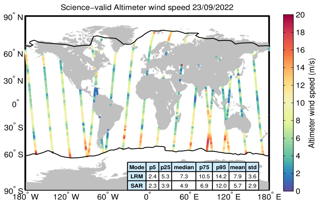
Figure 34. Geographical distribution of science-valid wind data over oceans and lakes for 23/09/2022. The statistical values shown in the table refer to the wind in m/s and are calculated separately for LRM and SAR regions. The black lines mark the outer limit of the Arctic and Antarctic polar polygons. Gray circles denote records that have been rejected based on the editing criteria described in Table 5.
