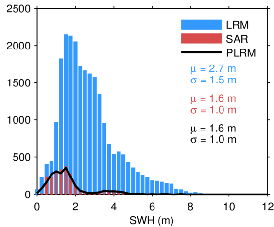
Figure 17. Histogram of flag-valid SWH over oceans and lakes for LRM (blue), SAR (red), and PLRM (black) for 23/09/2022. The mean ( \mu ) and standard deviation ( \sigma ) are also shown. Note that values larger than 12 m are excluded from the histogram for the sake of readability but not from the computation of \mu and \sigma .
