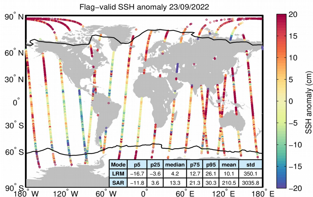
Figure 5. Geographical distribution of flag-valid 1-Hz SSH anomaly data over oceans and lakes for 23/09/2022. The statistical values shown in the table refer to the SSH anomaly in cm and are calculated separately for LRM and SAR regions. Measurements taken over polar polygons have been excluded from the computation of the statistical values. The black lines mark the outer limit of the Arctic and Antarctic polar polygons.
