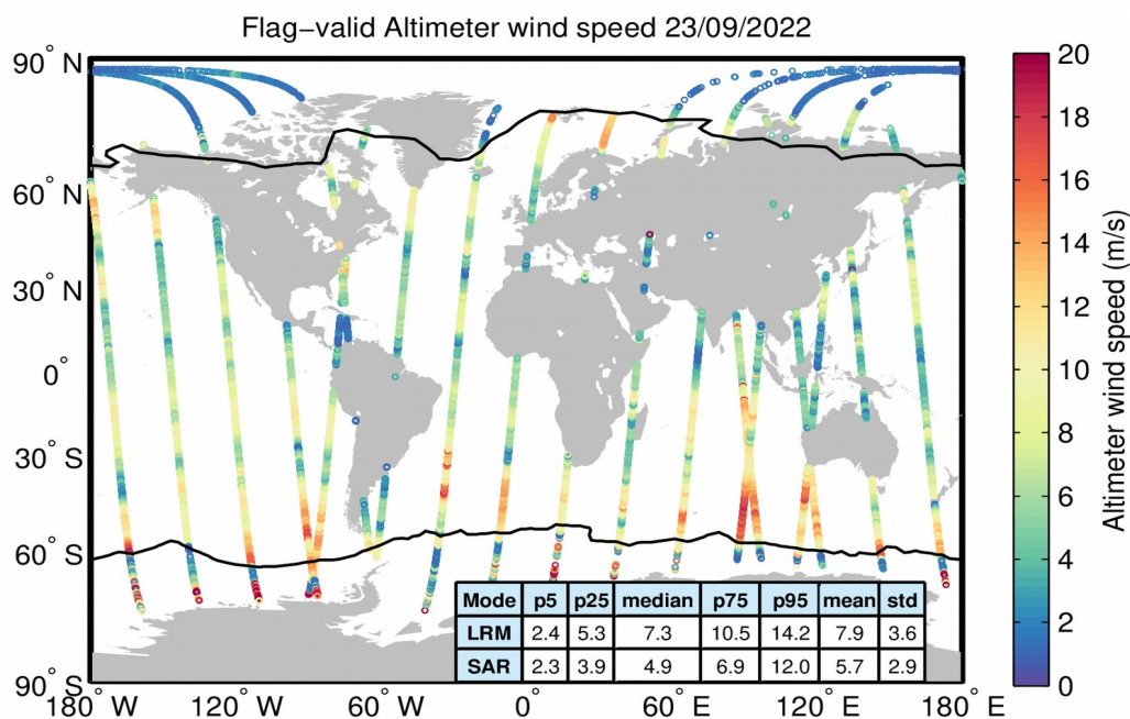
Figure 31. Geographical distribution of flag-valid wind data over oceans and lakes for 23/09/2022. The statistical values shown in the table refer to the wind in m/s and are calculated separately for LRM and SAR regions. Measurements taken over polar polygons have been excluded from the computation of the statistical values. The black lines mark the outer limit of the Arctic and Antarctic polar polygons.
