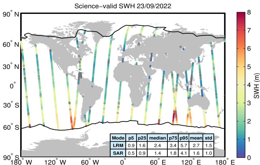
Figure 19. Geographical distribution of science-valid SWH data over oceans and lakes for 23/09/2022. The statistical values shown in the table refer to the SWH in m and are calculated separately for LRM and SAR regions. The black lines mark the outer limit of the Arctic and Antarctic polar polygons. Gray circles denote records that have been rejected based on the editing criteria described in Table 3.
