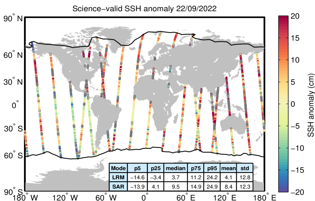
Figure 10. Geographical distribution of science-valid SSH anomaly data over oceans and lakes for 22/09/2022. The statistical values shown in the table refer to the SSH anomaly in cm and are calculated separately for LRM and SAR regions. The black lines mark the
