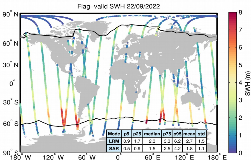
Figure 15. Geographical distribution of flag-valid SWH data over oceans and lakes for 22/09/2022. The statistical values shown in the table refer to the SWH in m and are calculated separately for LRM and SAR regions. Measurements taken over polar polygons have been excluded from the computation of the statistical values. The black lines mark the outer limit of the Arctic and Antarctic polar polygons.
