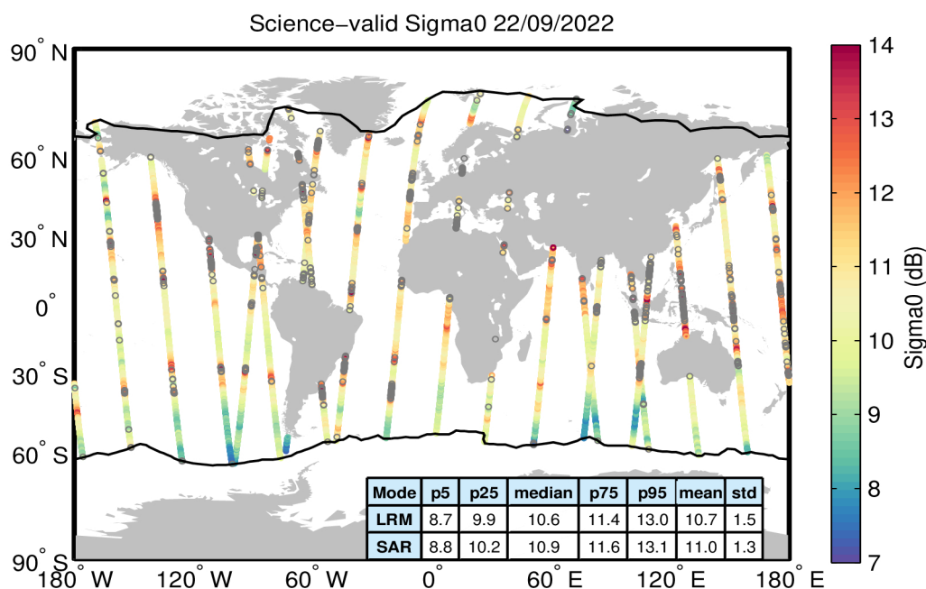
Figure 27. Geographical distribution of science-valid sigma0 data over oceans and lakes for 22/09/2022. The statistical values shown in the table refer to the sigma0 in dB and are calculated separately for LRM and SAR regions. The black lines mark the outer limit of the Arctic and Antarctic polar polygons. Gray circles denote records that have been rejected based on the editing criteria described in Table 4.
