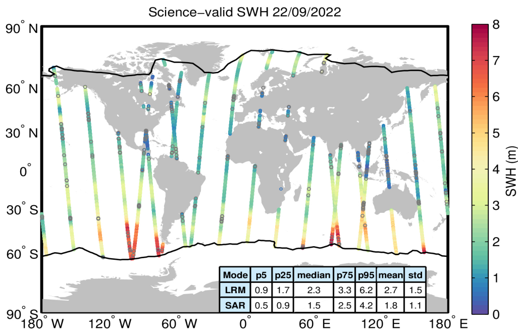
Figure 19. Geographical distribution of science-valid SWH data over oceans and lakes for 22/09/2022. The statistical values shown in the table refer to the SWH in m and are calculated separately for LRM and SAR regions. The black lines mark the outer limit of the Arctic and Antarctic polar polygons. Gray circles denote records that have been rejected based on the editing criteria described in Table 3.
