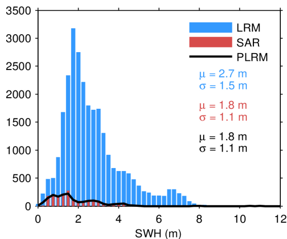
Figure 17. Histogram of flag-valid SWH over oceans and lakes for LRM (blue), SAR (red), and PLRM (black) for 22/09/2022. The mean ( \mu ) and standard deviation ( \sigma ) are also shown. Note that values larger than 12 m are excluded from the histogram for the sake of readability but not from the computation of \mu and \sigma .
