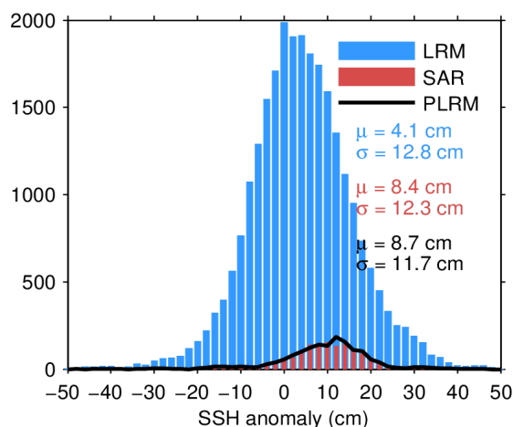
Figure 11. Histogram of science-valid SSH anomaly over oceans and lakes for LRM (blue), SAR (red), and PLRM (black) for 22/09/2022. The mean ( \mu ) and standard deviation ( \sigma ) are also shown. Note that values outside [-50, 50] cm are excluded from the histogram for the sake of readability but not from the computation of \mu and \sigma .
