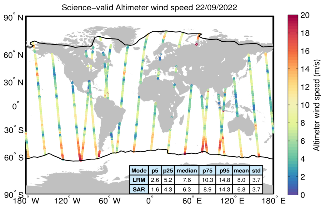
Figure 34. Geographical distribution of science-valid wind data over oceans and lakes for 22/09/2022. The statistical values shown in the table refer to the wind in m/s and are calculated separately for LRM and SAR regions. The black lines mark the outer limit of the Arctic and Antarctic polar polygons. Gray circles denote records that have been rejected based on the editing criteria described in Table 5.
