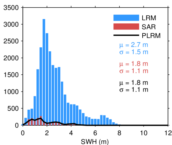
Figure 20. Histogram of science-valid SWH over oceans and lakes for LRM (blue), SAR (red), and PLRM (black) for 22/09/2022. The mean ( \mu ) and standard deviation ( \sigma ) are also
