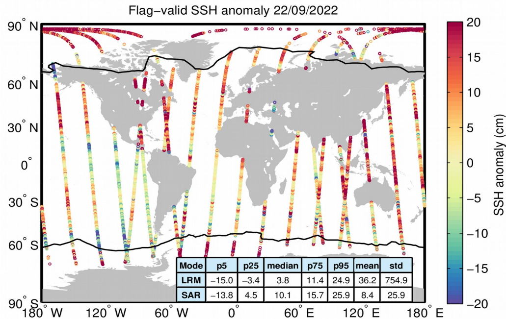
Figure 5. Geographical distribution of flag-valid 1-Hz SSH anomaly data over oceans and lakes for 22/09/2022. The statistical values shown in the table refer to the SSH anomaly in cm and are calculated separately for LRM and SAR regions. Measurements taken over polar polygons have been excluded from the computation of the statistical values. The black lines mark the outer limit of the Arctic and Antarctic polar polygons.
