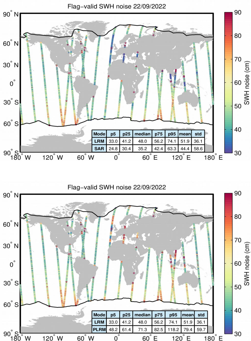
Figure 18. Geographical distribution of flag-valid 20-Hz SWH measurement noise over oceans and lakes for LRM/SAR (top) and LRM/PLRM (bottom) and for 22/09/2022. The statistical values shown in the table refer to the SWH noise and are calculated separately for LRM and SAR/PLRM regions. Measurements taken over polar polygons have been
