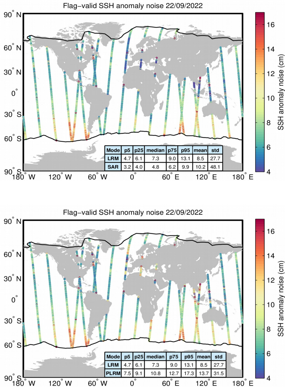
Figure 8. Geographical distribution of flag-valid 20-Hz SSH anomaly measurement noise over oceans and lakes for LRM/SAR (top) and LRM/PLRM (bottom) and for 22/09/2022. The statistical values shown in the tables refer to the SSH anomaly noise and are calculated separately for LRM and SAR/PLRM regions. Measurements taken over polar polygons have been excluded from the computation of the statistical values. The black lines mark the outer limit of the Arctic and Antarctic polar polygons.
