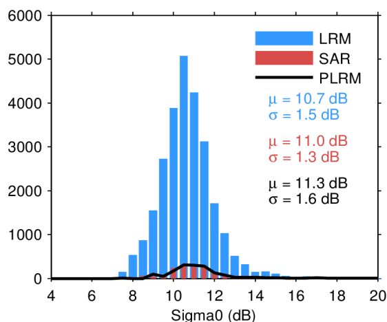
Figure 28. Histogram of science-valid sigma0 over oceans and lakes for LRM (blue), SAR (red), and PLRM (black) for 22/09/2022. The mean ( \mu ) and standard deviation ( \sigma ) are also shown. Note that values outside [4 20] dB are excluded from the histogram for the sake of readability but not from the computation of \mu and \sigma .
