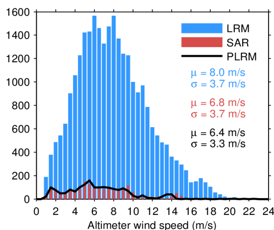
Figure 33. Histogram of flag-valid wind over oceans and lakes for LRM (blue), SAR (red), and PLRM (black) for 22/09/2022. The mean ( \mu ) and standard deviation ( \sigma ) are also shown. Note that values larger than 24 m/s are excluded from the histogram for the sake of readability but not from the computation of \mu and \sigma .
