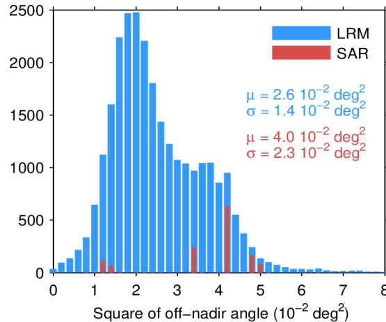
Figure 39. Histogram of flag-valid mispointing over oceans and lakes for LRM (blue) and SAR (red) for 22/09/2022. Only positive values have been considered. The mean ( \mu ) and standard deviation ( \sigma ) are also shown. Note that values larger than 8 \cdot 10^{-2} \text{ deg}^2 are excluded from the histogram for the sake of readability but not from the computation of \mu and \sigma .
