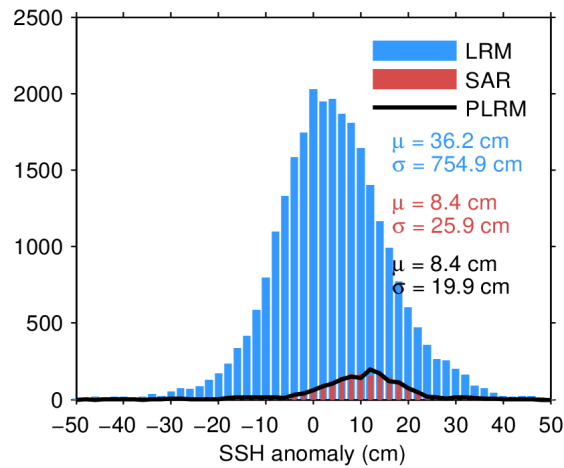
Figure 7. Histogram of flag-valid SSH anomaly over oceans and lakes for LRM (blue), SAR (red), and PLRM (black) for 22/09/2022. The mean ( \mu ) and standard deviation ( \sigma ) are also shown. Note that values outside [-50 50] cm are excluded from the histogram for the sake of readability but not from the computation of \mu and \sigma .
