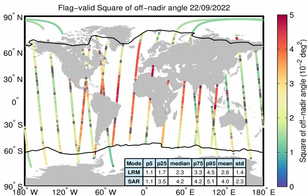
Figure 37. Geographical distribution of flag-valid mispointing data over oceans and lakes for 22/09/2022. The statistical values shown in the table refer to the mispointing in 10^{-2} \text{ deg}^2 and are calculated separately for LRM and SAR regions. Measurements taken over polar polygons have been excluded from the computation of the statistical values. The black lines mark the outer limit of the Arctic and Antarctic polar polygons. Gray circles denote negative values.
