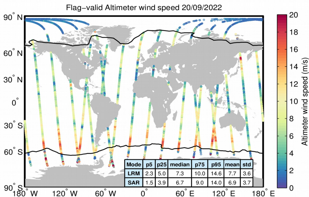
Figure 31. Geographical distribution of flag-valid wind data over oceans and lakes for 20/09/2022. The statistical values shown in the table refer to the wind in m/s and are calculated separately for LRM and SAR regions. Measurements taken over polar polygons have been excluded from the computation of the statistical values. The black lines mark the outer limit of the Arctic and Antarctic polar polygons.
