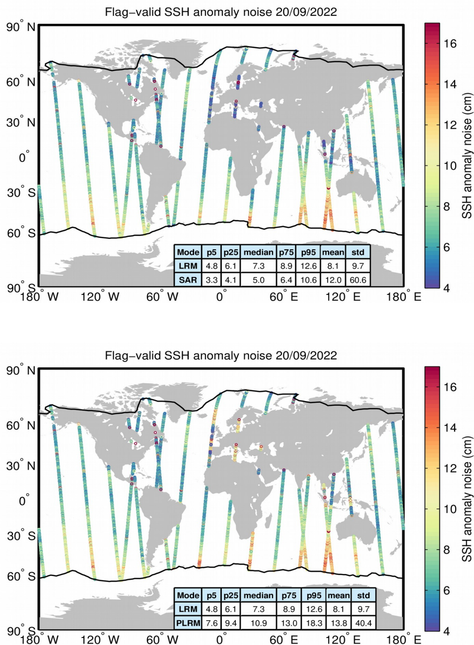
Figure 8. Geographical distribution of flag-valid 20-Hz SSH anomaly measurement noise over oceans and lakes for LRM/SAR (top) and LRM/PLRM (bottom) and for 20/09/2022. The statistical values shown in the tables refer to the SSH anomaly noise and are calculated separately for LRM and SAR/PLRM regions. Measurements taken over polar polygons have been excluded from the computation of the statistical values. The black lines mark the outer limit of the Arctic and Antarctic polar polygons.
