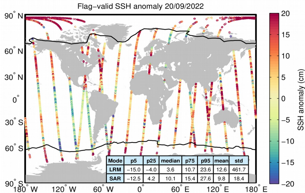
Figure 5. Geographical distribution of flag-valid 1-Hz SSH anomaly data over oceans and lakes for 20/09/2022. The statistical values shown in the table refer to the SSH anomaly in cm and are calculated separately for LRM and SAR regions. Measurements taken over polar polygons have been excluded from the computation of the statistical values. The black lines mark the outer limit of the Arctic and Antarctic polar polygons.
