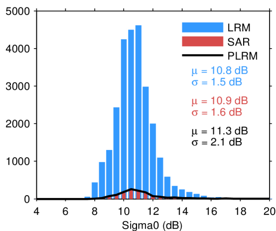
Figure 28. Histogram of science-valid sigma0 over oceans and lakes for LRM (blue), SAR (red), and PLRM (black) for 20/09/2022. The mean ( \mu ) and standard deviation ( \sigma ) are also shown. Note that values outside [4 20] dB are excluded from the histogram for the sake of readability but not from the computation of \mu and \sigma .
