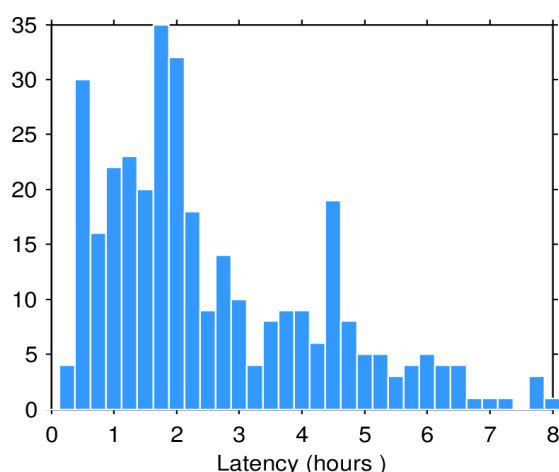
Figure 2. Histogram of the data latency for 20/09/2022. The y-axis denotes the number of files that are made available with a delay of x-hours with respect to the mean time of the records stored in the file.
