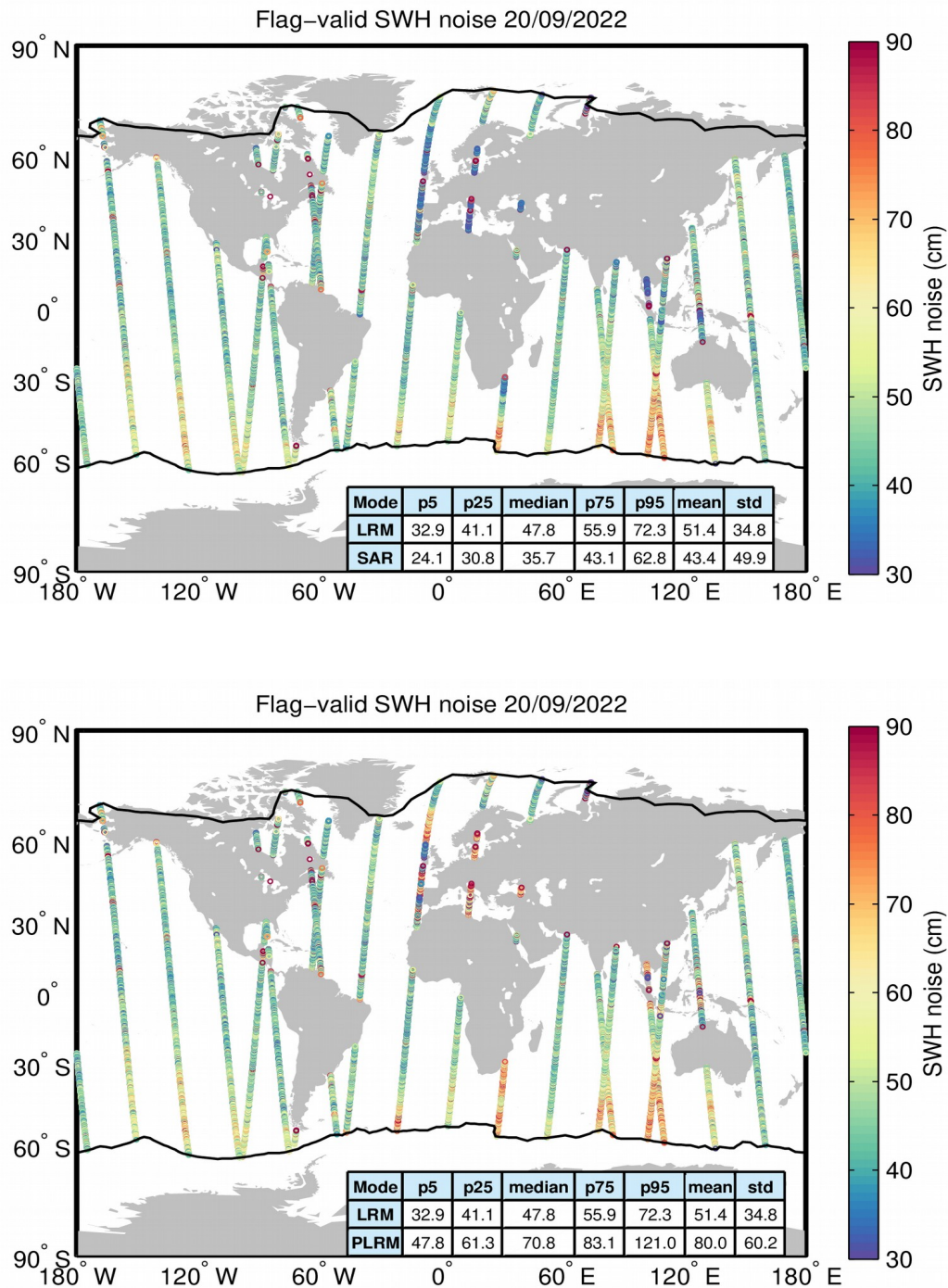
Figure 18. Geographical distribution of flag-valid 20-Hz SWH measurement noise over oceans and lakes for LRM/SAR (top) and LRM/PLRM (bottom) and for 20/09/2022. The statistical values shown in the table refer to the SWH noise and are calculated separately for LRM and SAR/PLRM regions. Measurements taken over polar polygons have been
