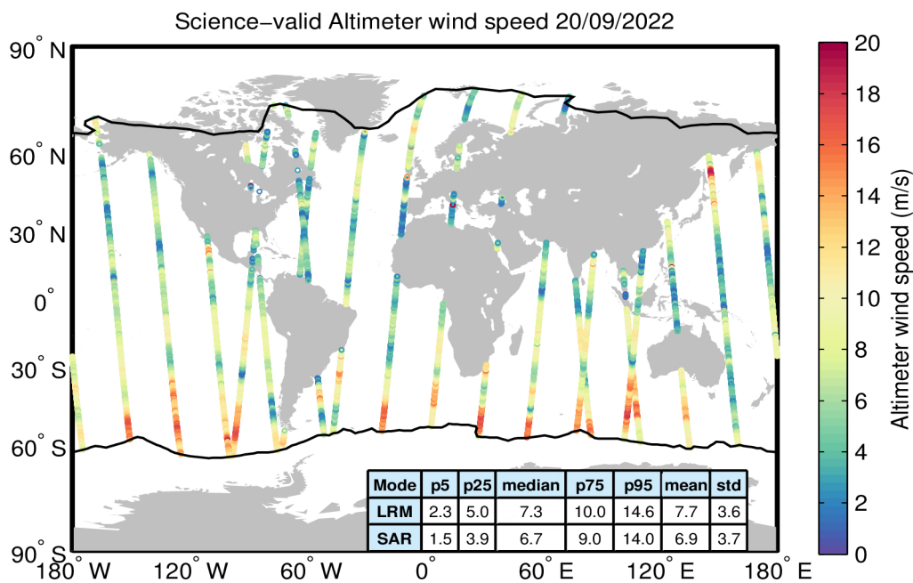
Figure 34. Geographical distribution of science-valid wind data over oceans and lakes for 20/09/2022. The statistical values shown in the table refer to the wind in m/s and are calculated separately for LRM and SAR regions. The black lines mark the outer limit of the Arctic and Antarctic polar polygons. Gray circles denote records that have been rejected based on the editing criteria described in Table 5.
