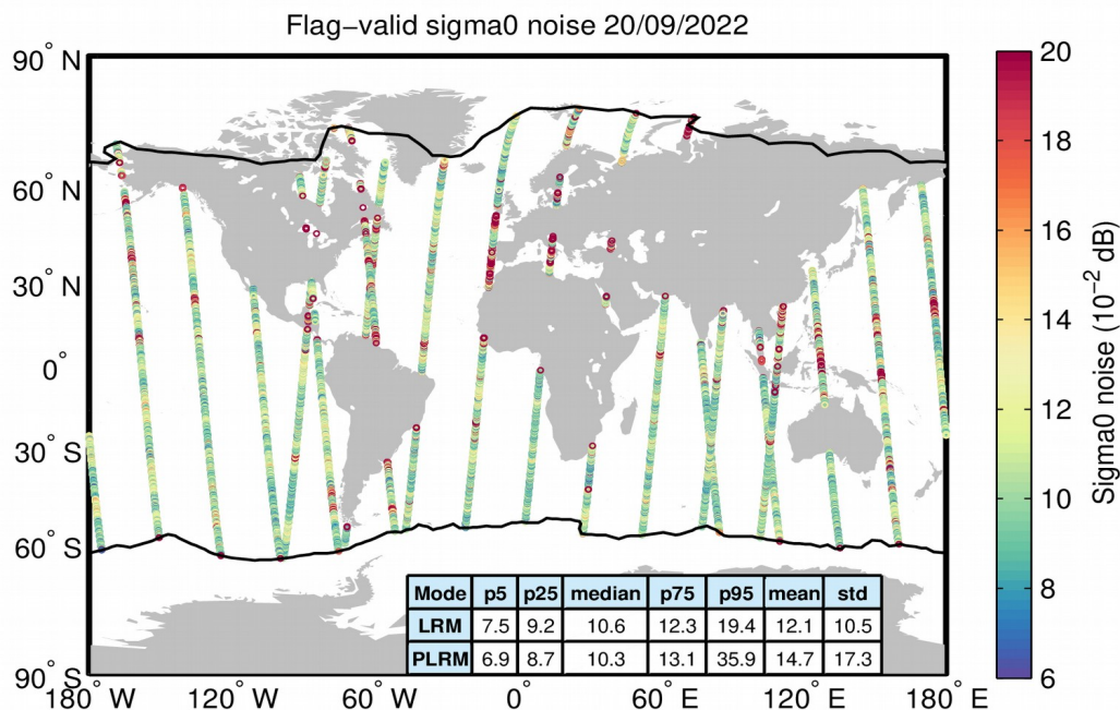
Figure 26. Geographical distribution of flag-valid 20-Hz sigma0 measurement noise over oceans and lakes for LRM/SAR (top) and LRM/PLRM (bottom) and for 20/09/2022. The statistical values shown in the table refer to the sigma0 noise and are calculated separately for LRM and SAR/PLRM regions. Measurements taken over polar polygons have been excluded from the computation of the statistical values. The black lines mark the outer limit of the Arctic and Antarctic polar polygons.
