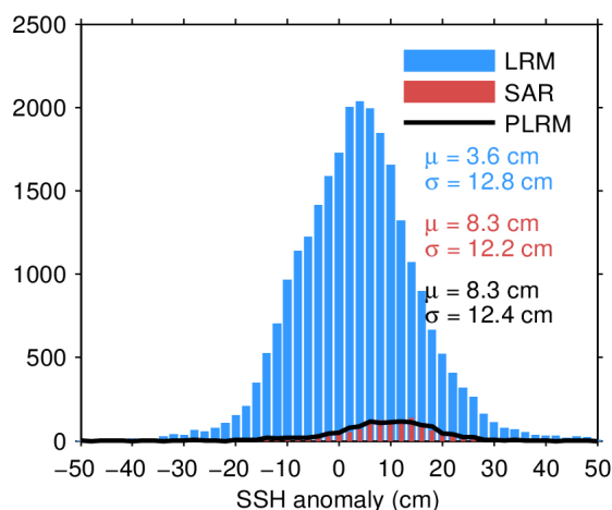
Figure 11. Histogram of science-valid SSH anomaly over oceans and lakes for LRM (blue), SAR (red), and PLRM (black) for 20/09/2022. The mean ( \mu ) and standard deviation ( \sigma ) are also shown. Note that values outside [-50 \ 50] cm are excluded from the histogram for the sake of readability but not from the computation of \mu and \sigma .
