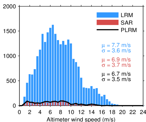
Figure 33. Histogram of flag-valid wind over oceans and lakes for LRM (blue), SAR (red), and PLRM (black) for 20/09/2022. The mean ( \mu ) and standard deviation ( \sigma ) are also shown. Note that values larger than 24 m/s are excluded from the histogram for the sake of readability but not from the computation of \mu and \sigma .
