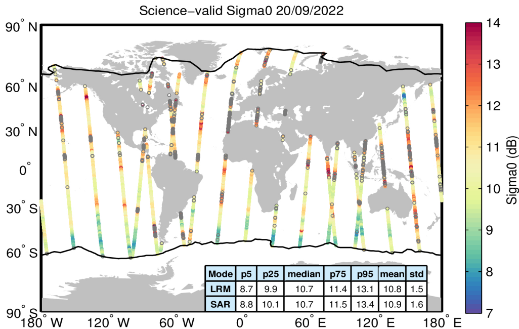
Figure 27. Geographical distribution of science-valid sigma0 data over oceans and lakes for 20/09/2022. The statistical values shown in the table refer to the sigma0 in dB and are calculated separately for LRM and SAR regions. The black lines mark the outer limit of the Arctic and Antarctic polar polygons. Gray circles denote records that have been rejected based on the editing criteria described in Table 4.
