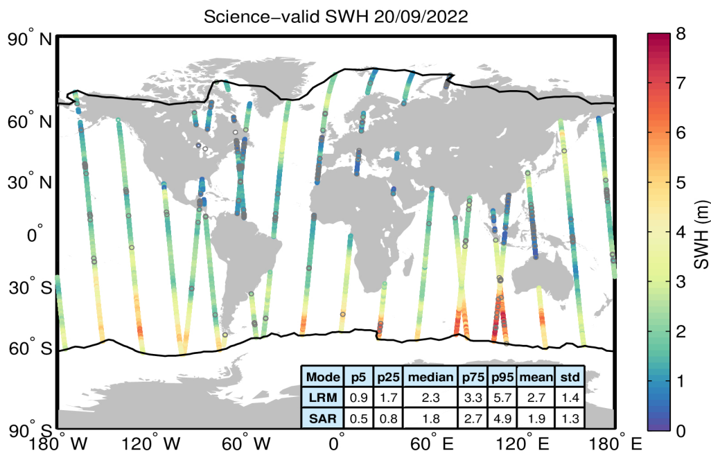
Figure 19. Geographical distribution of science-valid SWH data over oceans and lakes for 20/09/2022. The statistical values shown in the table refer to the SWH in m and are calculated separately for LRM and SAR regions. The black lines mark the outer limit of the Arctic and Antarctic polar polygons. Gray circles denote records that have been rejected based on the editing criteria described in Table 3.
