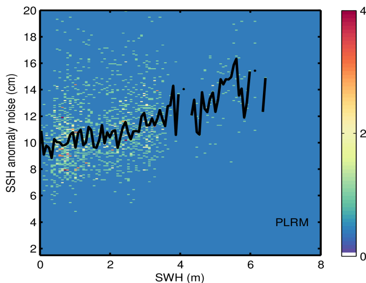
Figure 9. 2D histogram showing flag-valid SSH anomaly noise as a function of SWH for LRM (top), SAR (middle), and PLRM (bottom) for 20/09/2022. The black line denotes the median SSH anomaly noise as a function of SWH.
