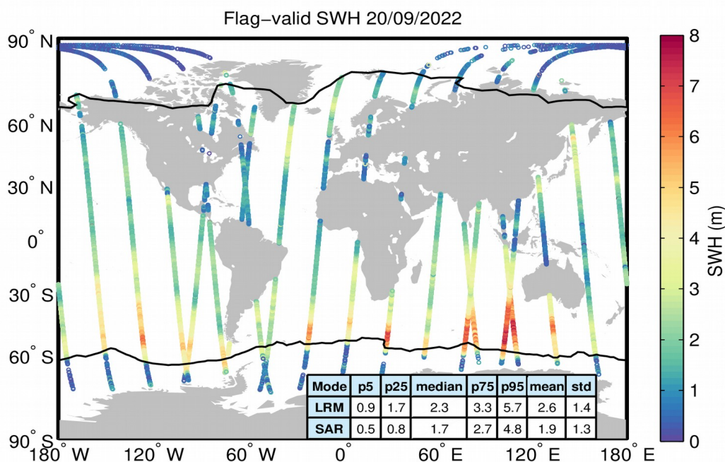
Figure 15. Geographical distribution of flag-valid SWH data over oceans and lakes for 20/09/2022. The statistical values shown in the table refer to the SWH in m and are calculated separately for LRM and SAR regions. Measurements taken over polar polygons have been excluded from the computation of the statistical values. The black lines mark the outer limit of the Arctic and Antarctic polar polygons.
