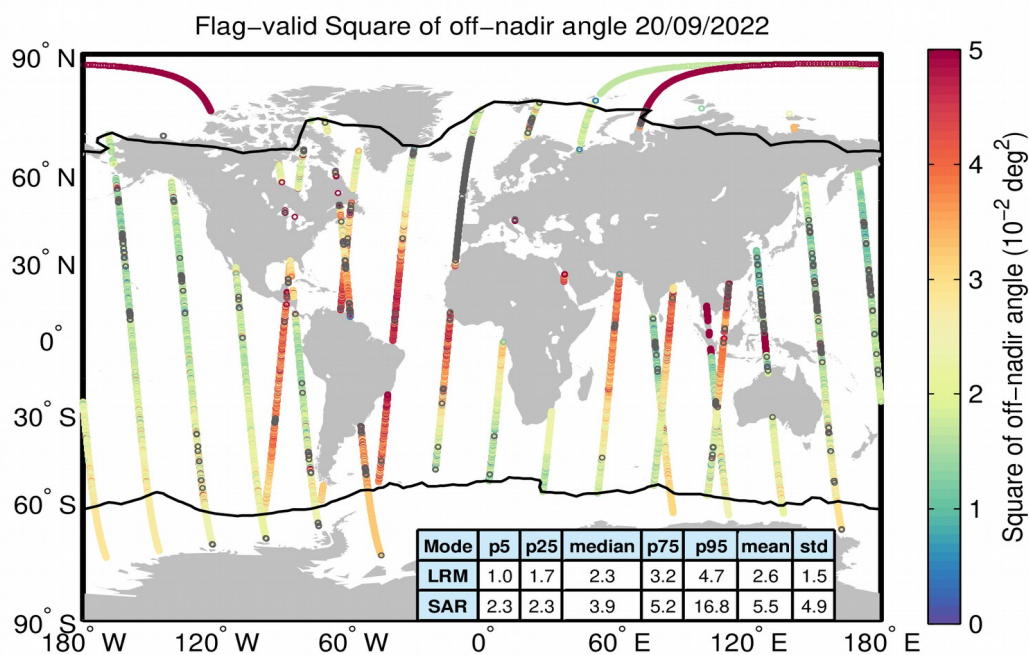
Figure 37. Geographical distribution of flag-valid mispointing data over oceans and lakes for 20/09/2022. The statistical values shown in the table refer to the mispointing in 10^{-2} \text{ deg}^2 and are calculated separately for LRM and SAR regions. Measurements taken over polar polygons have been excluded from the computation of the statistical values. The black lines mark the outer limit of the Arctic and Antarctic polar polygons. Gray circles denote negative values.
