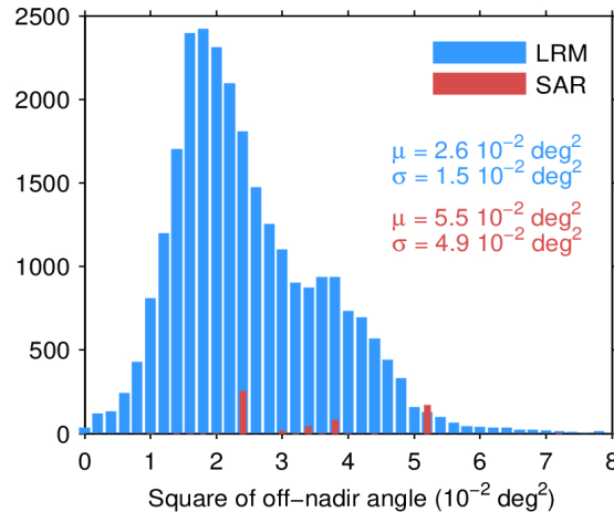
Figure 39. Histogram of flag-valid mispointing over oceans and lakes for LRM (blue) and SAR (red) for 20/09/2022. Only positive values have been considered. The mean ( \mu ) and standard deviation ( \sigma ) are also shown. Note that values larger than 8 \cdot 10^{-2} \text{ deg}^2 are excluded from the histogram for the sake of readability but not from the computation of \mu and \sigma .
