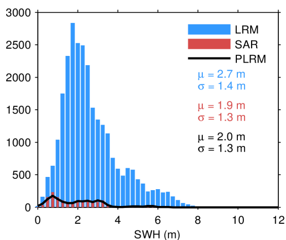
Figure 20. Histogram of science-valid SWH over oceans and lakes for LRM (blue), SAR (red), and PLRM (black) for 20/09/2022. The mean ( \mu ) and standard deviation ( \sigma ) are also
