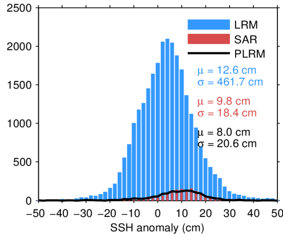
Figure 7. Histogram of flag-valid SSH anomaly over oceans and lakes for LRM (blue), SAR (red), and PLRM (black) for 20/09/2022. The mean ( \mu ) and standard deviation ( \sigma ) are also shown. Note that values outside [-50 50] cm are excluded from the histogram for the sake of readability but not from the computation of \mu and \sigma .
