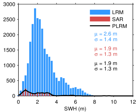
Figure 17. Histogram of flag-valid SWH over oceans and lakes for LRM (blue), SAR (red), and PLRM (black) for 20/09/2022. The mean ( \mu ) and standard deviation ( \sigma ) are also shown. Note that values larger than 12 m are excluded from the histogram for the sake of readability but not from the computation of \mu and \sigma .
