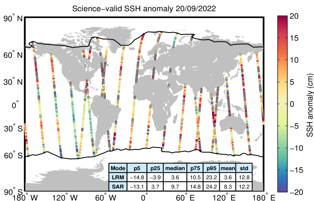
Figure 10. Geographical distribution of science-valid SSH anomaly data over oceans and lakes for 20/09/2022. The statistical values shown in the table refer to the SSH anomaly in cm and are calculated separately for LRM and SAR regions. The black lines mark the
