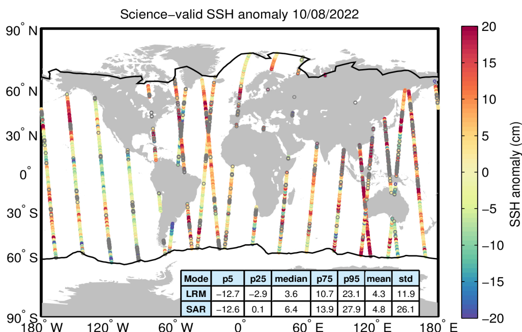
Figure 10. Geographical distribution of science-valid SSH anomaly data over oceans and lakes for 10/08/2022. The statistical values shown in the table refer to the SSH anomaly in cm and are calculated separately for LRM and SAR regions. The black lines mark the
