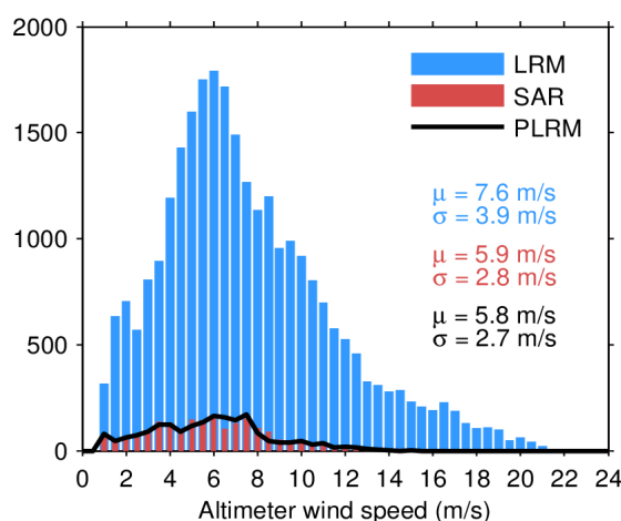
Figure 33. Histogram of flag-valid wind over oceans and lakes for LRM (blue), SAR (red), and PLRM (black) for 10/08/2022. The mean ( \mu ) and standard deviation ( \sigma ) are also shown. Note that values larger than 24 m/s are excluded from the histogram for the sake of readability but not from the computation of \mu and \sigma .
