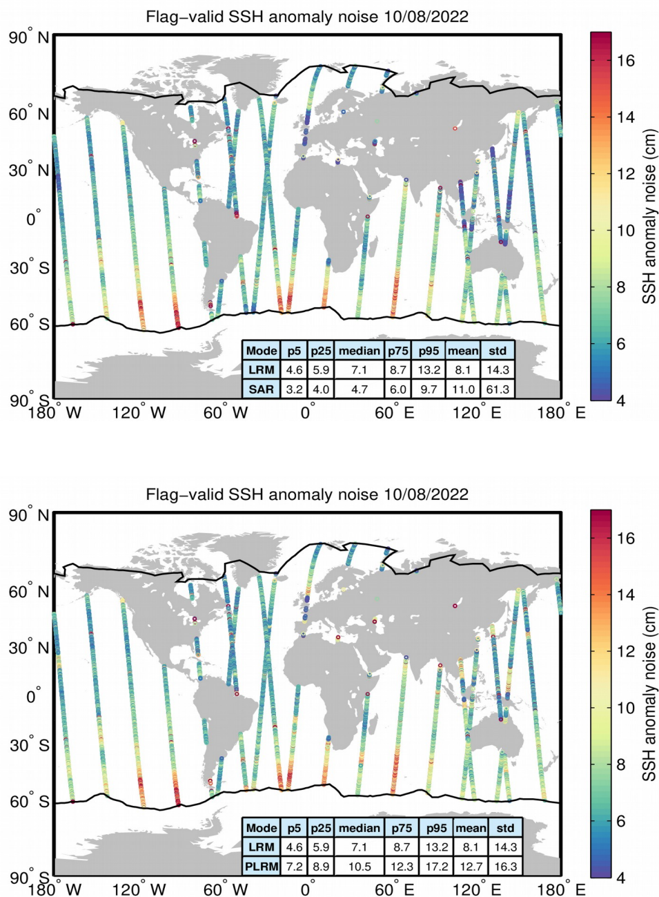
Figure 8. Geographical distribution of flag-valid 20-Hz SSH anomaly measurement noise over oceans and lakes for LRM/SAR (top) and LRM/PLRM (bottom) and for 10/08/2022. The statistical values shown in the tables refer to the SSH anomaly noise and are calculated separately for LRM and SAR/PLRM regions. Measurements taken over polar polygons have been excluded from the computation of the statistical values. The black lines mark the outer limit of the Arctic and Antarctic polar polygons.
