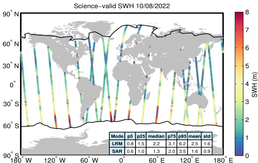
Figure 19. Geographical distribution of science-valid SWH data over oceans and lakes for 10/08/2022. The statistical values shown in the table refer to the SWH in m and are calculated separately for LRM and SAR regions. The black lines mark the outer limit of the Arctic and Antarctic polar polygons. Gray circles denote records that have been rejected based on the editing criteria described in Table 3.
