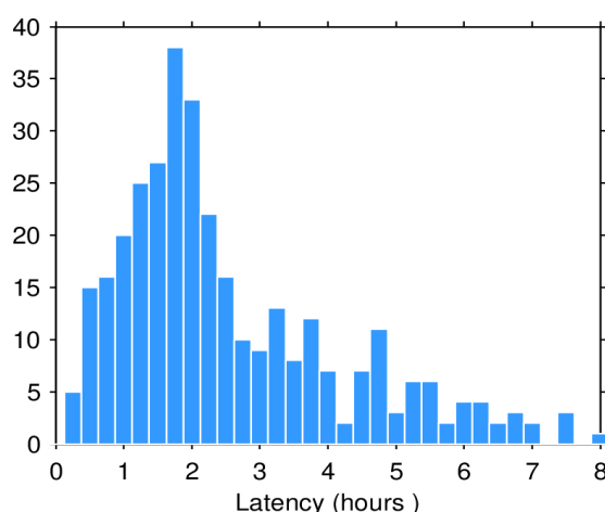
Figure 2. Histogram of the data latency for 10/08/2022. The y-axis denotes the number of files that are made available with a delay of x-hours with respect to the mean time of the records stored in the file.
