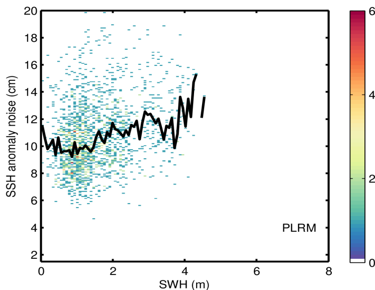
Figure 9. 2D histogram showing flag-valid SSH anomaly noise as a function of SWH for LRM (top), SAR (middle), and PLRM (bottom) for 10/08/2022. The black line denotes the median SSH anomaly noise as a function of SWH.
