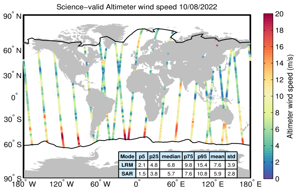
Figure 34. Geographical distribution of science-valid wind data over oceans and lakes for 10/08/2022. The statistical values shown in the table refer to the wind in m/s and are calculated separately for LRM and SAR regions. The black lines mark the outer limit of the Arctic and Antarctic polar polygons. Gray circles denote records that have been rejected based on the editing criteria described in Table 5.
