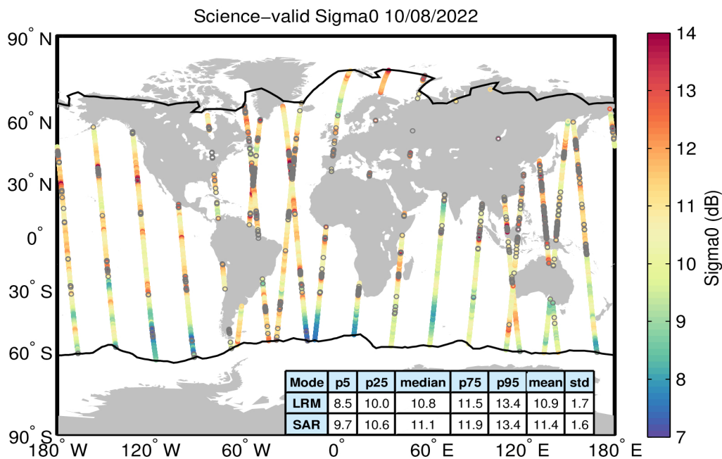
Figure 27. Geographical distribution of science-valid sigma0 data over oceans and lakes for 10/08/2022. The statistical values shown in the table refer to the sigma0 in dB and are calculated separately for LRM and SAR regions. The black lines mark the outer limit of the Arctic and Antarctic polar polygons. Gray circles denote records that have been rejected based on the editing criteria described in Table 4.
