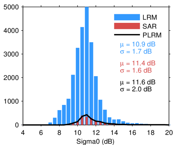
Figure 28. Histogram of science-valid sigma0 over oceans and lakes for LRM (blue), SAR (red), and PLRM (black) for 10/08/2022. The mean ( \mu ) and standard deviation ( \sigma ) are also shown. Note that values outside [4 20] dB are excluded from the histogram for the sake of readability but not from the computation of \mu and \sigma .
