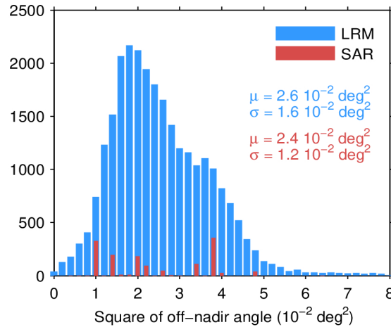
Figure 39. Histogram of flag-valid mispointing over oceans and lakes for LRM (blue) and SAR (red) for 10/08/2022. Only positive values have been considered. The mean ( \mu ) and standard deviation ( \sigma ) are also shown. Note that values larger than 8 \cdot 10^{-2} \text{ deg}^2 are excluded from the histogram for the sake of readability but not from the computation of \mu and \sigma .
