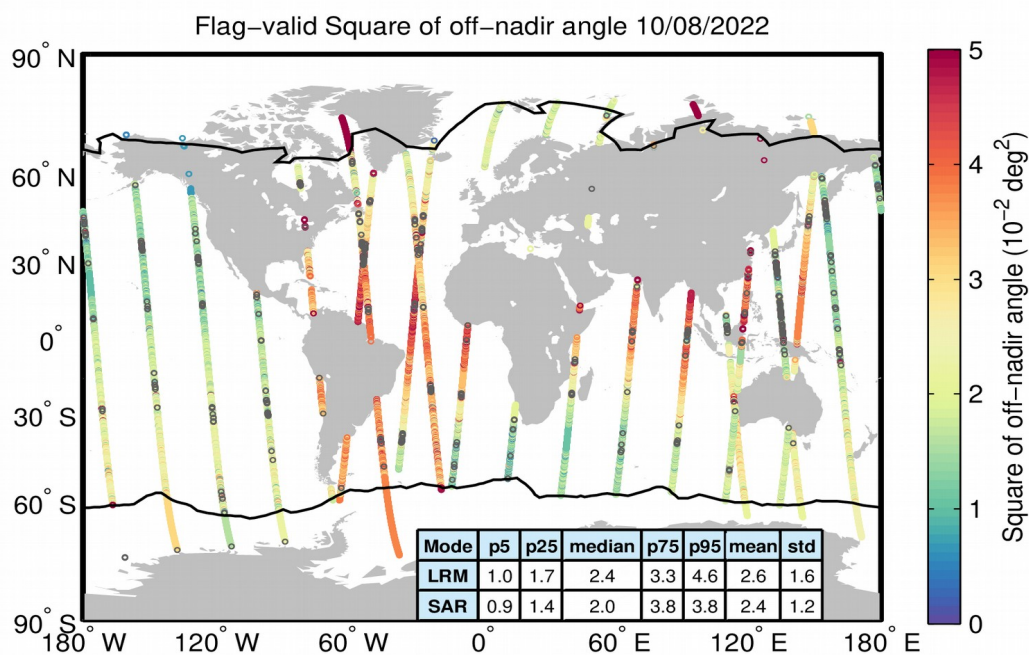
Figure 37. Geographical distribution of flag-valid mispointing data over oceans and lakes for 10/08/2022. The statistical values shown in the table refer to the mispointing in 10^{-2} \text{ deg}^2 and are calculated separately for LRM and SAR regions. Measurements taken over polar polygons have been excluded from the computation of the statistical values. The black lines mark the outer limit of the Arctic and Antarctic polar polygons. Gray circles denote negative values.
