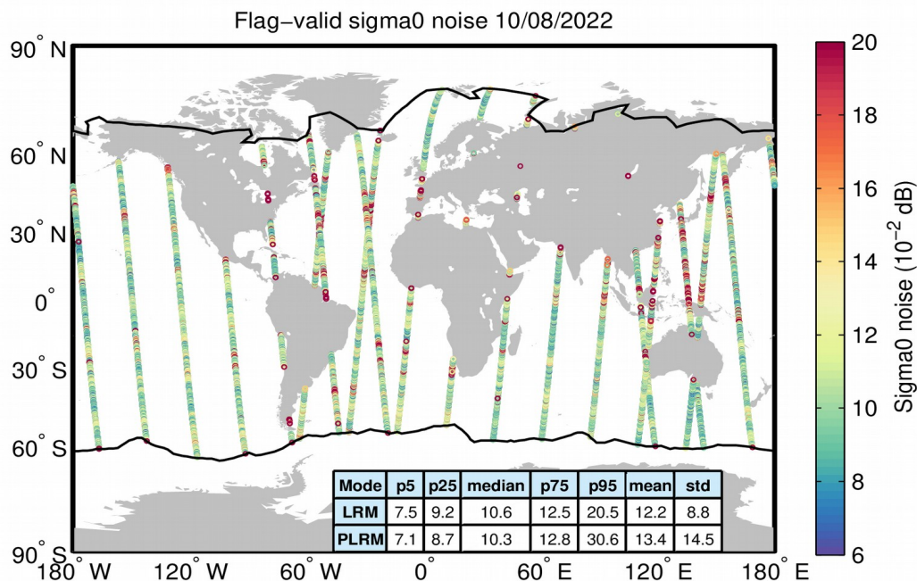
Figure 26. Geographical distribution of flag-valid 20-Hz sigma0 measurement noise over oceans and lakes for LRM/SAR (top) and LRM/PLRM (bottom) and for 10/08/2022. The statistical values shown in the table refer to the sigma0 noise and are calculated separately for LRM and SAR/PLRM regions. Measurements taken over polar polygons have been excluded from the computation of the statistical values. The black lines mark the outer limit of the Arctic and Antarctic polar polygons.
