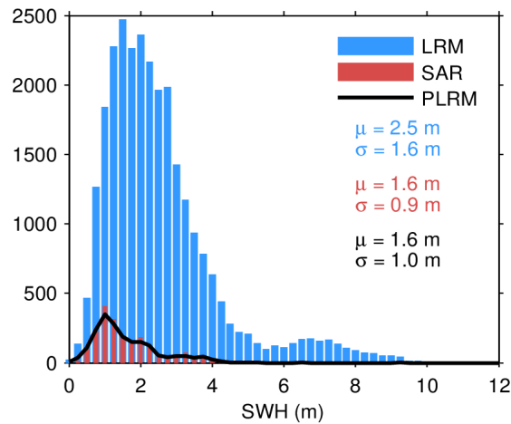
Figure 17. Histogram of flag-valid SWH over oceans and lakes for LRM (blue), SAR (red), and PLRM (black) for 10/08/2022. The mean ( \mu ) and standard deviation ( \sigma ) are also shown. Note that values larger than 12 m are excluded from the histogram for the sake of readability but not from the computation of \mu and \sigma .
