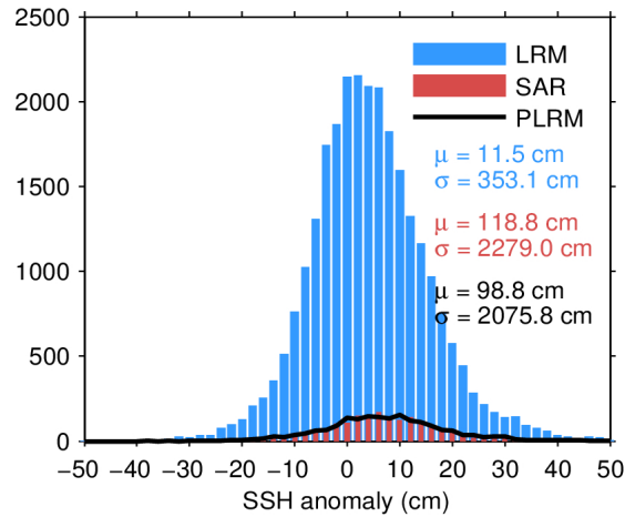
Figure 7. Histogram of flag-valid SSH anomaly over oceans and lakes for LRM (blue), SAR (red), and PLRM (black) for 10/08/2022. The mean ( \mu ) and standard deviation ( \sigma ) are also shown. Note that values outside [-50 50] cm are excluded from the histogram for the sake of readability but not from the computation of \mu and \sigma .
