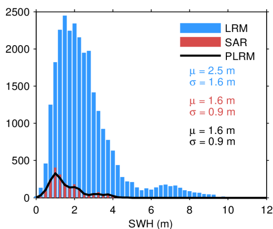
Figure 20. Histogram of science-valid SWH over oceans and lakes for LRM (blue), SAR (red), and PLRM (black) for 10/08/2022. The mean ( \mu ) and standard deviation ( \sigma ) are also
