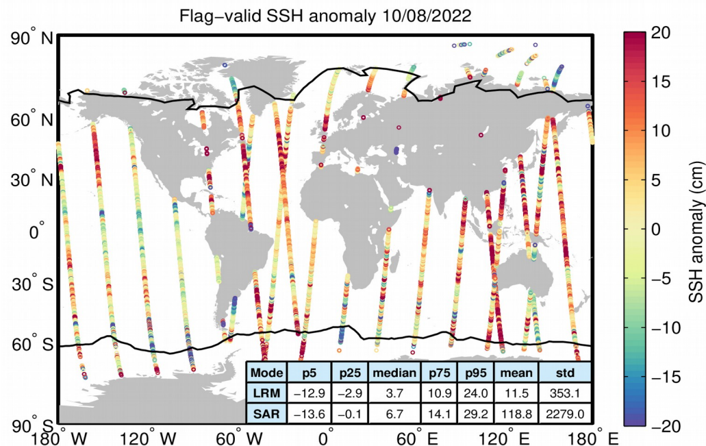
Figure 5. Geographical distribution of flag-valid 1-Hz SSH anomaly data over oceans and lakes for 10/08/2022. The statistical values shown in the table refer to the SSH anomaly in cm and are calculated separately for LRM and SAR regions. Measurements taken over polar polygons have been excluded from the computation of the statistical values. The black lines mark the outer limit of the Arctic and Antarctic polar polygons.
