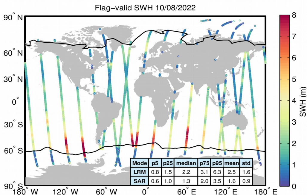
Figure 15. Geographical distribution of flag-valid SWH data over oceans and lakes for 10/08/2022. The statistical values shown in the table refer to the SWH in m and are calculated separately for LRM and SAR regions. Measurements taken over polar polygons have been excluded from the computation of the statistical values. The black lines mark the outer limit of the Arctic and Antarctic polar polygons.
