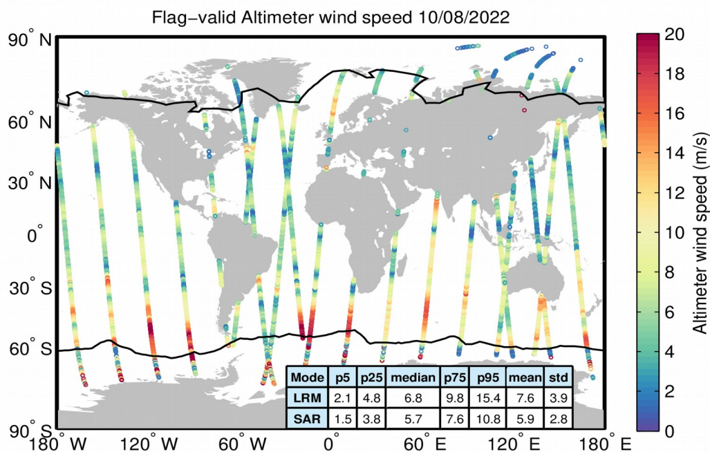
Figure 31. Geographical distribution of flag-valid wind data over oceans and lakes for 10/08/2022. The statistical values shown in the table refer to the wind in m/s and are calculated separately for LRM and SAR regions. Measurements taken over polar polygons have been excluded from the computation of the statistical values. The black lines mark the outer limit of the Arctic and Antarctic polar polygons.
