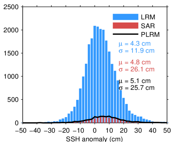
Figure 11. Histogram of science-valid SSH anomaly over oceans and lakes for LRM (blue), SAR (red), and PLRM (black) for 10/08/2022. The mean ( \mu ) and standard deviation ( \sigma ) are also shown. Note that values outside [-50\ 50] cm are excluded from the histogram for the sake of readability but not from the computation of \mu and \sigma .
