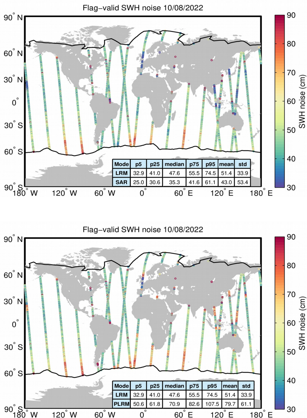
Figure 18. Geographical distribution of flag-valid 20-Hz SWH measurement noise over oceans and lakes for LRM/SAR (top) and LRM/PLRM (bottom) and for 10/08/2022. The statistical values shown in the table refer to the SWH noise and are calculated separately for LRM and SAR/PLRM regions. Measurements taken over polar polygons have been
