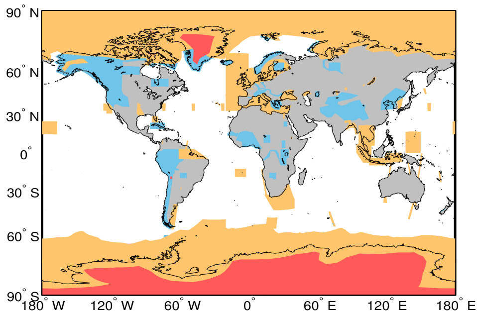
Figure A1. Extent of the regions defining the geographical mode mask for 10/08/2022. The regions where SAR, and SARIn are operated are denoted by the orange and blue polygons, respectively. LRM is operated over areas of the continental ice sheets (red polygons) and over oceans and land not covered by other modes.
