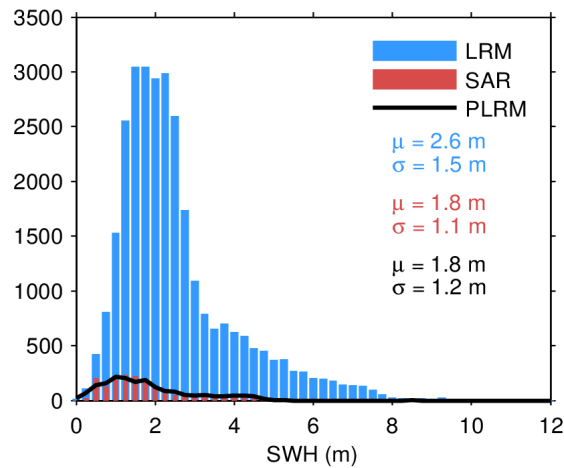
Figure 17. Histogram of flag-valid SWH over oceans and lakes for LRM (blue), SAR (red), and PLRM (black) for 29/06/2022. The mean ( \mu ) and standard deviation ( \sigma ) are also shown. Note that values larger than 12 m are excluded from the histogram for the sake of readability but not from the computation of \mu and \sigma .
