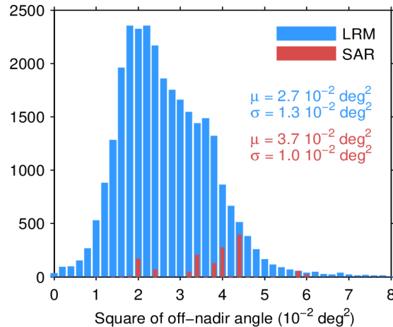
Figure 39. Histogram of flag-valid mispointing over oceans and lakes for LRM (blue) and SAR (red) for 29/06/2022. Only positive values have been considered. The mean ( \mu ) and standard deviation ( \sigma ) are also shown. Note that values larger than 8 \cdot 10^{-2} \text{ deg}^2 are excluded from the histogram for the sake of readability but not from the computation of \mu and \sigma .
