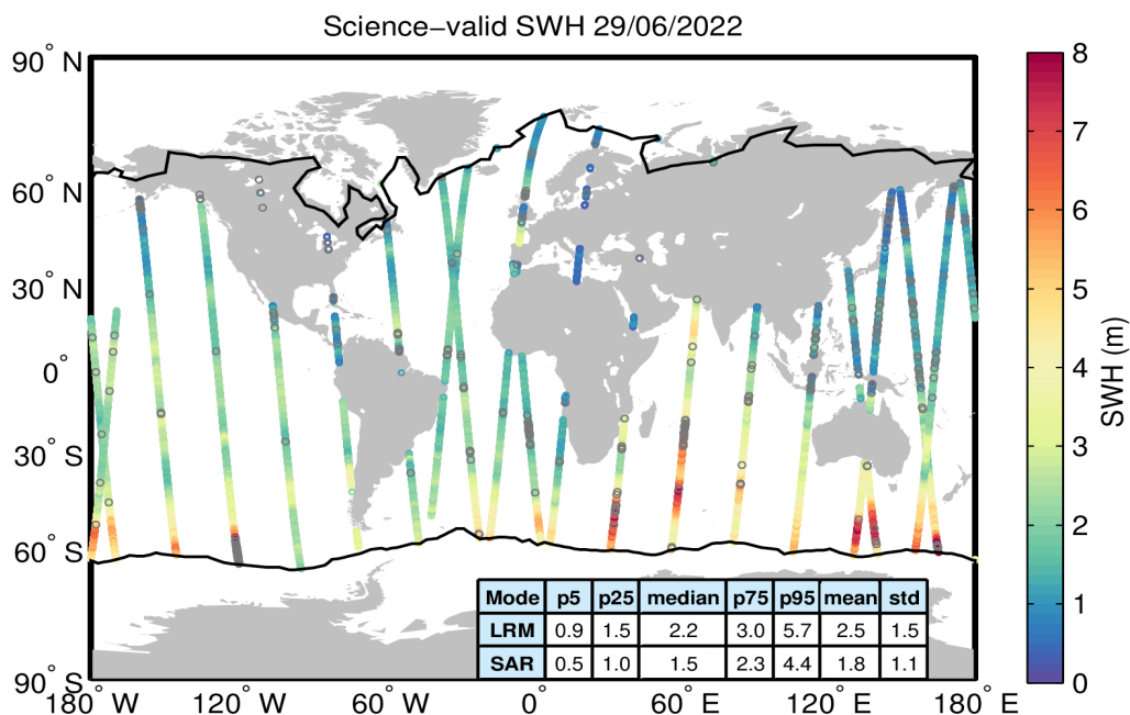
Figure 19. Geographical distribution of science-valid SWH data over oceans and lakes for 29/06/2022. The statistical values shown in the table refer to the SWH in m and are calculated separately for LRM and SAR regions. The black lines mark the outer limit of the Arctic and Antarctic polar polygons. Gray circles denote records that have been rejected based on the editing criteria described in Table 3.
