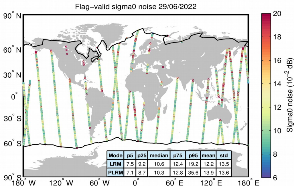
Figure 26. Geographical distribution of flag-valid 20-Hz sigma0 measurement noise over oceans and lakes for LRM/SAR (top) and LRM/PLRM (bottom) and for 29/06/2022. The statistical values shown in the table refer to the sigma0 noise and are calculated separately for LRM and SAR/PLRM regions. Measurements taken over polar polygons have been excluded from the computation of the statistical values. The black lines mark the outer limit of the Arctic and Antarctic polar polygons.
