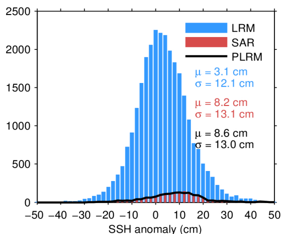
Figure 11. Histogram of science-valid SSH anomaly over oceans and lakes for LRM (blue), SAR (red), and PLRM (black) for 29/06/2022. The mean ( \mu ) and standard deviation ( \sigma ) are also shown. Note that values outside [-50\ 50] cm are excluded from the histogram for the sake of readability but not from the computation of \mu and \sigma .
