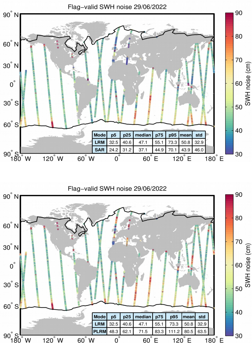
Figure 18. Geographical distribution of flag-valid 20-Hz SWH measurement noise over oceans and lakes for LRM/SAR (top) and LRM/PLRM (bottom) and for 29/06/2022. The statistical values shown in the table refer to the SWH noise and are calculated separately for LRM and SAR/PLRM regions. Measurements taken over polar polygons have been
