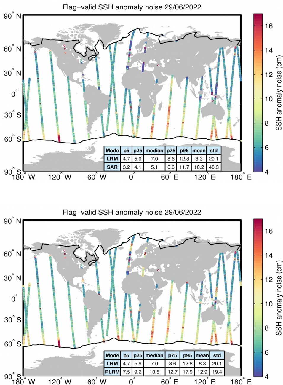
Figure 8. Geographical distribution of flag-valid 20-Hz SSH anomaly measurement noise over oceans and lakes for LRM/SAR (top) and LRM/PLRM (bottom) and for 29/06/2022. The statistical values shown in the tables refer to the SSH anomaly noise and are calculated separately for LRM and SAR/PLRM regions. Measurements taken over polar polygons have been excluded from the computation of the statistical values. The black lines mark the outer limit of the Arctic and Antarctic polar polygons.
