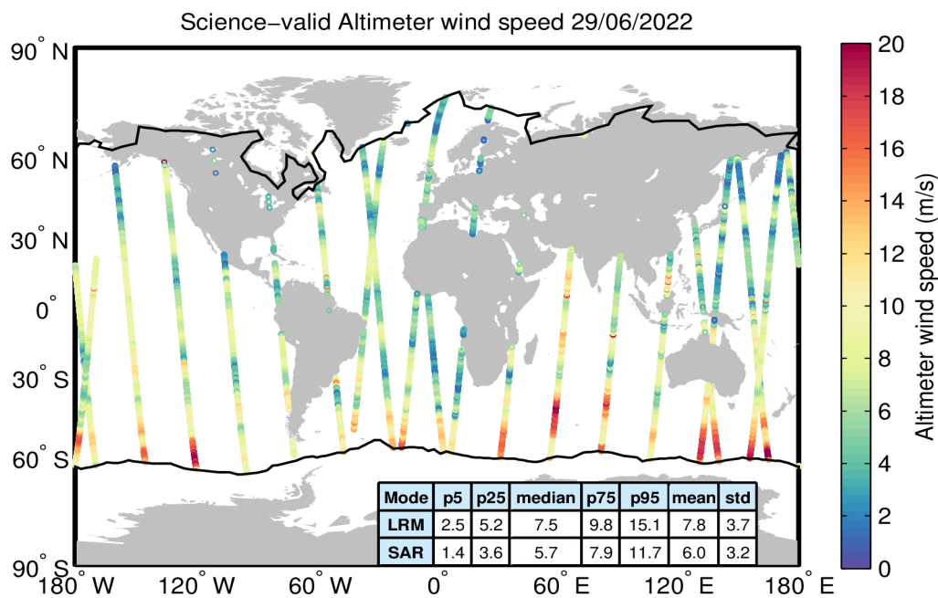
Figure 34. Geographical distribution of science-valid wind data over oceans and lakes for 29/06/2022. The statistical values shown in the table refer to the wind in m/s and are calculated separately for LRM and SAR regions. The black lines mark the outer limit of the Arctic and Antarctic polar polygons. Gray circles denote records that have been rejected based on the editing criteria described in Table 5.
