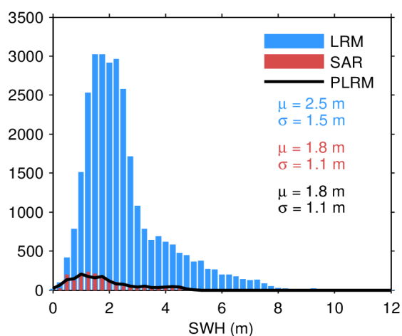
Figure 20. Histogram of science-valid SWH over oceans and lakes for LRM (blue), SAR (red), and PLRM (black) for 29/06/2022. The mean ( \mu ) and standard deviation ( \sigma ) are also
