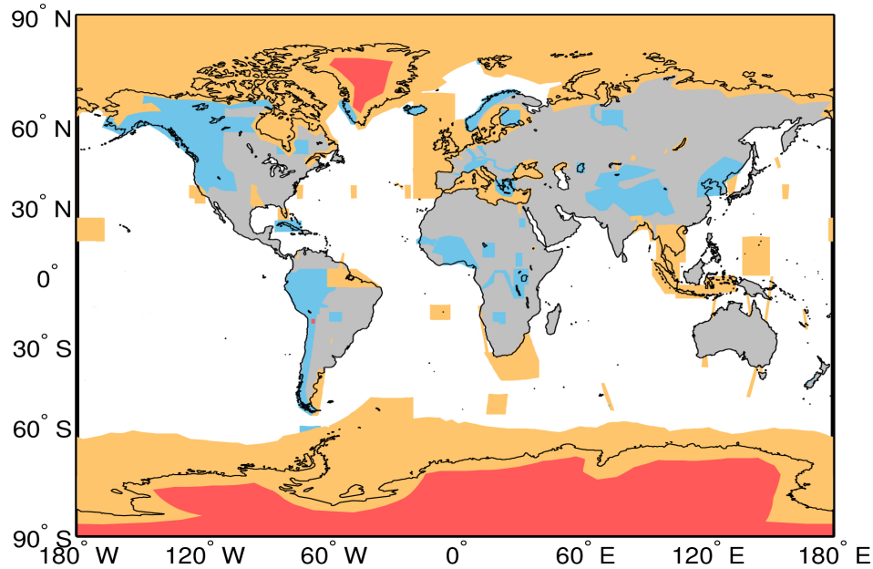
Figure A1. Extent of the regions defining the geographical mode mask for 29/06/2022. The regions where SAR, and SARIn are operated are denoted by the orange and blue polygons, respectively. LRM is operated over areas of the continental ice sheets (red polygons) and over oceans and land not covered by other modes.
