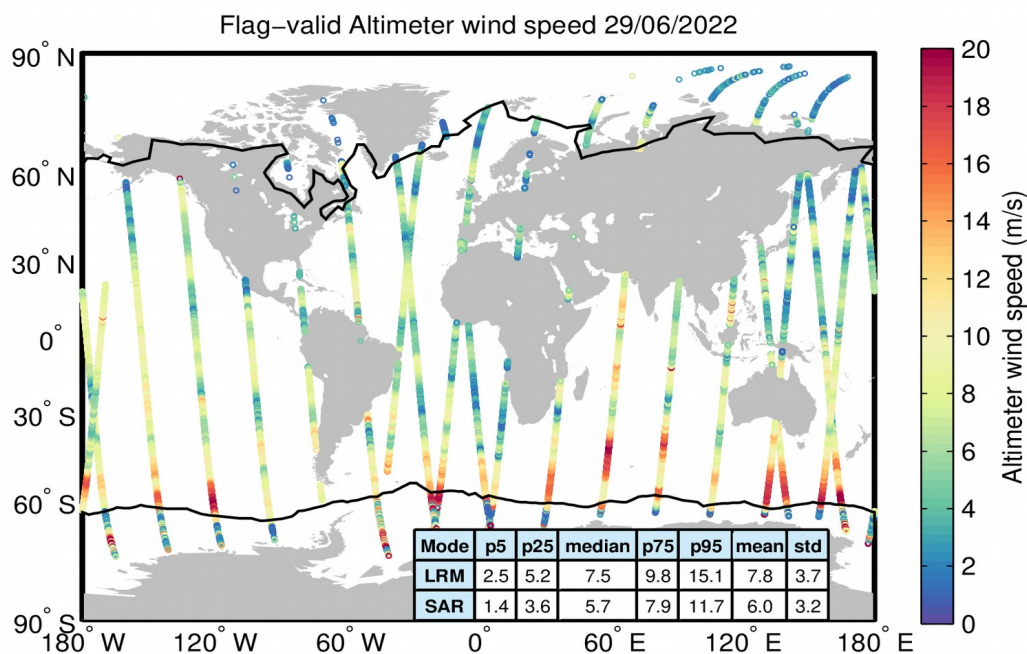
Figure 31. Geographical distribution of flag-valid wind data over oceans and lakes for 29/06/2022. The statistical values shown in the table refer to the wind in m/s and are calculated separately for LRM and SAR regions. Measurements taken over polar polygons have been excluded from the computation of the statistical values. The black lines mark the outer limit of the Arctic and Antarctic polar polygons.
