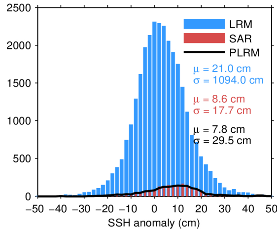
Figure 7. Histogram of flag-valid SSH anomaly over oceans and lakes for LRM (blue), SAR (red), and PLRM (black) for 29/06/2022. The mean ( \mu ) and standard deviation ( \sigma ) are also shown. Note that values outside [-50 50] cm are excluded from the histogram for the sake of readability but not from the computation of \mu and \sigma .
