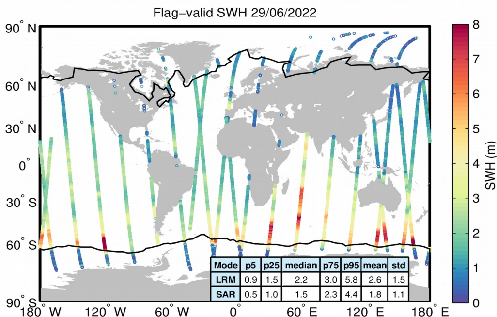
Figure 15. Geographical distribution of flag-valid SWH data over oceans and lakes for 29/06/2022. The statistical values shown in the table refer to the SWH in m and are calculated separately for LRM and SAR regions. Measurements taken over polar polygons have been excluded from the computation of the statistical values. The black lines mark the outer limit of the Arctic and Antarctic polar polygons.
