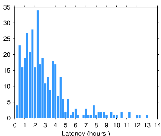
Figure 2. Histogram of the data latency for 29/06/2022. The y-axis denotes the number of files that are made available with a delay of x-hours with respect to the mean time of the records stored in the file.
