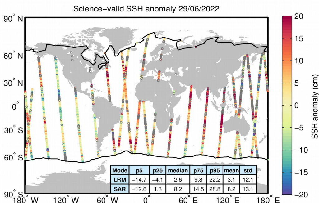
Figure 10. Geographical distribution of science-valid SSH anomaly data over oceans and lakes for 29/06/2022. The statistical values shown in the table refer to the SSH anomaly in cm and are calculated separately for LRM and SAR regions. The black lines mark the
