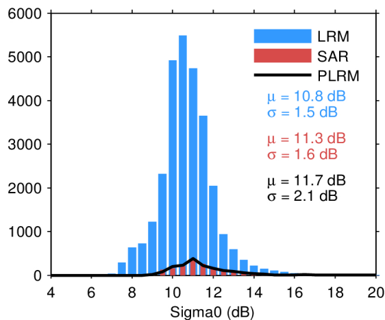
Figure 28. Histogram of science-valid sigma0 over oceans and lakes for LRM (blue), SAR (red), and PLRM (black) for 29/06/2022. The mean ( \mu ) and standard deviation ( \sigma ) are also shown. Note that values outside [4 20] dB are excluded from the histogram for the sake of readability but not from the computation of \mu and \sigma .
