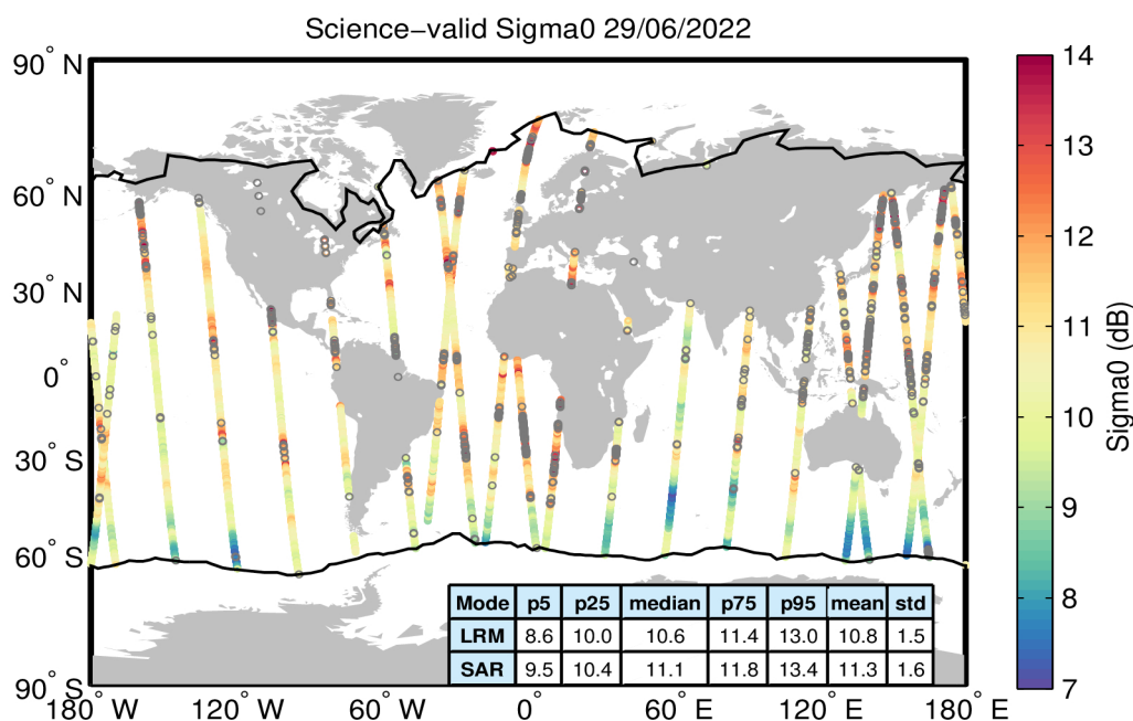
Figure 27. Geographical distribution of science-valid sigma0 data over oceans and lakes for 29/06/2022. The statistical values shown in the table refer to the sigma0 in dB and are calculated separately for LRM and SAR regions. The black lines mark the outer limit of the Arctic and Antarctic polar polygons. Gray circles denote records that have been rejected based on the editing criteria described in Table 4.
