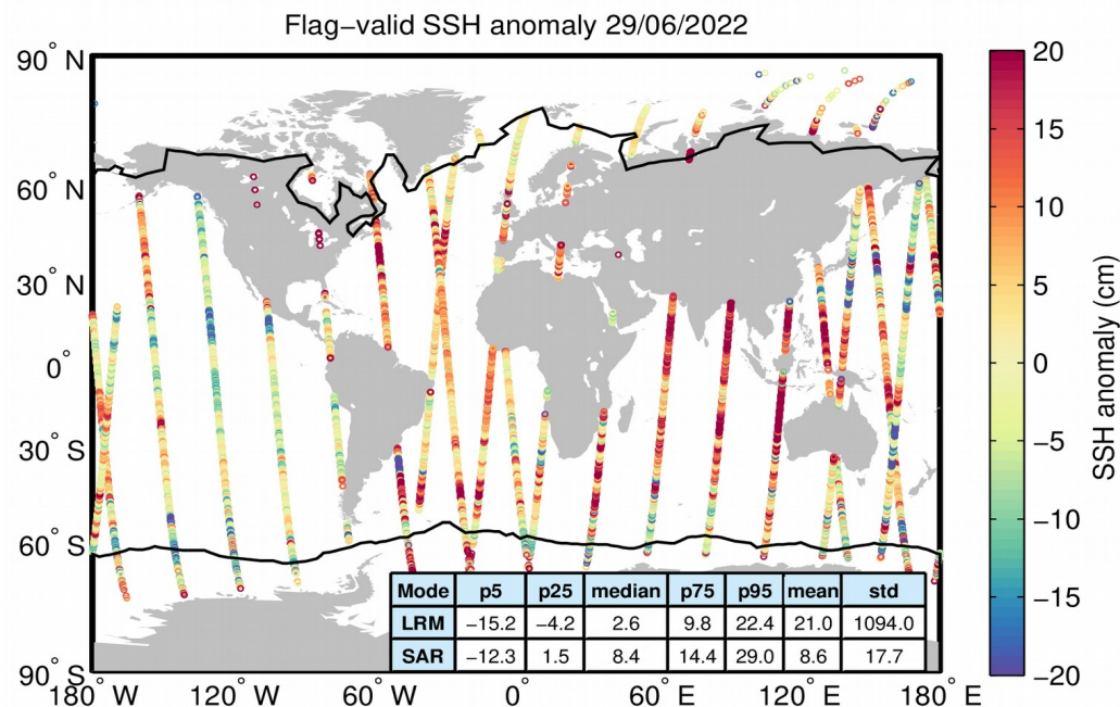
Figure 5. Geographical distribution of flag-valid 1-Hz SSH anomaly data over oceans and lakes for 29/06/2022. The statistical values shown in the table refer to the SSH anomaly in cm and are calculated separately for LRM and SAR regions. Measurements taken over polar polygons have been excluded from the computation of the statistical values. The black lines mark the outer limit of the Arctic and Antarctic polar polygons.
