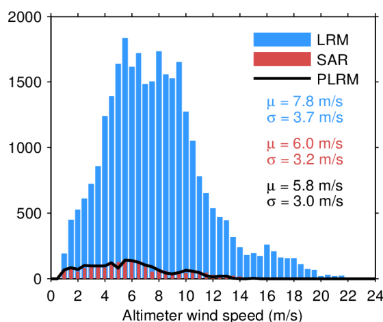
Figure 33. Histogram of flag-valid wind over oceans and lakes for LRM (blue), SAR (red), and PLRM (black) for 29/06/2022. The mean ( \mu ) and standard deviation ( \sigma ) are also shown. Note that values larger than 24 m/s are excluded from the histogram for the sake of readability but not from the computation of \mu and \sigma .
