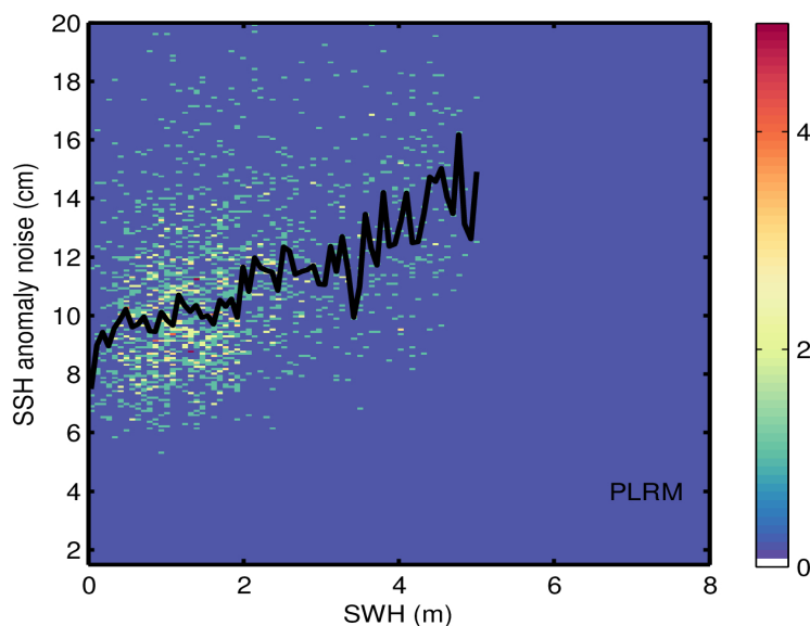
Figure 9. 2D histogram showing flag-valid SSH anomaly noise as a function of SWH for LRM (top), SAR (middle), and PLRM (bottom) for 29/06/2022. The black line denotes the median SSH anomaly noise as a function of SWH.
