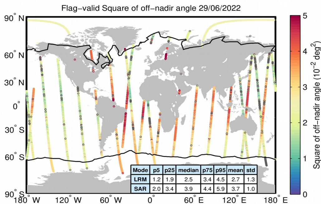
Figure 37. Geographical distribution of flag-valid mispointing data over oceans and lakes for 29/06/2022. The statistical values shown in the table refer to the mispointing in 10^{-2} \text{ deg}^2 and are calculated separately for LRM and SAR regions. Measurements taken over polar polygons have been excluded from the computation of the statistical values. The black lines mark the outer limit of the Arctic and Antarctic polar polygons. Gray circles denote negative values.
