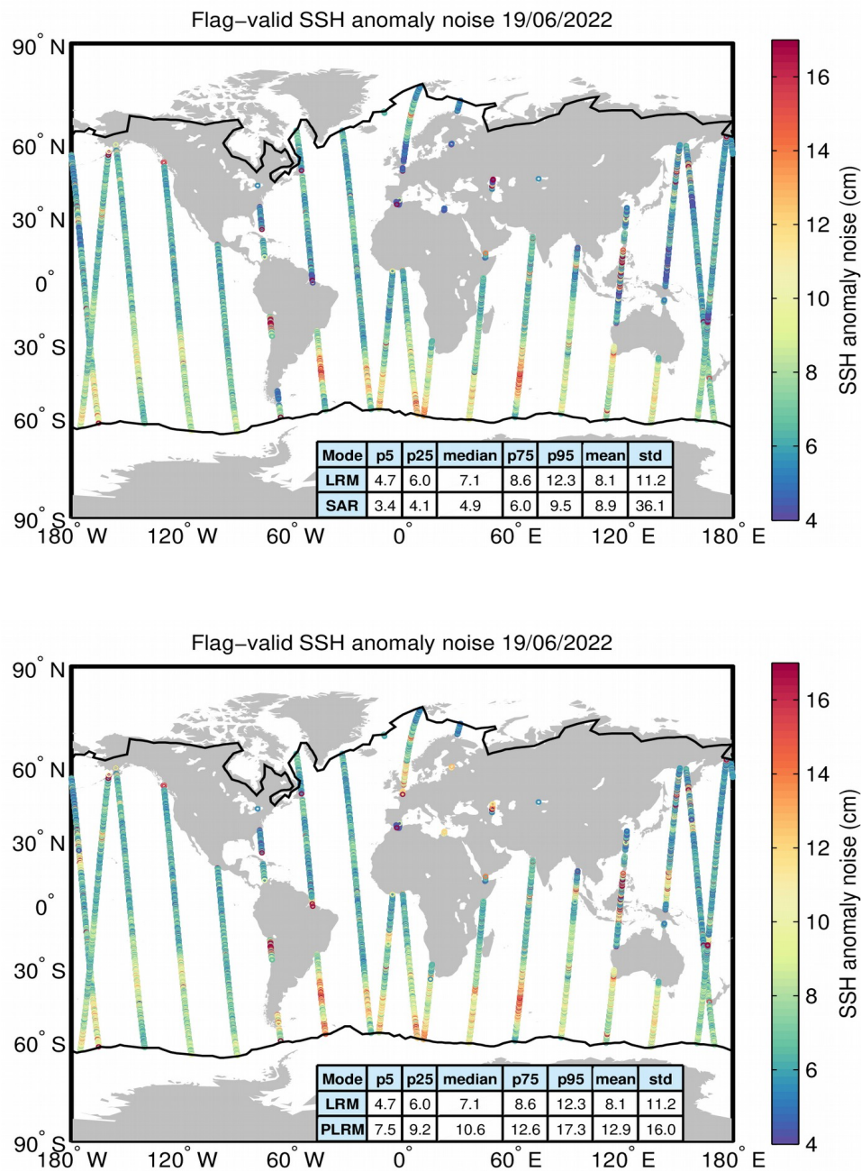
Figure 8. Geographical distribution of flag-valid 20-Hz SSH anomaly measurement noise over oceans and lakes for LRM/SAR (top) and LRM/PLRM (bottom) and for 19/06/2022. The statistical values shown in the tables refer to the SSH anomaly noise and are calculated separately for LRM and SAR/PLRM regions. Measurements taken over polar polygons have been excluded from the computation of the statistical values. The black lines mark the outer limit of the Arctic and Antarctic polar polygons.
