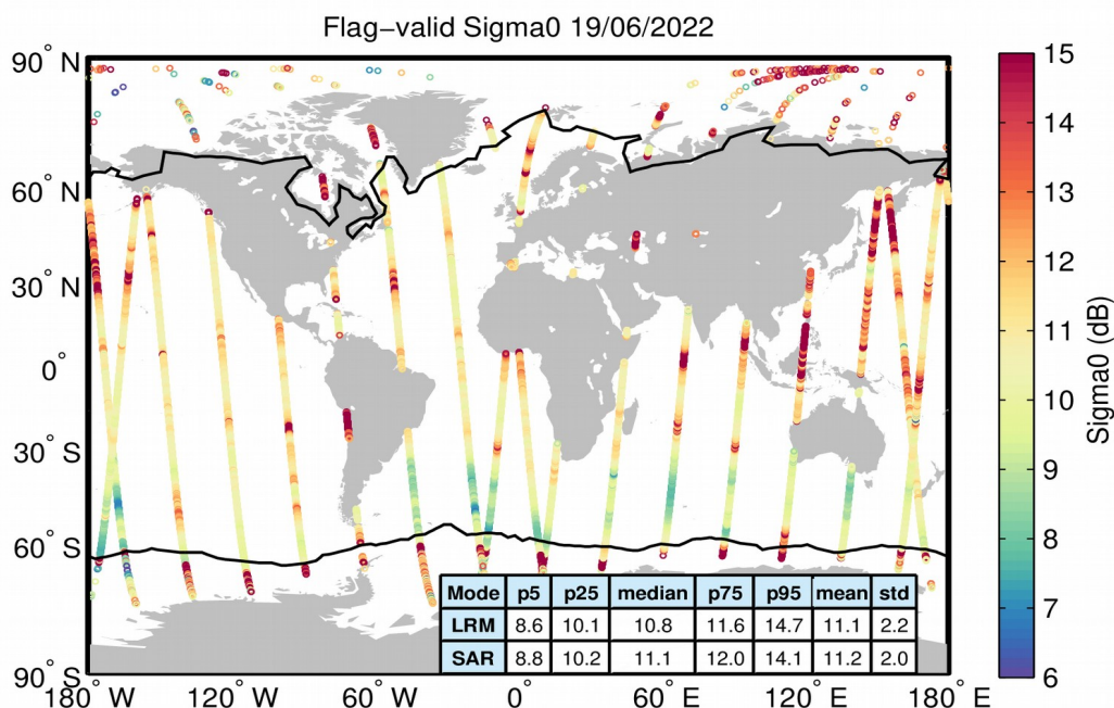
Figure 23. Geographical distribution of flag-valid sigma0 data over oceans and lakes for 19/06/2022. The statistical values shown in the table refer to the sigma0 in dB and are calculated separately for LRM and SAR regions. Measurements taken over polar polygons
