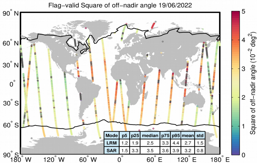
Figure 37. Geographical distribution of flag-valid mispointing data over oceans and lakes for 19/06/2022. The statistical values shown in the table refer to the mispointing in 10^{-2} \text{ deg}^2 and are calculated separately for LRM and SAR regions. Measurements taken over polar polygons have been excluded from the computation of the statistical values. The black lines mark the outer limit of the Arctic and Antarctic polar polygons. Gray circles denote negative values.
