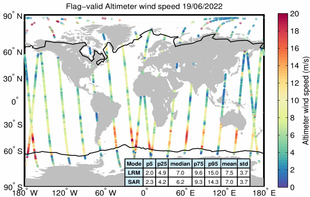
Figure 31. Geographical distribution of flag-valid wind data over oceans and lakes for 19/06/2022. The statistical values shown in the table refer to the wind in m/s and are calculated separately for LRM and SAR regions. Measurements taken over polar polygons have been excluded from the computation of the statistical values. The black lines mark the outer limit of the Arctic and Antarctic polar polygons.
