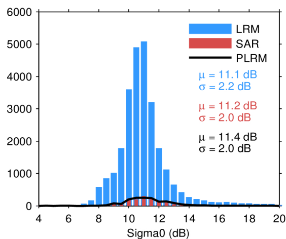
Figure 25. Histogram of flag-valid sigma0 over oceans and lakes for LRM (blue), SAR (red), and PLRM (black) for 19/06/2022. The mean ( \mu ) and standard deviation ( \sigma ) are also
