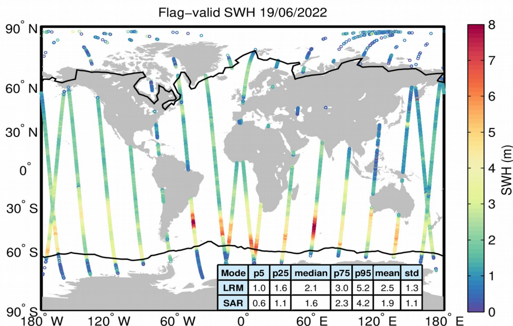
Figure 15. Geographical distribution of flag-valid SWH data over oceans and lakes for 19/06/2022. The statistical values shown in the table refer to the SWH in m and are calculated separately for LRM and SAR regions. Measurements taken over polar polygons
