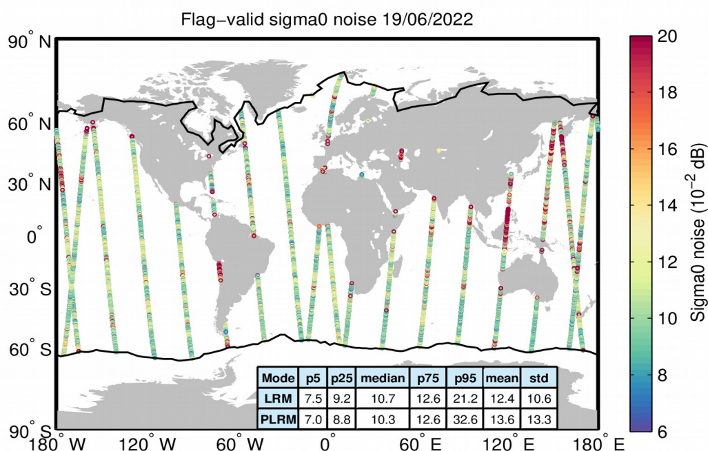
Figure 26. Geographical distribution of flag-valid 20-Hz sigma0 measurement noise over oceans and lakes for LRM/SAR (top) and LRM/PLRM (bottom) and for 19/06/2022. The statistical values shown in the table refer to the sigma0 noise and are calculated separately for LRM and SAR/PLRM regions. Measurements taken over polar polygons have been excluded from the computation of the statistical values. The black lines mark the outer limit of the Arctic and Antarctic polar polygons.
