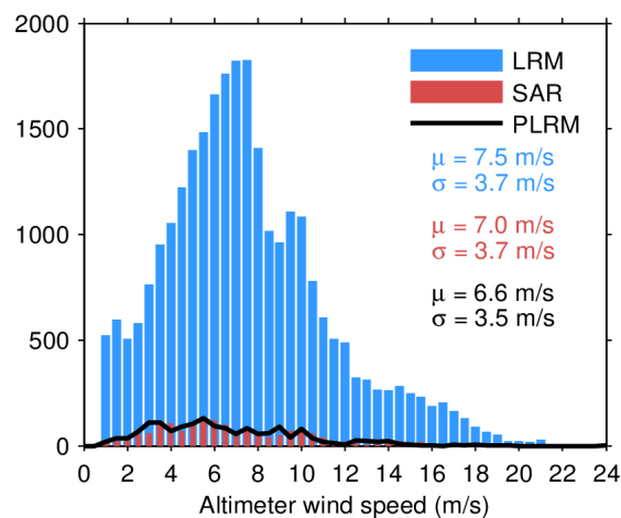
Figure 35. Histogram of science-valid wind over oceans and lakes for LRM (blue), SAR (red), and PLRM (black) for 19/06/2022. The mean ( \mu ) and standard deviation ( \sigma ) are also shown. Note that values larger than 24 m/s are excluded from the histogram for the sake of readability but not from the computation of \mu and \sigma .
