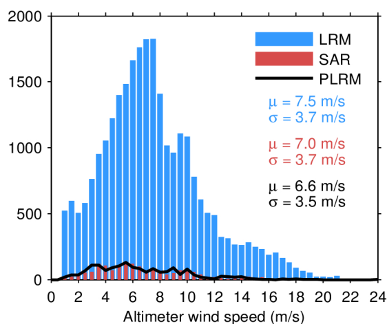
Figure 33. Histogram of flag-valid wind over oceans and lakes for LRM (blue), SAR (red), and PLRM (black) for 19/06/2022. The mean ( \mu ) and standard deviation ( \sigma ) are also shown. Note that values larger than 24 m/s are excluded from the histogram for the sake of readability but not from the computation of \mu and \sigma .
