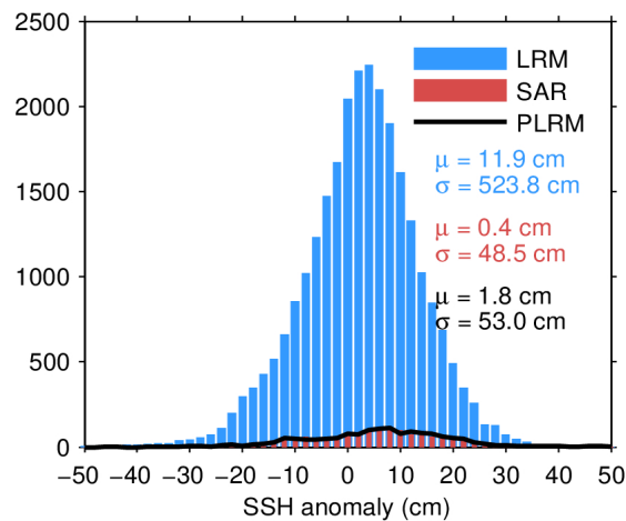
Figure 7. Histogram of flag-valid SSH anomaly over oceans and lakes for LRM (blue), SAR (red), and PLRM (black) for 19/06/2022. The mean ( \mu ) and standard deviation ( \sigma ) are also shown. Note that values outside [-50 50] cm are excluded from the histogram for the sake of readability but not from the computation of \mu and \sigma .
