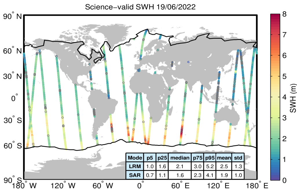
Figure 19. Geographical distribution of science-valid SWH data over oceans and lakes for 19/06/2022. The statistical values shown in the table refer to the SWH in m and are calculated separately for LRM and SAR regions. The black lines mark the outer limit of the Arctic and Antarctic polar polygons. Gray circles denote records that have been rejected based on the editing criteria described in Table 3.
