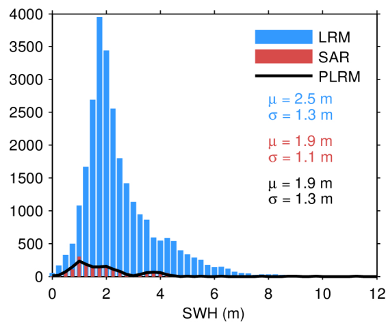
Figure 17. Histogram of flag-valid SWH over oceans and lakes for LRM (blue), SAR (red), and PLRM (black) for 19/06/2022. The mean ( \mu ) and standard deviation ( \sigma ) are also shown. Note that values larger than 12 m are excluded from the histogram for the sake of readability but not from the computation of \mu and \sigma .
