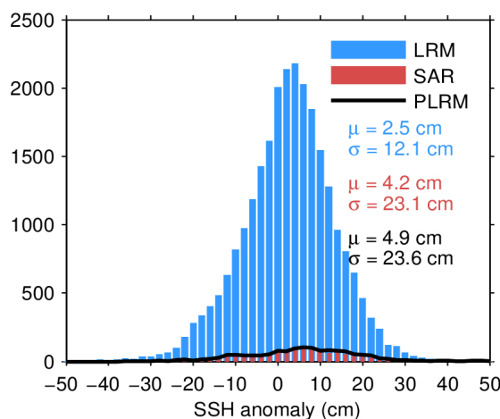
Figure 11. Histogram of science-valid SSH anomaly over oceans and lakes for LRM (blue), SAR (red), and PLRM (black) for 19/06/2022. The mean ( \mu ) and standard deviation ( \sigma ) are also shown. Note that values outside [-50, 50] cm are excluded from the histogram for the sake of readability but not from the computation of \mu and \sigma .
