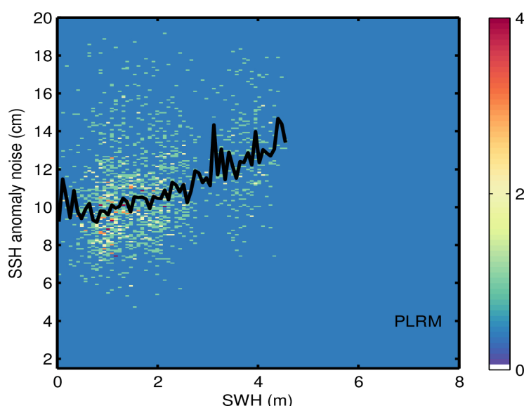
Figure 9. 2D histogram showing flag-valid SSH anomaly noise as a function of SWH for LRM (top), SAR (middle), and PLRM (bottom) for 19/06/2022. The black line denotes the median SSH anomaly noise as a function of SWH.
