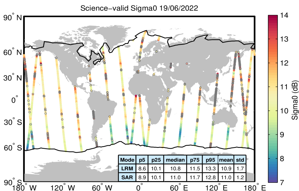
Figure 27. Geographical distribution of science-valid sigma0 data over oceans and lakes for 19/06/2022. The statistical values shown in the table refer to the sigma0 in dB and are calculated separately for LRM and SAR regions. The black lines mark the outer limit of the Arctic and Antarctic polar polygons. Gray circles denote records that have been rejected based on the editing criteria described in Table 4.
