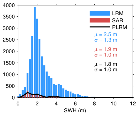
Figure 20. Histogram of science-valid SWH over oceans and lakes for LRM (blue), SAR (red), and PLRM (black) for 19/06/2022. The mean ( \mu ) and standard deviation ( \sigma ) are also shown. Note that values larger than 12 m are excluded from the histogram for the sake of readability but not from the computation of \mu and \sigma .
