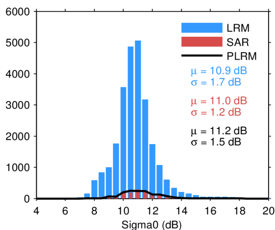
Figure 28. Histogram of science-valid sigma0 over oceans and lakes for LRM (blue), SAR (red), and PLRM (black) for 19/06/2022. The mean ( \mu ) and standard deviation ( \sigma ) are also shown. Note that values outside [4 20] dB are excluded from the histogram for the sake of readability but not from the computation of \mu and \sigma .
