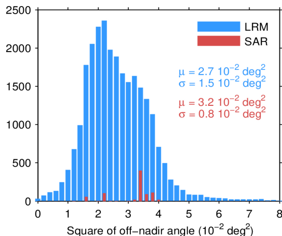
Figure 39. Histogram of flag-valid mispointing over oceans and lakes for LRM (blue) and SAR (red) for 19/06/2022. Only positive values have been considered. The mean ( \mu ) and standard deviation ( \sigma ) are also shown. Note that values larger than 8 \cdot 10^{-2} \text{ deg}^2 are excluded from the histogram for the sake of readability but not from the computation of \mu and \sigma .
