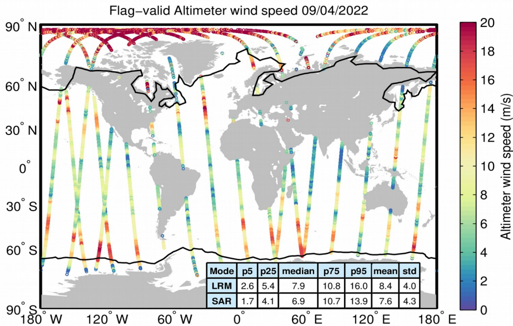
Figure 31. Geographical distribution of flag-valid wind data over oceans and lakes for 09/04/2022. The statistical values shown in the table refer to the wind in m/s and are calculated separately for LRM and SAR regions. Measurements taken over polar polygons have been excluded from the computation of the statistical values. The black lines mark the outer limit of the Arctic and Antarctic polar polygons.
