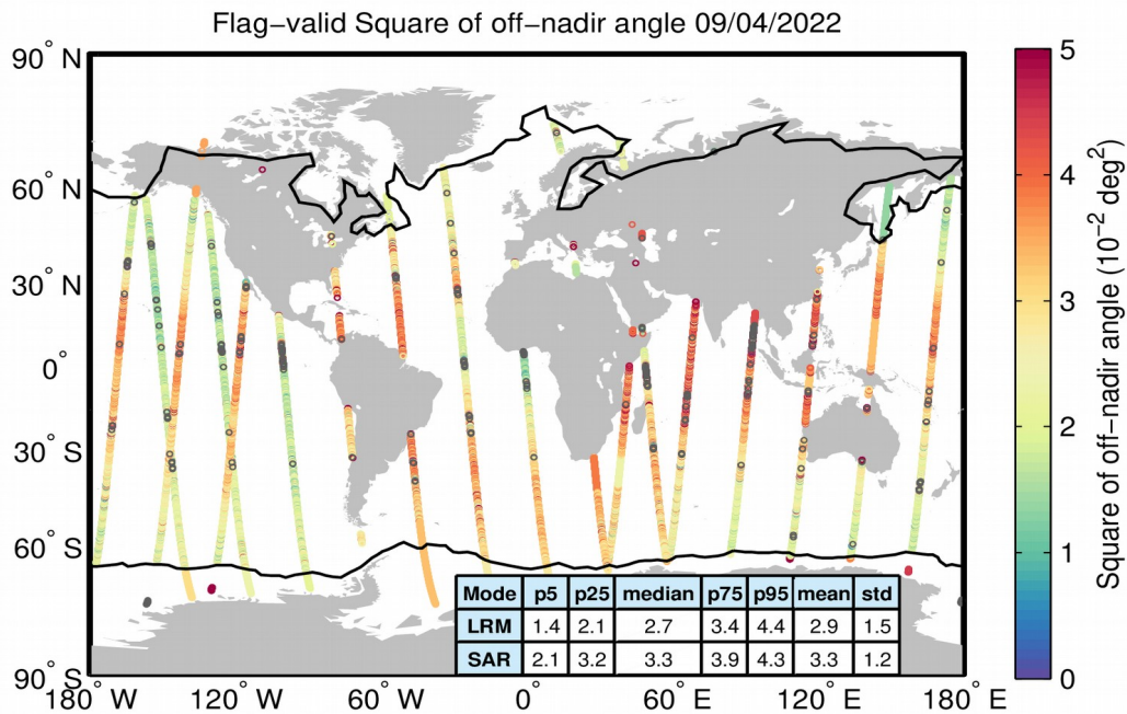
Figure 37. Geographical distribution of flag-valid mispointing data over oceans and lakes for 09/04/2022. The statistical values shown in the table refer to the mispointing in 10^{-2} \text{ deg}^2 and are calculated separately for LRM and SAR regions. Measurements taken over polar polygons have been excluded from the computation of the statistical values. The black lines mark the outer limit of the Arctic and Antarctic polar polygons. Gray circles denote negative values.
