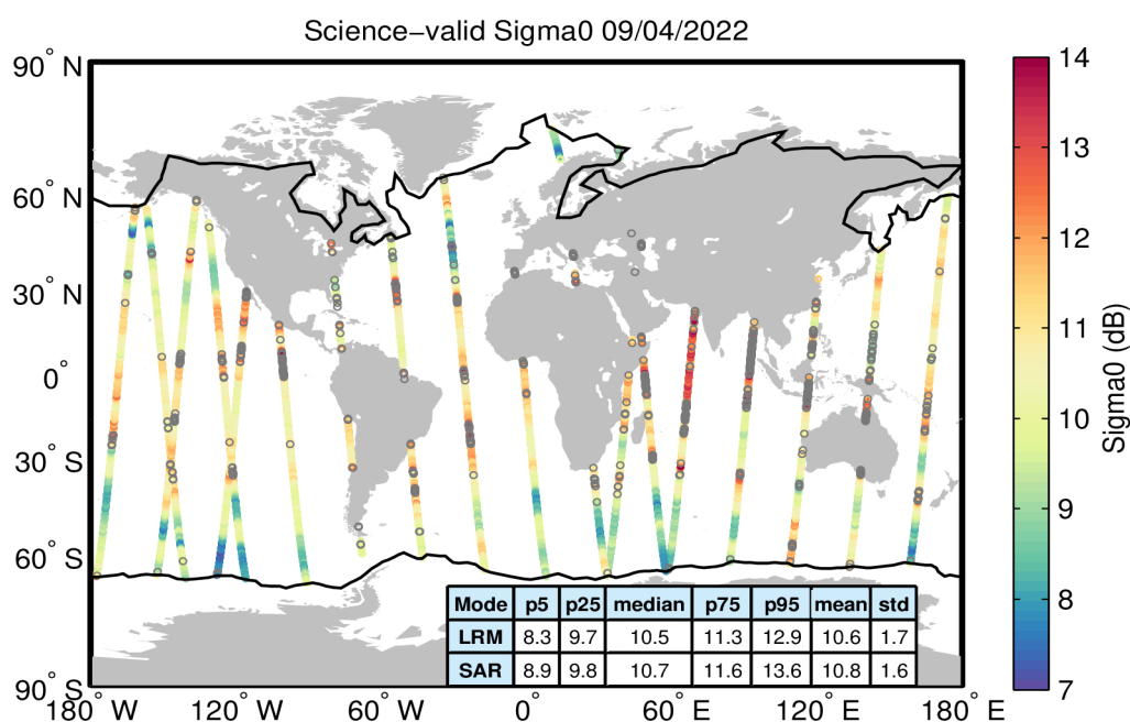
Figure 27. Geographical distribution of science-valid sigma0 data over oceans and lakes for 09/04/2022. The statistical values shown in the table refer to the sigma0 in dB and are calculated separately for LRM and SAR regions. The black lines mark the outer limit of the Arctic and Antarctic polar polygons. Gray circles denote records that have been rejected based on the editing criteria described in Table 4.
