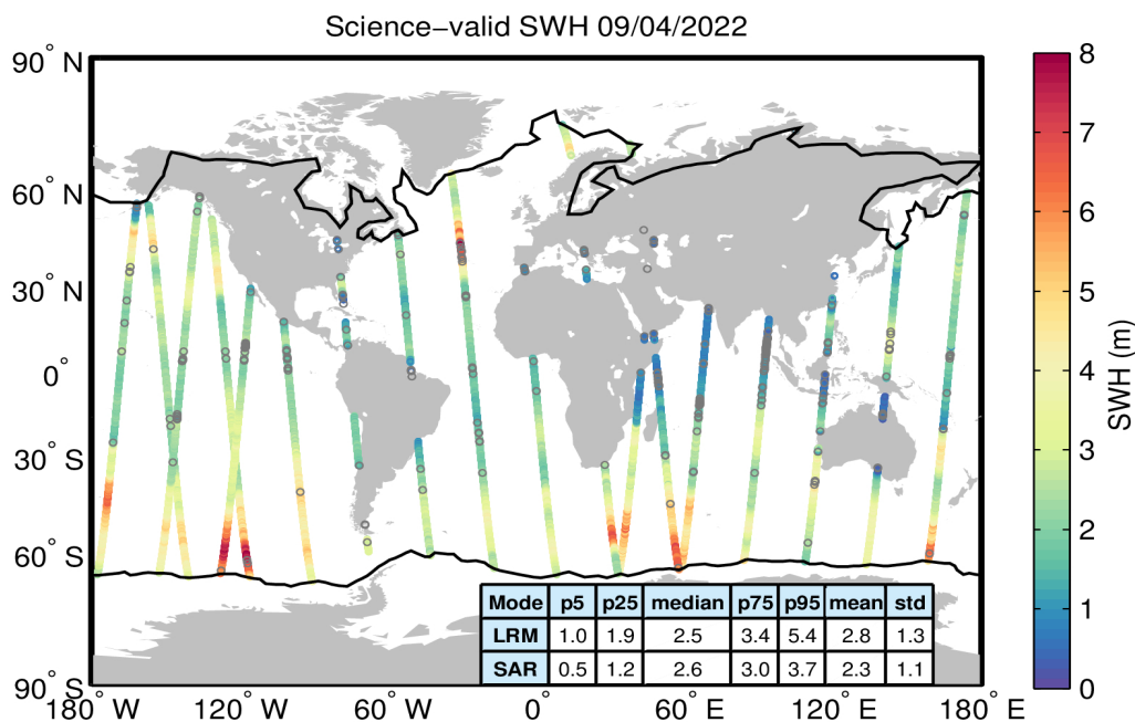
Figure 19. Geographical distribution of science-valid SWH data over oceans and lakes for 09/04/2022. The statistical values shown in the table refer to the SWH in m and are calculated separately for LRM and SAR regions. The black lines mark the outer limit of the Arctic and Antarctic polar polygons. Gray circles denote records that have been rejected based on the editing criteria described in Table 3.
