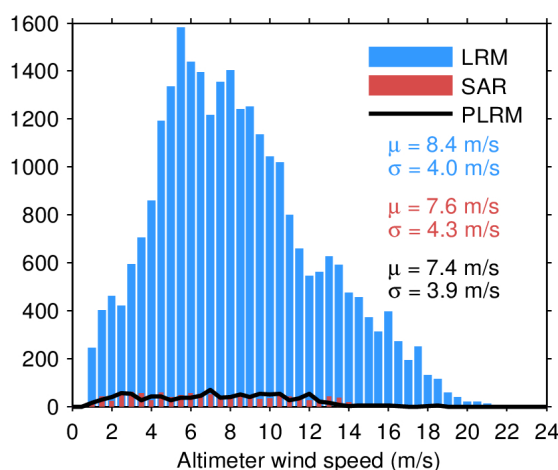
Figure 35. Histogram of science-valid wind over oceans and lakes for LRM (blue), SAR (red), and PLRM (black) for 09/04/2022. The mean ( \mu ) and standard deviation ( \sigma ) are also shown. Note that values larger than 24 m/s are excluded from the histogram for the sake of readability but not from the computation of \mu and \sigma .
