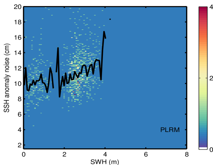
Figure 9. 2D histogram showing flag-valid SSH anomaly noise as a function of SWH for LRM (top), SAR (middle), and PLRM (bottom) for 09/04/2022. The black line denotes the median SSH anomaly noise as a function of SWH.
