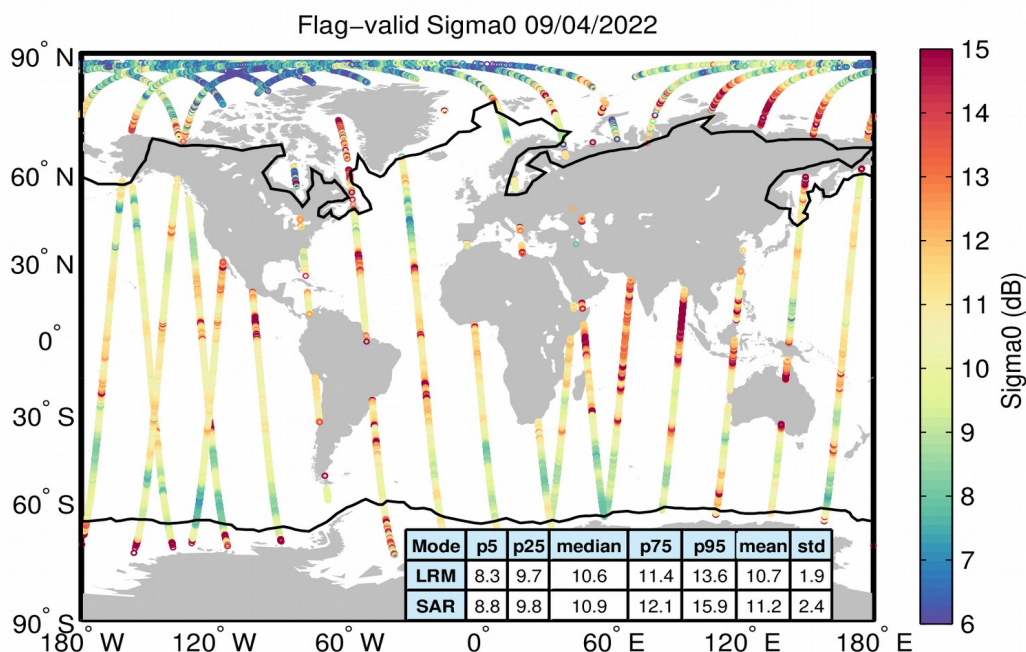
Figure 23. Geographical distribution of flag-valid sigma0 data over oceans and lakes for 09/04/2022. The statistical values shown in the table refer to the sigma0 in dB and are calculated separately for LRM and SAR regions. Measurements taken over polar polygons
