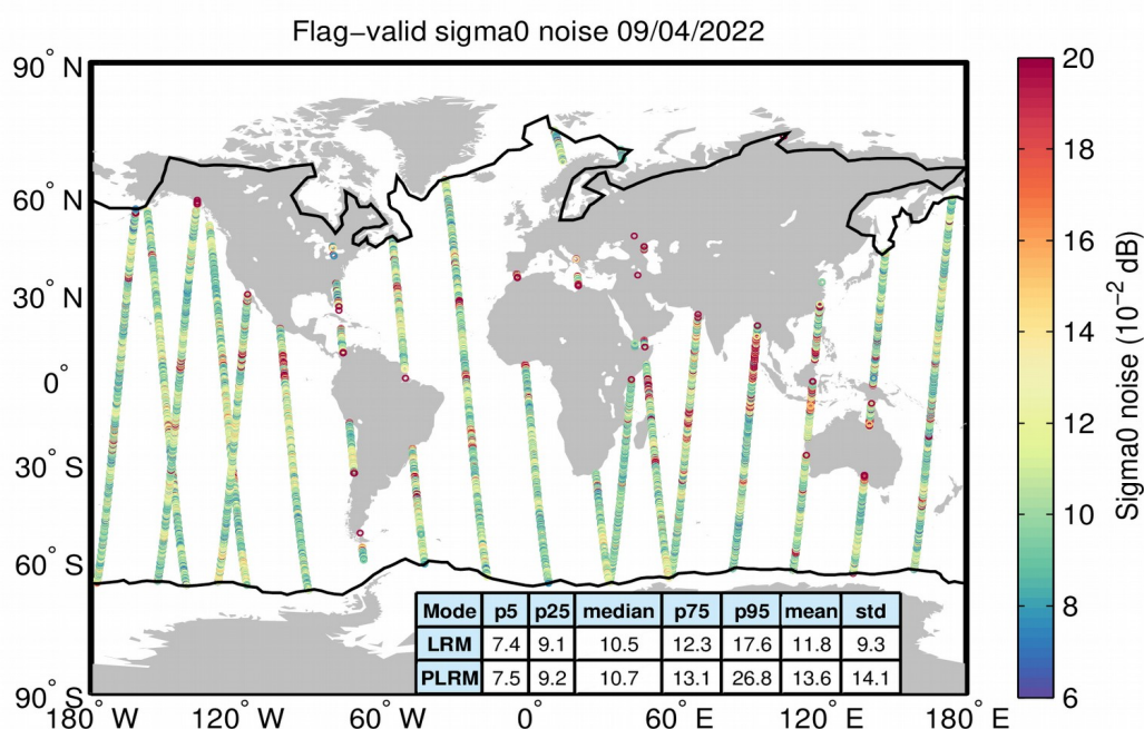
Figure 26. Geographical distribution of flag-valid 20-Hz sigma0 measurement noise over oceans and lakes for LRM/SAR (top) and LRM/PLRM (bottom) and for 09/04/2022. The statistical values shown in the table refer to the sigma0 noise and are calculated separately for LRM and SAR/PLRM regions. Measurements taken over polar polygons have been excluded from the computation of the statistical values. The black lines mark the outer limit of the Arctic and Antarctic polar polygons.
