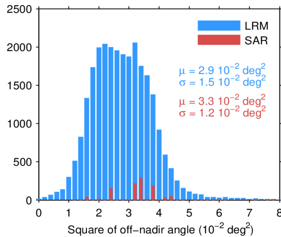
Figure 39. Histogram of flag-valid mispointing over oceans and lakes for LRM (blue) and SAR (red) for 09/04/2022. Only positive values have been considered. The mean ( \mu ) and standard deviation ( \sigma ) are also shown. Note that values larger than 8 \cdot 10^{-2} \text{ deg}^2 are excluded from the histogram for the sake of readability but not from the computation of \mu and \sigma .
