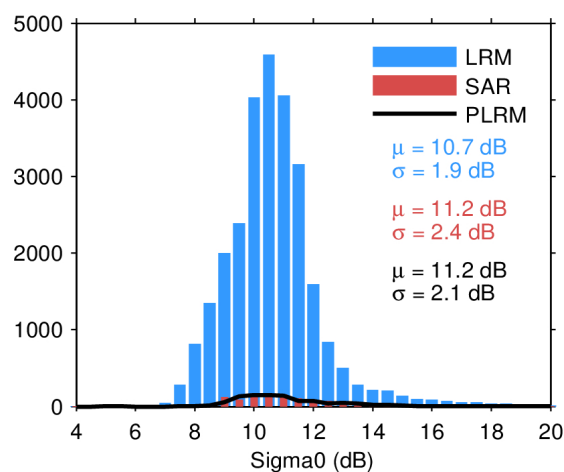
Figure 25. Histogram of flag-valid sigma0 over oceans and lakes for LRM (blue), SAR (red), and PLRM (black) for 09/04/2022. The mean ( \mu ) and standard deviation ( \sigma ) are also
