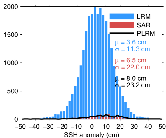
Figure 11. Histogram of science-valid SSH anomaly over oceans and lakes for LRM (blue), SAR (red), and PLRM (black) for 09/04/2022. The mean ( \mu ) and standard deviation ( \sigma ) are also shown. Note that values outside [-50, 50] cm are excluded from the histogram for the sake of readability but not from the computation of \mu and \sigma .
