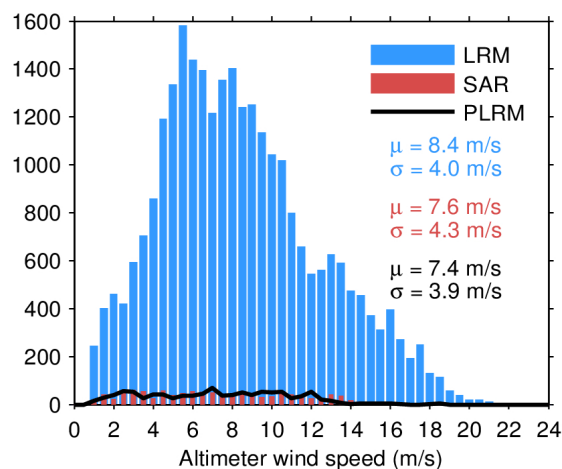
Figure 33. Histogram of flag-valid wind over oceans and lakes for LRM (blue), SAR (red), and PLRM (black) for 09/04/2022. The mean ( \mu ) and standard deviation ( \sigma ) are also shown. Note that values larger than 24 m/s are excluded from the histogram for the sake of readability but not from the computation of \mu and \sigma .
