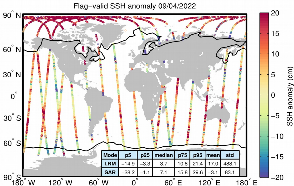
Figure 5. Geographical distribution of flag-valid 1-Hz SSH anomaly data over oceans and lakes for 09/04/2022. The statistical values shown in the table refer to the SSH anomaly in cm and are calculated separately for LRM and SAR regions. Measurements taken over polar polygons have been excluded from the computation of the statistical values. The black lines mark the outer limit of the Arctic and Antarctic polar polygons.
