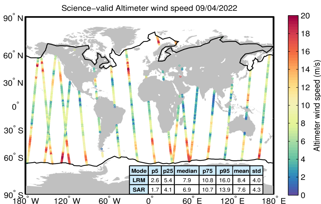
Figure 34. Geographical distribution of science-valid wind data over oceans and lakes for 09/04/2022. The statistical values shown in the table refer to the wind in m/s and are calculated separately for LRM and SAR regions. The black lines mark the outer limit of the Arctic and Antarctic polar polygons. Gray circles denote records that have been rejected based on the editing criteria described in Table 5.
