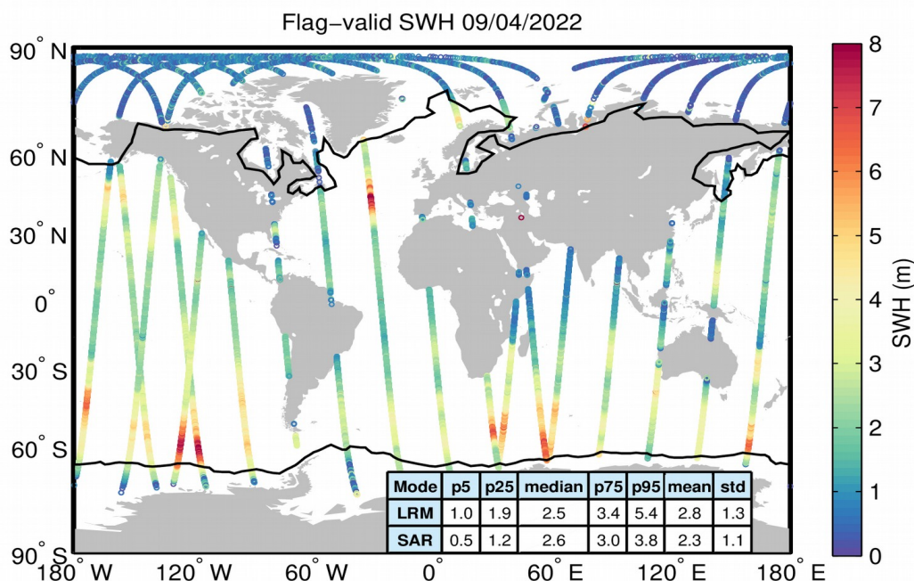
Figure 15. Geographical distribution of flag-valid SWH data over oceans and lakes for 09/04/2022. The statistical values shown in the table refer to the SWH in m and are calculated separately for LRM and SAR regions. Measurements taken over polar polygons
