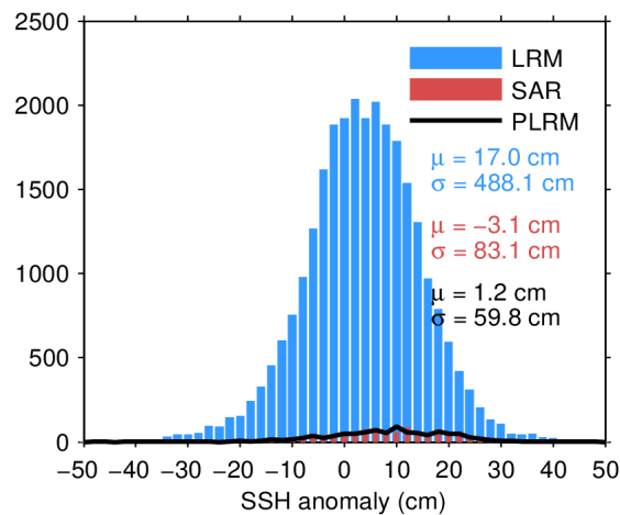
Figure 7. Histogram of flag-valid SSH anomaly over oceans and lakes for LRM (blue), SAR (red), and PLRM (black) for 09/04/2022. The mean ( \mu ) and standard deviation ( \sigma ) are also shown. Note that values outside [-50 50] cm are excluded from the histogram for the sake of readability but not from the computation of \mu and \sigma .
