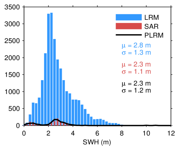
Figure 17. Histogram of flag-valid SWH over oceans and lakes for LRM (blue), SAR (red), and PLRM (black) for 09/04/2022. The mean ( \mu ) and standard deviation ( \sigma ) are also shown. Note that values larger than 12 m are excluded from the histogram for the sake of readability but not from the computation of \mu and \sigma .
