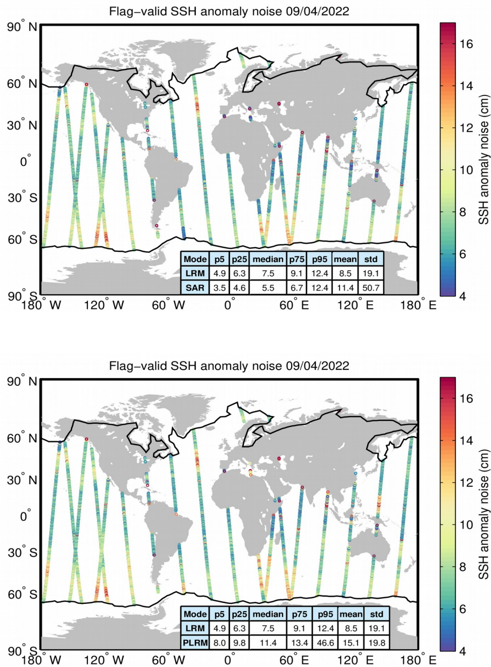
Figure 8. Geographical distribution of flag-valid 20-Hz SSH anomaly measurement noise over oceans and lakes for LRM/SAR (top) and LRM/PLRM (bottom) and for 09/04/2022. The statistical values shown in the tables refer to the SSH anomaly noise and are calculated separately for LRM and SAR/PLRM regions. Measurements taken over polar polygons have been excluded from the computation of the statistical values. The black lines mark the outer limit of the Arctic and Antarctic polar polygons.
