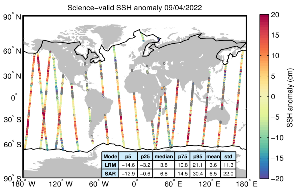
Figure 10. Geographical distribution of science-valid SSH anomaly data over oceans and lakes for 09/04/2022. The statistical values shown in the table refer to the SSH anomaly in cm and are calculated separately for LRM and SAR regions. The black lines mark the outer limit of the Arctic and Antarctic polar polygons. Gray circles denote records that have been rejected based on the editing criteria described in Table 2.
