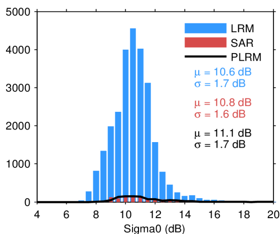
Figure 28. Histogram of science-valid sigma0 over oceans and lakes for LRM (blue), SAR (red), and PLRM (black) for 09/04/2022. The mean ( \mu ) and standard deviation ( \sigma ) are also shown. Note that values outside [4 20] dB are excluded from the histogram for the sake of readability but not from the computation of \mu and \sigma .
