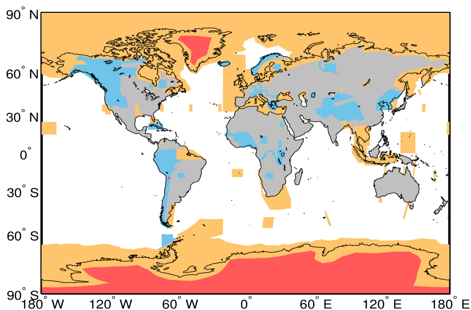
Figure A1. Extent of the regions defining the geographical mode mask for 09/04/2022. The regions where SAR, and SARin are operated are denoted by the orange and blue polygons, respectively. LRM is operated over areas of the continental ice sheets (red polygons) and over oceans and land not covered by other modes.
