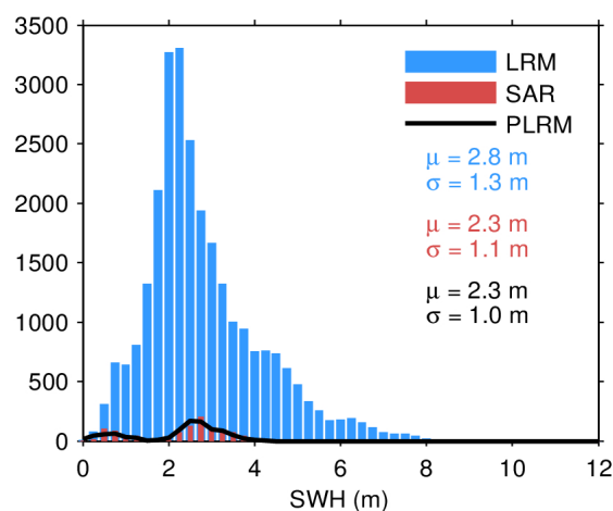
Figure 20. Histogram of science-valid SWH over oceans and lakes for LRM (blue), SAR (red), and PLRM (black) for 09/04/2022. The mean ( \mu ) and standard deviation ( \sigma ) are also shown. Note that values larger than 12 m are excluded from the histogram for the sake of readability but not from the computation of \mu and \sigma .
