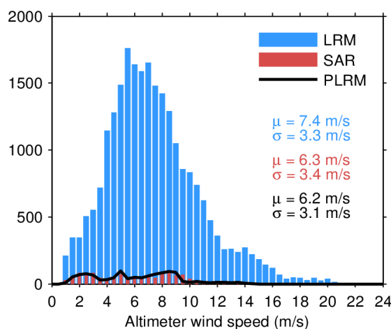
Figure 33. Histogram of flag-valid wind over oceans and lakes for LRM (blue), SAR (red), and PLRM (black) for 24/01/2022. The mean ( \mu ) and standard deviation ( \sigma ) are also shown. Note that values larger than 24 m/s are excluded from the histogram for the sake of readability but not from the computation of \mu and \sigma .
