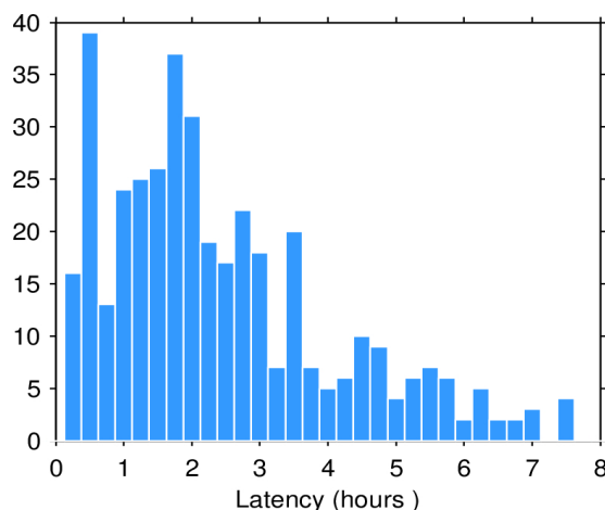
Figure 2. Histogram of the data latency for 24/01/2022. The y-axis denotes the number of files that are made available with a delay of x-hours with respect to the mean time of the records stored in the file.
