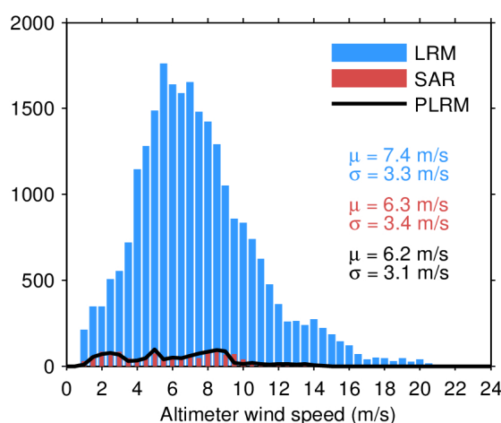
Figure 35. Histogram of science-valid wind over oceans and lakes for LRM (blue), SAR (red), and PLRM (black) for 24/01/2022. The mean ( \mu ) and standard deviation ( \sigma ) are also shown. Note that values larger than 24 m/s are excluded from the histogram for the sake of readability but not from the computation of \mu and \sigma .
