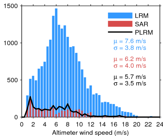
Figure 35. Histogram of science-valid wind over oceans and lakes for LRM (blue), SAR (red), and PLRM (black) for 11/08/2020. The mean ( \mu ) and standard deviation ( \sigma ) are also shown. Note that values larger than 24 m/s are excluded from the histogram for the sake of readability but not from the computation of \mu and \sigma .
