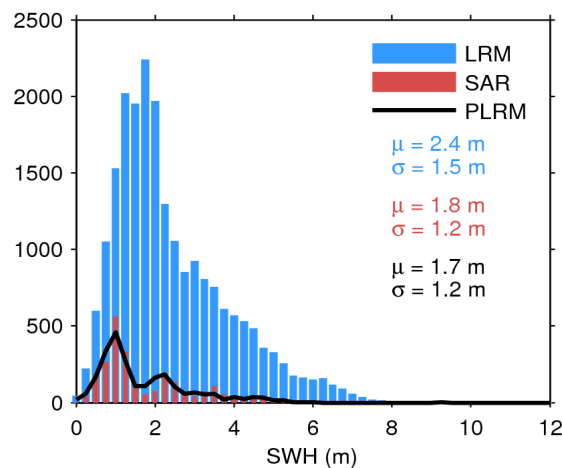
Figure 17. Histogram of flag-valid SWH over oceans and lakes for LRM (blue), SAR (red), and PLRM(black) for 11/08/2020. The mean ( \mu ) and standard deviation ( \sigma ) are also shown. Note that values larger than 12 m are excluded from the histogram for the sake of readability but not from the computation of \mu and \sigma .
