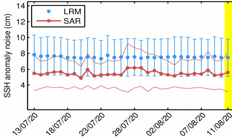
Figure 13. Average science-valid SSH anomaly noise for LRM (blue dot) and SAR (red dot). The corresponding standard deviation (blue error bar and thin red lines, respectively) for each day in last 30-day window is also shown. The yellow shading highlights the day analyzed in this report.
