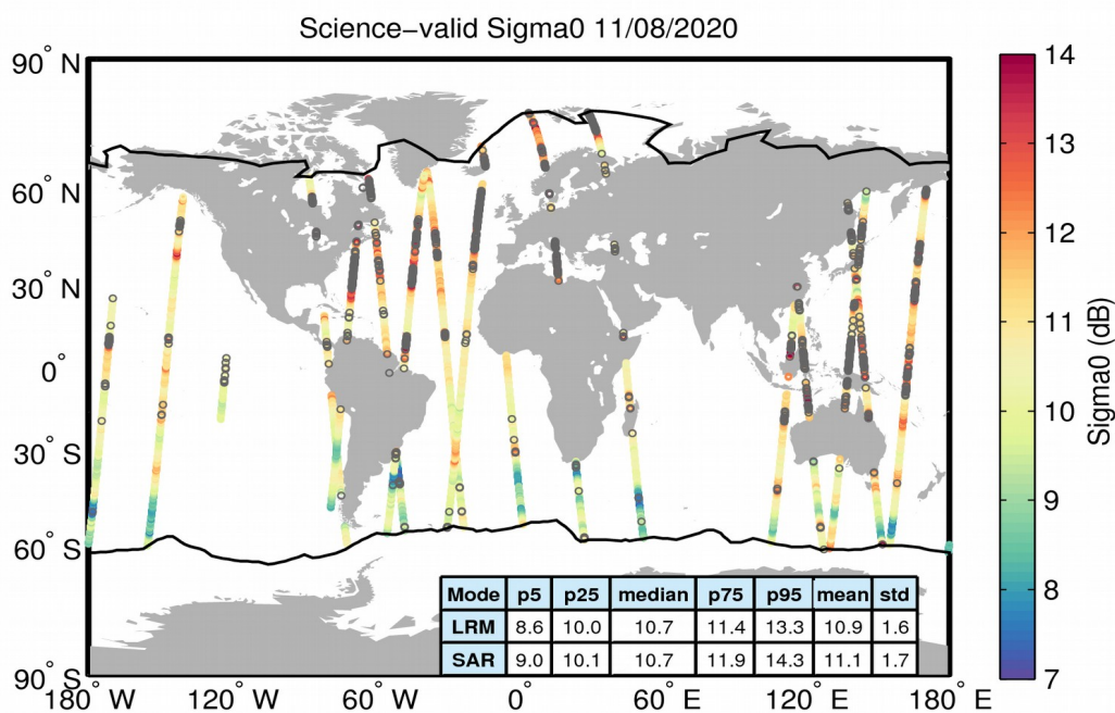
Figure 27. Geographical distribution of science-valid sigma0 data over oceans and lakes for 11/08/2020. The statistical values shown in the table refer to the sigma0 in dB and are calculated separately for LRM and SAR regions. The black lines mark the outer limit of the Arctic and Antarctic polar polygons. Gray circles denote records that have been rejected based on the editing criteria described in Table 4.
