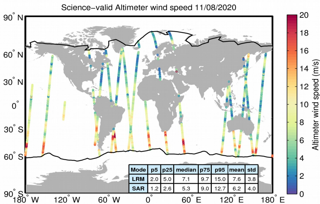
Figure 34. Geographical distribution of science-valid wind data over oceans and lakes for 11/08/2020. The statistical values shown in the table refer to the wind in m/s and are calculated separately for LRM and SAR regions. The black lines mark the outer limit of the Arctic and Antarctic polar polygons. Gray circles denote records that have been rejected based on the editing criteria described in Table 5.
