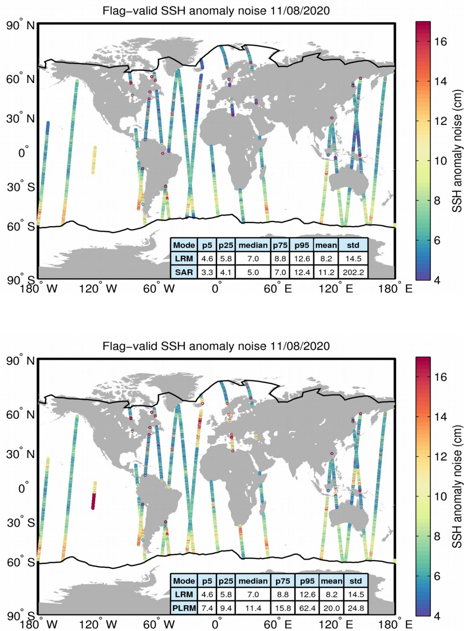
Figure 8. Geographical distribution of flag-valid 20-Hz SSH anomaly measurement noise over oceans and lakes for LRM/SAR (top) and LRM/PLRM (bottom) and for 11/08/2020. The statistical values shown in the tables refer to the SSH anomaly noise and are calculated separately for LRM and SAR/PLRM regions. Measurements taken over polar polygons have been excluded from the computation of the statistical values. The black lines mark the outer limit of the Arctic and Antarctic polar polygons.
