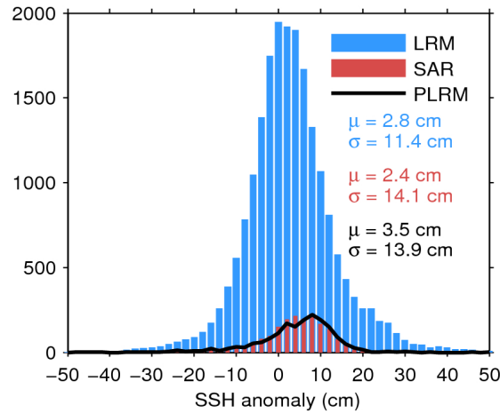
Figure 11. Histogram of science-valid SSH anomaly over oceans and lakes for LRM (blue), SAR (red), and PLRM (black) for 11/08/2020. The mean ( \mu ) and standard deviation ( \sigma ) are also shown. Note that values outside [-50\ 50] cm are excluded from the histogram for the sake of readability but not from the computation of \mu and \sigma .
