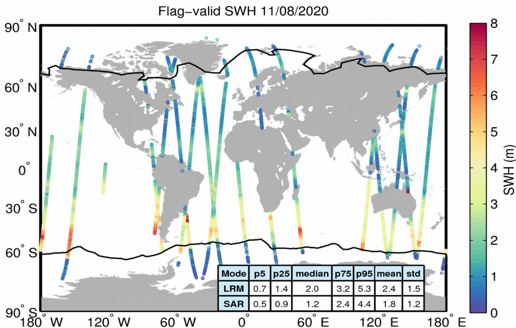
Figure 15. Geographical distribution of flag-valid SWH data over oceans and lakes for 11/08/2020. The statistical values shown in the table refer to the SWH in m and are calculated separately for LRM and SAR regions. Measurements taken over polar polygons
