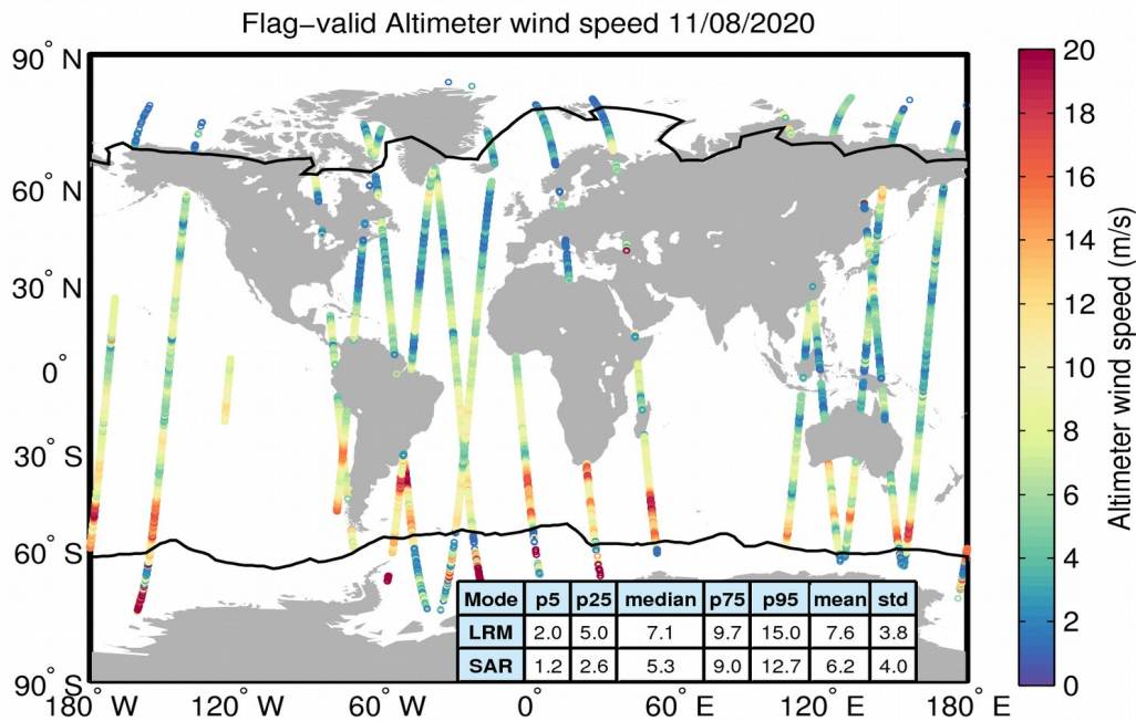
Figure 31. Geographical distribution of flag-valid wind data over oceans and lakes for 11/08/2020. The statistical values shown in the table refer to the wind in m/s and are calculated separately for LRM and SAR regions. Measurements taken over polar polygons have been excluded from the computation of the statistical values. The black lines mark the outer limit of the Arctic and Antarctic polar polygons.
