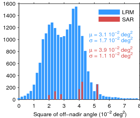
Figure 39. Histogram of flag-valid mispointing over oceans and lakes for LRM (blue) and SAR (red) for 11/08/2020. Only positive values have been considered. The mean ( \mu ) and standard deviation ( \sigma ) are also shown. Note that values larger than 8 \cdot 10^{-2} \text{ deg}^2 are excluded from the histogram for the sake of readability but not from the computation of \mu and \sigma .
