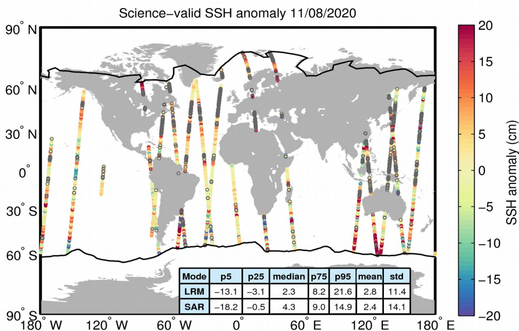
Figure 10. Geographical distribution of science-valid SSH anomaly data over oceans and lakes for 11/08/2020. The statistical values shown in the table refer to the SSH anomaly in cm and are calculated separately for LRM and SAR regions. The black lines mark the outer limit of the Arctic and Antarctic polar polygons. Gray circles denote records that have been rejected based on the editing criteria described in Table 2.
