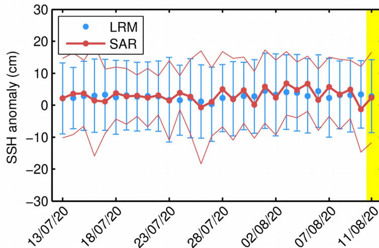
Figure 12. Mean science-valid SSH anomaly for LRM (blue dot) and SAR (red dot). The corresponding standard deviation (blue error bar and thin red lines, respectively) for each day in last 30-day window is also shown. The yellow shading highlights the day analyzed in this report.
