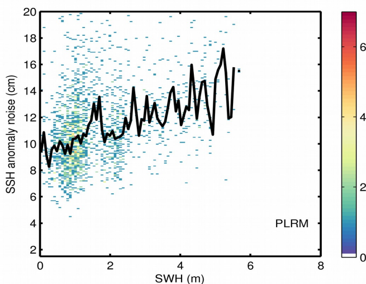
Figure 9. 2D histogram showing flag-valid SSH anomaly noise as a function of SWH for LRM (top), SAR (middle), and PLRM (bottom) for 11/08/2020. The black line denotes the median SSH anomaly noise as a function of SWH.
