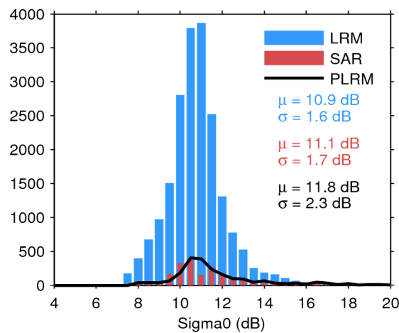
Figure 28. Histogram of science-valid sigma0 over oceans and lakes for LRM (blue), SAR (red), and PLRM (black) for 11/08/2020. The mean ( \mu ) and standard deviation ( \sigma ) are also shown. Note that values outside [4 20] dB are excluded from the histogram for the sake of readability but not from the computation of \mu and \sigma .
