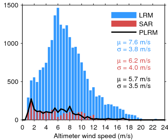
Figure 33. Histogram of flag-valid wind over oceans and lakes for LRM (blue), SAR (red), and PLRM (black) for 11/08/2020. The mean ( \mu ) and standard deviation ( \sigma ) are also shown. Note that values larger than 24 m/s are excluded from the histogram for the sake of readability but not from the computation of \mu and \sigma .
