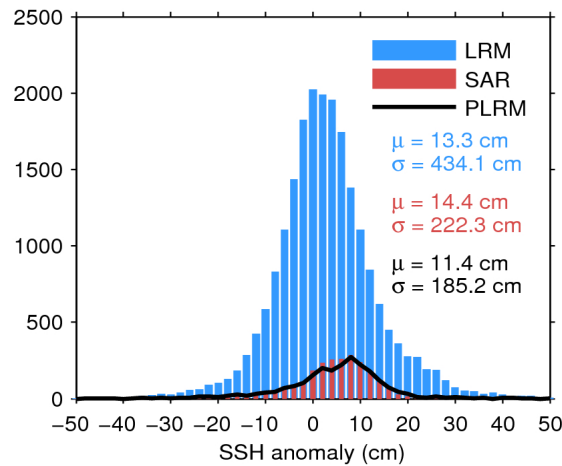
Figure 7. Histogram of flag-valid SSH anomaly over oceans and lakes for LRM (blue), SAR (red), and PLRM (black) for 11/08/2020. The mean ( \mu ) and standard deviation ( \sigma ) are also shown. Note that values outside [-50 50] cm are excluded from the histogram for the sake of readability but not from the computation of \mu and \sigma .
