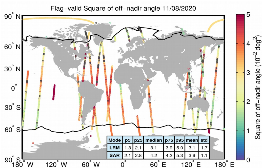
Figure 37. Geographical distribution of flag-valid mispointing data over oceans and lakes for 11/08/2020. The statistical values shown in the table refer to the mispointing in 10^{-2} deg 2 and are calculated separately for LRM and SAR regions. Measurements taken over polar polygons have been excluded from the computation of the statistical values. The black lines mark the outer limit of the Arctic and Antarctic polar polygons. Gray circles denote negative values.
