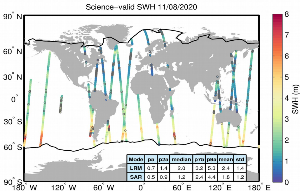
Figure 19. Geographical distribution of science-valid SWH data over oceans and lakes for 11/08/2020. The statistical values shown in the table refer to the SWH in m and are calculated separately for LRM and SAR regions. The black lines mark the outer limit of the Arctic and Antarctic polar polygons. Gray circles denote records that have been rejected based on the editing criteria described in Table 3.
