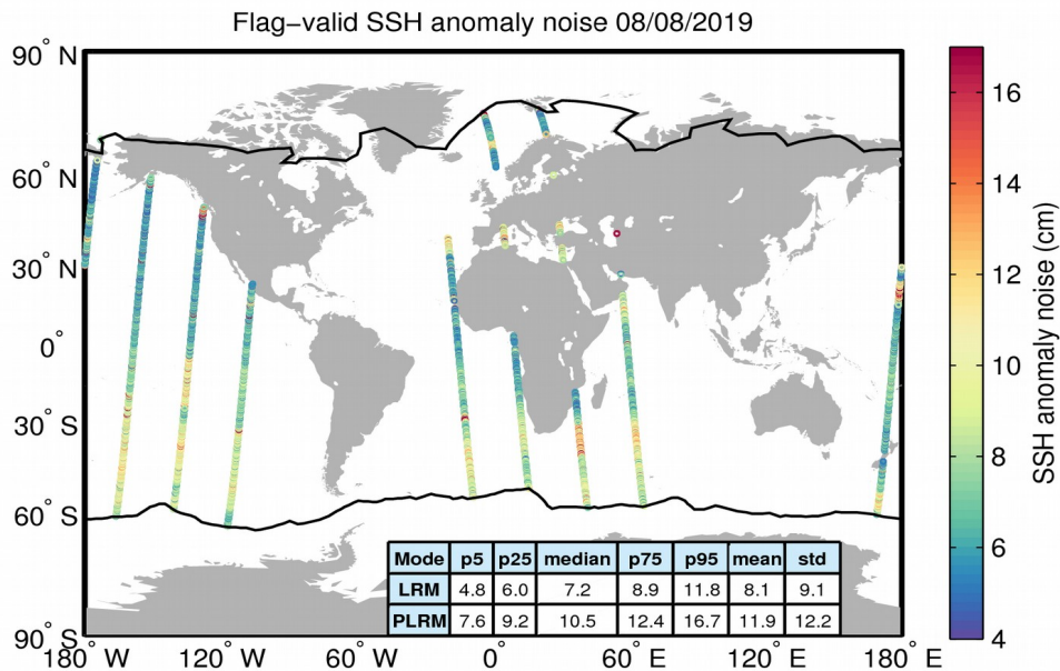
Figure 8. Geographical distribution of flag-valid 20-Hz SSH anomaly measurement noise over oceans and lakes for LRM/SAR (top) and LRM/PLRM (bottom) and for 08/08/2019. The statistical values shown in the tables refer to the SSH anomaly noise and are calculated separately for LRM and SAR/PLRM regions. Measurements taken over polar
