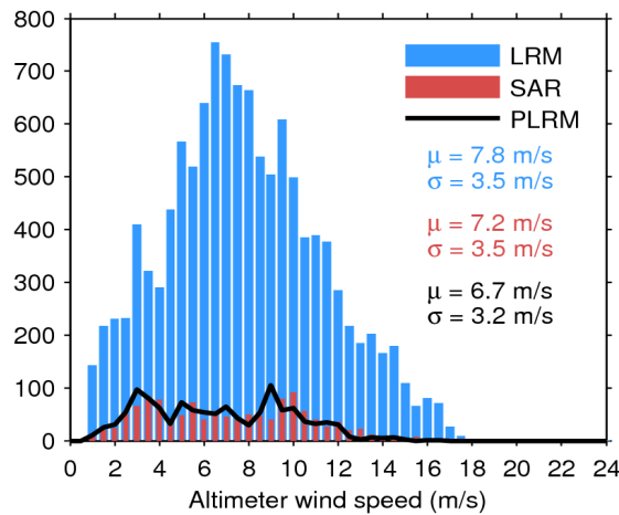
Figure 33. Histogram of flag-valid wind over oceans and lakes for LRM (blue), SAR (red), and PLRM (black) for 08/08/2019. The mean ( \mu ) and standard deviation ( \sigma ) are also shown. Note that values larger than 24 m/s are excluded from the histogram for the sake of readability but not from the computation of \mu and \sigma .
