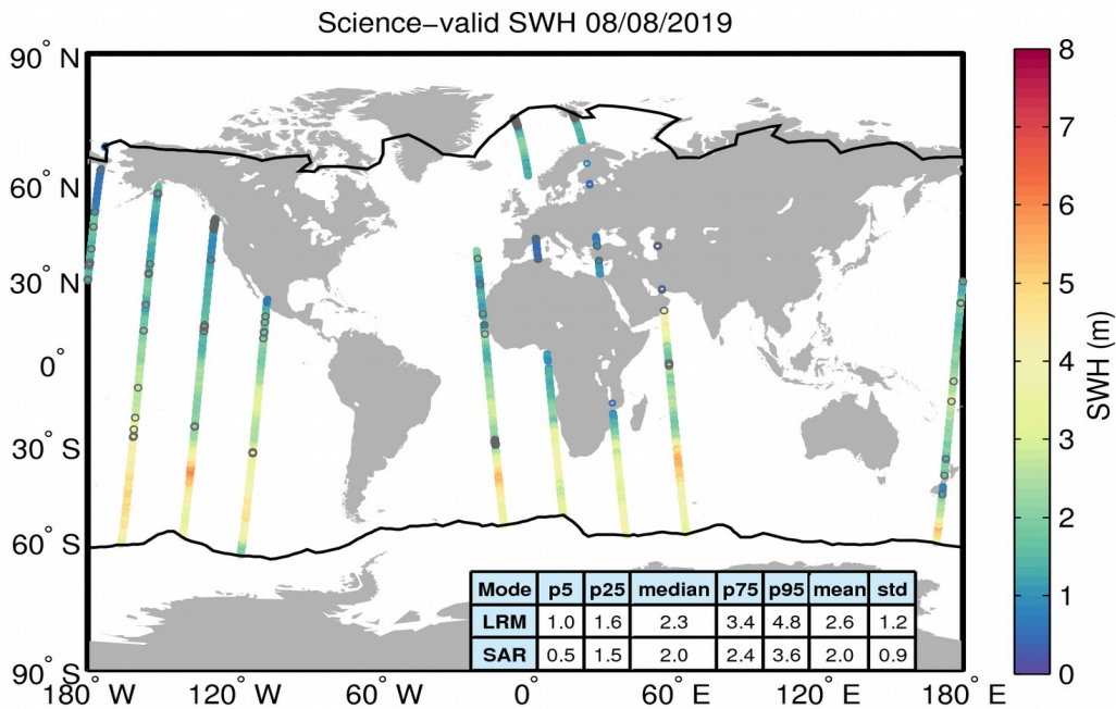
Figure 19. Geographical distribution of science-valid SWH data over oceans and lakes for 08/08/2019. The statistical values shown in the table refer to the SWH in m and are calculated separately for LRM and SAR regions. The black lines mark the outer limit of the Arctic and Antarctic polar polygons. Gray circles denote records that have been rejected based on the editing criteria described in Table 3.
