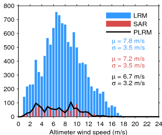
Figure 35. Histogram of science-valid wind over oceans and lakes for LRM (blue), SAR (red), and PLRM (black) for 08/08/2019. The mean ( \mu ) and standard deviation ( \sigma ) are also shown. Note that values larger than 24 m/s are excluded from the histogram for the sake of readability but not from the computation of \mu and \sigma .
