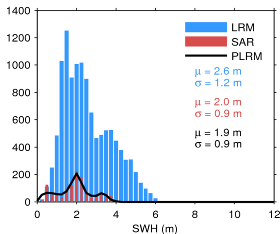
Figure 20. Histogram of science-valid SWH over oceans and lakes for LRM (blue), SAR (red), and PLRM (black) for 08/08/2019. The mean ( \mu ) and standard deviation ( \sigma ) are also
