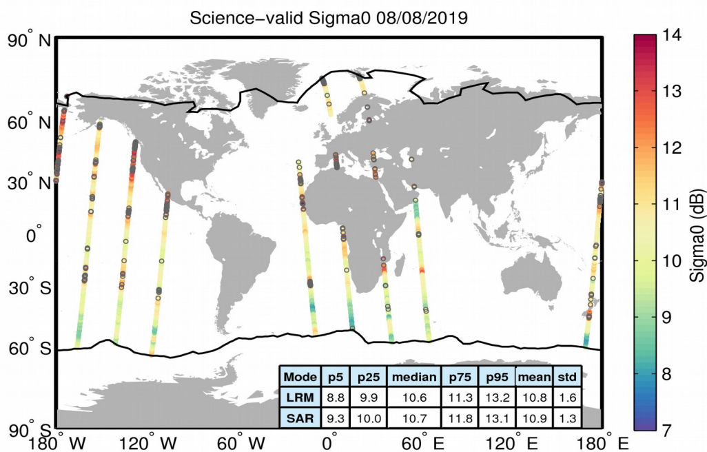
Figure 27. Geographical distribution of science-valid sigma0 data over oceans and lakes for 08/08/2019. The statistical values shown in the table refer to the sigma0 in dB and are calculated separately for LRM and SAR regions. The black lines mark the outer limit of the Arctic and Antarctic polar polygons. Gray circles denote records that have been rejected based on the editing criteria described in Table 4.
