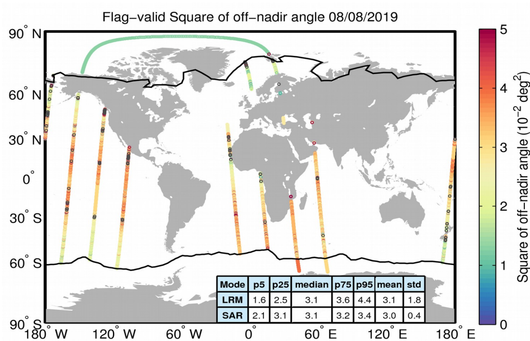
Figure 37. Geographical distribution of flag-valid mispointing data over oceans and lakes for 08/08/2019. The statistical values shown in the table refer to the mispointing in 10^{-2} deg 2 and are calculated separately for LRM and SAR regions. Measurements taken over polar polygons have been excluded from the computation of the statistical values. The black lines mark the outer limit of the Arctic and Antarctic polar polygons. Gray circles denote negative values.
