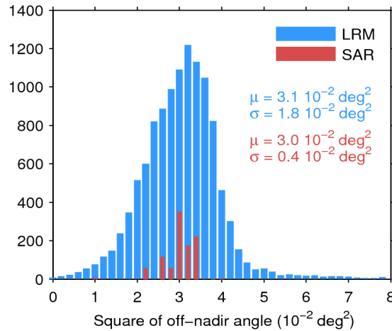
Figure 39. Histogram of flag-valid mispointing over oceans and lakes for LRM (blue) and SAR (red) for 08/08/2019. Only positive values have been considered. The mean ( \mu ) and standard deviation ( \sigma ) are also shown. Note that values larger than 8 \cdot 10^{-2} \text{ deg}^2 are excluded from the histogram for the sake of readability but not from the computation of \mu and \sigma .
