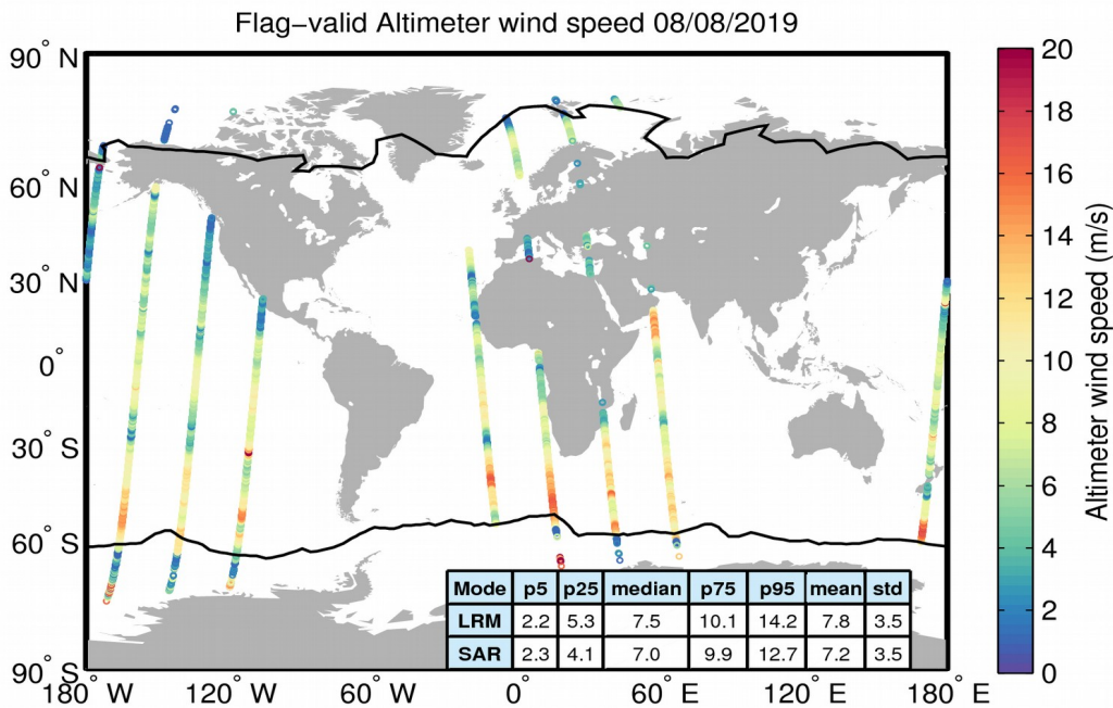
Figure 31. Geographical distribution of flag-valid wind data over oceans and lakes for 08/08/2019. The statistical values shown in the table refer to the wind in m/s and are calculated separately for LRM and SAR regions. Measurements taken over polar polygons have been excluded from the computation of the statistical values. The black lines mark the outer limit of the Arctic and Antarctic polar polygons.
