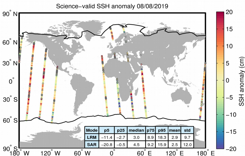
Figure 10. Geographical distribution of science-valid SSH anomaly data over oceans and lakes for 08/08/2019. The statistical values shown in the table refer to the SSH anomaly in cm and are calculated separately for LRM and SAR regions. The black lines mark the outer limit of the Arctic and Antarctic polar polygons. Gray circles denote records that have been rejected based on the editing criteria described in Table 2.
