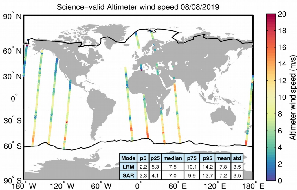
Figure 34. Geographical distribution of science-valid wind data over oceans and lakes for 08/08/2019. The statistical values shown in the table refer to the wind in m/s and are calculated separately for LRM and SAR regions. The black lines mark the outer limit of the Arctic and Antarctic polar polygons. Gray circles denote records that have been rejected based on the editing criteria described in Table 5.
