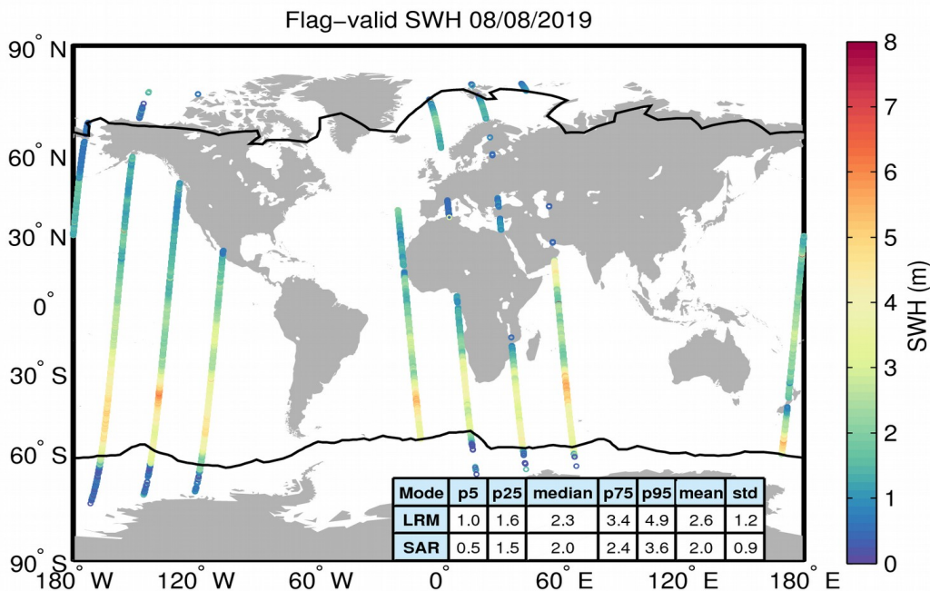
Figure 15. Geographical distribution of flag-valid SWH data over oceans and lakes for 08/08/2019. The statistical values shown in the table refer to the SWH in m and are calculated separately for LRM and SAR regions. Measurements taken over polar polygons
