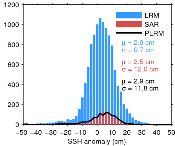
Figure 11. Histogram of science-valid SSH anomaly over oceans and lakes for LRM (blue), SAR (red), and PLRM (black) for 08/08/2019. The mean ( \mu ) and standard deviation ( \sigma ) are also shown. Note that values outside [-50\ 50] cm are excluded from the histogram for the sake of readability but not from the computation of \mu and \sigma .
