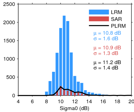
Figure 28. Histogram of science-valid sigma0 over oceans and lakes for LRM (blue), SAR (red), and PLRM (black) for 08/08/2019. The mean ( \mu ) and standard deviation ( \sigma ) are also shown. Note that values outside [4 20] dB are excluded from the histogram for the sake of readability but not from the computation of \mu and \sigma .
