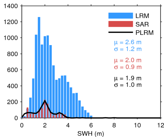
Figure 17. Histogram of flag-valid SWH over oceans and lakes for LRM (blue), SAR (red), and PLRM (black) for 08/08/2019. The mean ( \mu ) and standard deviation ( \sigma ) are also shown. Note that values larger than 12 m are excluded from the histogram for the sake of readability but not from the computation of \mu and \sigma .
