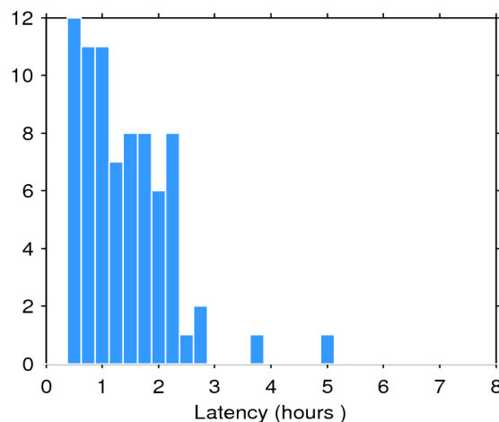
Figure 2. Histogram of the data latency for 08/08/2019. The y-axis denotes the number of files that are made available with a delay of x-hours with respect to the mean time of the records stored in the file.
