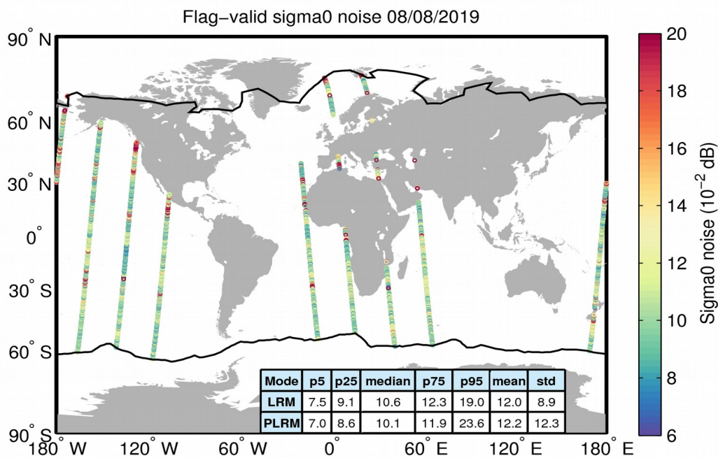
Figure 26. Geographical distribution of flag-valid 20-Hz sigma0 measurement noise over oceans and lakes for LRM/SAR (top) and LRM/PLRM (bottom) and for 08/08/2019. The statistical values shown in the table refer to the sigma0 noise and are calculated separately for LRM and SAR/PLRM regions. Measurements taken over polar polygons have been excluded from the computation of the statistical values. The black lines mark the outer limit of the Arctic and Antarctic polar polygons.
