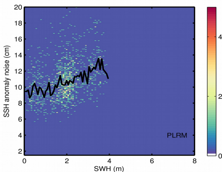
Figure 9. 2D histogram showing flag-valid SSH anomaly noise as a function of SWH for LRM (top), SAR (middle), and PLRM (bottom) for 08/08/2019. The black line denotes the median SSH anomaly noise as a function of SWH.
