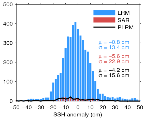
Figure 7. Histogram of flag-valid SSH anomaly over oceans and lakes for LRM (blue), SAR (red), and PLRM (black) for 22/05/2019. The mean ( \mu ) and standard deviation ( \sigma ) are also shown. Note that values outside [-50 50] cm are excluded from the histogram for the sake of readability but not from the computation of \mu and \sigma .
