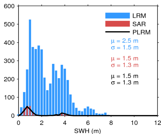
Figure 20. Histogram of science-valid SWH over oceans and lakes for LRM (blue), SAR (red), and PLRM (black) for 22/05/2019. The mean ( \mu ) and standard deviation ( \sigma ) are also
