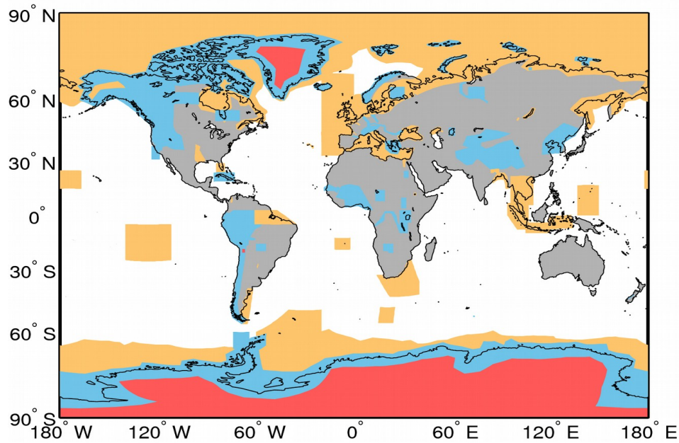
Figure A1. Extent of the regions defining the geographical mode mask for 22/05/2019. The regions where SAR, and SARIn are operated are denoted by the orange and blue polygons, respectively. LRM is operated over areas of the continental ice sheets (red polygons) and over oceans and land not covered by other modes.
