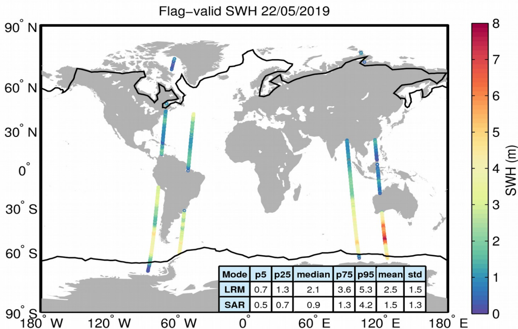
Figure 15. Geographical distribution of flag-valid SWH data over oceans and lakes for 22/05/2019. The statistical values shown in the table refer to the SWH in m and are calculated separately for LRM and SAR regions. Measurements taken over polar polygons
