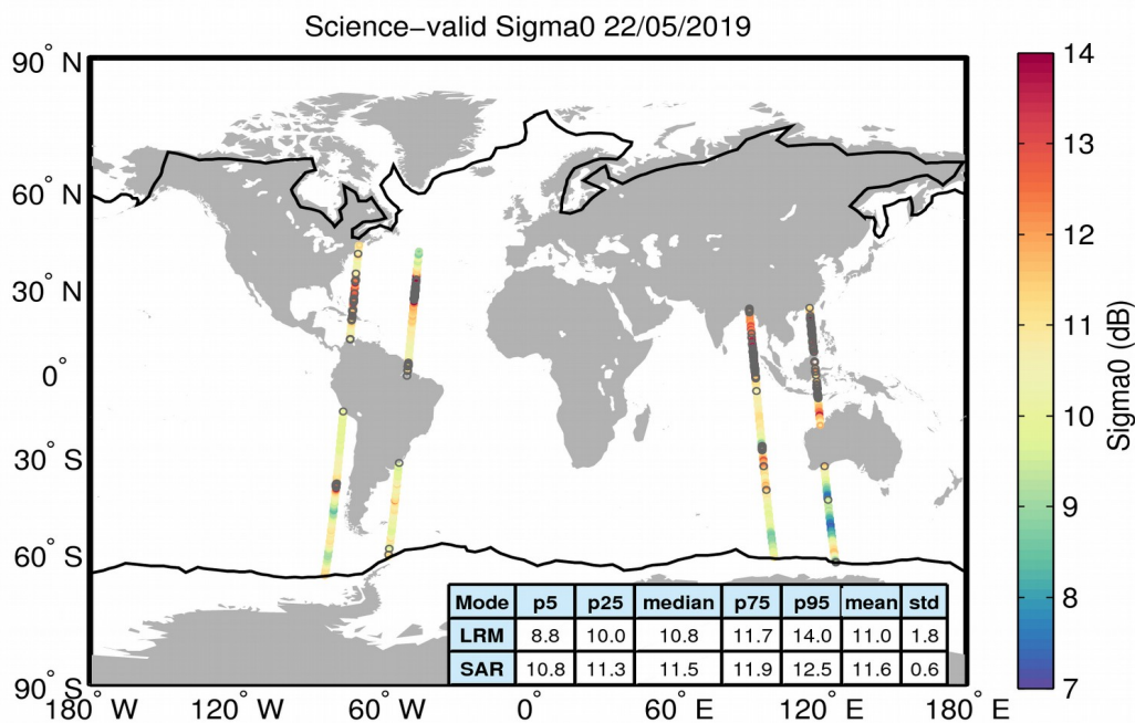
Figure 27. Geographical distribution of science-valid sigma0 data over oceans and lakes for 22/05/2019. The statistical values shown in the table refer to the sigma0 in dB and are calculated separately for LRM and SAR regions. The black lines mark the outer limit of the Arctic and Antarctic polar polygons. Gray circles denote records that have been rejected based on the editing criteria described in Table 4.
