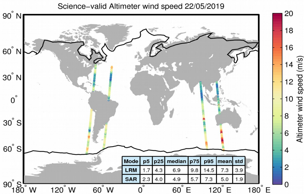
Figure 34. Geographical distribution of science-valid wind data over oceans and lakes for 22/05/2019. The statistical values shown in the table refer to the wind in m/s and are calculated separately for LRM and SAR regions. The black lines mark the outer limit of the Arctic and Antarctic polar polygons. Gray circles denote records that have been rejected based on the editing criteria described in Table 5.
