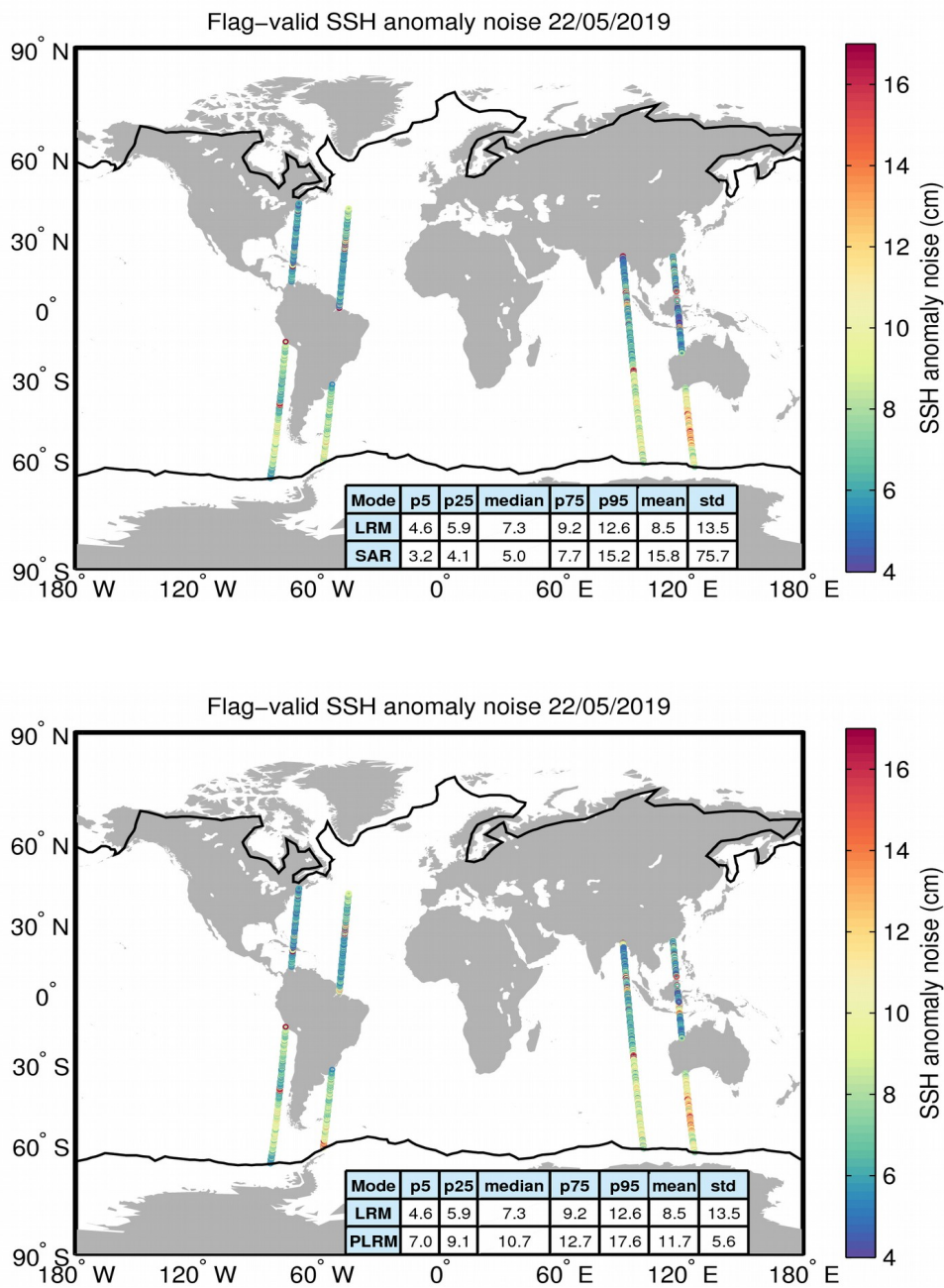
Figure 8. Geographical distribution of flag-valid 20-Hz SSH anomaly measurement noise over oceans and lakes for LRM/SAR (top) and LRM/PLRM (bottom) and for 22/05/2019. The statistical values shown in the tables refer to the SSH anomaly noise and are calculated separately for LRM and SAR/PLRM regions. Measurements taken over polar polygons have been excluded from the computation of the statistical values. The black lines mark the outer limit of the Arctic and Antarctic polar polygons.
