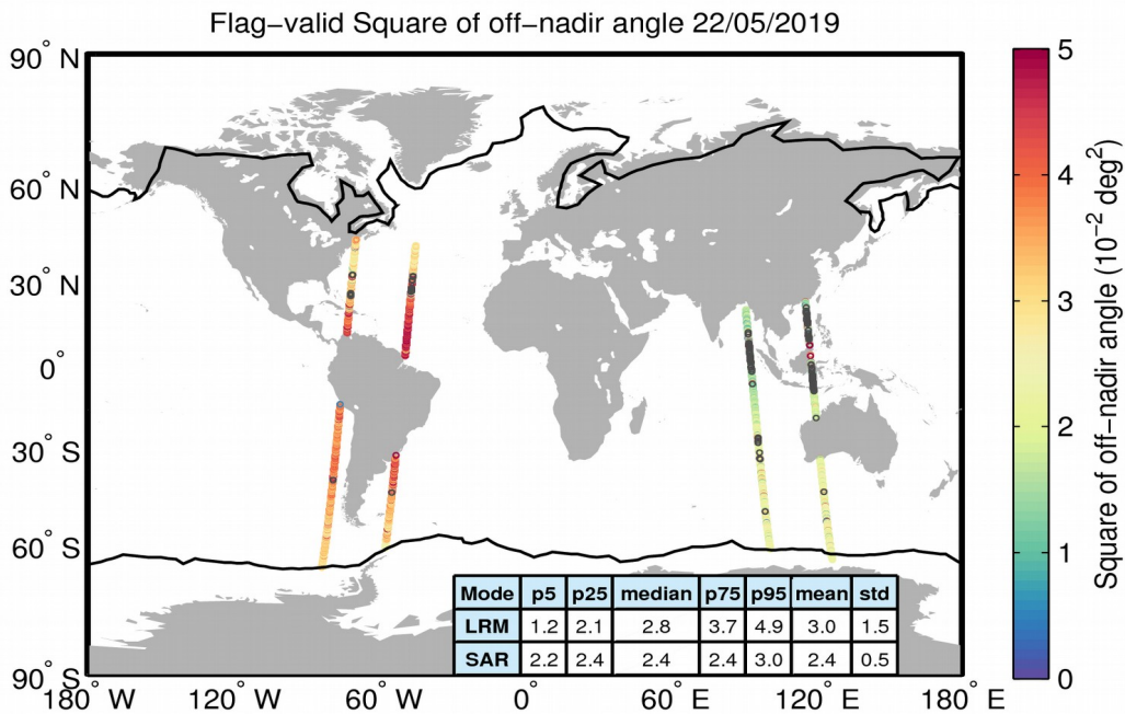
Figure 37. Geographical distribution of flag-valid mispointing data over oceans and lakes for 22/05/2019. The statistical values shown in the table refer to the mispointing in 10^{-2} deg 2 and are calculated separately for LRM and SAR regions. Measurements taken over polar polygons have been excluded from the computation of the statistical values. The black lines mark the outer limit of the Arctic and Antarctic polar polygons. Gray circles denote negative values.
