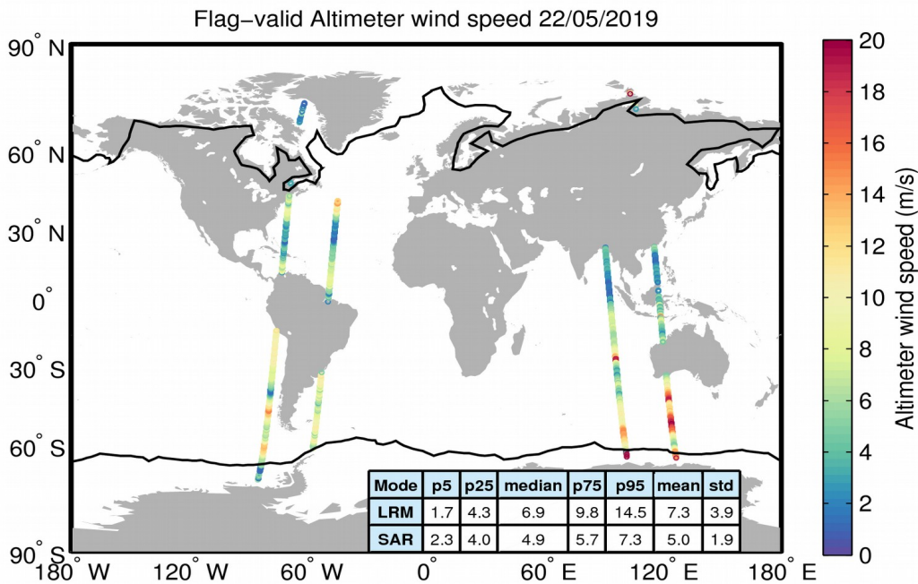
Figure 31. Geographical distribution of flag-valid wind data over oceans and lakes for 22/05/2019. The statistical values shown in the table refer to the wind in m/s and are calculated separately for LRM and SAR regions. Measurements taken over polar polygons have been excluded from the computation of the statistical values. The black lines mark the outer limit of the Arctic and Antarctic polar polygons.
