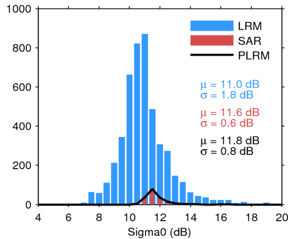
Figure 28. Histogram of science-valid sigma0 over oceans and lakes for LRM (blue), SAR (red), and PLRM (black) for 22/05/2019. The mean ( \mu ) and standard deviation ( \sigma ) are also shown. Note that values outside [4 20] dB are excluded from the histogram for the sake of readability but not from the computation of \mu and \sigma .
