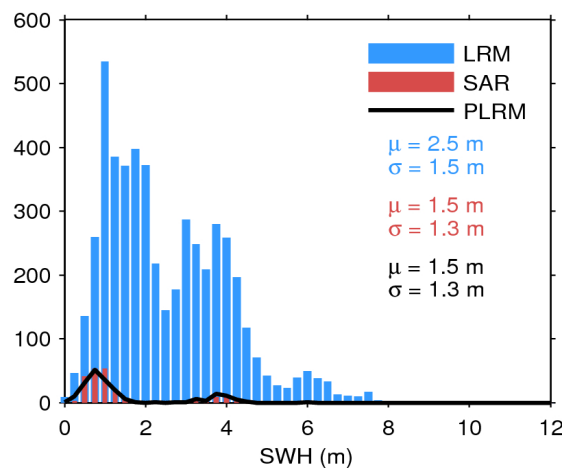
Figure 17. Histogram of flag-valid SWH over oceans and lakes for LRM (blue), SAR (red), and PLRM (black) for 22/05/2019. The mean ( \mu ) and standard deviation ( \sigma ) are also shown. Note that values larger than 12 m are excluded from the histogram for the sake of readability but not from the computation of \mu and \sigma .
