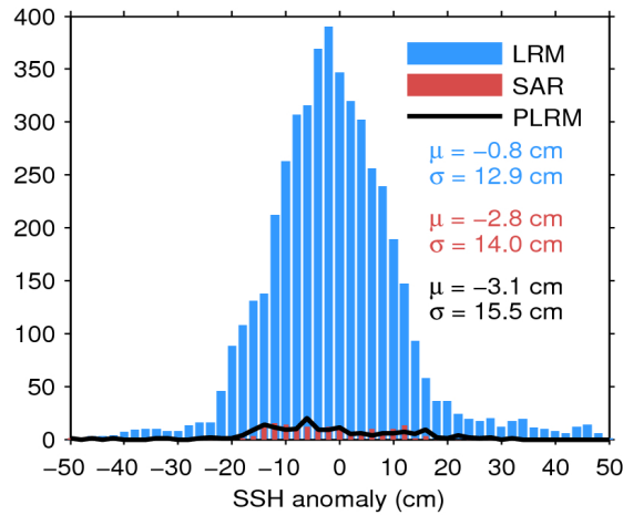
Figure 11. Histogram of science-valid SSH anomaly over oceans and lakes for LRM (blue), SAR (red), and PLRM (black) for 22/05/2019. The mean ( \mu ) and standard deviation ( \sigma ) are also shown. Note that values outside [-50\ 50] cm are excluded from the histogram for the sake of readability but not from the computation of \mu and \sigma .
