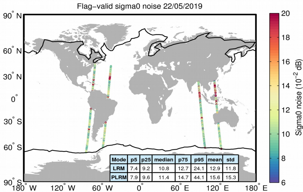
Figure 26. Geographical distribution of flag-valid 20-Hz sigma0 measurement noise over oceans and lakes for LRM/SAR (top) and LRM/PLRM (bottom) and for 22/05/2019. The statistical values shown in the table refer to the sigma0 noise and are calculated separately for LRM and SAR/PLRM regions. Measurements taken over polar polygons have been excluded from the computation of the statistical values. The black lines mark the outer limit of the Arctic and Antarctic polar polygons.
