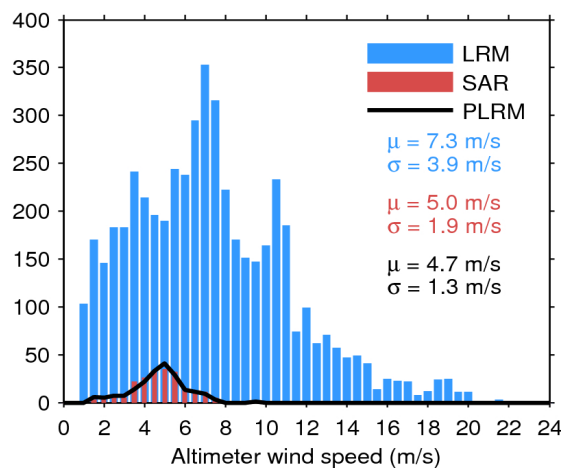
Figure 35. Histogram of science-valid wind over oceans and lakes for LRM (blue), SAR (red), and PLRM (black) for 22/05/2019. The mean ( \mu ) and standard deviation ( \sigma ) are also shown. Note that values larger than 24 m/s are excluded from the histogram for the sake of readability but not from the computation of \mu and \sigma .
