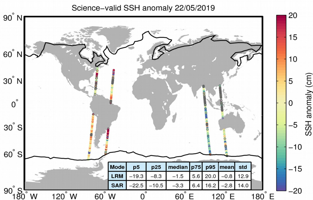
Figure 10. Geographical distribution of science-valid SSH anomaly data over oceans and lakes for 22/05/2019. The statistical values shown in the table refer to the SSH anomaly in cm and are calculated separately for LRM and SAR regions. The black lines mark the outer limit of the Arctic and Antarctic polar polygons. Gray circles denote records that have been rejected based on the editing criteria described in Table 2.
