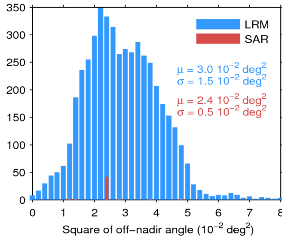
Figure 39. Histogram of flag-valid mispointing over oceans and lakes for LRM (blue) and SAR (red) for 22/05/2019. Only positive values have been considered. The mean ( \mu ) and standard deviation ( \sigma ) are also shown. Note that values larger than 8 \cdot 10^{-2} \text{ deg}^2 are excluded from the histogram for the sake of readability but not from the computation of \mu and \sigma .
