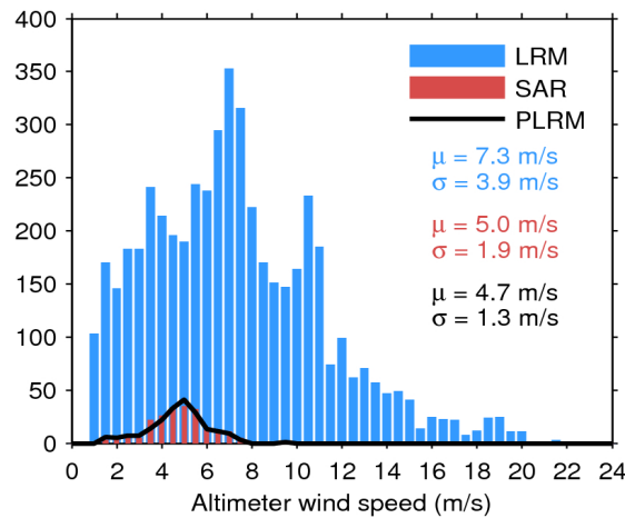
Figure 33. Histogram of flag-valid wind over oceans and lakes for LRM (blue), SAR (red), and PLRM(black) for 22/05/2019. The mean ( \mu ) and standard deviation ( \sigma ) are also shown. Note that values larger than 24 m/s are excluded from the histogram for the sake of readability but not from the computation of \mu and \sigma .
