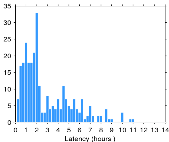
Figure 2. Histogram of the data latency for 15/05/2019. The y-axis denotes the number of files that are made available with a delay of x-hours with respect to the mean time of the records stored in the file.
