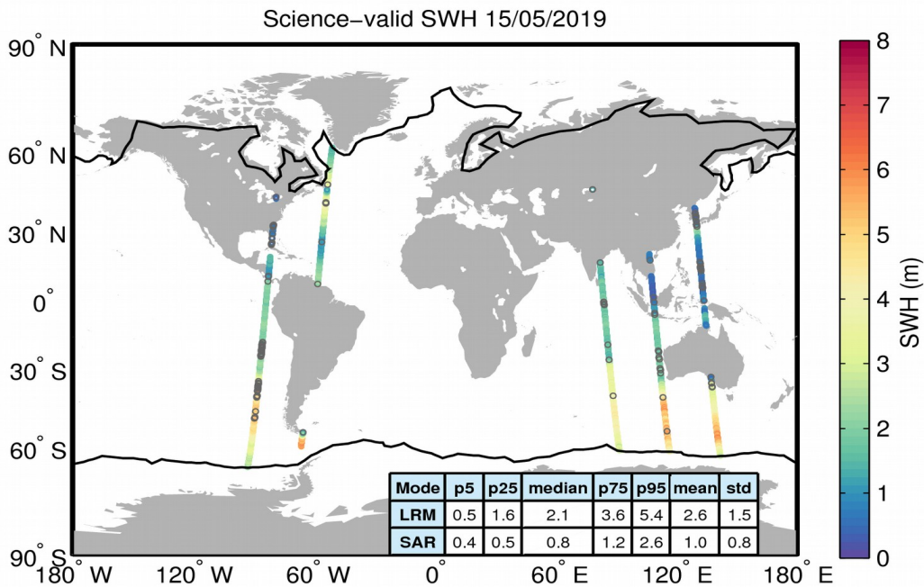
Figure 19. Geographical distribution of science-valid SWH data over oceans and lakes for 15/05/2019. The statistical values shown in the table refer to the SWH in m and are calculated separately for LRM and SAR regions. The black lines mark the outer limit of the Arctic and Antarctic polar polygons. Gray circles denote records that have been rejected based on the editing criteria described in Table 3.
