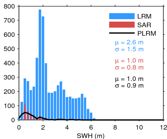
Figure 20. Histogram of science-valid SWH over oceans and lakes for LRM (blue), SAR (red), and PLRM (black) for 15/05/2019. The mean ( \mu ) and standard deviation ( \sigma ) are also
