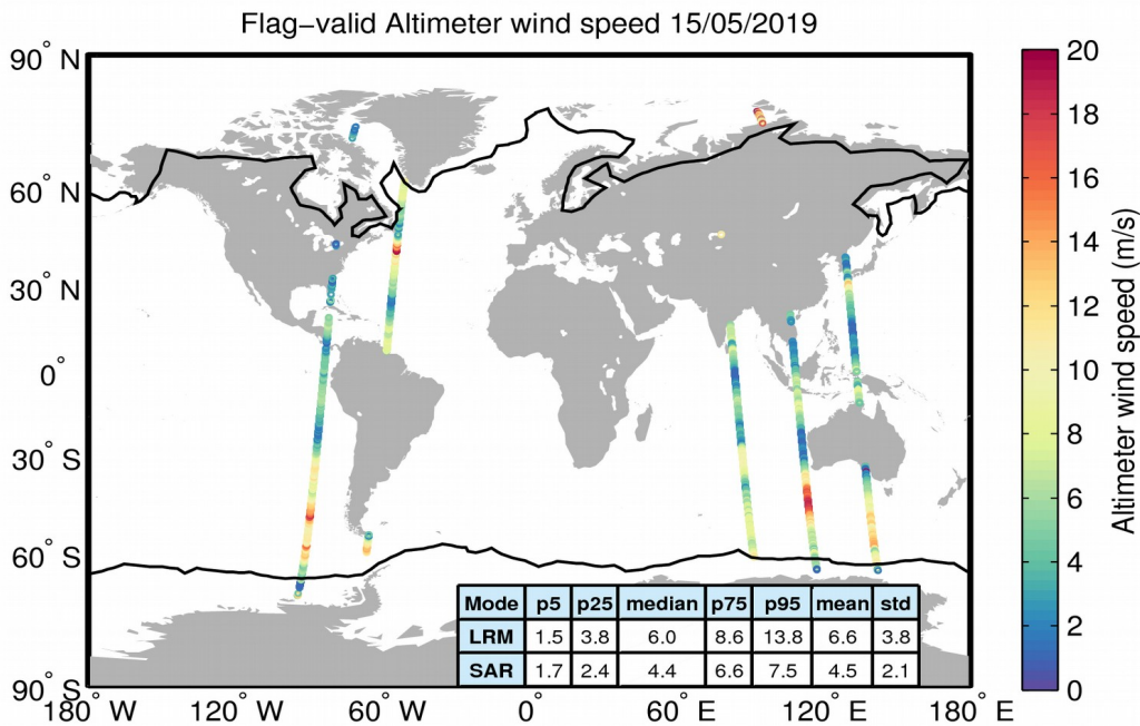
Figure 31. Geographical distribution of flag-valid wind data over oceans and lakes for 15/05/2019. The statistical values shown in the table refer to the wind in m/s and are calculated separately for LRM and SAR regions. Measurements taken over polar polygons have been excluded from the computation of the statistical values. The black lines mark the outer limit of the Arctic and Antarctic polar polygons.
