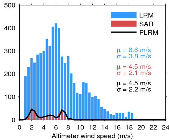
Figure 33. Histogram of flag-valid wind over oceans and lakes for LRM (blue), SAR (red), and PLRM(black) for 15/05/2019. The mean ( \mu ) and standard deviation ( \sigma ) are also shown. Note that values larger than 24 m/s are excluded from the histogram for the sake of readability but not from the computation of \mu and \sigma .
