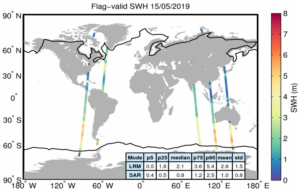
Figure 15. Geographical distribution of flag-valid SWH data over oceans and lakes for 15/05/2019. The statistical values shown in the table refer to the SWH in m and are calculated separately for LRM and SAR regions. Measurements taken over polar polygons
