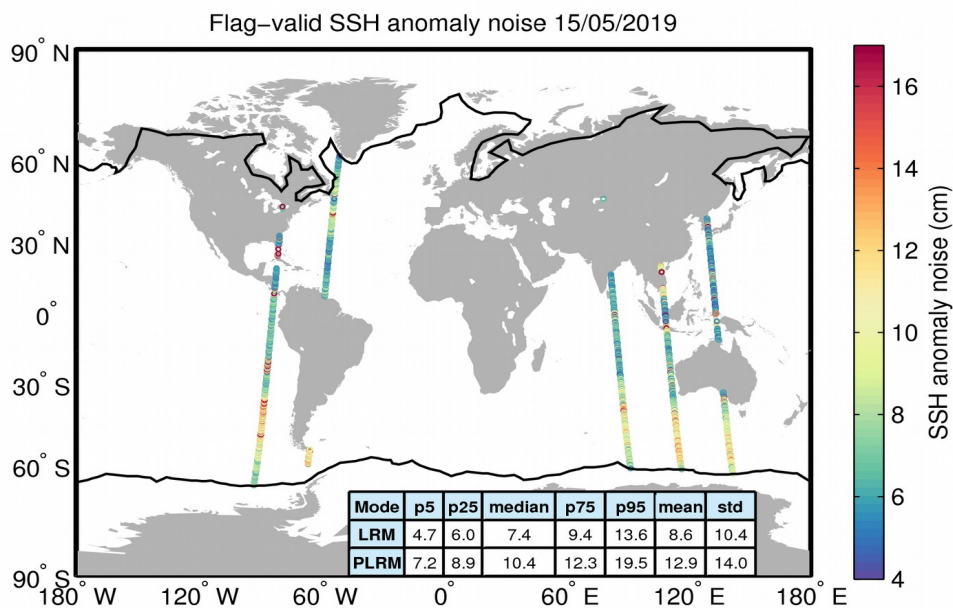
Figure 8. Geographical distribution of flag-valid 20-Hz SSH anomaly measurement noise over oceans and lakes for LRM/SAR (top) and LRM/PLRM (bottom) and for 15/05/2019. The statistical values shown in the tables refer to the SSH anomaly noise and are calculated separately for LRM and SAR/PLRM regions. Measurements taken over polar polygons have been excluded from the computation of the statistical values. The black lines mark the outer limit of the Arctic and Antarctic polar polygons.
