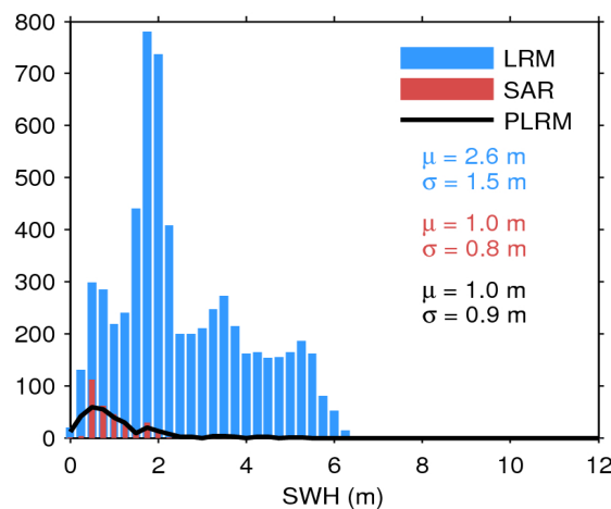
Figure 17. Histogram of flag-valid SWH over oceans and lakes for LRM (blue), SAR (red), and PLRM (black) for 15/05/2019. The mean ( \mu ) and standard deviation ( \sigma ) are also shown. Note that values larger than 12 m are excluded from the histogram for the sake of readability but not from the computation of \mu and \sigma .
