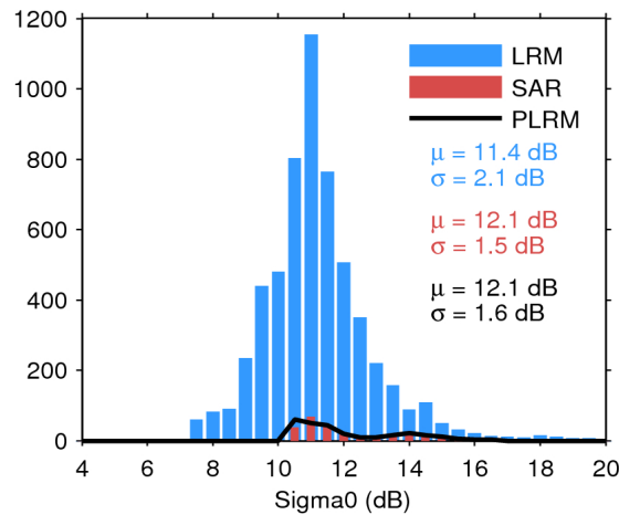
Figure 28. Histogram of science-valid sigma0 over oceans and lakes for LRM (blue), SAR (red), and PLRM (black) for 15/05/2019. The mean ( \mu ) and standard deviation ( \sigma ) are also shown. Note that values outside [4 20] dB are excluded from the histogram for the sake of readability but not from the computation of \mu and \sigma .
