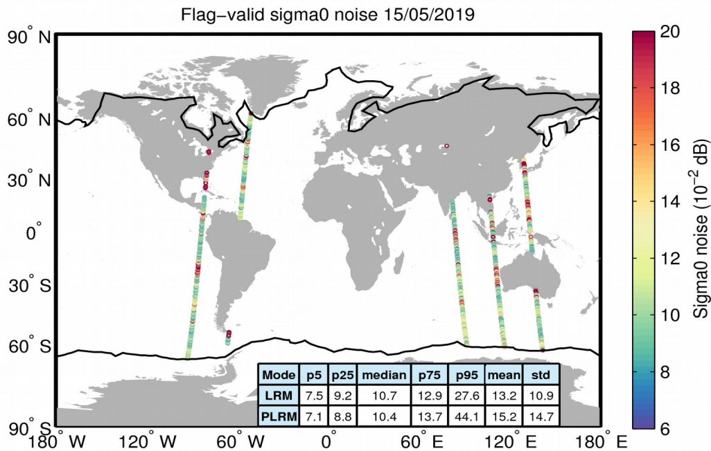
Figure 26. Geographical distribution of flag-valid 20-Hz sigma0 measurement noise over oceans and lakes for LRM/SAR (top) and LRM/PLRM (bottom) and for 15/05/2019. The statistical values shown in the table refer to the sigma0 noise and are calculated separately for LRM and SAR/PLRM regions. Measurements taken over polar polygons have been excluded from the computation of the statistical values. The black lines mark the outer limit of the Arctic and Antarctic polar polygons.
