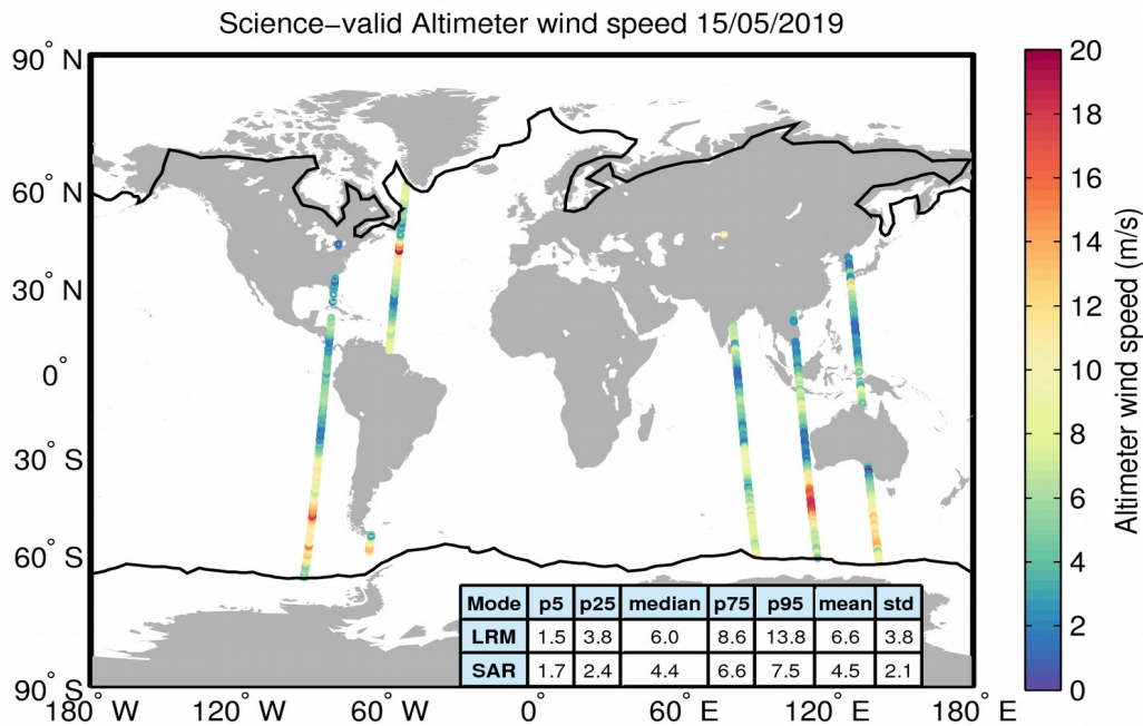
Figure 34. Geographical distribution of science-valid wind data over oceans and lakes for 15/05/2019. The statistical values shown in the table refer to the wind in m/s and are calculated separately for LRM and SAR regions. The black lines mark the outer limit of the Arctic and Antarctic polar polygons. Gray circles denote records that have been rejected based on the editing criteria described in Table 5.
