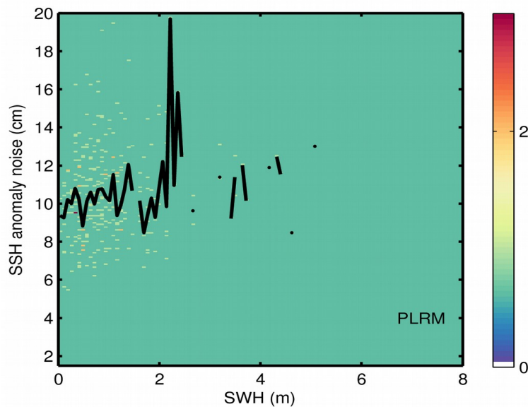
Figure 9. 2D histogram showing flag-valid SSH anomaly noise as a function of SWH for LRM (top), SAR (middle), and PLRM (bottom) for 15/05/2019. The black line denotes the median SSH anomaly noise as a function of SWH.
