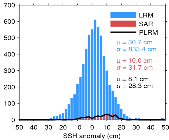
Figure 7. Histogram of flag-valid SSH anomaly over oceans and lakes for LRM (blue), SAR (red), and PLRM (black) for 15/05/2019. The mean ( \mu ) and standard deviation ( \sigma ) are also shown. Note that values outside [-50 50] cm are excluded from the histogram for the sake of readability but not from the computation of \mu and \sigma .
