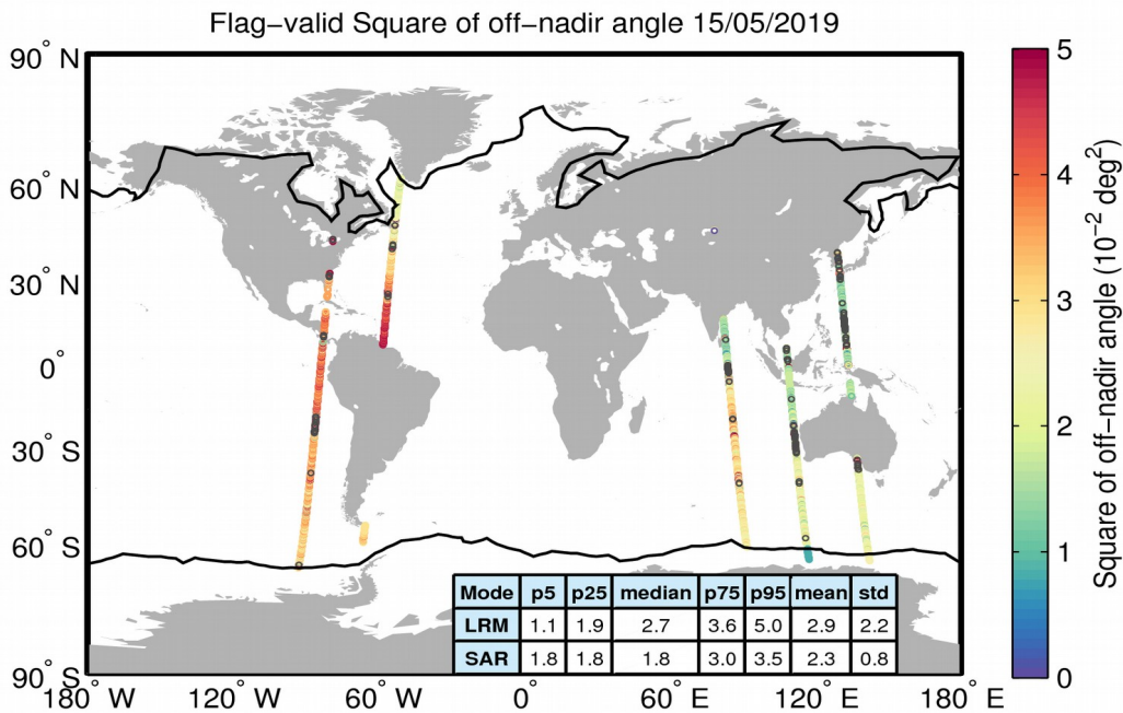
Figure 37. Geographical distribution of flag-valid mispointing data over oceans and lakes for 15/05/2019. The statistical values shown in the table refer to the mispointing in 10^{-2} deg 2 and are calculated separately for LRM and SAR regions. Measurements taken over polar polygons have been excluded from the computation of the statistical values. The black lines mark the outer limit of the Arctic and Antarctic polar polygons. Gray circles denote negative values.
