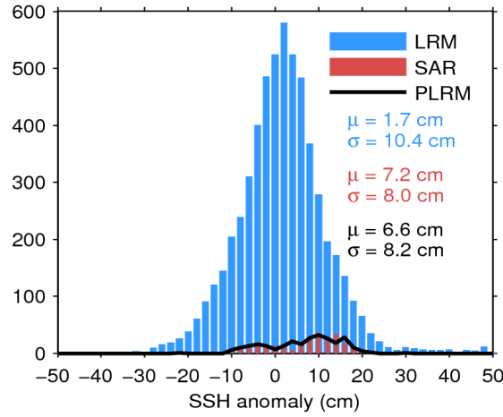
Figure 11. Histogram of science-valid SSH anomaly over oceans and lakes for LRM (blue), SAR (red), and PLRM (black) for 15/05/2019. The mean ( \mu ) and standard deviation ( \sigma ) are also shown. Note that values outside [-50\ 50] cm are excluded from the histogram for the sake of readability but not from the computation of \mu and \sigma .
