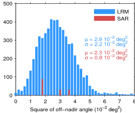
Figure 39. Histogram of flag-valid mispointing over oceans and lakes for LRM (blue) and SAR (red) for 15/05/2019. Only positive values have been considered. The mean ( \mu ) and standard deviation ( \sigma ) are also shown. Note that values larger than 8 \cdot 10^{-2} \text{ deg}^2 are excluded from the histogram for the sake of readability but not from the computation of \mu and \sigma .
