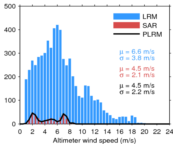
Figure 35. Histogram of science-valid wind over oceans and lakes for LRM (blue), SAR (red), and PLRM (black) for 15/05/2019. The mean ( \mu ) and standard deviation ( \sigma ) are also shown. Note that values larger than 24 m/s are excluded from the histogram for the sake of readability but not from the computation of \mu and \sigma .
