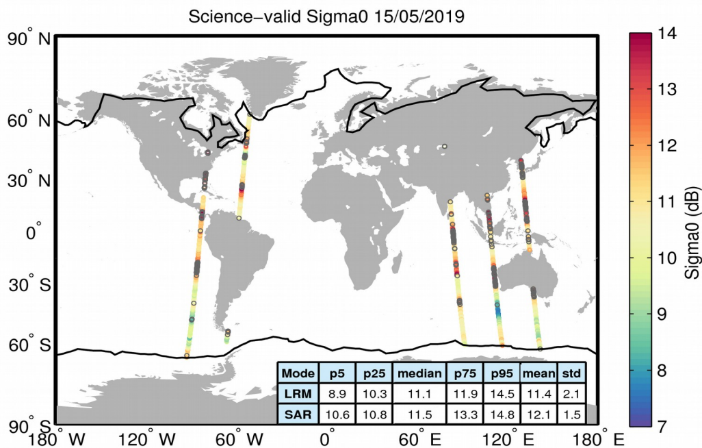
Figure 27. Geographical distribution of science-valid sigma0 data over oceans and lakes for 15/05/2019. The statistical values shown in the table refer to the sigma0 in dB and are calculated separately for LRM and SAR regions. The black lines mark the outer limit of the Arctic and Antarctic polar polygons. Gray circles denote records that have been rejected based on the editing criteria described in Table 4.
