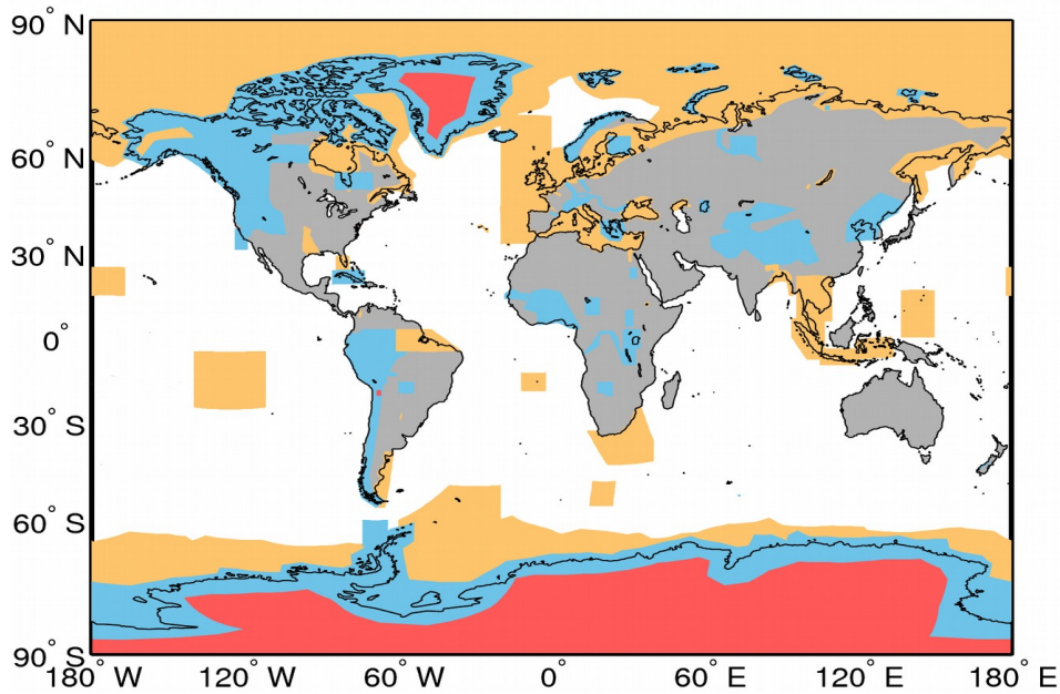
Figure A1. Extent of the regions defining the geographical mode mask for 15/05/2019. The regions where SAR, and SARIn are operated are denoted by the orange and blue polygons, respectively. LRM is operated over areas of the continental ice sheets (red polygons) and over oceans and land not covered by other modes.
