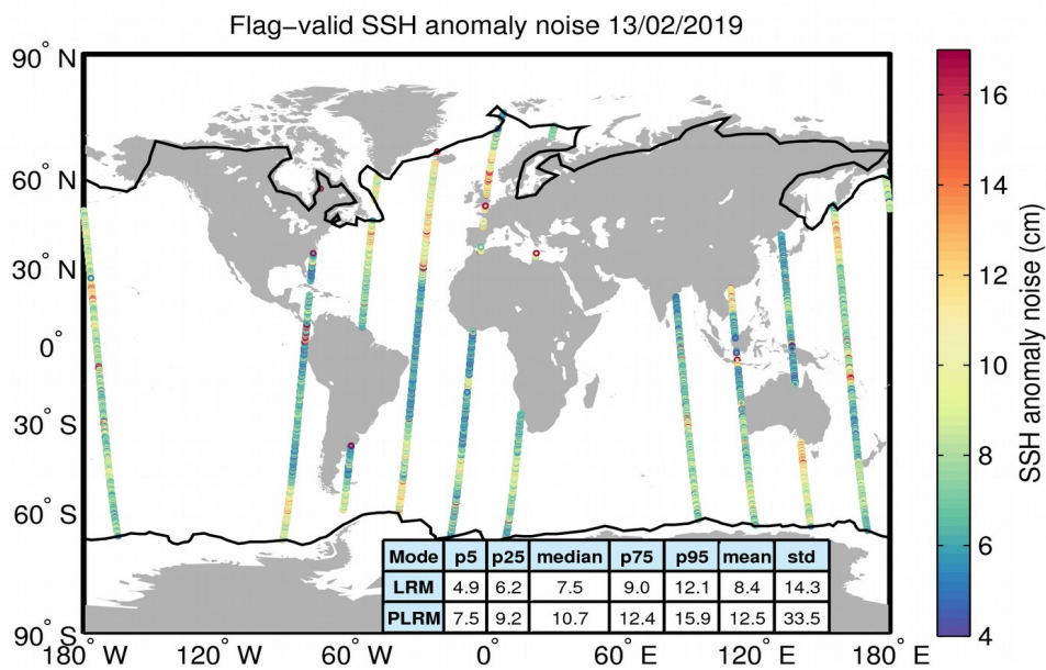
Figure 8. Geographical distribution of flag-valid 20-Hz SSH anomaly measurement noise over oceans and lakes for LRM/SAR (top) and LRM/PLRM (bottom) and for 13/02/2019. The statistical values shown in the tables refer to the SSH anomaly noise and are calculated separately for LRM and SAR/PLRM regions. Measurements taken over polar polygons have been excluded from the computation of the statistical values. The black lines mark the outer limit of the Arctic and Antarctic polar polygons.
