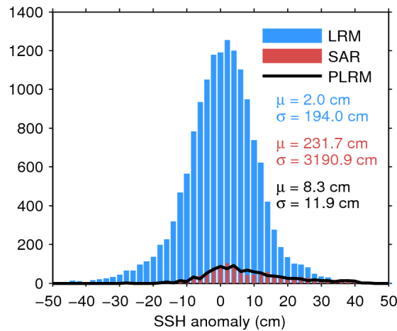
Figure 7. Histogram of flag-valid SSH anomaly over oceans and lakes for LRM (blue), SAR (red), and PLRM (black) for 13/02/2019. The mean ( \mu ) and standard deviation ( \sigma ) are also shown. Note that values outside [-50 50] cm are excluded from the histogram for the sake of readability but not from the computation of \mu and \sigma .
