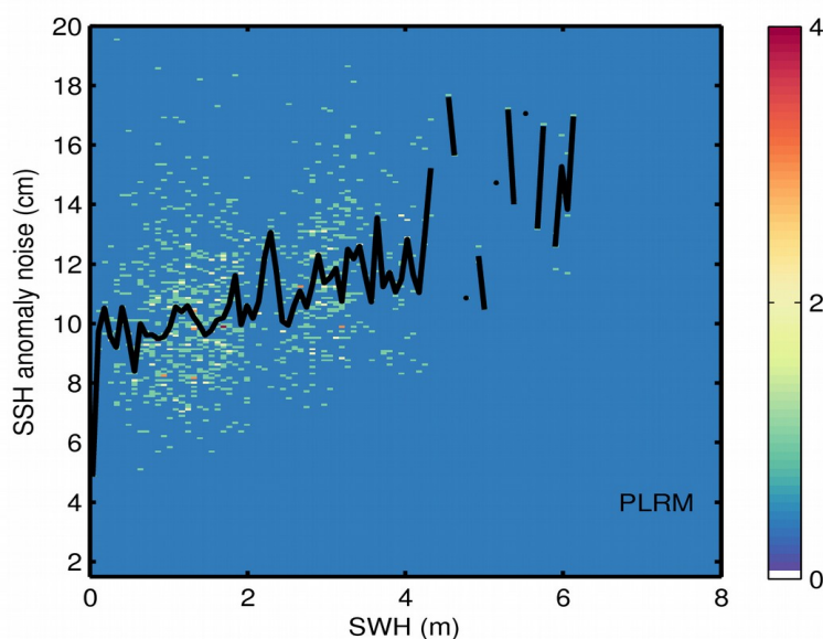
Figure 9. 2D histogram showing flag-valid SSH anomaly noise as a function of SWH for LRM (top), SAR (middle), and PLRM (bottom) for 13/02/2019. The black line denotes the median SSH anomaly noise as a function of SWH.
