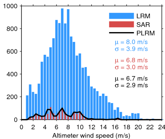
Figure 35. Histogram of science-valid wind over oceans and lakes for LRM (blue), SAR (red), and PLRM (black) for 13/02/2019. The mean ( \mu ) and standard deviation ( \sigma ) are also shown. Note that values larger than 24 m/s are excluded from the histogram for the sake of readability but not from the computation of \mu and \sigma .
