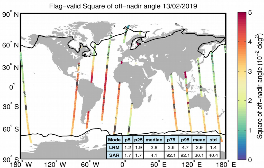
Figure 37. Geographical distribution of flag-valid mispointing data over oceans and lakes for 13/02/2019. The statistical values shown in the table refer to the mispointing in 10^{-2} deg 2 and are calculated separately for LRM and SAR regions. Measurements taken over polar polygons have been excluded from the computation of the statistical values. The black lines mark the outer limit of the Arctic and Antarctic polar polygons. Gray circles denote negative values.
