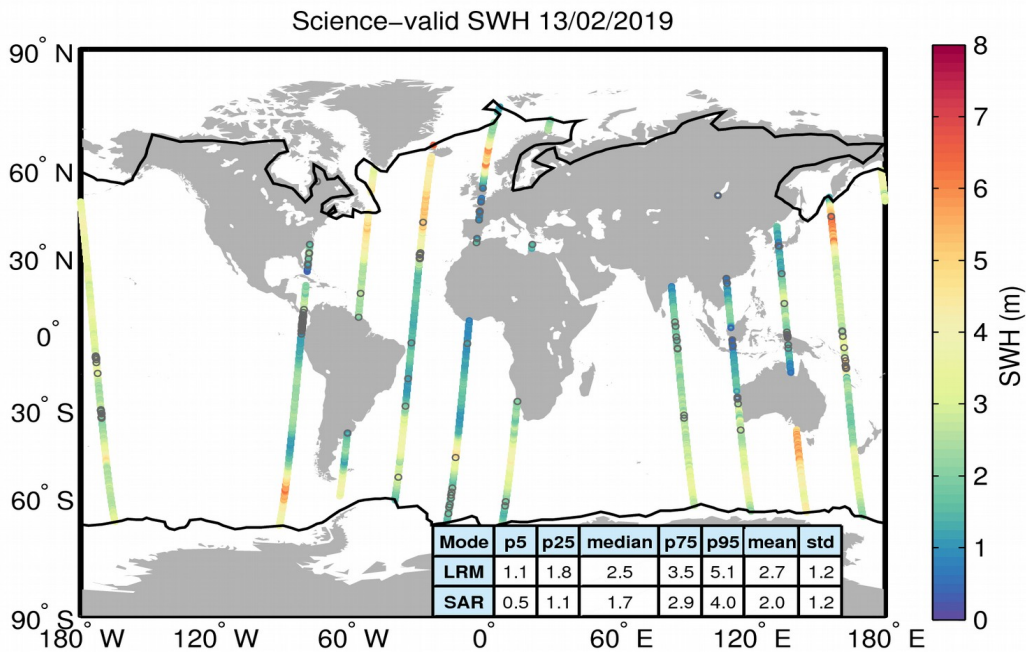
Figure 19. Geographical distribution of science-valid SWH data over oceans and lakes for 13/02/2019. The statistical values shown in the table refer to the SWH in m and are calculated separately for LRM and SAR regions. The black lines mark the outer limit of the Arctic and Antarctic polar polygons. Gray circles denote records that have been rejected based on the editing criteria described in Table 3.
