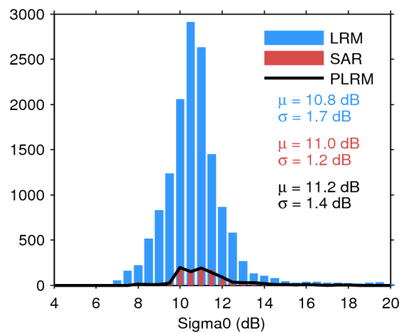
Figure 28. Histogram of science-valid sigma0 over oceans and lakes for LRM (blue), SAR (red), and PLRM (black) for 13/02/2019. The mean ( \mu ) and standard deviation ( \sigma ) are also shown. Note that values outside [4 20] dB are excluded from the histogram for the sake of readability but not from the computation of \mu and \sigma .
