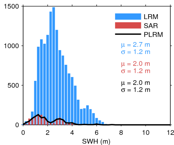
Figure 17. Histogram of flag-valid SWH over oceans and lakes for LRM (blue), SAR (red), and PLRM (black) for 13/02/2019. The mean ( \mu ) and standard deviation ( \sigma ) are also shown. Note that values larger than 12 m are excluded from the histogram for the sake of readability but not from the computation of \mu and \sigma .
