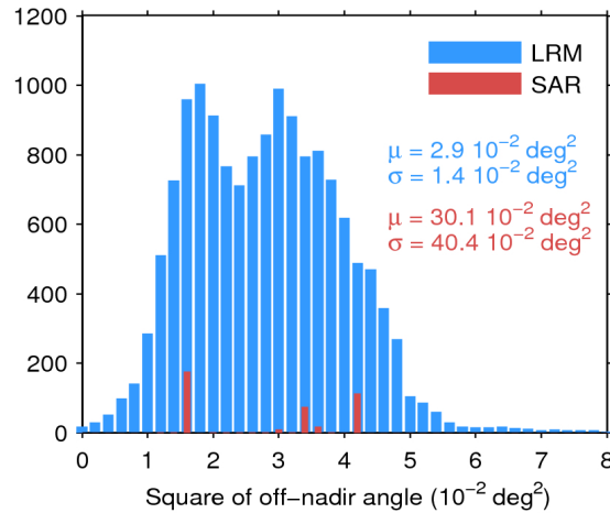
Figure 39. Histogram of flag-valid mispointing over oceans and lakes for LRM (blue) and SAR (red) for 13/02/2019. Only positive values have been considered. The mean ( \mu ) and standard deviation ( \sigma ) are also shown. Note that values larger than 8 \cdot 10^{-2} \text{ deg}^2 are excluded from the histogram for the sake of readability but not from the computation of \mu and \sigma .
