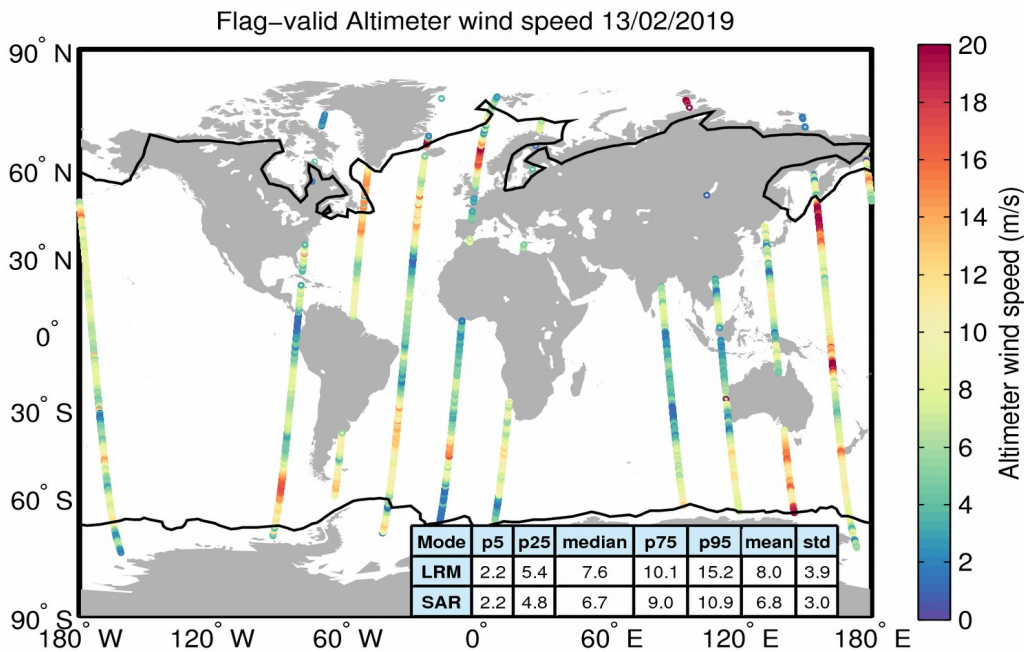
Figure 31. Geographical distribution of flag-valid wind data over oceans and lakes for 13/02/2019. The statistical values shown in the table refer to the wind in m/s and are calculated separately for LRM and SAR regions. Measurements taken over polar polygons have been excluded from the computation of the statistical values. The black lines mark the outer limit of the Arctic and Antarctic polar polygons.
