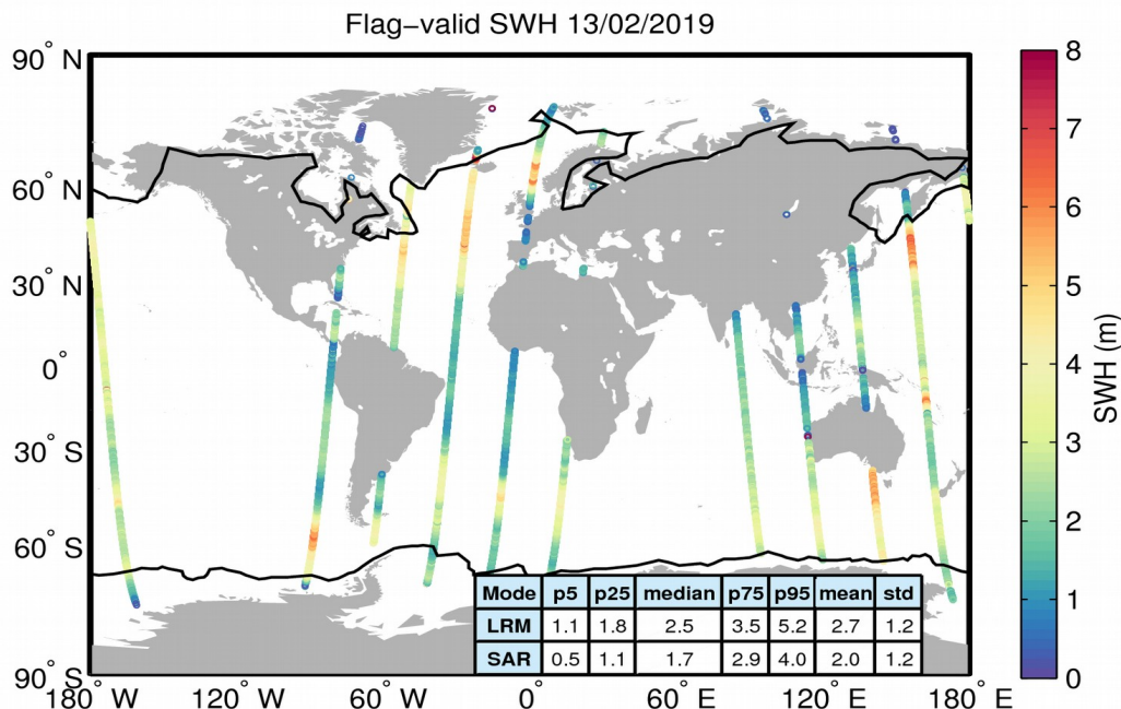
Figure 15. Geographical distribution of flag-valid SWH data over oceans and lakes for 13/02/2019. The statistical values shown in the table refer to the SWH in m and are calculated separately for LRM and SAR regions. Measurements taken over polar polygons
