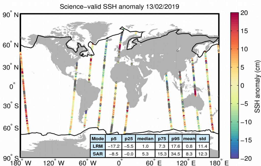
Figure 10. Geographical distribution of science-valid SSH anomaly data over oceans and lakes for 13/02/2019. The statistical values shown in the table refer to the SSH anomaly in cm and are calculated separately for LRM and SAR regions. The black lines mark the outer limit of the Arctic and Antarctic polar polygons. Gray circles denote records that have been rejected based on the editing criteria described in Table 2.
