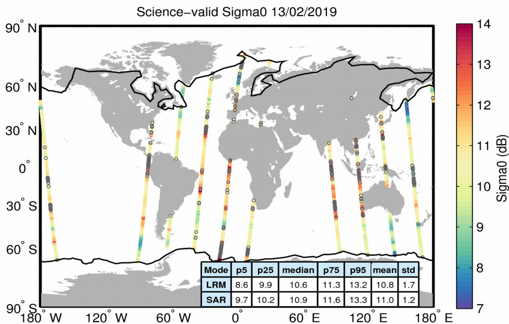
Figure 27. Geographical distribution of science-valid sigma0 data over oceans and lakes for 13/02/2019. The statistical values shown in the table refer to the sigma0 in dB and are calculated separately for LRM and SAR regions. The black lines mark the outer limit of the Arctic and Antarctic polar polygons. Gray circles denote records that have been rejected based on the editing criteria described in Table 4.
