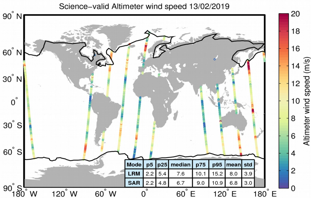
Figure 34. Geographical distribution of science-valid wind data over oceans and lakes for 13/02/2019. The statistical values shown in the table refer to the wind in m/s and are calculated separately for LRM and SAR regions. The black lines mark the outer limit of the Arctic and Antarctic polar polygons. Gray circles denote records that have been rejected based on the editing criteria described in Table 5.
