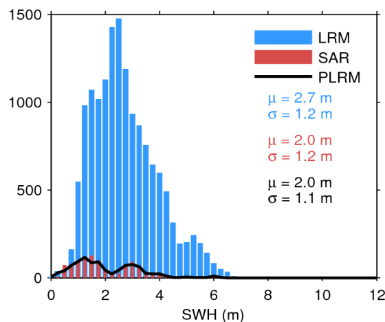
Figure 20. Histogram of science-valid SWH over oceans and lakes for LRM (blue), SAR (red), and PLRM (black) for 13/02/2019. The mean ( \mu ) and standard deviation ( \sigma ) are also
