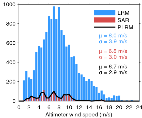
Figure 33. Histogram of flag-valid wind over oceans and lakes for LRM (blue), SAR (red), and PLRM (black) for 13/02/2019. The mean ( \mu ) and standard deviation ( \sigma ) are also shown. Note that values larger than 24 m/s are excluded from the histogram for the sake of readability but not from the computation of \mu and \sigma .
