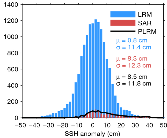
Figure 11. Histogram of science-valid SSH anomaly over oceans and lakes for LRM (blue), SAR (red), and PLRM (black) for 13/02/2019. The mean ( \mu ) and standard deviation ( \sigma ) are also shown. Note that values outside [-50\ 50] cm are excluded from the histogram for the sake of readability but not from the computation of \mu and \sigma .
