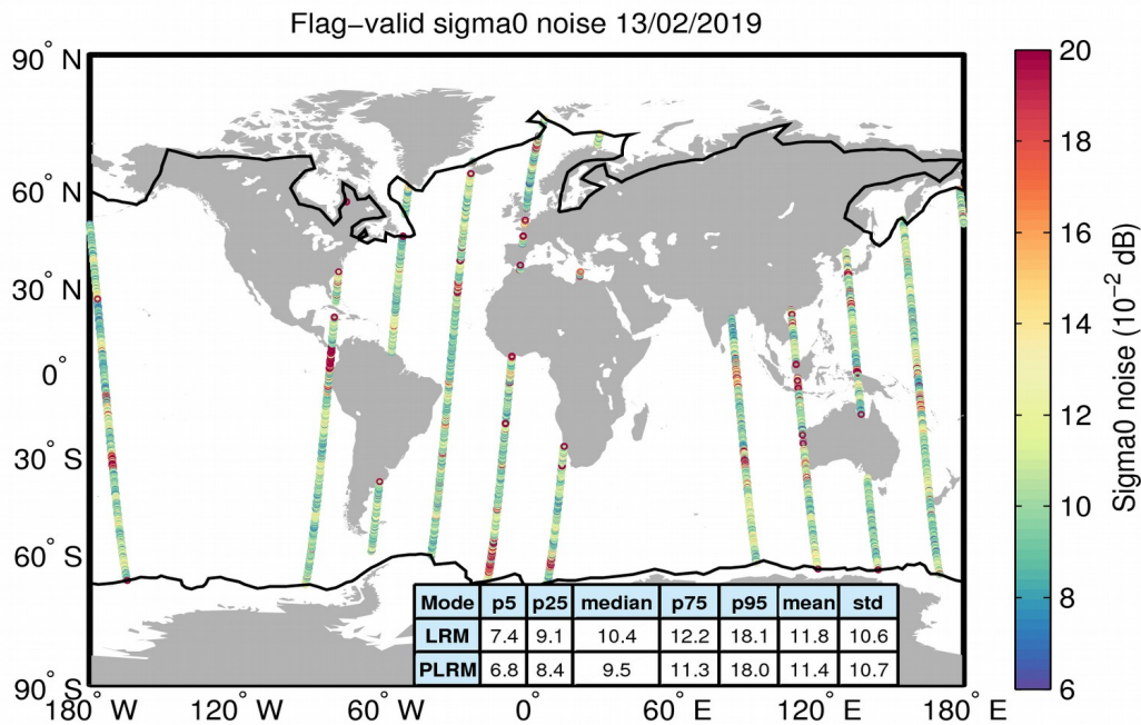
Figure 26. Geographical distribution of flag-valid 20-Hz sigma0 measurement noise over oceans and lakes for LRM/SAR (top) and LRM/PLRM (bottom) and for 13/02/2019. The statistical values shown in the table refer to the sigma0 noise and are calculated separately for LRM and SAR/PLRM regions. Measurements taken over polar polygons have been excluded from the computation of the statistical values. The black lines mark the outer limit of the Arctic and Antarctic polar polygons.
