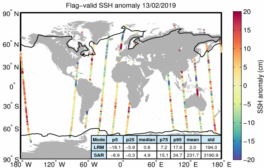
Figure 5. Geographical distribution of flag-valid 1-Hz SSH anomaly data over oceans and lakes for 13/02/2019. The statistical values shown in the table refer to the SSH anomaly in cm and are calculated separately for LRM and SAR regions. Measurements taken over polar polygons have been excluded from the computation of the statistical values. The black lines mark the outer limit of the Arctic and Antarctic polar polygons.
