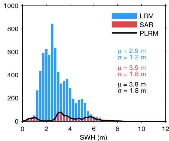
Figure 17. Histogram of flag-valid SWH over oceans and lakes for LRM (blue), SAR (red), and PLRM (black) for 24/01/2019. The mean ( \mu ) and standard deviation ( \sigma ) are also shown. Note that values larger than 12 m are excluded from the histogram for the sake of readability but not from the computation of \mu and \sigma .
