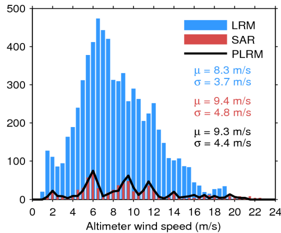
Figure 33. Histogram of flag-valid wind over oceans and lakes for LRM (blue), SAR (red), and PLRM (black) for 24/01/2019. The mean ( \mu ) and standard deviation ( \sigma ) are also shown. Note that values larger than 24 m/s are excluded from the histogram for the sake of readability but not from the computation of \mu and \sigma .
