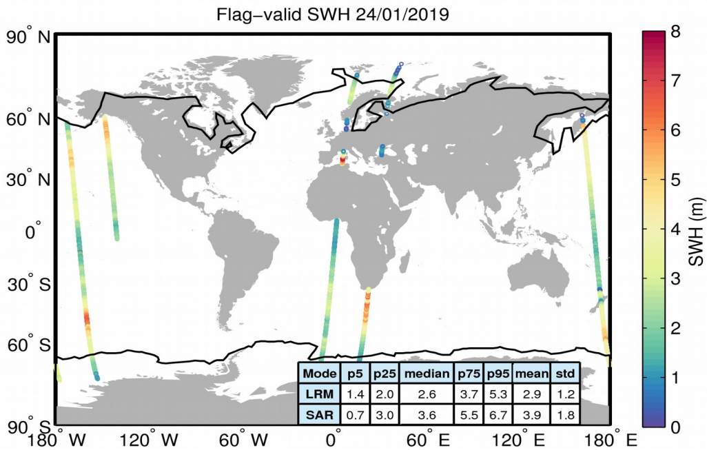
Figure 15. Geographical distribution of flag-valid SWH data over oceans and lakes for 24/01/2019. The statistical values shown in the table refer to the SWH in m and are calculated separately for LRM and SAR regions. Measurements taken over polar polygons have been excluded from the computation of the statistical values. The black lines mark the outer limit of the Arctic and Antarctic polar polygons.
