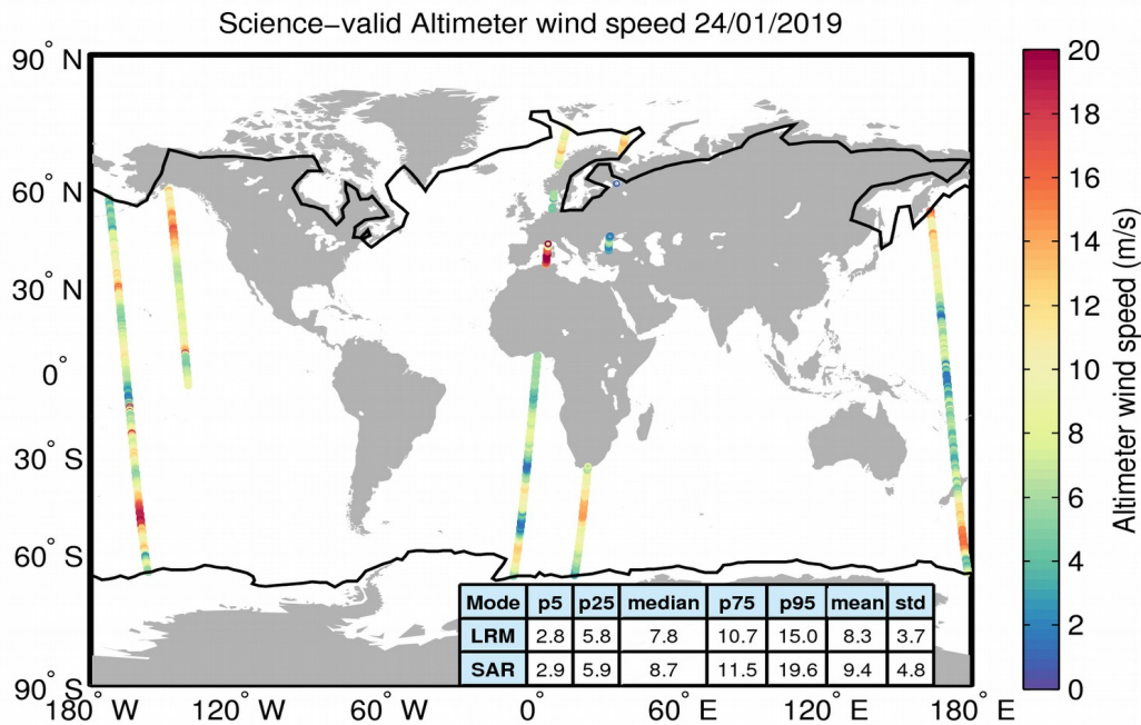
Figure 34. Geographical distribution of science-valid wind data over oceans and lakes for 24/01/2019. The statistical values shown in the table refer to the wind in m/s and are calculated separately for LRM and SAR regions. The black lines mark the outer limit of the Arctic and Antarctic polar polygons. Gray circles denote records that have been rejected based on the editing criteria described in Table 5.
