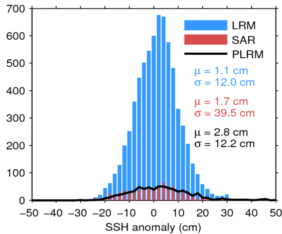
Figure 7. Histogram of flag-valid SSH anomaly over oceans and lakes for LRM (blue), SAR (red), and PLRM (black) for 24/01/2019. The mean ( \mu ) and standard deviation ( \sigma ) are also shown. Note that values outside [-50 50] cm are excluded from the histogram for the sake of readability but not from the computation of \mu and \sigma .
