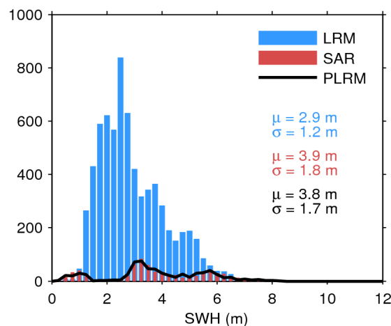
Figure 20. Histogram of science-valid SWH over oceans and lakes for LRM (blue), SAR (red), and PLRM (black) for 24/01/2019. The mean ( \mu ) and standard deviation ( \sigma ) are also
