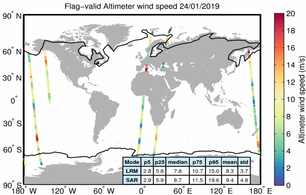
Figure 31. Geographical distribution of flag-valid wind data over oceans and lakes for 24/01/2019. The statistical values shown in the table refer to the wind in m/s and are calculated separately for LRM and SAR regions. Measurements taken over polar polygons have been excluded from the computation of the statistical values. The black lines mark the outer limit of the Arctic and Antarctic polar polygons.
