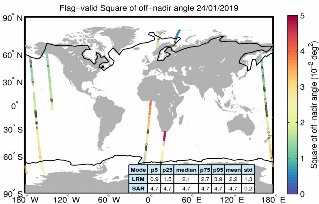
Figure 37. Geographical distribution of flag-valid mispointing data over oceans and lakes for 24/01/2019. The statistical values shown in the table refer to the mispointing in 10^{-2} deg 2 and are calculated separately for LRM and SAR regions. Measurements taken over polar polygons have been excluded from the computation of the statistical values. The black lines mark the outer limit of the Arctic and Antarctic polar polygons. Gray circles denote negative values.
