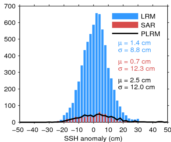
Figure 11. Histogram of science-valid SSH anomaly over oceans and lakes for LRM (blue), SAR (red), and PLRM (black) for 24/01/2019. The mean ( \mu ) and standard deviation ( \sigma ) are also shown. Note that values outside [-50 50] cm are excluded from the histogram for the sake of readability but not from the computation of \mu and \sigma .
