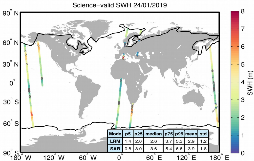
Figure 19. Geographical distribution of science-valid SWH data over oceans and lakes for 24/01/2019. The statistical values shown in the table refer to the SWH in m and are calculated separately for LRM and SAR regions. The black lines mark the outer limit of the Arctic and Antarctic polar polygons. Gray circles denote records that have been rejected based on the editing criteria described in Table 3.
