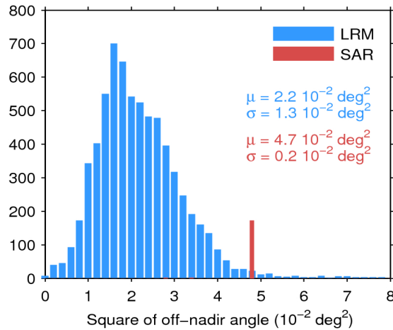
Figure 39. Histogram of flag-valid mispointing over oceans and lakes for LRM (blue) and SAR (red) for 24/01/2019. Only positive values have been considered. The mean ( \mu ) and standard deviation ( \sigma ) are also shown. Note that values larger than 8 \cdot 10^{-2} \text{ deg}^2 are excluded from the histogram for the sake of readability but not from the computation of \mu and \sigma .
