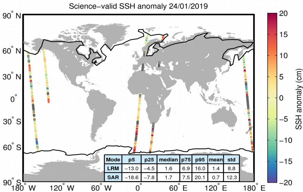
Figure 10. Geographical distribution of science-valid SSH anomaly data over oceans and lakes for 24/01/2019. The statistical values shown in the table refer to the SSH anomaly in cm and are calculated separately for LRM and SAR regions. The black lines mark the outer limit of the Arctic and Antarctic polar polygons. Gray circles denote records that have been rejected based on the editing criteria described in Table 2.
