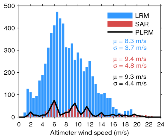
Figure 35. Histogram of science-valid wind over oceans and lakes for LRM (blue), SAR (red), and PLRM (black) for 24/01/2019. The mean ( \mu ) and standard deviation ( \sigma ) are also shown. Note that values larger than 24 m/s are excluded from the histogram for the sake of readability but not from the computation of \mu and \sigma .
