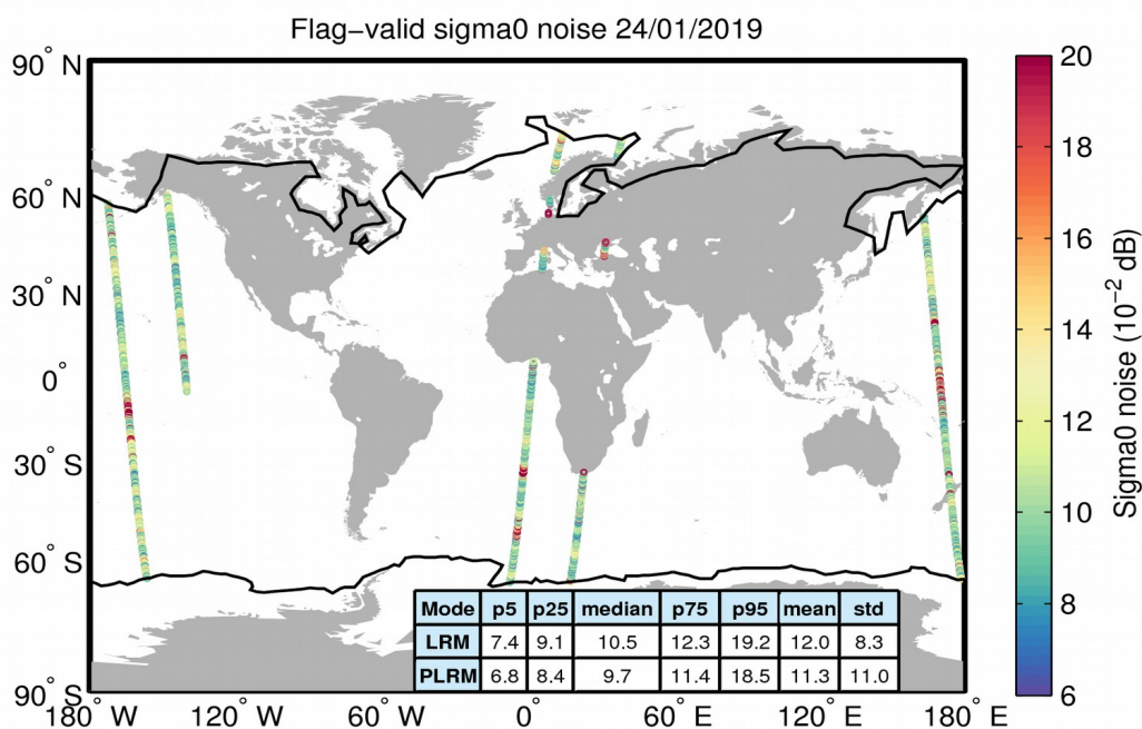
Figure 26. Geographical distribution of flag-valid 20-Hz sigma0 measurement noise over oceans and lakes for LRM/SAR (top) and LRM/PLRM (bottom) and for 24/01/2019. The statistical values shown in the table refer to the sigma0 noise and are calculated separately for LRM and SAR/PLRM regions. Measurements taken over polar polygons have been excluded from the computation of the statistical values. The black lines mark the outer limit of the Arctic and Antarctic polar polygons.
