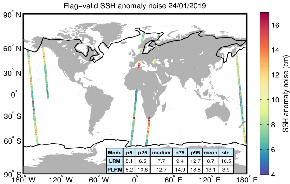
Figure 8. Geographical distribution of flag-valid 20-Hz SSH anomaly measurement noise over oceans and lakes for LRM/SAR (top) and LRM/PLRM (bottom) and for 24/01/2019. The statistical values shown in the tables refer to the SSH anomaly noise and are calculated separately for LRM and SAR/PLRM regions. Measurements taken over polar polygons have been excluded from the computation of the statistical values. The black lines mark the outer limit of the Arctic and Antarctic polar polygons.
