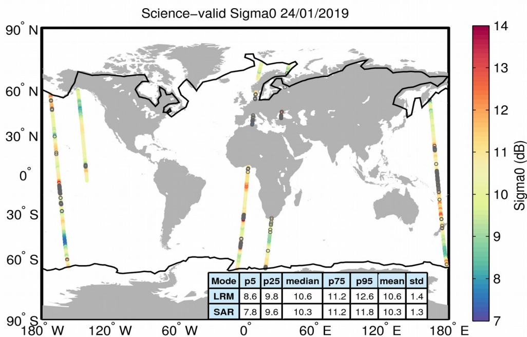
Figure 27. Geographical distribution of science-valid sigma0 data over oceans and lakes for 24/01/2019. The statistical values shown in the table refer to the sigma0 in dB and are calculated separately for LRM and SAR regions. The black lines mark the outer limit of the Arctic and Antarctic polar polygons. Gray circles denote records that have been rejected based on the editing criteria described in Table 4.
