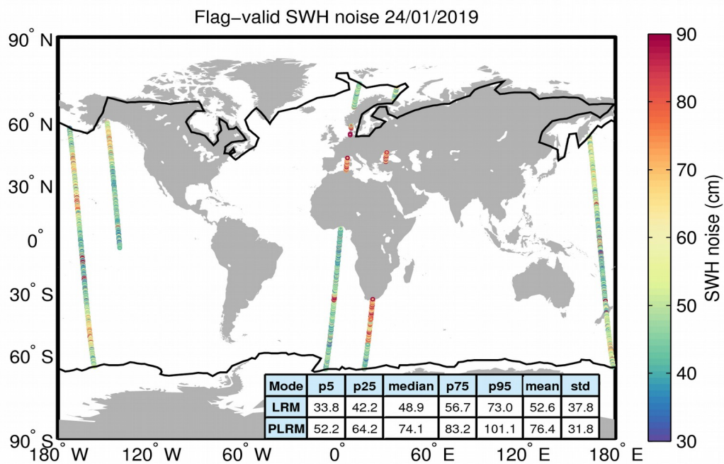
Figure 18. Geographical distribution of flag-valid 20-Hz SWH measurement noise over oceans and lakes for LRM/SAR (top) and LRM/PLRM (bottom) and for 24/01/2019. The statistical values shown in the table refer to the SWH noise and are calculated separately for LRM and SAR/PLRM regions. Measurements taken over polar polygons have been excluded from the computation of the statistical values. The black lines mark the outer limit of the Arctic and Antarctic polar polygons.
