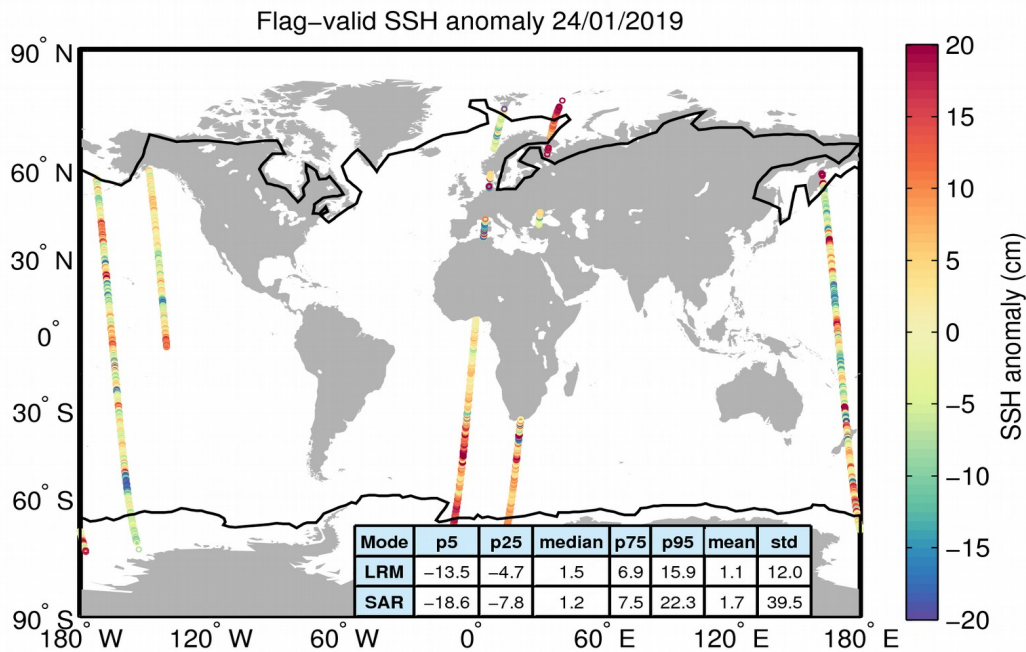
Figure 5. Geographical distribution of flag-valid 1-Hz SSH anomaly data over oceans and lakes for 24/01/2019. The statistical values shown in the table refer to the SSH anomaly in cm and are calculated separately for LRM and SAR regions. Measurements taken over polar polygons have been excluded from the computation of the statistical values. The black lines mark the outer limit of the Arctic and Antarctic polar polygons.
