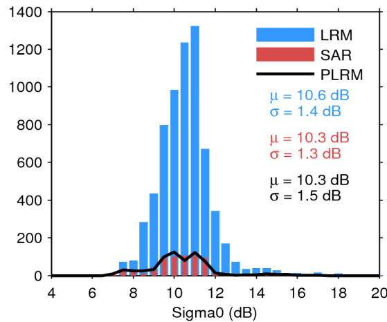
Figure 28. Histogram of science-valid sigma0 over oceans and lakes for LRM (blue), SAR (red), and PLRM (black) for 24/01/2019. The mean ( \mu ) and standard deviation ( \sigma ) are also shown. Note that values outside [4 20] dB are excluded from the histogram for the sake of readability but not from the computation of \mu and \sigma .
