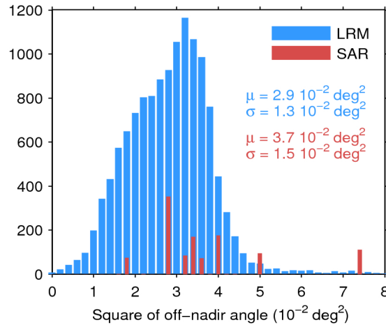
Figure 39. Histogram of flag-valid mispointing over oceans and lakes for LRM (blue) and SAR (red) for 02/08/2018. Only positive values have been considered. The mean ( \mu ) and standard deviation ( \sigma ) are also shown. Note that values larger than 8 \cdot 10^{-2} \text{ deg}^2 are excluded from the histogram for the sake of readability but not from the computation of \mu and \sigma .
