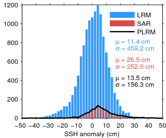
Figure 7. Histogram of flag-valid SSH anomaly over oceans and lakes for LRM (blue), SAR (red), and PLRM (black) for 02/08/2018. The mean ( \mu ) and standard deviation ( \sigma ) are also shown. Note that values outside [-50 50] cm are excluded from the histogram for the sake of readability but not from the computation of \mu and \sigma .
