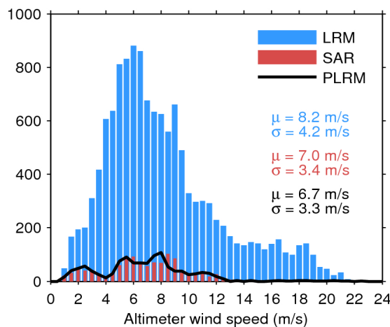
Figure 35. Histogram of science-valid wind over oceans and lakes for LRM (blue), SAR (red), and PLRM (black) for 02/08/2018. The mean ( \mu ) and standard deviation ( \sigma ) are also shown. Note that values larger than 24 m/s are excluded from the histogram for the sake of readability but not from the computation of \mu and \sigma .
