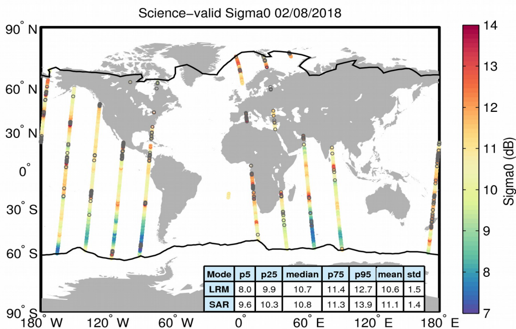
Figure 27. Geographical distribution of science-valid sigma0 data over oceans and lakes for 02/08/2018. The statistical values shown in the table refer to the sigma0 in dB and are calculated separately for LRM and SAR regions. The black lines mark the outer limit of the Arctic and Antarctic polar polygons. Gray circles denote records that have been rejected based on the editing criteria described in Table 4.
