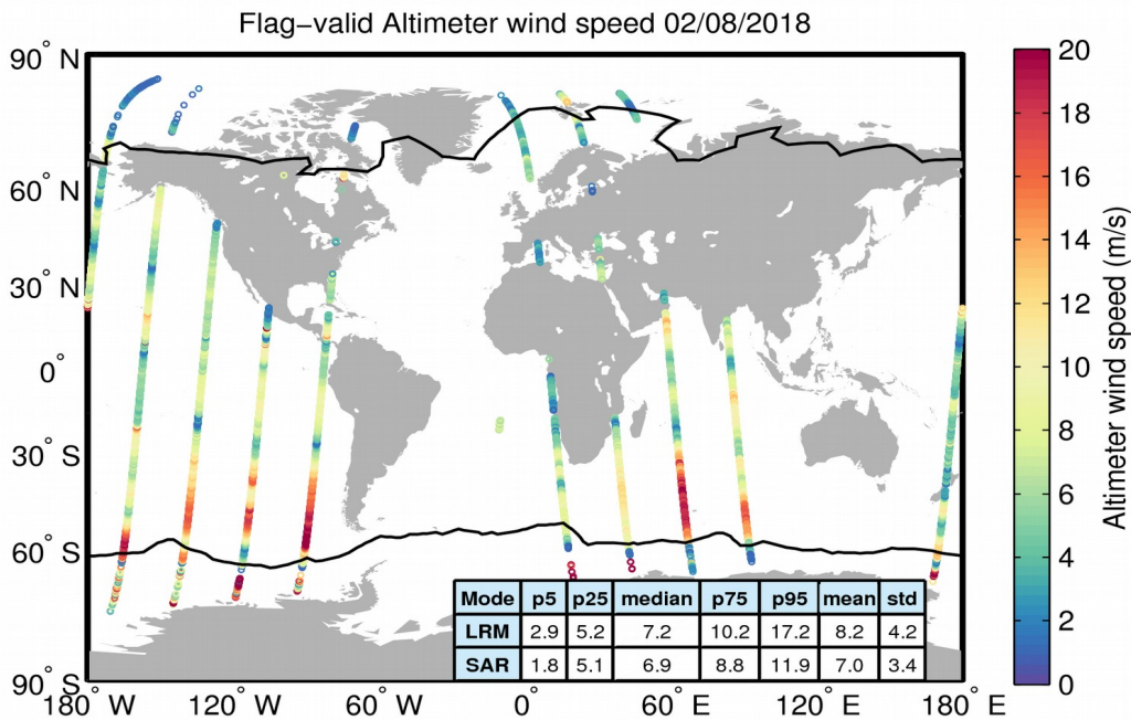
Figure 31. Geographical distribution of flag-valid wind data over oceans and lakes for 02/08/2018. The statistical values shown in the table refer to the wind in m/s and are calculated separately for LRM and SAR regions. Measurements taken over polar polygons have been excluded from the computation of the statistical values. The black lines mark the outer limit of the Arctic and Antarctic polar polygons.
