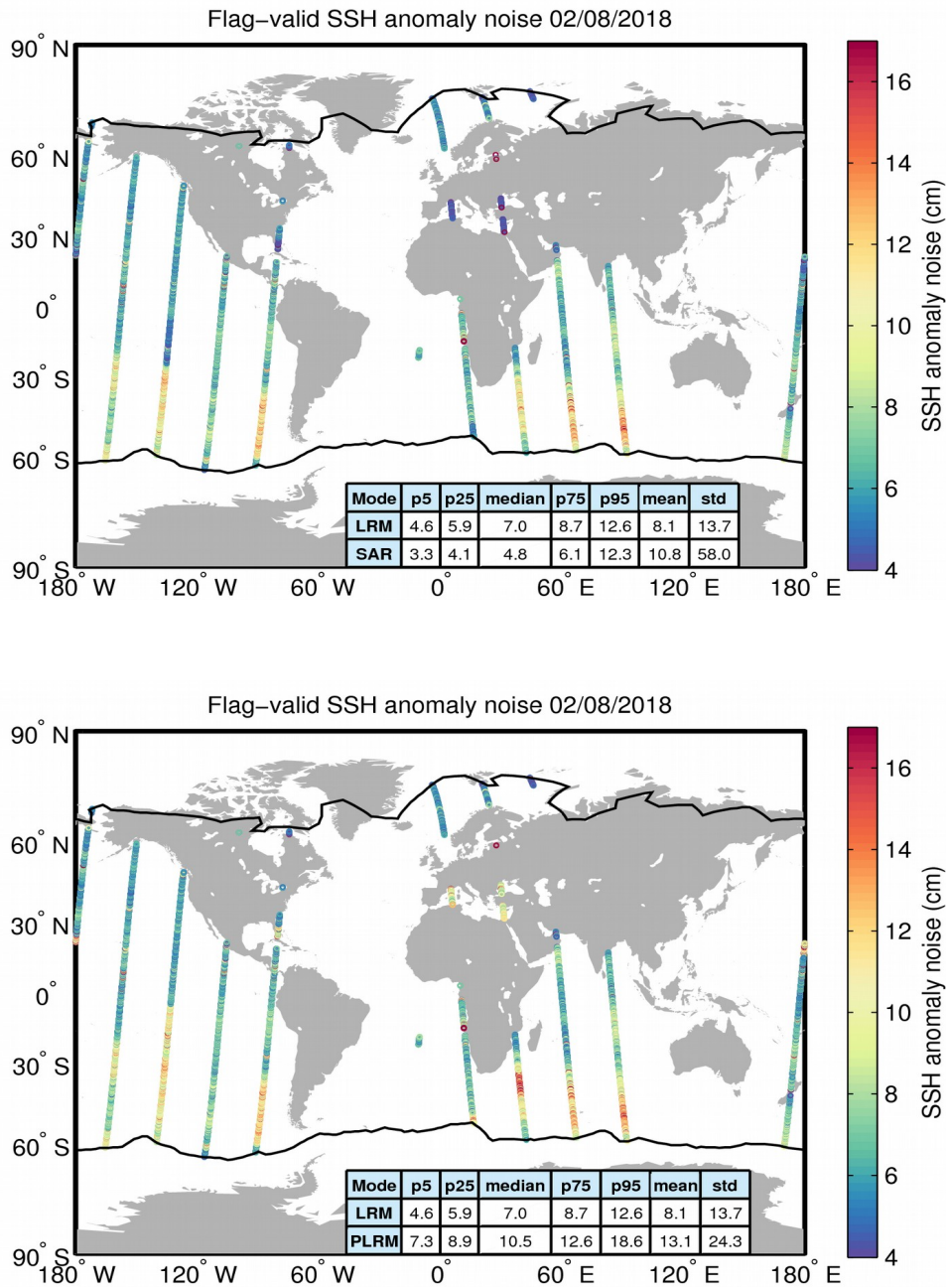
Figure 8. Geographical distribution of flag-valid 20-Hz SSH anomaly measurement noise over oceans and lakes for LRM/SAR (top) and LRM/PLRM (bottom) and for 02/08/2018. The statistical values shown in the tables refer to the SSH anomaly noise and are calculated separately for LRM and SAR/PLRM regions. Measurements taken over polar polygons have been excluded from the computation of the statistical values. The black lines mark the outer limit of the Arctic and Antarctic polar polygons.
