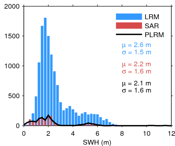
Figure 17. Histogram of flag-valid SWH over oceans and lakes for LRM (blue), SAR (red), and PLRM (black) for 02/08/2018. The mean ( \mu ) and standard deviation ( \sigma ) are also shown. Note that values larger than 12 m are excluded from the histogram for the sake of readability but not from the computation of \mu and \sigma .
