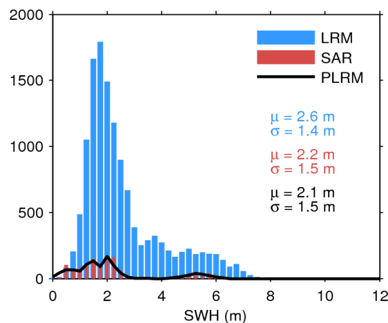
Figure 20. Histogram of science-valid SWH over oceans and lakes for LRM (blue), SAR (red), and PLRM (black) for 02/08/2018. The mean ( \mu ) and standard deviation ( \sigma ) are also
