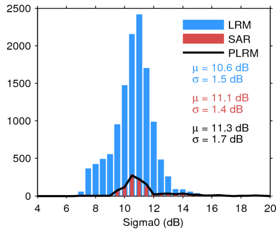
Figure 28. Histogram of science-valid sigma0 over oceans and lakes for LRM (blue), SAR (red), and PLRM (black) for 02/08/2018. The mean ( \mu ) and standard deviation ( \sigma ) are also shown. Note that values outside [4 20] dB are excluded from the histogram for the sake of readability but not from the computation of \mu and \sigma .
