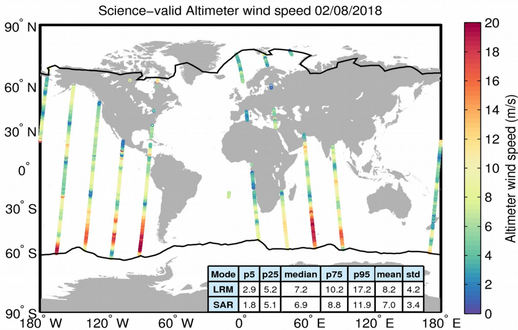
Figure 34. Geographical distribution of science-valid wind data over oceans and lakes for 02/08/2018. The statistical values shown in the table refer to the wind in m/s and are calculated separately for LRM and SAR regions. The black lines mark the outer limit of the Arctic and Antarctic polar polygons. Gray circles denote records that have been rejected based on the editing criteria described in Table 5.
