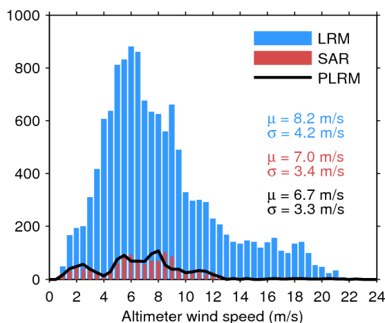
Figure 33. Histogram of flag-valid wind over oceans and lakes for LRM (blue), SAR (red), and PLRM (black) for 02/08/2018. The mean ( \mu ) and standard deviation ( \sigma ) are also shown. Note that values larger than 24 m/s are excluded from the histogram for the sake of readability but not from the computation of \mu and \sigma .
