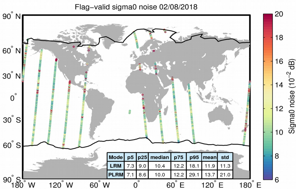
Figure 26. Geographical distribution of flag-valid 20-Hz sigma0 measurement noise over oceans and lakes for LRM/SAR (top) and LRM/PLRM (bottom) and for 02/08/2018. The statistical values shown in the table refer to the sigma0 noise and are calculated separately for LRM and SAR/PLRM regions. Measurements taken over polar polygons have been excluded from the computation of the statistical values. The black lines mark the outer limit of the Arctic and Antarctic polar polygons.
