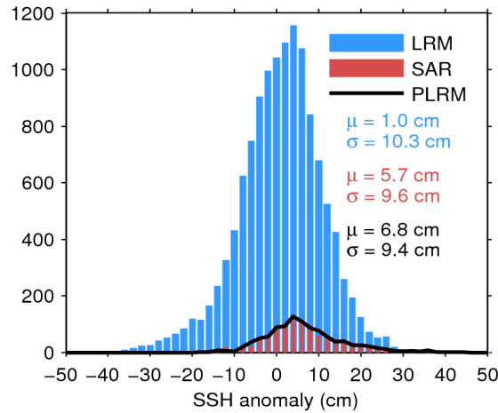
Figure 11. Histogram of science-valid SSH anomaly over oceans and lakes for LRM (blue), SAR (red), and PLRM (black) for 02/08/2018. The mean ( \mu ) and standard deviation ( \sigma ) are also shown. Note that values outside [-50 50] cm are excluded from the histogram for the sake of readability but not from the computation of \mu and \sigma .
