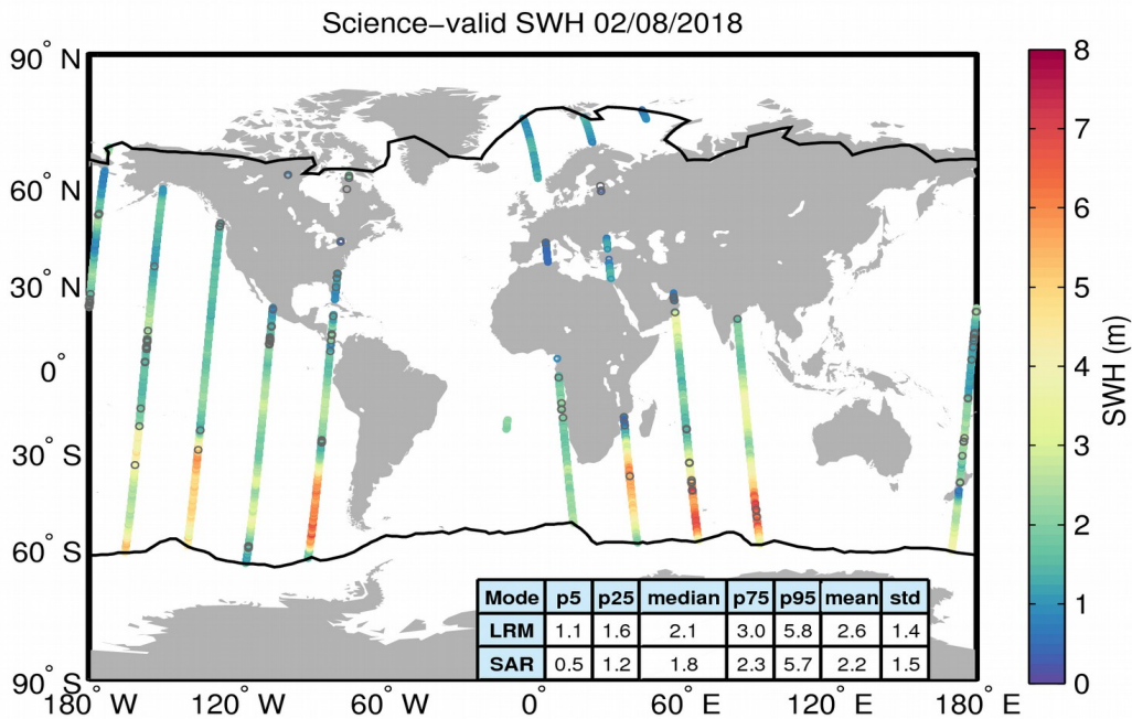
Figure 19. Geographical distribution of science-valid SWH data over oceans and lakes for 02/08/2018. The statistical values shown in the table refer to the SWH in m and are calculated separately for LRM and SAR regions. The black lines mark the outer limit of the Arctic and Antarctic polar polygons. Gray circles denote records that have been rejected based on the editing criteria described in Table 3.
