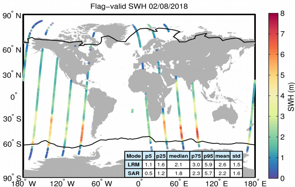
Figure 15. Geographical distribution of flag-valid SWH data over oceans and lakes for 02/08/2018. The statistical values shown in the table refer to the SWH in m and are calculated separately for LRM and SAR regions. Measurements taken over polar polygons
