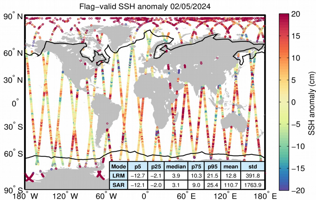
Figure 5. Geographical distribution of flag-valid 1-Hz SSH anomaly data over oceans and lakes for 02/05/2024. The statistical values shown in the table refer to the SSH anomaly in cm and are calculated separately for LRM and SAR regions. Measurements taken over polar polygons have been excluded from the computation of the statistical values. The black lines mark the outer limit of the Arctic and Antarctic polar polygons.
