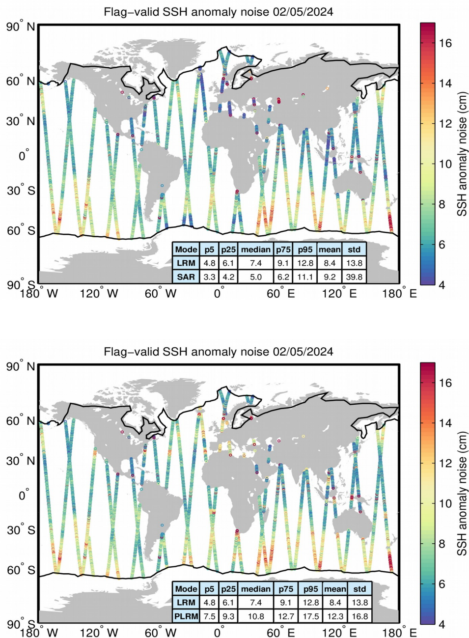
Figure 8. Geographical distribution of flag-valid 20-Hz SSH anomaly measurement noise over oceans and lakes for LRM/SAR (top) and LRM/PLRM (bottom) and for 02/05/2024. The statistical values shown in the tables refer to the SSH anomaly noise and are calculated separately for LRM and SAR/PLRM regions. Measurements taken over polar polygons have been excluded from the computation of the statistical values. The black lines mark the outer limit of the Arctic and Antarctic polar polygons.
