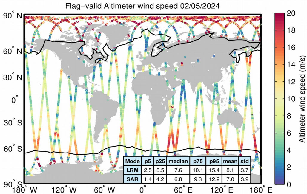
Figure 31. Geographical distribution of flag-valid wind data over oceans and lakes for 02/05/2024. The statistical values shown in the table refer to the wind in m/s and are calculated separately for LRM and SAR regions. Measurements taken over polar polygons have been excluded from the computation of the statistical values. The black lines mark the outer limit of the Arctic and Antarctic polar polygons.
