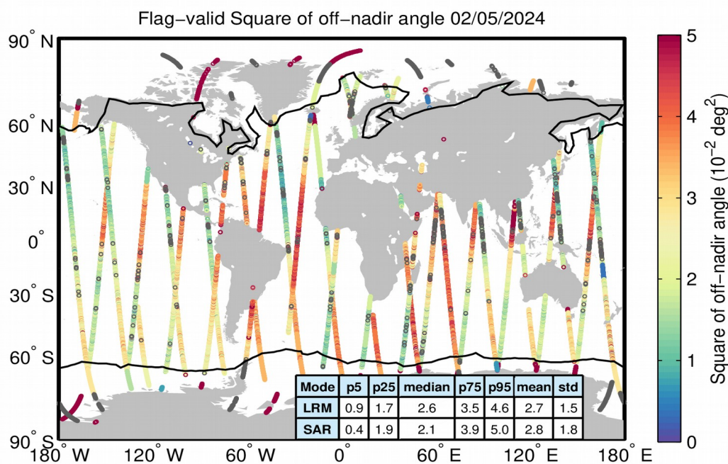
Figure 37. Geographical distribution of flag-valid mispointing data over oceans and lakes for 02/05/2024. The statistical values shown in the table refer to the mispointing in 10^{-2} \text{ deg}^2 and are calculated separately for LRM and SAR regions. Measurements taken over polar polygons have been excluded from the computation of the statistical values. The black lines mark the outer limit of the Arctic and Antarctic polar polygons. Gray circles denote negative values.
