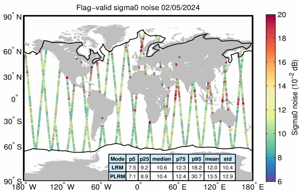
Figure 26. Geographical distribution of flag-valid 20-Hz sigma0 measurement noise over oceans and lakes for LRM/SAR (top) and LRM/PLRM (bottom) and for 02/05/2024. The statistical values shown in the table refer to the sigma0 noise and are calculated separately for LRM and SAR/PLRM regions. Measurements taken over polar polygons have been excluded from the computation of the statistical values. The black lines mark the outer limit of the Arctic and Antarctic polar polygons.
