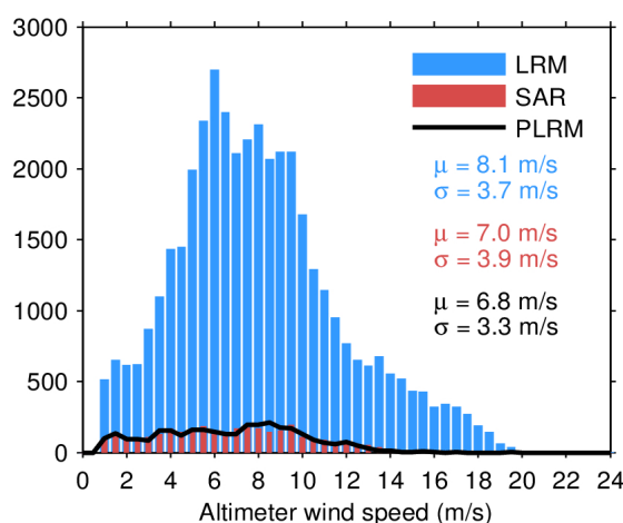
Figure 33. Histogram of flag-valid wind over oceans and lakes for LRM (blue), SAR (red), and PLRM (black) for 02/05/2024. The mean ( \mu ) and standard deviation ( \sigma ) are also shown. Note that values larger than 24 m/s are excluded from the histogram for the sake of readability but not from the computation of \mu and \sigma .
