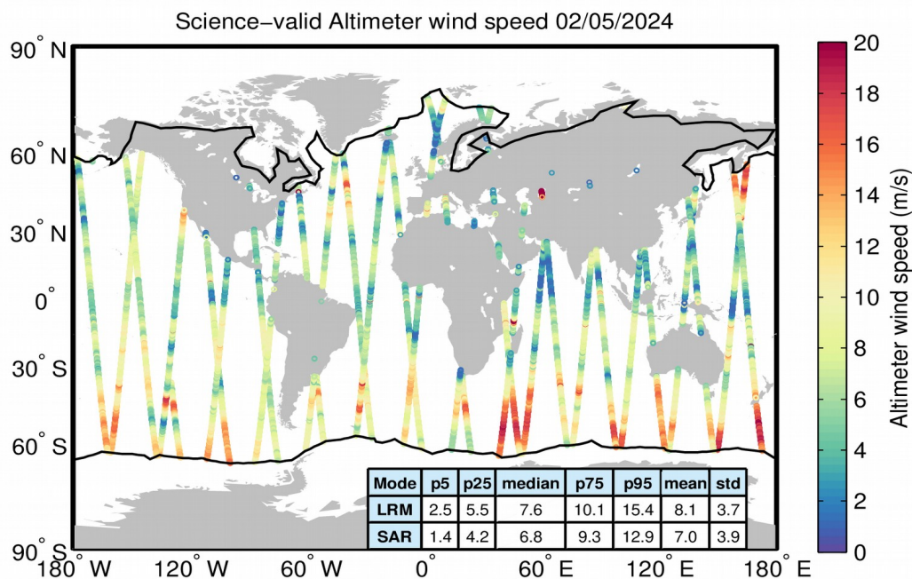
Figure 34. Geographical distribution of science-valid wind data over oceans and lakes for 02/05/2024. The statistical values shown in the table refer to the wind in m/s and are calculated separately for LRM and SAR regions. The black lines mark the outer limit of the Arctic and Antarctic polar polygons. Gray circles denote records that have been rejected based on the editing criteria described in Table 5.
