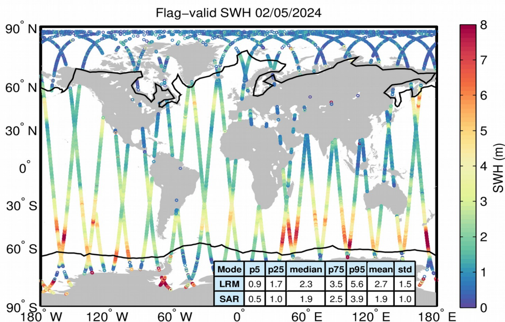
Figure 15. Geographical distribution of flag-valid SWH data over oceans and lakes for 02/05/2024. The statistical values shown in the table refer to the SWH in m and are calculated separately for LRM and SAR regions. Measurements taken over polar polygons have been excluded from the computation of the statistical values. The black lines mark the outer limit of the Arctic and Antarctic polar polygons.
