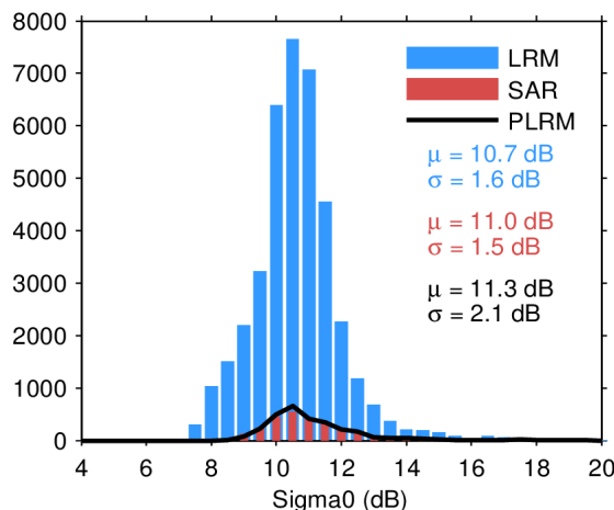
Figure 28. Histogram of science-valid sigma0 over oceans and lakes for LRM (blue), SAR (red), and PLRM (black) for 02/05/2024. The mean ( \mu ) and standard deviation ( \sigma ) are also shown. Note that values outside [4 20] dB are excluded from the histogram for the sake of readability but not from the computation of \mu and \sigma .
