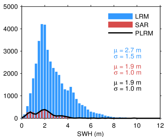
Figure 17. Histogram of flag-valid SWH over oceans and lakes for LRM (blue), SAR (red), and PLRM (black) for 02/05/2024. The mean ( \mu ) and standard deviation ( \sigma ) are also shown. Note that values larger than 12 m are excluded from the histogram for the sake of readability but not from the computation of \mu and \sigma .
