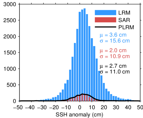
Figure 11. Histogram of science-valid SSH anomaly over oceans and lakes for LRM (blue), SAR (red), and PLRM (black) for 02/05/2024. The mean ( \mu ) and standard deviation ( \sigma ) are also shown. Note that values outside [-50\ 50] cm are excluded from the histogram for the sake of readability but not from the computation of \mu and \sigma .
