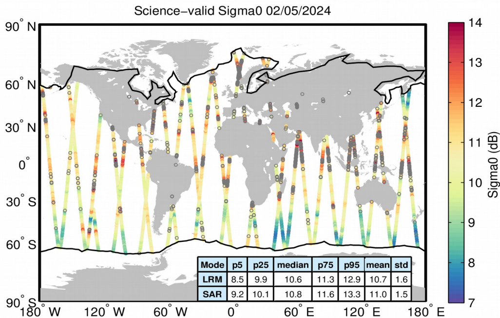
Figure 27. Geographical distribution of science-valid sigma0 data over oceans and lakes for 02/05/2024. The statistical values shown in the table refer to the sigma0 in dB and are calculated separately for LRM and SAR regions. The black lines mark the outer limit of the Arctic and Antarctic polar polygons. Gray circles denote records that have been rejected based on the editing criteria described in Table 4.
