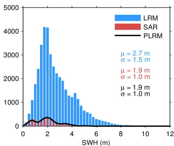
Figure 20. Histogram of science-valid SWH over oceans and lakes for LRM (blue), SAR (red), and PLRM (black) for 02/05/2024. The mean ( \mu ) and standard deviation ( \sigma ) are also
