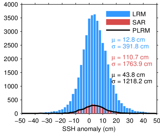
Figure 7. Histogram of flag-valid SSH anomaly over oceans and lakes for LRM (blue), SAR (red), and PLRM (black) for 02/05/2024. The mean ( \mu ) and standard deviation ( \sigma ) are also shown. Note that values outside [-50\ 50] cm are excluded from the histogram for the sake of readability but not from the computation of \mu and \sigma .
