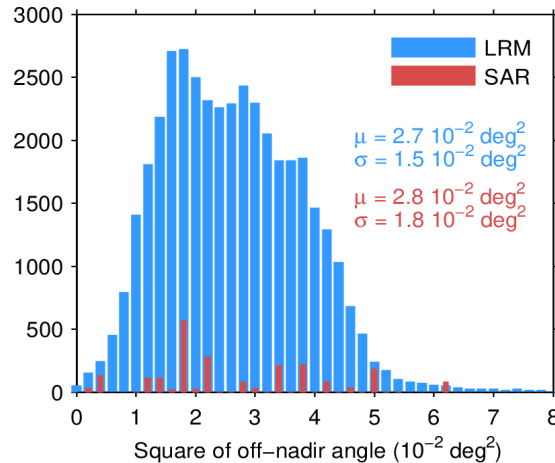
Figure 39. Histogram of flag-valid mispointing over oceans and lakes for LRM (blue) and SAR (red) for 02/05/2024. Only positive values have been considered. The mean ( \mu ) and standard deviation ( \sigma ) are also shown. Note that values larger than 8 \cdot 10^{-2} \text{ deg}^2 are excluded from the histogram for the sake of readability but not from the computation of \mu and \sigma .
