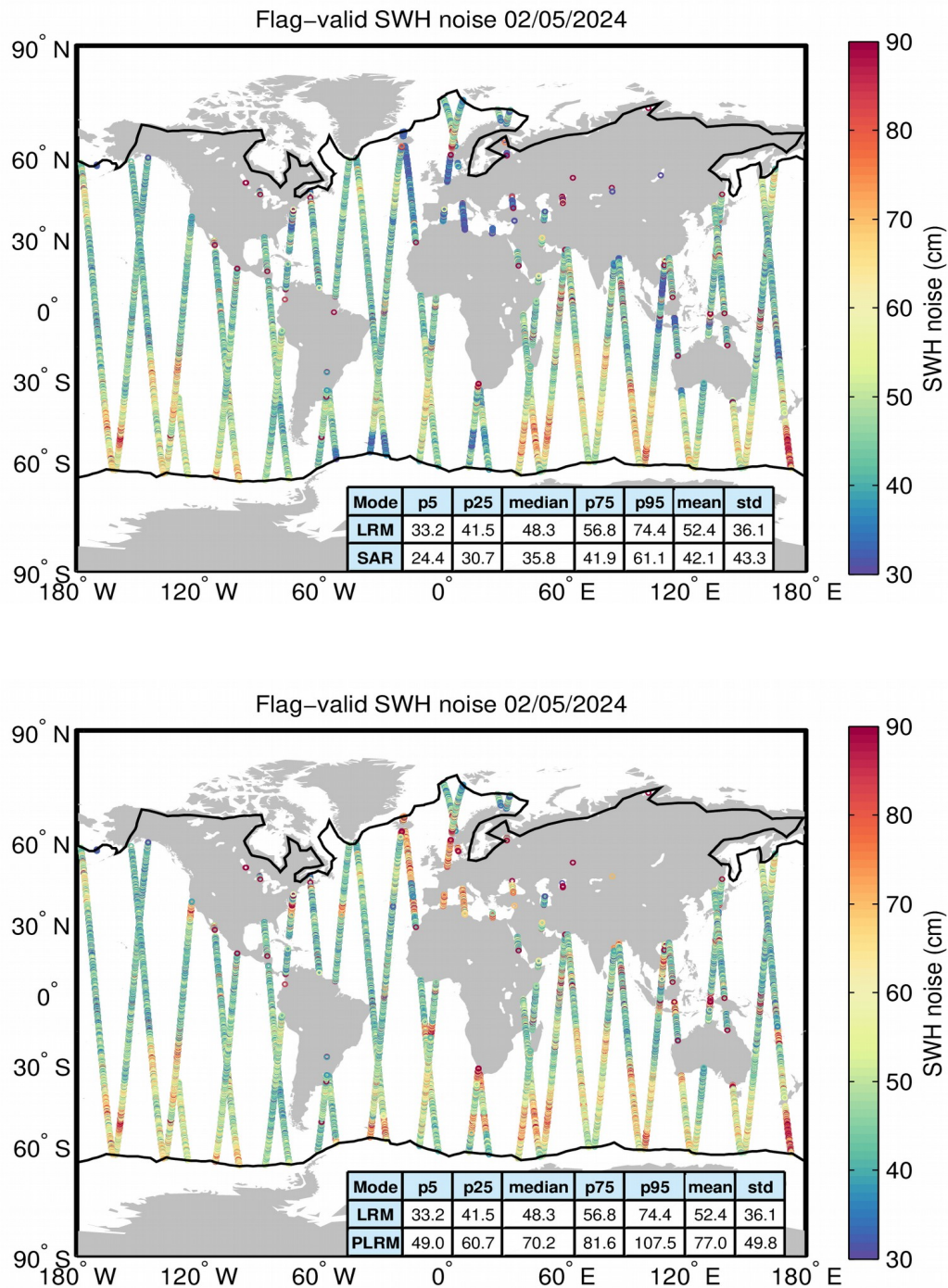
Figure 18. Geographical distribution of flag-valid 20-Hz SWH measurement noise over oceans and lakes for LRM/SAR (top) and LRM/PLRM (bottom) and for 02/05/2024. The statistical values shown in the table refer to the SWH noise and are calculated separately for LRM and SAR/PLRM regions. Measurements taken over polar polygons have been
