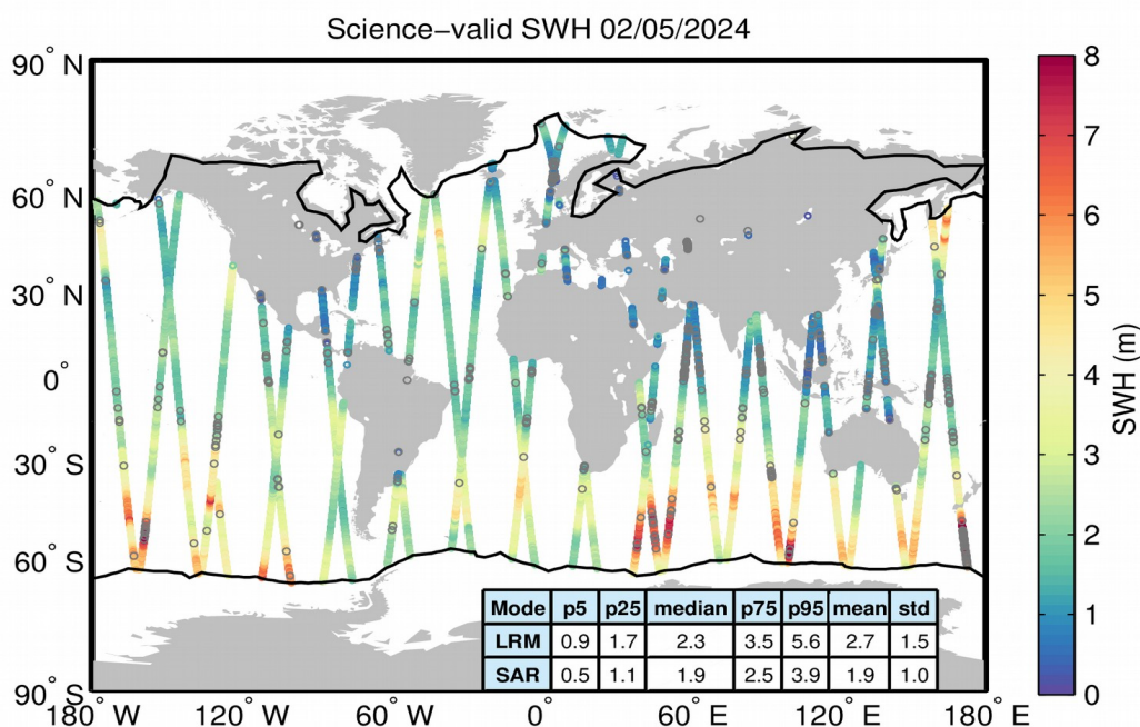
Figure 19. Geographical distribution of science-valid SWH data over oceans and lakes for 02/05/2024. The statistical values shown in the table refer to the SWH in m and are calculated separately for LRM and SAR regions. The black lines mark the outer limit of the Arctic and Antarctic polar polygons. Gray circles denote records that have been rejected based on the editing criteria described in Table 3.
