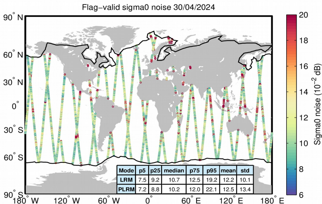
Figure 26. Geographical distribution of flag-valid 20-Hz sigma0 measurement noise over oceans and lakes for LRM/SAR (top) and LRM/PLRM (bottom) and for 30/04/2024. The statistical values shown in the table refer to the sigma0 noise and are calculated separately for LRM and SAR/PLRM regions. Measurements taken over polar polygons have been excluded from the computation of the statistical values. The black lines mark the outer limit of the Arctic and Antarctic polar polygons.
