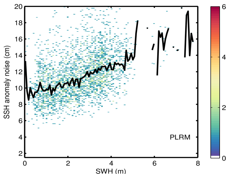
Figure 9. 2D histogram showing flag-valid SSH anomaly noise as a function of SWH for LRM (top), SAR (middle), and PLRM (bottom) for 30/04/2024. The black line denotes the median SSH anomaly noise as a function of SWH.
