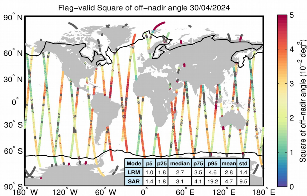
Figure 37. Geographical distribution of flag-valid mispointing data over oceans and lakes for 30/04/2024. The statistical values shown in the table refer to the mispointing in 10^{-2} \text{ deg}^2 and are calculated separately for LRM and SAR regions. Measurements taken over polar polygons have been excluded from the computation of the statistical values. The black lines mark the outer limit of the Arctic and Antarctic polar polygons. Gray circles denote negative values.
