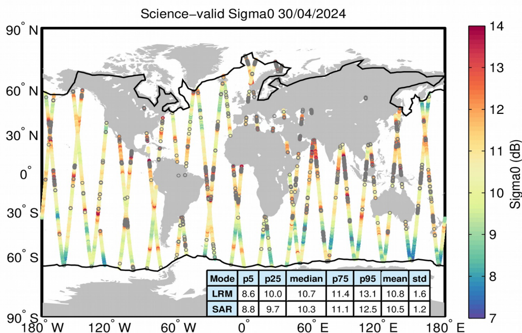
Figure 27. Geographical distribution of science-valid sigma0 data over oceans and lakes for 30/04/2024. The statistical values shown in the table refer to the sigma0 in dB and are calculated separately for LRM and SAR regions. The black lines mark the outer limit of the Arctic and Antarctic polar polygons. Gray circles denote records that have been rejected based on the editing criteria described in Table 4.
