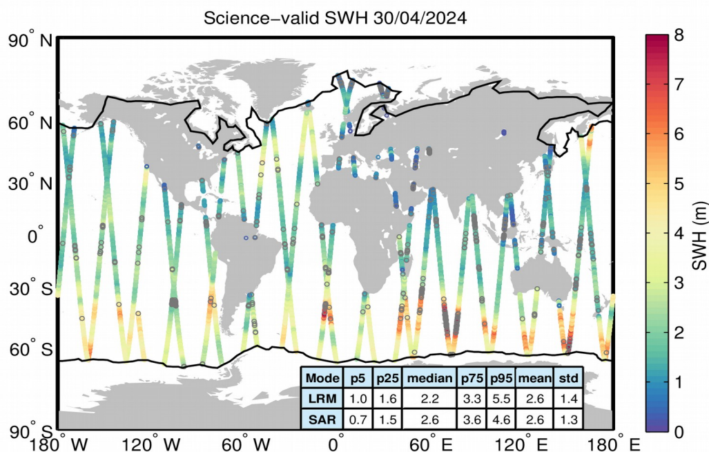
Figure 19. Geographical distribution of science-valid SWH data over oceans and lakes for 30/04/2024. The statistical values shown in the table refer to the SWH in m and are calculated separately for LRM and SAR regions. The black lines mark the outer limit of the Arctic and Antarctic polar polygons. Gray circles denote records that have been rejected based on the editing criteria described in Table 3.
