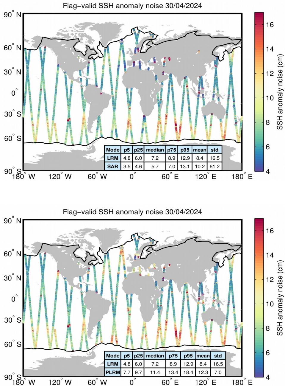
Figure 8. Geographical distribution of flag-valid 20-Hz SSH anomaly measurement noise over oceans and lakes for LRM/SAR (top) and LRM/PLRM (bottom) and for 30/04/2024. The statistical values shown in the tables refer to the SSH anomaly noise and are calculated separately for LRM and SAR/PLRM regions. Measurements taken over polar polygons have been excluded from the computation of the statistical values. The black lines mark the outer limit of the Arctic and Antarctic polar polygons.
