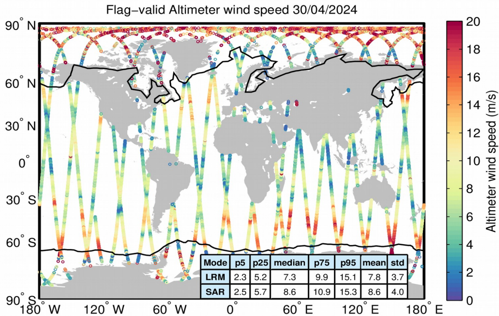
Figure 31. Geographical distribution of flag-valid wind data over oceans and lakes for 30/04/2024. The statistical values shown in the table refer to the wind in m/s and are calculated separately for LRM and SAR regions. Measurements taken over polar polygons have been excluded from the computation of the statistical values. The black lines mark the outer limit of the Arctic and Antarctic polar polygons.
