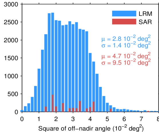
Figure 39. Histogram of flag-valid mispointing over oceans and lakes for LRM (blue) and SAR (red) for 30/04/2024. Only positive values have been considered. The mean ( \mu ) and standard deviation ( \sigma ) are also shown. Note that values larger than 8 \cdot 10^{-2} \text{ deg}^2 are excluded from the histogram for the sake of readability but not from the computation of \mu and \sigma .
