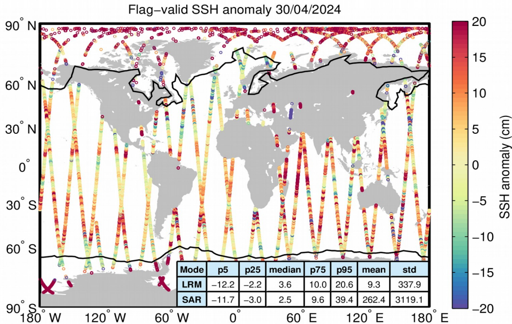
Figure 5. Geographical distribution of flag-valid 1-Hz SSH anomaly data over oceans and lakes for 30/04/2024. The statistical values shown in the table refer to the SSH anomaly in cm and are calculated separately for LRM and SAR regions. Measurements taken over polar polygons have been excluded from the computation of the statistical values. The black lines mark the outer limit of the Arctic and Antarctic polar polygons.
