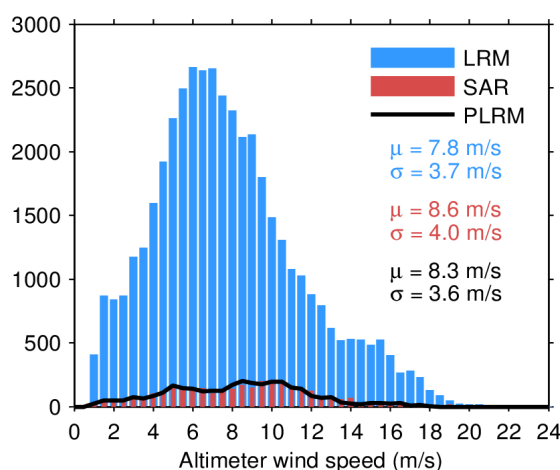
Figure 33. Histogram of flag-valid wind over oceans and lakes for LRM (blue), SAR (red), and PLRM (black) for 30/04/2024. The mean ( \mu ) and standard deviation ( \sigma ) are also shown. Note that values larger than 24 m/s are excluded from the histogram for the sake of readability but not from the computation of \mu and \sigma .
