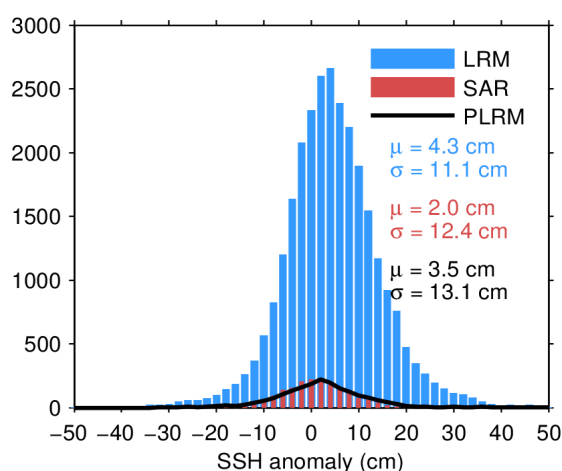
Figure 11. Histogram of science-valid SSH anomaly over oceans and lakes for LRM (blue), SAR (red), and PLRM (black) for 30/04/2024. The mean ( \mu ) and standard deviation ( \sigma ) are also shown. Note that values outside [-50, 50] cm are excluded from the histogram for the sake of readability but not from the computation of \mu and \sigma .
