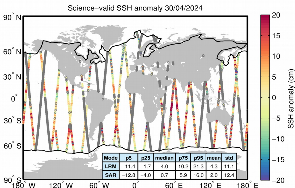
Figure 10. Geographical distribution of science-valid SSH anomaly data over oceans and lakes for 30/04/2024. The statistical values shown in the table refer to the SSH anomaly in cm and are calculated separately for LRM and SAR regions. The black lines mark the
