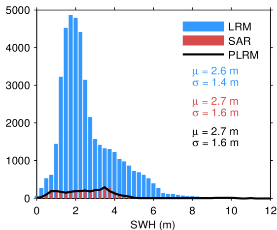
Figure 17. Histogram of flag-valid SWH over oceans and lakes for LRM (blue), SAR (red), and PLRM (black) for 30/04/2024. The mean ( \mu ) and standard deviation ( \sigma ) are also shown. Note that values larger than 12 m are excluded from the histogram for the sake of readability but not from the computation of \mu and \sigma .
