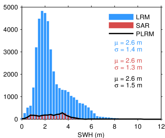
Figure 20. Histogram of science-valid SWH over oceans and lakes for LRM (blue), SAR (red), and PLRM (black) for 30/04/2024. The mean ( \mu ) and standard deviation ( \sigma ) are also
