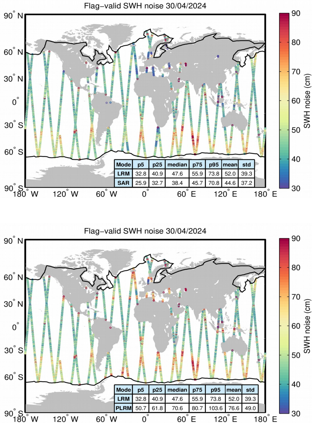
Figure 18. Geographical distribution of flag-valid 20-Hz SWH measurement noise over oceans and lakes for LRM/SAR (top) and LRM/PLRM (bottom) and for 30/04/2024. The statistical values shown in the table refer to the SWH noise and are calculated separately for LRM and SAR/PLRM regions. Measurements taken over polar polygons have been
