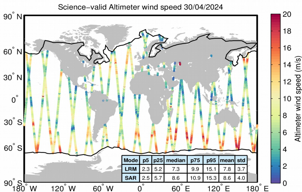
Figure 34. Geographical distribution of science-valid wind data over oceans and lakes for 30/04/2024. The statistical values shown in the table refer to the wind in m/s and are calculated separately for LRM and SAR regions. The black lines mark the outer limit of the Arctic and Antarctic polar polygons. Gray circles denote records that have been rejected based on the editing criteria described in Table 5.
