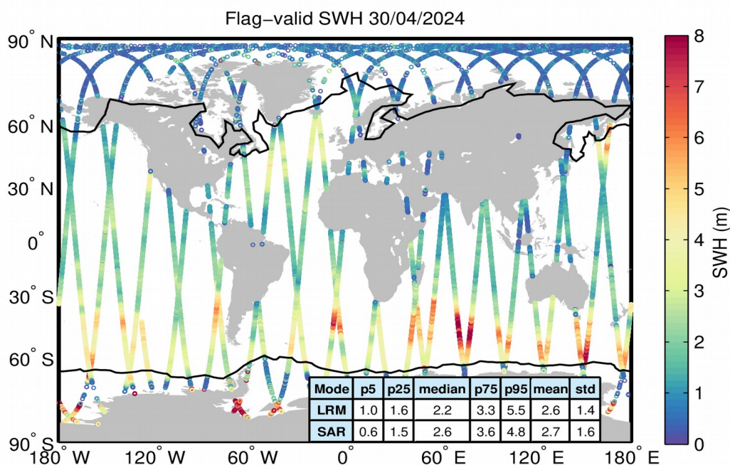
Figure 15. Geographical distribution of flag-valid SWH data over oceans and lakes for 30/04/2024. The statistical values shown in the table refer to the SWH in m and are calculated separately for LRM and SAR regions. Measurements taken over polar polygons have been excluded from the computation of the statistical values. The black lines mark the outer limit of the Arctic and Antarctic polar polygons.
