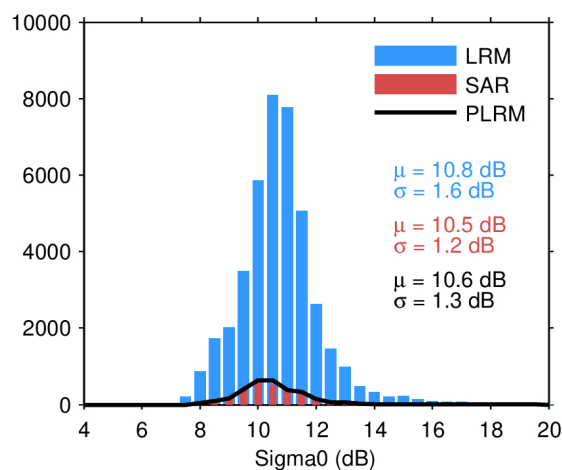
Figure 28. Histogram of science-valid sigma0 over oceans and lakes for LRM (blue), SAR (red), and PLRM (black) for 30/04/2024. The mean ( \mu ) and standard deviation ( \sigma ) are also shown. Note that values outside [4 20] dB are excluded from the histogram for the sake of readability but not from the computation of \mu and \sigma .
