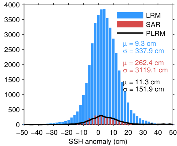
Figure 7. Histogram of flag-valid SSH anomaly over oceans and lakes for LRM (blue), SAR (red), and PLRM (black) for 30/04/2024. The mean ( \mu ) and standard deviation ( \sigma ) are also shown. Note that values outside [-50\ 50] cm are excluded from the histogram for the sake of readability but not from the computation of \mu and \sigma .
