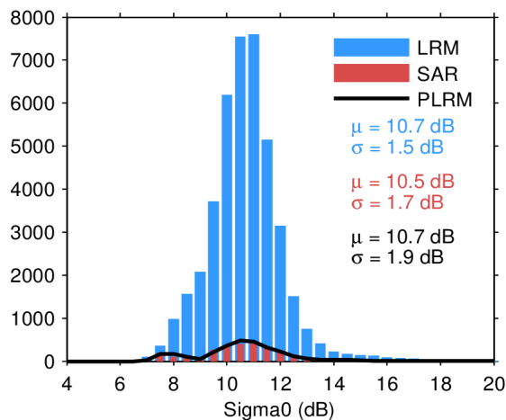
Figure 28. Histogram of science-valid sigma0 over oceans and lakes for LRM (blue), SAR (red), and PLRM (black) for 28/04/2024. The mean ( \mu ) and standard deviation ( \sigma ) are also shown. Note that values outside [4 20] dB are excluded from the histogram for the sake of readability but not from the computation of \mu and \sigma .
