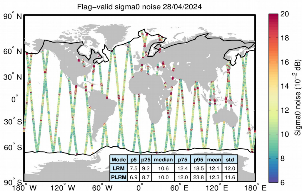
Figure 26. Geographical distribution of flag-valid 20-Hz sigma0 measurement noise over oceans and lakes for LRM/SAR (top) and LRM/PLRM (bottom) and for 28/04/2024. The statistical values shown in the table refer to the sigma0 noise and are calculated separately for LRM and SAR/PLRM regions. Measurements taken over polar polygons have been excluded from the computation of the statistical values. The black lines mark the outer limit of the Arctic and Antarctic polar polygons.
