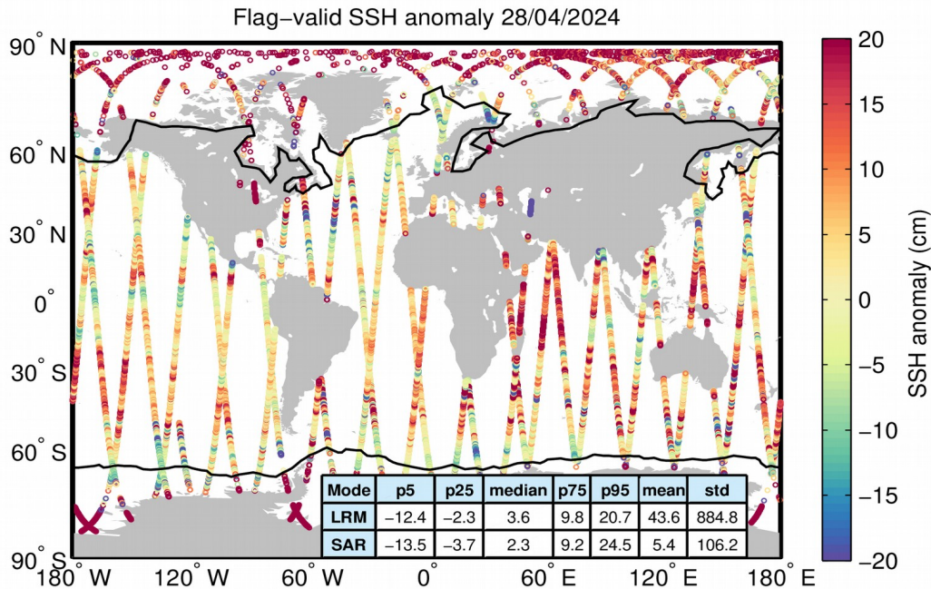
Figure 5. Geographical distribution of flag-valid 1-Hz SSH anomaly data over oceans and lakes for 28/04/2024. The statistical values shown in the table refer to the SSH anomaly in cm and are calculated separately for LRM and SAR regions. Measurements taken over polar polygons have been excluded from the computation of the statistical values. The black lines mark the outer limit of the Arctic and Antarctic polar polygons.
