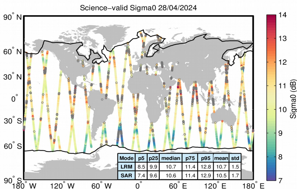
Figure 27. Geographical distribution of science-valid sigma0 data over oceans and lakes for 28/04/2024. The statistical values shown in the table refer to the sigma0 in dB and are calculated separately for LRM and SAR regions. The black lines mark the outer limit of the Arctic and Antarctic polar polygons. Gray circles denote records that have been rejected based on the editing criteria described in Table 4.
