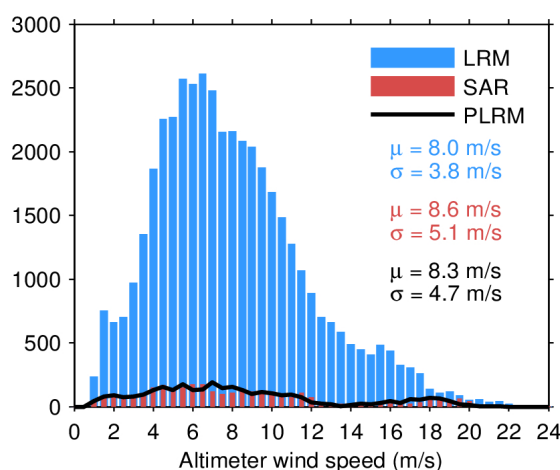
Figure 33. Histogram of flag-valid wind over oceans and lakes for LRM (blue), SAR (red), and PLRM (black) for 28/04/2024. The mean ( \mu ) and standard deviation ( \sigma ) are also shown. Note that values larger than 24 m/s are excluded from the histogram for the sake of readability but not from the computation of \mu and \sigma .
