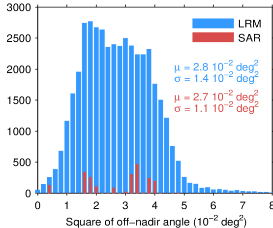
Figure 39. Histogram of flag-valid mispointing over oceans and lakes for LRM (blue) and SAR (red) for 28/04/2024. Only positive values have been considered. The mean ( \mu ) and standard deviation ( \sigma ) are also shown. Note that values larger than 8 \cdot 10^{-2} \text{ deg}^2 are excluded from the histogram for the sake of readability but not from the computation of \mu and \sigma .
