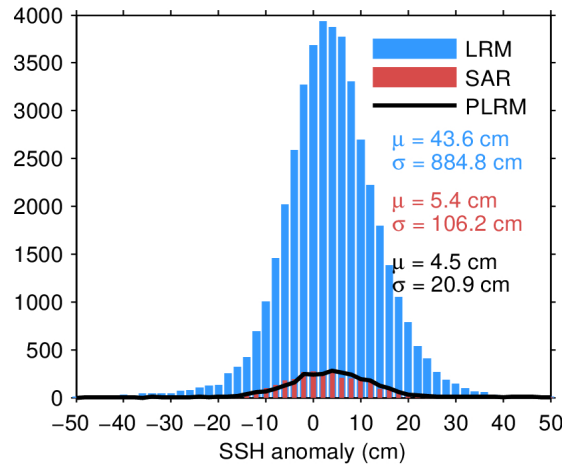
Figure 7. Histogram of flag-valid SSH anomaly over oceans and lakes for LRM (blue), SAR (red), and PLRM (black) for 28/04/2024. The mean ( \mu ) and standard deviation ( \sigma ) are also shown. Note that values outside [-50 50] cm are excluded from the histogram for the sake of readability but not from the computation of \mu and \sigma .
