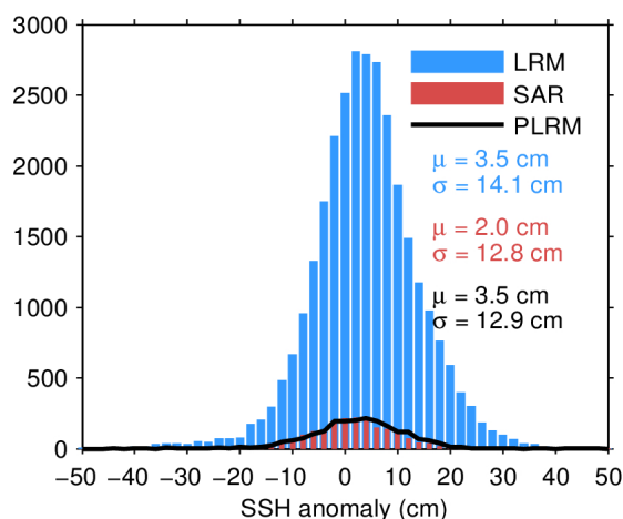
Figure 11. Histogram of science-valid SSH anomaly over oceans and lakes for LRM (blue), SAR (red), and PLRM (black) for 28/04/2024. The mean ( \mu ) and standard deviation ( \sigma ) are also shown. Note that values outside [-50, 50] cm are excluded from the histogram for the sake of readability but not from the computation of \mu and \sigma .
