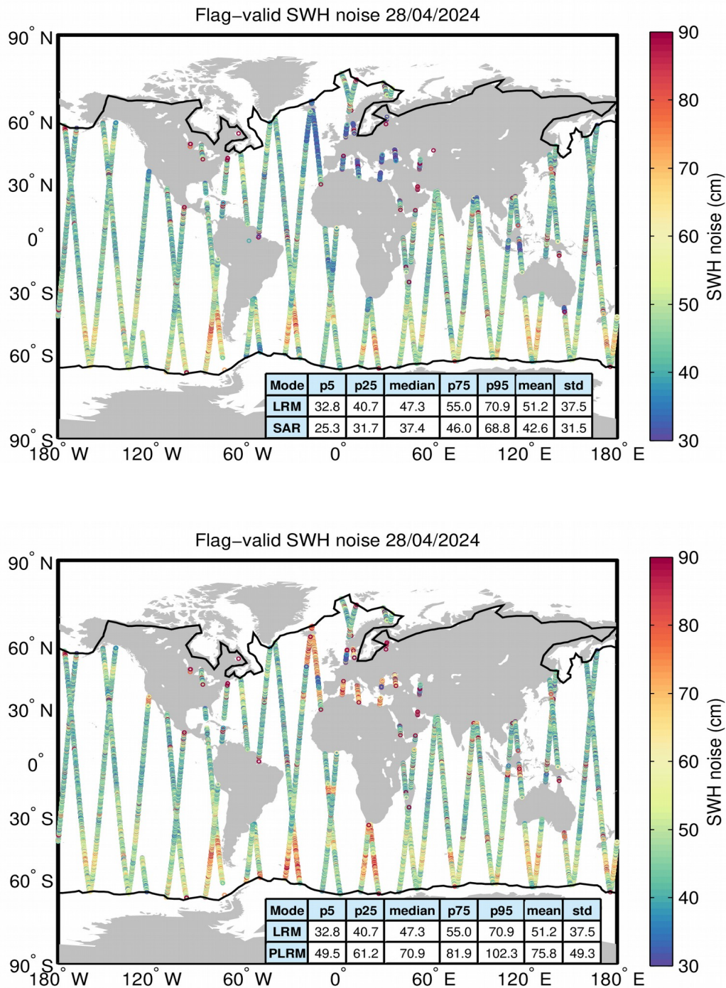
Figure 18. Geographical distribution of flag-valid 20-Hz SWH measurement noise over oceans and lakes for LRM/SAR (top) and LRM/PLRM (bottom) and for 28/04/2024. The statistical values shown in the table refer to the SWH noise and are calculated separately for LRM and SAR/PLRM regions. Measurements taken over polar polygons have been
