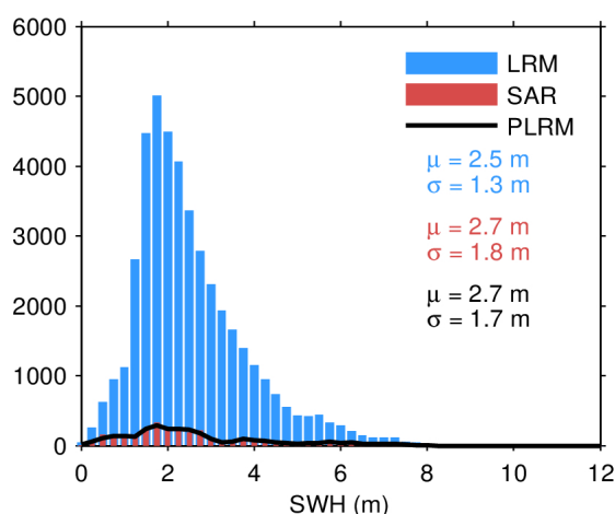
Figure 20. Histogram of science-valid SWH over oceans and lakes for LRM (blue), SAR (red), and PLRM (black) for 28/04/2024. The mean ( \mu ) and standard deviation ( \sigma ) are also
