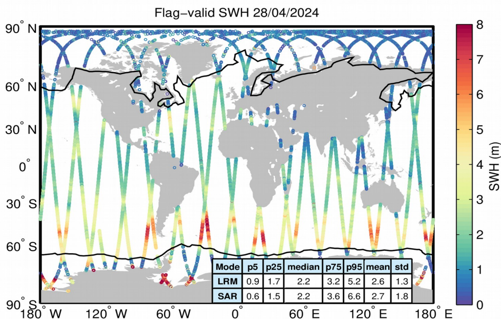
Figure 15. Geographical distribution of flag-valid SWH data over oceans and lakes for 28/04/2024. The statistical values shown in the table refer to the SWH in m and are calculated separately for LRM and SAR regions. Measurements taken over polar polygons have been excluded from the computation of the statistical values. The black lines mark the outer limit of the Arctic and Antarctic polar polygons.
