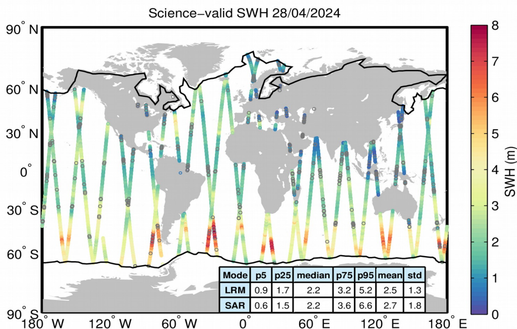
Figure 19. Geographical distribution of science-valid SWH data over oceans and lakes for 28/04/2024. The statistical values shown in the table refer to the SWH in m and are calculated separately for LRM and SAR regions. The black lines mark the outer limit of the Arctic and Antarctic polar polygons. Gray circles denote records that have been rejected based on the editing criteria described in Table 3.
