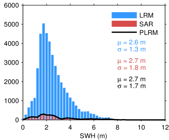
Figure 17. Histogram of flag-valid SWH over oceans and lakes for LRM (blue), SAR (red), and PLRM (black) for 28/04/2024. The mean ( \mu ) and standard deviation ( \sigma ) are also shown. Note that values larger than 12 m are excluded from the histogram for the sake of readability but not from the computation of \mu and \sigma .
