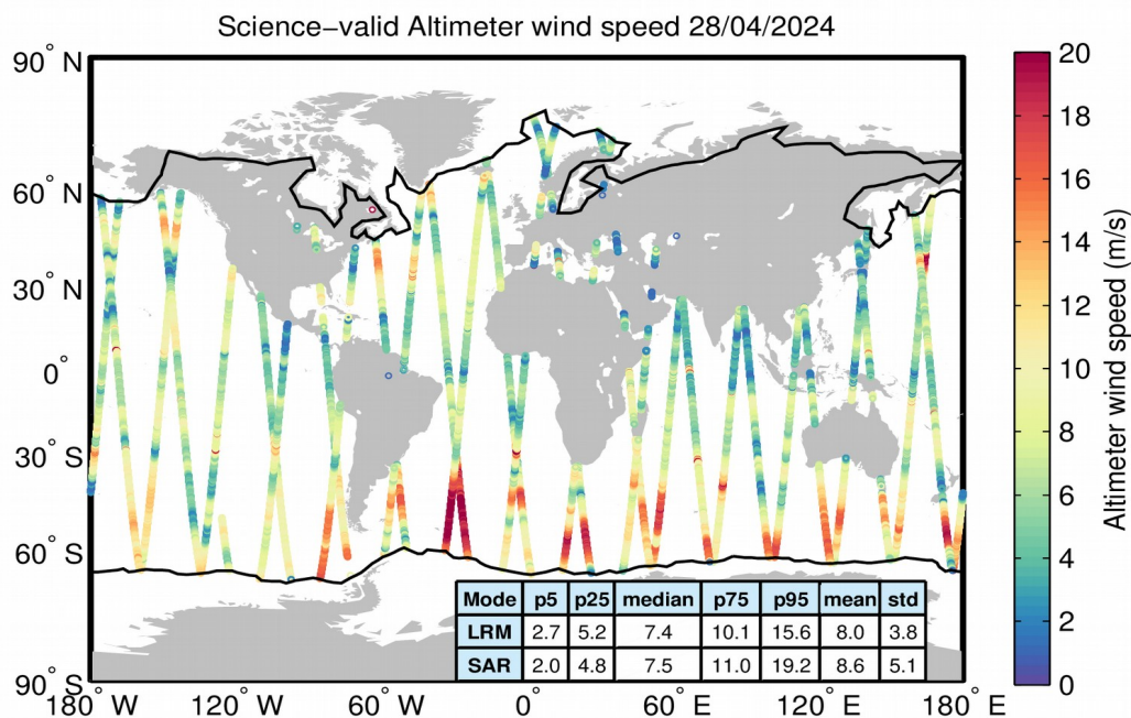
Figure 34. Geographical distribution of science-valid wind data over oceans and lakes for 28/04/2024. The statistical values shown in the table refer to the wind in m/s and are calculated separately for LRM and SAR regions. The black lines mark the outer limit of the Arctic and Antarctic polar polygons. Gray circles denote records that have been rejected based on the editing criteria described in Table 5.
