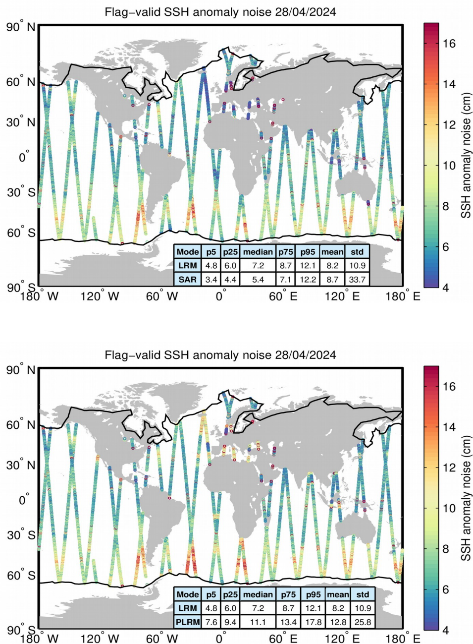
Figure 8. Geographical distribution of flag-valid 20-Hz SSH anomaly measurement noise over oceans and lakes for LRM/SAR (top) and LRM/PLRM (bottom) and for 28/04/2024. The statistical values shown in the tables refer to the SSH anomaly noise and are calculated separately for LRM and SAR/PLRM regions. Measurements taken over polar polygons have been excluded from the computation of the statistical values. The black lines mark the outer limit of the Arctic and Antarctic polar polygons.
