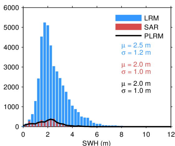
Figure 20. Histogram of science-valid SWH over oceans and lakes for LRM (blue), SAR (red), and PLRM (black) for 27/04/2024. The mean ( \mu ) and standard deviation ( \sigma ) are also
