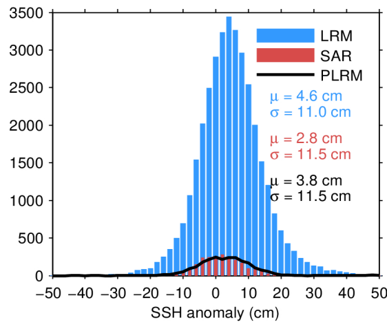
Figure 11. Histogram of science-valid SSH anomaly over oceans and lakes for LRM (blue), SAR (red), and PLRM (black) for 26/04/2024. The mean ( \mu ) and standard deviation ( \sigma ) are also shown. Note that values outside [-50\ 50] cm are excluded from the histogram for the sake of readability but not from the computation of \mu and \sigma .
