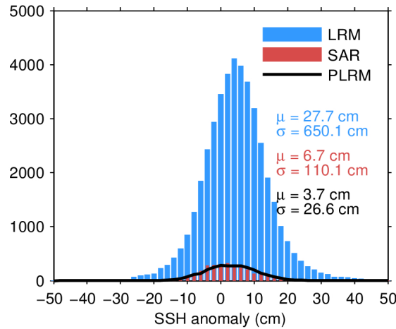
Figure 7. Histogram of flag-valid SSH anomaly over oceans and lakes for LRM (blue), SAR (red), and PLRM (black) for 26/04/2024. The mean ( \mu ) and standard deviation ( \sigma ) are also shown. Note that values outside [-50\ 50] cm are excluded from the histogram for the sake of readability but not from the computation of \mu and \sigma .
