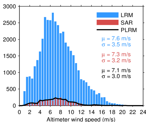
Figure 33. Histogram of flag-valid wind over oceans and lakes for LRM (blue), SAR (red), and PLRM (black) for 26/04/2024. The mean ( \mu ) and standard deviation ( \sigma ) are also shown. Note that values larger than 24 m/s are excluded from the histogram for the sake of readability but not from the computation of \mu and \sigma .
