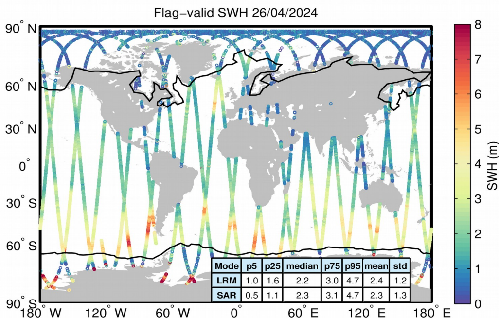
Figure 15. Geographical distribution of flag-valid SWH data over oceans and lakes for 26/04/2024. The statistical values shown in the table refer to the SWH in m and are calculated separately for LRM and SAR regions. Measurements taken over polar polygons have been excluded from the computation of the statistical values. The black lines mark the outer limit of the Arctic and Antarctic polar polygons.
