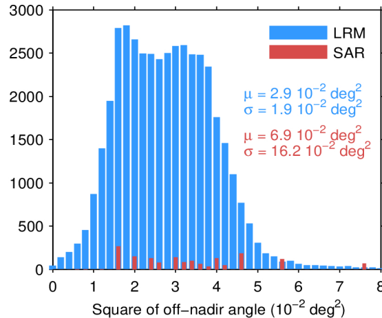
Figure 39. Histogram of flag-valid mispointing over oceans and lakes for LRM (blue) and SAR (red) for 26/04/2024. Only positive values have been considered. The mean ( \mu ) and standard deviation ( \sigma ) are also shown. Note that values larger than 8 \cdot 10^{-2} \text{ deg}^2 are excluded from the histogram for the sake of readability but not from the computation of \mu and \sigma .
