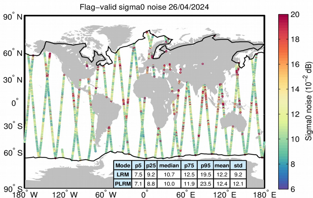
Figure 26. Geographical distribution of flag-valid 20-Hz sigma0 measurement noise over oceans and lakes for LRM/SAR (top) and LRM/PLRM (bottom) and for 26/04/2024. The statistical values shown in the table refer to the sigma0 noise and are calculated separately for LRM and SAR/PLRM regions. Measurements taken over polar polygons have been excluded from the computation of the statistical values. The black lines mark the outer limit of the Arctic and Antarctic polar polygons.
