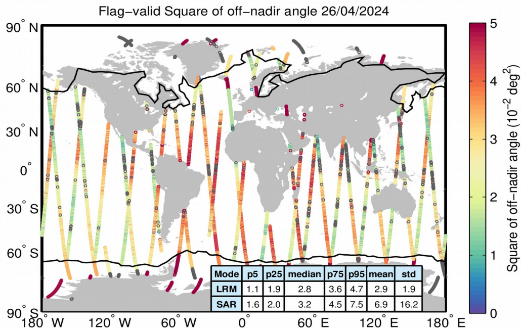
Figure 37. Geographical distribution of flag-valid mispointing data over oceans and lakes for 26/04/2024. The statistical values shown in the table refer to the mispointing in 10^{-2} \text{ deg}^2 and are calculated separately for LRM and SAR regions. Measurements taken over polar polygons have been excluded from the computation of the statistical values. The black lines mark the outer limit of the Arctic and Antarctic polar polygons. Gray circles denote negative values.
