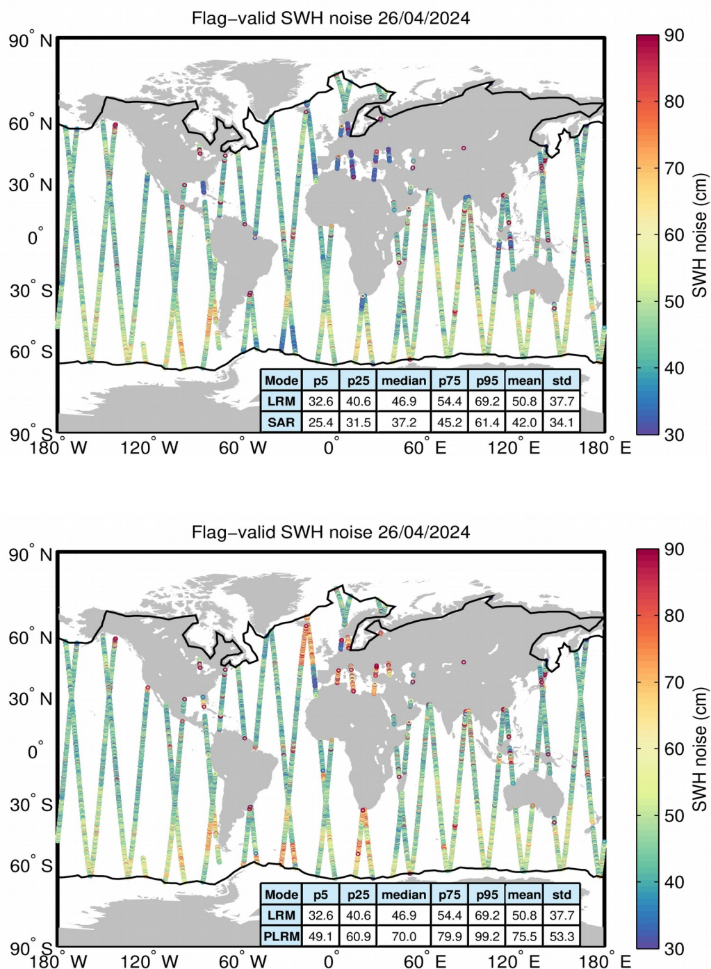
Figure 18. Geographical distribution of flag-valid 20-Hz SWH measurement noise over oceans and lakes for LRM/SAR (top) and LRM/PLRM (bottom) and for 26/04/2024. The statistical values shown in the table refer to the SWH noise and are calculated separately for LRM and SAR/PLRM regions. Measurements taken over polar polygons have been
