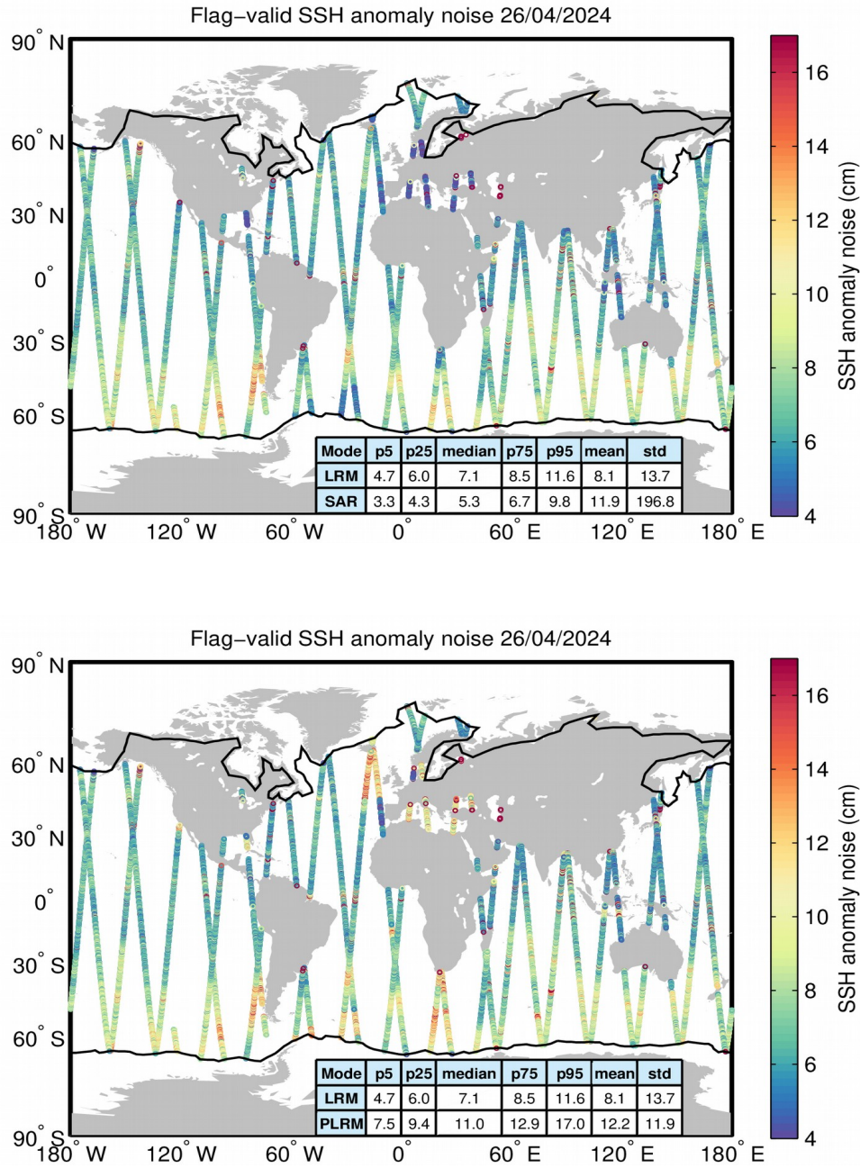
Figure 8. Geographical distribution of flag-valid 20-Hz SSH anomaly measurement noise over oceans and lakes for LRM/SAR (top) and LRM/PLRM (bottom) and for 26/04/2024. The statistical values shown in the tables refer to the SSH anomaly noise and are calculated separately for LRM and SAR/PLRM regions. Measurements taken over polar polygons have been excluded from the computation of the statistical values. The black lines mark the outer limit of the Arctic and Antarctic polar polygons.
