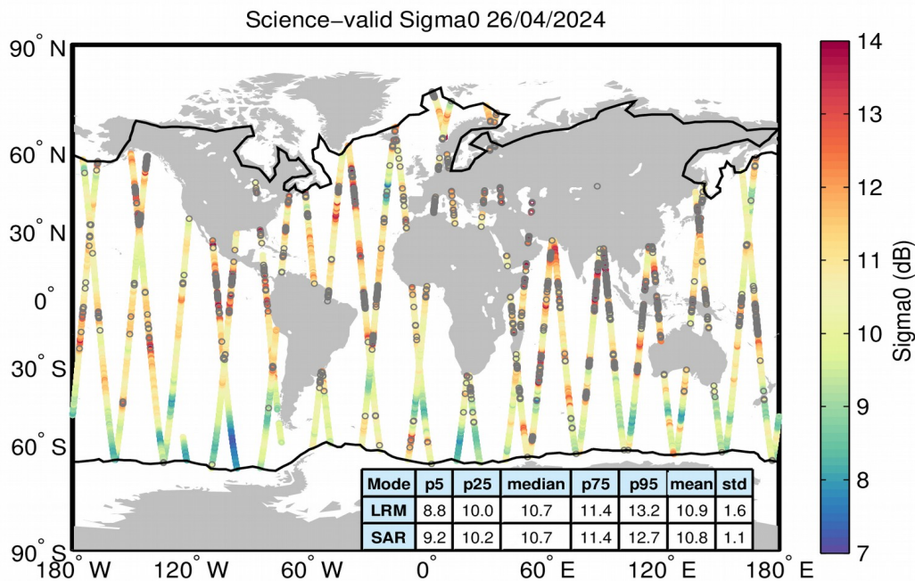
Figure 27. Geographical distribution of science-valid sigma0 data over oceans and lakes for 26/04/2024. The statistical values shown in the table refer to the sigma0 in dB and are calculated separately for LRM and SAR regions. The black lines mark the outer limit of the Arctic and Antarctic polar polygons. Gray circles denote records that have been rejected based on the editing criteria described in Table 4.
