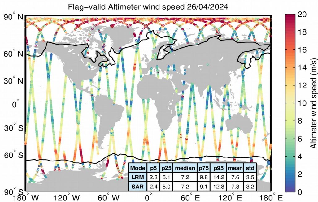
Figure 31. Geographical distribution of flag-valid wind data over oceans and lakes for 26/04/2024. The statistical values shown in the table refer to the wind in m/s and are calculated separately for LRM and SAR regions. Measurements taken over polar polygons have been excluded from the computation of the statistical values. The black lines mark the outer limit of the Arctic and Antarctic polar polygons.
