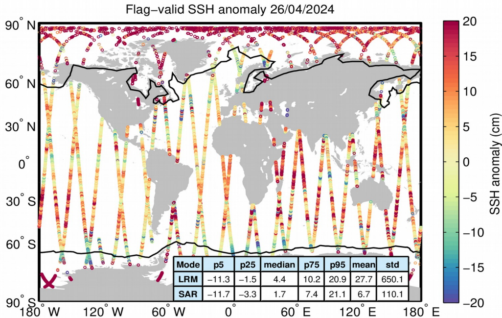
Figure 5. Geographical distribution of flag-valid 1-Hz SSH anomaly data over oceans and lakes for 26/04/2024. The statistical values shown in the table refer to the SSH anomaly in cm and are calculated separately for LRM and SAR regions. Measurements taken over polar polygons have been excluded from the computation of the statistical values. The black lines mark the outer limit of the Arctic and Antarctic polar polygons.
