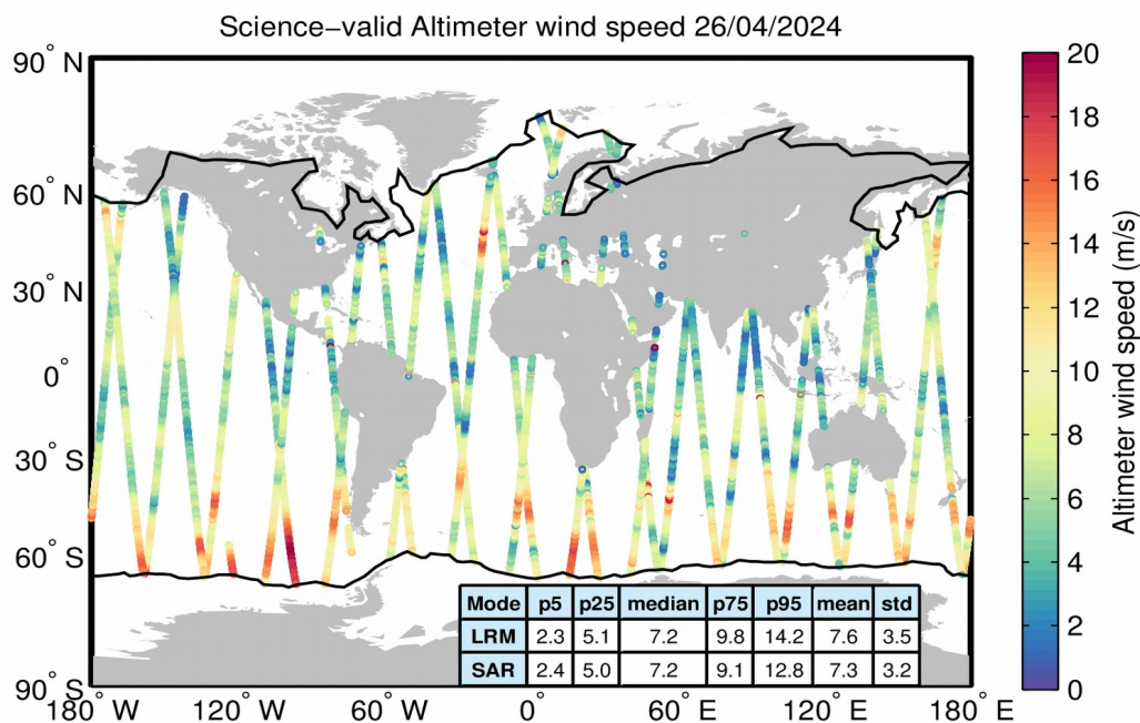
Figure 34. Geographical distribution of science-valid wind data over oceans and lakes for 26/04/2024. The statistical values shown in the table refer to the wind in m/s and are calculated separately for LRM and SAR regions. The black lines mark the outer limit of the Arctic and Antarctic polar polygons. Gray circles denote records that have been rejected based on the editing criteria described in Table 5.
