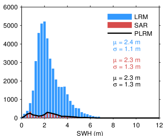
Figure 20. Histogram of science-valid SWH over oceans and lakes for LRM (blue), SAR (red), and PLRM (black) for 26/04/2024. The mean ( \mu ) and standard deviation ( \sigma ) are also
