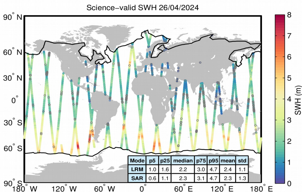
Figure 19. Geographical distribution of science-valid SWH data over oceans and lakes for 26/04/2024. The statistical values shown in the table refer to the SWH in m and are calculated separately for LRM and SAR regions. The black lines mark the outer limit of the Arctic and Antarctic polar polygons. Gray circles denote records that have been rejected based on the editing criteria described in Table 3.
