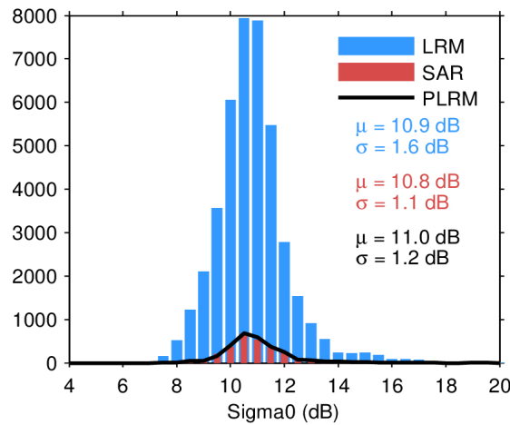
Figure 28. Histogram of science-valid sigma0 over oceans and lakes for LRM (blue), SAR (red), and PLRM (black) for 26/04/2024. The mean ( \mu ) and standard deviation ( \sigma ) are also shown. Note that values outside [4 20] dB are excluded from the histogram for the sake of readability but not from the computation of \mu and \sigma .
