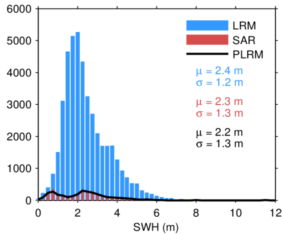
Figure 17. Histogram of flag-valid SWH over oceans and lakes for LRM (blue), SAR (red), and PLRM (black) for 26/04/2024. The mean ( \mu ) and standard deviation ( \sigma ) are also shown. Note that values larger than 12 m are excluded from the histogram for the sake of readability but not from the computation of \mu and \sigma .
