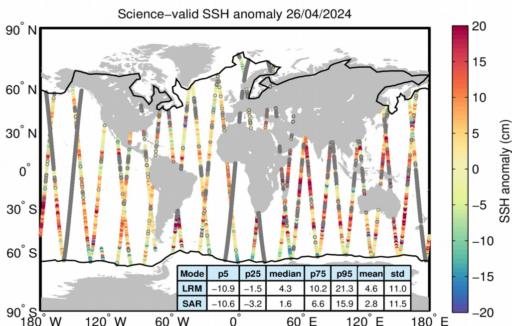
Figure 10. Geographical distribution of science-valid SSH anomaly data over oceans and lakes for 26/04/2024. The statistical values shown in the table refer to the SSH anomaly in cm and are calculated separately for LRM and SAR regions. The black lines mark the
