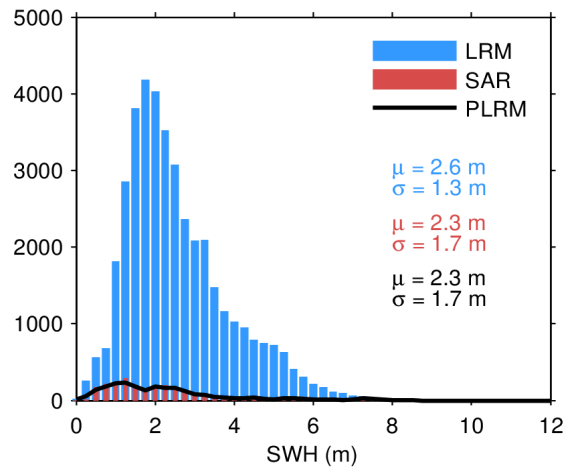
Figure 17. Histogram of flag-valid SWH over oceans and lakes for LRM (blue), SAR (red), and PLRM (black) for 24/04/2024. The mean ( \mu ) and standard deviation ( \sigma ) are also shown. Note that values larger than 12 m are excluded from the histogram for the sake of readability but not from the computation of \mu and \sigma .
