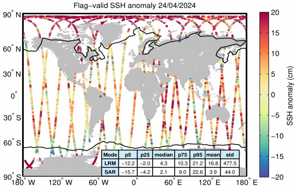
Figure 5. Geographical distribution of flag-valid 1-Hz SSH anomaly data over oceans and lakes for 24/04/2024. The statistical values shown in the table refer to the SSH anomaly in cm and are calculated separately for LRM and SAR regions. Measurements taken over polar polygons have been excluded from the computation of the statistical values. The black lines mark the outer limit of the Arctic and Antarctic polar polygons.
