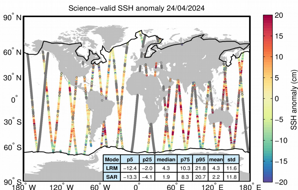
Figure 10. Geographical distribution of science-valid SSH anomaly data over oceans and lakes for 24/04/2024. The statistical values shown in the table refer to the SSH anomaly in cm and are calculated separately for LRM and SAR regions. The black lines mark the
