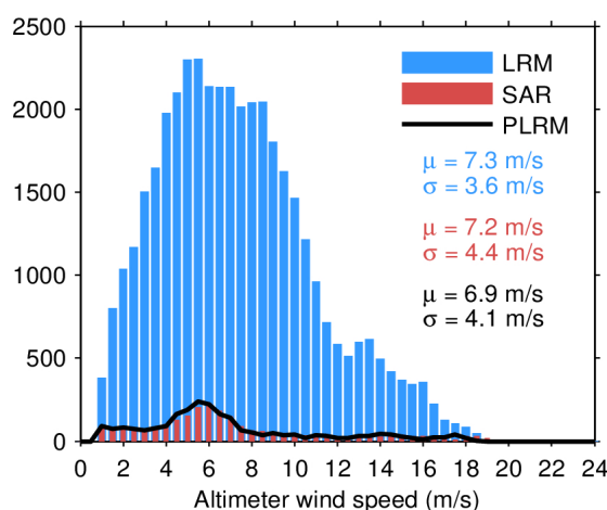
Figure 33. Histogram of flag-valid wind over oceans and lakes for LRM (blue), SAR (red), and PLRM (black) for 24/04/2024. The mean ( \mu ) and standard deviation ( \sigma ) are also shown. Note that values larger than 24 m/s are excluded from the histogram for the sake of readability but not from the computation of \mu and \sigma .
