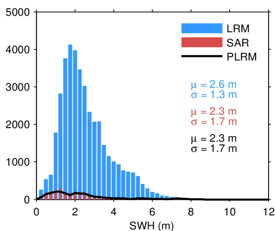
Figure 20. Histogram of science-valid SWH over oceans and lakes for LRM (blue), SAR (red), and PLRM (black) for 24/04/2024. The mean ( \mu ) and standard deviation ( \sigma ) are also
