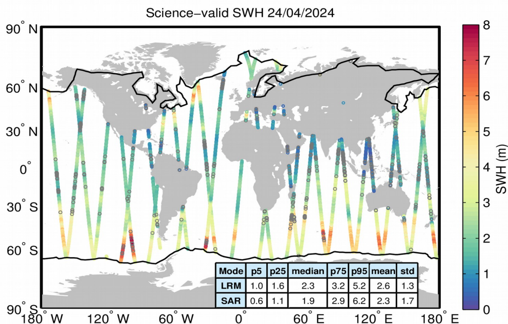
Figure 19. Geographical distribution of science-valid SWH data over oceans and lakes for 24/04/2024. The statistical values shown in the table refer to the SWH in m and are calculated separately for LRM and SAR regions. The black lines mark the outer limit of the Arctic and Antarctic polar polygons. Gray circles denote records that have been rejected based on the editing criteria described in Table 3.
