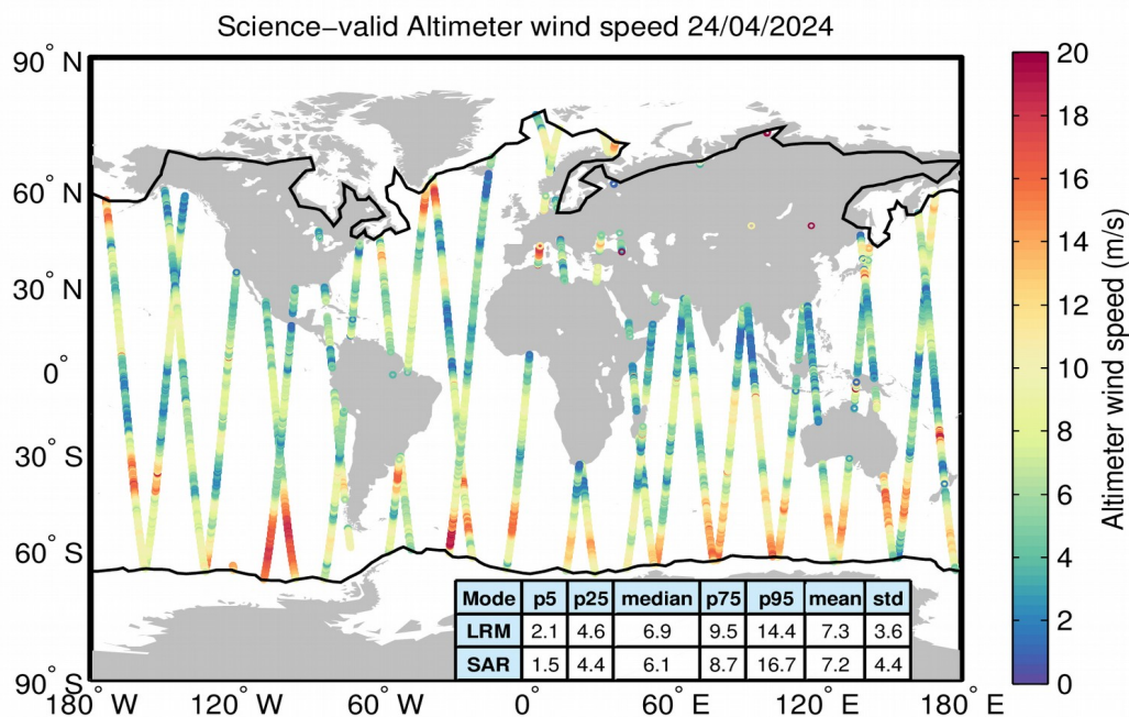
Figure 34. Geographical distribution of science-valid wind data over oceans and lakes for 24/04/2024. The statistical values shown in the table refer to the wind in m/s and are calculated separately for LRM and SAR regions. The black lines mark the outer limit of the Arctic and Antarctic polar polygons. Gray circles denote records that have been rejected based on the editing criteria described in Table 5.
