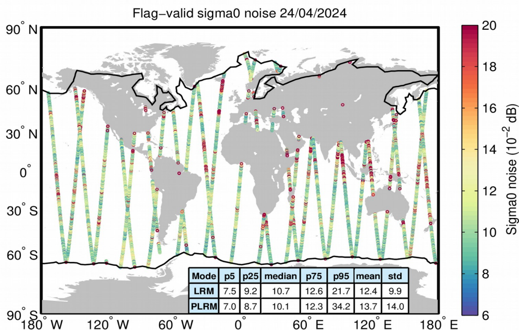
Figure 26. Geographical distribution of flag-valid 20-Hz sigma0 measurement noise over oceans and lakes for LRM/SAR (top) and LRM/PLRM (bottom) and for 24/04/2024. The statistical values shown in the table refer to the sigma0 noise and are calculated separately for LRM and SAR/PLRM regions. Measurements taken over polar polygons have been excluded from the computation of the statistical values. The black lines mark the outer limit of the Arctic and Antarctic polar polygons.
