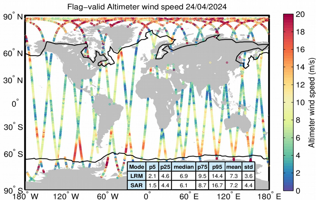
Figure 31. Geographical distribution of flag-valid wind data over oceans and lakes for 24/04/2024. The statistical values shown in the table refer to the wind in m/s and are calculated separately for LRM and SAR regions. Measurements taken over polar polygons have been excluded from the computation of the statistical values. The black lines mark the outer limit of the Arctic and Antarctic polar polygons.
