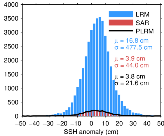
Figure 7. Histogram of flag-valid SSH anomaly over oceans and lakes for LRM (blue), SAR (red), and PLRM (black) for 24/04/2024. The mean ( \mu ) and standard deviation ( \sigma ) are also shown. Note that values outside [-50 50] cm are excluded from the histogram for the sake of readability but not from the computation of \mu and \sigma .
