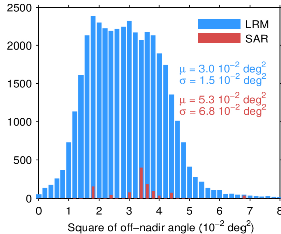
Figure 39. Histogram of flag-valid mispointing over oceans and lakes for LRM (blue) and SAR (red) for 24/04/2024. Only positive values have been considered. The mean ( \mu ) and standard deviation ( \sigma ) are also shown. Note that values larger than 8 \cdot 10^{-2} \text{ deg}^2 are excluded from the histogram for the sake of readability but not from the computation of \mu and \sigma .
