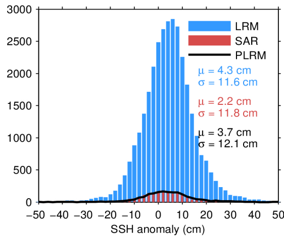
Figure 11. Histogram of science-valid SSH anomaly over oceans and lakes for LRM (blue), SAR (red), and PLRM (black) for 24/04/2024. The mean ( \mu ) and standard deviation ( \sigma ) are also shown. Note that values outside [-50, 50] cm are excluded from the histogram for the sake of readability but not from the computation of \mu and \sigma .
