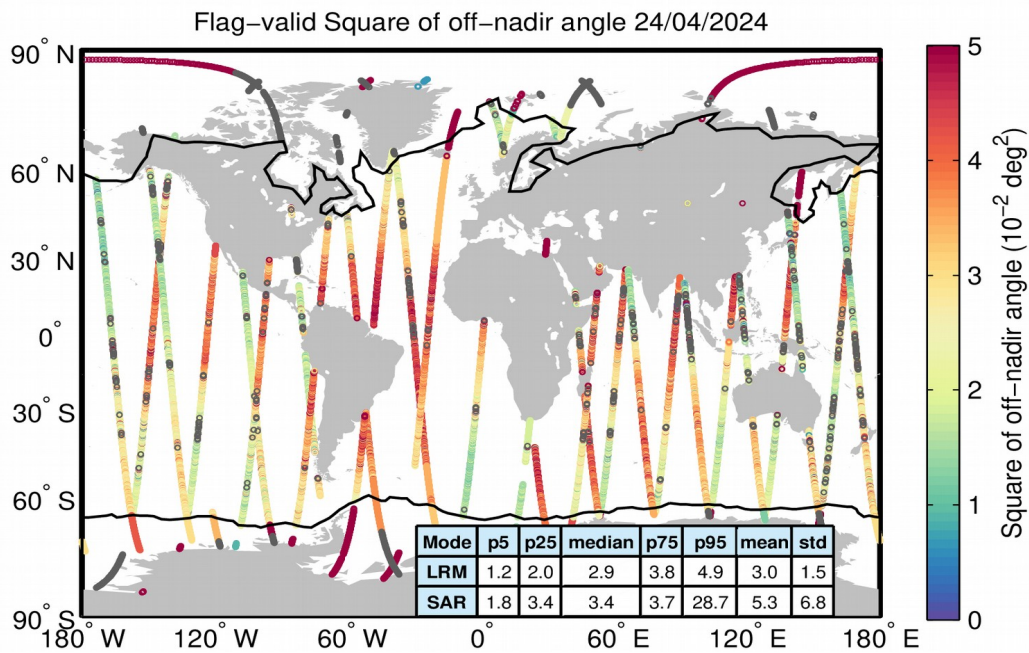
Figure 37. Geographical distribution of flag-valid mispointing data over oceans and lakes for 24/04/2024. The statistical values shown in the table refer to the mispointing in 10^{-2} \text{ deg}^2 and are calculated separately for LRM and SAR regions. Measurements taken over polar polygons have been excluded from the computation of the statistical values. The black lines mark the outer limit of the Arctic and Antarctic polar polygons. Gray circles denote negative values.
