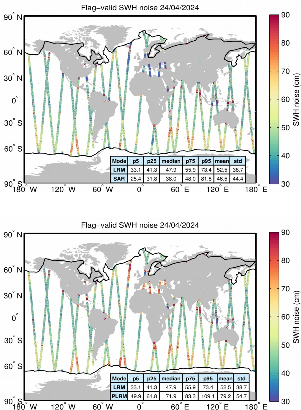
Figure 18. Geographical distribution of flag-valid 20-Hz SWH measurement noise over oceans and lakes for LRM/SAR (top) and LRM/PLRM (bottom) and for 24/04/2024. The statistical values shown in the table refer to the SWH noise and are calculated separately for LRM and SAR/PLRM regions. Measurements taken over polar polygons have been
