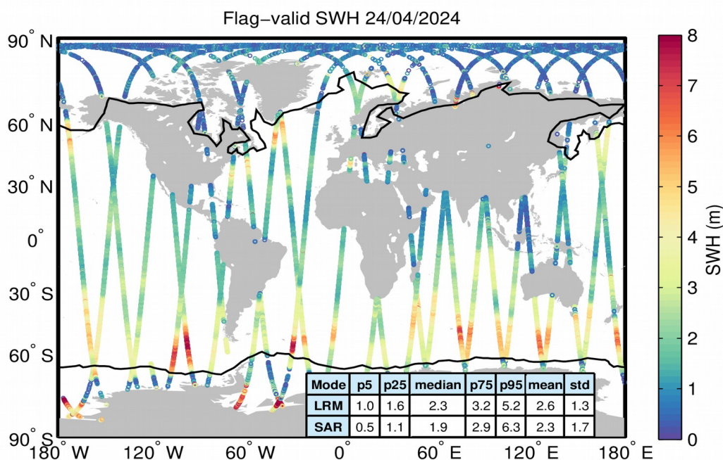
Figure 15. Geographical distribution of flag-valid SWH data over oceans and lakes for 24/04/2024. The statistical values shown in the table refer to the SWH in m and are calculated separately for LRM and SAR regions. Measurements taken over polar polygons have been excluded from the computation of the statistical values. The black lines mark the outer limit of the Arctic and Antarctic polar polygons.
