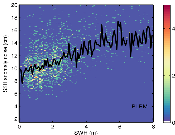
Figure 9. 2D histogram showing flag-valid SSH anomaly noise as a function of SWH for LRM (top), SAR (middle), and PLRM (bottom) for 24/04/2024. The black line denotes the median SSH anomaly noise as a function of SWH.
