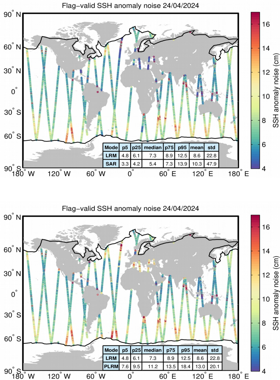
Figure 8. Geographical distribution of flag-valid 20-Hz SSH anomaly measurement noise over oceans and lakes for LRM/SAR (top) and LRM/PLRM (bottom) and for 24/04/2024. The statistical values shown in the tables refer to the SSH anomaly noise and are calculated separately for LRM and SAR/PLRM regions. Measurements taken over polar polygons have been excluded from the computation of the statistical values. The black lines mark the outer limit of the Arctic and Antarctic polar polygons.
