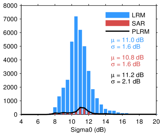
Figure 28. Histogram of science-valid sigma0 over oceans and lakes for LRM (blue), SAR (red), and PLRM (black) for 24/04/2024. The mean ( \mu ) and standard deviation ( \sigma ) are also shown. Note that values outside [4 20] dB are excluded from the histogram for the sake of readability but not from the computation of \mu and \sigma .
