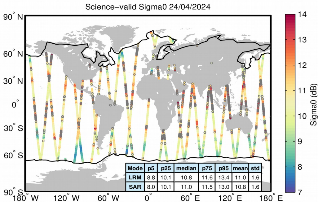
Figure 27. Geographical distribution of science-valid sigma0 data over oceans and lakes for 24/04/2024. The statistical values shown in the table refer to the sigma0 in dB and are calculated separately for LRM and SAR regions. The black lines mark the outer limit of the Arctic and Antarctic polar polygons. Gray circles denote records that have been rejected based on the editing criteria described in Table 4.
