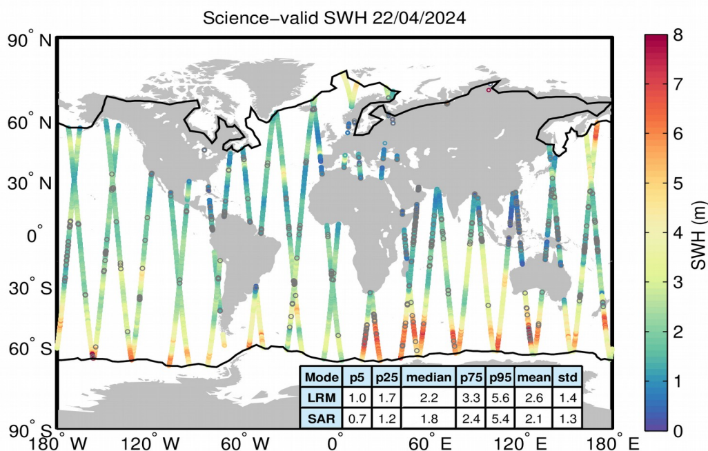
Figure 19. Geographical distribution of science-valid SWH data over oceans and lakes for 22/04/2024. The statistical values shown in the table refer to the SWH in m and are calculated separately for LRM and SAR regions. The black lines mark the outer limit of the Arctic and Antarctic polar polygons. Gray circles denote records that have been rejected based on the editing criteria described in Table 3.
