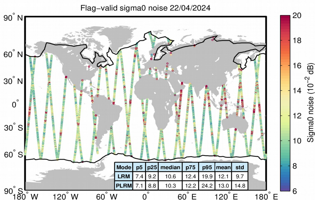
Figure 26. Geographical distribution of flag-valid 20-Hz sigma0 measurement noise over oceans and lakes for LRM/SAR (top) and LRM/PLRM (bottom) and for 22/04/2024. The statistical values shown in the table refer to the sigma0 noise and are calculated separately for LRM and SAR/PLRM regions. Measurements taken over polar polygons have been excluded from the computation of the statistical values. The black lines mark the outer limit of the Arctic and Antarctic polar polygons.
