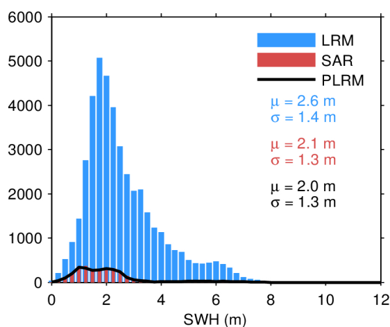
Figure 20. Histogram of science-valid SWH over oceans and lakes for LRM (blue), SAR (red), and PLRM (black) for 22/04/2024. The mean ( \mu ) and standard deviation ( \sigma ) are also
