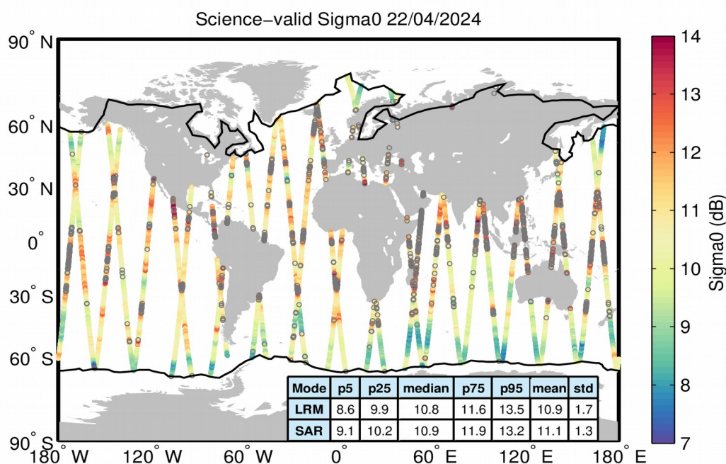
Figure 27. Geographical distribution of science-valid sigma0 data over oceans and lakes for 22/04/2024. The statistical values shown in the table refer to the sigma0 in dB and are calculated separately for LRM and SAR regions. The black lines mark the outer limit of the Arctic and Antarctic polar polygons. Gray circles denote records that have been rejected based on the editing criteria described in Table 4.
