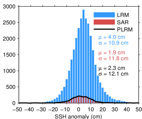
Figure 11. Histogram of science-valid SSH anomaly over oceans and lakes for LRM (blue), SAR (red), and PLRM (black) for 22/04/2024. The mean ( \mu ) and standard deviation ( \sigma ) are also shown. Note that values outside [-50, 50] cm are excluded from the histogram for the sake of readability but not from the computation of \mu and \sigma .
