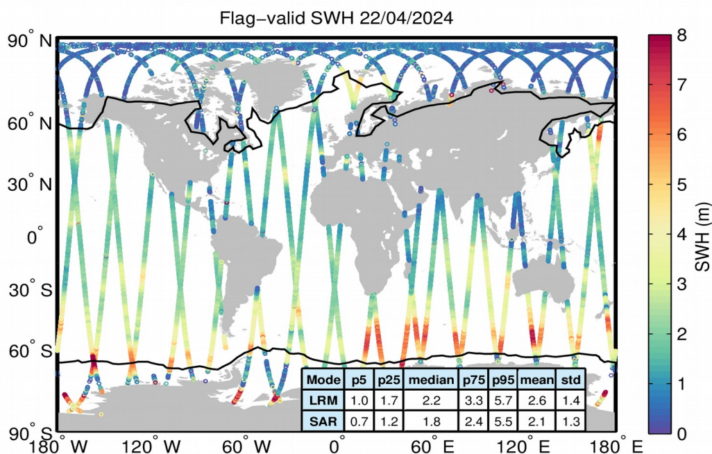
Figure 15. Geographical distribution of flag-valid SWH data over oceans and lakes for 22/04/2024. The statistical values shown in the table refer to the SWH in m and are calculated separately for LRM and SAR regions. Measurements taken over polar polygons have been excluded from the computation of the statistical values. The black lines mark the outer limit of the Arctic and Antarctic polar polygons.
