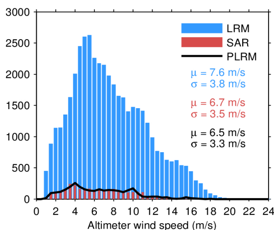
Figure 33. Histogram of flag-valid wind over oceans and lakes for LRM (blue), SAR (red), and PLRM (black) for 22/04/2024. The mean ( \mu ) and standard deviation ( \sigma ) are also shown. Note that values larger than 24 m/s are excluded from the histogram for the sake of readability but not from the computation of \mu and \sigma .
