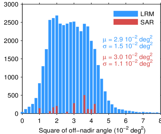
Figure 39. Histogram of flag-valid mispointing over oceans and lakes for LRM (blue) and SAR (red) for 22/04/2024. Only positive values have been considered. The mean ( \mu ) and standard deviation ( \sigma ) are also shown. Note that values larger than 8 \cdot 10^{-2} \text{ deg}^2 are excluded from the histogram for the sake of readability but not from the computation of \mu and \sigma .
