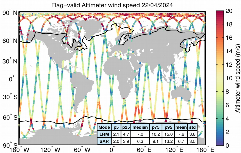
Figure 31. Geographical distribution of flag-valid wind data over oceans and lakes for 22/04/2024. The statistical values shown in the table refer to the wind in m/s and are calculated separately for LRM and SAR regions. Measurements taken over polar polygons have been excluded from the computation of the statistical values. The black lines mark the outer limit of the Arctic and Antarctic polar polygons.
