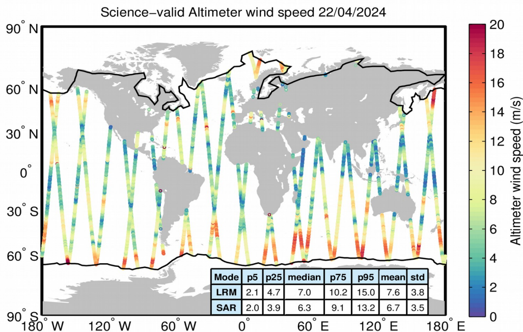
Figure 34. Geographical distribution of science-valid wind data over oceans and lakes for 22/04/2024. The statistical values shown in the table refer to the wind in m/s and are calculated separately for LRM and SAR regions. The black lines mark the outer limit of the Arctic and Antarctic polar polygons. Gray circles denote records that have been rejected based on the editing criteria described in Table 5.
