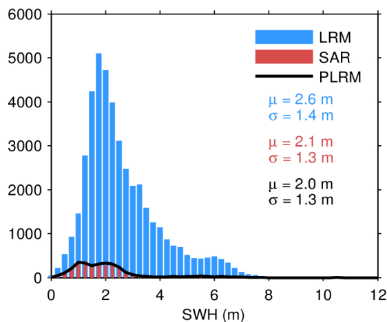
Figure 17. Histogram of flag-valid SWH over oceans and lakes for LRM (blue), SAR (red), and PLRM (black) for 22/04/2024. The mean ( \mu ) and standard deviation ( \sigma ) are also shown. Note that values larger than 12 m are excluded from the histogram for the sake of readability but not from the computation of \mu and \sigma .
