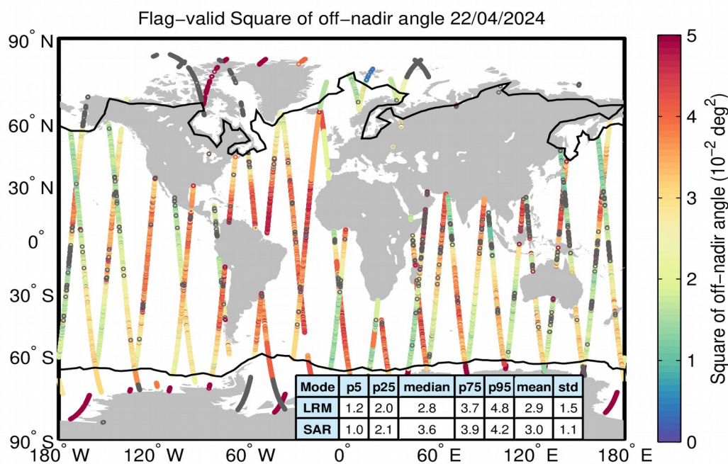
Figure 37. Geographical distribution of flag-valid mispointing data over oceans and lakes for 22/04/2024. The statistical values shown in the table refer to the mispointing in 10^{-2} \text{ deg}^2 and are calculated separately for LRM and SAR regions. Measurements taken over polar polygons have been excluded from the computation of the statistical values. The black lines mark the outer limit of the Arctic and Antarctic polar polygons. Gray circles denote negative values.
