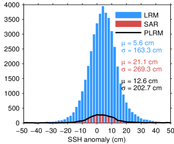
Figure 7. Histogram of flag-valid SSH anomaly over oceans and lakes for LRM (blue), SAR (red), and PLRM (black) for 22/04/2024. The mean ( \mu ) and standard deviation ( \sigma ) are also shown. Note that values outside [-50 50] cm are excluded from the histogram for the sake of readability but not from the computation of \mu and \sigma .
