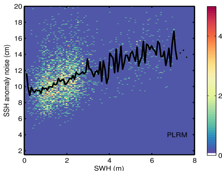
Figure 9. 2D histogram showing flag-valid SSH anomaly noise as a function of SWH for LRM (top), SAR (middle), and PLRM (bottom) for 22/04/2024. The black line denotes the median SSH anomaly noise as a function of SWH.
