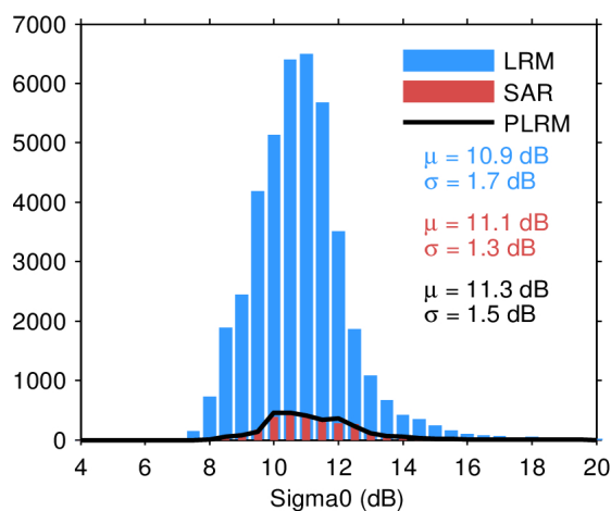
Figure 28. Histogram of science-valid sigma0 over oceans and lakes for LRM (blue), SAR (red), and PLRM (black) for 22/04/2024. The mean ( \mu ) and standard deviation ( \sigma ) are also shown. Note that values outside [4 20] dB are excluded from the histogram for the sake of readability but not from the computation of \mu and \sigma .
