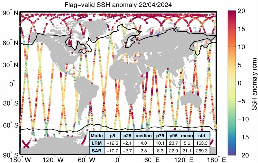
Figure 5. Geographical distribution of flag-valid 1-Hz SSH anomaly data over oceans and lakes for 22/04/2024. The statistical values shown in the table refer to the SSH anomaly in cm and are calculated separately for LRM and SAR regions. Measurements taken over polar polygons have been excluded from the computation of the statistical values. The black lines mark the outer limit of the Arctic and Antarctic polar polygons.
