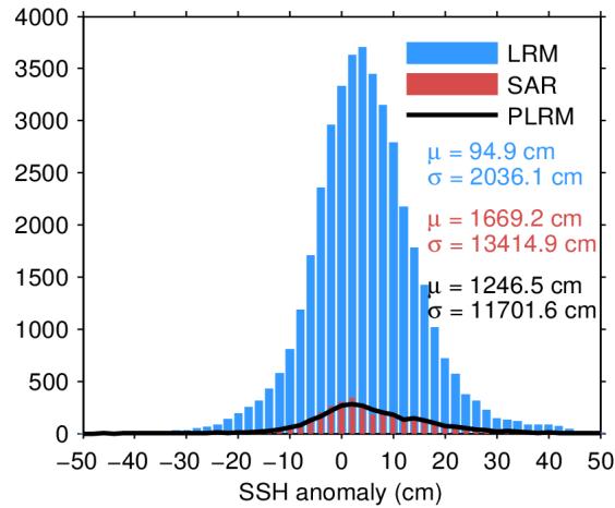
Figure 7. Histogram of flag-valid SSH anomaly over oceans and lakes for LRM (blue), SAR (red), and PLRM (black) for 21/04/2024. The mean ( \mu ) and standard deviation ( \sigma ) are also shown. Note that values outside [-50\ 50] cm are excluded from the histogram for the sake of readability but not from the computation of \mu and \sigma .
