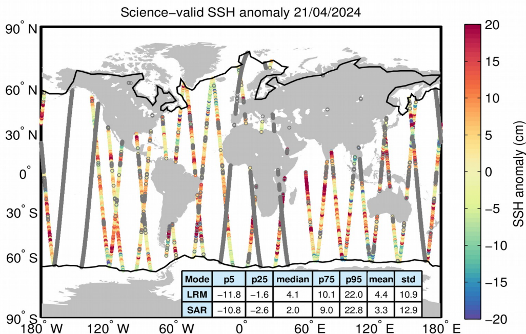
Figure 10. Geographical distribution of science-valid SSH anomaly data over oceans and lakes for 21/04/2024. The statistical values shown in the table refer to the SSH anomaly in cm and are calculated separately for LRM and SAR regions. The black lines mark the
