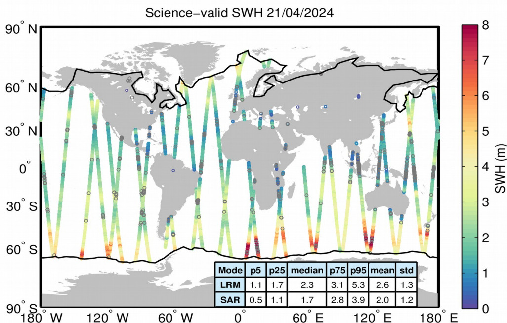
Figure 19. Geographical distribution of science-valid SWH data over oceans and lakes for 21/04/2024. The statistical values shown in the table refer to the SWH in m and are calculated separately for LRM and SAR regions. The black lines mark the outer limit of the Arctic and Antarctic polar polygons. Gray circles denote records that have been rejected based on the editing criteria described in Table 3.
