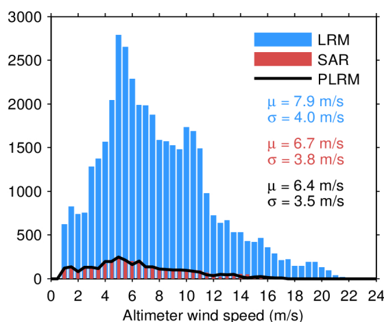
Figure 33. Histogram of flag-valid wind over oceans and lakes for LRM (blue), SAR (red), and PLRM (black) for 21/04/2024. The mean ( \mu ) and standard deviation ( \sigma ) are also shown. Note that values larger than 24 m/s are excluded from the histogram for the sake of readability but not from the computation of \mu and \sigma .
