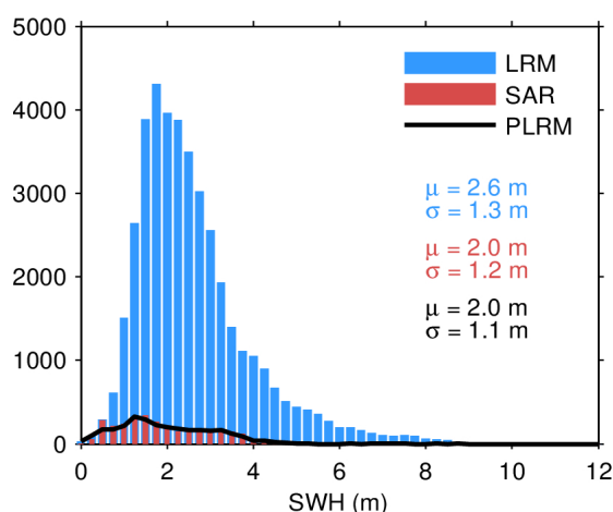
Figure 20. Histogram of science-valid SWH over oceans and lakes for LRM (blue), SAR (red), and PLRM (black) for 21/04/2024. The mean ( \mu ) and standard deviation ( \sigma ) are also
