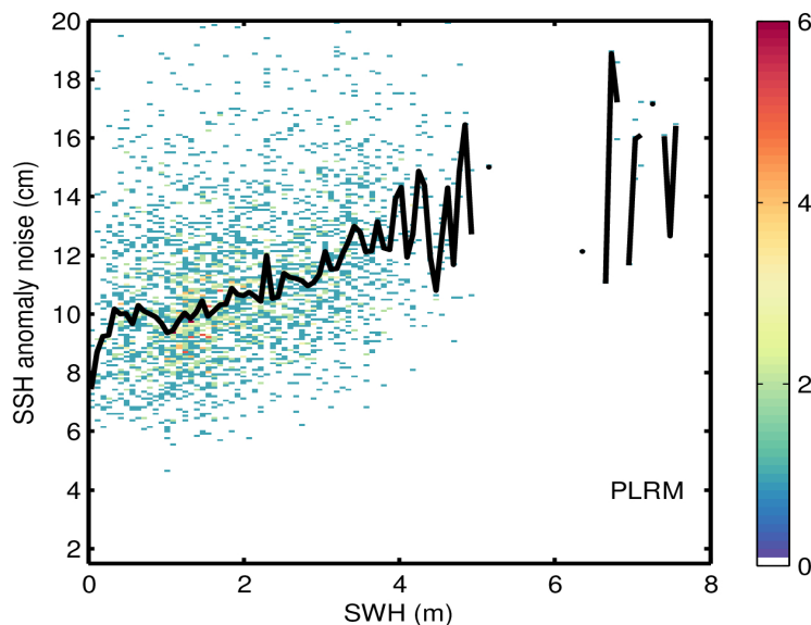
Figure 9. 2D histogram showing flag-valid SSH anomaly noise as a function of SWH for LRM (top), SAR (middle), and PLRM (bottom) for 21/04/2024. The black line denotes the median SSH anomaly noise as a function of SWH.
