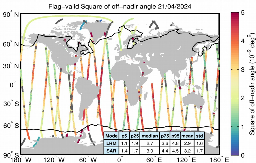
Figure 37. Geographical distribution of flag-valid mispointing data over oceans and lakes for 21/04/2024. The statistical values shown in the table refer to the mispointing in 10^{-2} \text{ deg}^2 and are calculated separately for LRM and SAR regions. Measurements taken over polar polygons have been excluded from the computation of the statistical values. The black lines mark the outer limit of the Arctic and Antarctic polar polygons. Gray circles denote negative values.
