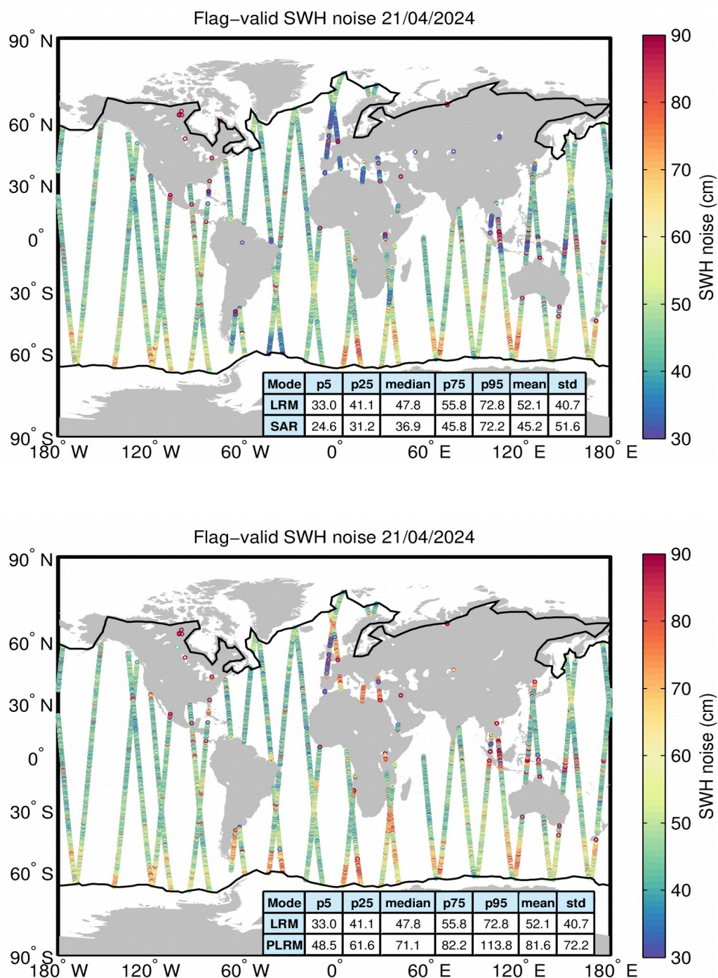
Figure 18. Geographical distribution of flag-valid 20-Hz SWH measurement noise over oceans and lakes for LRM/SAR (top) and LRM/PLRM (bottom) and for 21/04/2024. The statistical values shown in the table refer to the SWH noise and are calculated separately for LRM and SAR/PLRM regions. Measurements taken over polar polygons have been
