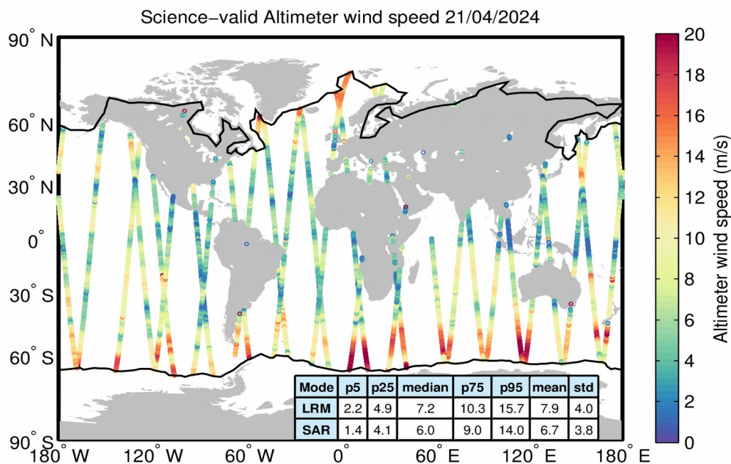
Figure 34. Geographical distribution of science-valid wind data over oceans and lakes for 21/04/2024. The statistical values shown in the table refer to the wind in m/s and are calculated separately for LRM and SAR regions. The black lines mark the outer limit of the Arctic and Antarctic polar polygons. Gray circles denote records that have been rejected based on the editing criteria described in Table 5.
