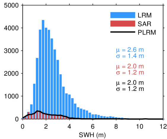
Figure 17. Histogram of flag-valid SWH over oceans and lakes for LRM (blue), SAR (red), and PLRM (black) for 21/04/2024. The mean ( \mu ) and standard deviation ( \sigma ) are also shown. Note that values larger than 12 m are excluded from the histogram for the sake of readability but not from the computation of \mu and \sigma .
