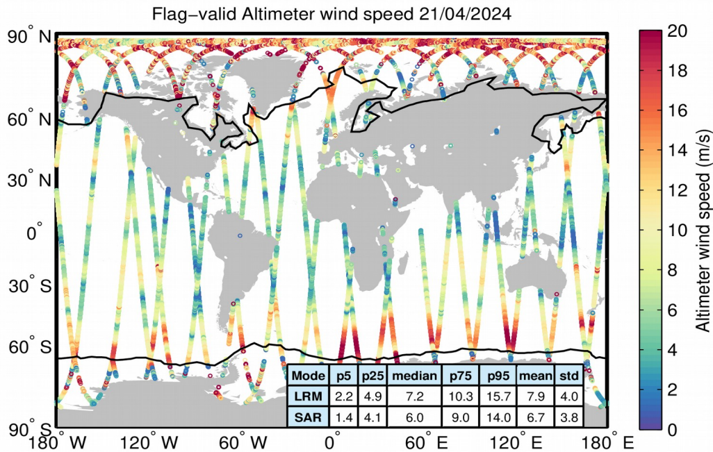
Figure 31. Geographical distribution of flag-valid wind data over oceans and lakes for 21/04/2024. The statistical values shown in the table refer to the wind in m/s and are calculated separately for LRM and SAR regions. Measurements taken over polar polygons have been excluded from the computation of the statistical values. The black lines mark the outer limit of the Arctic and Antarctic polar polygons.
