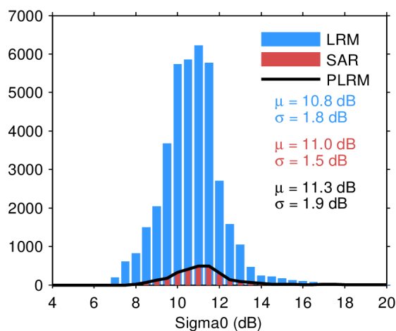
Figure 28. Histogram of science-valid sigma0 over oceans and lakes for LRM (blue), SAR (red), and PLRM (black) for 21/04/2024. The mean ( \mu ) and standard deviation ( \sigma ) are also shown. Note that values outside [4 20] dB are excluded from the histogram for the sake of readability but not from the computation of \mu and \sigma .
