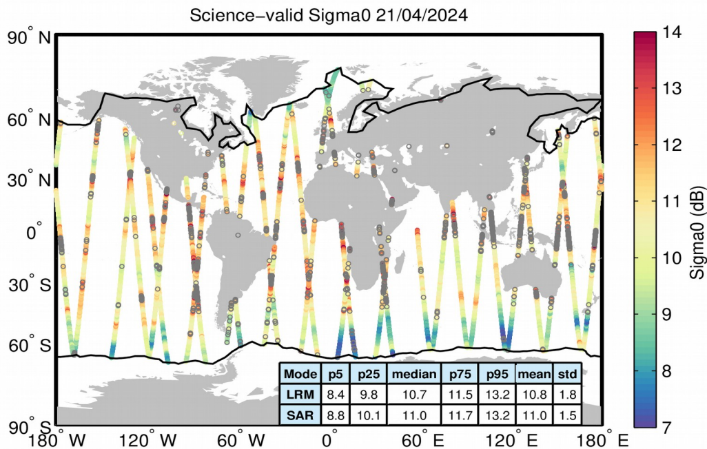
Figure 27. Geographical distribution of science-valid sigma0 data over oceans and lakes for 21/04/2024. The statistical values shown in the table refer to the sigma0 in dB and are calculated separately for LRM and SAR regions. The black lines mark the outer limit of the Arctic and Antarctic polar polygons. Gray circles denote records that have been rejected based on the editing criteria described in Table 4.
