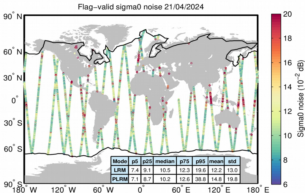
Figure 26. Geographical distribution of flag-valid 20-Hz sigma0 measurement noise over oceans and lakes for LRM/SAR (top) and LRM/PLRM (bottom) and for 21/04/2024. The statistical values shown in the table refer to the sigma0 noise and are calculated separately for LRM and SAR/PLRM regions. Measurements taken over polar polygons have been excluded from the computation of the statistical values. The black lines mark the outer limit of the Arctic and Antarctic polar polygons.
