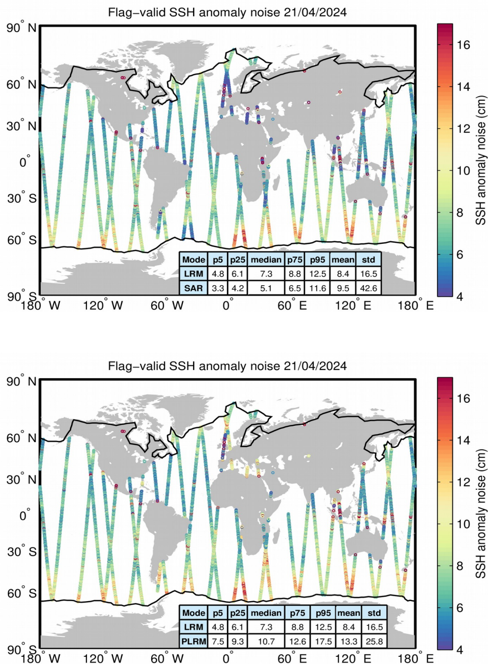
Figure 8. Geographical distribution of flag-valid 20-Hz SSH anomaly measurement noise over oceans and lakes for LRM/SAR (top) and LRM/PLRM (bottom) and for 21/04/2024. The statistical values shown in the tables refer to the SSH anomaly noise and are calculated separately for LRM and SAR/PLRM regions. Measurements taken over polar polygons have been excluded from the computation of the statistical values. The black lines mark the outer limit of the Arctic and Antarctic polar polygons.
