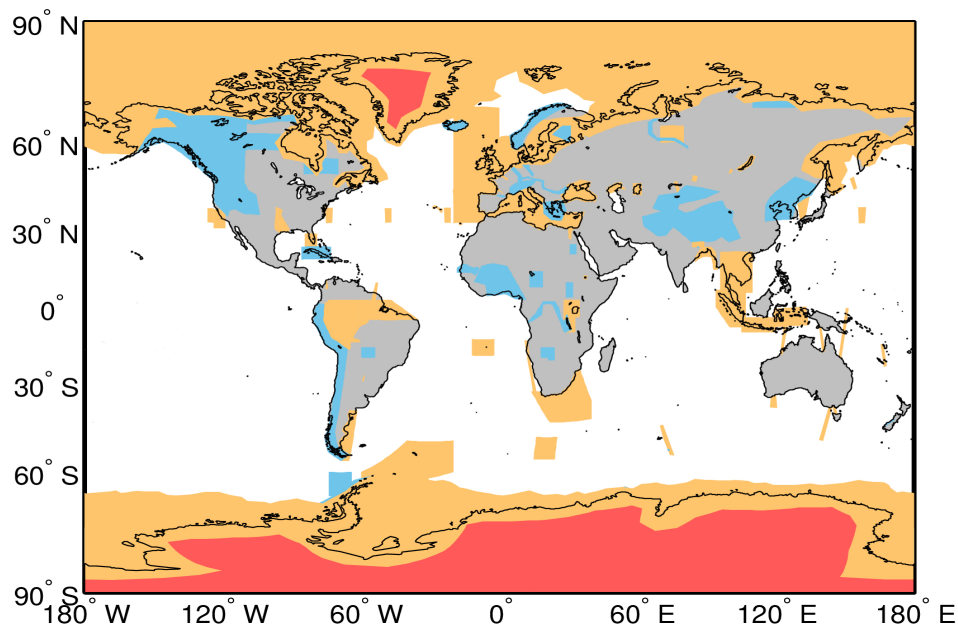
Figure A1. Extent of the regions defining the geographical mode mask for 21/04/2024. The regions where SAR, and SARIn are operated are denoted by the orange and blue polygons, respectively. LRM is operated over areas of the continental ice sheets (red polygons) and over oceans and land not covered by other modes.
