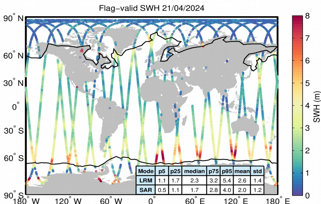
Figure 15. Geographical distribution of flag-valid SWH data over oceans and lakes for 21/04/2024. The statistical values shown in the table refer to the SWH in m and are calculated separately for LRM and SAR regions. Measurements taken over polar polygons have been excluded from the computation of the statistical values. The black lines mark the outer limit of the Arctic and Antarctic polar polygons.
