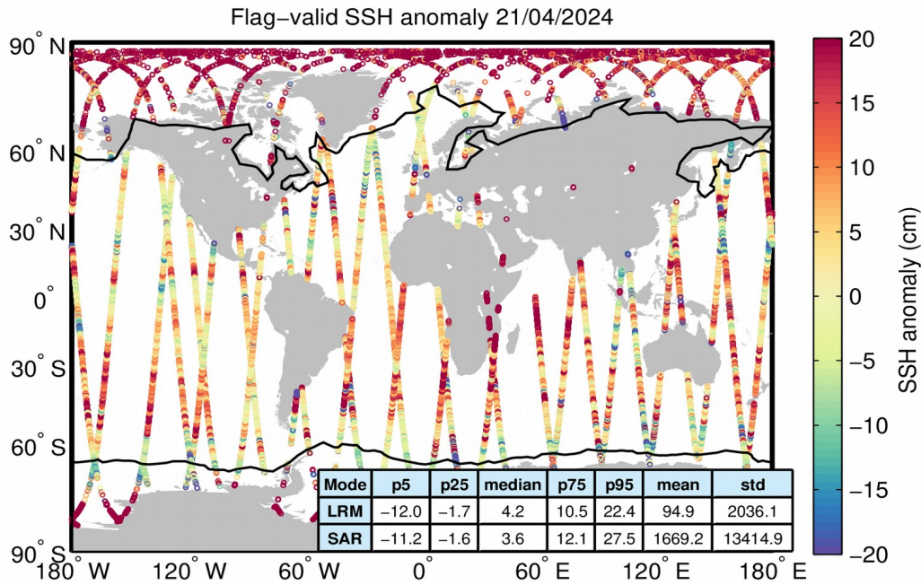
Figure 5. Geographical distribution of flag-valid 1-Hz SSH anomaly data over oceans and lakes for 21/04/2024. The statistical values shown in the table refer to the SSH anomaly in cm and are calculated separately for LRM and SAR regions. Measurements taken over polar polygons have been excluded from the computation of the statistical values. The black lines mark the outer limit of the Arctic and Antarctic polar polygons.
