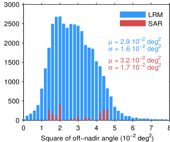
Figure 39. Histogram of flag-valid mispointing over oceans and lakes for LRM (blue) and SAR (red) for 21/04/2024. Only positive values have been considered. The mean ( \mu ) and standard deviation ( \sigma ) are also shown. Note that values larger than 8 \cdot 10^{-2} \text{ deg}^2 are excluded from the histogram for the sake of readability but not from the computation of \mu and \sigma .
