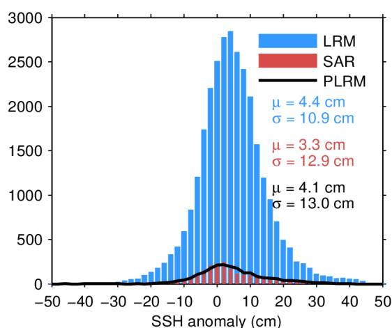
Figure 11. Histogram of science-valid SSH anomaly over oceans and lakes for LRM (blue), SAR (red), and PLRM (black) for 21/04/2024. The mean ( \mu ) and standard deviation ( \sigma ) are also shown. Note that values outside [-50\ 50] cm are excluded from the histogram for the sake of readability but not from the computation of \mu and \sigma .
