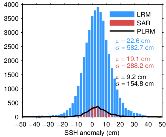
Figure 7. Histogram of flag-valid SSH anomaly over oceans and lakes for LRM (blue), SAR (red), and PLRM (black) for 20/04/2024. The mean ( \mu ) and standard deviation ( \sigma ) are also shown. Note that values outside [-50 50] cm are excluded from the histogram for the sake of readability but not from the computation of \mu and \sigma .
