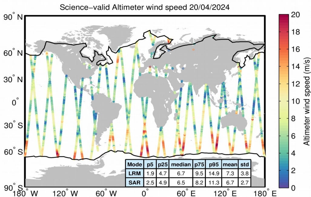
Figure 34. Geographical distribution of science-valid wind data over oceans and lakes for 20/04/2024. The statistical values shown in the table refer to the wind in m/s and are calculated separately for LRM and SAR regions. The black lines mark the outer limit of the Arctic and Antarctic polar polygons. Gray circles denote records that have been rejected based on the editing criteria described in Table 5.
