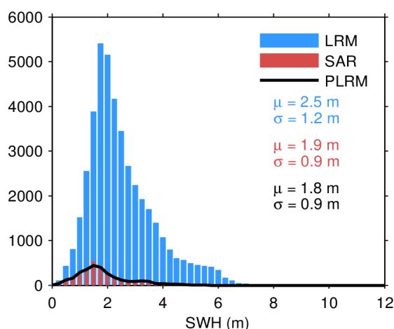
Figure 20. Histogram of science-valid SWH over oceans and lakes for LRM (blue), SAR (red), and PLRM (black) for 20/04/2024. The mean ( \mu ) and standard deviation ( \sigma ) are also
