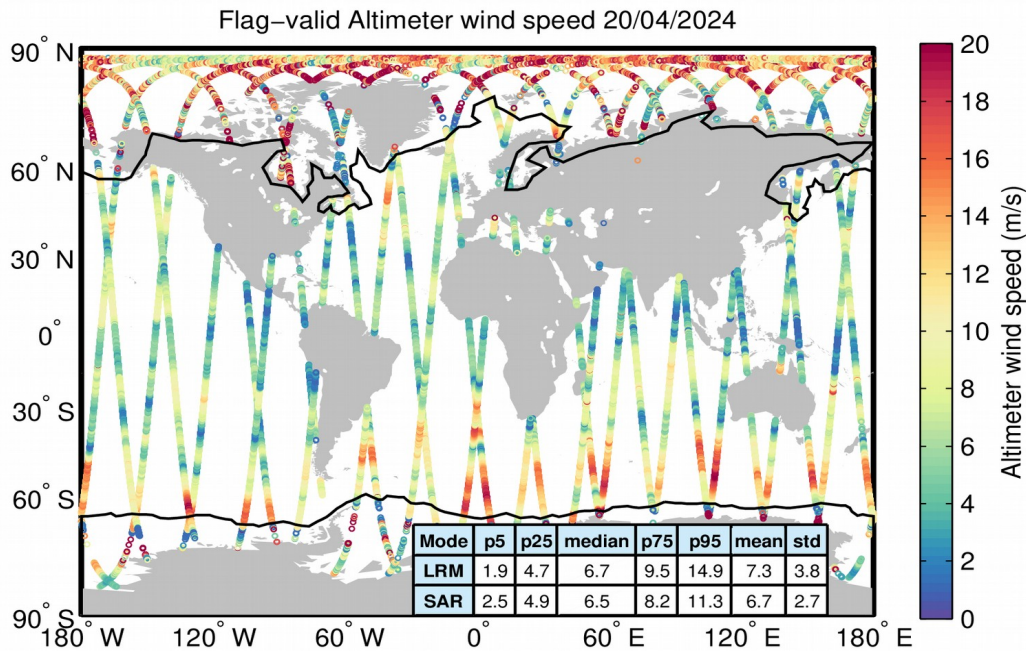
Figure 31. Geographical distribution of flag-valid wind data over oceans and lakes for 20/04/2024. The statistical values shown in the table refer to the wind in m/s and are calculated separately for LRM and SAR regions. Measurements taken over polar polygons have been excluded from the computation of the statistical values. The black lines mark the outer limit of the Arctic and Antarctic polar polygons.
