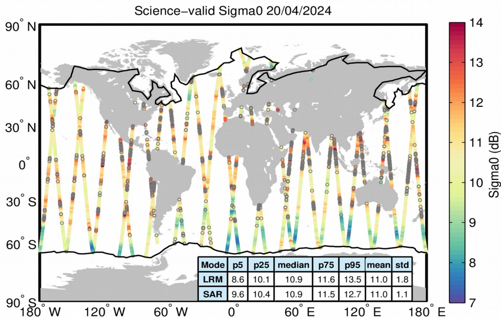
Figure 27. Geographical distribution of science-valid sigma0 data over oceans and lakes for 20/04/2024. The statistical values shown in the table refer to the sigma0 in dB and are calculated separately for LRM and SAR regions. The black lines mark the outer limit of the Arctic and Antarctic polar polygons. Gray circles denote records that have been rejected based on the editing criteria described in Table 4.
