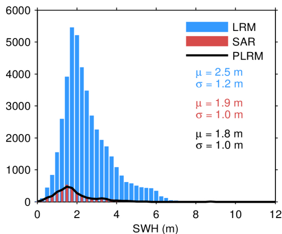
Figure 17. Histogram of flag-valid SWH over oceans and lakes for LRM (blue), SAR (red), and PLRM (black) for 20/04/2024. The mean ( \mu ) and standard deviation ( \sigma ) are also shown. Note that values larger than 12 m are excluded from the histogram for the sake of readability but not from the computation of \mu and \sigma .
