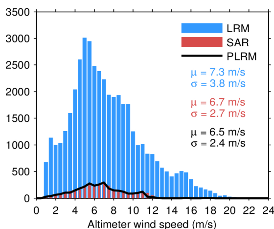
Figure 33. Histogram of flag-valid wind over oceans and lakes for LRM (blue), SAR (red), and PLRM (black) for 20/04/2024. The mean ( \mu ) and standard deviation ( \sigma ) are also shown. Note that values larger than 24 m/s are excluded from the histogram for the sake of readability but not from the computation of \mu and \sigma .
