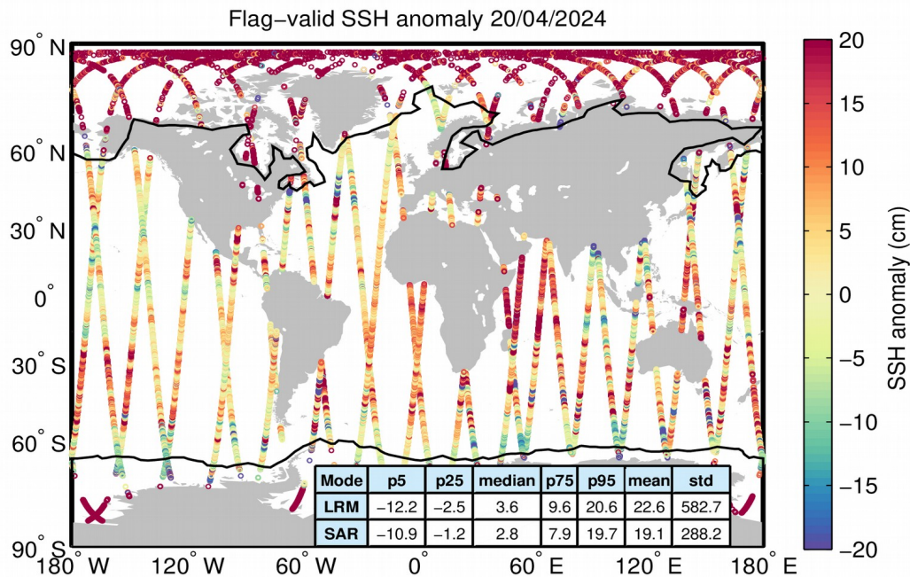
Figure 5. Geographical distribution of flag-valid 1-Hz SSH anomaly data over oceans and lakes for 20/04/2024. The statistical values shown in the table refer to the SSH anomaly in cm and are calculated separately for LRM and SAR regions. Measurements taken over polar polygons have been excluded from the computation of the statistical values. The black lines mark the outer limit of the Arctic and Antarctic polar polygons.
