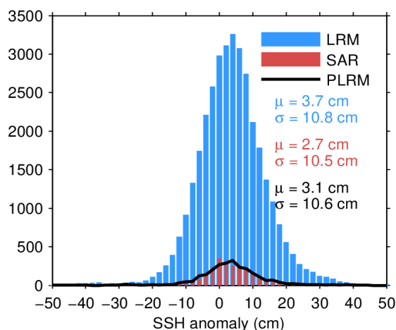
Figure 11. Histogram of science-valid SSH anomaly over oceans and lakes for LRM (blue), SAR (red), and PLRM (black) for 20/04/2024. The mean ( \mu ) and standard deviation ( \sigma ) are also shown. Note that values outside [-50, 50] cm are excluded from the histogram for the sake of readability but not from the computation of \mu and \sigma .
