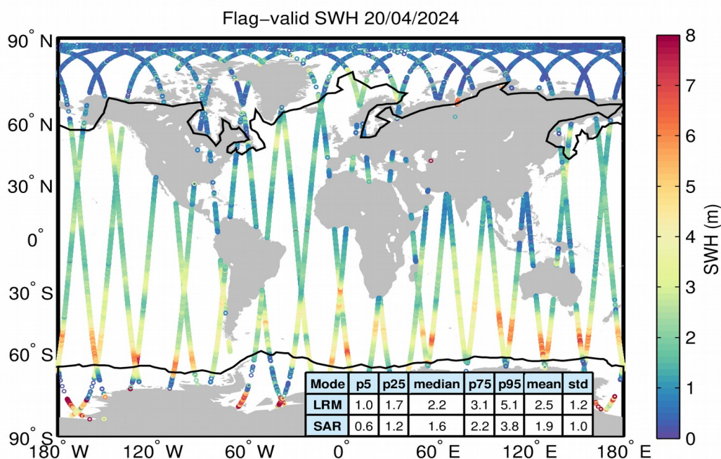
Figure 15. Geographical distribution of flag-valid SWH data over oceans and lakes for 20/04/2024. The statistical values shown in the table refer to the SWH in m and are calculated separately for LRM and SAR regions. Measurements taken over polar polygons have been excluded from the computation of the statistical values. The black lines mark the outer limit of the Arctic and Antarctic polar polygons.
