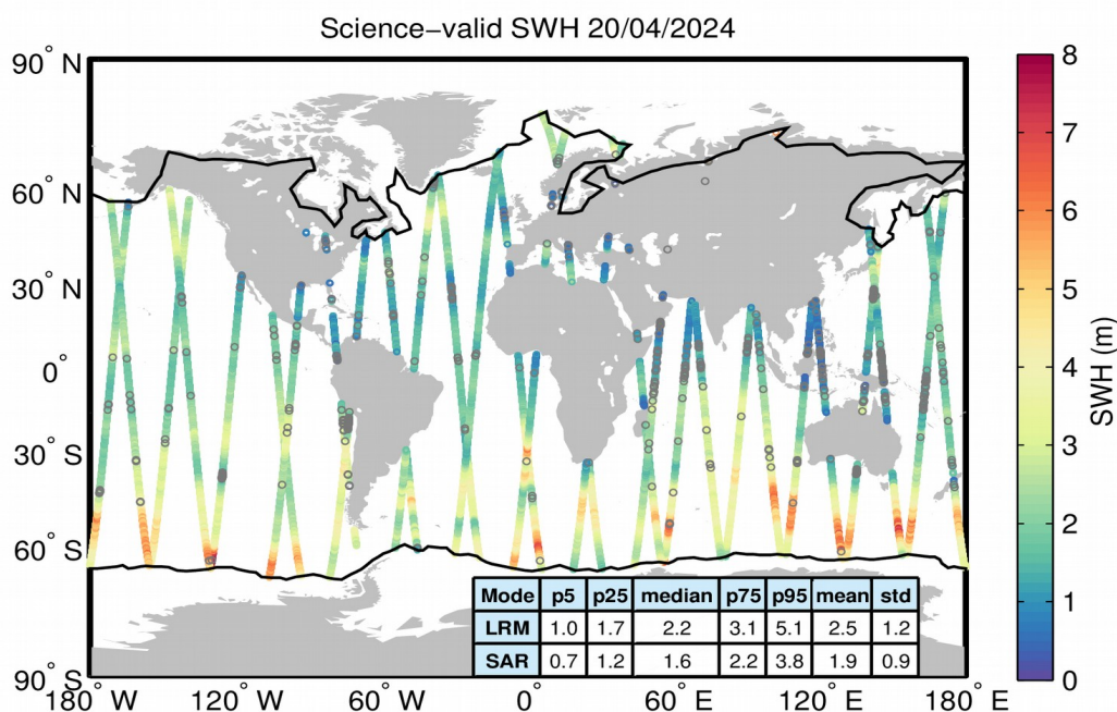
Figure 19. Geographical distribution of science-valid SWH data over oceans and lakes for 20/04/2024. The statistical values shown in the table refer to the SWH in m and are calculated separately for LRM and SAR regions. The black lines mark the outer limit of the Arctic and Antarctic polar polygons. Gray circles denote records that have been rejected based on the editing criteria described in Table 3.
