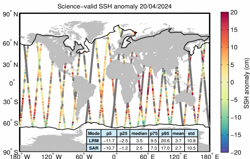
Figure 10. Geographical distribution of science-valid SSH anomaly data over oceans and lakes for 20/04/2024. The statistical values shown in the table refer to the SSH anomaly in cm and are calculated separately for LRM and SAR regions. The black lines mark the
