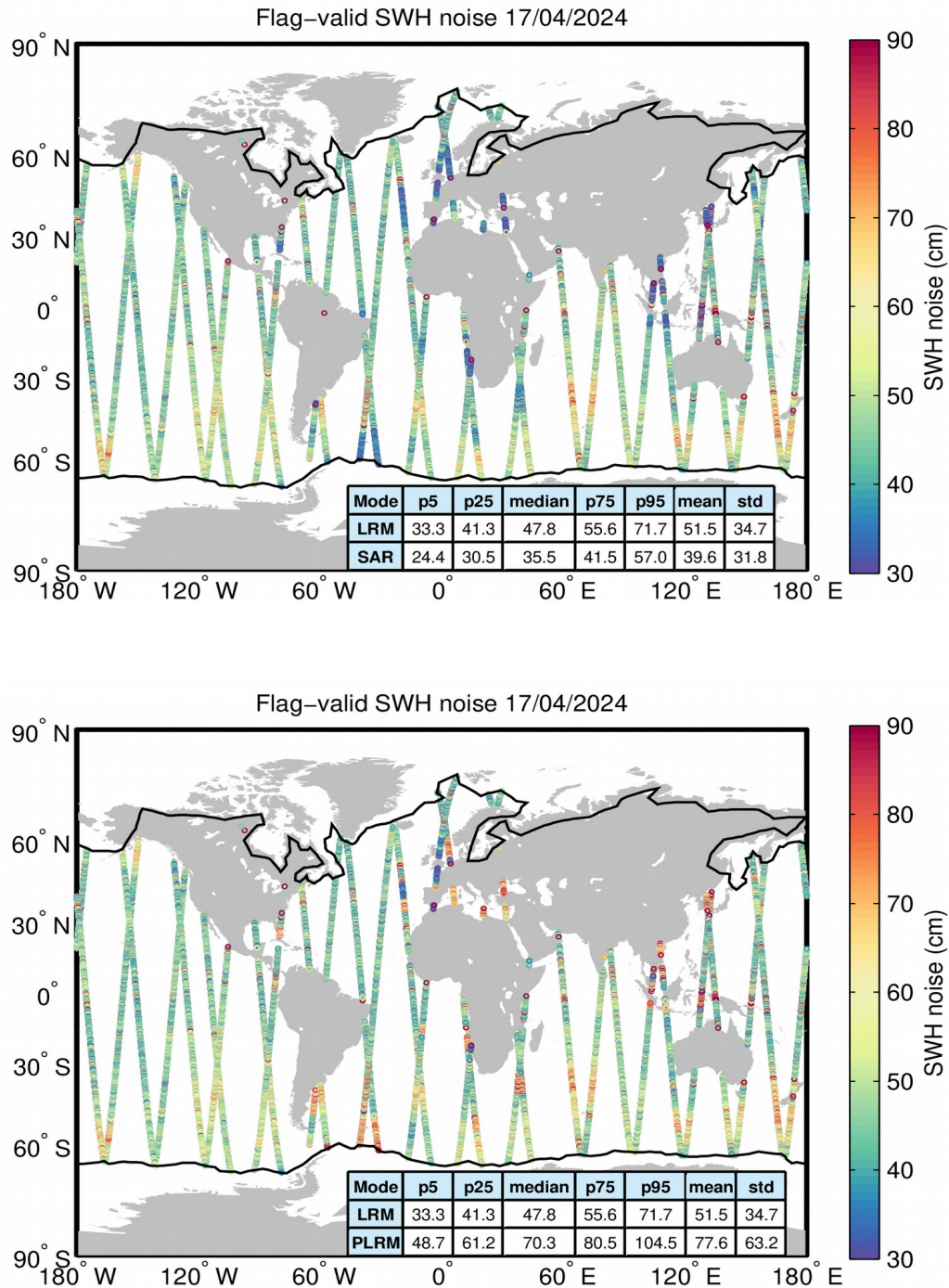
Figure 18. Geographical distribution of flag-valid 20-Hz SWH measurement noise over oceans and lakes for LRM/SAR (top) and LRM/PLRM (bottom) and for 17/04/2024. The statistical values shown in the table refer to the SWH noise and are calculated separately for LRM and SAR/PLRM regions. Measurements taken over polar polygons have been
