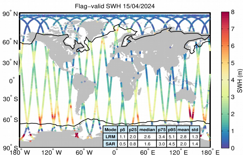
Figure 15. Geographical distribution of flag-valid SWH data over oceans and lakes for 15/04/2024. The statistical values shown in the table refer to the SWH in m and are calculated separately for LRM and SAR regions. Measurements taken over polar polygons have been excluded from the computation of the statistical values. The black lines mark the outer limit of the Arctic and Antarctic polar polygons.
