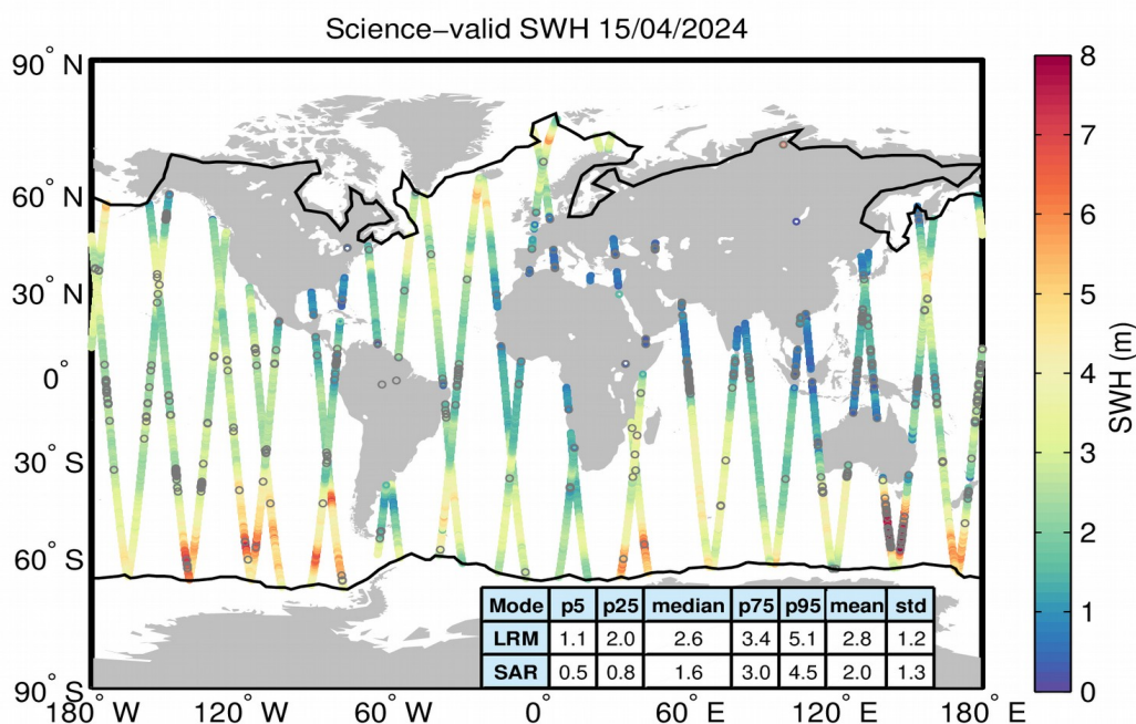
Figure 19. Geographical distribution of science-valid SWH data over oceans and lakes for 15/04/2024. The statistical values shown in the table refer to the SWH in m and are calculated separately for LRM and SAR regions. The black lines mark the outer limit of the Arctic and Antarctic polar polygons. Gray circles denote records that have been rejected based on the editing criteria described in Table 3.
