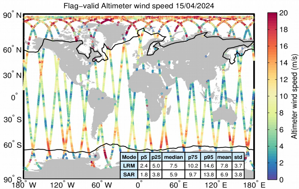
Figure 31. Geographical distribution of flag-valid wind data over oceans and lakes for 15/04/2024. The statistical values shown in the table refer to the wind in m/s and are calculated separately for LRM and SAR regions. Measurements taken over polar polygons have been excluded from the computation of the statistical values. The black lines mark the outer limit of the Arctic and Antarctic polar polygons.
