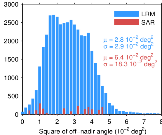
Figure 39. Histogram of flag-valid mispointing over oceans and lakes for LRM (blue) and SAR (red) for 15/04/2024. Only positive values have been considered. The mean ( \mu ) and standard deviation ( \sigma ) are also shown. Note that values larger than 8 \cdot 10^{-2} \text{ deg}^2 are excluded from the histogram for the sake of readability but not from the computation of \mu and \sigma .
