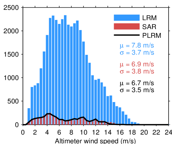
Figure 33. Histogram of flag-valid wind over oceans and lakes for LRM (blue), SAR (red), and PLRM (black) for 15/04/2024. The mean ( \mu ) and standard deviation ( \sigma ) are also shown. Note that values larger than 24 m/s are excluded from the histogram for the sake of readability but not from the computation of \mu and \sigma .
