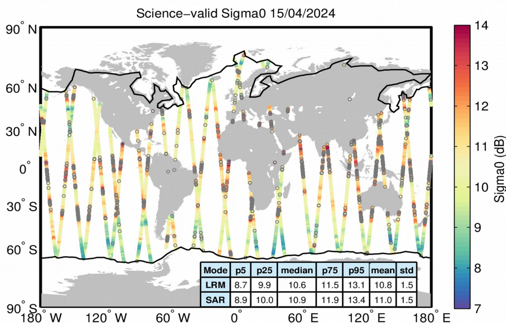
Figure 27. Geographical distribution of science-valid sigma0 data over oceans and lakes for 15/04/2024. The statistical values shown in the table refer to the sigma0 in dB and are calculated separately for LRM and SAR regions. The black lines mark the outer limit of the Arctic and Antarctic polar polygons. Gray circles denote records that have been rejected based on the editing criteria described in Table 4.
