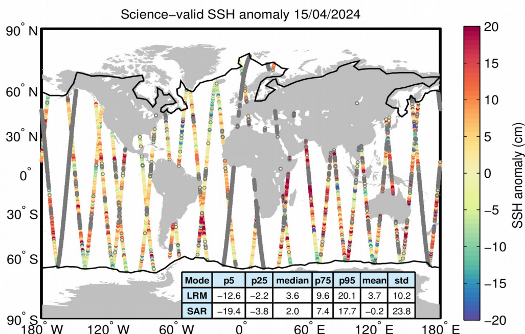
Figure 10. Geographical distribution of science-valid SSH anomaly data over oceans and lakes for 15/04/2024. The statistical values shown in the table refer to the SSH anomaly in cm and are calculated separately for LRM and SAR regions. The black lines mark the
