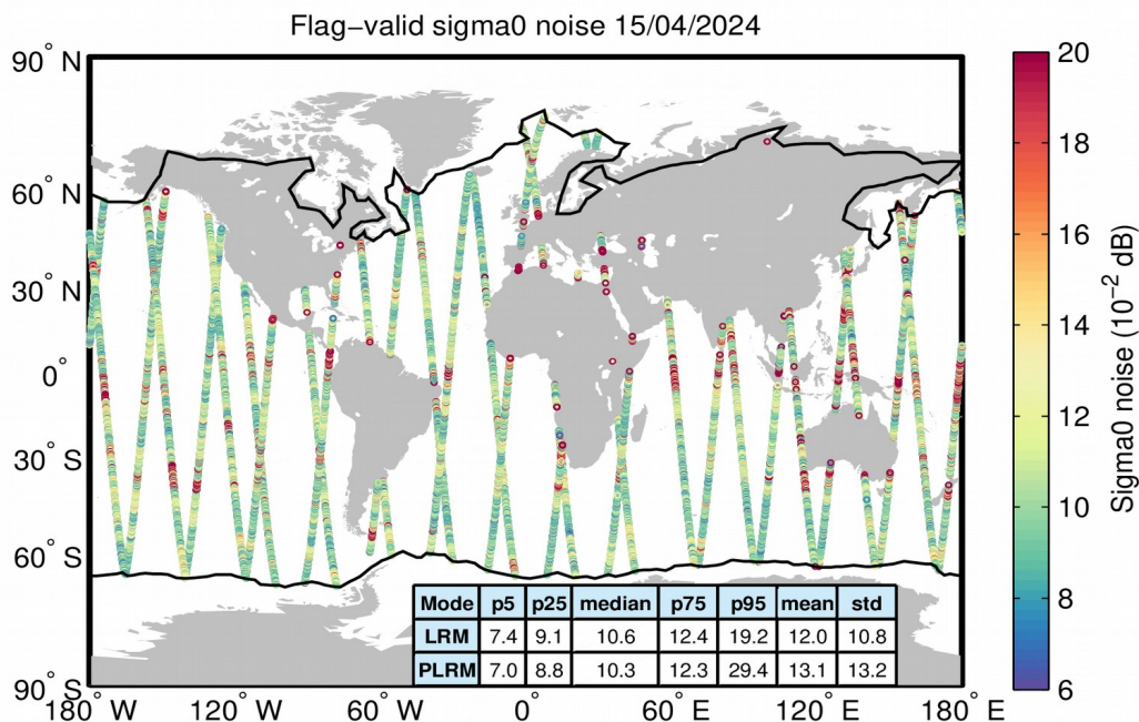
Figure 26. Geographical distribution of flag-valid 20-Hz sigma0 measurement noise over oceans and lakes for LRM/SAR (top) and LRM/PLRM (bottom) and for 15/04/2024. The statistical values shown in the table refer to the sigma0 noise and are calculated separately for LRM and SAR/PLRM regions. Measurements taken over polar polygons have been excluded from the computation of the statistical values. The black lines mark the outer limit of the Arctic and Antarctic polar polygons.
