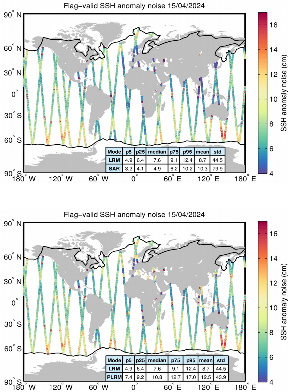
Figure 8. Geographical distribution of flag-valid 20-Hz SSH anomaly measurement noise over oceans and lakes for LRM/SAR (top) and LRM/PLRM (bottom) and for 15/04/2024. The statistical values shown in the tables refer to the SSH anomaly noise and are calculated separately for LRM and SAR/PLRM regions. Measurements taken over polar polygons have been excluded from the computation of the statistical values. The black lines mark the outer limit of the Arctic and Antarctic polar polygons.
