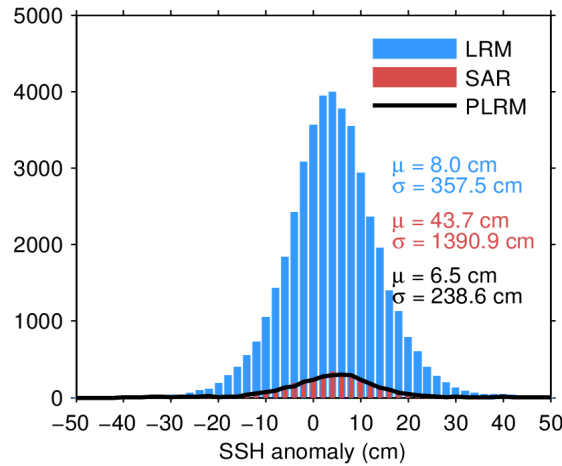
Figure 7. Histogram of flag-valid SSH anomaly over oceans and lakes for LRM (blue), SAR (red), and PLRM (black) for 15/04/2024. The mean ( \mu ) and standard deviation ( \sigma ) are also shown. Note that values outside [-50 50] cm are excluded from the histogram for the sake of readability but not from the computation of \mu and \sigma .
