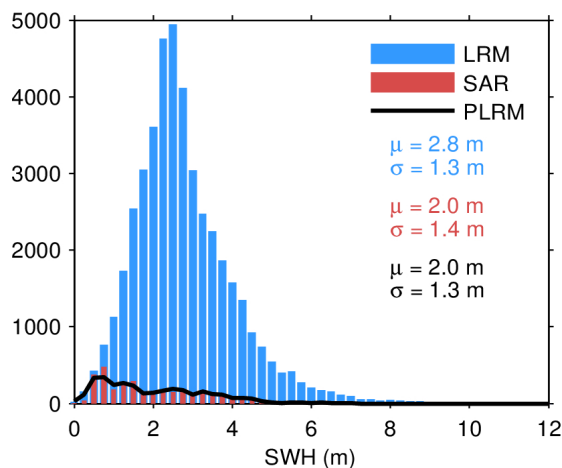
Figure 17. Histogram of flag-valid SWH over oceans and lakes for LRM (blue), SAR (red), and PLRM (black) for 15/04/2024. The mean ( \mu ) and standard deviation ( \sigma ) are also shown. Note that values larger than 12 m are excluded from the histogram for the sake of readability but not from the computation of \mu and \sigma .
