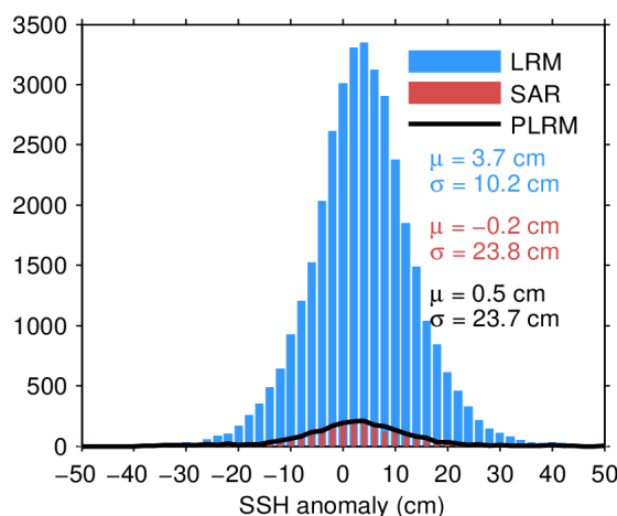
Figure 11. Histogram of science-valid SSH anomaly over oceans and lakes for LRM (blue), SAR (red), and PLRM (black) for 15/04/2024. The mean ( \mu ) and standard deviation ( \sigma ) are also shown. Note that values outside [-50, 50] cm are excluded from the histogram for the sake of readability but not from the computation of \mu and \sigma .
