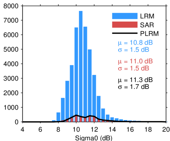
Figure 28. Histogram of science-valid sigma0 over oceans and lakes for LRM (blue), SAR (red), and PLRM (black) for 15/04/2024. The mean ( \mu ) and standard deviation ( \sigma ) are also shown. Note that values outside [4 20] dB are excluded from the histogram for the sake of readability but not from the computation of \mu and \sigma .
