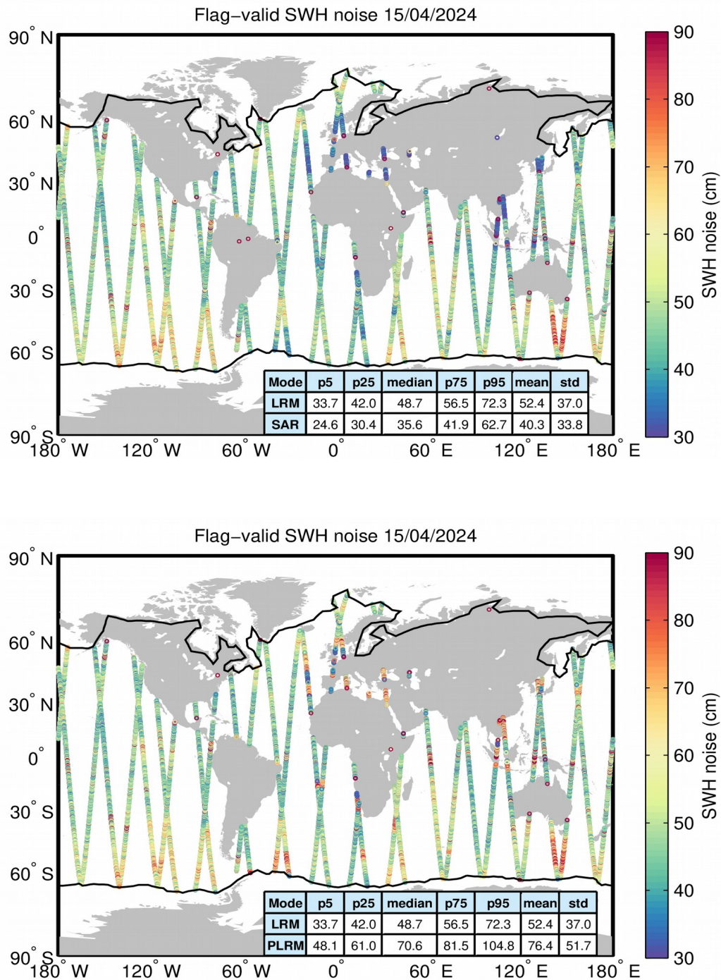
Figure 18. Geographical distribution of flag-valid 20-Hz SWH measurement noise over oceans and lakes for LRM/SAR (top) and LRM/PLRM (bottom) and for 15/04/2024. The statistical values shown in the table refer to the SWH noise and are calculated separately for LRM and SAR/PLRM regions. Measurements taken over polar polygons have been
