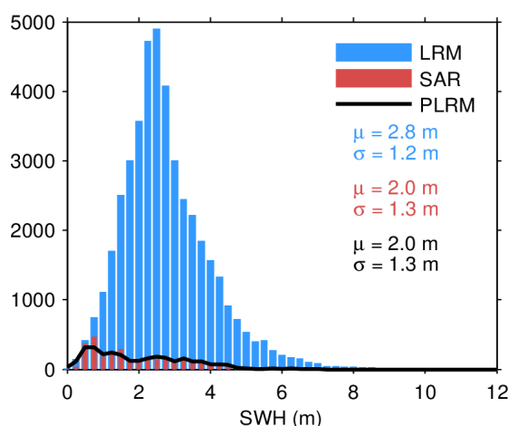
Figure 20. Histogram of science-valid SWH over oceans and lakes for LRM (blue), SAR (red), and PLRM (black) for 15/04/2024. The mean ( \mu ) and standard deviation ( \sigma ) are also
