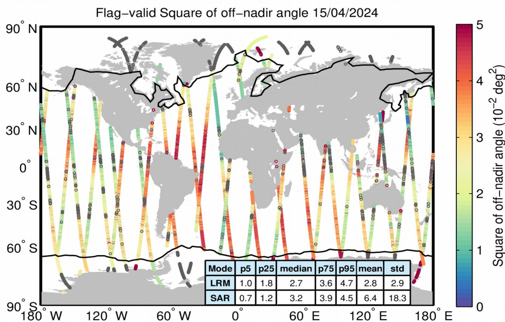
Figure 37. Geographical distribution of flag-valid mispointing data over oceans and lakes for 15/04/2024. The statistical values shown in the table refer to the mispointing in 10^{-2} \text{ deg}^2 and are calculated separately for LRM and SAR regions. Measurements taken over polar polygons have been excluded from the computation of the statistical values. The black lines mark the outer limit of the Arctic and Antarctic polar polygons. Gray circles denote negative values.
