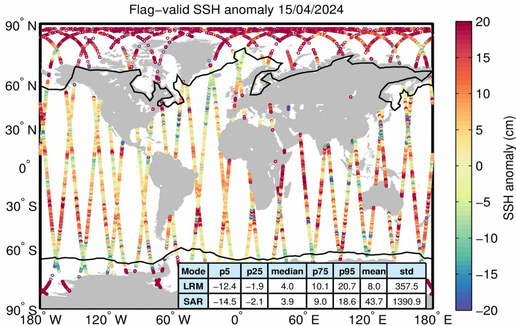
Figure 5. Geographical distribution of flag-valid 1-Hz SSH anomaly data over oceans and lakes for 15/04/2024. The statistical values shown in the table refer to the SSH anomaly in cm and are calculated separately for LRM and SAR regions. Measurements taken over polar polygons have been excluded from the computation of the statistical values. The black lines mark the outer limit of the Arctic and Antarctic polar polygons.
