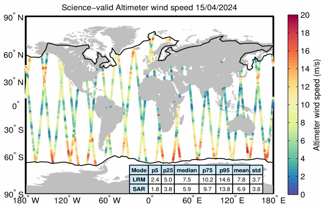
Figure 34. Geographical distribution of science-valid wind data over oceans and lakes for 15/04/2024. The statistical values shown in the table refer to the wind in m/s and are calculated separately for LRM and SAR regions. The black lines mark the outer limit of the Arctic and Antarctic polar polygons. Gray circles denote records that have been rejected based on the editing criteria described in Table 5.
