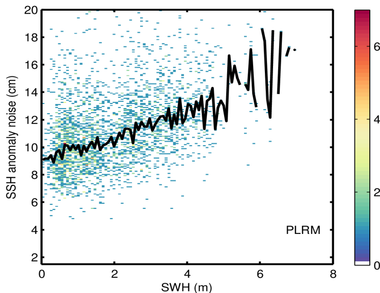
Figure 9. 2D histogram showing flag-valid SSH anomaly noise as a function of SWH for LRM (top), SAR (middle), and PLRM (bottom) for 15/04/2024. The black line denotes the median SSH anomaly noise as a function of SWH.
