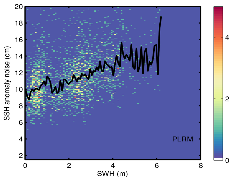
Figure 9. 2D histogram showing flag-valid SSH anomaly noise as a function of SWH for LRM (top), SAR (middle), and PLRM (bottom) for 14/04/2024. The black line denotes the median SSH anomaly noise as a function of SWH.
