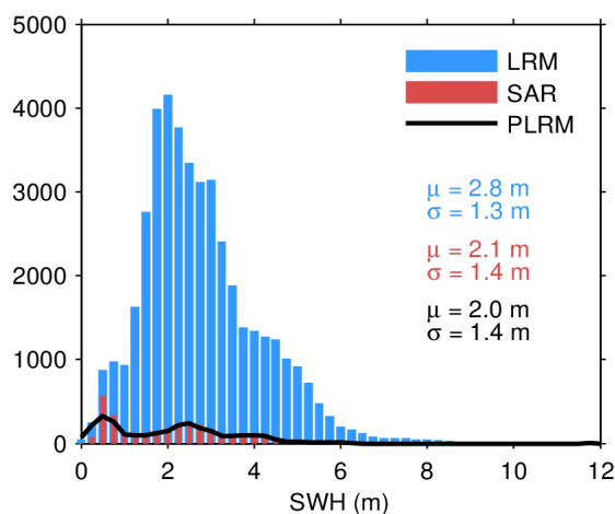
Figure 17. Histogram of flag-valid SWH over oceans and lakes for LRM (blue), SAR (red), and PLRM (black) for 14/04/2024. The mean ( \mu ) and standard deviation ( \sigma ) are also shown. Note that values larger than 12 m are excluded from the histogram for the sake of readability but not from the computation of \mu and \sigma .
