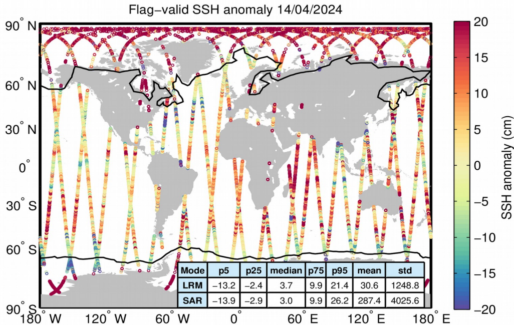
Figure 5. Geographical distribution of flag-valid 1-Hz SSH anomaly data over oceans and lakes for 14/04/2024. The statistical values shown in the table refer to the SSH anomaly in cm and are calculated separately for LRM and SAR regions. Measurements taken over polar polygons have been excluded from the computation of the statistical values. The black lines mark the outer limit of the Arctic and Antarctic polar polygons.
