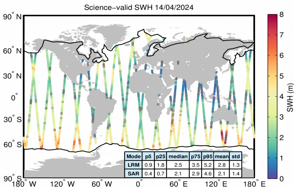
Figure 19. Geographical distribution of science-valid SWH data over oceans and lakes for 14/04/2024. The statistical values shown in the table refer to the SWH in m and are calculated separately for LRM and SAR regions. The black lines mark the outer limit of the Arctic and Antarctic polar polygons. Gray circles denote records that have been rejected based on the editing criteria described in Table 3.
