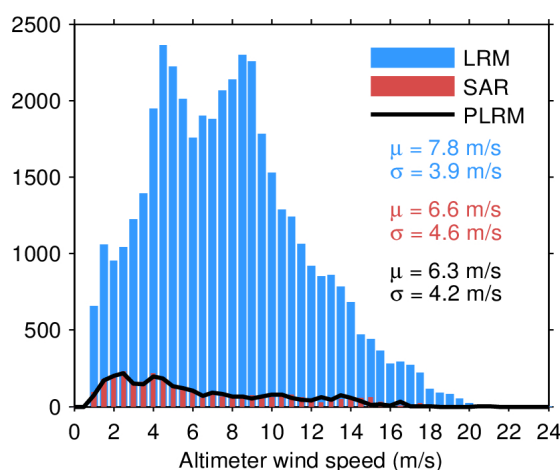
Figure 33. Histogram of flag-valid wind over oceans and lakes for LRM (blue), SAR (red), and PLRM (black) for 14/04/2024. The mean ( \mu ) and standard deviation ( \sigma ) are also shown. Note that values larger than 24 m/s are excluded from the histogram for the sake of readability but not from the computation of \mu and \sigma .
