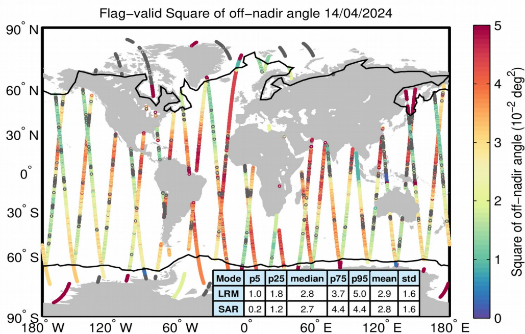
Figure 37. Geographical distribution of flag-valid mispointing data over oceans and lakes for 14/04/2024. The statistical values shown in the table refer to the mispointing in 10^{-2} \text{ deg}^2 and are calculated separately for LRM and SAR regions. Measurements taken over polar polygons have been excluded from the computation of the statistical values. The black lines mark the outer limit of the Arctic and Antarctic polar polygons. Gray circles denote negative values.
