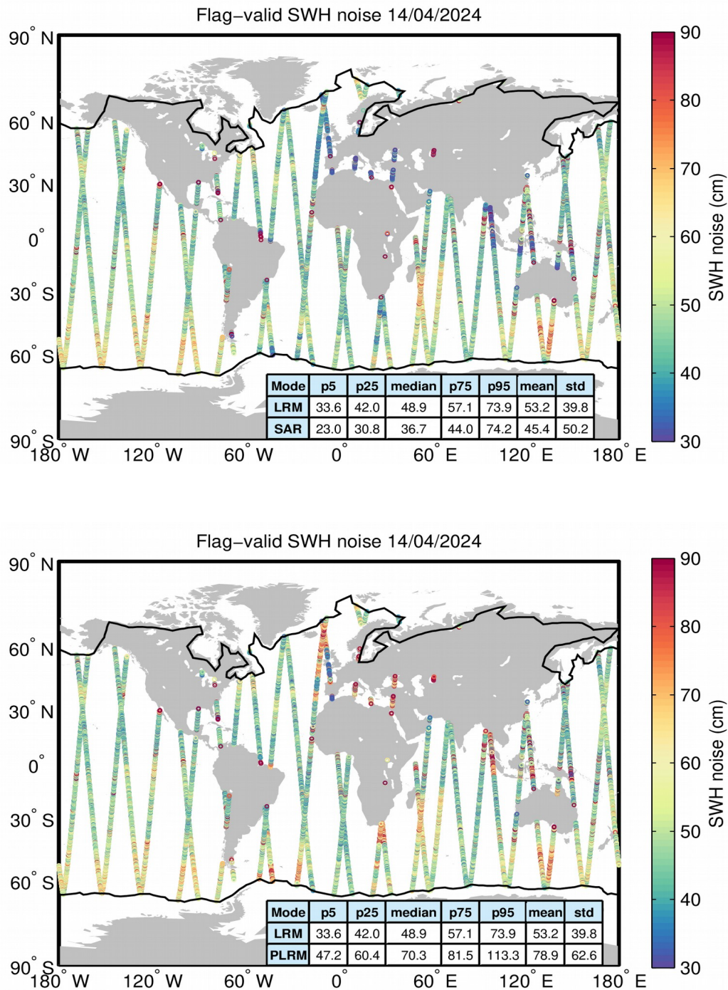
Figure 18. Geographical distribution of flag-valid 20-Hz SWH measurement noise over oceans and lakes for LRM/SAR (top) and LRM/PLRM (bottom) and for 14/04/2024. The statistical values shown in the table refer to the SWH noise and are calculated separately for LRM and SAR/PLRM regions. Measurements taken over polar polygons have been
