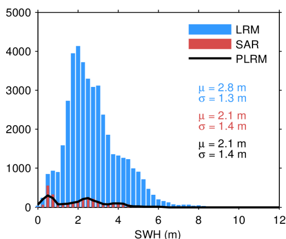
Figure 20. Histogram of science-valid SWH over oceans and lakes for LRM (blue), SAR (red), and PLRM (black) for 14/04/2024. The mean ( \mu ) and standard deviation ( \sigma ) are also
