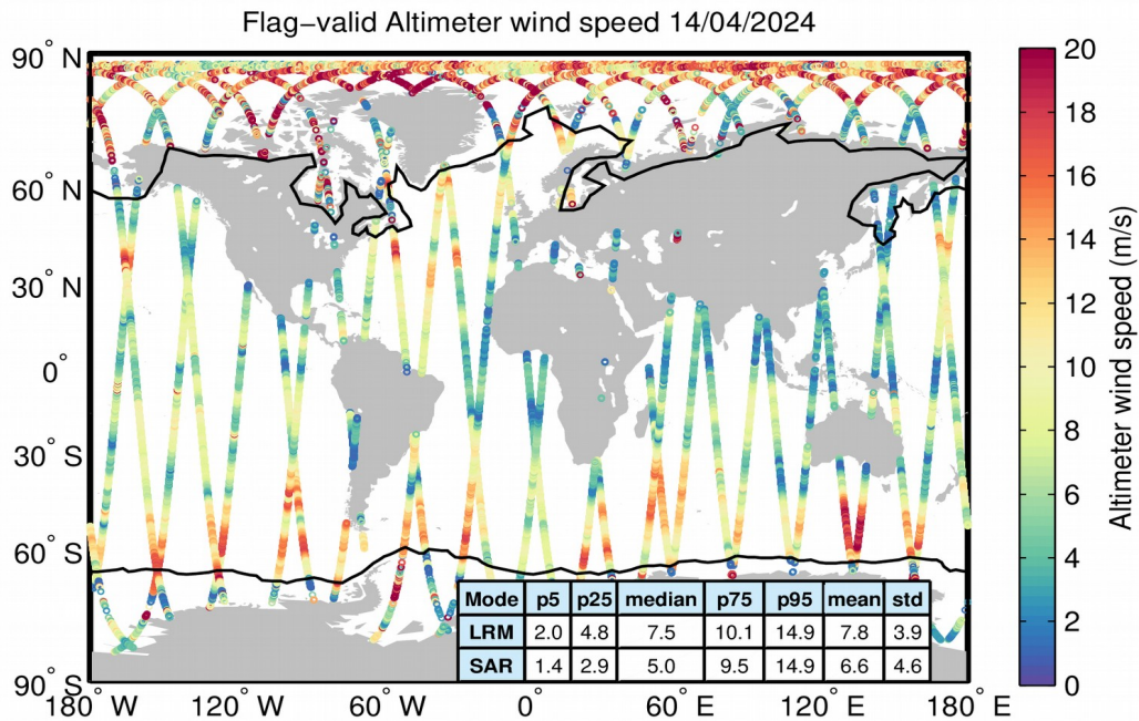
Figure 31. Geographical distribution of flag-valid wind data over oceans and lakes for 14/04/2024. The statistical values shown in the table refer to the wind in m/s and are calculated separately for LRM and SAR regions. Measurements taken over polar polygons have been excluded from the computation of the statistical values. The black lines mark the outer limit of the Arctic and Antarctic polar polygons.
