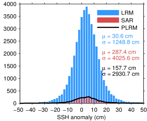
Figure 7. Histogram of flag-valid SSH anomaly over oceans and lakes for LRM (blue), SAR (red), and PLRM (black) for 14/04/2024. The mean ( \mu ) and standard deviation ( \sigma ) are also shown. Note that values outside [-50 50] cm are excluded from the histogram for the sake of readability but not from the computation of \mu and \sigma .
