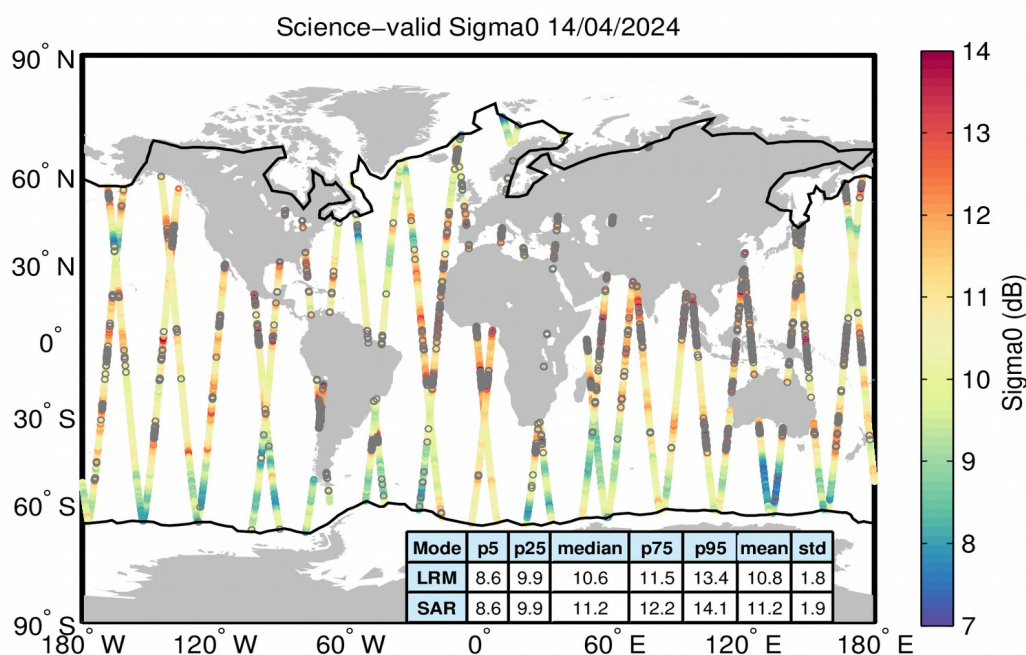
Figure 27. Geographical distribution of science-valid sigma0 data over oceans and lakes for 14/04/2024. The statistical values shown in the table refer to the sigma0 in dB and are calculated separately for LRM and SAR regions. The black lines mark the outer limit of the Arctic and Antarctic polar polygons. Gray circles denote records that have been rejected based on the editing criteria described in Table 4.
