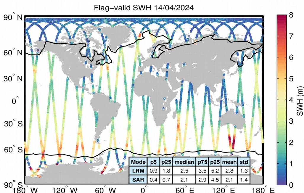
Figure 15. Geographical distribution of flag-valid SWH data over oceans and lakes for 14/04/2024. The statistical values shown in the table refer to the SWH in m and are calculated separately for LRM and SAR regions. Measurements taken over polar polygons have been excluded from the computation of the statistical values. The black lines mark the outer limit of the Arctic and Antarctic polar polygons.
