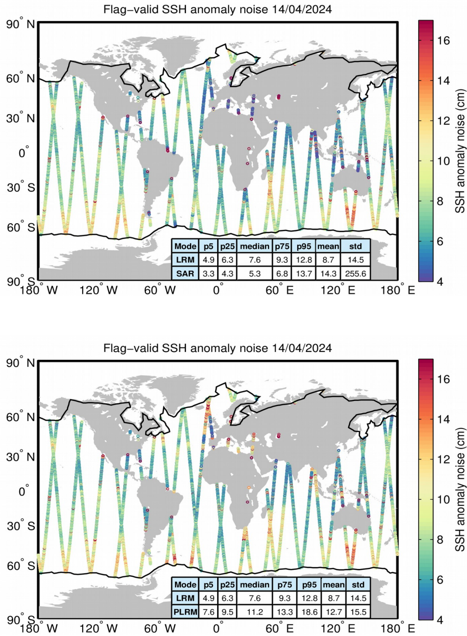
Figure 8. Geographical distribution of flag-valid 20-Hz SSH anomaly measurement noise over oceans and lakes for LRM/SAR (top) and LRM/PLRM (bottom) and for 14/04/2024. The statistical values shown in the tables refer to the SSH anomaly noise and are calculated separately for LRM and SAR/PLRM regions. Measurements taken over polar polygons have been excluded from the computation of the statistical values. The black lines mark the outer limit of the Arctic and Antarctic polar polygons.
