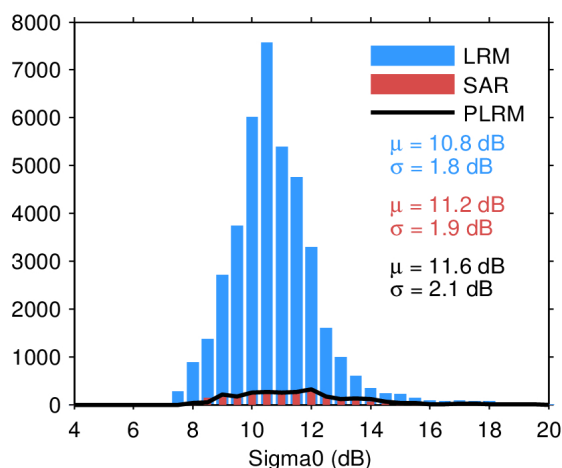
Figure 28. Histogram of science-valid sigma0 over oceans and lakes for LRM (blue), SAR (red), and PLRM (black) for 14/04/2024. The mean ( \mu ) and standard deviation ( \sigma ) are also shown. Note that values outside [4 20] dB are excluded from the histogram for the sake of readability but not from the computation of \mu and \sigma .
