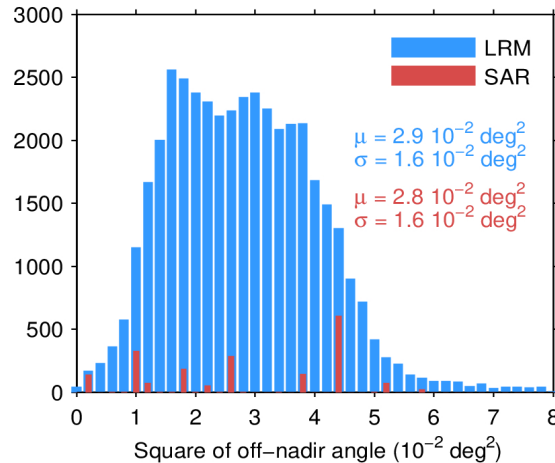
Figure 39. Histogram of flag-valid mispointing over oceans and lakes for LRM (blue) and SAR (red) for 14/04/2024. Only positive values have been considered. The mean ( \mu ) and standard deviation ( \sigma ) are also shown. Note that values larger than 8 \cdot 10^{-2} \text{ deg}^2 are excluded from the histogram for the sake of readability but not from the computation of \mu and \sigma .
