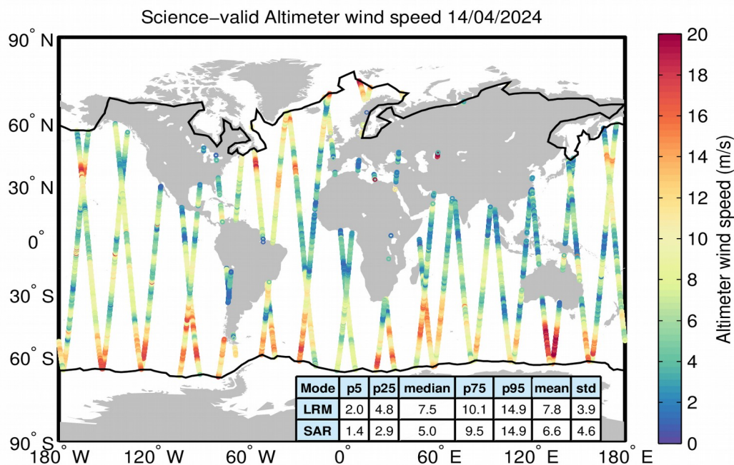
Figure 34. Geographical distribution of science-valid wind data over oceans and lakes for 14/04/2024. The statistical values shown in the table refer to the wind in m/s and are calculated separately for LRM and SAR regions. The black lines mark the outer limit of the Arctic and Antarctic polar polygons. Gray circles denote records that have been rejected based on the editing criteria described in Table 5.
