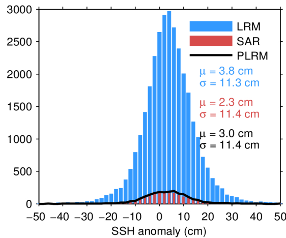
Figure 11. Histogram of science-valid SSH anomaly over oceans and lakes for LRM (blue), SAR (red), and PLRM (black) for 14/04/2024. The mean ( \mu ) and standard deviation ( \sigma ) are also shown. Note that values outside [-50\ 50] cm are excluded from the histogram for the sake of readability but not from the computation of \mu and \sigma .
