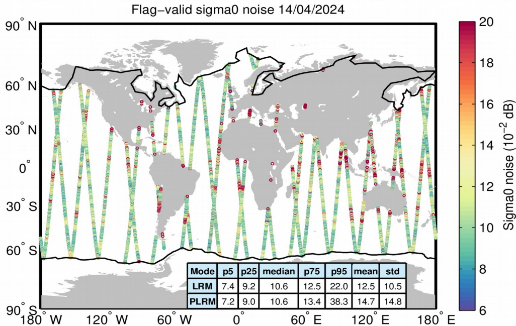
Figure 26. Geographical distribution of flag-valid 20-Hz sigma0 measurement noise over oceans and lakes for LRM/SAR (top) and LRM/PLRM (bottom) and for 14/04/2024. The statistical values shown in the table refer to the sigma0 noise and are calculated separately for LRM and SAR/PLRM regions. Measurements taken over polar polygons have been excluded from the computation of the statistical values. The black lines mark the outer limit of the Arctic and Antarctic polar polygons.
