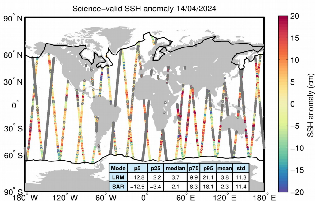
Figure 10. Geographical distribution of science-valid SSH anomaly data over oceans and lakes for 14/04/2024. The statistical values shown in the table refer to the SSH anomaly in cm and are calculated separately for LRM and SAR regions. The black lines mark the
