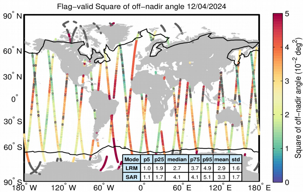
Figure 37. Geographical distribution of flag-valid mispointing data over oceans and lakes for 12/04/2024. The statistical values shown in the table refer to the mispointing in 10^{-2} \text{ deg}^2 and are calculated separately for LRM and SAR regions. Measurements taken over polar polygons have been excluded from the computation of the statistical values. The black lines mark the outer limit of the Arctic and Antarctic polar polygons. Gray circles denote negative values.
