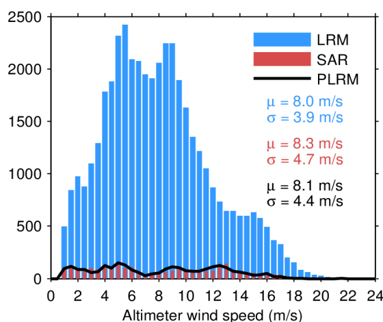
Figure 33. Histogram of flag-valid wind over oceans and lakes for LRM (blue), SAR (red), and PLRM (black) for 12/04/2024. The mean ( \mu ) and standard deviation ( \sigma ) are also shown. Note that values larger than 24 m/s are excluded from the histogram for the sake of readability but not from the computation of \mu and \sigma .
