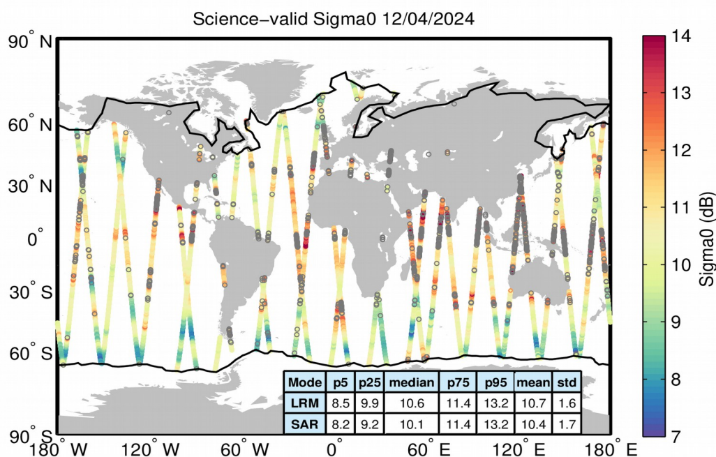
Figure 27. Geographical distribution of science-valid sigma0 data over oceans and lakes for 12/04/2024. The statistical values shown in the table refer to the sigma0 in dB and are calculated separately for LRM and SAR regions. The black lines mark the outer limit of the Arctic and Antarctic polar polygons. Gray circles denote records that have been rejected based on the editing criteria described in Table 4.
