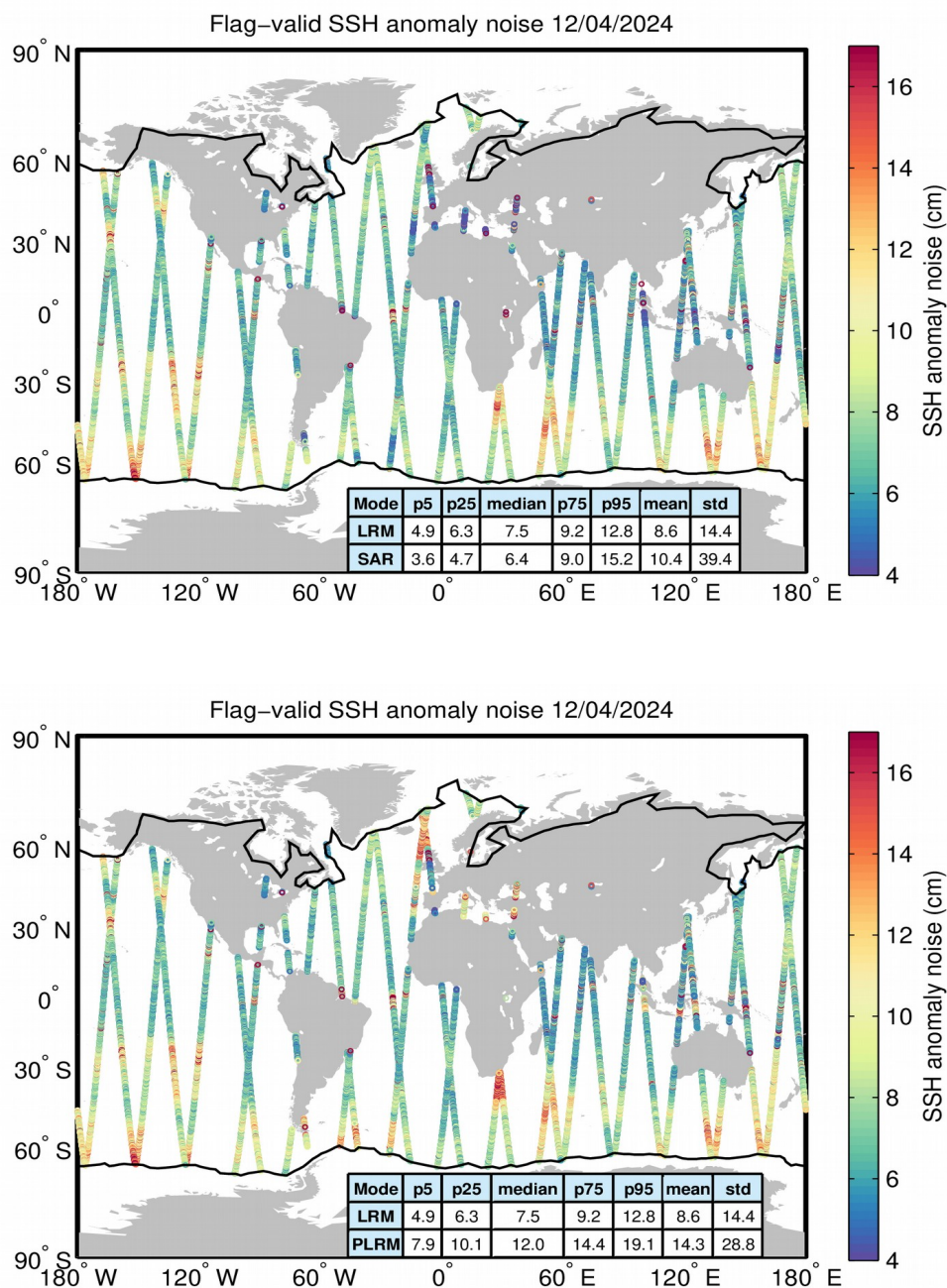
Figure 8. Geographical distribution of flag-valid 20-Hz SSH anomaly measurement noise over oceans and lakes for LRM/SAR (top) and LRM/PLRM (bottom) and for 12/04/2024. The statistical values shown in the tables refer to the SSH anomaly noise and are calculated separately for LRM and SAR/PLRM regions. Measurements taken over polar polygons have been excluded from the computation of the statistical values. The black lines mark the outer limit of the Arctic and Antarctic polar polygons.
