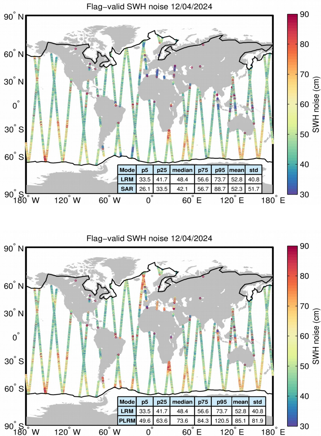
Figure 18. Geographical distribution of flag-valid 20-Hz SWH measurement noise over oceans and lakes for LRM/SAR (top) and LRM/PLRM (bottom) and for 12/04/2024. The statistical values shown in the table refer to the SWH noise and are calculated separately for LRM and SAR/PLRM regions. Measurements taken over polar polygons have been
