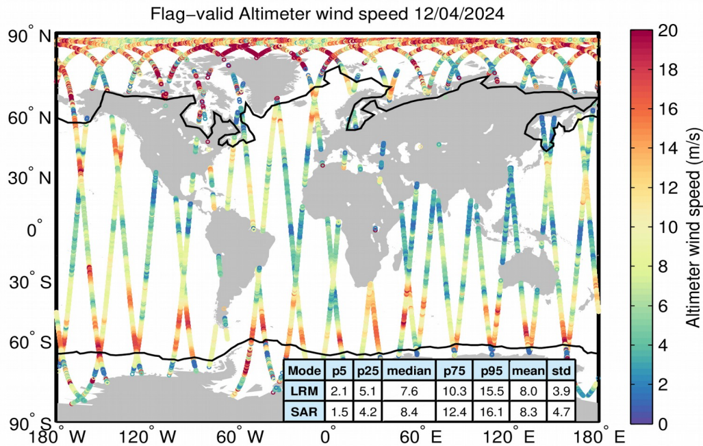
Figure 31. Geographical distribution of flag-valid wind data over oceans and lakes for 12/04/2024. The statistical values shown in the table refer to the wind in m/s and are calculated separately for LRM and SAR regions. Measurements taken over polar polygons have been excluded from the computation of the statistical values. The black lines mark the outer limit of the Arctic and Antarctic polar polygons.
