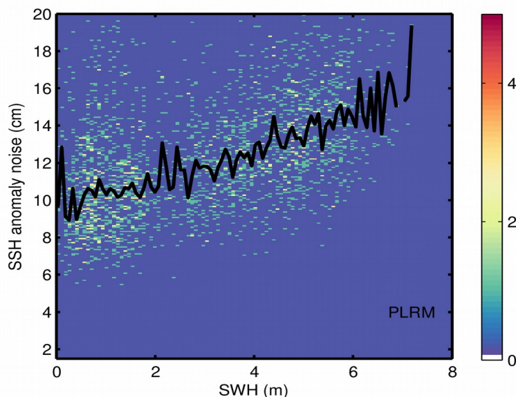
Figure 9. 2D histogram showing flag-valid SSH anomaly noise as a function of SWH for LRM (top), SAR (middle), and PLRM (bottom) for 12/04/2024. The black line denotes the median SSH anomaly noise as a function of SWH.
