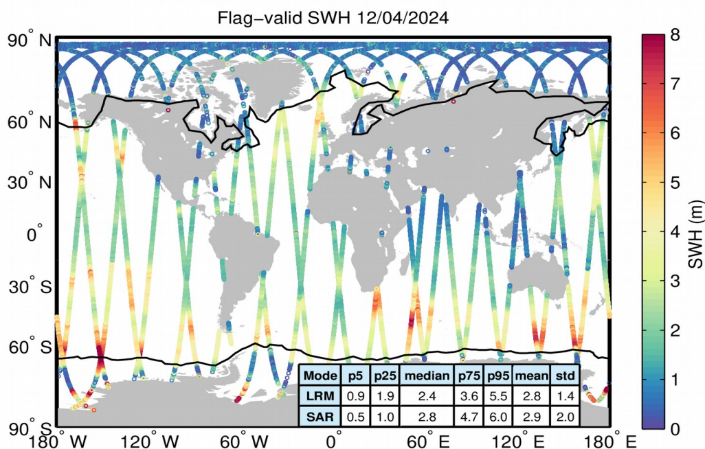
Figure 15. Geographical distribution of flag-valid SWH data over oceans and lakes for 12/04/2024. The statistical values shown in the table refer to the SWH in m and are calculated separately for LRM and SAR regions. Measurements taken over polar polygons have been excluded from the computation of the statistical values. The black lines mark the outer limit of the Arctic and Antarctic polar polygons.
