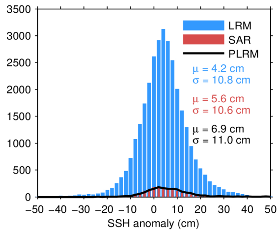
Figure 11. Histogram of science-valid SSH anomaly over oceans and lakes for LRM (blue), SAR (red), and PLRM (black) for 12/04/2024. The mean ( \mu ) and standard deviation ( \sigma ) are also shown. Note that values outside [-50\ 50] cm are excluded from the histogram for the sake of readability but not from the computation of \mu and \sigma .
