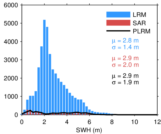
Figure 17. Histogram of flag-valid SWH over oceans and lakes for LRM (blue), SAR (red), and PLRM (black) for 12/04/2024. The mean ( \mu ) and standard deviation ( \sigma ) are also shown. Note that values larger than 12 m are excluded from the histogram for the sake of readability but not from the computation of \mu and \sigma .
