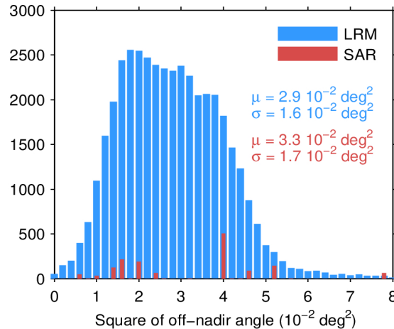
Figure 39. Histogram of flag-valid mispointing over oceans and lakes for LRM (blue) and SAR (red) for 12/04/2024. Only positive values have been considered. The mean ( \mu ) and standard deviation ( \sigma ) are also shown. Note that values larger than 8 \cdot 10^{-2} \text{ deg}^2 are excluded from the histogram for the sake of readability but not from the computation of \mu and \sigma .
