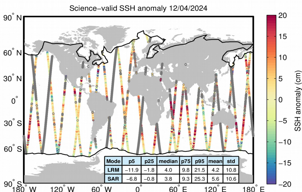
Figure 10. Geographical distribution of science-valid SSH anomaly data over oceans and lakes for 12/04/2024. The statistical values shown in the table refer to the SSH anomaly in cm and are calculated separately for LRM and SAR regions. The black lines mark the
