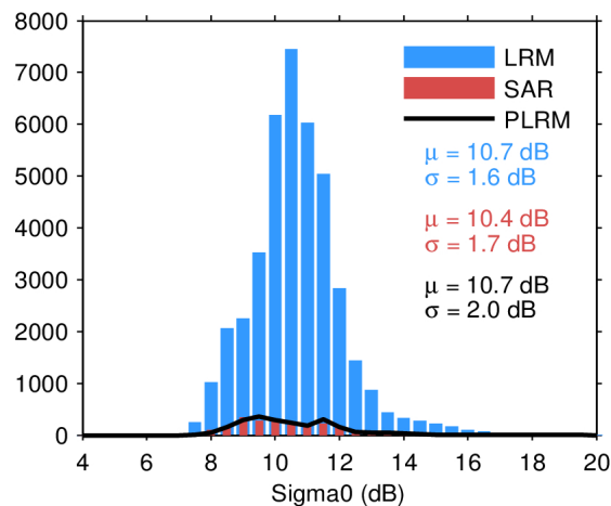
Figure 28. Histogram of science-valid sigma0 over oceans and lakes for LRM (blue), SAR (red), and PLRM (black) for 12/04/2024. The mean ( \mu ) and standard deviation ( \sigma ) are also shown. Note that values outside [4 20] dB are excluded from the histogram for the sake of readability but not from the computation of \mu and \sigma .
