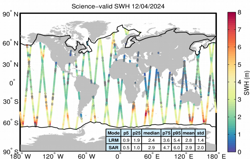
Figure 19. Geographical distribution of science-valid SWH data over oceans and lakes for 12/04/2024. The statistical values shown in the table refer to the SWH in m and are calculated separately for LRM and SAR regions. The black lines mark the outer limit of the Arctic and Antarctic polar polygons. Gray circles denote records that have been rejected based on the editing criteria described in Table 3.
