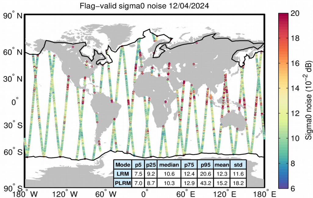
Figure 26. Geographical distribution of flag-valid 20-Hz sigma0 measurement noise over oceans and lakes for LRM/SAR (top) and LRM/PLRM (bottom) and for 12/04/2024. The statistical values shown in the table refer to the sigma0 noise and are calculated separately for LRM and SAR/PLRM regions. Measurements taken over polar polygons have been excluded from the computation of the statistical values. The black lines mark the outer limit of the Arctic and Antarctic polar polygons.
