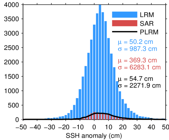
Figure 7. Histogram of flag-valid SSH anomaly over oceans and lakes for LRM (blue), SAR (red), and PLRM (black) for 12/04/2024. The mean ( \mu ) and standard deviation ( \sigma ) are also shown. Note that values outside [-50 50] cm are excluded from the histogram for the sake of readability but not from the computation of \mu and \sigma .
