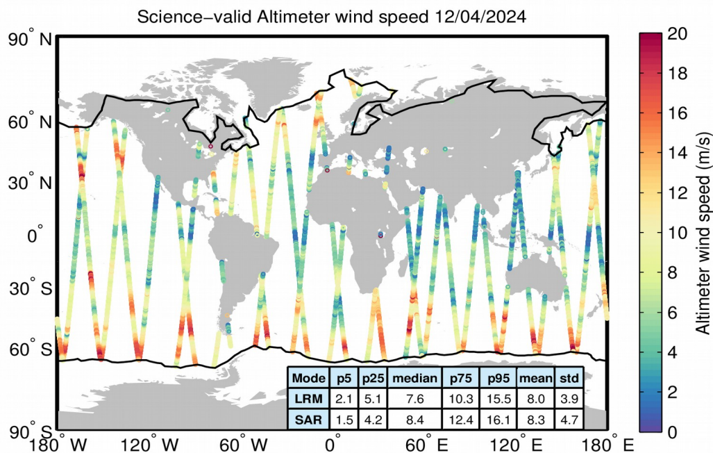
Figure 34. Geographical distribution of science-valid wind data over oceans and lakes for 12/04/2024. The statistical values shown in the table refer to the wind in m/s and are calculated separately for LRM and SAR regions. The black lines mark the outer limit of the Arctic and Antarctic polar polygons. Gray circles denote records that have been rejected based on the editing criteria described in Table 5.
