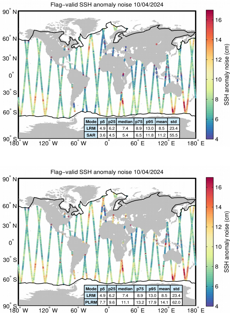
Figure 8. Geographical distribution of flag-valid 20-Hz SSH anomaly measurement noise over oceans and lakes for LRM/SAR (top) and LRM/PLRM (bottom) and for 10/04/2024. The statistical values shown in the tables refer to the SSH anomaly noise and are calculated separately for LRM and SAR/PLRM regions. Measurements taken over polar polygons have been excluded from the computation of the statistical values. The black lines mark the outer limit of the Arctic and Antarctic polar polygons.
