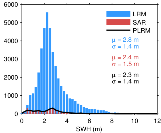
Figure 17. Histogram of flag-valid SWH over oceans and lakes for LRM (blue), SAR (red), and PLRM (black) for 10/04/2024. The mean ( \mu ) and standard deviation ( \sigma ) are also shown. Note that values larger than 12 m are excluded from the histogram for the sake of readability but not from the computation of \mu and \sigma .
