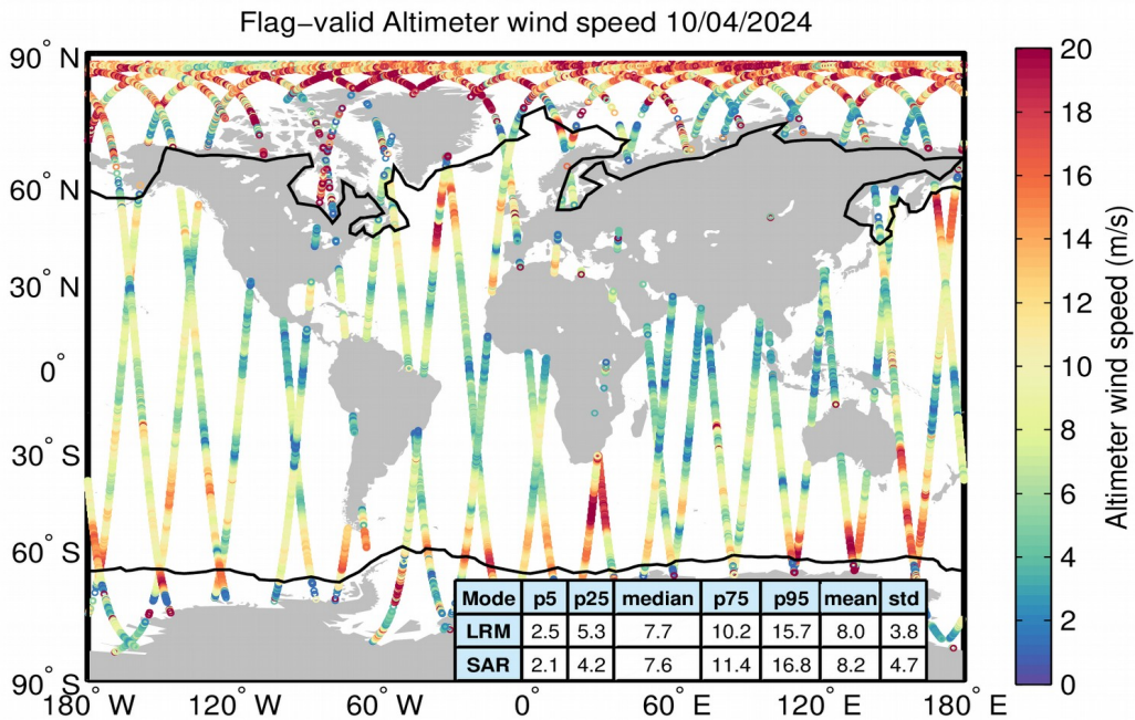
Figure 31. Geographical distribution of flag-valid wind data over oceans and lakes for 10/04/2024. The statistical values shown in the table refer to the wind in m/s and are calculated separately for LRM and SAR regions. Measurements taken over polar polygons have been excluded from the computation of the statistical values. The black lines mark the outer limit of the Arctic and Antarctic polar polygons.
