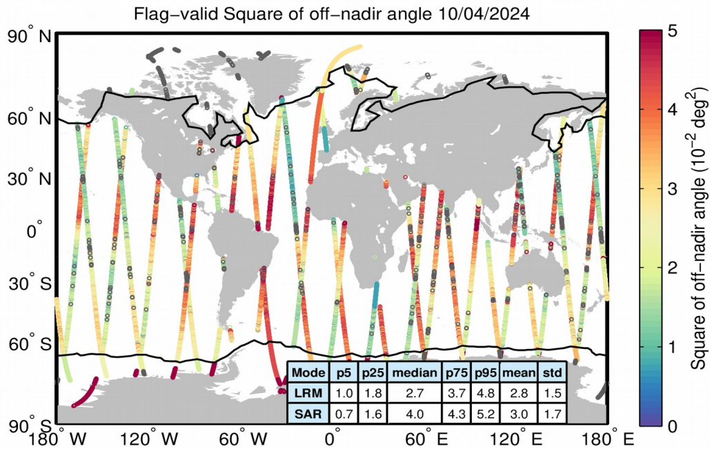
Figure 37. Geographical distribution of flag-valid mispointing data over oceans and lakes for 10/04/2024. The statistical values shown in the table refer to the mispointing in 10^{-2} \text{ deg}^2 and are calculated separately for LRM and SAR regions. Measurements taken over polar polygons have been excluded from the computation of the statistical values. The black lines mark the outer limit of the Arctic and Antarctic polar polygons. Gray circles denote negative values.
