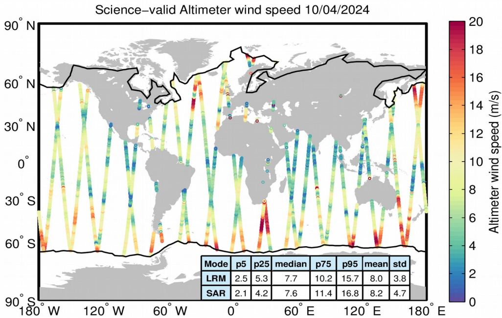
Figure 34. Geographical distribution of science-valid wind data over oceans and lakes for 10/04/2024. The statistical values shown in the table refer to the wind in m/s and are calculated separately for LRM and SAR regions. The black lines mark the outer limit of the Arctic and Antarctic polar polygons. Gray circles denote records that have been rejected based on the editing criteria described in Table 5.
