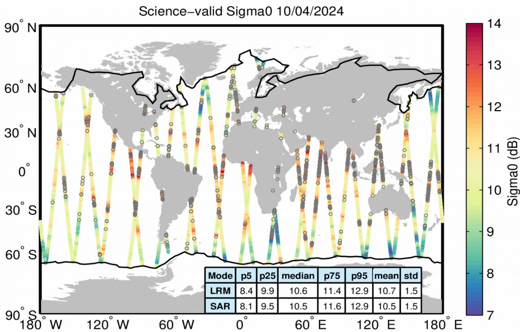
Figure 27. Geographical distribution of science-valid sigma0 data over oceans and lakes for 10/04/2024. The statistical values shown in the table refer to the sigma0 in dB and are calculated separately for LRM and SAR regions. The black lines mark the outer limit of the Arctic and Antarctic polar polygons. Gray circles denote records that have been rejected based on the editing criteria described in Table 4.
