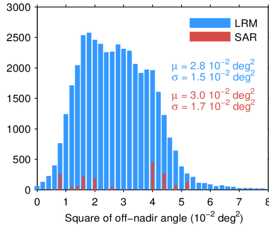
Figure 39. Histogram of flag-valid mispointing over oceans and lakes for LRM (blue) and SAR (red) for 10/04/2024. Only positive values have been considered. The mean ( \mu ) and standard deviation ( \sigma ) are also shown. Note that values larger than 8 \cdot 10^{-2} \text{ deg}^2 are excluded from the histogram for the sake of readability but not from the computation of \mu and \sigma .
