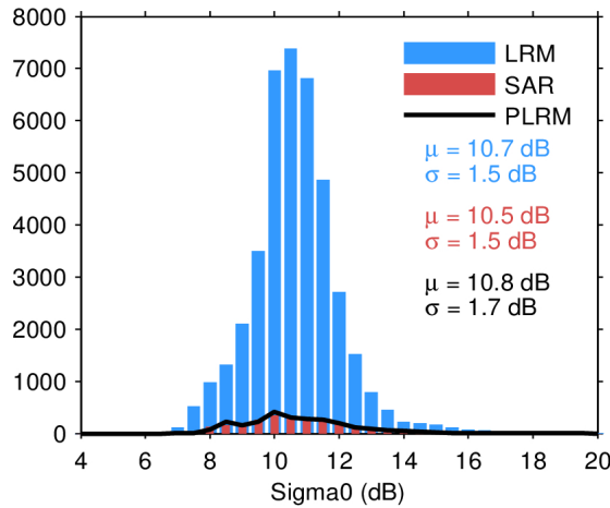
Figure 28. Histogram of science-valid sigma0 over oceans and lakes for LRM (blue), SAR (red), and PLRM (black) for 10/04/2024. The mean ( \mu ) and standard deviation ( \sigma ) are also shown. Note that values outside [4 20] dB are excluded from the histogram for the sake of readability but not from the computation of \mu and \sigma .
