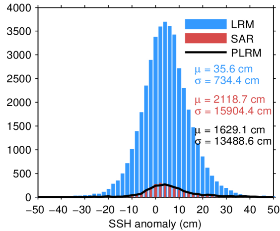
Figure 7. Histogram of flag-valid SSH anomaly over oceans and lakes for LRM (blue), SAR (red), and PLRM (black) for 10/04/2024. The mean ( \mu ) and standard deviation ( \sigma ) are also shown. Note that values outside [-50 50] cm are excluded from the histogram for the sake of readability but not from the computation of \mu and \sigma .
