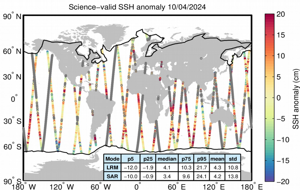
Figure 10. Geographical distribution of science-valid SSH anomaly data over oceans and lakes for 10/04/2024. The statistical values shown in the table refer to the SSH anomaly in cm and are calculated separately for LRM and SAR regions. The black lines mark the
