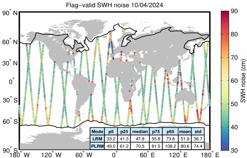
Figure 18. Geographical distribution of flag-valid 20-Hz SWH measurement noise over oceans and lakes for LRM/SAR (top) and LRM/PLRM (bottom) and for 10/04/2024. The statistical values shown in the table refer to the SWH noise and are calculated separately for LRM and SAR/PLRM regions. Measurements taken over polar polygons have been
