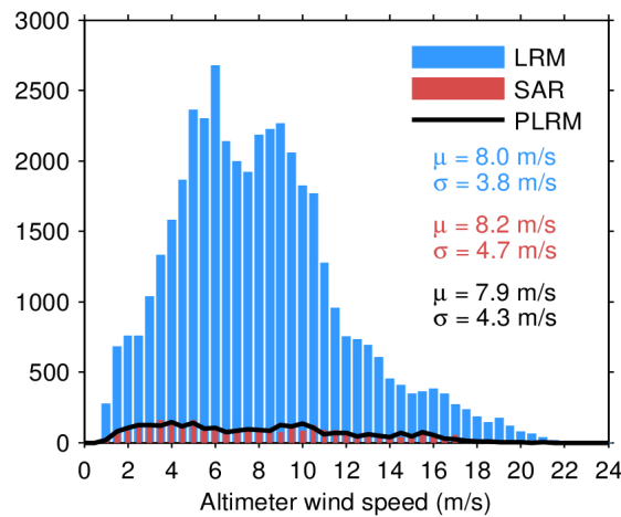
Figure 33. Histogram of flag-valid wind over oceans and lakes for LRM (blue), SAR (red), and PLRM (black) for 10/04/2024. The mean ( \mu ) and standard deviation ( \sigma ) are also shown. Note that values larger than 24 m/s are excluded from the histogram for the sake of readability but not from the computation of \mu and \sigma .
