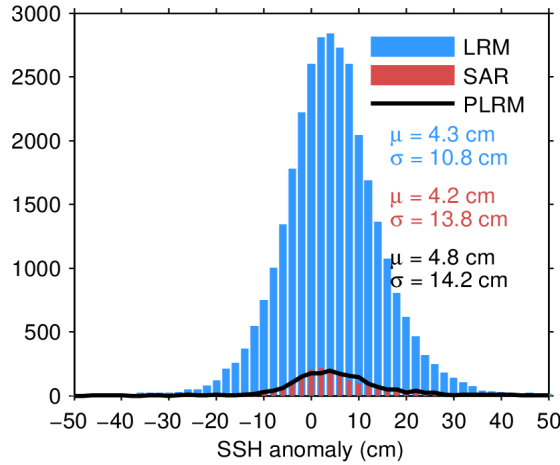
Figure 11. Histogram of science-valid SSH anomaly over oceans and lakes for LRM (blue), SAR (red), and PLRM (black) for 10/04/2024. The mean ( \mu ) and standard deviation ( \sigma ) are also shown. Note that values outside [-50 50] cm are excluded from the histogram for the sake of readability but not from the computation of \mu and \sigma .
