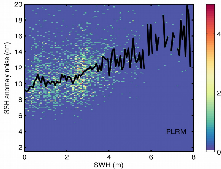
Figure 9. 2D histogram showing flag-valid SSH anomaly noise as a function of SWH for LRM (top), SAR (middle), and PLRM (bottom) for 10/04/2024. The black line denotes the median SSH anomaly noise as a function of SWH.
