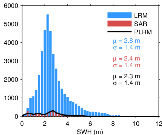
Figure 20. Histogram of science-valid SWH over oceans and lakes for LRM (blue), SAR (red), and PLRM (black) for 10/04/2024. The mean ( \mu ) and standard deviation ( \sigma ) are also
