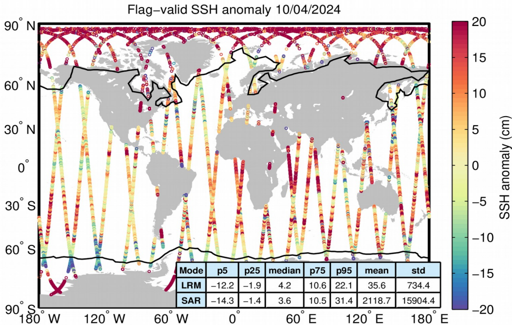
Figure 5. Geographical distribution of flag-valid 1-Hz SSH anomaly data over oceans and lakes for 10/04/2024. The statistical values shown in the table refer to the SSH anomaly in cm and are calculated separately for LRM and SAR regions. Measurements taken over polar polygons have been excluded from the computation of the statistical values. The black lines mark the outer limit of the Arctic and Antarctic polar polygons.
