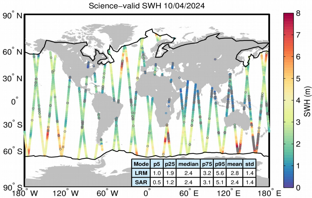
Figure 19. Geographical distribution of science-valid SWH data over oceans and lakes for 10/04/2024. The statistical values shown in the table refer to the SWH in m and are calculated separately for LRM and SAR regions. The black lines mark the outer limit of the Arctic and Antarctic polar polygons. Gray circles denote records that have been rejected based on the editing criteria described in Table 3.
