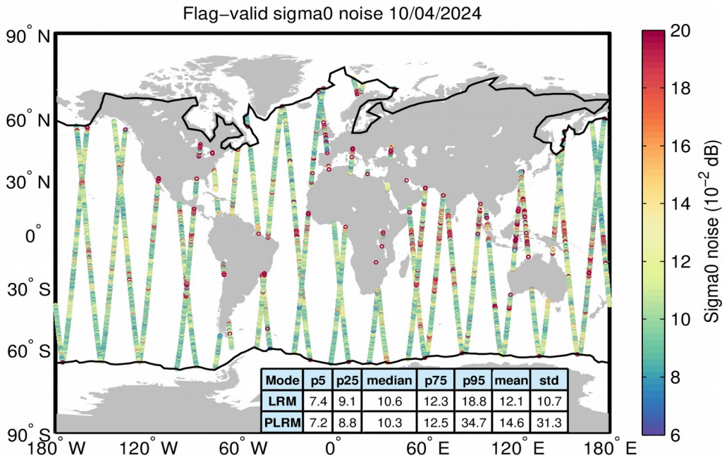
Figure 26. Geographical distribution of flag-valid 20-Hz sigma0 measurement noise over oceans and lakes for LRM/SAR (top) and LRM/PLRM (bottom) and for 10/04/2024. The statistical values shown in the table refer to the sigma0 noise and are calculated separately for LRM and SAR/PLRM regions. Measurements taken over polar polygons have been excluded from the computation of the statistical values. The black lines mark the outer limit of the Arctic and Antarctic polar polygons.
