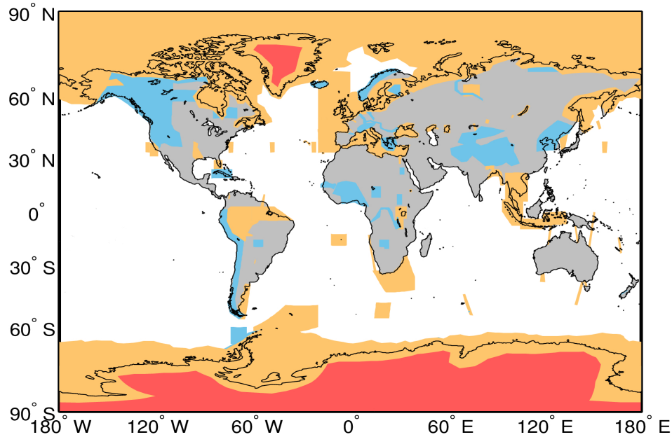
Figure A1. Extent of the regions defining the geographical mode mask for 09/04/2024. The regions where SAR, and SARIn are operated are denoted by the orange and blue polygons, respectively. LRM is operated over areas of the continental ice sheets (red polygons) and over oceans and land not covered by other modes.
