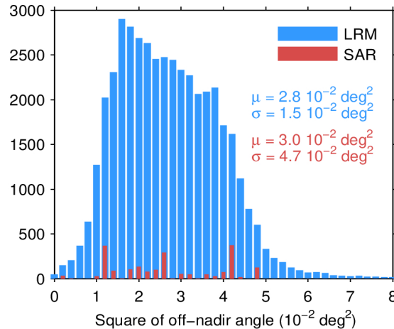
Figure 39. Histogram of flag-valid mispointing over oceans and lakes for LRM (blue) and SAR (red) for 09/04/2024. Only positive values have been considered. The mean ( \mu ) and standard deviation ( \sigma ) are also shown. Note that values larger than 8 \cdot 10^{-2} \text{ deg}^2 are excluded from the histogram for the sake of readability but not from the computation of \mu and \sigma .
