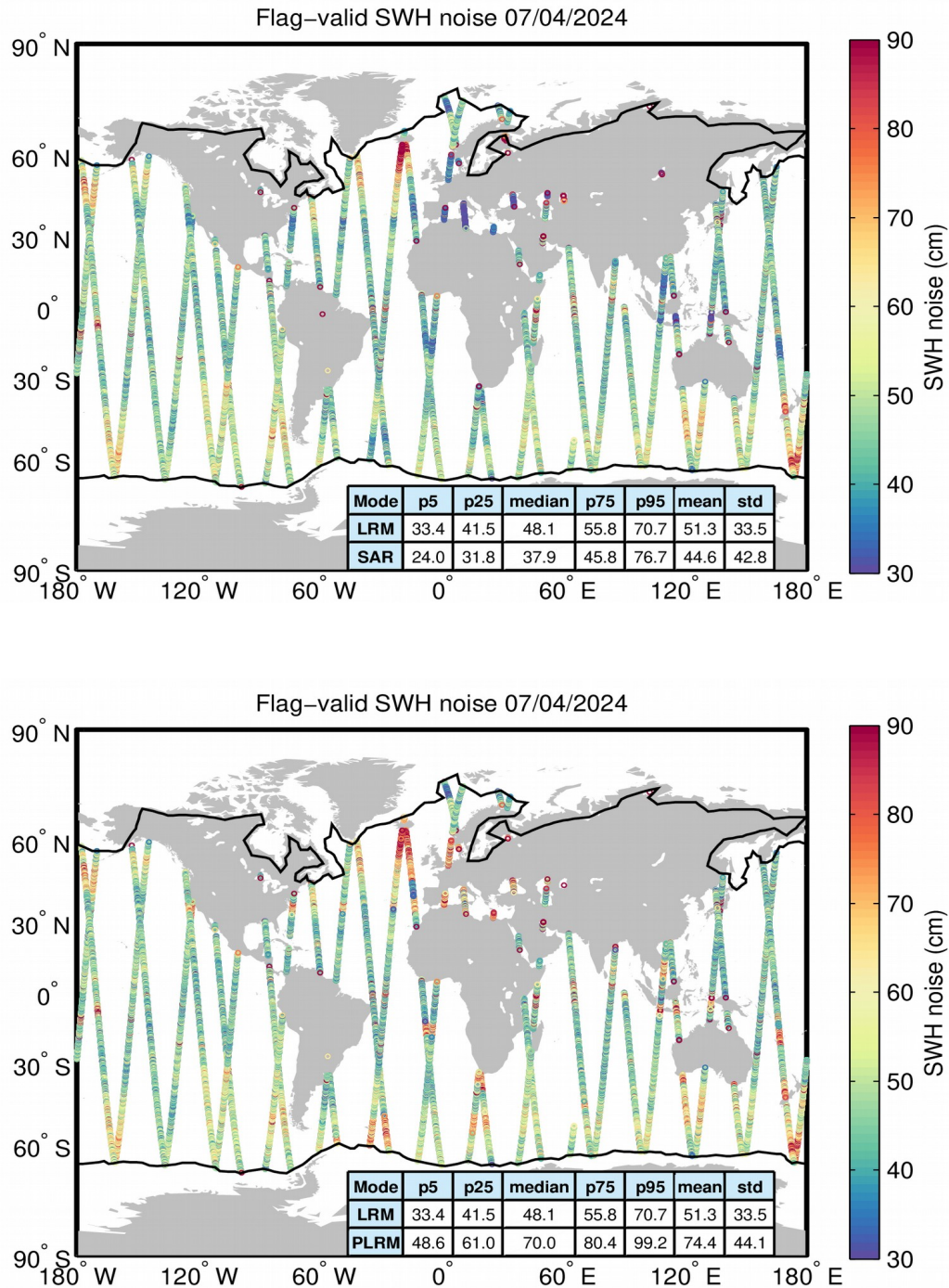
Figure 18. Geographical distribution of flag-valid 20-Hz SWH measurement noise over oceans and lakes for LRM/SAR (top) and LRM/PLRM (bottom) and for 07/04/2024. The statistical values shown in the table refer to the SWH noise and are calculated separately for LRM and SAR/PLRM regions. Measurements taken over polar polygons have been
