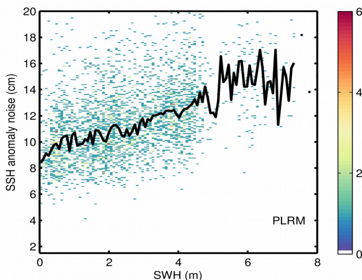
Figure 9. 2D histogram showing flag-valid SSH anomaly noise as a function of SWH for LRM (top), SAR (middle), and PLRM (bottom) for 07/04/2024. The black line denotes the median SSH anomaly noise as a function of SWH.
