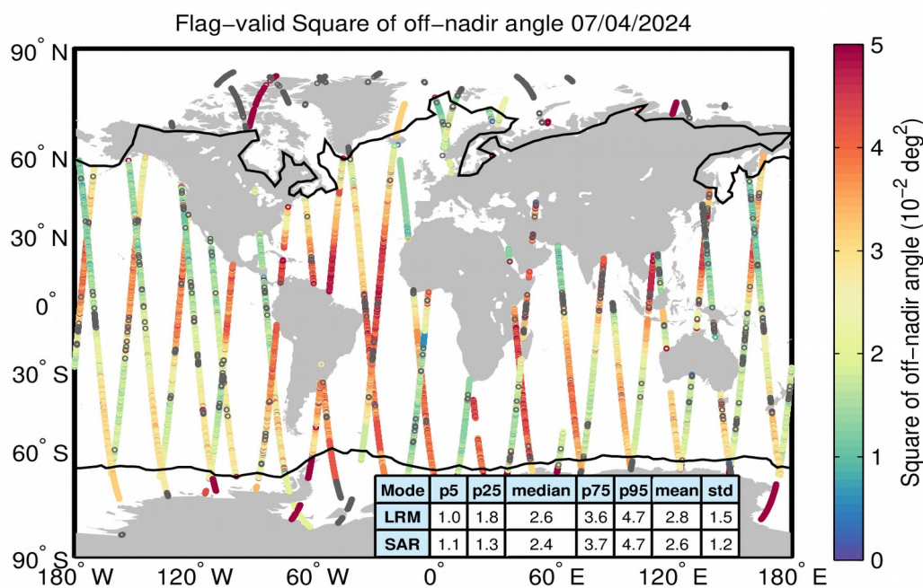
Figure 37. Geographical distribution of flag-valid mispointing data over oceans and lakes for 07/04/2024. The statistical values shown in the table refer to the mispointing in 10^{-2} \text{ deg}^2 and are calculated separately for LRM and SAR regions. Measurements taken over polar polygons have been excluded from the computation of the statistical values. The black lines mark the outer limit of the Arctic and Antarctic polar polygons. Gray circles denote negative values.
