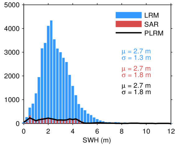
Figure 17. Histogram of flag-valid SWH over oceans and lakes for LRM (blue), SAR (red), and PLRM (black) for 07/04/2024. The mean ( \mu ) and standard deviation ( \sigma ) are also shown. Note that values larger than 12 m are excluded from the histogram for the sake of readability but not from the computation of \mu and \sigma .
