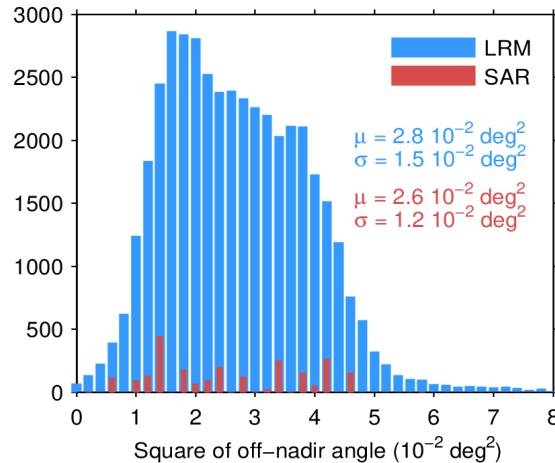
Figure 39. Histogram of flag-valid mispointing over oceans and lakes for LRM (blue) and SAR (red) for 07/04/2024. Only positive values have been considered. The mean ( \mu ) and standard deviation ( \sigma ) are also shown. Note that values larger than 8 \cdot 10^{-2} \text{ deg}^2 are excluded from the histogram for the sake of readability but not from the computation of \mu and \sigma .
