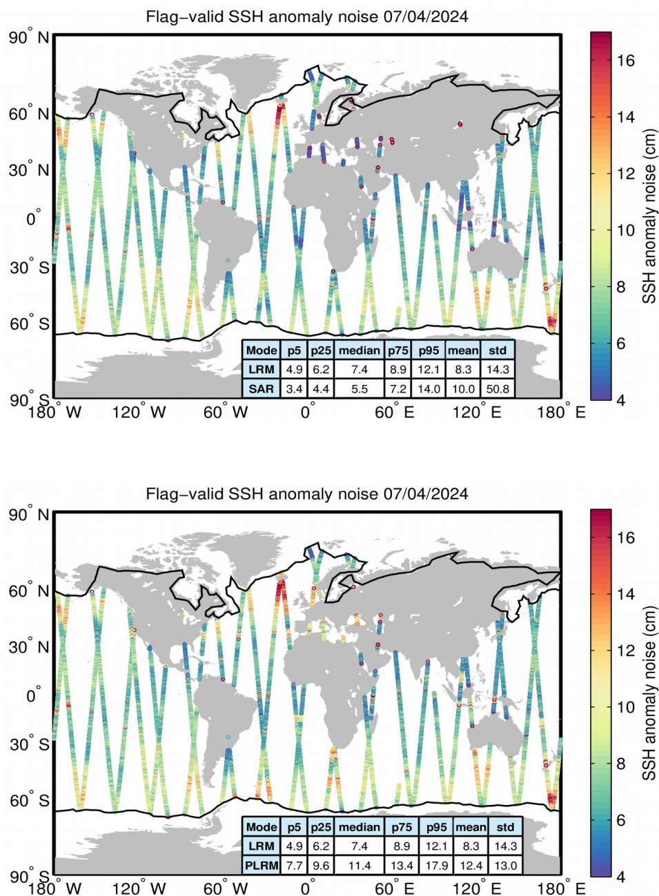
Figure 8. Geographical distribution of flag-valid 20-Hz SSH anomaly measurement noise over oceans and lakes for LRM/SAR (top) and LRM/PLRM (bottom) and for 07/04/2024. The statistical values shown in the tables refer to the SSH anomaly noise and are calculated separately for LRM and SAR/PLRM regions. Measurements taken over polar polygons have been excluded from the computation of the statistical values. The black lines mark the outer limit of the Arctic and Antarctic polar polygons.
