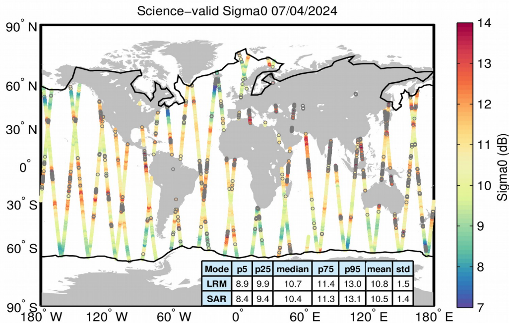
Figure 27. Geographical distribution of science-valid sigma0 data over oceans and lakes for 07/04/2024. The statistical values shown in the table refer to the sigma0 in dB and are calculated separately for LRM and SAR regions. The black lines mark the outer limit of the Arctic and Antarctic polar polygons. Gray circles denote records that have been rejected based on the editing criteria described in Table 4.
