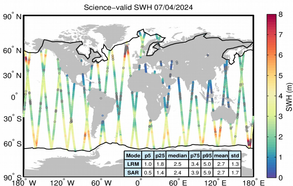
Figure 19. Geographical distribution of science-valid SWH data over oceans and lakes for 07/04/2024. The statistical values shown in the table refer to the SWH in m and are calculated separately for LRM and SAR regions. The black lines mark the outer limit of the Arctic and Antarctic polar polygons. Gray circles denote records that have been rejected based on the editing criteria described in Table 3.
