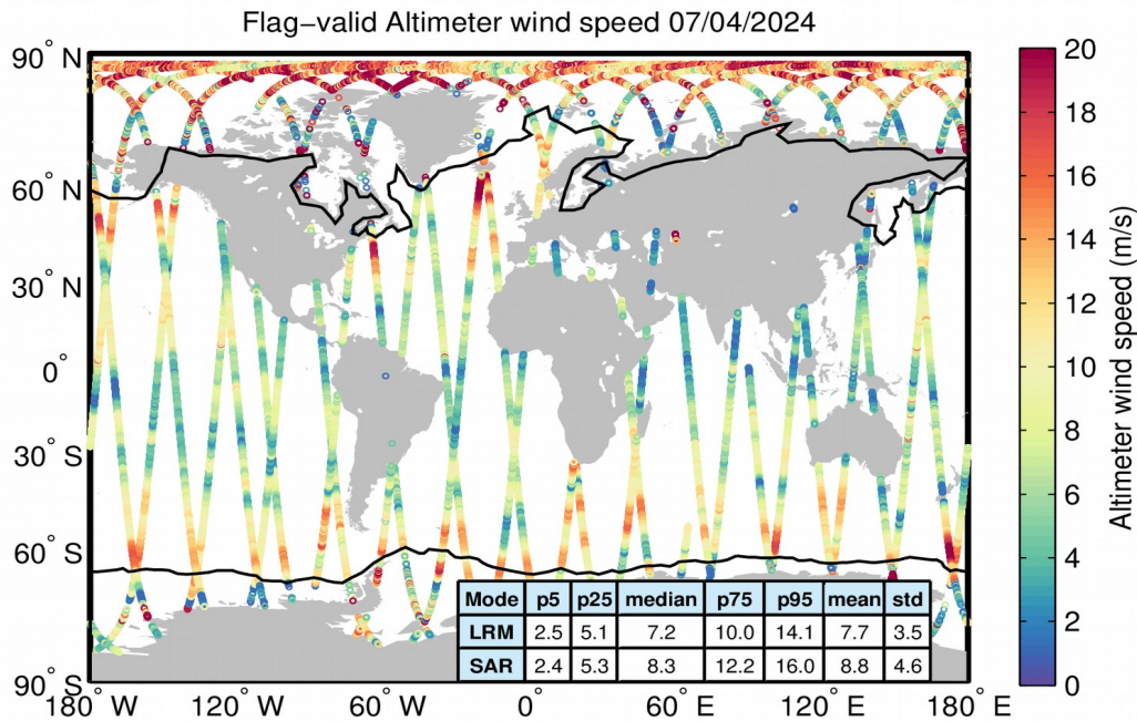
Figure 31. Geographical distribution of flag-valid wind data over oceans and lakes for 07/04/2024. The statistical values shown in the table refer to the wind in m/s and are calculated separately for LRM and SAR regions. Measurements taken over polar polygons have been excluded from the computation of the statistical values. The black lines mark the outer limit of the Arctic and Antarctic polar polygons.
