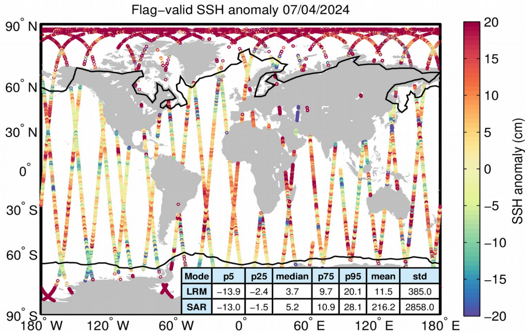
Figure 5. Geographical distribution of flag-valid 1-Hz SSH anomaly data over oceans and lakes for 07/04/2024. The statistical values shown in the table refer to the SSH anomaly in cm and are calculated separately for LRM and SAR regions. Measurements taken over polar polygons have been excluded from the computation of the statistical values. The black lines mark the outer limit of the Arctic and Antarctic polar polygons.
