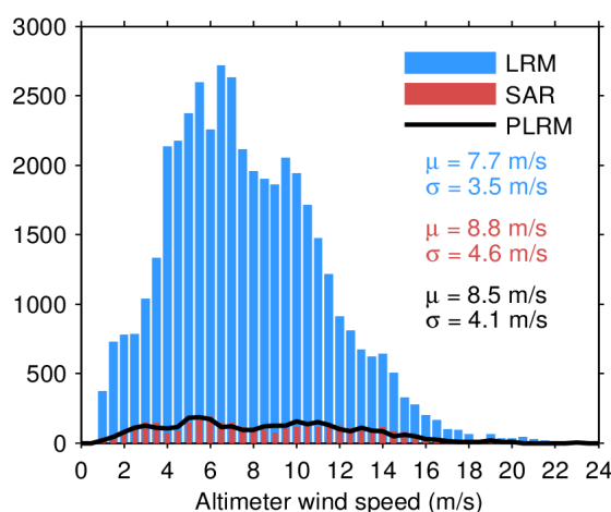
Figure 33. Histogram of flag-valid wind over oceans and lakes for LRM (blue), SAR (red), and PLRM (black) for 07/04/2024. The mean ( \mu ) and standard deviation ( \sigma ) are also shown. Note that values larger than 24 m/s are excluded from the histogram for the sake of readability but not from the computation of \mu and \sigma .
