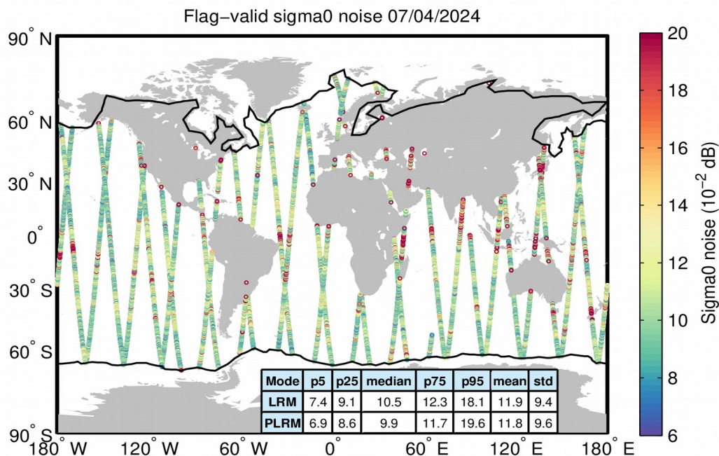
Figure 26. Geographical distribution of flag-valid 20-Hz sigma0 measurement noise over oceans and lakes for LRM/SAR (top) and LRM/PLRM (bottom) and for 07/04/2024. The statistical values shown in the table refer to the sigma0 noise and are calculated separately for LRM and SAR/PLRM regions. Measurements taken over polar polygons have been excluded from the computation of the statistical values. The black lines mark the outer limit of the Arctic and Antarctic polar polygons.
