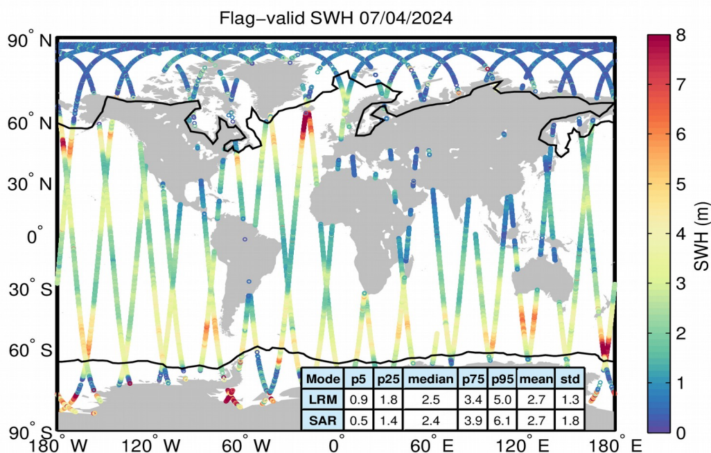
Figure 15. Geographical distribution of flag-valid SWH data over oceans and lakes for 07/04/2024. The statistical values shown in the table refer to the SWH in m and are calculated separately for LRM and SAR regions. Measurements taken over polar polygons have been excluded from the computation of the statistical values. The black lines mark the outer limit of the Arctic and Antarctic polar polygons.
