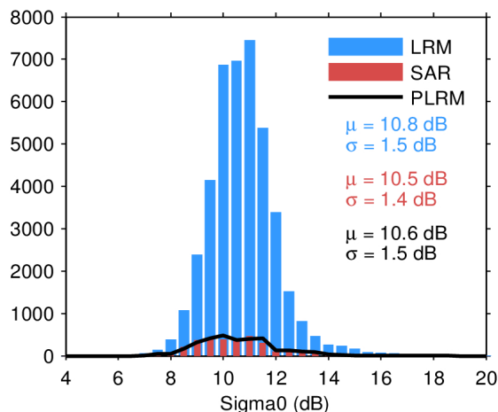
Figure 28. Histogram of science-valid sigma0 over oceans and lakes for LRM (blue), SAR (red), and PLRM (black) for 07/04/2024. The mean ( \mu ) and standard deviation ( \sigma ) are also shown. Note that values outside [4 20] dB are excluded from the histogram for the sake of readability but not from the computation of \mu and \sigma .
