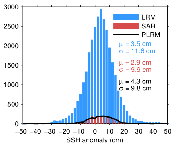
Figure 11. Histogram of science-valid SSH anomaly over oceans and lakes for LRM (blue), SAR (red), and PLRM (black) for 07/04/2024. The mean ( \mu ) and standard deviation ( \sigma ) are also shown. Note that values outside [-50\ 50] cm are excluded from the histogram for the sake of readability but not from the computation of \mu and \sigma .
