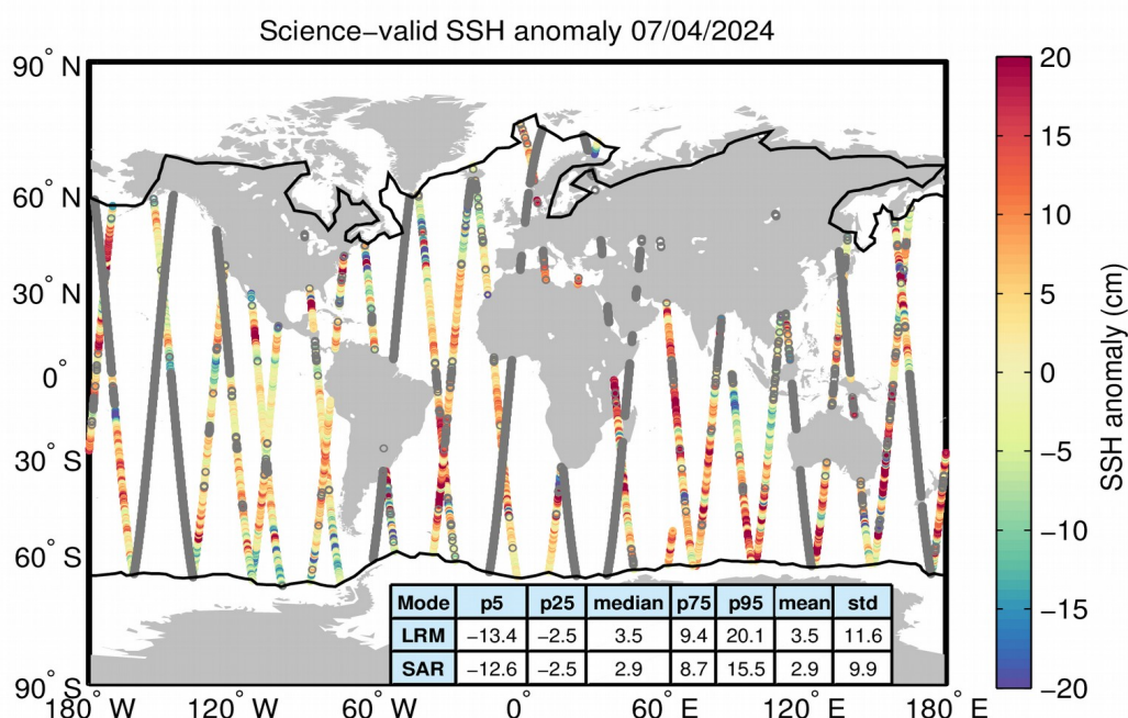
Figure 10. Geographical distribution of science-valid SSH anomaly data over oceans and lakes for 07/04/2024. The statistical values shown in the table refer to the SSH anomaly in cm and are calculated separately for LRM and SAR regions. The black lines mark the
