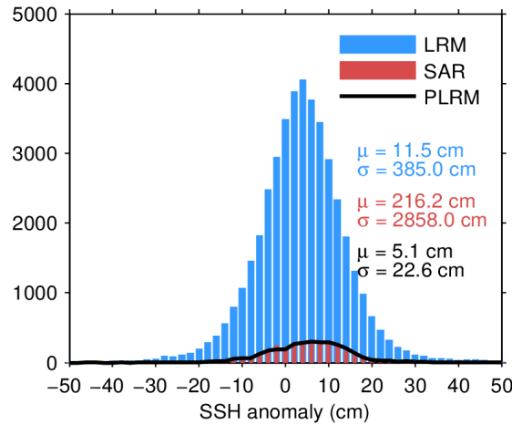
Figure 7. Histogram of flag-valid SSH anomaly over oceans and lakes for LRM (blue), SAR (red), and PLRM (black) for 07/04/2024. The mean ( \mu ) and standard deviation ( \sigma ) are also shown. Note that values outside [-50\ 50] cm are excluded from the histogram for the sake of readability but not from the computation of \mu and \sigma .
