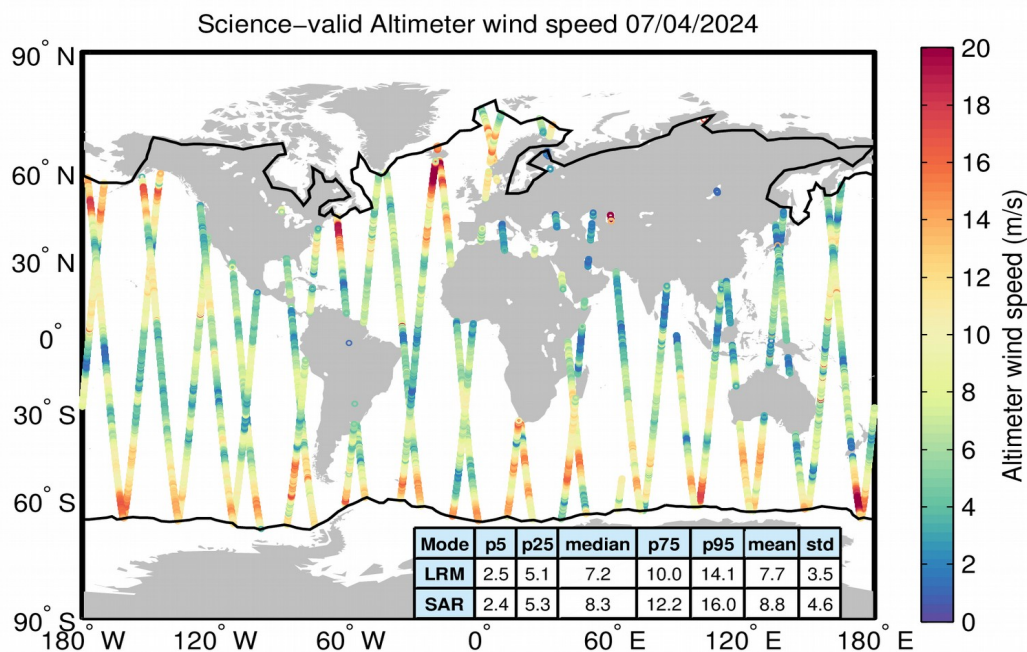
Figure 34. Geographical distribution of science-valid wind data over oceans and lakes for 07/04/2024. The statistical values shown in the table refer to the wind in m/s and are calculated separately for LRM and SAR regions. The black lines mark the outer limit of the Arctic and Antarctic polar polygons. Gray circles denote records that have been rejected based on the editing criteria described in Table 5.
