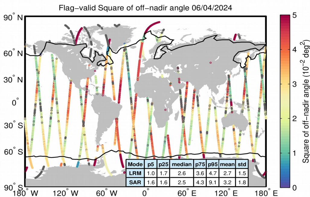
Figure 37. Geographical distribution of flag-valid mispointing data over oceans and lakes for 06/04/2024. The statistical values shown in the table refer to the mispointing in 10^{-2} \text{ deg}^2 and are calculated separately for LRM and SAR regions. Measurements taken over polar polygons have been excluded from the computation of the statistical values. The black lines mark the outer limit of the Arctic and Antarctic polar polygons. Gray circles denote negative values.
