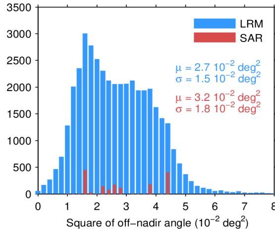
Figure 39. Histogram of flag-valid mispointing over oceans and lakes for LRM (blue) and SAR (red) for 06/04/2024. Only positive values have been considered. The mean ( \mu ) and standard deviation ( \sigma ) are also shown. Note that values larger than 8 \cdot 10^{-2} \text{ deg}^2 are excluded from the histogram for the sake of readability but not from the computation of \mu and \sigma .
