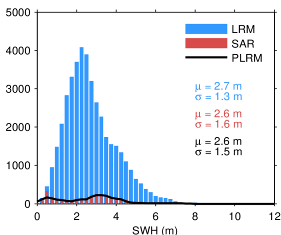
Figure 20. Histogram of science-valid SWH over oceans and lakes for LRM (blue), SAR (red), and PLRM (black) for 06/04/2024. The mean ( \mu ) and standard deviation ( \sigma ) are also
