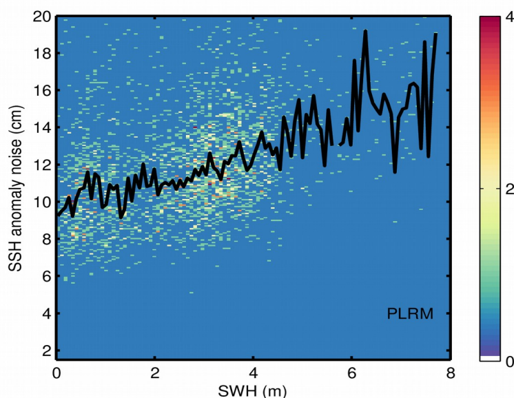
Figure 9. 2D histogram showing flag-valid SSH anomaly noise as a function of SWH for LRM (top), SAR (middle), and PLRM (bottom) for 06/04/2024. The black line denotes the median SSH anomaly noise as a function of SWH.
