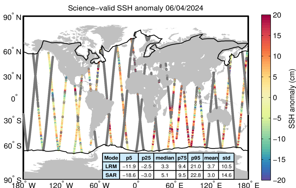
Figure 10. Geographical distribution of science-valid SSH anomaly data over oceans and lakes for 06/04/2024. The statistical values shown in the table refer to the SSH anomaly in cm and are calculated separately for LRM and SAR regions. The black lines mark the
