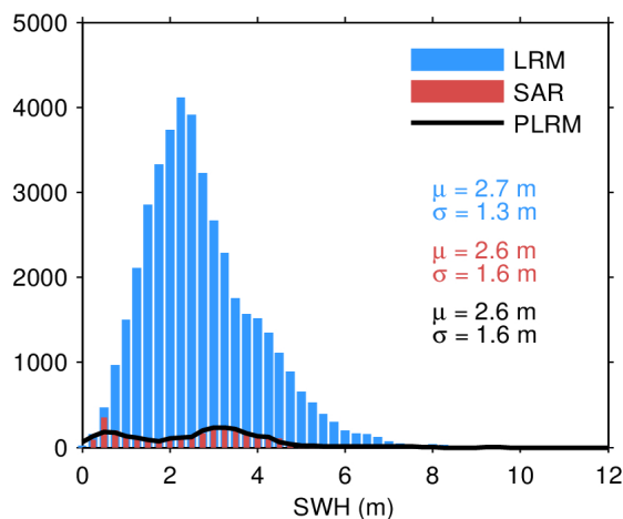
Figure 17. Histogram of flag-valid SWH over oceans and lakes for LRM (blue), SAR (red), and PLRM (black) for 06/04/2024. The mean ( \mu ) and standard deviation ( \sigma ) are also shown. Note that values larger than 12 m are excluded from the histogram for the sake of readability but not from the computation of \mu and \sigma .
