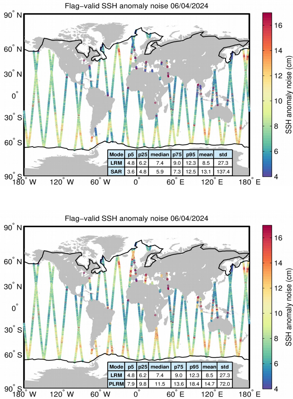
Figure 8. Geographical distribution of flag-valid 20-Hz SSH anomaly measurement noise over oceans and lakes for LRM/SAR (top) and LRM/PLRM (bottom) and for 06/04/2024. The statistical values shown in the tables refer to the SSH anomaly noise and are calculated separately for LRM and SAR/PLRM regions. Measurements taken over polar polygons have been excluded from the computation of the statistical values. The black lines mark the outer limit of the Arctic and Antarctic polar polygons.
