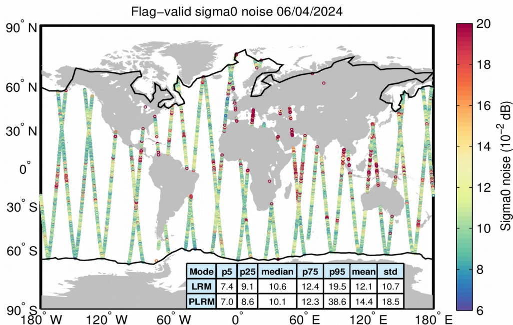
Figure 26. Geographical distribution of flag-valid 20-Hz sigma0 measurement noise over oceans and lakes for LRM/SAR (top) and LRM/PLRM (bottom) and for 06/04/2024. The statistical values shown in the table refer to the sigma0 noise and are calculated separately for LRM and SAR/PLRM regions. Measurements taken over polar polygons have been excluded from the computation of the statistical values. The black lines mark the outer limit of the Arctic and Antarctic polar polygons.
