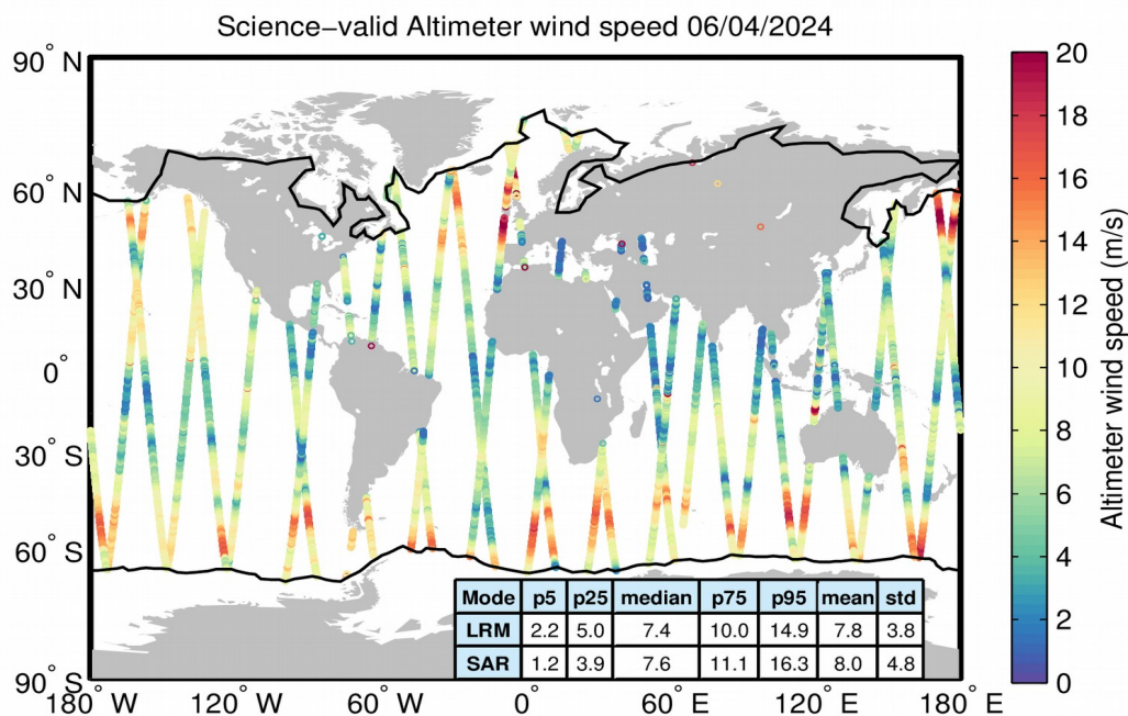
Figure 34. Geographical distribution of science-valid wind data over oceans and lakes for 06/04/2024. The statistical values shown in the table refer to the wind in m/s and are calculated separately for LRM and SAR regions. The black lines mark the outer limit of the Arctic and Antarctic polar polygons. Gray circles denote records that have been rejected based on the editing criteria described in Table 5.
