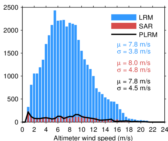
Figure 33. Histogram of flag-valid wind over oceans and lakes for LRM (blue), SAR (red), and PLRM (black) for 06/04/2024. The mean ( \mu ) and standard deviation ( \sigma ) are also shown. Note that values larger than 24 m/s are excluded from the histogram for the sake of readability but not from the computation of \mu and \sigma .
