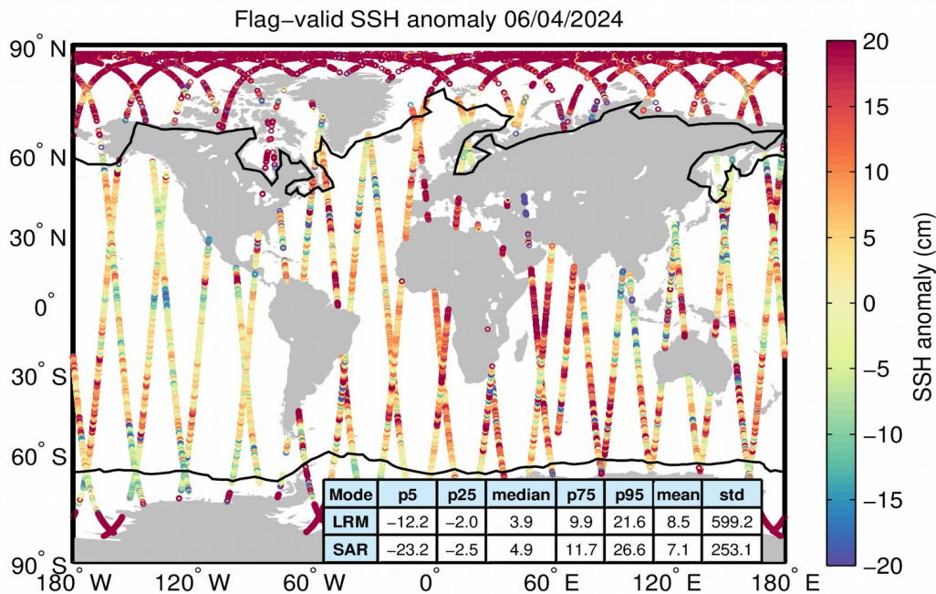
Figure 5. Geographical distribution of flag-valid 1-Hz SSH anomaly data over oceans and lakes for 06/04/2024. The statistical values shown in the table refer to the SSH anomaly in cm and are calculated separately for LRM and SAR regions. Measurements taken over polar polygons have been excluded from the computation of the statistical values. The black lines mark the outer limit of the Arctic and Antarctic polar polygons.
