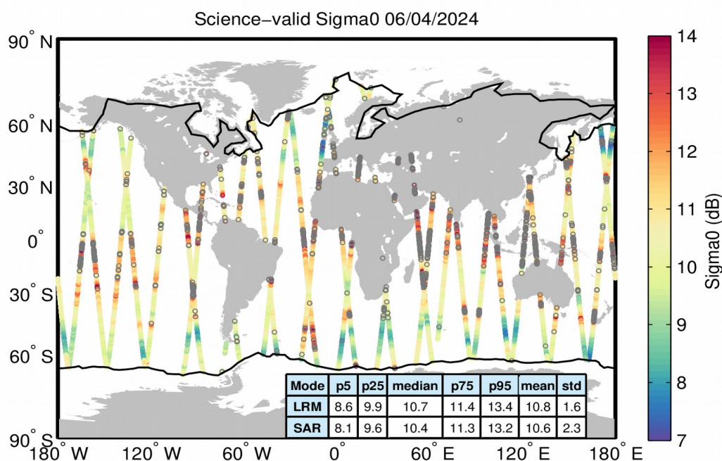
Figure 27. Geographical distribution of science-valid sigma0 data over oceans and lakes for 06/04/2024. The statistical values shown in the table refer to the sigma0 in dB and are calculated separately for LRM and SAR regions. The black lines mark the outer limit of the Arctic and Antarctic polar polygons. Gray circles denote records that have been rejected based on the editing criteria described in Table 4.
