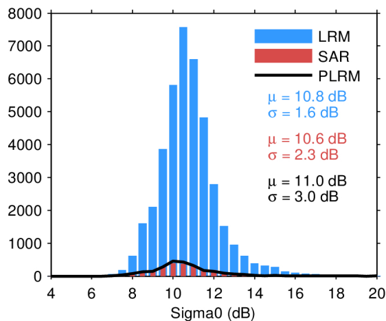
Figure 28. Histogram of science-valid sigma0 over oceans and lakes for LRM (blue), SAR (red), and PLRM (black) for 06/04/2024. The mean ( \mu ) and standard deviation ( \sigma ) are also shown. Note that values outside [4 20] dB are excluded from the histogram for the sake of readability but not from the computation of \mu and \sigma .
