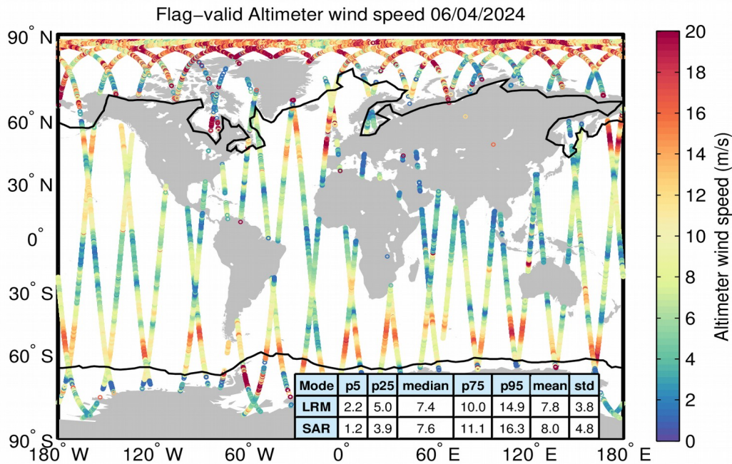
Figure 31. Geographical distribution of flag-valid wind data over oceans and lakes for 06/04/2024. The statistical values shown in the table refer to the wind in m/s and are calculated separately for LRM and SAR regions. Measurements taken over polar polygons have been excluded from the computation of the statistical values. The black lines mark the outer limit of the Arctic and Antarctic polar polygons.
