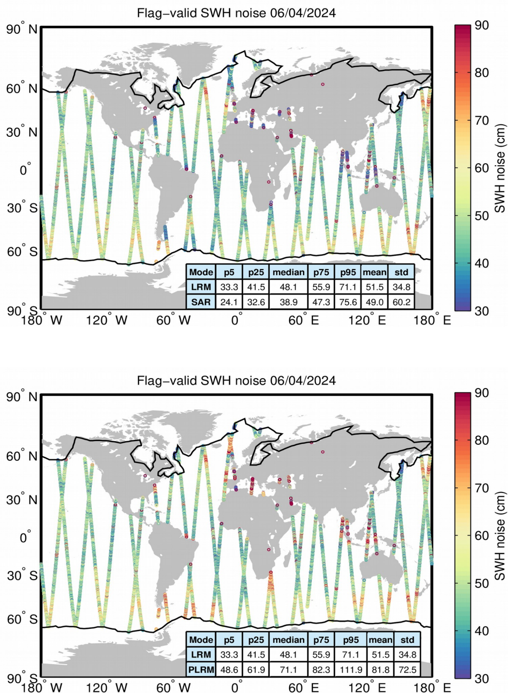
Figure 18. Geographical distribution of flag-valid 20-Hz SWH measurement noise over oceans and lakes for LRM/SAR (top) and LRM/PLRM (bottom) and for 06/04/2024. The statistical values shown in the table refer to the SWH noise and are calculated separately for LRM and SAR/PLRM regions. Measurements taken over polar polygons have been
