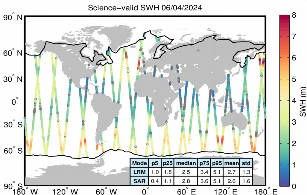
Figure 19. Geographical distribution of science-valid SWH data over oceans and lakes for 06/04/2024. The statistical values shown in the table refer to the SWH in m and are calculated separately for LRM and SAR regions. The black lines mark the outer limit of the Arctic and Antarctic polar polygons. Gray circles denote records that have been rejected based on the editing criteria described in Table 3.
