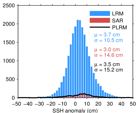
Figure 11. Histogram of science-valid SSH anomaly over oceans and lakes for LRM (blue), SAR (red), and PLRM (black) for 06/04/2024. The mean ( \mu ) and standard deviation ( \sigma ) are also shown. Note that values outside [-50, 50] cm are excluded from the histogram for the sake of readability but not from the computation of \mu and \sigma .
