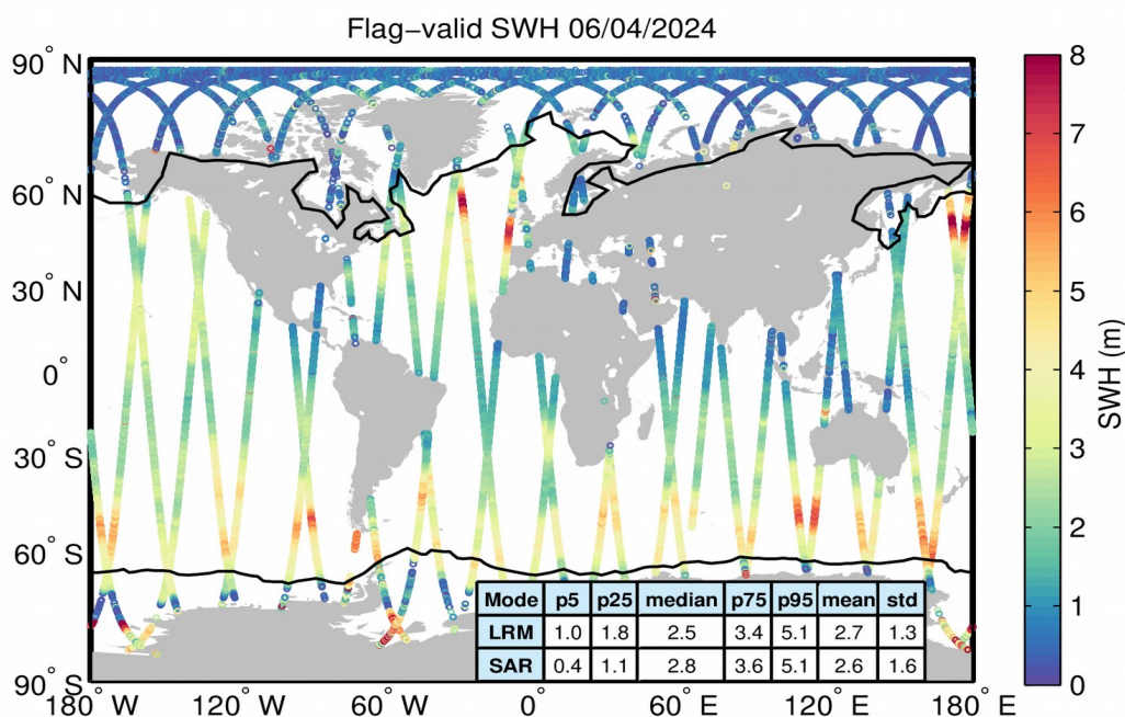
Figure 15. Geographical distribution of flag-valid SWH data over oceans and lakes for 06/04/2024. The statistical values shown in the table refer to the SWH in m and are calculated separately for LRM and SAR regions. Measurements taken over polar polygons have been excluded from the computation of the statistical values. The black lines mark the outer limit of the Arctic and Antarctic polar polygons.
