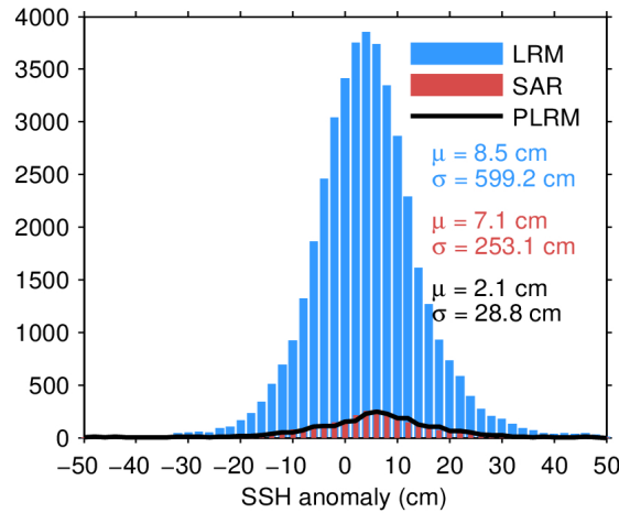
Figure 7. Histogram of flag-valid SSH anomaly over oceans and lakes for LRM (blue), SAR (red), and PLRM (black) for 06/04/2024. The mean ( \mu ) and standard deviation ( \sigma ) are also shown. Note that values outside [-50 50] cm are excluded from the histogram for the sake of readability but not from the computation of \mu and \sigma .
