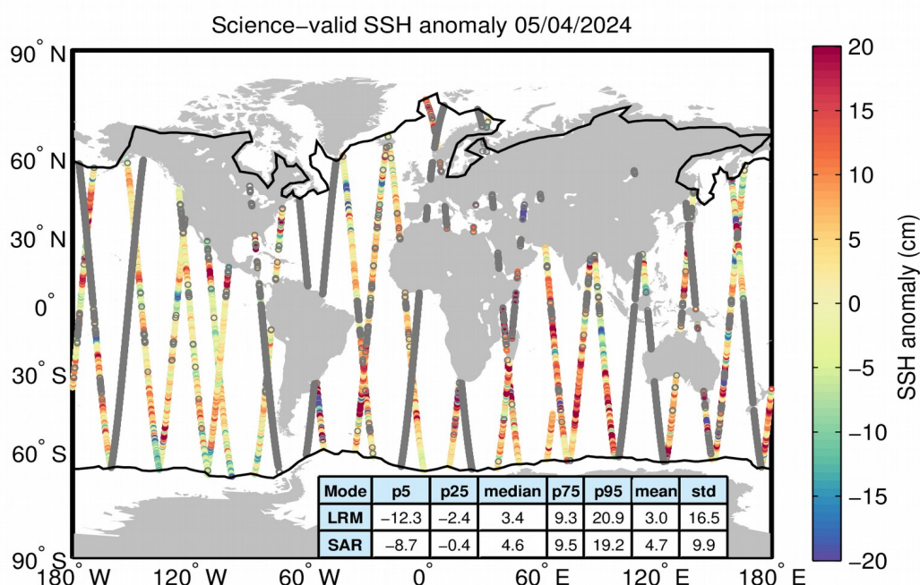
Figure 10. Geographical distribution of science-valid SSH anomaly data over oceans and lakes for 05/04/2024. The statistical values shown in the table refer to the SSH anomaly in cm and are calculated separately for LRM and SAR regions. The black lines mark the
