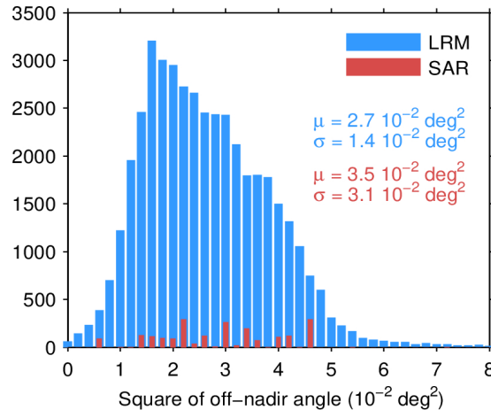
Figure 39. Histogram of flag-valid mispointing over oceans and lakes for LRM (blue) and SAR (red) for 05/04/2024. Only positive values have been considered. The mean ( \mu ) and standard deviation ( \sigma ) are also shown. Note that values larger than 8 \cdot 10^{-2} \text{ deg}^2 are excluded from the histogram for the sake of readability but not from the computation of \mu and \sigma .
