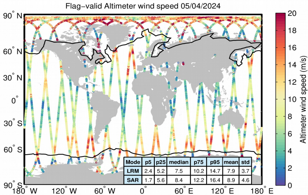
Figure 31. Geographical distribution of flag-valid wind data over oceans and lakes for 05/04/2024. The statistical values shown in the table refer to the wind in m/s and are calculated separately for LRM and SAR regions. Measurements taken over polar polygons have been excluded from the computation of the statistical values. The black lines mark the outer limit of the Arctic and Antarctic polar polygons.
