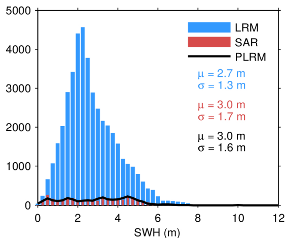
Figure 17. Histogram of flag-valid SWH over oceans and lakes for LRM (blue), SAR (red), and PLRM (black) for 05/04/2024. The mean ( \mu ) and standard deviation ( \sigma ) are also shown. Note that values larger than 12 m are excluded from the histogram for the sake of readability but not from the computation of \mu and \sigma .
