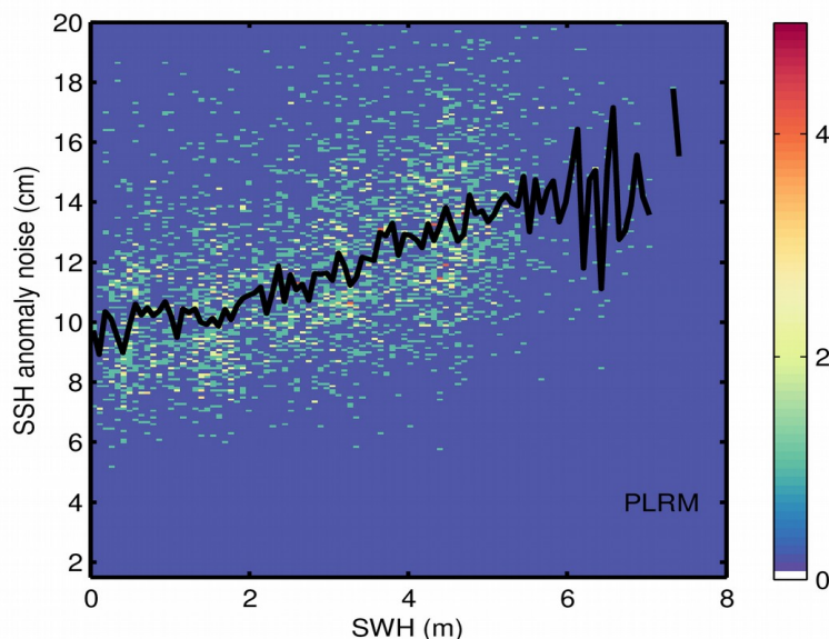
Figure 9. 2D histogram showing flag-valid SSH anomaly noise as a function of SWH for LRM (top), SAR (middle), and PLRM (bottom) for 05/04/2024. The black line denotes the median SSH anomaly noise as a function of SWH.
