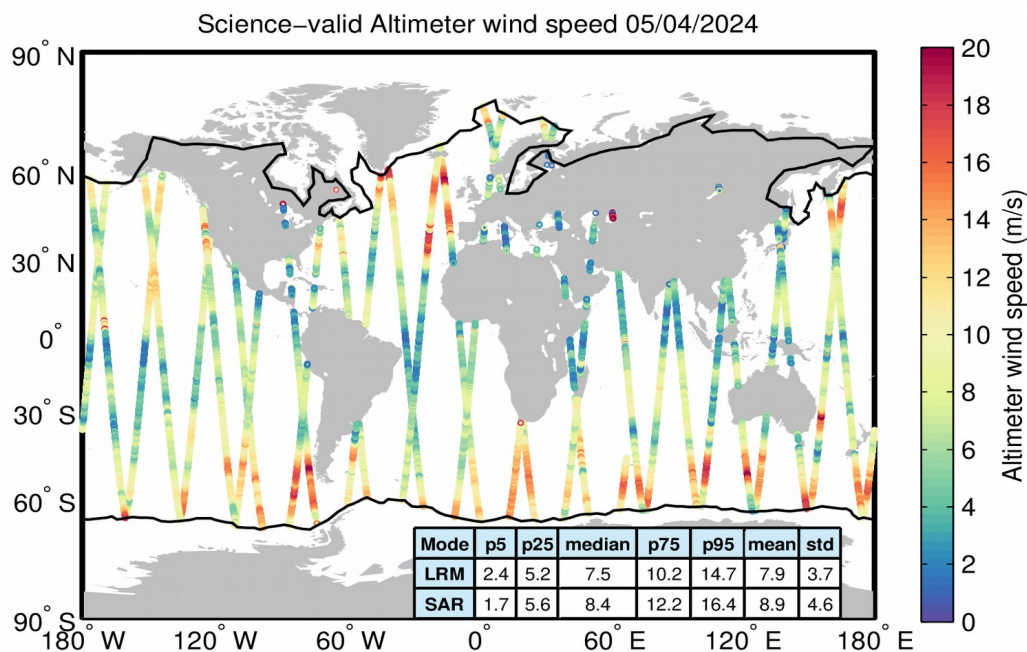
Figure 34. Geographical distribution of science-valid wind data over oceans and lakes for 05/04/2024. The statistical values shown in the table refer to the wind in m/s and are calculated separately for LRM and SAR regions. The black lines mark the outer limit of the Arctic and Antarctic polar polygons. Gray circles denote records that have been rejected based on the editing criteria described in Table 5.
