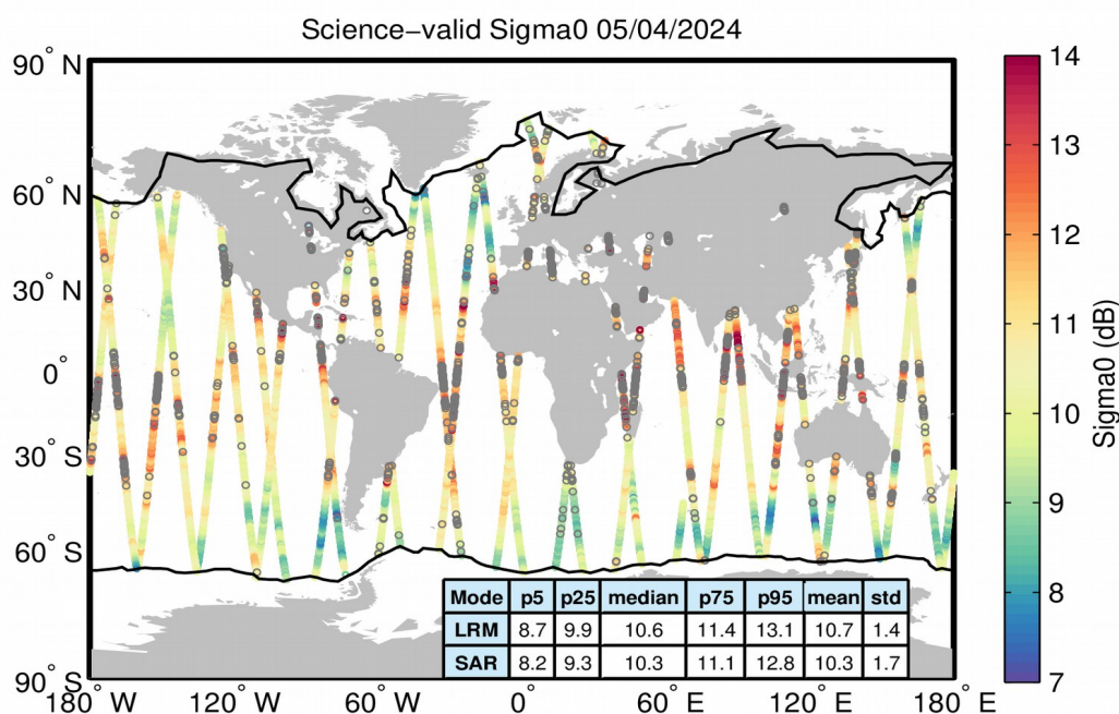
Figure 27. Geographical distribution of science-valid sigma0 data over oceans and lakes for 05/04/2024. The statistical values shown in the table refer to the sigma0 in dB and are calculated separately for LRM and SAR regions. The black lines mark the outer limit of the Arctic and Antarctic polar polygons. Gray circles denote records that have been rejected based on the editing criteria described in Table 4.
