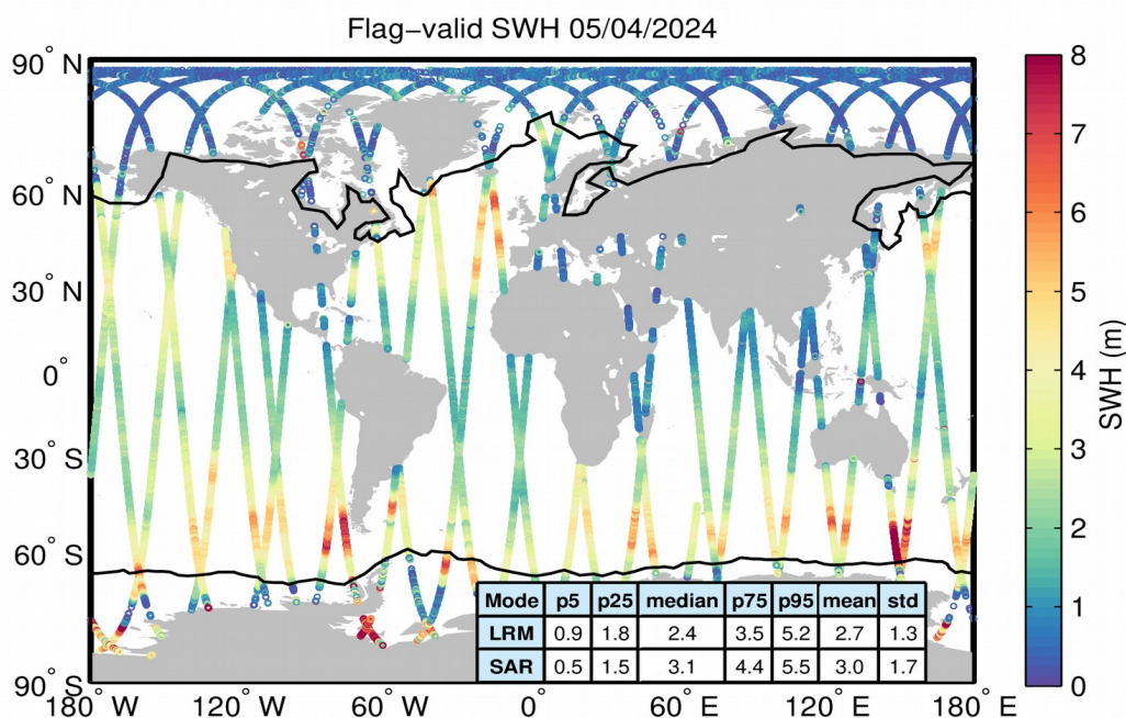
Figure 15. Geographical distribution of flag-valid SWH data over oceans and lakes for 05/04/2024. The statistical values shown in the table refer to the SWH in m and are calculated separately for LRM and SAR regions. Measurements taken over polar polygons have been excluded from the computation of the statistical values. The black lines mark the outer limit of the Arctic and Antarctic polar polygons.
