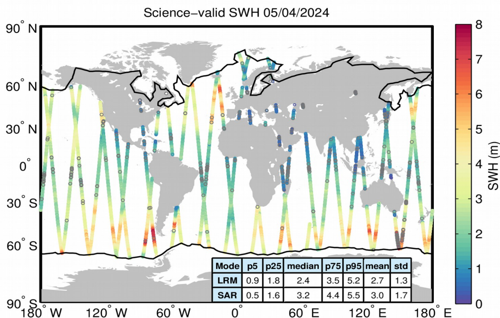
Figure 19. Geographical distribution of science-valid SWH data over oceans and lakes for 05/04/2024. The statistical values shown in the table refer to the SWH in m and are calculated separately for LRM and SAR regions. The black lines mark the outer limit of the Arctic and Antarctic polar polygons. Gray circles denote records that have been rejected based on the editing criteria described in Table 3.
