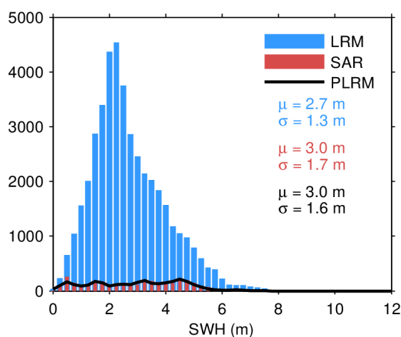
Figure 20. Histogram of science-valid SWH over oceans and lakes for LRM (blue), SAR (red), and PLRM (black) for 05/04/2024. The mean ( \mu ) and standard deviation ( \sigma ) are also
