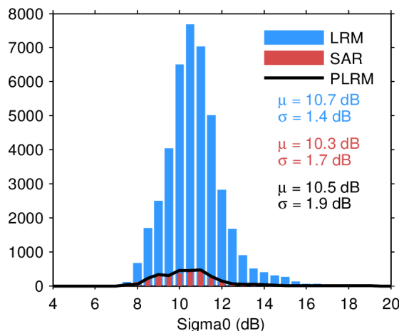
Figure 28. Histogram of science-valid sigma0 over oceans and lakes for LRM (blue), SAR (red), and PLRM (black) for 05/04/2024. The mean ( \mu ) and standard deviation ( \sigma ) are also shown. Note that values outside [4 20] dB are excluded from the histogram for the sake of readability but not from the computation of \mu and \sigma .
