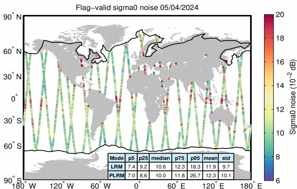
Figure 26. Geographical distribution of flag-valid 20-Hz sigma0 measurement noise over oceans and lakes for LRM/SAR (top) and LRM/PLRM (bottom) and for 05/04/2024. The statistical values shown in the table refer to the sigma0 noise and are calculated separately for LRM and SAR/PLRM regions. Measurements taken over polar polygons have been excluded from the computation of the statistical values. The black lines mark the outer limit of the Arctic and Antarctic polar polygons.
