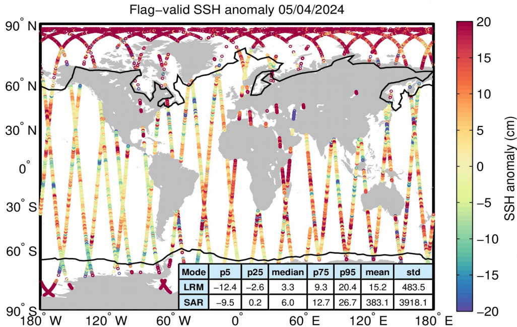
Figure 5. Geographical distribution of flag-valid 1-Hz SSH anomaly data over oceans and lakes for 05/04/2024. The statistical values shown in the table refer to the SSH anomaly in cm and are calculated separately for LRM and SAR regions. Measurements taken over polar polygons have been excluded from the computation of the statistical values. The black lines mark the outer limit of the Arctic and Antarctic polar polygons.
