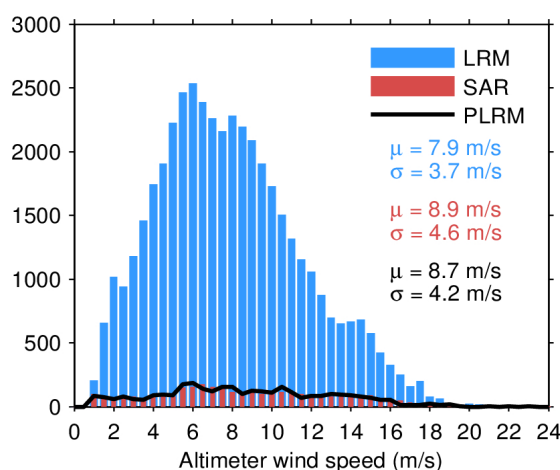
Figure 33. Histogram of flag-valid wind over oceans and lakes for LRM (blue), SAR (red), and PLRM (black) for 05/04/2024. The mean ( \mu ) and standard deviation ( \sigma ) are also shown. Note that values larger than 24 m/s are excluded from the histogram for the sake of readability but not from the computation of \mu and \sigma .
