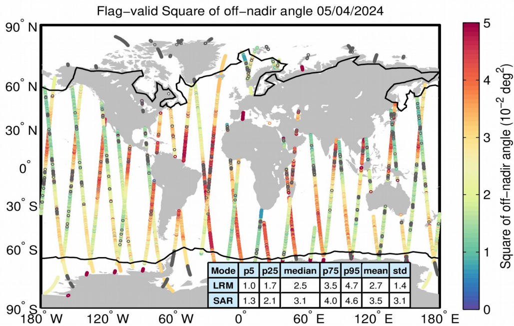
Figure 37. Geographical distribution of flag-valid mispointing data over oceans and lakes for 05/04/2024. The statistical values shown in the table refer to the mispointing in 10^{-2} \text{ deg}^2 and are calculated separately for LRM and SAR regions. Measurements taken over polar polygons have been excluded from the computation of the statistical values. The black lines mark the outer limit of the Arctic and Antarctic polar polygons. Gray circles denote negative values.
