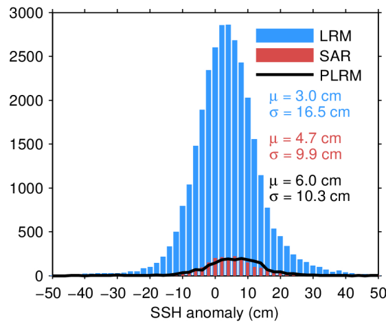
Figure 11. Histogram of science-valid SSH anomaly over oceans and lakes for LRM (blue), SAR (red), and PLRM (black) for 05/04/2024. The mean ( \mu ) and standard deviation ( \sigma ) are also shown. Note that values outside [-50\ 50] cm are excluded from the histogram for the sake of readability but not from the computation of \mu and \sigma .
