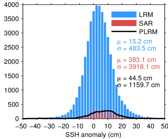
Figure 7. Histogram of flag-valid SSH anomaly over oceans and lakes for LRM (blue), SAR (red), and PLRM (black) for 05/04/2024. The mean ( \mu ) and standard deviation ( \sigma ) are also shown. Note that values outside [-50 50] cm are excluded from the histogram for the sake of readability but not from the computation of \mu and \sigma .
