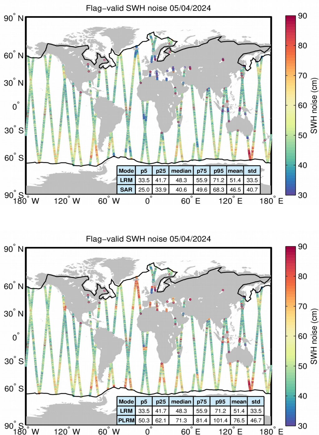
Figure 18. Geographical distribution of flag-valid 20-Hz SWH measurement noise over oceans and lakes for LRM/SAR (top) and LRM/PLRM (bottom) and for 05/04/2024. The statistical values shown in the table refer to the SWH noise and are calculated separately for LRM and SAR/PLRM regions. Measurements taken over polar polygons have been
