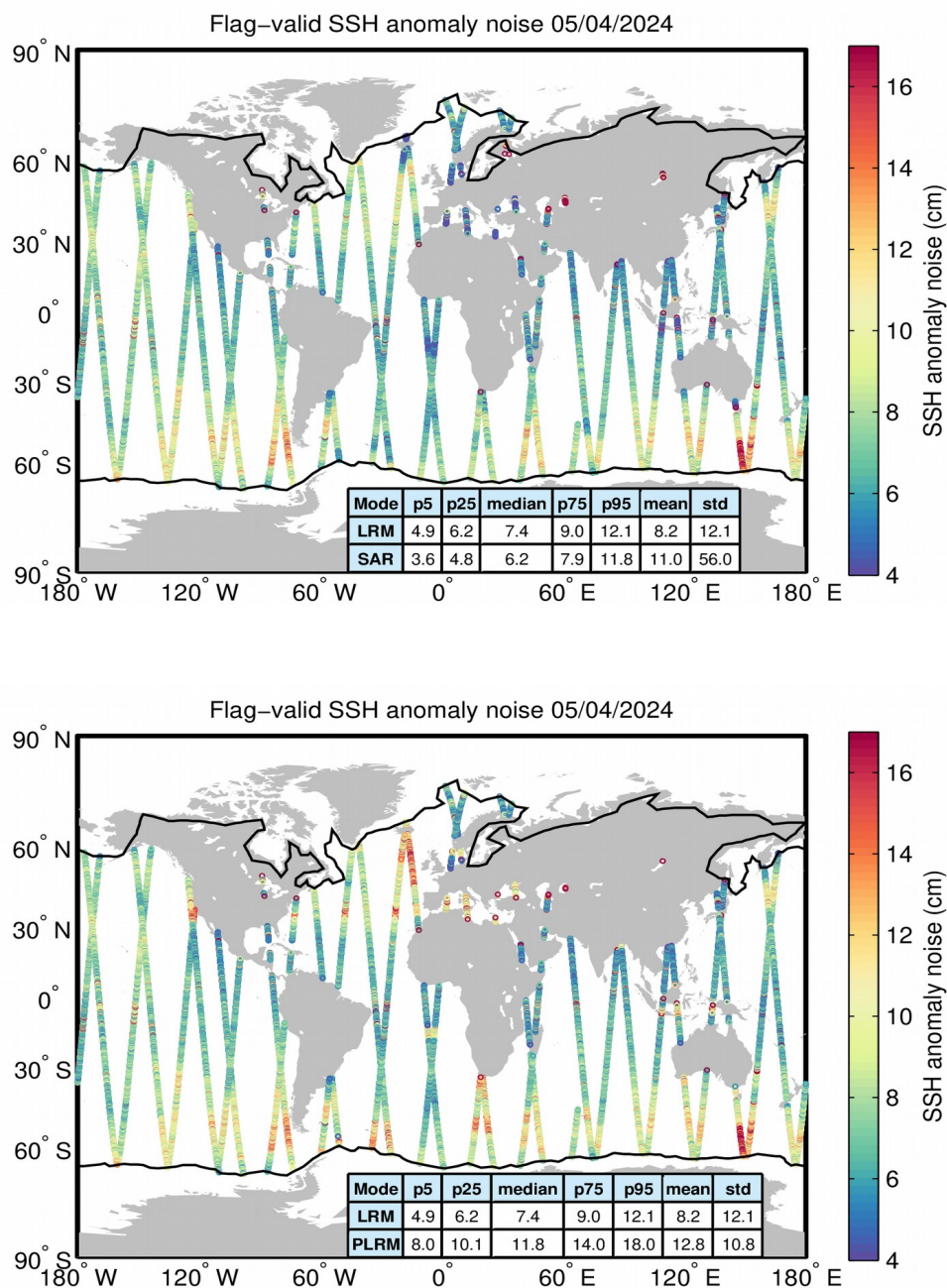
Figure 8. Geographical distribution of flag-valid 20-Hz SSH anomaly measurement noise over oceans and lakes for LRM/SAR (top) and LRM/PLRM (bottom) and for 05/04/2024. The statistical values shown in the tables refer to the SSH anomaly noise and are calculated separately for LRM and SAR/PLRM regions. Measurements taken over polar polygons have been excluded from the computation of the statistical values. The black lines mark the outer limit of the Arctic and Antarctic polar polygons.
