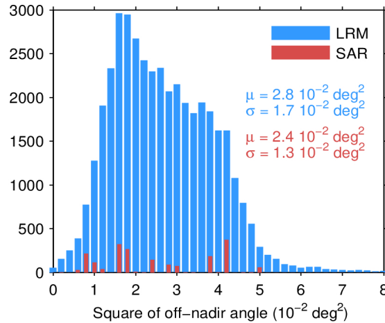
Figure 39. Histogram of flag-valid mispointing over oceans and lakes for LRM (blue) and SAR (red) for 04/04/2024. Only positive values have been considered. The mean ( \mu ) and standard deviation ( \sigma ) are also shown. Note that values larger than 8 \cdot 10^{-2} \text{ deg}^2 are excluded from the histogram for the sake of readability but not from the computation of \mu and \sigma .
