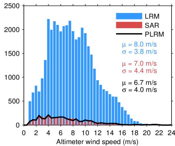
Figure 33. Histogram of flag-valid wind over oceans and lakes for LRM (blue), SAR (red), and PLRM (black) for 04/04/2024. The mean ( \mu ) and standard deviation ( \sigma ) are also shown. Note that values larger than 24 m/s are excluded from the histogram for the sake of readability but not from the computation of \mu and \sigma .
