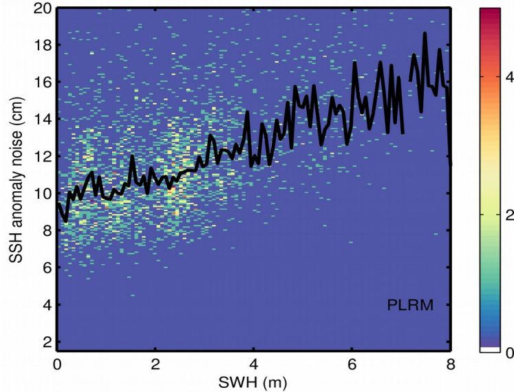
Figure 9. 2D histogram showing flag-valid SSH anomaly noise as a function of SWH for LRM (top), SAR (middle), and PLRM (bottom) for 04/04/2024. The black line denotes the median SSH anomaly noise as a function of SWH.
