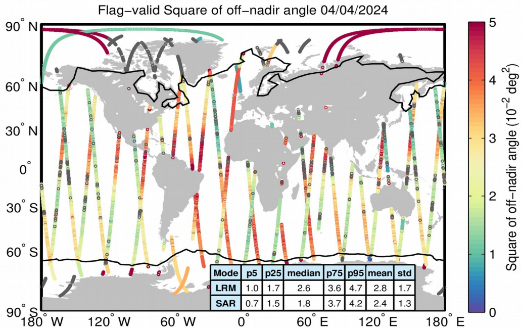
Figure 37. Geographical distribution of flag-valid mispointing data over oceans and lakes for 04/04/2024. The statistical values shown in the table refer to the mispointing in 10^{-2} \text{ deg}^2 and are calculated separately for LRM and SAR regions. Measurements taken over polar polygons have been excluded from the computation of the statistical values. The black lines mark the outer limit of the Arctic and Antarctic polar polygons. Gray circles denote negative values.
