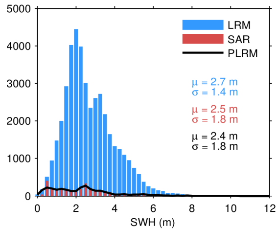
Figure 17. Histogram of flag-valid SWH over oceans and lakes for LRM (blue), SAR (red), and PLRM (black) for 04/04/2024. The mean ( \mu ) and standard deviation ( \sigma ) are also shown. Note that values larger than 12 m are excluded from the histogram for the sake of readability but not from the computation of \mu and \sigma .
