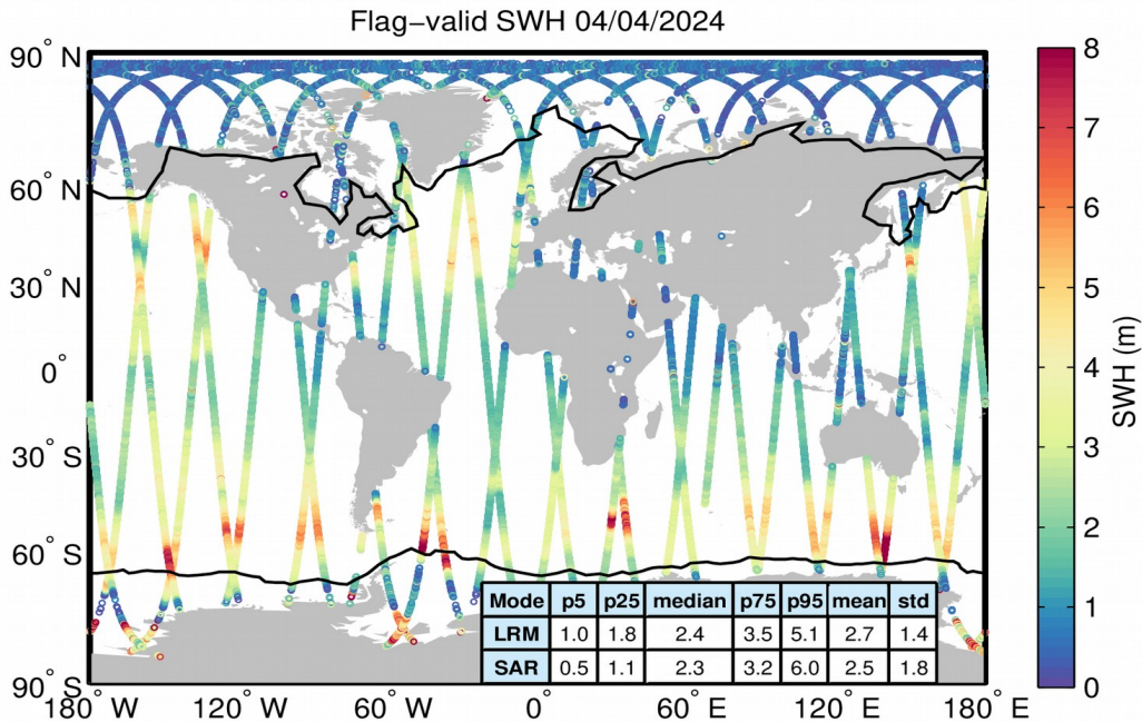
Figure 15. Geographical distribution of flag-valid SWH data over oceans and lakes for 04/04/2024. The statistical values shown in the table refer to the SWH in m and are calculated separately for LRM and SAR regions. Measurements taken over polar polygons have been excluded from the computation of the statistical values. The black lines mark the outer limit of the Arctic and Antarctic polar polygons.
