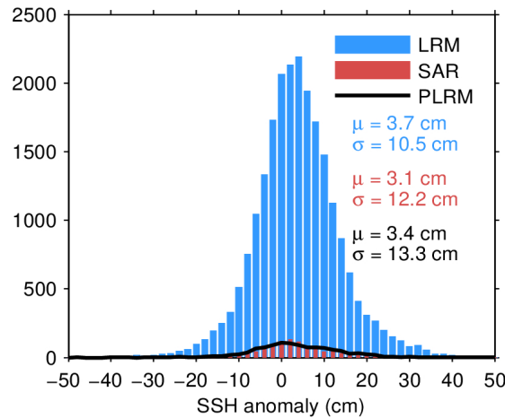
Figure 11. Histogram of science-valid SSH anomaly over oceans and lakes for LRM (blue), SAR (red), and PLRM (black) for 04/04/2024. The mean ( \mu ) and standard deviation ( \sigma ) are also shown. Note that values outside [-50\ 50] cm are excluded from the histogram for the sake of readability but not from the computation of \mu and \sigma .
