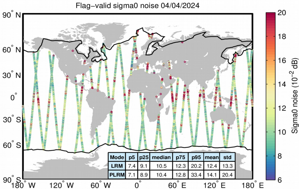
Figure 26. Geographical distribution of flag-valid 20-Hz sigma0 measurement noise over oceans and lakes for LRM/SAR (top) and LRM/PLRM (bottom) and for 04/04/2024. The statistical values shown in the table refer to the sigma0 noise and are calculated separately for LRM and SAR/PLRM regions. Measurements taken over polar polygons have been excluded from the computation of the statistical values. The black lines mark the outer limit of the Arctic and Antarctic polar polygons.
