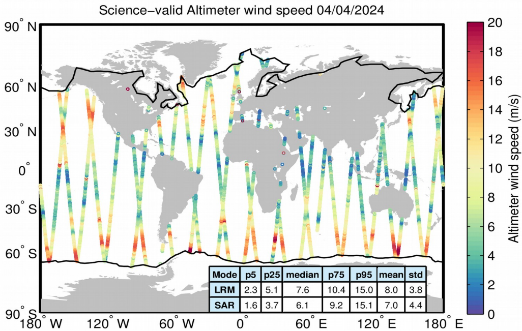
Figure 34. Geographical distribution of science-valid wind data over oceans and lakes for 04/04/2024. The statistical values shown in the table refer to the wind in m/s and are calculated separately for LRM and SAR regions. The black lines mark the outer limit of the Arctic and Antarctic polar polygons. Gray circles denote records that have been rejected based on the editing criteria described in Table 5.
