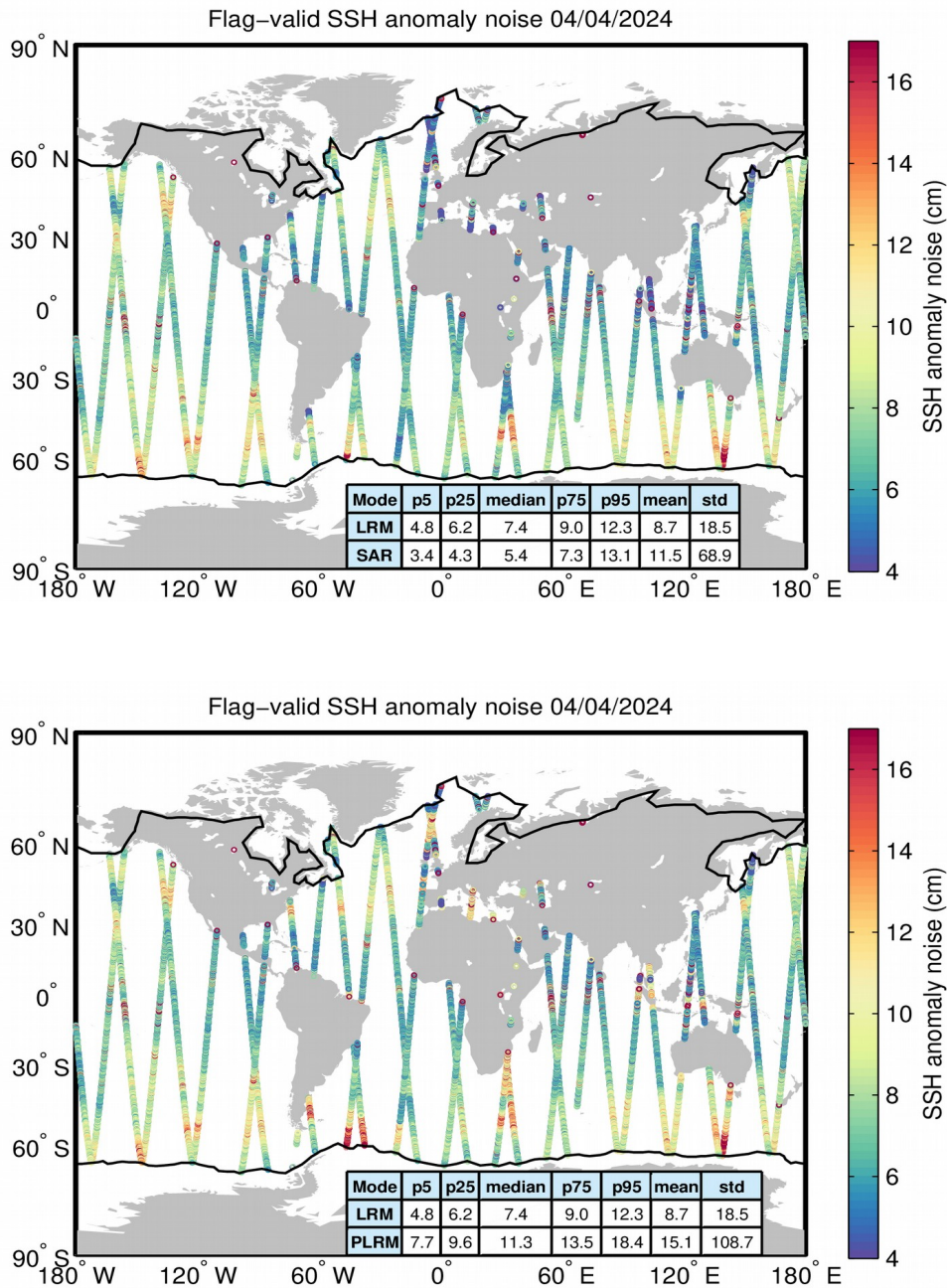
Figure 8. Geographical distribution of flag-valid 20-Hz SSH anomaly measurement noise over oceans and lakes for LRM/SAR (top) and LRM/PLRM (bottom) and for 04/04/2024. The statistical values shown in the tables refer to the SSH anomaly noise and are calculated separately for LRM and SAR/PLRM regions. Measurements taken over polar polygons have been excluded from the computation of the statistical values. The black lines mark the outer limit of the Arctic and Antarctic polar polygons.
