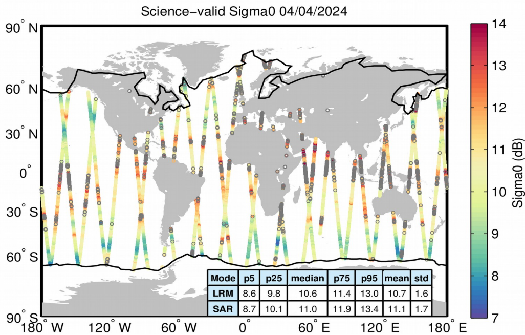
Figure 27. Geographical distribution of science-valid sigma0 data over oceans and lakes for 04/04/2024. The statistical values shown in the table refer to the sigma0 in dB and are calculated separately for LRM and SAR regions. The black lines mark the outer limit of the Arctic and Antarctic polar polygons. Gray circles denote records that have been rejected based on the editing criteria described in Table 4.
