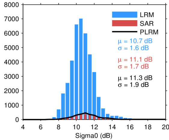
Figure 28. Histogram of science-valid sigma0 over oceans and lakes for LRM (blue), SAR (red), and PLRM (black) for 04/04/2024. The mean ( \mu ) and standard deviation ( \sigma ) are also shown. Note that values outside [4 20] dB are excluded from the histogram for the sake of readability but not from the computation of \mu and \sigma .
