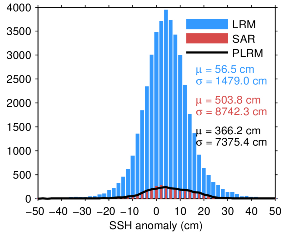
Figure 7. Histogram of flag-valid SSH anomaly over oceans and lakes for LRM (blue), SAR (red), and PLRM (black) for 04/04/2024. The mean ( \mu ) and standard deviation ( \sigma ) are also shown. Note that values outside [-50 50] cm are excluded from the histogram for the sake of readability but not from the computation of \mu and \sigma .
