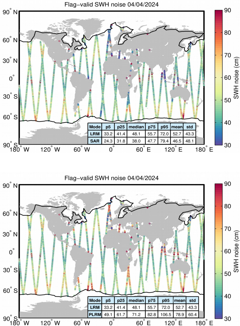
Figure 18. Geographical distribution of flag-valid 20-Hz SWH measurement noise over oceans and lakes for LRM/SAR (top) and LRM/PLRM (bottom) and for 04/04/2024. The statistical values shown in the table refer to the SWH noise and are calculated separately for LRM and SAR/PLRM regions. Measurements taken over polar polygons have been
