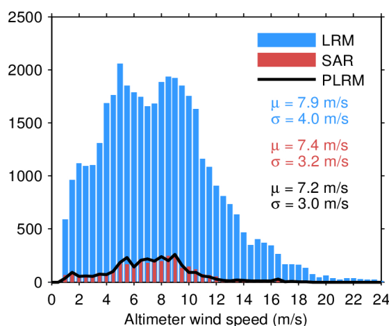
Figure 33. Histogram of flag-valid wind over oceans and lakes for LRM (blue), SAR (red), and PLRM (black) for 25/03/2024. The mean ( \mu ) and standard deviation ( \sigma ) are also shown. Note that values larger than 24 m/s are excluded from the histogram for the sake of readability but not from the computation of \mu and \sigma .
