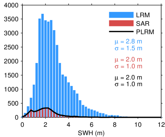
Figure 17. Histogram of flag-valid SWH over oceans and lakes for LRM (blue), SAR (red), and PLRM (black) for 25/03/2024. The mean ( \mu ) and standard deviation ( \sigma ) are also shown. Note that values larger than 12 m are excluded from the histogram for the sake of readability but not from the computation of \mu and \sigma .
