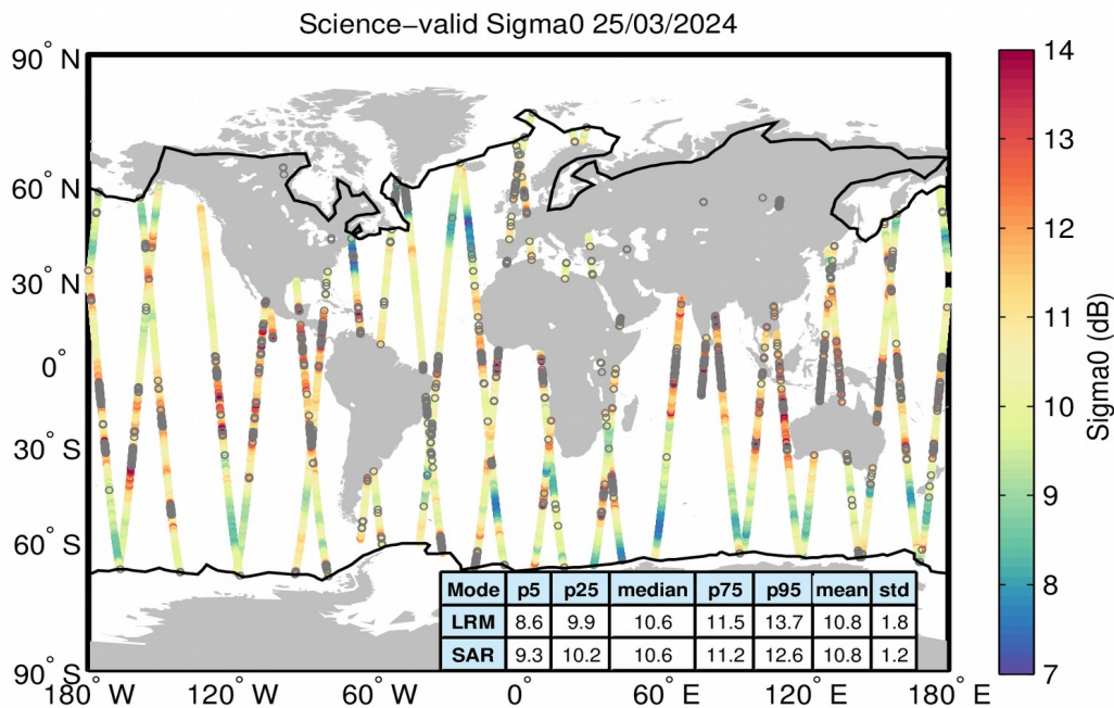
Figure 27. Geographical distribution of science-valid sigma0 data over oceans and lakes for 25/03/2024. The statistical values shown in the table refer to the sigma0 in dB and are calculated separately for LRM and SAR regions. The black lines mark the outer limit of the Arctic and Antarctic polar polygons. Gray circles denote records that have been rejected based on the editing criteria described in Table 4.
