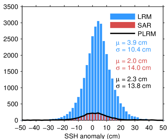
Figure 11. Histogram of science-valid SSH anomaly over oceans and lakes for LRM (blue), SAR (red), and PLRM (black) for 25/03/2024. The mean ( \mu ) and standard deviation ( \sigma ) are also shown. Note that values outside [-50\ 50] cm are excluded from the histogram for the sake of readability but not from the computation of \mu and \sigma .
