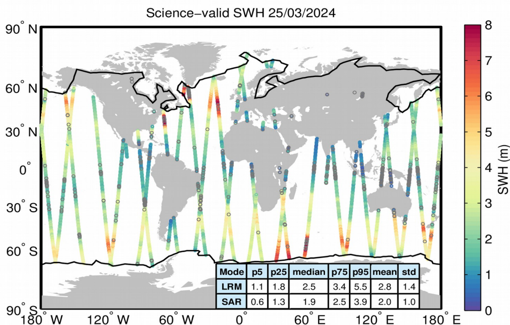
Figure 19. Geographical distribution of science-valid SWH data over oceans and lakes for 25/03/2024. The statistical values shown in the table refer to the SWH in m and are calculated separately for LRM and SAR regions. The black lines mark the outer limit of the Arctic and Antarctic polar polygons. Gray circles denote records that have been rejected based on the editing criteria described in Table 3.
