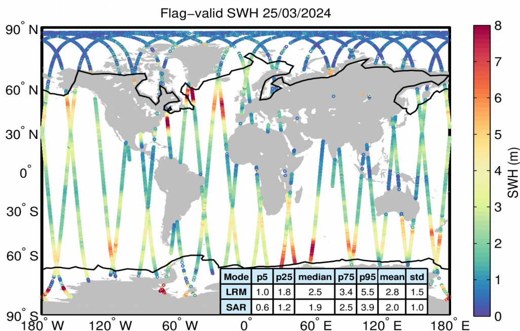
Figure 15. Geographical distribution of flag-valid SWH data over oceans and lakes for 25/03/2024. The statistical values shown in the table refer to the SWH in m and are calculated separately for LRM and SAR regions. Measurements taken over polar polygons have been excluded from the computation of the statistical values. The black lines mark the outer limit of the Arctic and Antarctic polar polygons.
