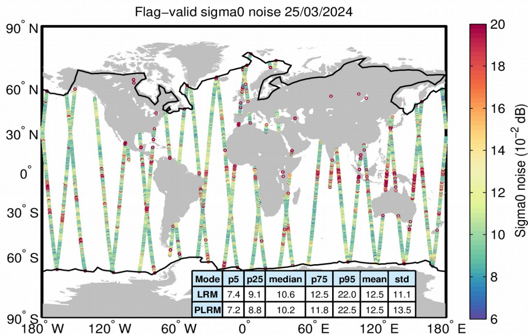
Figure 26. Geographical distribution of flag-valid 20-Hz sigma0 measurement noise over oceans and lakes for LRM/SAR (top) and LRM/PLRM (bottom) and for 25/03/2024. The statistical values shown in the table refer to the sigma0 noise and are calculated separately for LRM and SAR/PLRM regions. Measurements taken over polar polygons have been excluded from the computation of the statistical values. The black lines mark the outer limit of the Arctic and Antarctic polar polygons.
