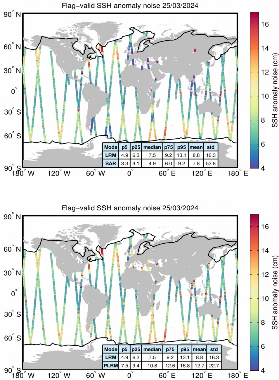
Figure 8. Geographical distribution of flag-valid 20-Hz SSH anomaly measurement noise over oceans and lakes for LRM/SAR (top) and LRM/PLRM (bottom) and for 25/03/2024. The statistical values shown in the tables refer to the SSH anomaly noise and are calculated separately for LRM and SAR/PLRM regions. Measurements taken over polar polygons have been excluded from the computation of the statistical values. The black lines mark the outer limit of the Arctic and Antarctic polar polygons.
