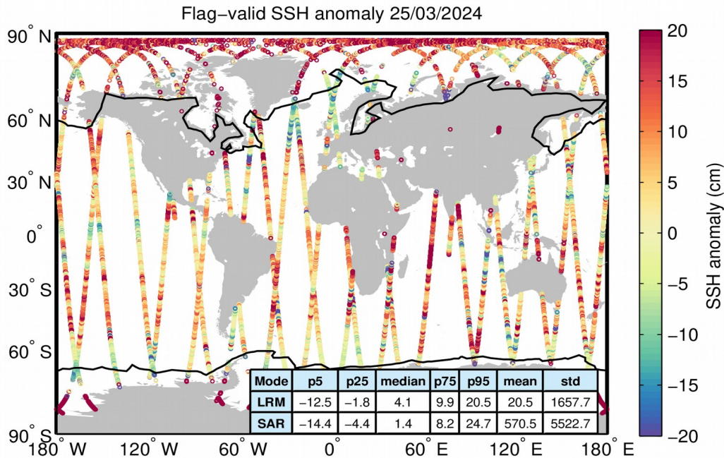
Figure 5. Geographical distribution of flag-valid 1-Hz SSH anomaly data over oceans and lakes for 25/03/2024. The statistical values shown in the table refer to the SSH anomaly in cm and are calculated separately for LRM and SAR regions. Measurements taken over polar polygons have been excluded from the computation of the statistical values. The black lines mark the outer limit of the Arctic and Antarctic polar polygons.
