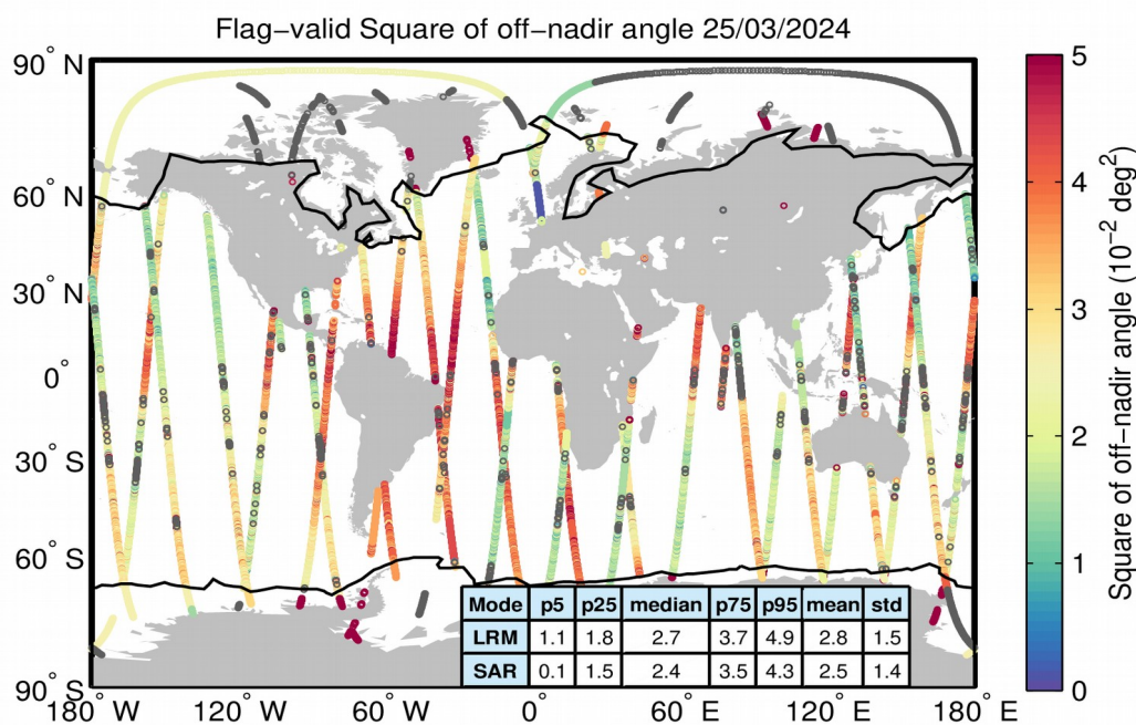
Figure 37. Geographical distribution of flag-valid mispointing data over oceans and lakes for 25/03/2024. The statistical values shown in the table refer to the mispointing in 10^{-2} \text{ deg}^2 and are calculated separately for LRM and SAR regions. Measurements taken over polar polygons have been excluded from the computation of the statistical values. The black lines mark the outer limit of the Arctic and Antarctic polar polygons. Gray circles denote negative values.
