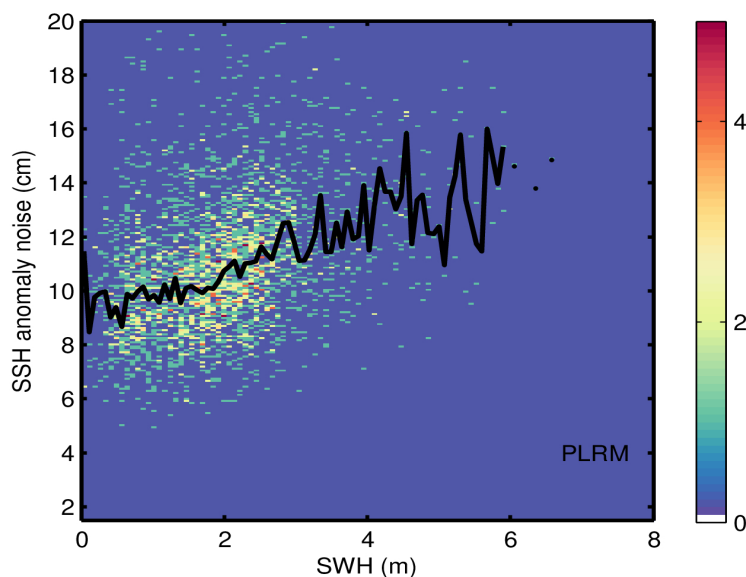
Figure 9. 2D histogram showing flag-valid SSH anomaly noise as a function of SWH for LRM (top), SAR (middle), and PLRM (bottom) for 25/03/2024. The black line denotes the median SSH anomaly noise as a function of SWH.
