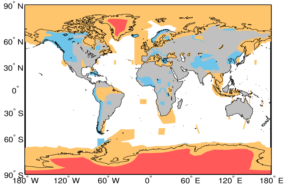
Figure A1. Extent of the regions defining the geographical mode mask for 25/03/2024. The regions where SAR, and SARIn are operated are denoted by the orange and blue polygons, respectively. LRM is operated over areas of the continental ice sheets (red polygons) and over oceans and land not covered by other modes.
