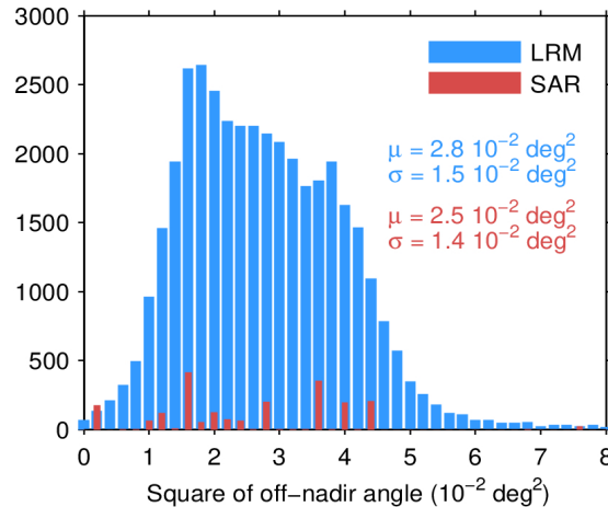
Figure 39. Histogram of flag-valid mispointing over oceans and lakes for LRM (blue) and SAR (red) for 25/03/2024. Only positive values have been considered. The mean ( \mu ) and standard deviation ( \sigma ) are also shown. Note that values larger than 8 \cdot 10^{-2} \text{ deg}^2 are excluded from the histogram for the sake of readability but not from the computation of \mu and \sigma .
