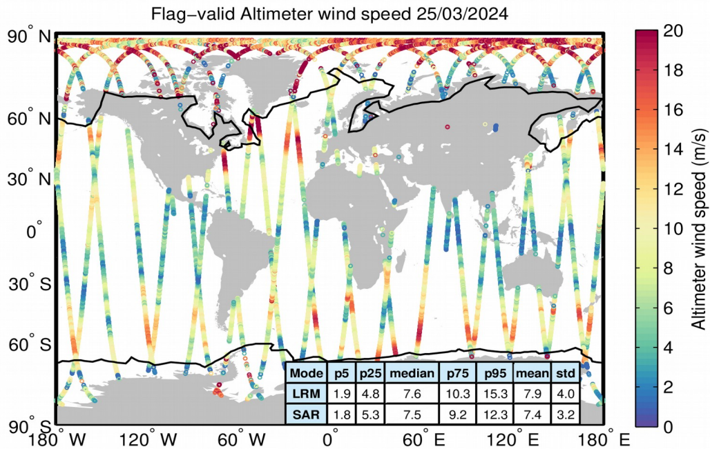
Figure 31. Geographical distribution of flag-valid wind data over oceans and lakes for 25/03/2024. The statistical values shown in the table refer to the wind in m/s and are calculated separately for LRM and SAR regions. Measurements taken over polar polygons have been excluded from the computation of the statistical values. The black lines mark the outer limit of the Arctic and Antarctic polar polygons.
