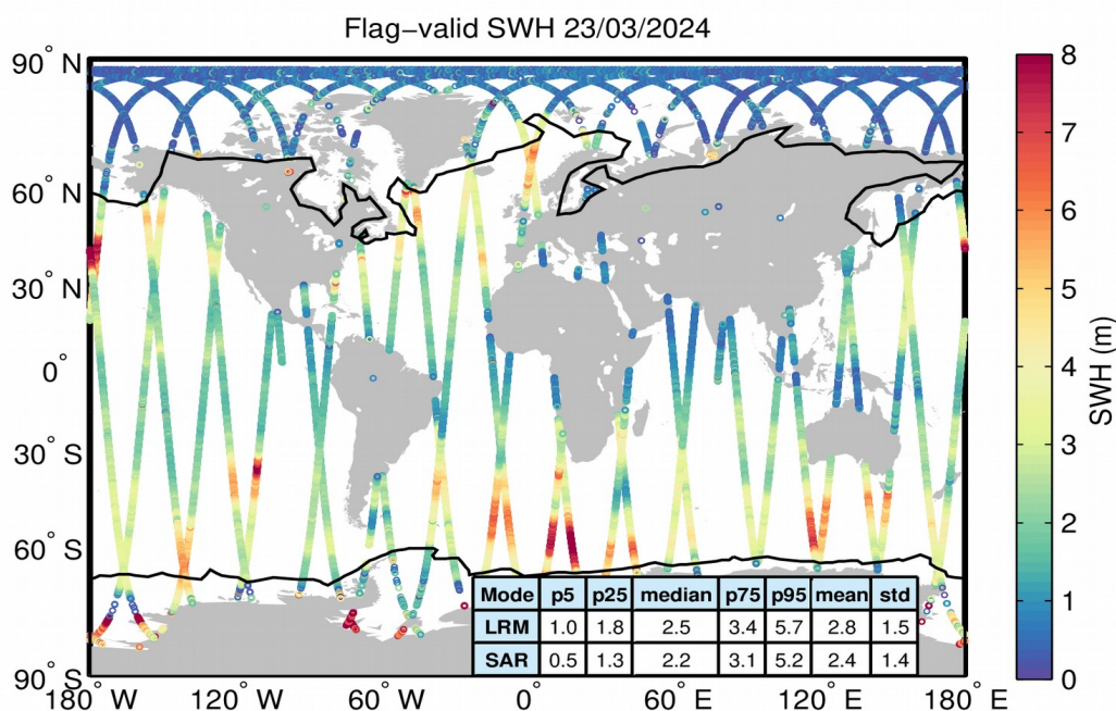
Figure 15. Geographical distribution of flag-valid SWH data over oceans and lakes for 23/03/2024. The statistical values shown in the table refer to the SWH in m and are calculated separately for LRM and SAR regions. Measurements taken over polar polygons have been excluded from the computation of the statistical values. The black lines mark the outer limit of the Arctic and Antarctic polar polygons.
