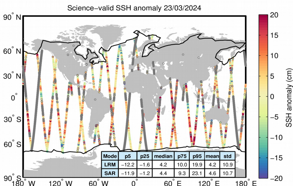
Figure 10. Geographical distribution of science-valid SSH anomaly data over oceans and lakes for 23/03/2024. The statistical values shown in the table refer to the SSH anomaly in cm and are calculated separately for LRM and SAR regions. The black lines mark the
