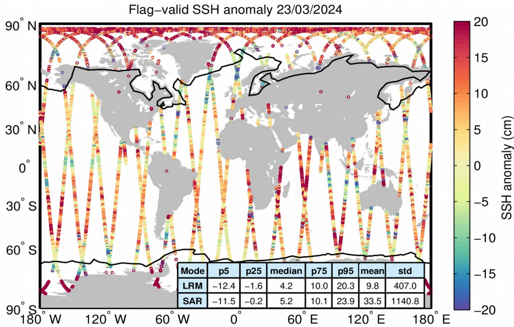
Figure 5. Geographical distribution of flag-valid 1-Hz SSH anomaly data over oceans and lakes for 23/03/2024. The statistical values shown in the table refer to the SSH anomaly in cm and are calculated separately for LRM and SAR regions. Measurements taken over polar polygons have been excluded from the computation of the statistical values. The black lines mark the outer limit of the Arctic and Antarctic polar polygons.
