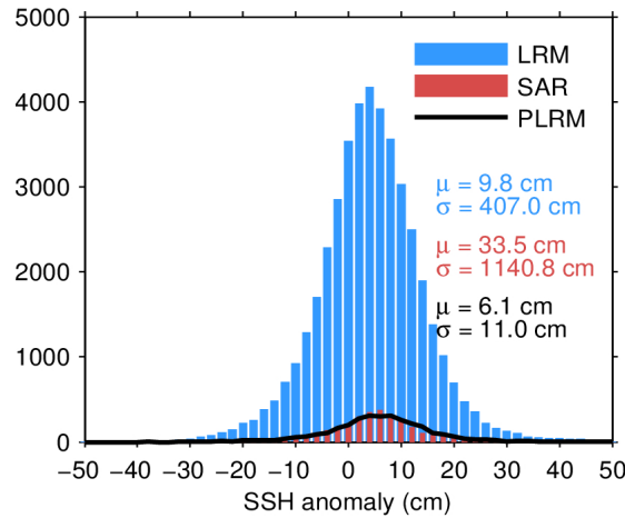
Figure 7. Histogram of flag-valid SSH anomaly over oceans and lakes for LRM (blue), SAR (red), and PLRM (black) for 23/03/2024. The mean ( \mu ) and standard deviation ( \sigma ) are also shown. Note that values outside [-50\ 50] cm are excluded from the histogram for the sake of readability but not from the computation of \mu and \sigma .
