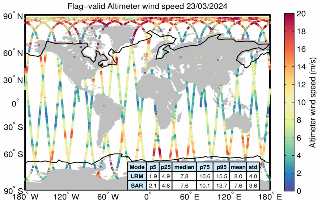
Figure 31. Geographical distribution of flag-valid wind data over oceans and lakes for 23/03/2024. The statistical values shown in the table refer to the wind in m/s and are calculated separately for LRM and SAR regions. Measurements taken over polar polygons have been excluded from the computation of the statistical values. The black lines mark the outer limit of the Arctic and Antarctic polar polygons.
