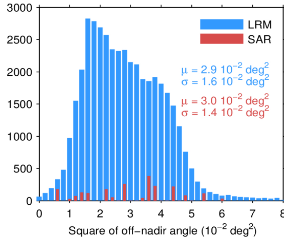
Figure 39. Histogram of flag-valid mispointing over oceans and lakes for LRM (blue) and SAR (red) for 23/03/2024. Only positive values have been considered. The mean ( \mu ) and standard deviation ( \sigma ) are also shown. Note that values larger than 8 \cdot 10^{-2} \text{ deg}^2 are excluded from the histogram for the sake of readability but not from the computation of \mu and \sigma .
