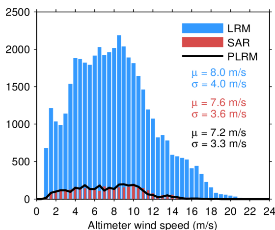
Figure 33. Histogram of flag-valid wind over oceans and lakes for LRM (blue), SAR (red), and PLRM (black) for 23/03/2024. The mean ( \mu ) and standard deviation ( \sigma ) are also shown. Note that values larger than 24 m/s are excluded from the histogram for the sake of readability but not from the computation of \mu and \sigma .
