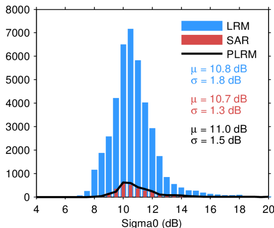
Figure 28. Histogram of science-valid sigma0 over oceans and lakes for LRM (blue), SAR (red), and PLRM (black) for 23/03/2024. The mean ( \mu ) and standard deviation ( \sigma ) are also shown. Note that values outside [4 20] dB are excluded from the histogram for the sake of readability but not from the computation of \mu and \sigma .
