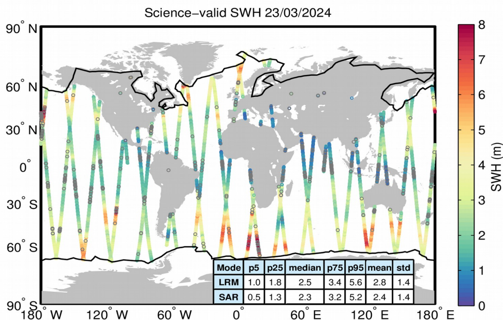
Figure 19. Geographical distribution of science-valid SWH data over oceans and lakes for 23/03/2024. The statistical values shown in the table refer to the SWH in m and are calculated separately for LRM and SAR regions. The black lines mark the outer limit of the Arctic and Antarctic polar polygons. Gray circles denote records that have been rejected based on the editing criteria described in Table 3.
