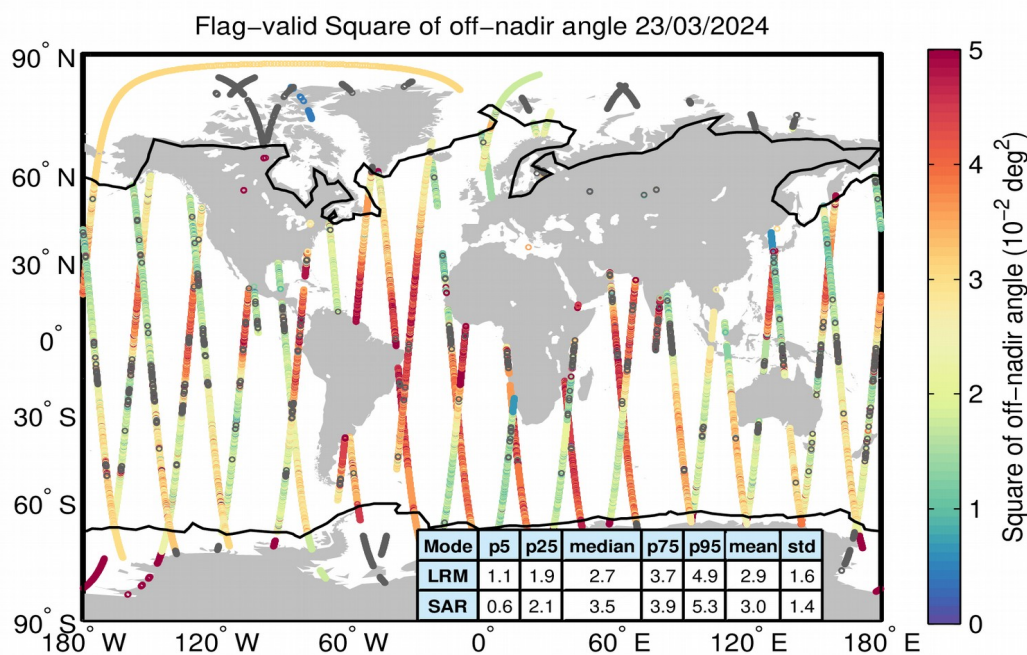
Figure 37. Geographical distribution of flag-valid mispointing data over oceans and lakes for 23/03/2024. The statistical values shown in the table refer to the mispointing in 10^{-2} \text{ deg}^2 and are calculated separately for LRM and SAR regions. Measurements taken over polar polygons have been excluded from the computation of the statistical values. The black lines mark the outer limit of the Arctic and Antarctic polar polygons. Gray circles denote negative values.
