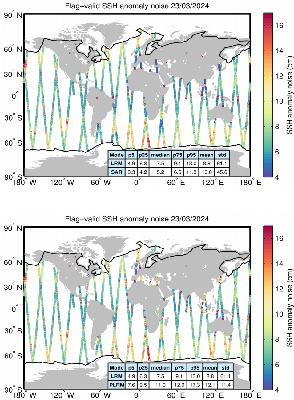
Figure 8. Geographical distribution of flag-valid 20-Hz SSH anomaly measurement noise over oceans and lakes for LRM/SAR (top) and LRM/PLRM (bottom) and for 23/03/2024. The statistical values shown in the tables refer to the SSH anomaly noise and are calculated separately for LRM and SAR/PLRM regions. Measurements taken over polar polygons have been excluded from the computation of the statistical values. The black lines mark the outer limit of the Arctic and Antarctic polar polygons.
