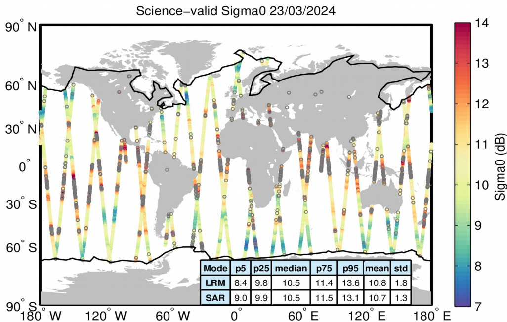
Figure 27. Geographical distribution of science-valid sigma0 data over oceans and lakes for 23/03/2024. The statistical values shown in the table refer to the sigma0 in dB and are calculated separately for LRM and SAR regions. The black lines mark the outer limit of the Arctic and Antarctic polar polygons. Gray circles denote records that have been rejected based on the editing criteria described in Table 4.
