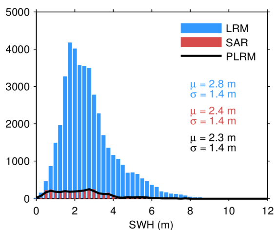
Figure 20. Histogram of science-valid SWH over oceans and lakes for LRM (blue), SAR (red), and PLRM (black) for 23/03/2024. The mean ( \mu ) and standard deviation ( \sigma ) are also
