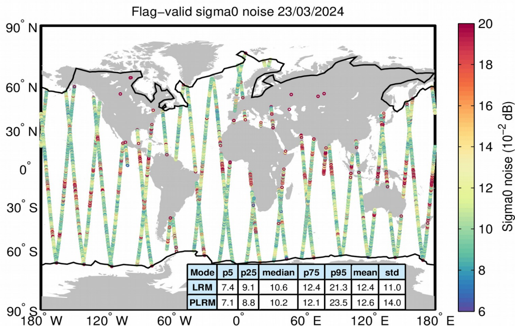
Figure 26. Geographical distribution of flag-valid 20-Hz sigma0 measurement noise over oceans and lakes for LRM/SAR (top) and LRM/PLRM (bottom) and for 23/03/2024. The statistical values shown in the table refer to the sigma0 noise and are calculated separately for LRM and SAR/PLRM regions. Measurements taken over polar polygons have been excluded from the computation of the statistical values. The black lines mark the outer limit of the Arctic and Antarctic polar polygons.
