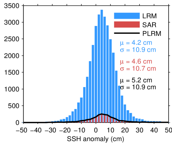
Figure 11. Histogram of science-valid SSH anomaly over oceans and lakes for LRM (blue), SAR (red), and PLRM (black) for 23/03/2024. The mean ( \mu ) and standard deviation ( \sigma ) are also shown. Note that values outside [-50\ 50] cm are excluded from the histogram for the sake of readability but not from the computation of \mu and \sigma .
