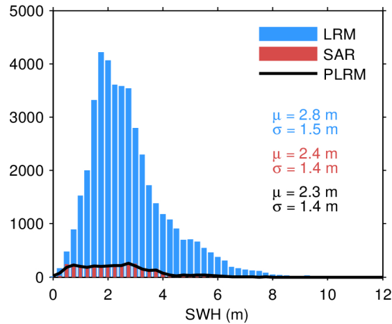
Figure 17. Histogram of flag-valid SWH over oceans and lakes for LRM (blue), SAR (red), and PLRM (black) for 23/03/2024. The mean ( \mu ) and standard deviation ( \sigma ) are also shown. Note that values larger than 12 m are excluded from the histogram for the sake of readability but not from the computation of \mu and \sigma .
