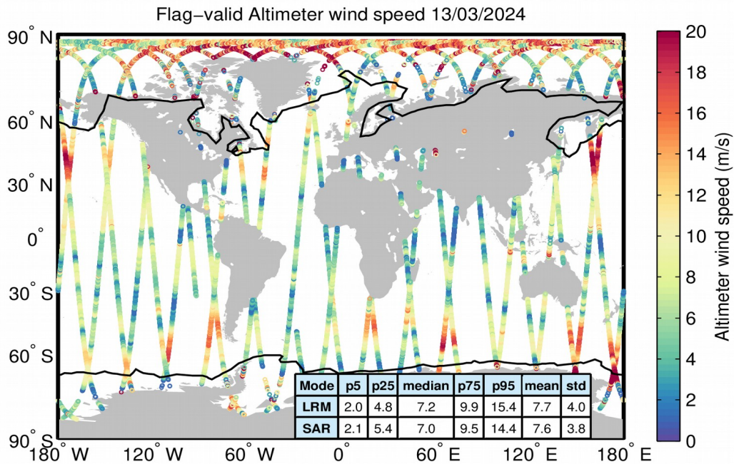
Figure 31. Geographical distribution of flag-valid wind data over oceans and lakes for 13/03/2024. The statistical values shown in the table refer to the wind in m/s and are calculated separately for LRM and SAR regions. Measurements taken over polar polygons have been excluded from the computation of the statistical values. The black lines mark the outer limit of the Arctic and Antarctic polar polygons.
