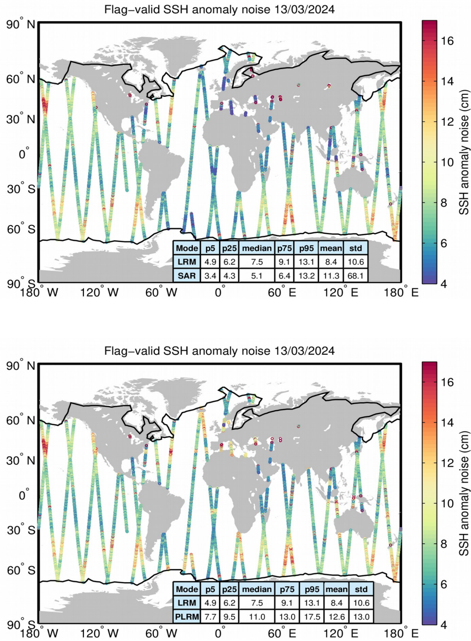
Figure 8. Geographical distribution of flag-valid 20-Hz SSH anomaly measurement noise over oceans and lakes for LRM/SAR (top) and LRM/PLRM (bottom) and for 13/03/2024. The statistical values shown in the tables refer to the SSH anomaly noise and are calculated separately for LRM and SAR/PLRM regions. Measurements taken over polar polygons have been excluded from the computation of the statistical values. The black lines mark the outer limit of the Arctic and Antarctic polar polygons.
