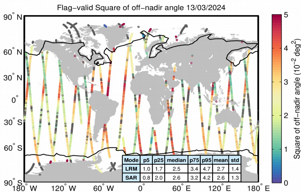
Figure 37. Geographical distribution of flag-valid mispointing data over oceans and lakes for 13/03/2024. The statistical values shown in the table refer to the mispointing in 10^{-2} \text{ deg}^2 and are calculated separately for LRM and SAR regions. Measurements taken over polar polygons have been excluded from the computation of the statistical values. The black lines mark the outer limit of the Arctic and Antarctic polar polygons. Gray circles denote negative values.
