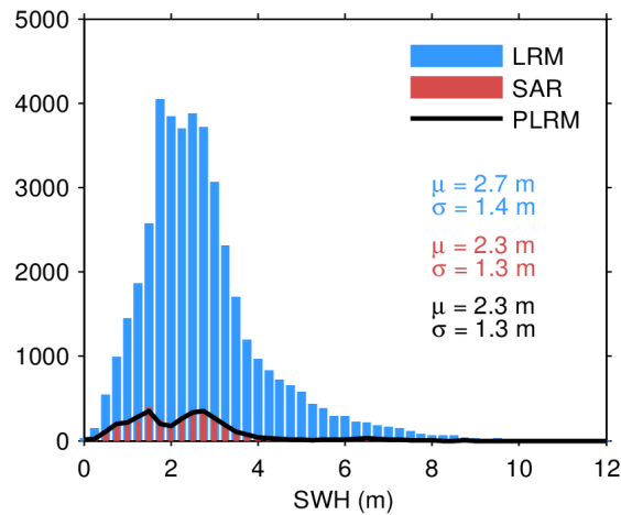
Figure 17. Histogram of flag-valid SWH over oceans and lakes for LRM (blue), SAR (red), and PLRM (black) for 13/03/2024. The mean ( \mu ) and standard deviation ( \sigma ) are also shown. Note that values larger than 12 m are excluded from the histogram for the sake of readability but not from the computation of \mu and \sigma .
