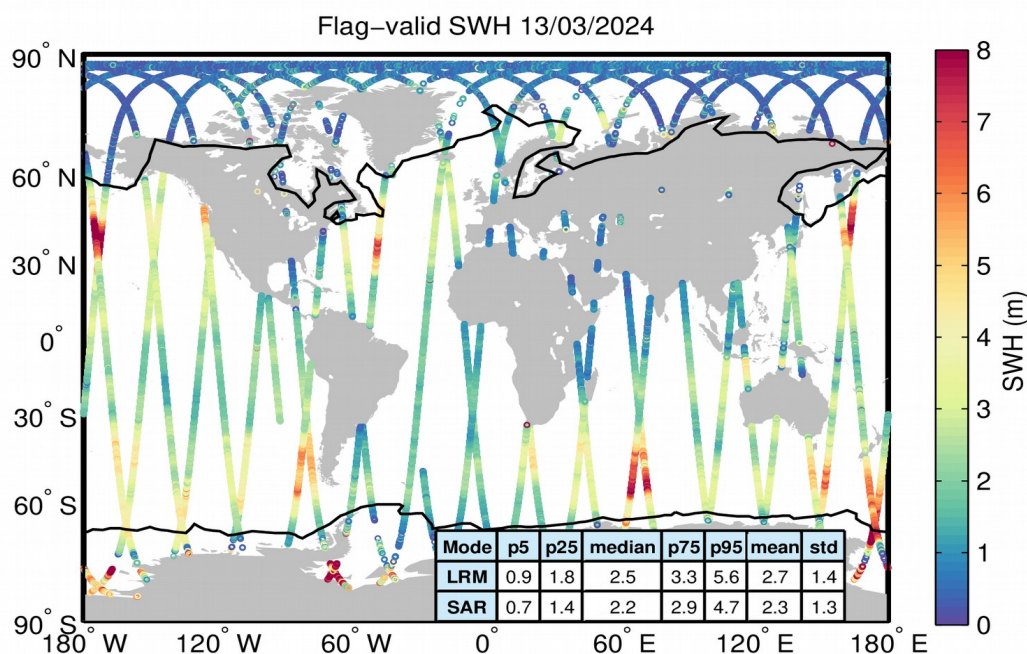
Figure 15. Geographical distribution of flag-valid SWH data over oceans and lakes for 13/03/2024. The statistical values shown in the table refer to the SWH in m and are calculated separately for LRM and SAR regions. Measurements taken over polar polygons have been excluded from the computation of the statistical values. The black lines mark the outer limit of the Arctic and Antarctic polar polygons.
