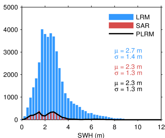
Figure 20. Histogram of science-valid SWH over oceans and lakes for LRM (blue), SAR (red), and PLRM (black) for 13/03/2024. The mean ( \mu ) and standard deviation ( \sigma ) are also
