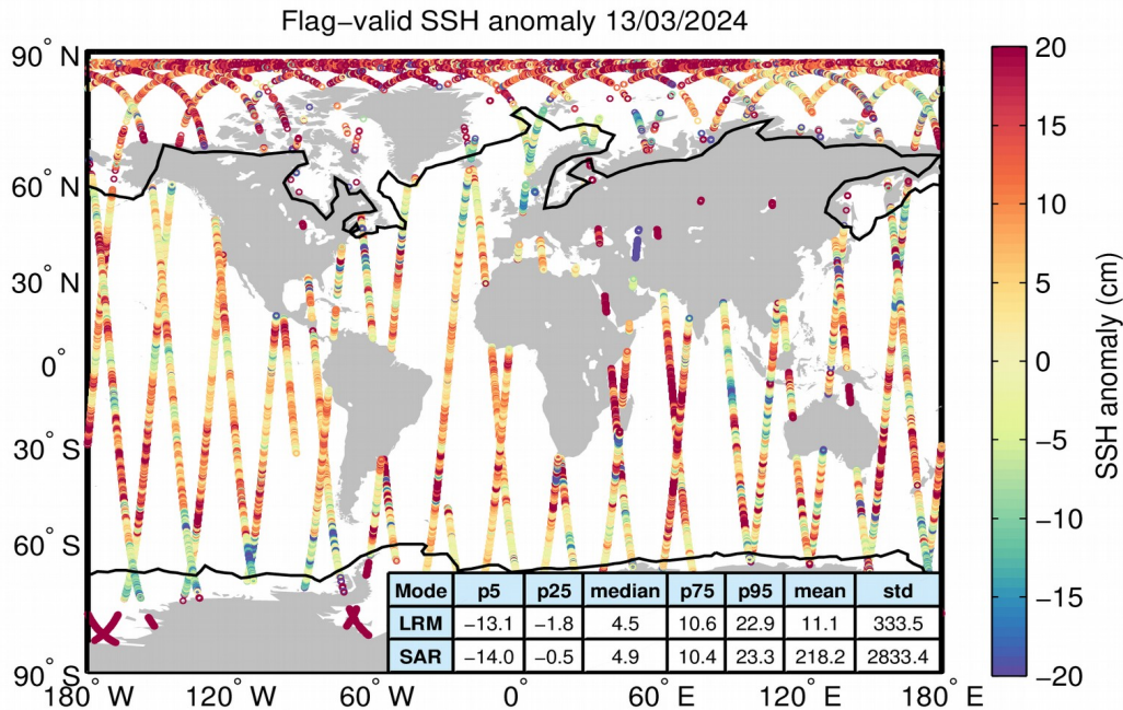
Figure 5. Geographical distribution of flag-valid 1-Hz SSH anomaly data over oceans and lakes for 13/03/2024. The statistical values shown in the table refer to the SSH anomaly in cm and are calculated separately for LRM and SAR regions. Measurements taken over polar polygons have been excluded from the computation of the statistical values. The black lines mark the outer limit of the Arctic and Antarctic polar polygons.
