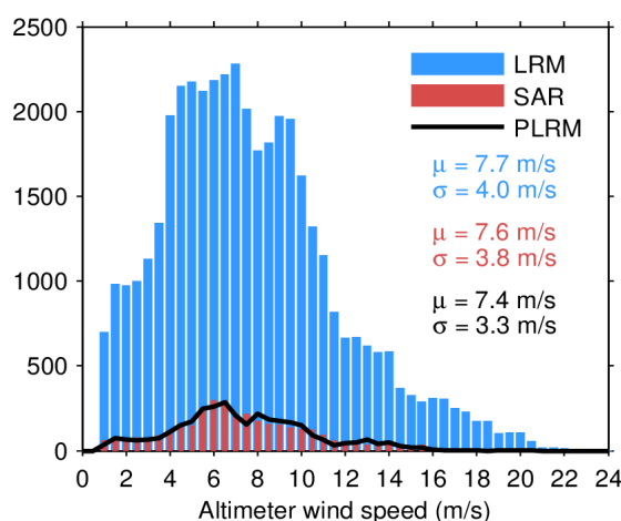
Figure 33. Histogram of flag-valid wind over oceans and lakes for LRM (blue), SAR (red), and PLRM (black) for 13/03/2024. The mean ( \mu ) and standard deviation ( \sigma ) are also shown. Note that values larger than 24 m/s are excluded from the histogram for the sake of readability but not from the computation of \mu and \sigma .
