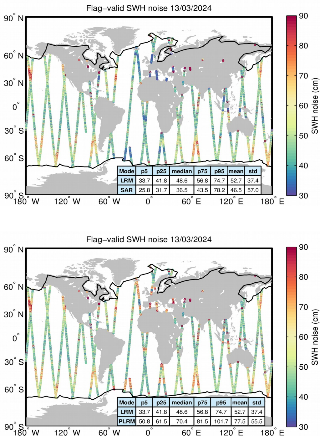
Figure 18. Geographical distribution of flag-valid 20-Hz SWH measurement noise over oceans and lakes for LRM/SAR (top) and LRM/PLRM (bottom) and for 13/03/2024. The statistical values shown in the table refer to the SWH noise and are calculated separately for LRM and SAR/PLRM regions. Measurements taken over polar polygons have been
