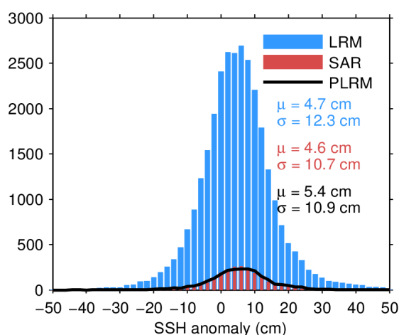
Figure 11. Histogram of science-valid SSH anomaly over oceans and lakes for LRM (blue), SAR (red), and PLRM (black) for 13/03/2024. The mean ( \mu ) and standard deviation ( \sigma ) are also shown. Note that values outside [-50, 50] cm are excluded from the histogram for the sake of readability but not from the computation of \mu and \sigma .
