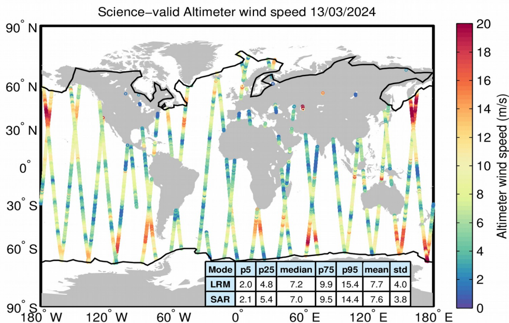
Figure 34. Geographical distribution of science-valid wind data over oceans and lakes for 13/03/2024. The statistical values shown in the table refer to the wind in m/s and are calculated separately for LRM and SAR regions. The black lines mark the outer limit of the Arctic and Antarctic polar polygons. Gray circles denote records that have been rejected based on the editing criteria described in Table 5.
