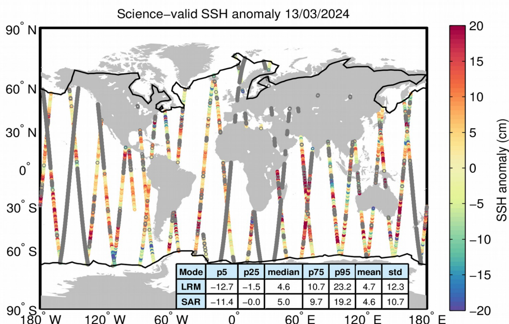
Figure 10. Geographical distribution of science-valid SSH anomaly data over oceans and lakes for 13/03/2024. The statistical values shown in the table refer to the SSH anomaly in cm and are calculated separately for LRM and SAR regions. The black lines mark the
