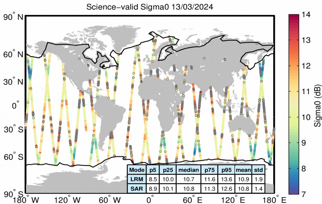
Figure 27. Geographical distribution of science-valid sigma0 data over oceans and lakes for 13/03/2024. The statistical values shown in the table refer to the sigma0 in dB and are calculated separately for LRM and SAR regions. The black lines mark the outer limit of the Arctic and Antarctic polar polygons. Gray circles denote records that have been rejected based on the editing criteria described in Table 4.
