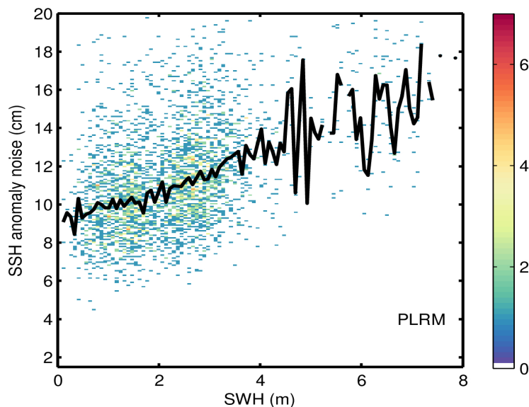
Figure 9. 2D histogram showing flag-valid SSH anomaly noise as a function of SWH for LRM (top), SAR (middle), and PLRM (bottom) for 13/03/2024. The black line denotes the median SSH anomaly noise as a function of SWH.
