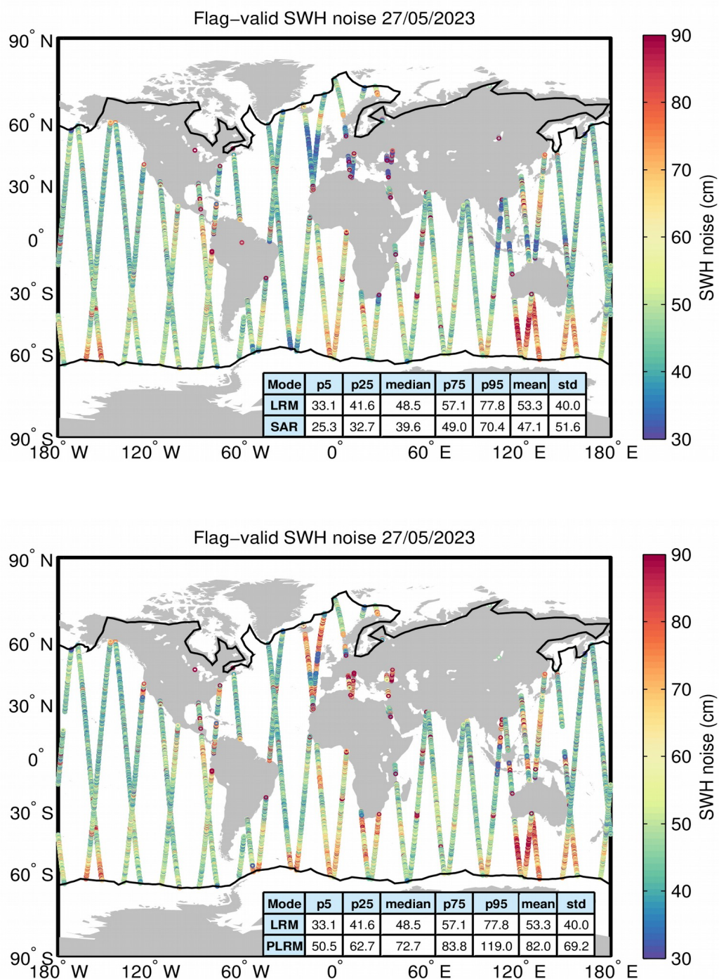
Figure 18. Geographical distribution of flag-valid 20-Hz SWH measurement noise over oceans and lakes for LRM/SAR (top) and LRM/PLRM (bottom) and for 27/05/2023. The statistical values shown in the table refer to the SWH noise and are calculated separately for LRM and SAR/PLRM regions. Measurements taken over polar polygons have been
