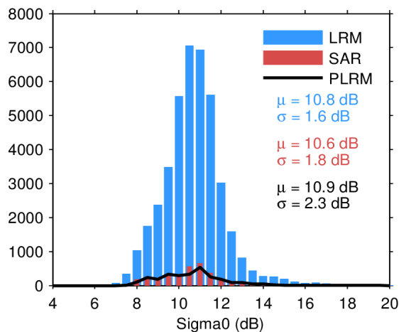
Figure 28. Histogram of science-valid sigma0 over oceans and lakes for LRM (blue), SAR (red), and PLRM (black) for 27/05/2023. The mean ( \mu ) and standard deviation ( \sigma ) are also shown. Note that values outside [4 20] dB are excluded from the histogram for the sake of readability but not from the computation of \mu and \sigma .
