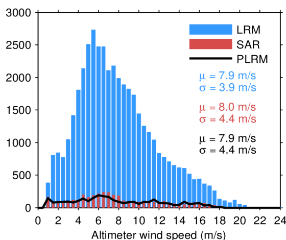
Figure 33. Histogram of flag-valid wind over oceans and lakes for LRM (blue), SAR (red), and PLRM (black) for 27/05/2023. The mean ( \mu ) and standard deviation ( \sigma ) are also shown. Note that values larger than 24 m/s are excluded from the histogram for the sake of readability but not from the computation of \mu and \sigma .
