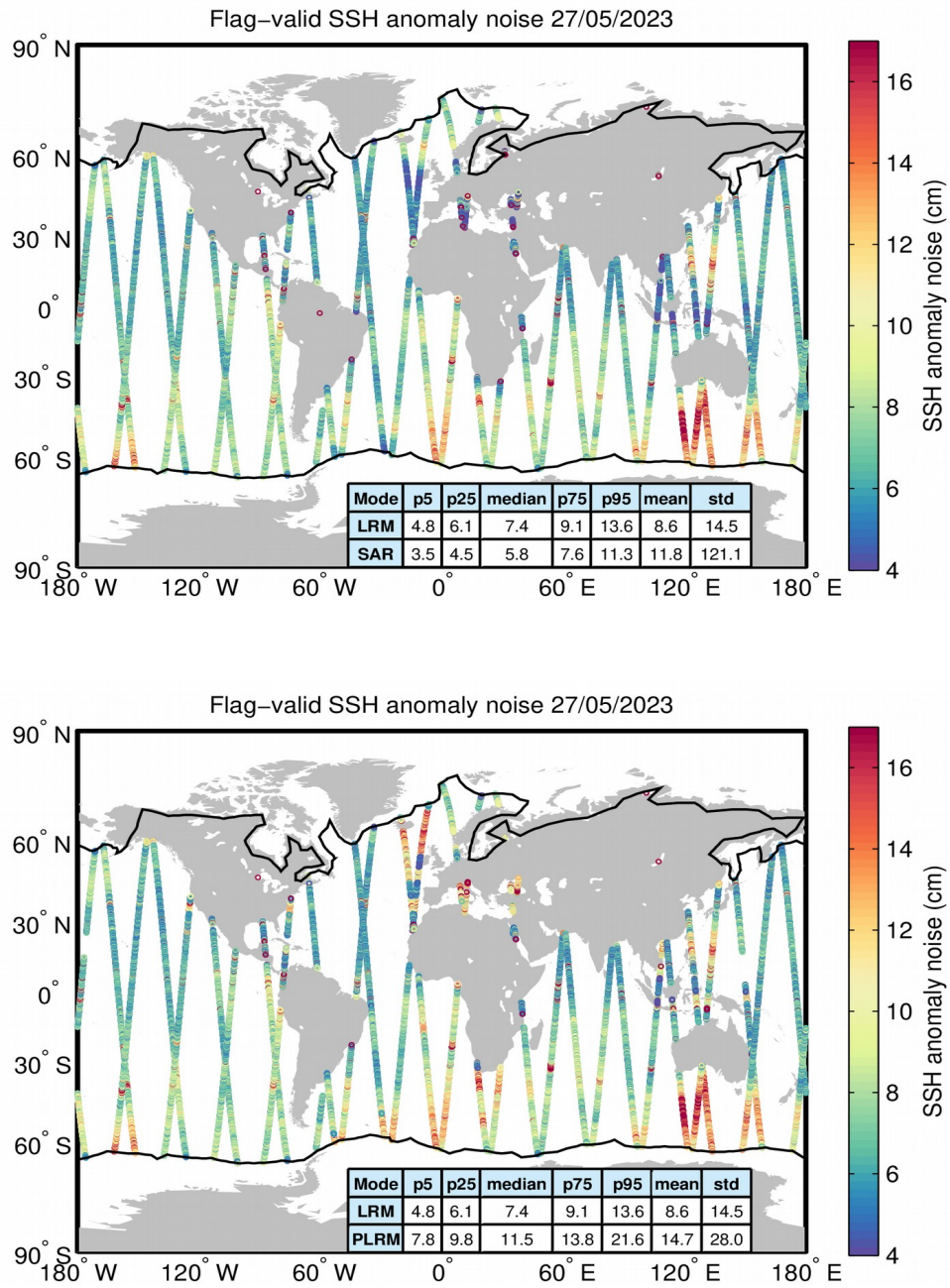
Figure 8. Geographical distribution of flag-valid 20-Hz SSH anomaly measurement noise over oceans and lakes for LRM/SAR (top) and LRM/PLRM (bottom) and for 27/05/2023. The statistical values shown in the tables refer to the SSH anomaly noise and are calculated separately for LRM and SAR/PLRM regions. Measurements taken over polar polygons have been excluded from the computation of the statistical values. The black lines mark the outer limit of the Arctic and Antarctic polar polygons.
