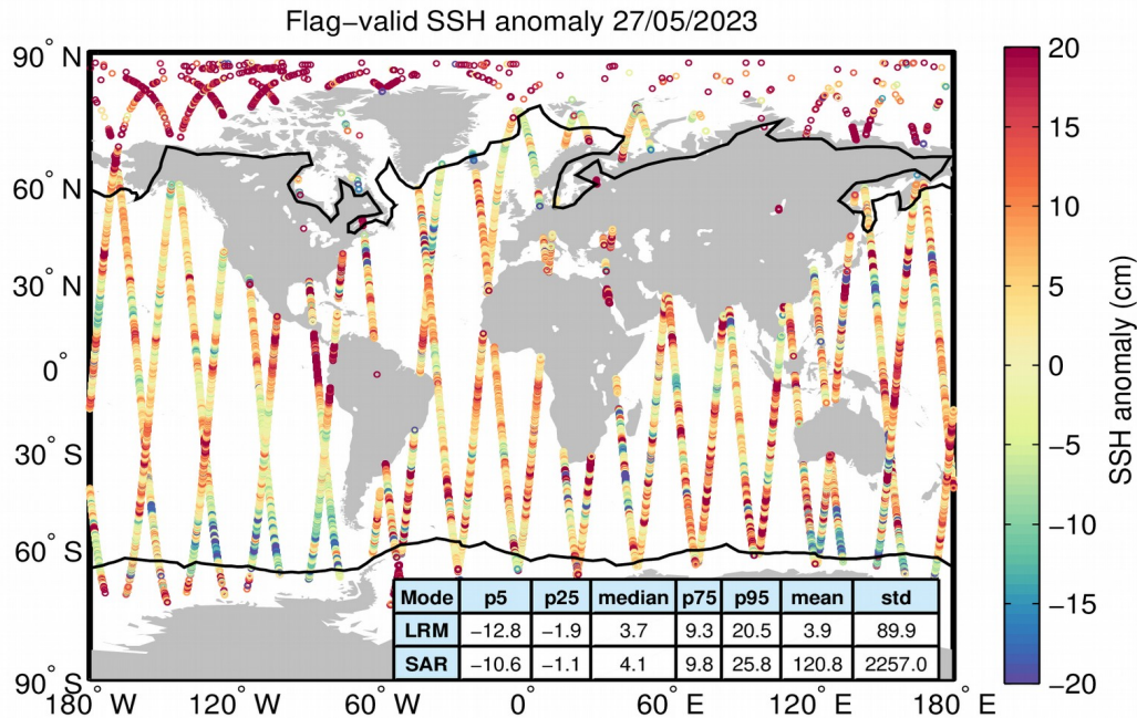
Figure 5. Geographical distribution of flag-valid 1-Hz SSH anomaly data over oceans and lakes for 27/05/2023. The statistical values shown in the table refer to the SSH anomaly in cm and are calculated separately for LRM and SAR regions. Measurements taken over polar polygons have been excluded from the computation of the statistical values. The black lines mark the outer limit of the Arctic and Antarctic polar polygons.
