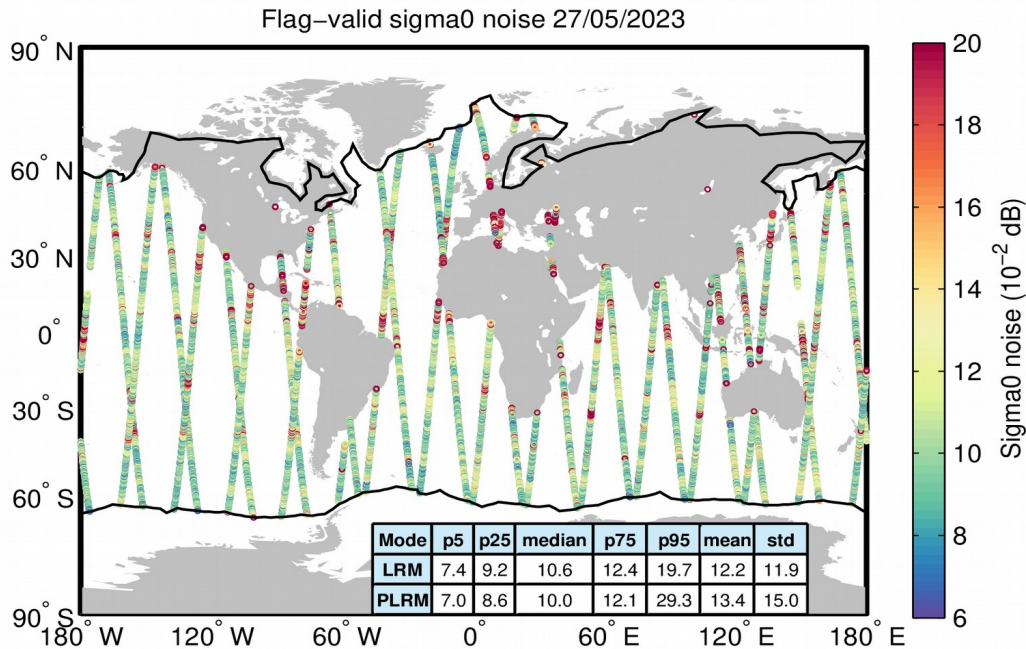
Figure 26. Geographical distribution of flag-valid 20-Hz sigma0 measurement noise over oceans and lakes for LRM/SAR (top) and LRM/PLRM (bottom) and for 27/05/2023. The statistical values shown in the table refer to the sigma0 noise and are calculated separately for LRM and SAR/PLRM regions. Measurements taken over polar polygons have been excluded from the computation of the statistical values. The black lines mark the outer limit of the Arctic and Antarctic polar polygons.
