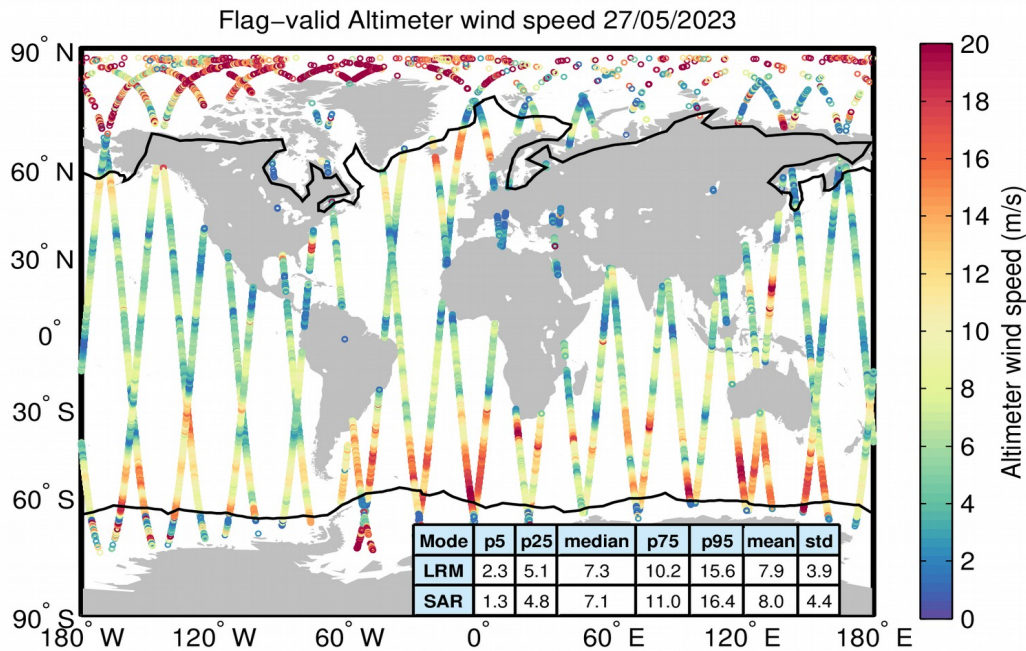
Figure 31. Geographical distribution of flag-valid wind data over oceans and lakes for 27/05/2023. The statistical values shown in the table refer to the wind in m/s and are calculated separately for LRM and SAR regions. Measurements taken over polar polygons have been excluded from the computation of the statistical values. The black lines mark the outer limit of the Arctic and Antarctic polar polygons.
