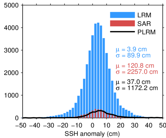
Figure 7. Histogram of flag-valid SSH anomaly over oceans and lakes for LRM (blue), SAR (red), and PLRM (black) for 27/05/2023. The mean ( \mu ) and standard deviation ( \sigma ) are also shown. Note that values outside [-50 50] cm are excluded from the histogram for the sake of readability but not from the computation of \mu and \sigma .
