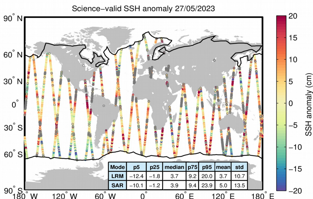
Figure 10. Geographical distribution of science-valid SSH anomaly data over oceans and lakes for 27/05/2023. The statistical values shown in the table refer to the SSH anomaly in cm and are calculated separately for LRM and SAR regions. The black lines mark the
