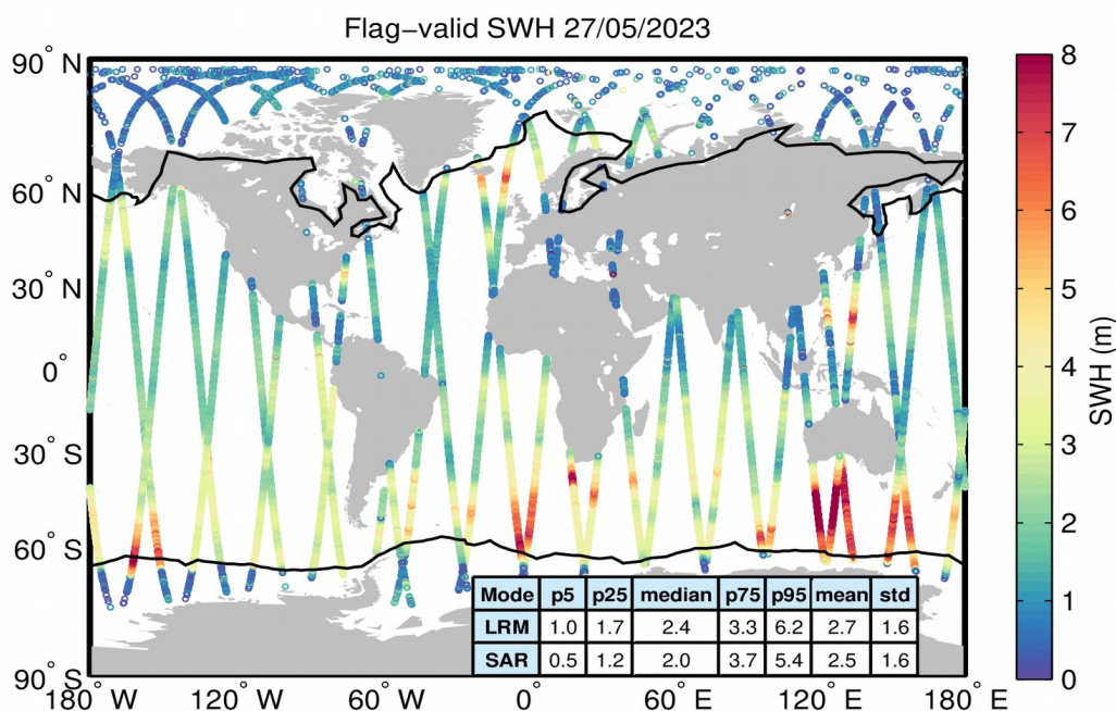
Figure 15. Geographical distribution of flag-valid SWH data over oceans and lakes for 27/05/2023. The statistical values shown in the table refer to the SWH in m and are calculated separately for LRM and SAR regions. Measurements taken over polar polygons have been excluded from the computation of the statistical values. The black lines mark the outer limit of the Arctic and Antarctic polar polygons.
