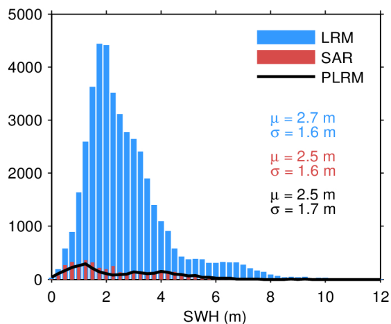
Figure 17. Histogram of flag-valid SWH over oceans and lakes for LRM (blue), SAR (red), and PLRM (black) for 27/05/2023. The mean ( \mu ) and standard deviation ( \sigma ) are also shown. Note that values larger than 12 m are excluded from the histogram for the sake of readability but not from the computation of \mu and \sigma .
