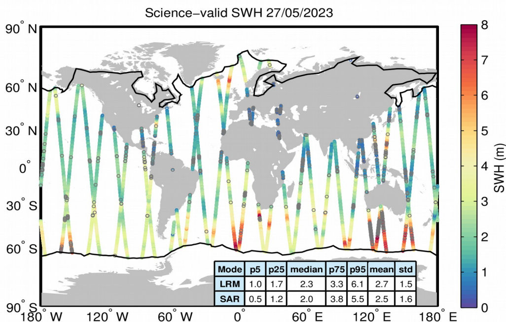
Figure 19. Geographical distribution of science-valid SWH data over oceans and lakes for 27/05/2023. The statistical values shown in the table refer to the SWH in m and are calculated separately for LRM and SAR regions. The black lines mark the outer limit of the Arctic and Antarctic polar polygons. Gray circles denote records that have been rejected based on the editing criteria described in Table 3.
