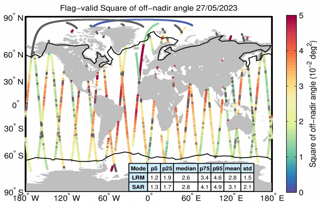
Figure 37. Geographical distribution of flag-valid mispointing data over oceans and lakes for 27/05/2023. The statistical values shown in the table refer to the mispointing in 10^{-2} \text{ deg}^2 and are calculated separately for LRM and SAR regions. Measurements taken over polar polygons have been excluded from the computation of the statistical values. The black lines mark the outer limit of the Arctic and Antarctic polar polygons. Gray circles denote negative values.
