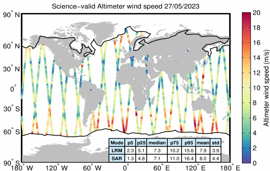
Figure 34. Geographical distribution of science-valid wind data over oceans and lakes for 27/05/2023. The statistical values shown in the table refer to the wind in m/s and are calculated separately for LRM and SAR regions. The black lines mark the outer limit of the Arctic and Antarctic polar polygons. Gray circles denote records that have been rejected based on the editing criteria described in Table 5.
