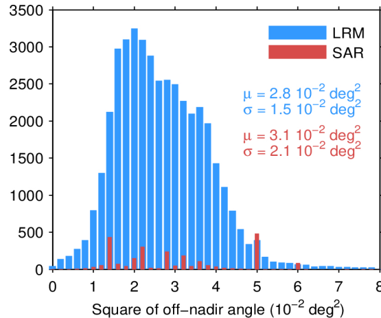
Figure 39. Histogram of flag-valid mispointing over oceans and lakes for LRM (blue) and SAR (red) for 27/05/2023. Only positive values have been considered. The mean ( \mu ) and standard deviation ( \sigma ) are also shown. Note that values larger than 8 \cdot 10^{-2} \text{ deg}^2 are excluded from the histogram for the sake of readability but not from the computation of \mu and \sigma .
