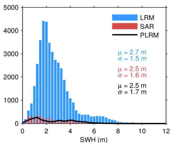
Figure 20. Histogram of science-valid SWH over oceans and lakes for LRM (blue), SAR (red), and PLRM (black) for 27/05/2023. The mean ( \mu ) and standard deviation ( \sigma ) are also
