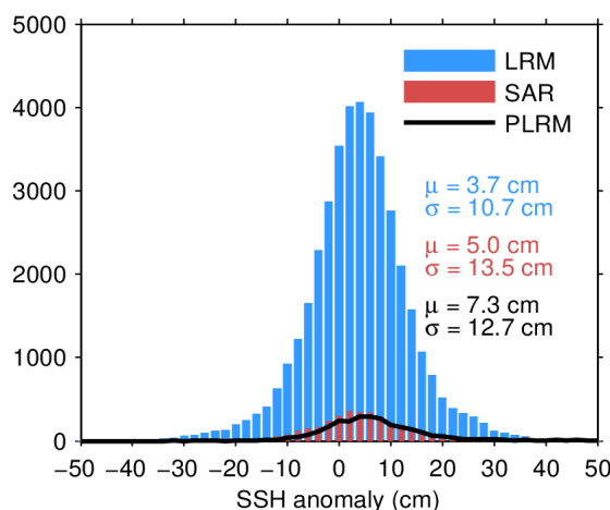
Figure 11. Histogram of science-valid SSH anomaly over oceans and lakes for LRM (blue), SAR (red), and PLRM (black) for 27/05/2023. The mean ( \mu ) and standard deviation ( \sigma ) are also shown. Note that values outside [-50, 50] cm are excluded from the histogram for the sake of readability but not from the computation of \mu and \sigma .
