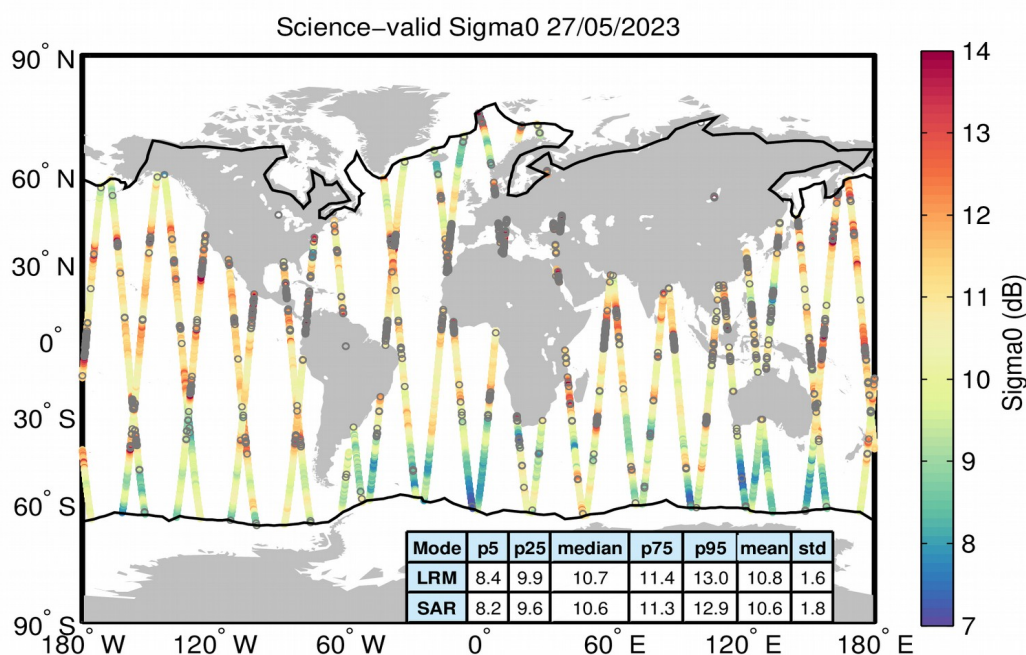
Figure 27. Geographical distribution of science-valid sigma0 data over oceans and lakes for 27/05/2023. The statistical values shown in the table refer to the sigma0 in dB and are calculated separately for LRM and SAR regions. The black lines mark the outer limit of the Arctic and Antarctic polar polygons. Gray circles denote records that have been rejected based on the editing criteria described in Table 4.
