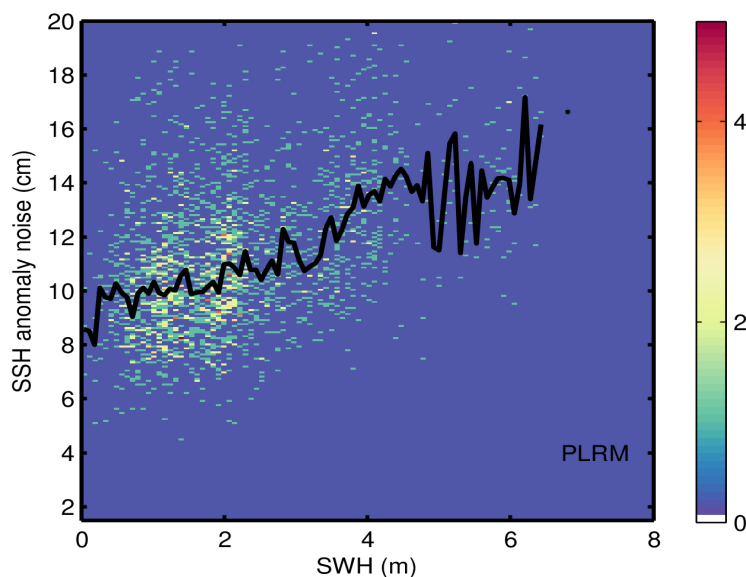
Figure 9. 2D histogram showing flag-valid SSH anomaly noise as a function of SWH for LRM (top), SAR (middle), and PLRM (bottom) for 26/05/2023. The black line denotes the median SSH anomaly noise as a function of SWH.
