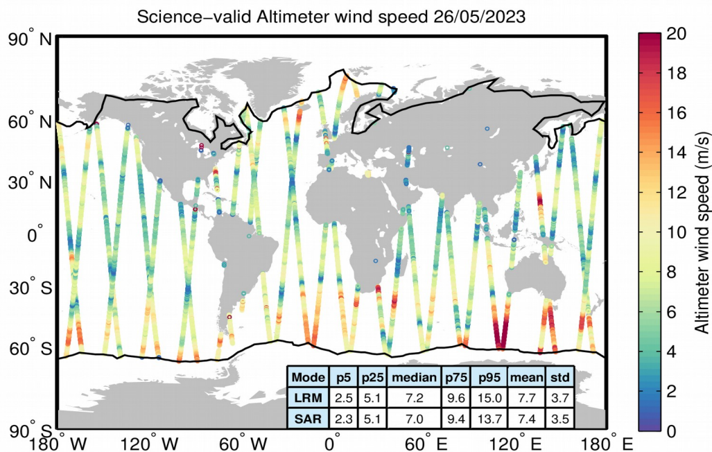
Figure 34. Geographical distribution of science-valid wind data over oceans and lakes for 26/05/2023. The statistical values shown in the table refer to the wind in m/s and are calculated separately for LRM and SAR regions. The black lines mark the outer limit of the Arctic and Antarctic polar polygons. Gray circles denote records that have been rejected based on the editing criteria described in Table 5.
