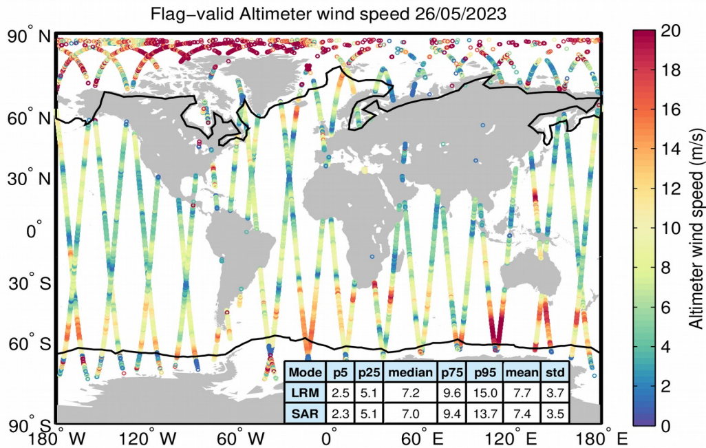
Figure 31. Geographical distribution of flag-valid wind data over oceans and lakes for 26/05/2023. The statistical values shown in the table refer to the wind in m/s and are calculated separately for LRM and SAR regions. Measurements taken over polar polygons have been excluded from the computation of the statistical values. The black lines mark the outer limit of the Arctic and Antarctic polar polygons.
