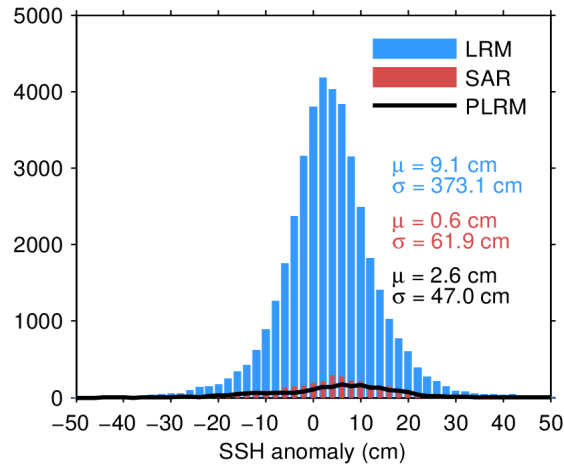
Figure 7. Histogram of flag-valid SSH anomaly over oceans and lakes for LRM (blue), SAR (red), and PLRM (black) for 26/05/2023. The mean ( \mu ) and standard deviation ( \sigma ) are also shown. Note that values outside [-50 50] cm are excluded from the histogram for the sake of readability but not from the computation of \mu and \sigma .
