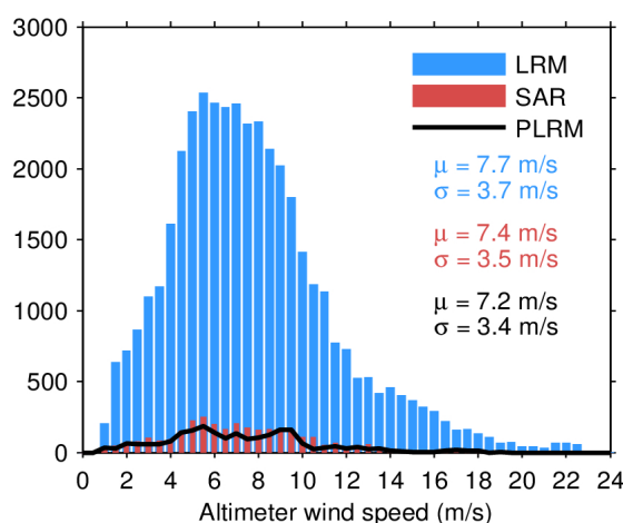
Figure 33. Histogram of flag-valid wind over oceans and lakes for LRM (blue), SAR (red), and PLRM (black) for 26/05/2023. The mean ( \mu ) and standard deviation ( \sigma ) are also shown. Note that values larger than 24 m/s are excluded from the histogram for the sake of readability but not from the computation of \mu and \sigma .
