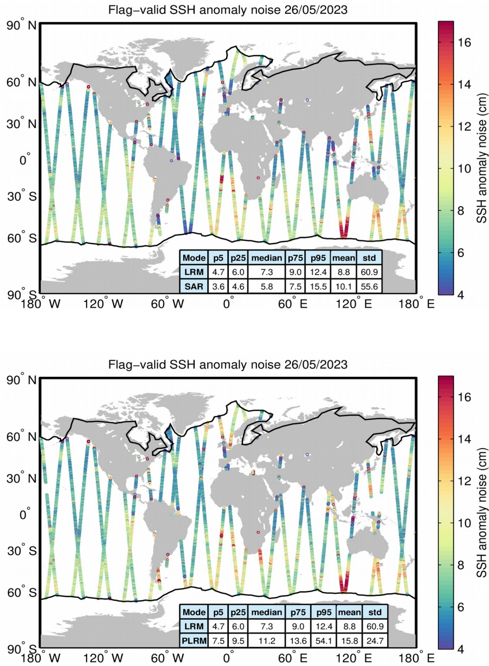
Figure 8. Geographical distribution of flag-valid 20-Hz SSH anomaly measurement noise over oceans and lakes for LRM/SAR (top) and LRM/PLRM (bottom) and for 26/05/2023. The statistical values shown in the tables refer to the SSH anomaly noise and are calculated separately for LRM and SAR/PLRM regions. Measurements taken over polar polygons have been excluded from the computation of the statistical values. The black lines mark the outer limit of the Arctic and Antarctic polar polygons.
