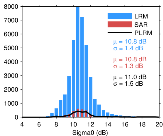
Figure 28. Histogram of science-valid sigma0 over oceans and lakes for LRM (blue), SAR (red), and PLRM (black) for 26/05/2023. The mean ( \mu ) and standard deviation ( \sigma ) are also shown. Note that values outside [4 20] dB are excluded from the histogram for the sake of readability but not from the computation of \mu and \sigma .
