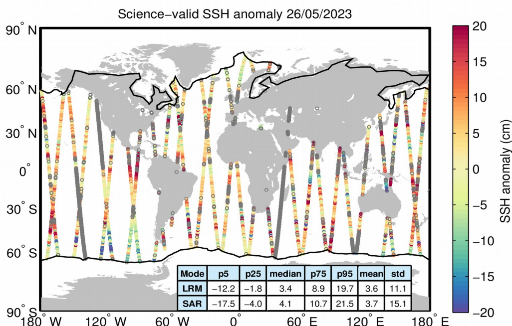
Figure 10. Geographical distribution of science-valid SSH anomaly data over oceans and lakes for 26/05/2023. The statistical values shown in the table refer to the SSH anomaly in cm and are calculated separately for LRM and SAR regions. The black lines mark the
