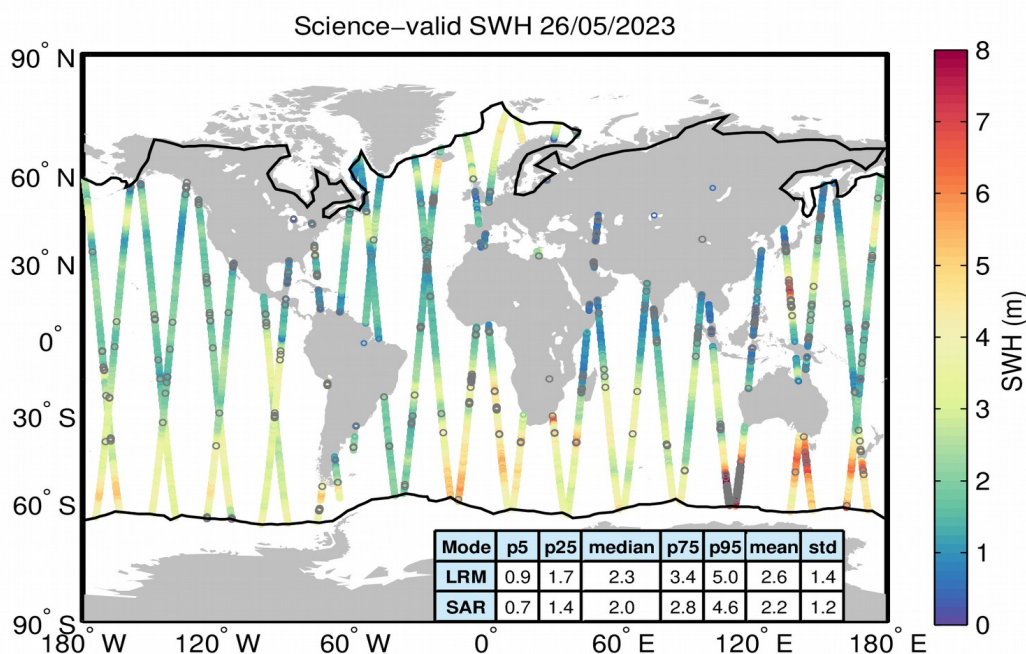
Figure 19. Geographical distribution of science-valid SWH data over oceans and lakes for 26/05/2023. The statistical values shown in the table refer to the SWH in m and are calculated separately for LRM and SAR regions. The black lines mark the outer limit of the Arctic and Antarctic polar polygons. Gray circles denote records that have been rejected based on the editing criteria described in Table 3.
