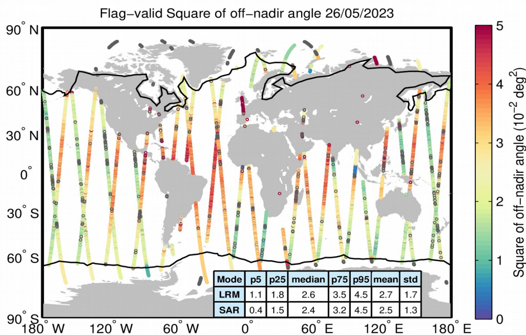
Figure 37. Geographical distribution of flag-valid mispointing data over oceans and lakes for 26/05/2023. The statistical values shown in the table refer to the mispointing in 10^{-2} \text{ deg}^2 and are calculated separately for LRM and SAR regions. Measurements taken over polar polygons have been excluded from the computation of the statistical values. The black lines mark the outer limit of the Arctic and Antarctic polar polygons. Gray circles denote negative values.
