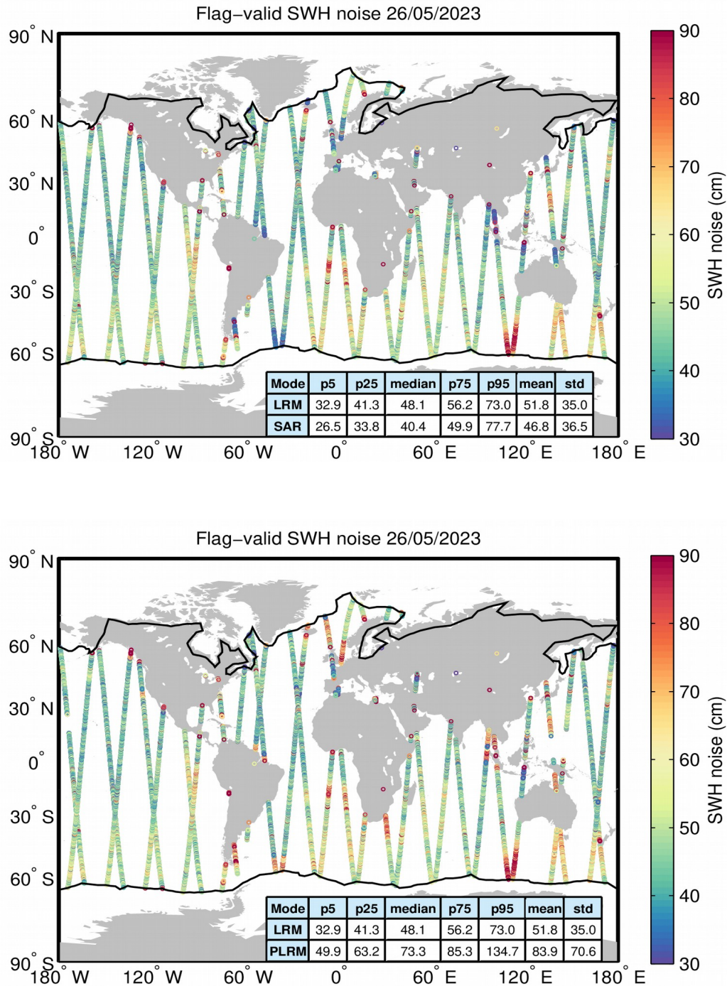
Figure 18. Geographical distribution of flag-valid 20-Hz SWH measurement noise over oceans and lakes for LRM/SAR (top) and LRM/PLRM (bottom) and for 26/05/2023. The statistical values shown in the table refer to the SWH noise and are calculated separately for LRM and SAR/PLRM regions. Measurements taken over polar polygons have been
