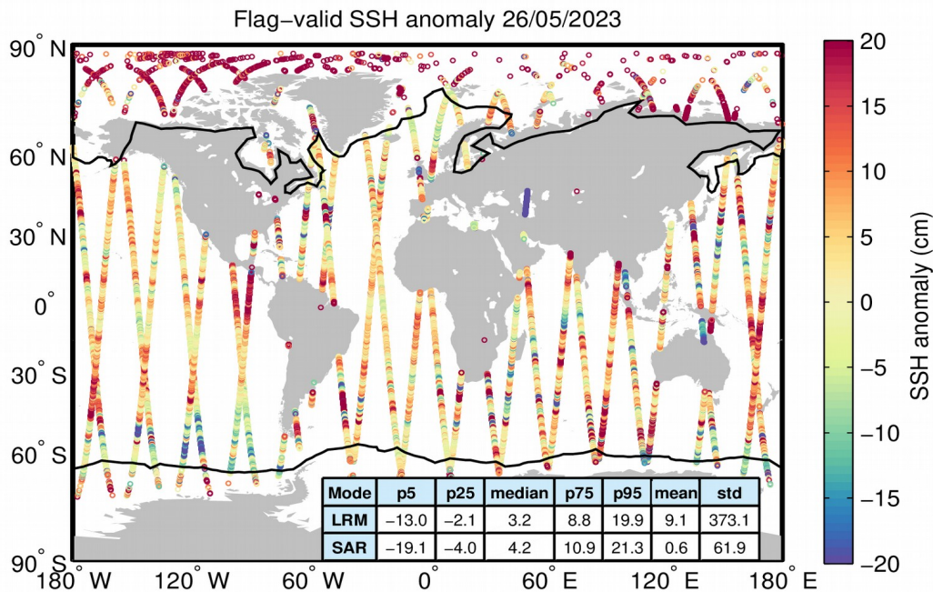
Figure 5. Geographical distribution of flag-valid 1-Hz SSH anomaly data over oceans and lakes for 26/05/2023. The statistical values shown in the table refer to the SSH anomaly in cm and are calculated separately for LRM and SAR regions. Measurements taken over polar polygons have been excluded from the computation of the statistical values. The black lines mark the outer limit of the Arctic and Antarctic polar polygons.
