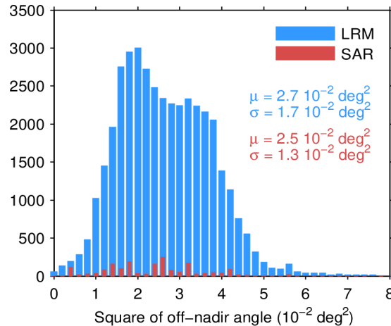
Figure 39. Histogram of flag-valid mispointing over oceans and lakes for LRM (blue) and SAR (red) for 26/05/2023. Only positive values have been considered. The mean ( \mu ) and standard deviation ( \sigma ) are also shown. Note that values larger than 8 \cdot 10^{-2} \text{ deg}^2 are excluded from the histogram for the sake of readability but not from the computation of \mu and \sigma .
