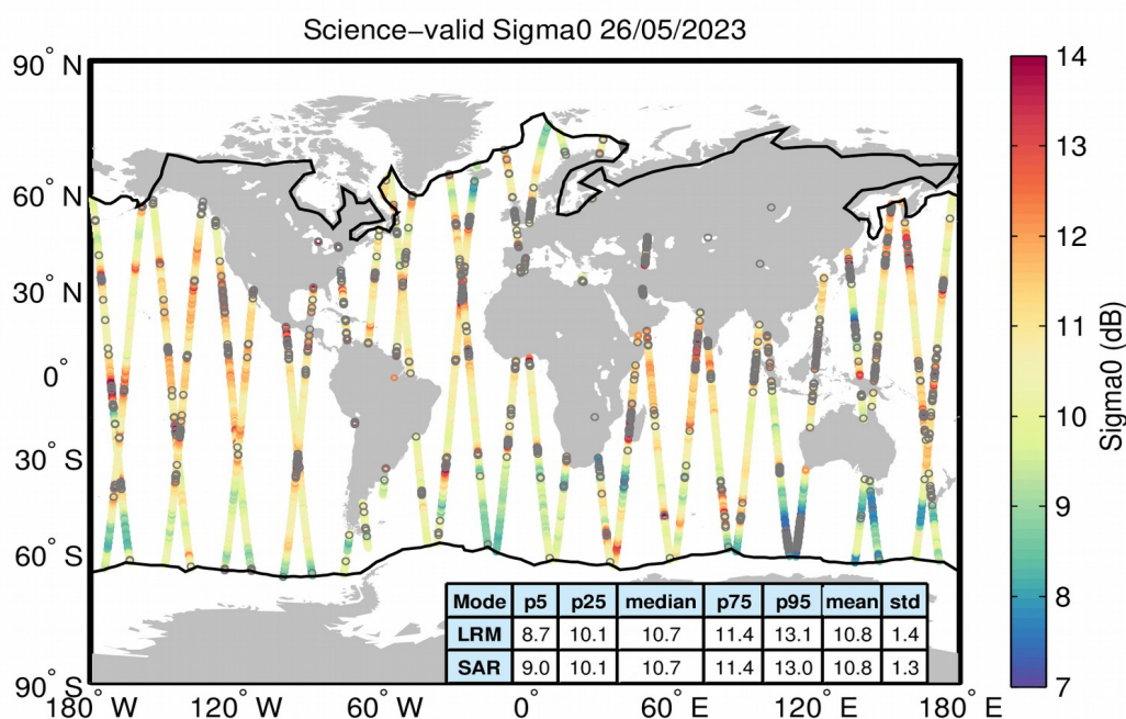
Figure 27. Geographical distribution of science-valid sigma0 data over oceans and lakes for 26/05/2023. The statistical values shown in the table refer to the sigma0 in dB and are calculated separately for LRM and SAR regions. The black lines mark the outer limit of the Arctic and Antarctic polar polygons. Gray circles denote records that have been rejected based on the editing criteria described in Table 4.
