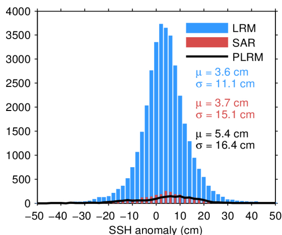
Figure 11. Histogram of science-valid SSH anomaly over oceans and lakes for LRM (blue), SAR (red), and PLRM (black) for 26/05/2023. The mean ( \mu ) and standard deviation ( \sigma ) are also shown. Note that values outside [-50, 50] cm are excluded from the histogram for the sake of readability but not from the computation of \mu and \sigma .
