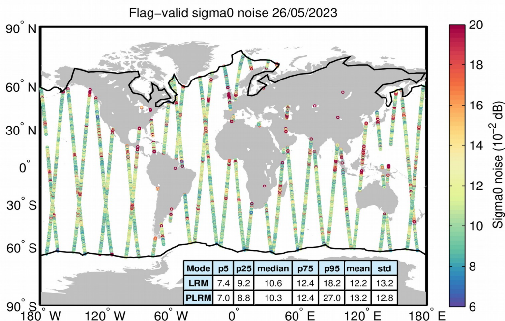
Figure 26. Geographical distribution of flag-valid 20-Hz sigma0 measurement noise over oceans and lakes for LRM/SAR (top) and LRM/PLRM (bottom) and for 26/05/2023. The statistical values shown in the table refer to the sigma0 noise and are calculated separately for LRM and SAR/PLRM regions. Measurements taken over polar polygons have been excluded from the computation of the statistical values. The black lines mark the outer limit of the Arctic and Antarctic polar polygons.
