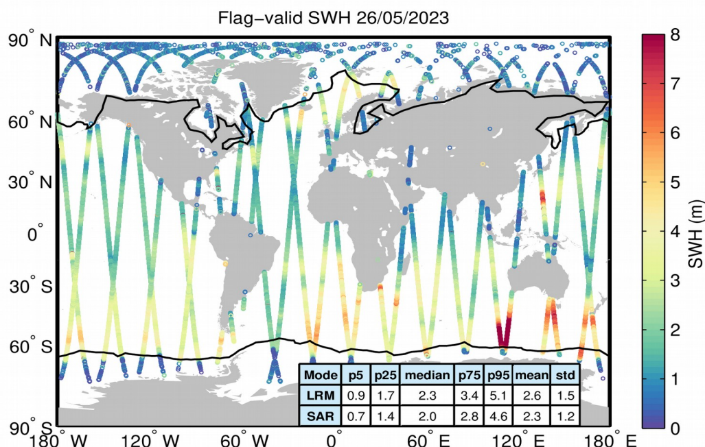
Figure 15. Geographical distribution of flag-valid SWH data over oceans and lakes for 26/05/2023. The statistical values shown in the table refer to the SWH in m and are calculated separately for LRM and SAR regions. Measurements taken over polar polygons have been excluded from the computation of the statistical values. The black lines mark the outer limit of the Arctic and Antarctic polar polygons.
