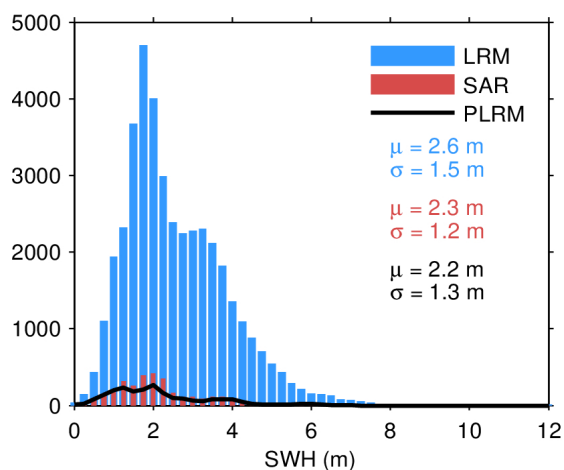
Figure 17. Histogram of flag-valid SWH over oceans and lakes for LRM (blue), SAR (red), and PLRM (black) for 26/05/2023. The mean ( \mu ) and standard deviation ( \sigma ) are also shown. Note that values larger than 12 m are excluded from the histogram for the sake of readability but not from the computation of \mu and \sigma .
