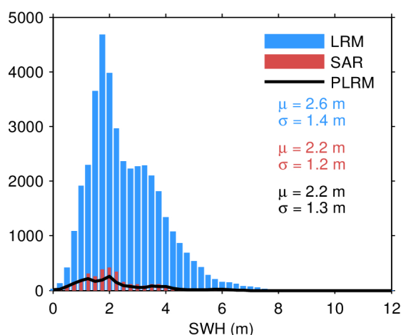
Figure 20. Histogram of science-valid SWH over oceans and lakes for LRM (blue), SAR (red), and PLRM (black) for 26/05/2023. The mean ( \mu ) and standard deviation ( \sigma ) are also
