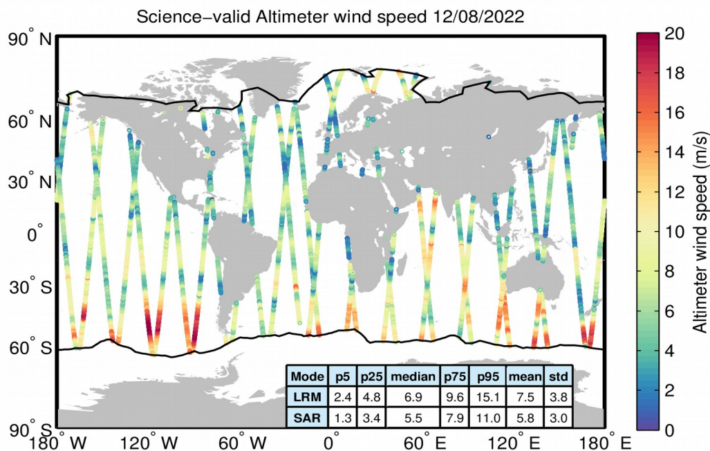
Figure 34. Geographical distribution of science-valid wind data over oceans and lakes for 12/08/2022. The statistical values shown in the table refer to the wind in m/s and are calculated separately for LRM and SAR regions. The black lines mark the outer limit of the Arctic and Antarctic polar polygons. Gray circles denote records that have been rejected based on the editing criteria described in Table 5.
