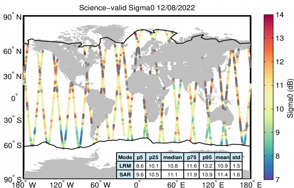
Figure 27. Geographical distribution of science-valid sigma0 data over oceans and lakes for 12/08/2022. The statistical values shown in the table refer to the sigma0 in dB and are calculated separately for LRM and SAR regions. The black lines mark the outer limit of the Arctic and Antarctic polar polygons. Gray circles denote records that have been rejected based on the editing criteria described in Table 4.
