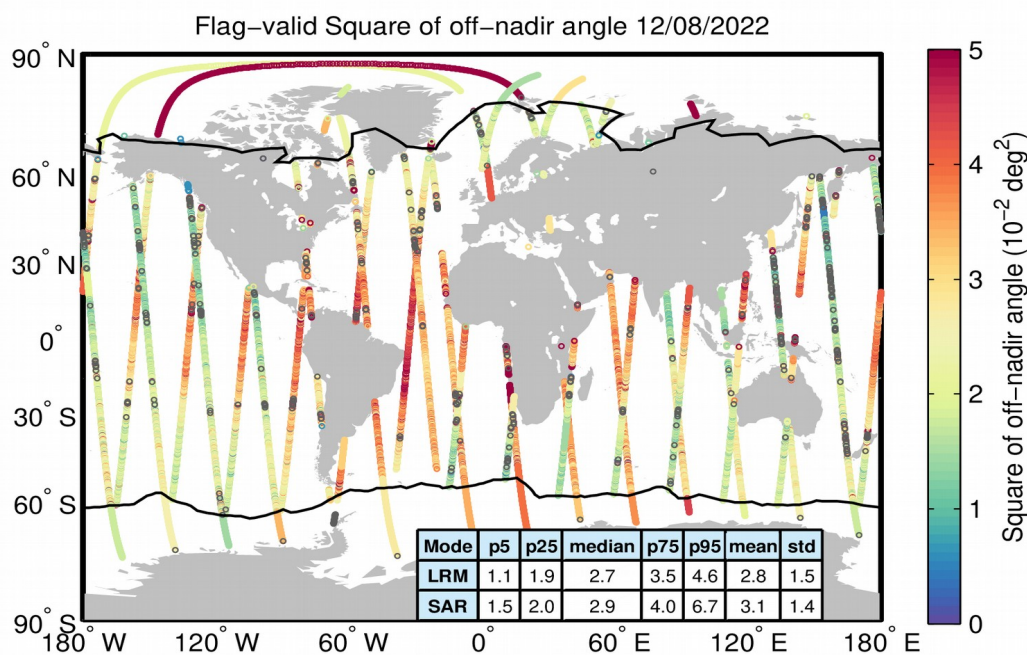
Figure 37. Geographical distribution of flag-valid mispointing data over oceans and lakes for 12/08/2022. The statistical values shown in the table refer to the mispointing in 10^{-2} \text{ deg}^2 and are calculated separately for LRM and SAR regions. Measurements taken over polar polygons have been excluded from the computation of the statistical values. The black lines mark the outer limit of the Arctic and Antarctic polar polygons. Gray circles denote negative values.
