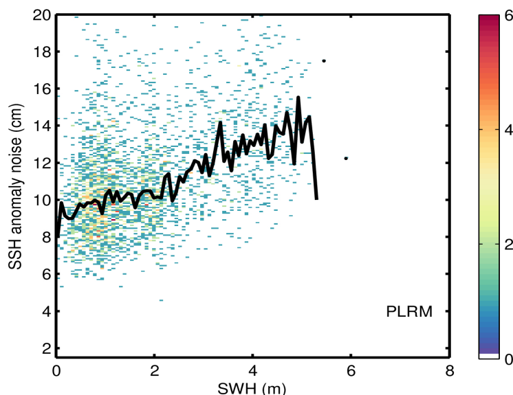
Figure 9. 2D histogram showing flag-valid SSH anomaly noise as a function of SWH for LRM (top), SAR (middle), and PLRM (bottom) for 12/08/2022. The black line denotes the median SSH anomaly noise as a function of SWH.
