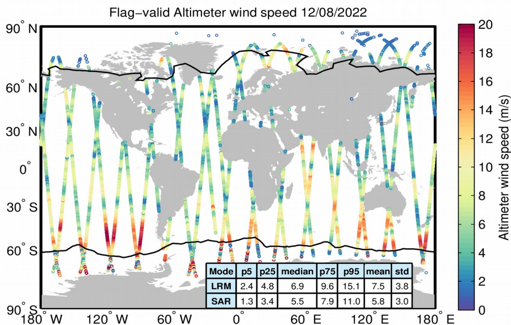
Figure 31. Geographical distribution of flag-valid wind data over oceans and lakes for 12/08/2022. The statistical values shown in the table refer to the wind in m/s and are calculated separately for LRM and SAR regions. Measurements taken over polar polygons have been excluded from the computation of the statistical values. The black lines mark the outer limit of the Arctic and Antarctic polar polygons.
