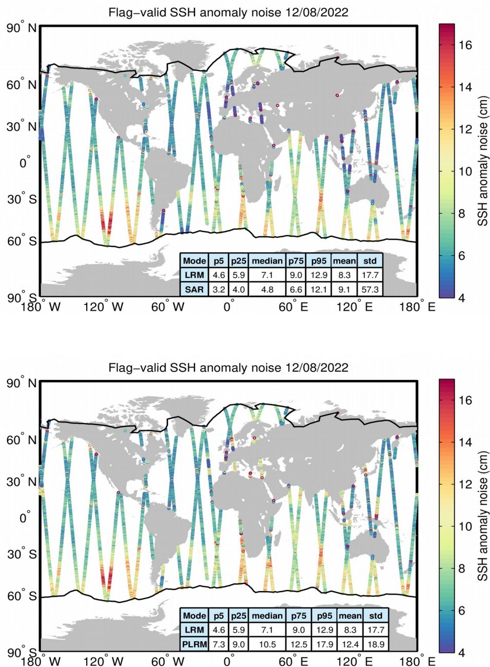
Figure 8. Geographical distribution of flag-valid 20-Hz SSH anomaly measurement noise over oceans and lakes for LRM/SAR (top) and LRM/PLRM (bottom) and for 12/08/2022. The statistical values shown in the tables refer to the SSH anomaly noise and are calculated separately for LRM and SAR/PLRM regions. Measurements taken over polar polygons have been excluded from the computation of the statistical values. The black lines mark the outer limit of the Arctic and Antarctic polar polygons.
