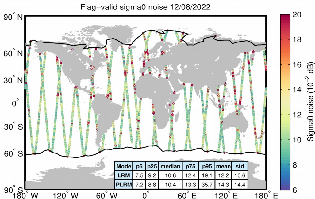
Figure 26. Geographical distribution of flag-valid 20-Hz sigma0 measurement noise over oceans and lakes for LRM/SAR (top) and LRM/PLRM (bottom) and for 12/08/2022. The statistical values shown in the table refer to the sigma0 noise and are calculated separately for LRM and SAR/PLRM regions. Measurements taken over polar polygons have been excluded from the computation of the statistical values. The black lines mark the outer limit of the Arctic and Antarctic polar polygons.
