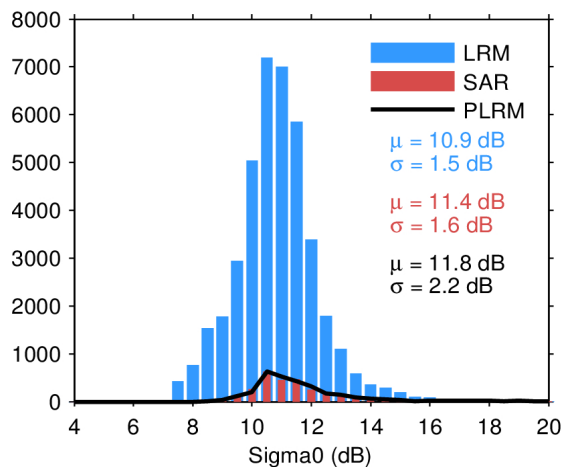
Figure 28. Histogram of science-valid sigma0 over oceans and lakes for LRM (blue), SAR (red), and PLRM (black) for 12/08/2022. The mean ( \mu ) and standard deviation ( \sigma ) are also shown. Note that values outside [4 20] dB are excluded from the histogram for the sake of readability but not from the computation of \mu and \sigma .
