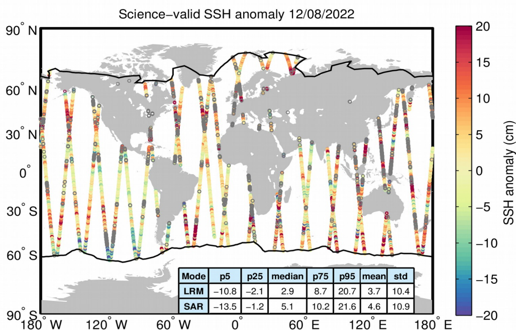
Figure 10. Geographical distribution of science-valid SSH anomaly data over oceans and lakes for 12/08/2022. The statistical values shown in the table refer to the SSH anomaly in cm and are calculated separately for LRM and SAR regions. The black lines mark the
