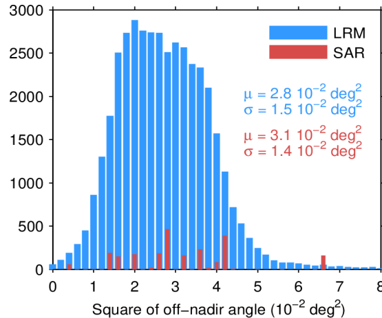
Figure 39. Histogram of flag-valid mispointing over oceans and lakes for LRM (blue) and SAR (red) for 12/08/2022. Only positive values have been considered. The mean ( \mu ) and standard deviation ( \sigma ) are also shown. Note that values larger than 8 \cdot 10^{-2} \text{ deg}^2 are excluded from the histogram for the sake of readability but not from the computation of \mu and \sigma .
