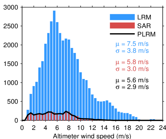
Figure 33. Histogram of flag-valid wind over oceans and lakes for LRM (blue), SAR (red), and PLRM (black) for 12/08/2022. The mean ( \mu ) and standard deviation ( \sigma ) are also shown. Note that values larger than 24 m/s are excluded from the histogram for the sake of readability but not from the computation of \mu and \sigma .
