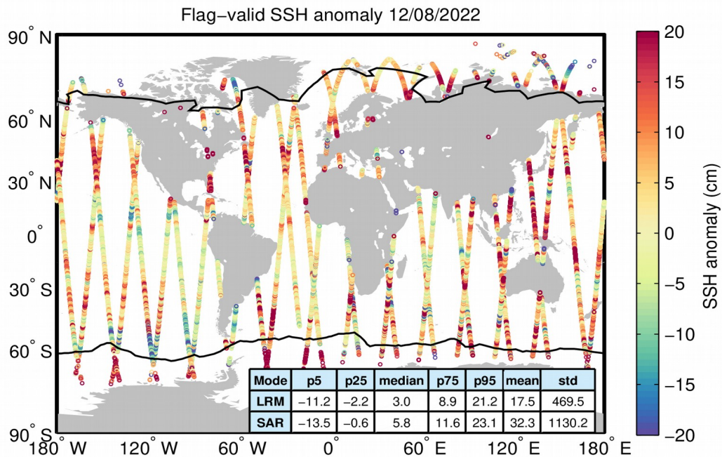
Figure 5. Geographical distribution of flag-valid 1-Hz SSH anomaly data over oceans and lakes for 12/08/2022. The statistical values shown in the table refer to the SSH anomaly in cm and are calculated separately for LRM and SAR regions. Measurements taken over polar polygons have been excluded from the computation of the statistical values. The black lines mark the outer limit of the Arctic and Antarctic polar polygons.
