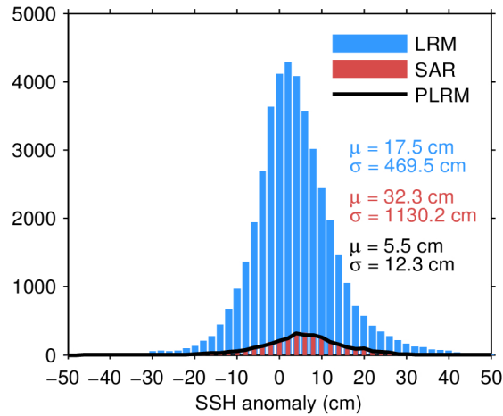
Figure 7. Histogram of flag-valid SSH anomaly over oceans and lakes for LRM (blue), SAR (red), and PLRM (black) for 12/08/2022. The mean ( \mu ) and standard deviation ( \sigma ) are also shown. Note that values outside [-50 50] cm are excluded from the histogram for the sake of readability but not from the computation of \mu and \sigma .
