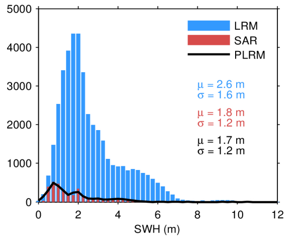
Figure 17. Histogram of flag-valid SWH over oceans and lakes for LRM (blue), SAR (red), and PLRM (black) for 12/08/2022. The mean ( \mu ) and standard deviation ( \sigma ) are also shown. Note that values larger than 12 m are excluded from the histogram for the sake of readability but not from the computation of \mu and \sigma .
