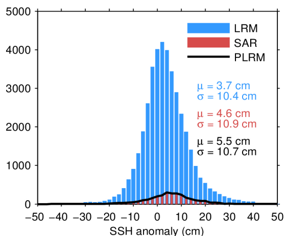
Figure 11. Histogram of science-valid SSH anomaly over oceans and lakes for LRM (blue), SAR (red), and PLRM (black) for 12/08/2022. The mean ( \mu ) and standard deviation ( \sigma ) are also shown. Note that values outside [-50, 50] cm are excluded from the histogram for the sake of readability but not from the computation of \mu and \sigma .
