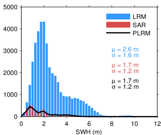
Figure 20. Histogram of science-valid SWH over oceans and lakes for LRM (blue), SAR (red), and PLRM (black) for 12/08/2022. The mean ( \mu ) and standard deviation ( \sigma ) are also
