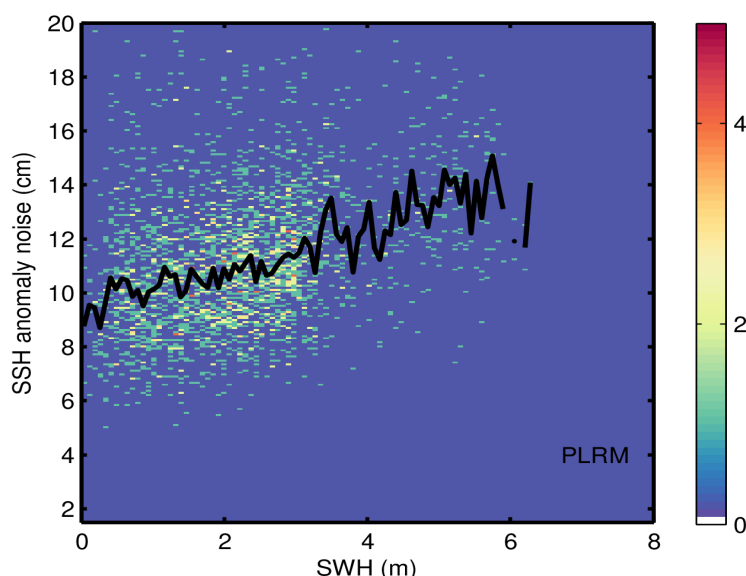
Figure 9. 2D histogram showing flag-valid SSH anomaly noise as a function of SWH for LRM (top), SAR (middle), and PLRM (bottom) for 24/01/2022. The black line denotes the median SSH anomaly noise as a function of SWH.
