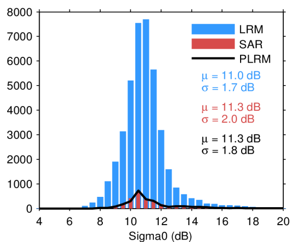
Figure 25. Histogram of flag-valid sigma0 over oceans and lakes for LRM (blue), SAR (red), and PLRM (black) for 24/01/2022. The mean ( \mu ) and standard deviation ( \sigma ) are also
