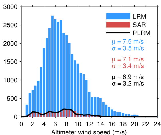
Figure 35. Histogram of science-valid wind over oceans and lakes for LRM (blue), SAR (red), and PLRM (black) for 24/01/2022. The mean ( \mu ) and standard deviation ( \sigma ) are also shown. Note that values larger than 24 m/s are excluded from the histogram for the sake of readability but not from the computation of \mu and \sigma .
