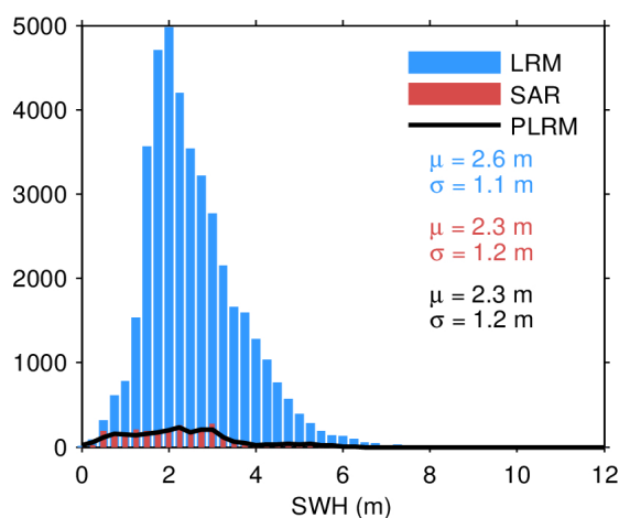
Figure 20. Histogram of science-valid SWH over oceans and lakes for LRM (blue), SAR (red), and PLRM (black) for 24/01/2022. The mean ( \mu ) and standard deviation ( \sigma ) are also shown. Note that values larger than 12 m are excluded from the histogram for the sake of readability but not from the computation of \mu and \sigma .
