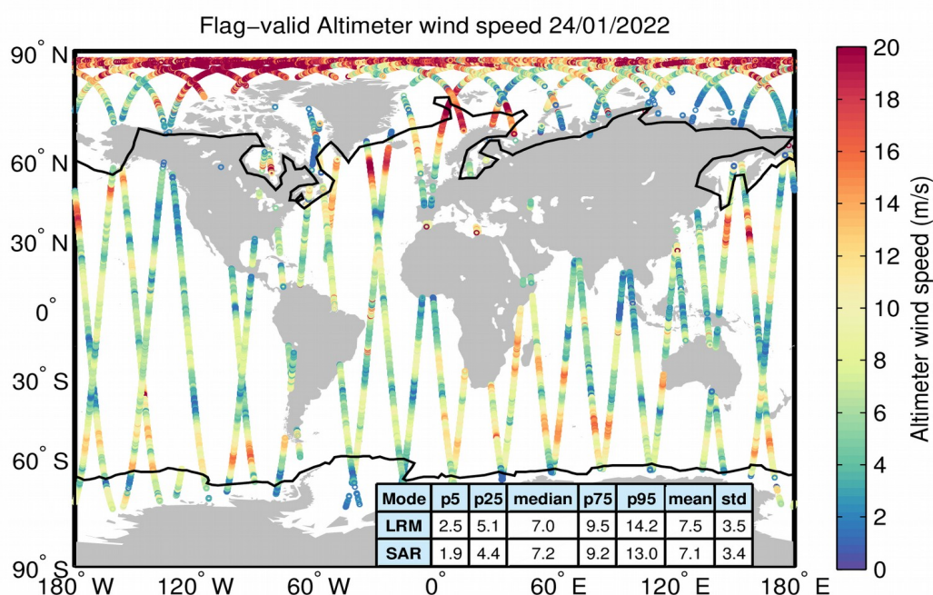
Figure 31. Geographical distribution of flag-valid wind data over oceans and lakes for 24/01/2022. The statistical values shown in the table refer to the wind in m/s and are calculated separately for LRM and SAR regions. Measurements taken over polar polygons have been excluded from the computation of the statistical values. The black lines mark the outer limit of the Arctic and Antarctic polar polygons.
