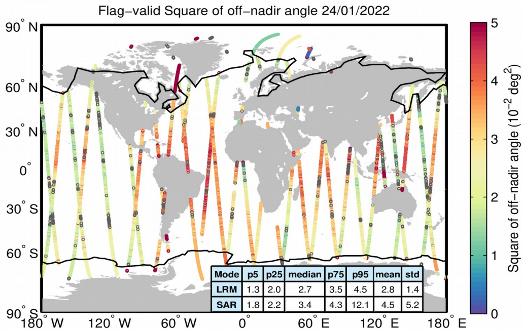
Figure 37. Geographical distribution of flag-valid mispointing data over oceans and lakes for 24/01/2022. The statistical values shown in the table refer to the mispointing in 10^{-2} \text{ deg}^2 and are calculated separately for LRM and SAR regions. Measurements taken over polar polygons have been excluded from the computation of the statistical values. The black lines mark the outer limit of the Arctic and Antarctic polar polygons. Gray circles denote negative values.
