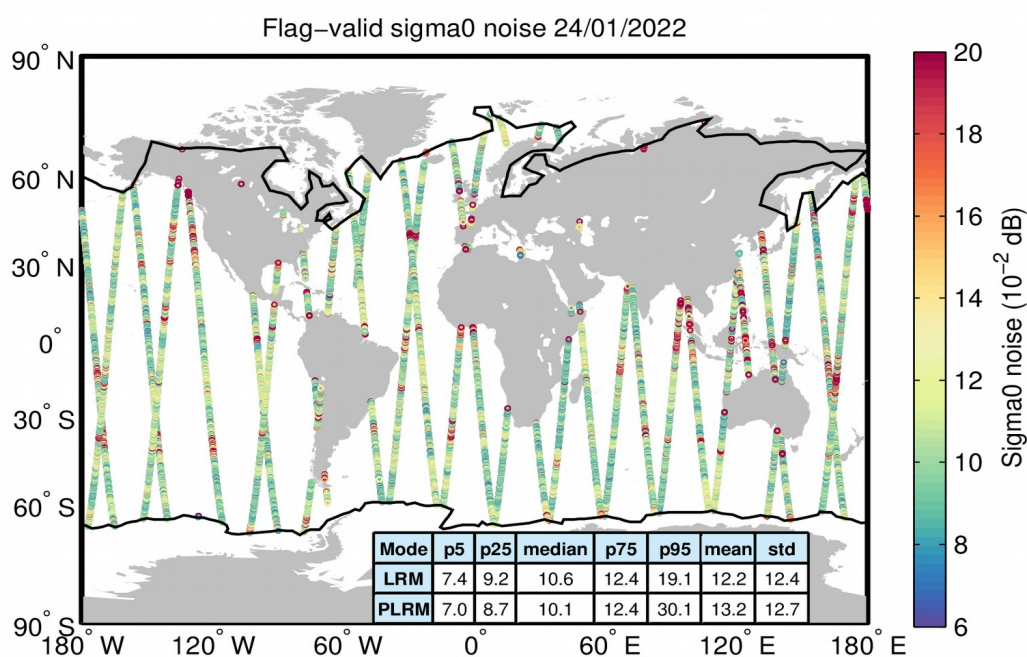
Figure 26. Geographical distribution of flag-valid 20-Hz sigma0 measurement noise over oceans and lakes for LRM/SAR (top) and LRM/PLRM (bottom) and for 24/01/2022. The statistical values shown in the table refer to the sigma0 noise and are calculated separately for LRM and SAR/PLRM regions. Measurements taken over polar polygons have been excluded from the computation of the statistical values. The black lines mark the outer limit of the Arctic and Antarctic polar polygons.
