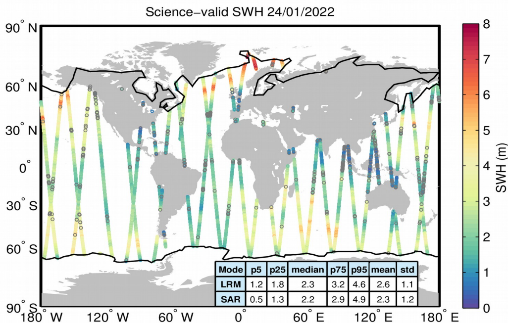
Figure 19. Geographical distribution of science-valid SWH data over oceans and lakes for 24/01/2022. The statistical values shown in the table refer to the SWH in m and are calculated separately for LRM and SAR regions. The black lines mark the outer limit of the Arctic and Antarctic polar polygons. Gray circles denote records that have been rejected based on the editing criteria described in Table 3.
