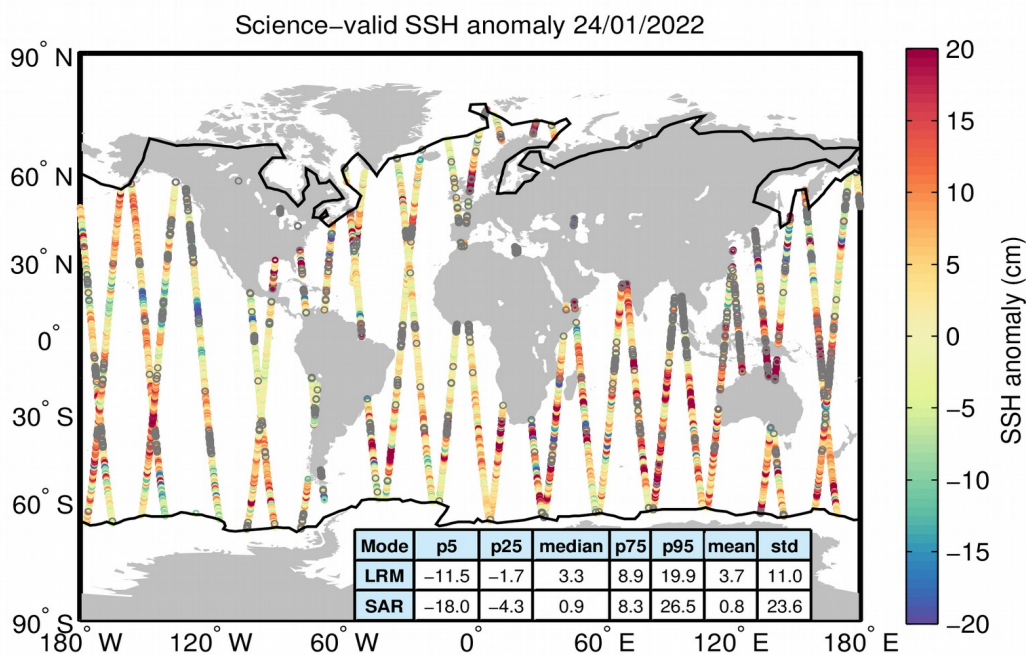
Figure 10. Geographical distribution of science-valid SSH anomaly data over oceans and lakes for 24/01/2022. The statistical values shown in the table refer to the SSH anomaly in cm and are calculated separately for LRM and SAR regions. The black lines mark the outer limit of the Arctic and Antarctic polar polygons. Gray circles denote records that have been rejected based on the editing criteria described in Table 2.
