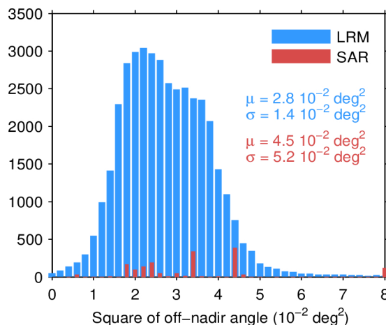
Figure 39. Histogram of flag-valid mispointing over oceans and lakes for LRM (blue) and SAR (red) for 24/01/2022. Only positive values have been considered. The mean ( \mu ) and standard deviation ( \sigma ) are also shown. Note that values larger than 8 \cdot 10^{-2} \text{ deg}^2 are excluded from the histogram for the sake of readability but not from the computation of \mu and \sigma .
