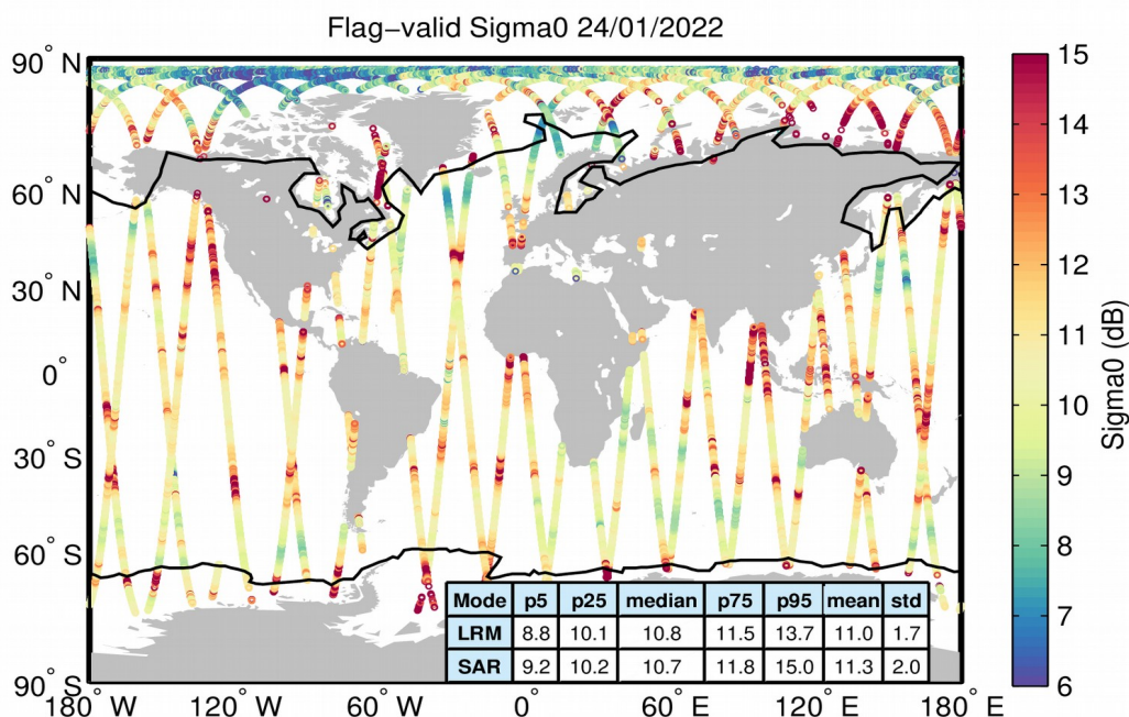
Figure 23. Geographical distribution of flag-valid sigma0 data over oceans and lakes for 24/01/2022. The statistical values shown in the table refer to the sigma0 in dB and are calculated separately for LRM and SAR regions. Measurements taken over polar polygons
