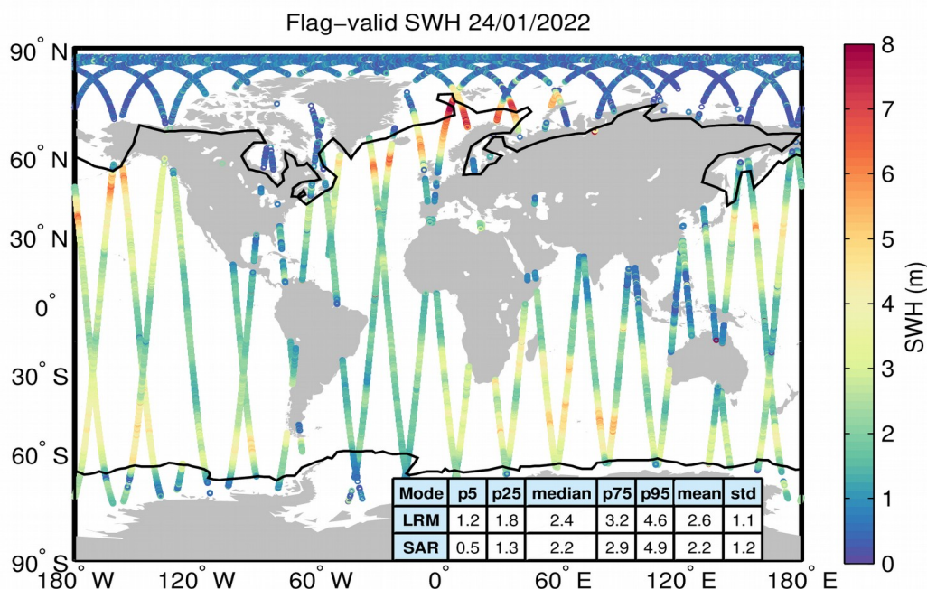
Figure 15. Geographical distribution of flag-valid SWH data over oceans and lakes for 24/01/2022. The statistical values shown in the table refer to the SWH in m and are calculated separately for LRM and SAR regions. Measurements taken over polar polygons
