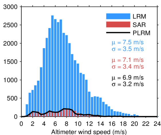
Figure 33. Histogram of flag-valid wind over oceans and lakes for LRM (blue), SAR (red), and PLRM (black) for 24/01/2022. The mean ( \mu ) and standard deviation ( \sigma ) are also shown. Note that values larger than 24 m/s are excluded from the histogram for the sake of readability but not from the computation of \mu and \sigma .
