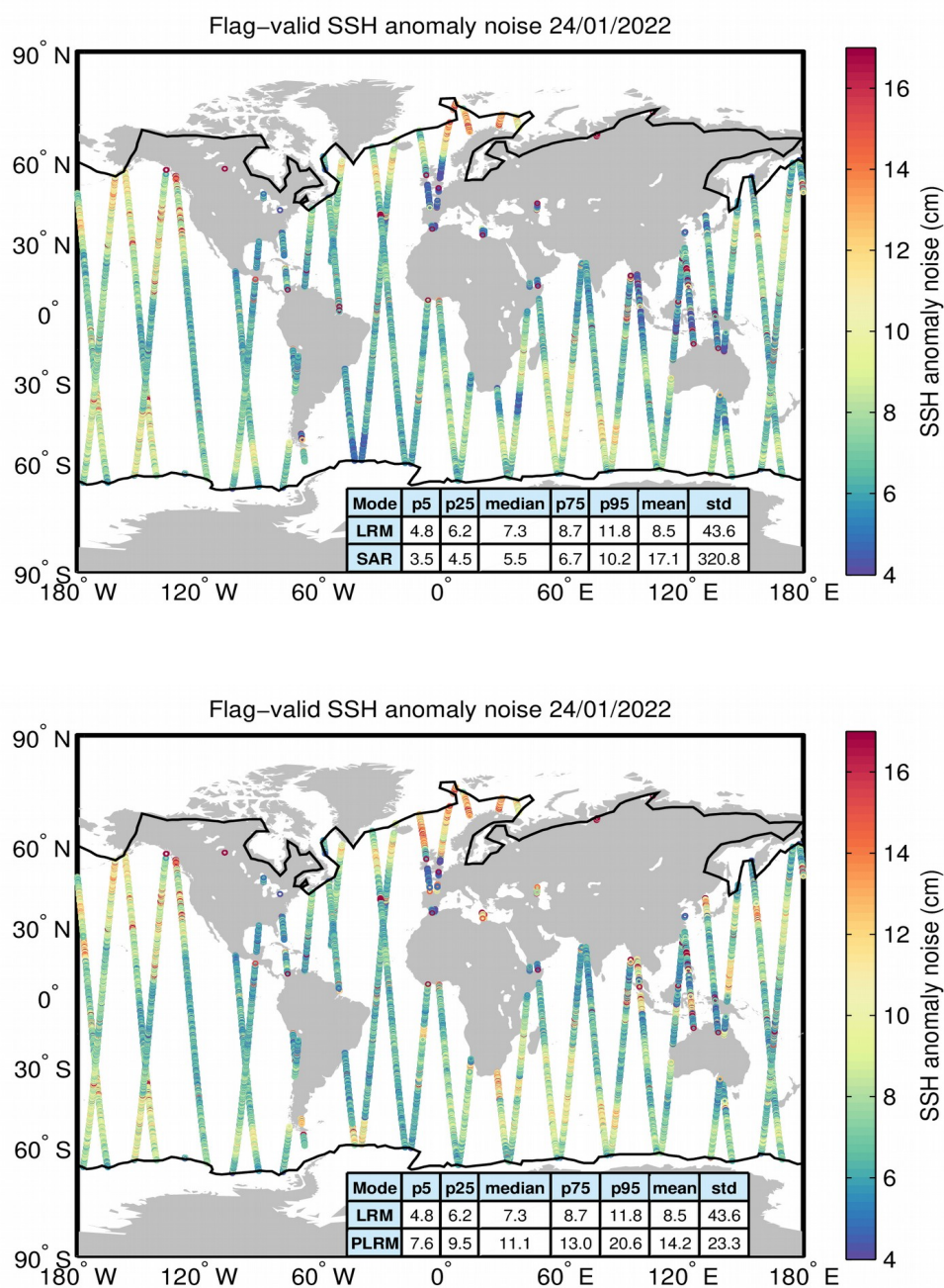
Figure 8. Geographical distribution of flag-valid 20-Hz SSH anomaly measurement noise over oceans and lakes for LRM/SAR (top) and LRM/PLRM (bottom) and for 24/01/2022. The statistical values shown in the tables refer to the SSH anomaly noise and are calculated separately for LRM and SAR/PLRM regions. Measurements taken over polar polygons have been excluded from the computation of the statistical values. The black lines mark the outer limit of the Arctic and Antarctic polar polygons.
