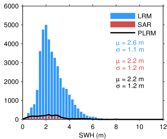
Figure 17. Histogram of flag-valid SWH over oceans and lakes for LRM (blue), SAR (red), and PLRM (black) for 24/01/2022. The mean ( \mu ) and standard deviation ( \sigma ) are also shown. Note that values larger than 12 m are excluded from the histogram for the sake of readability but not from the computation of \mu and \sigma .
