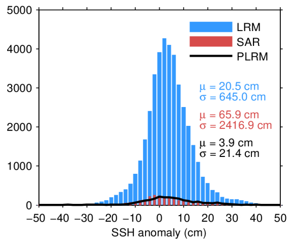
Figure 7. Histogram of flag-valid SSH anomaly over oceans and lakes for LRM (blue), SAR (red), and PLRM (black) for 24/01/2022. The mean ( \mu ) and standard deviation ( \sigma ) are also shown. Note that values outside [-50 50] cm are excluded from the histogram for the sake of readability but not from the computation of \mu and \sigma .
