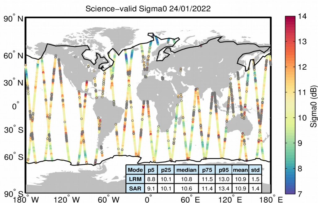
Figure 27. Geographical distribution of science-valid sigma0 data over oceans and lakes for 24/01/2022. The statistical values shown in the table refer to the sigma0 in dB and are calculated separately for LRM and SAR regions. The black lines mark the outer limit of the Arctic and Antarctic polar polygons. Gray circles denote records that have been rejected based on the editing criteria described in Table 4.
