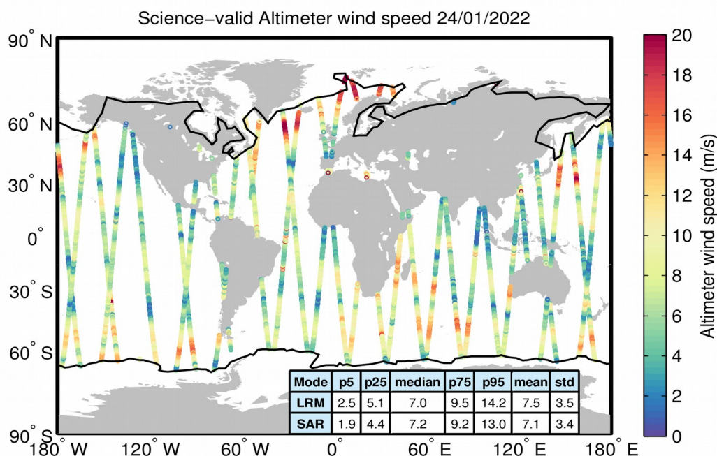
Figure 34. Geographical distribution of science-valid wind data over oceans and lakes for 24/01/2022. The statistical values shown in the table refer to the wind in m/s and are calculated separately for LRM and SAR regions. The black lines mark the outer limit of the Arctic and Antarctic polar polygons. Gray circles denote records that have been rejected based on the editing criteria described in Table 5.
