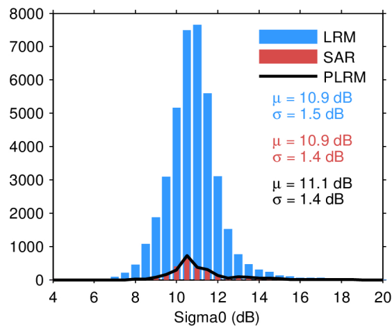
Figure 28. Histogram of science-valid sigma0 over oceans and lakes for LRM (blue), SAR (red), and PLRM (black) for 24/01/2022. The mean ( \mu ) and standard deviation ( \sigma ) are also shown. Note that values outside [4 20] dB are excluded from the histogram for the sake of readability but not from the computation of \mu and \sigma .
