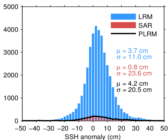
Figure 11. Histogram of science-valid SSH anomaly over oceans and lakes for LRM (blue), SAR (red), and PLRM (black) for 24/01/2022. The mean ( \mu ) and standard deviation ( \sigma ) are also shown. Note that values outside [-50, 50] cm are excluded from the histogram for the sake of readability but not from the computation of \mu and \sigma .
