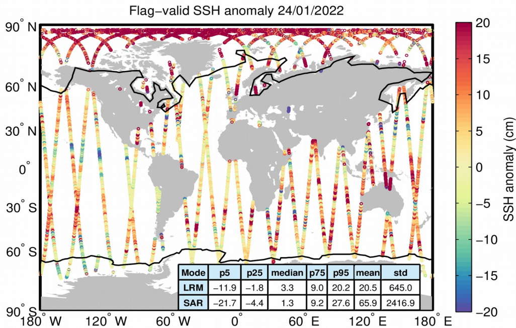
Figure 5. Geographical distribution of flag-valid 1-Hz SSH anomaly data over oceans and lakes for 24/01/2022. The statistical values shown in the table refer to the SSH anomaly in cm and are calculated separately for LRM and SAR regions. Measurements taken over polar polygons have been excluded from the computation of the statistical values. The black lines mark the outer limit of the Arctic and Antarctic polar polygons.
