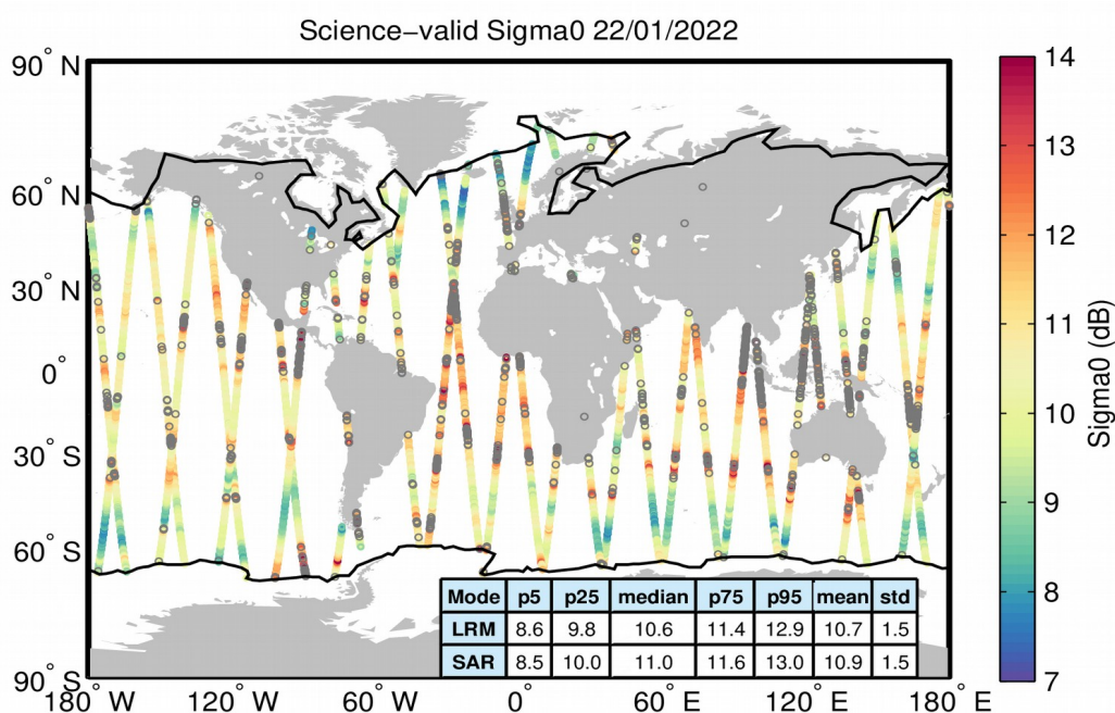
Figure 27. Geographical distribution of science-valid sigma0 data over oceans and lakes for 22/01/2022. The statistical values shown in the table refer to the sigma0 in dB and are calculated separately for LRM and SAR regions. The black lines mark the outer limit of the Arctic and Antarctic polar polygons. Gray circles denote records that have been rejected based on the editing criteria described in Table 4.
