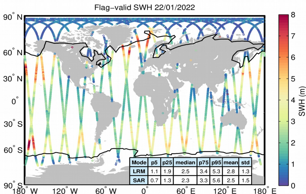
Figure 15. Geographical distribution of flag-valid SWH data over oceans and lakes for 22/01/2022. The statistical values shown in the table refer to the SWH in m and are calculated separately for LRM and SAR regions. Measurements taken over polar polygons
