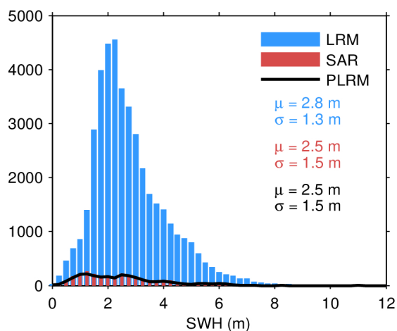
Figure 17. Histogram of flag-valid SWH over oceans and lakes for LRM (blue), SAR (red), and PLRM (black) for 22/01/2022. The mean ( \mu ) and standard deviation ( \sigma ) are also shown. Note that values larger than 12 m are excluded from the histogram for the sake of readability but not from the computation of \mu and \sigma .
