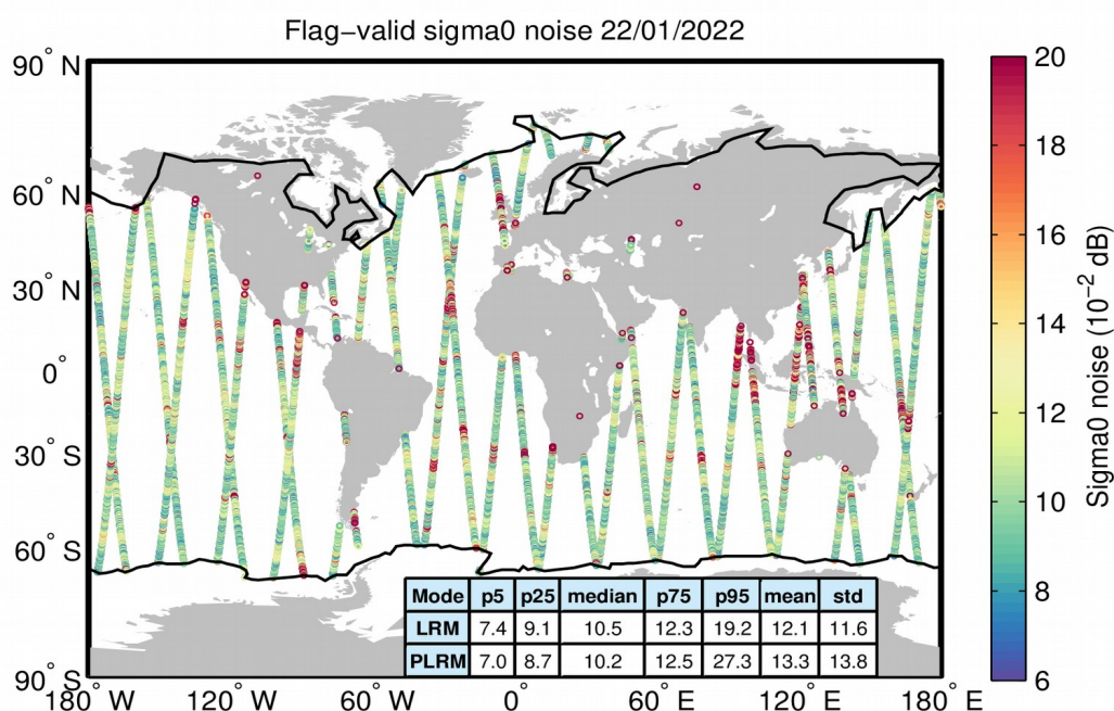
Figure 26. Geographical distribution of flag-valid 20-Hz sigma0 measurement noise over oceans and lakes for LRM/SAR (top) and LRM/PLRM (bottom) and for 22/01/2022. The statistical values shown in the table refer to the sigma0 noise and are calculated separately for LRM and SAR/PLRM regions. Measurements taken over polar polygons have been excluded from the computation of the statistical values. The black lines mark the outer limit of the Arctic and Antarctic polar polygons.
