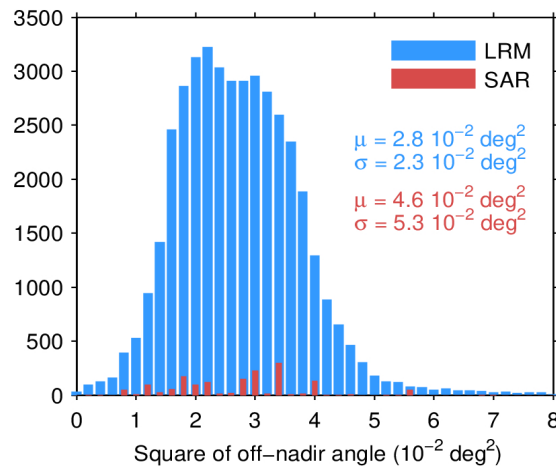
Figure 39. Histogram of flag-valid mispointing over oceans and lakes for LRM (blue) and SAR (red) for 22/01/2022. Only positive values have been considered. The mean ( \mu ) and standard deviation ( \sigma ) are also shown. Note that values larger than 8 \cdot 10^{-2} \text{ deg}^2 are excluded from the histogram for the sake of readability but not from the computation of \mu and \sigma .
