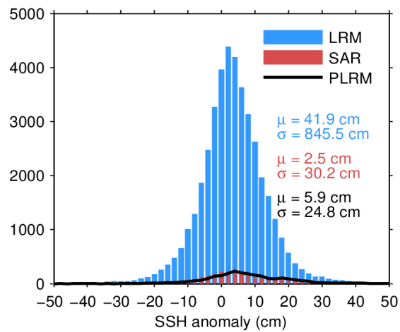
Figure 7. Histogram of flag-valid SSH anomaly over oceans and lakes for LRM (blue), SAR (red), and PLRM (black) for 22/01/2022. The mean ( \mu ) and standard deviation ( \sigma ) are also shown. Note that values outside [-50 50] cm are excluded from the histogram for the sake of readability but not from the computation of \mu and \sigma .
