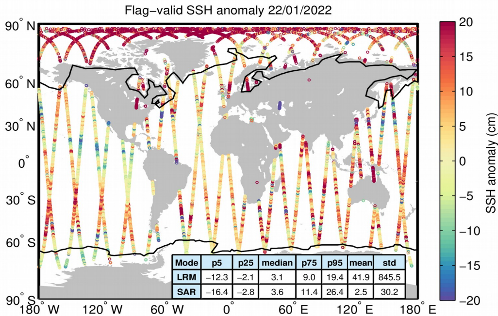
Figure 5. Geographical distribution of flag-valid 1-Hz SSH anomaly data over oceans and lakes for 22/01/2022. The statistical values shown in the table refer to the SSH anomaly in cm and are calculated separately for LRM and SAR regions. Measurements taken over polar polygons have been excluded from the computation of the statistical values. The black lines mark the outer limit of the Arctic and Antarctic polar polygons.
