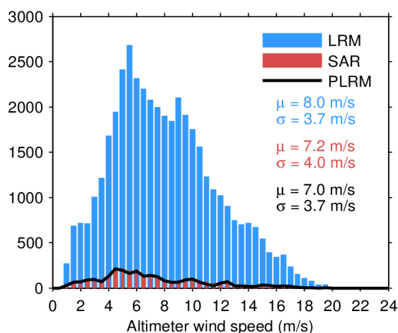
Figure 35. Histogram of science-valid wind over oceans and lakes for LRM (blue), SAR (red), and PLRM (black) for 22/01/2022. The mean ( \mu ) and standard deviation ( \sigma ) are also shown. Note that values larger than 24 m/s are excluded from the histogram for the sake of readability but not from the computation of \mu and \sigma .
