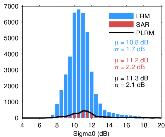
Figure 25. Histogram of flag-valid sigma0 over oceans and lakes for LRM (blue), SAR (red), and PLRM (black) for 22/01/2022. The mean ( \mu ) and standard deviation ( \sigma ) are also
