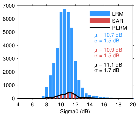
Figure 28. Histogram of science-valid sigma0 over oceans and lakes for LRM (blue), SAR (red), and PLRM (black) for 22/01/2022. The mean ( \mu ) and standard deviation ( \sigma ) are also shown. Note that values outside [4 20] dB are excluded from the histogram for the sake of readability but not from the computation of \mu and \sigma .
