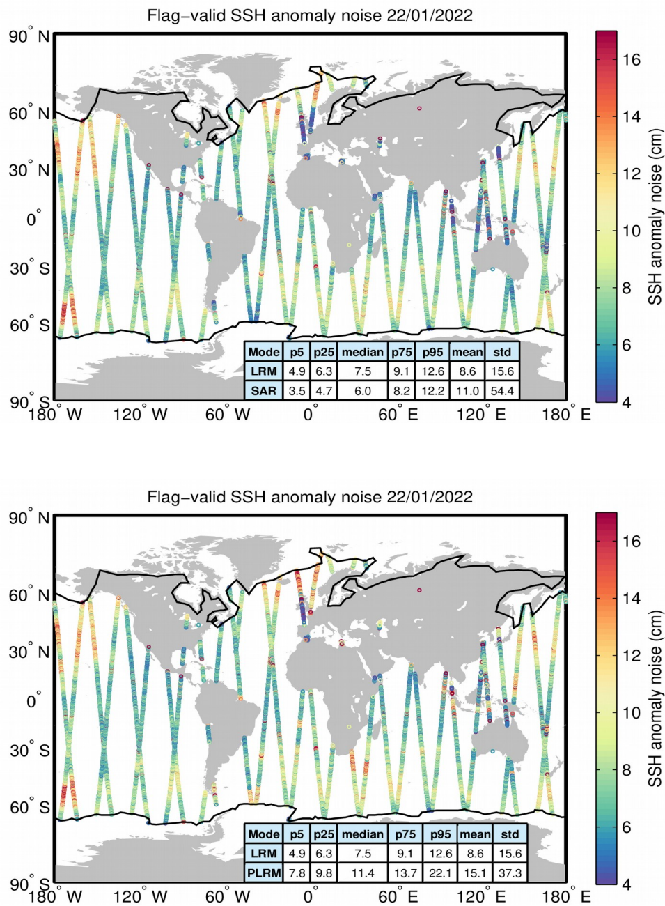
Figure 8. Geographical distribution of flag-valid 20-Hz SSH anomaly measurement noise over oceans and lakes for LRM/SAR (top) and LRM/PLRM (bottom) and for 22/01/2022. The statistical values shown in the tables refer to the SSH anomaly noise and are calculated separately for LRM and SAR/PLRM regions. Measurements taken over polar polygons have been excluded from the computation of the statistical values. The black lines mark the outer limit of the Arctic and Antarctic polar polygons.
