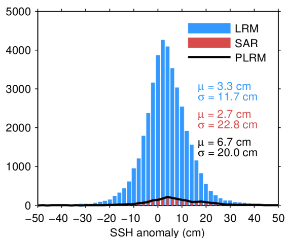
Figure 11. Histogram of science-valid SSH anomaly over oceans and lakes for LRM (blue), SAR (red), and PLRM (black) for 22/01/2022. The mean ( \mu ) and standard deviation ( \sigma ) are also shown. Note that values outside [-50, 50] cm are excluded from the histogram for the sake of readability but not from the computation of \mu and \sigma .
