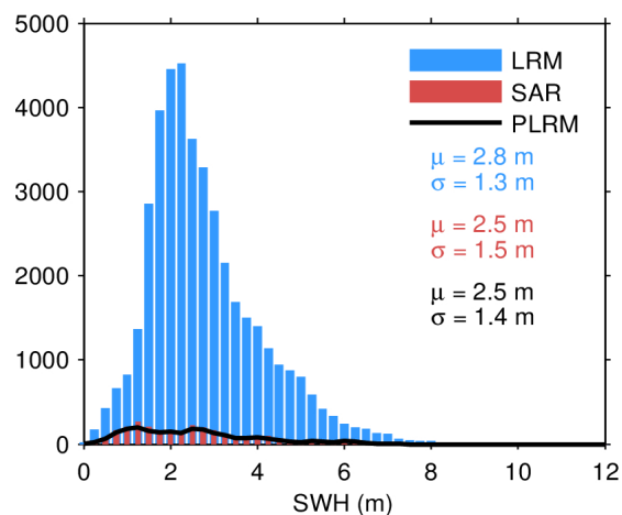
Figure 20. Histogram of science-valid SWH over oceans and lakes for LRM (blue), SAR (red), and PLRM (black) for 22/01/2022. The mean ( \mu ) and standard deviation ( \sigma ) are also shown. Note that values larger than 12 m are excluded from the histogram for the sake of readability but not from the computation of \mu and \sigma .
