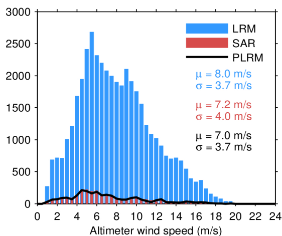
Figure 33. Histogram of flag-valid wind over oceans and lakes for LRM (blue), SAR (red), and PLRM (black) for 22/01/2022. The mean ( \mu ) and standard deviation ( \sigma ) are also shown. Note that values larger than 24 m/s are excluded from the histogram for the sake of readability but not from the computation of \mu and \sigma .
