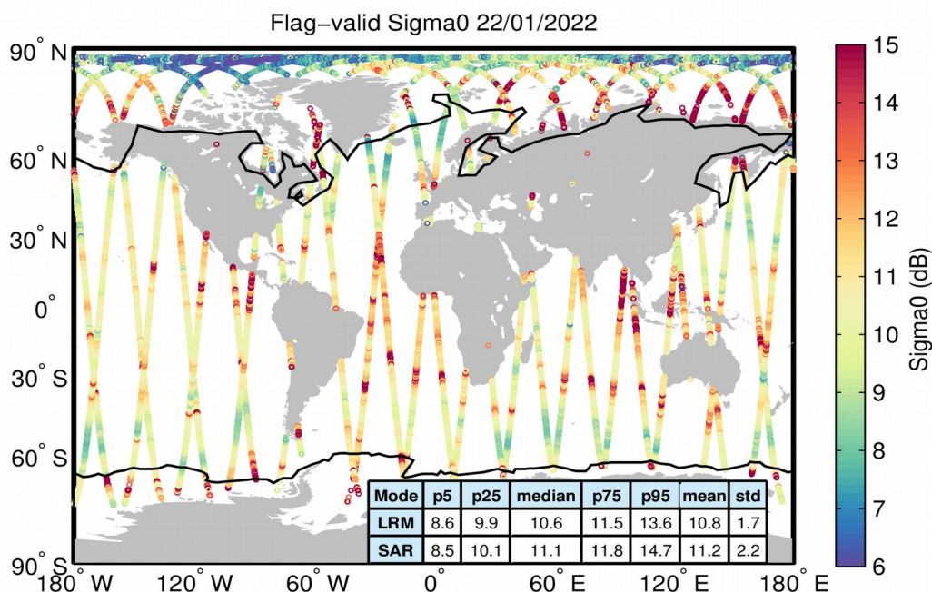
Figure 23. Geographical distribution of flag-valid sigma0 data over oceans and lakes for 22/01/2022. The statistical values shown in the table refer to the sigma0 in dB and are calculated separately for LRM and SAR regions. Measurements taken over polar polygons
