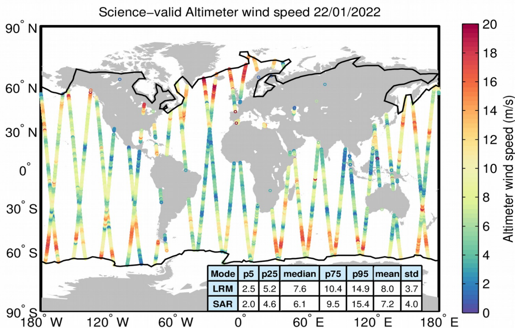
Figure 34. Geographical distribution of science-valid wind data over oceans and lakes for 22/01/2022. The statistical values shown in the table refer to the wind in m/s and are calculated separately for LRM and SAR regions. The black lines mark the outer limit of the Arctic and Antarctic polar polygons. Gray circles denote records that have been rejected based on the editing criteria described in Table 5.
