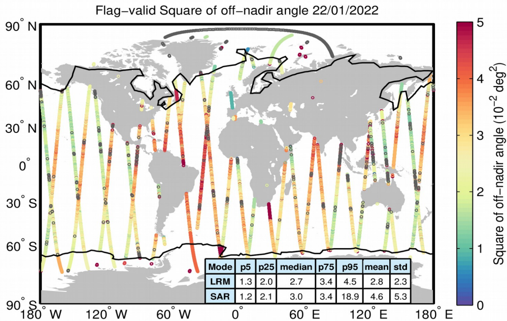
Figure 37. Geographical distribution of flag-valid mispointing data over oceans and lakes for 22/01/2022. The statistical values shown in the table refer to the mispointing in 10^{-2} \text{ deg}^2 and are calculated separately for LRM and SAR regions. Measurements taken over polar polygons have been excluded from the computation of the statistical values. The black lines mark the outer limit of the Arctic and Antarctic polar polygons. Gray circles denote negative values.
