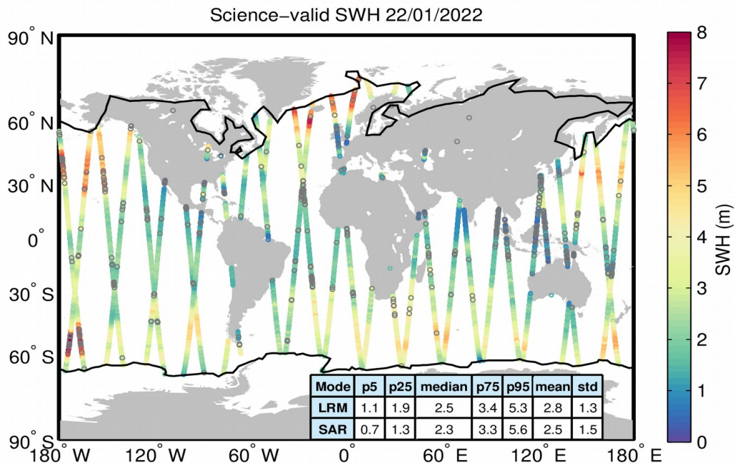
Figure 19. Geographical distribution of science-valid SWH data over oceans and lakes for 22/01/2022. The statistical values shown in the table refer to the SWH in m and are calculated separately for LRM and SAR regions. The black lines mark the outer limit of the Arctic and Antarctic polar polygons. Gray circles denote records that have been rejected based on the editing criteria described in Table 3.
