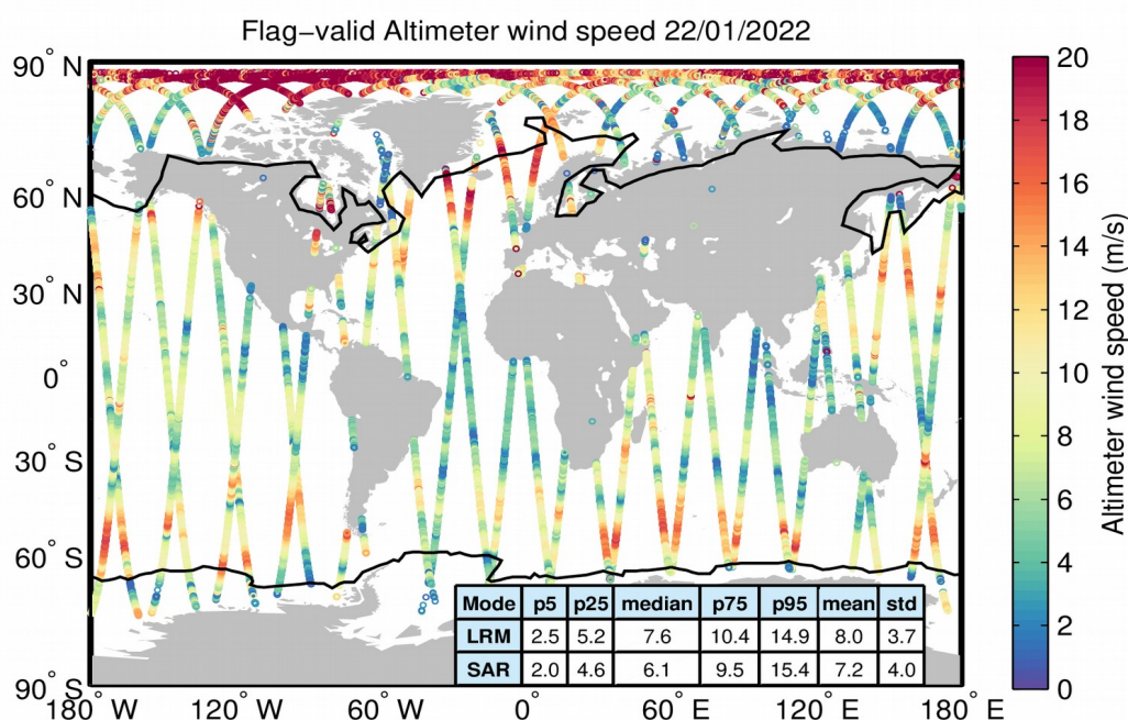
Figure 31. Geographical distribution of flag-valid wind data over oceans and lakes for 22/01/2022. The statistical values shown in the table refer to the wind in m/s and are calculated separately for LRM and SAR regions. Measurements taken over polar polygons have been excluded from the computation of the statistical values. The black lines mark the outer limit of the Arctic and Antarctic polar polygons.
