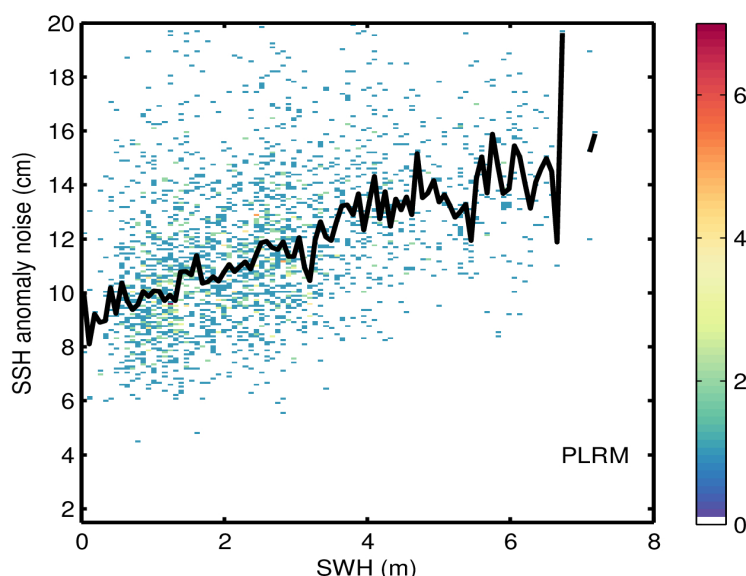
Figure 9. 2D histogram showing flag-valid SSH anomaly noise as a function of SWH for LRM (top), SAR (middle), and PLRM (bottom) for 22/01/2022. The black line denotes the median SSH anomaly noise as a function of SWH.
